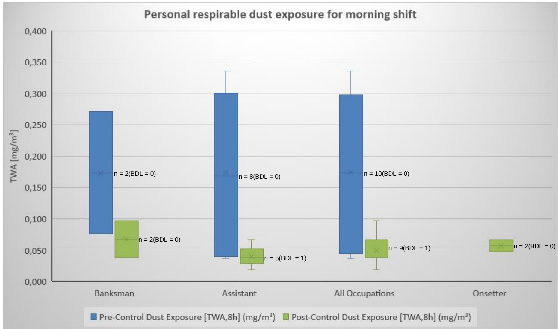
Figure 8: A “box and whisker” plot to summarise the personal respirable dust exposure for morning shifts
