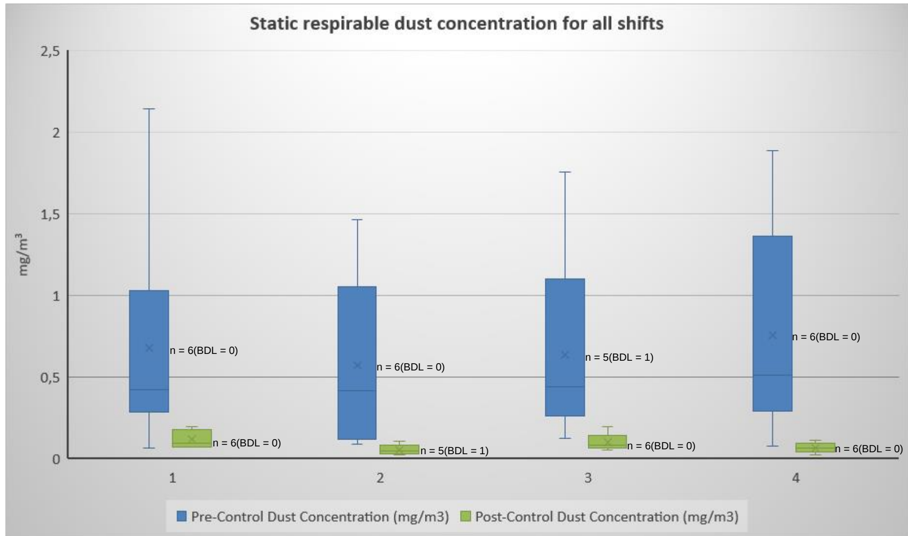
Figure 14: A “box and whisker” plot to summarise the static respirable dust concentration for all shifts
