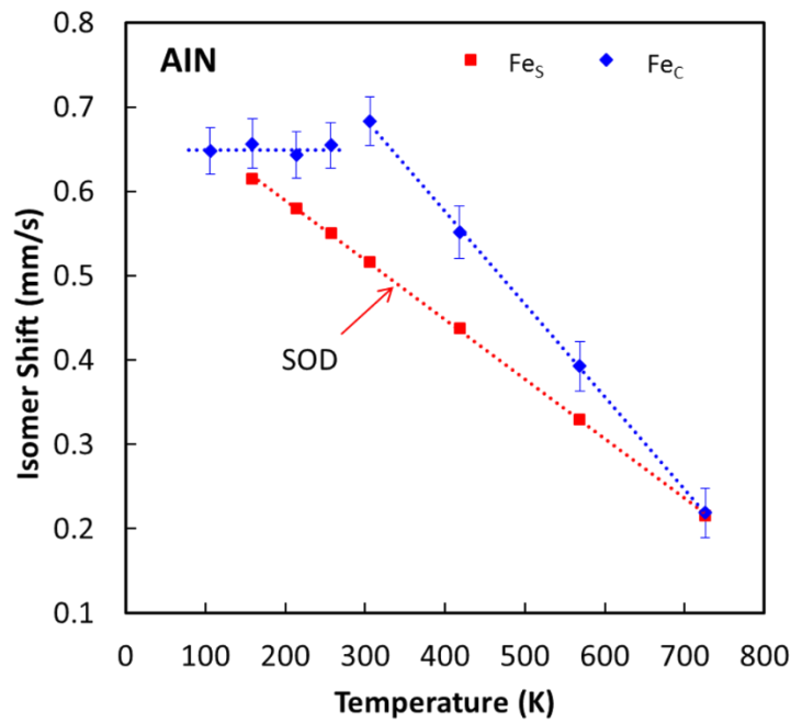
Figure 4.13: Temperature dependence of the isomer shifts for \text{Fe}_\text{C} and \text{Fe}_\text{S} observed in the Mössbauer spectra for Fe implanted AlN. (The dotted line is to guide the eye)
