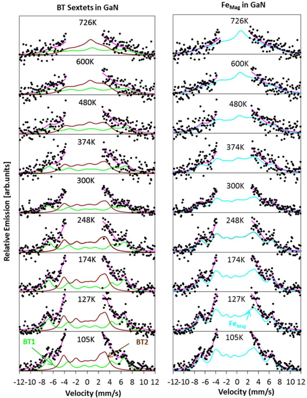
Figure 4.7: Two Blume-Tjon sextets and their sum, \text{Fe}_{\text{Mag}} , (in blue) shown in the central region of the emission Mössbauer spectra of ^{57}\text{Mn}^* implanted GaN at temperatures indicated.
