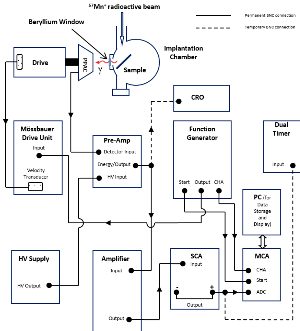
Figure 3.13: Schematic diagram of the experimental set-up and electronics [177] at ISOLDE.
