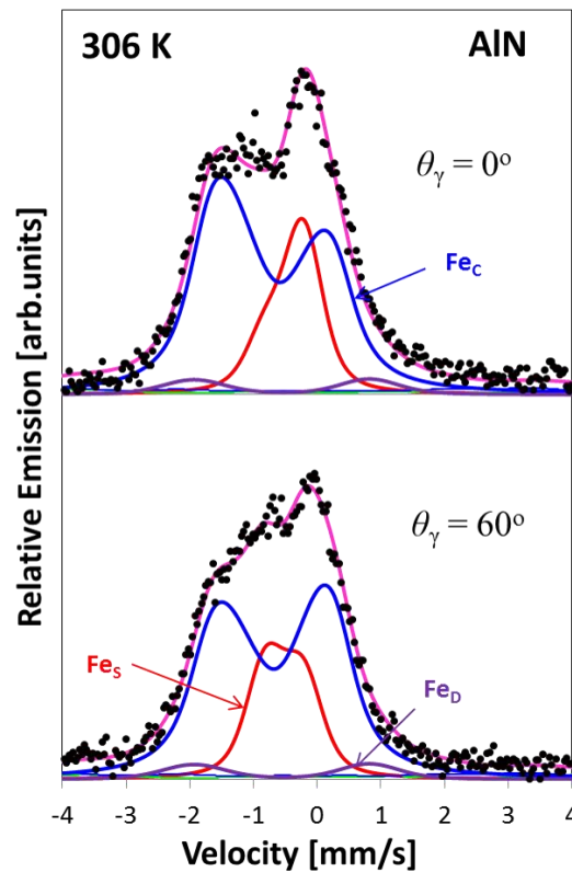
Figure 4.11: ^{57}\text{Fe} emission Mössbauer spectra obtained at 306 K after implantation of ^{57}\text{Mn}^* into AlN at emission angles indicated.
