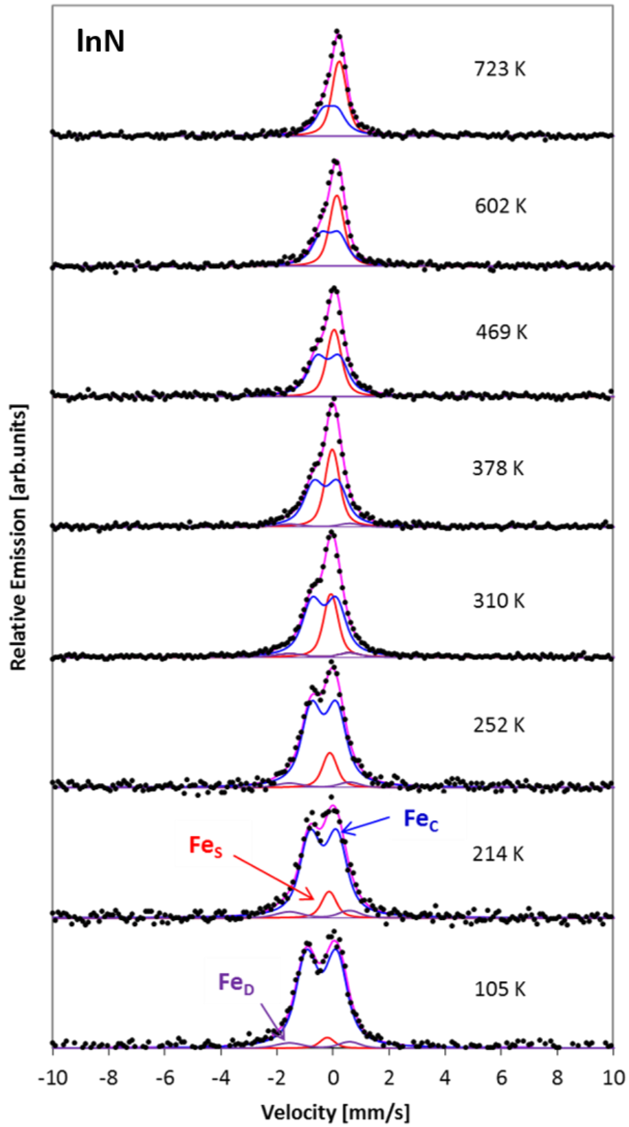
Figure 4.20: ^{57}\text{Fe} emission Mössbauer spectra obtained after implantation of ^{57}\text{Mn}^* into InN at the temperatures indicated and \theta_i = 60^\circ .
