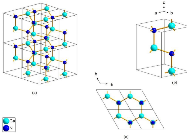
Figure 1.1: Wurtzite crystal structure of GaN: (a) 2×2 unit cells, (b) unit cell and (c) view along the c -axis.
