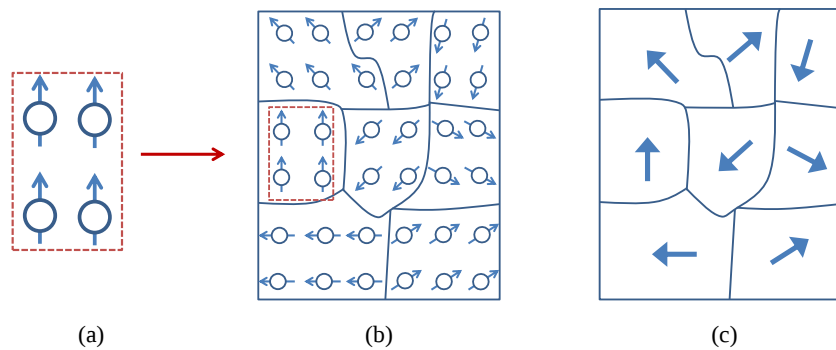
Figure A.4: (a) Neighbouring moments in a ferromagnetic material, (b) Parallel alignment of neighbouring spins in different magnetic domains, (c) Overall spontaneous magnetisation in magnetic domains.
