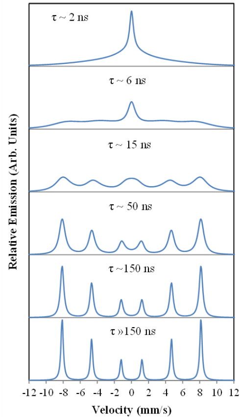
Figure 4.3: ^{57}\text{Fe} Mössbauer spectra simulated with Blume-Tjon model using hyperfine field of \pm 50\text{ T} at relaxation time indicated.
