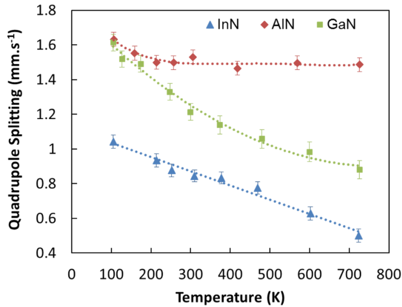
Figure 4.22: Temperature dependence of the quadrupole splitting for \text{Fe}_\text{C} observed in the Mössbauer spectra for ^{57}\text{Mn}^* implanted III-nitrides. (The dotted line is to guide the eye).
