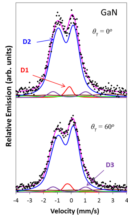
Figure 4.2: Room temperature ^{57}\text{Fe} emission Mössbauer spectra obtained after implantation of ^{57}\text{Mn}^* into GaN at emission angles of 0^\circ and 60^\circ relative to the sample c -axis.
