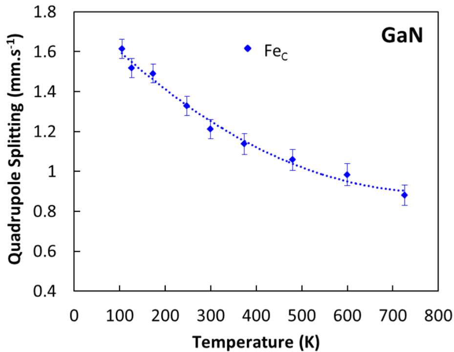
Figure 4.6: Temperature dependence of the quadrupole splitting for \text{Fe}_\text{C} observed in the Mössbauer spectra for Fe implanted GaN. (The dotted line is to guide the eye)
