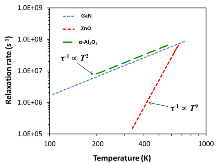
Figure 4.9: A plot of relaxation rates as a function of temperature obtained for GaN compared with data from previous studies of oxides [153].
