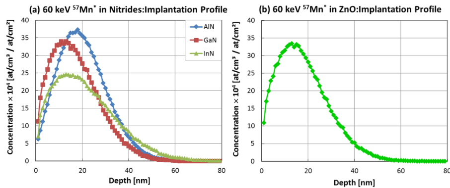
Figure 3.5: Implantation profile for ^{57}\text{Mn}^* in (a) nitrides and (b) ZnO at \theta_i = 60^\circ .
