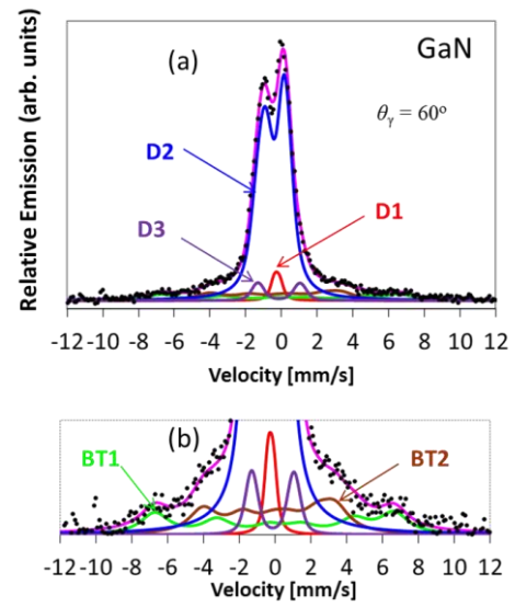
Figure 4.1: (a) Emission Mössbauer spectrum of GaN obtained at 300 K and at an emission angle of 60^\circ and (b) zoomed-in view of the two BT sextets used to analyse the magnetic structure in (a).
