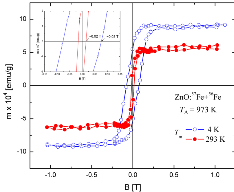
Figure 4.34: Magnetisation curves of \text{ZnO}:\text{}^{57}\text{Fe}+\text{}^{56}\text{Fe} measured at 4 K and 293 K after annealing at 973 K.
