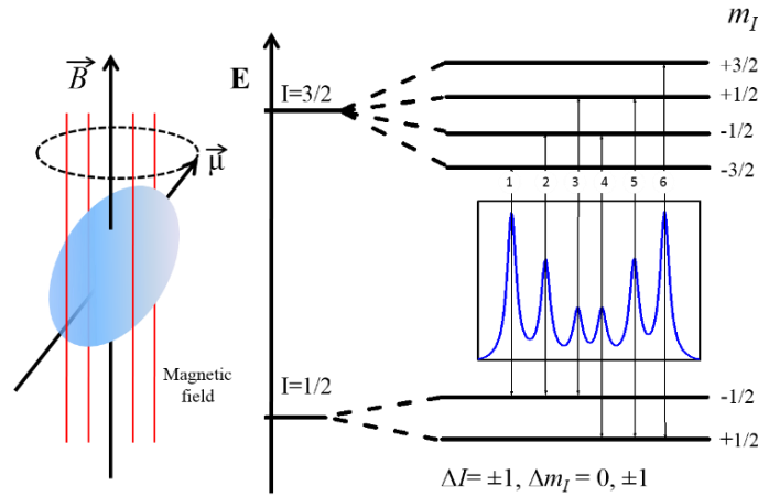
Figure 2.9: Magnetic dipole interaction resulting in the nuclear Zeeman splitting of the energy levels and the Mössbauer spectrum showing a sextet [177] .
