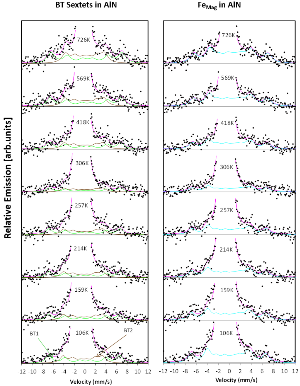
Figure 4.15: Two Blume-Tjon sextets (and their sum) showing the magnetic structure fitted for Fe implanted AlN spectra at the temperatures indicated.
