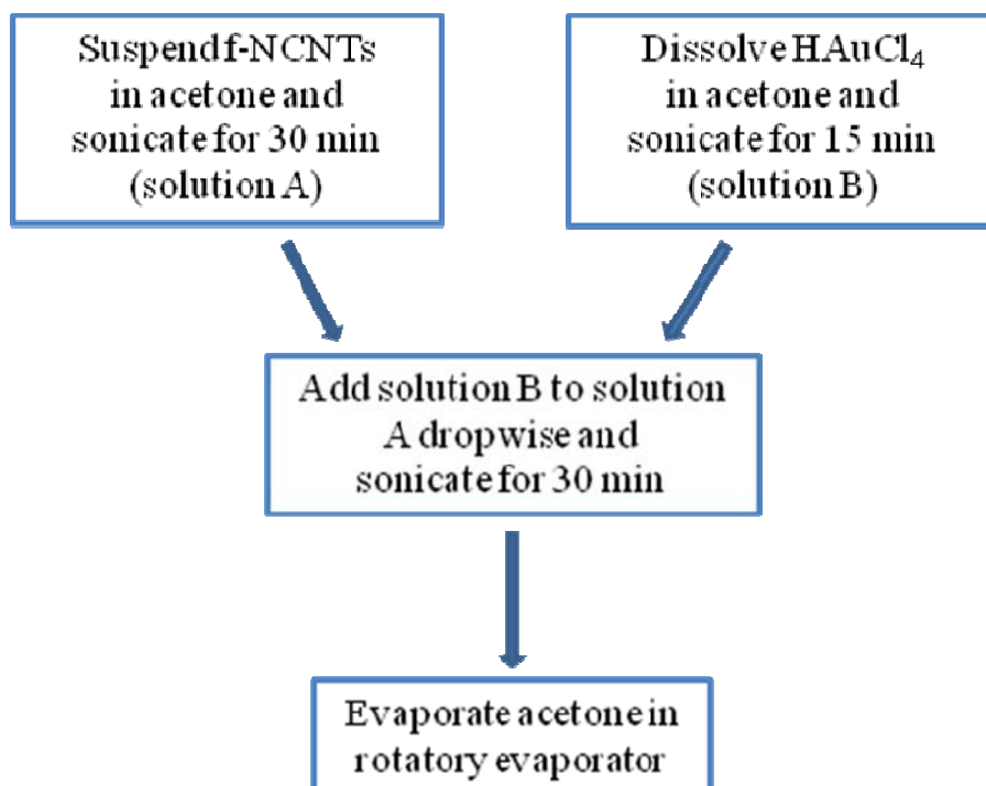
Fig. 10.1: Method for the synthesis of Au/N-CNT hybrid nanostructures.
