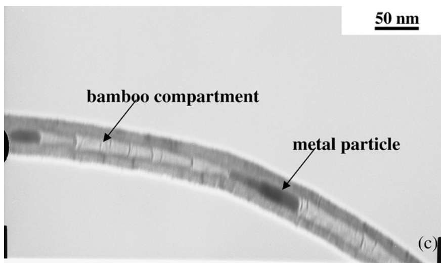
Fig. 2.8. TEM pictures of CNT grown from ferrocene/aniline mixtures. Note the bamboo compartments and metal catalyst particle trapped in the tube [18].
