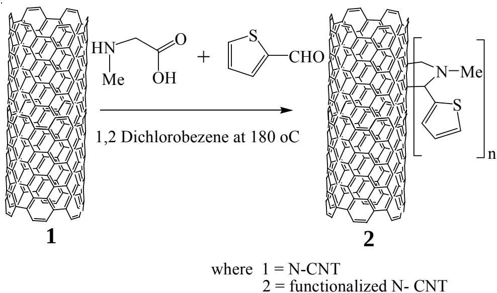
Scheme 10.1. Functionalization of N-CNTs with Prato reaction [23].
