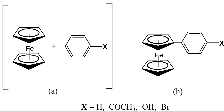
Fig. 8.1. The precursors used for synthesis of SCNMs in toluene: (a) ferrocene (FcH) and para -substituted benzenes; (b) arylferrocenes (FcPhX).
