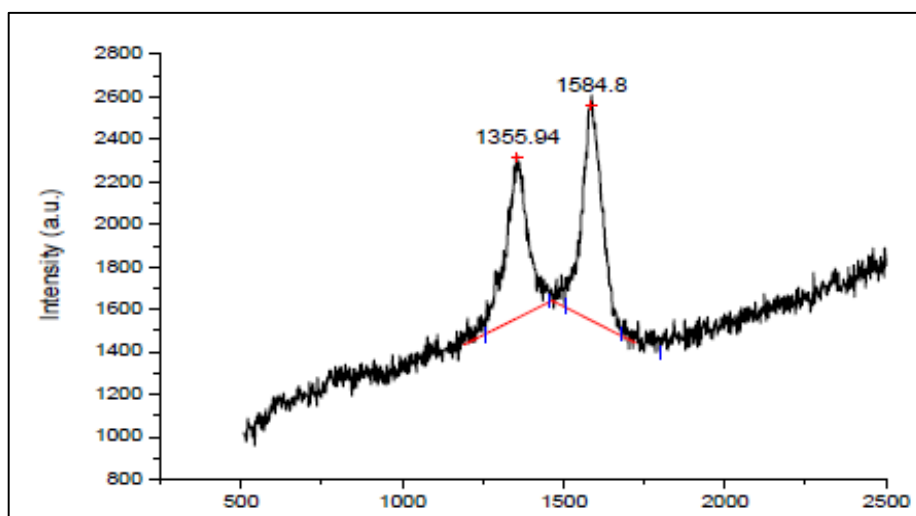
Fig. A7.9. Raman spectrum of CNTs obtained from the pyrolysis of toluene/FcH in the presence of 8% diethylamine.
