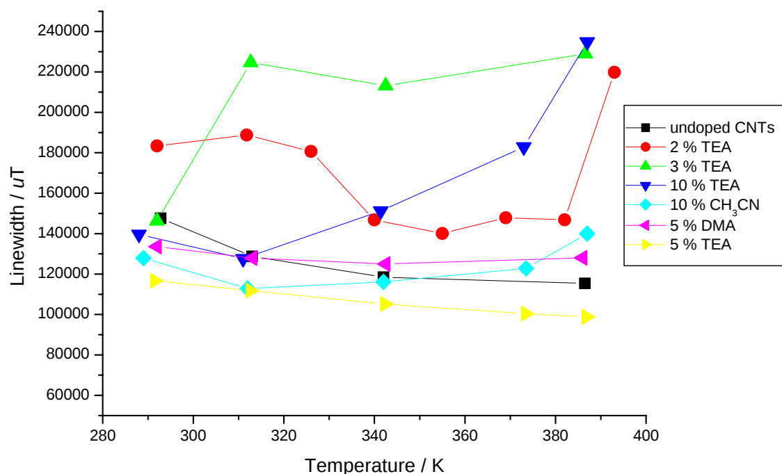
Fig. 9.5. Line width graphs for N-CNTs and MWCNTs at different temperatures. TEA = triethylamine, CH 3 CN = acetonitrile, DMA = dimethylamine.
