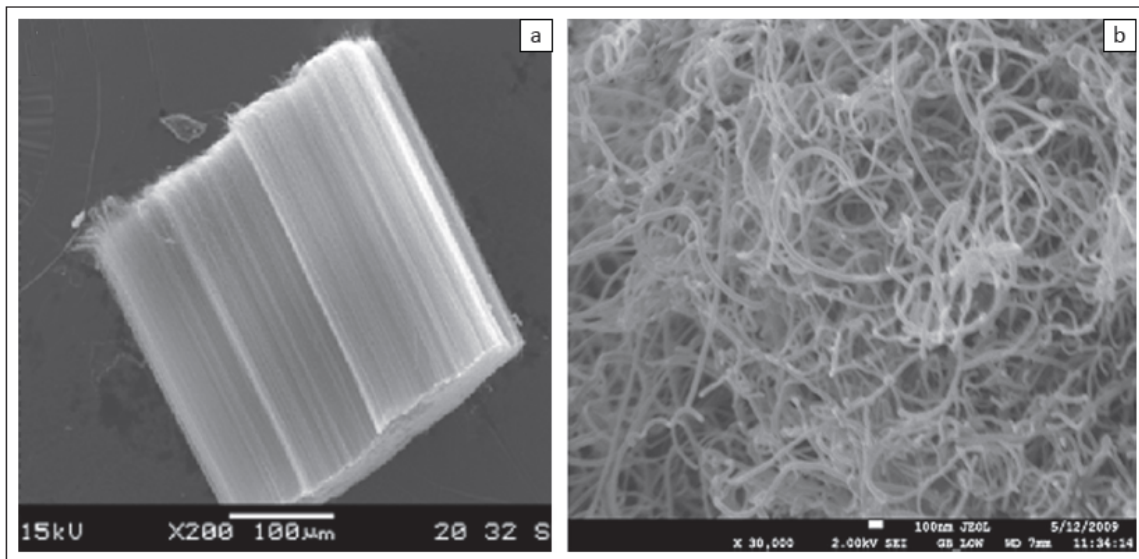
Fig. 2.5. SEM micrographs showing (a) aligned CNFs and (b) ‘cooked spaghetti type’ CNFs.
