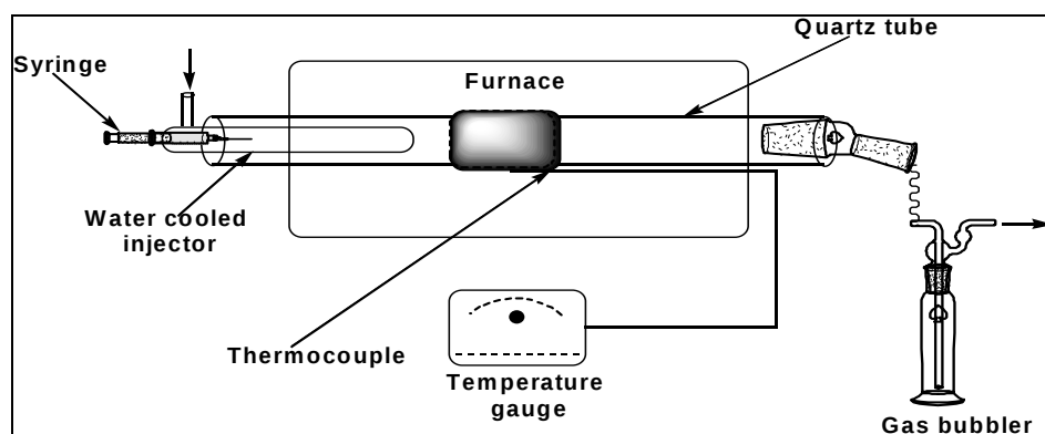
Fig. A5.1. A typical horizontal furnace system used for the synthesis of CNTs.
