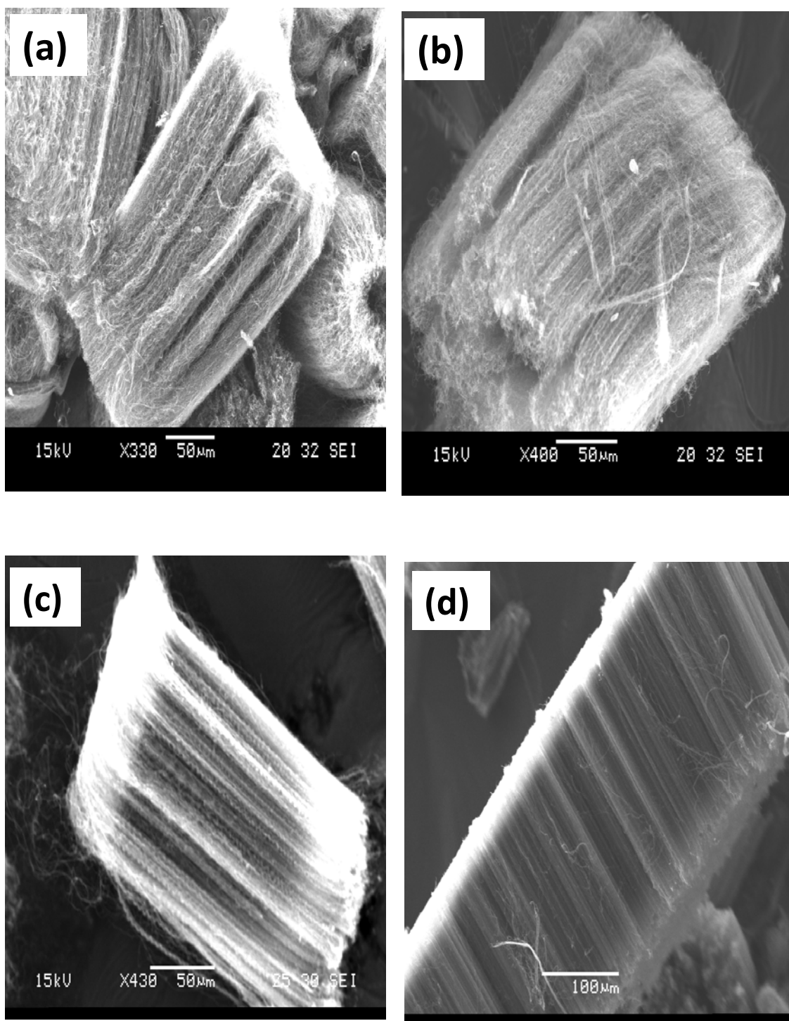
Fig. A7.4. SEM images of CNTs obtained from the pyrolysis of toluene and ferrocene in the presence of (a) 1%; and (b) 8% quinoline; and (c) 1%; and (d) 8% N,N -dimethylacetamide.
