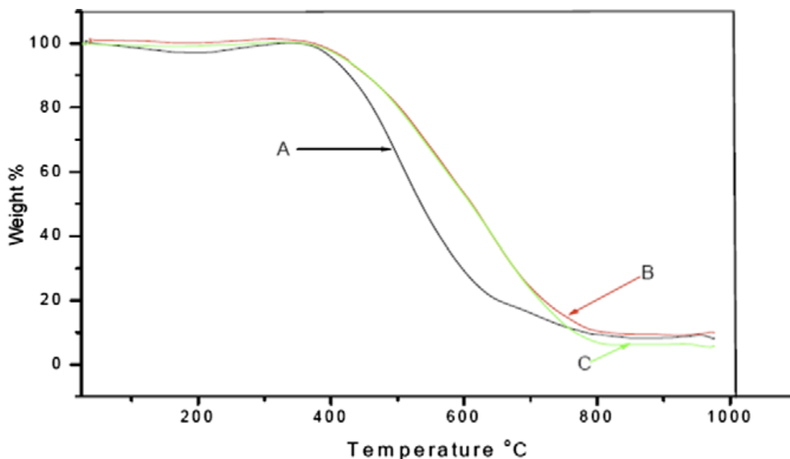
Fig. 6.7. TGA curves of CNTs grown from (A) FcH/1-methylimidazole (10:90); (B) FcH/2-methylimidazole (10:90) and (C) FcH/4-methylimidazole (10:90).
