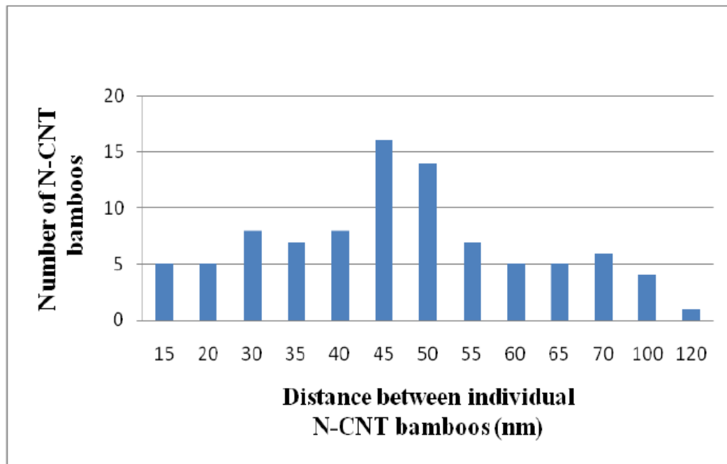
Fig. 6.6. Distance between individual bamboo compartments obtained from the pyrolysis of ferrocenylimidazole.
