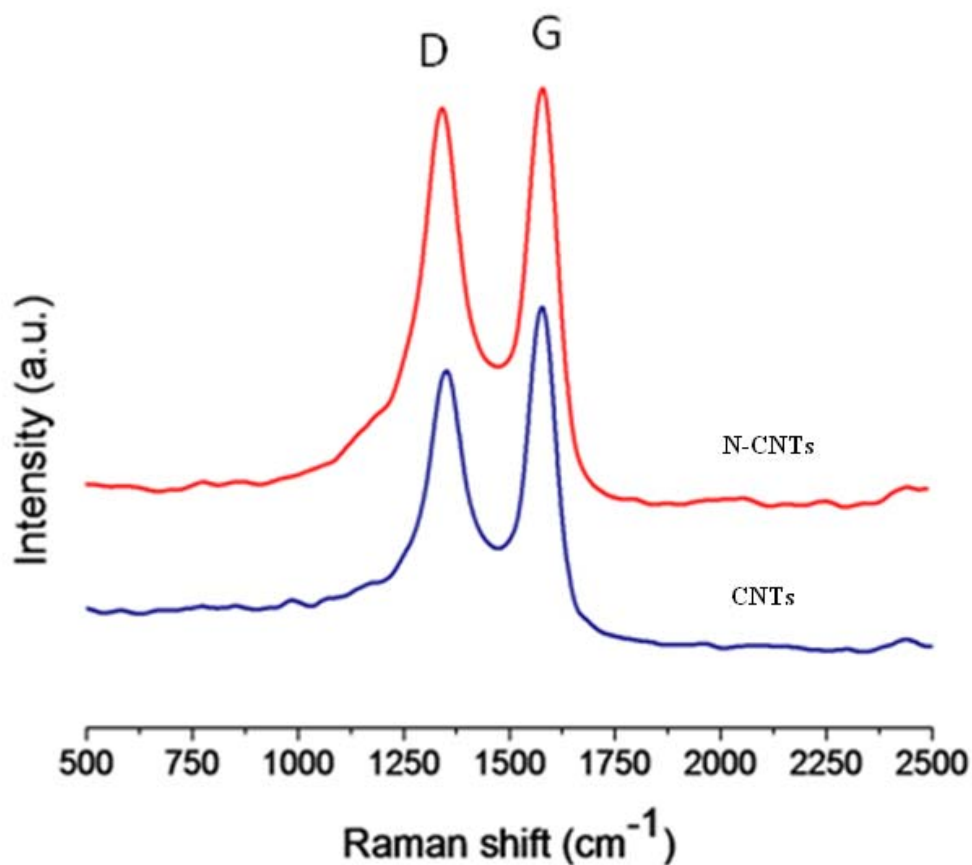
Fig. 9.2. Raman spectra of MWCNTs and N-CNTs showing the D- and G- bands (laser excitation 514 nm).
