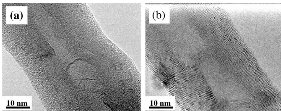
Fig. 6.3. HRTEM images of N-CNTs grown from the pyrolysis of (a) FcH/4-methylimidazole (50:50) and (b) ferrocenylmethylimidazole.
