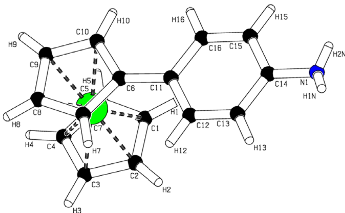
Fig. 5.1. Crystal structure for 4-ferrocenyamine.
