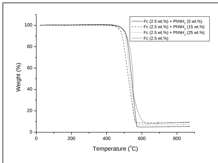
Fig. A5.3. TGA curves of CNTs grown from FcH (2.5 wt.%) / PhNH 2 (0, 5, 15 and 25 wt.% aniline).
