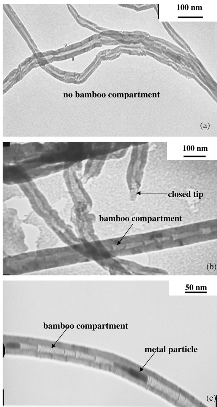
Fig. 5.4. TEM pictures of CNTs grown from (a) FcH (2.5 wt.%) (b) FePhNH 2 (2.5%) and (c) FcH (2.5 wt.%) / PhNH 2 (5 wt.%).
