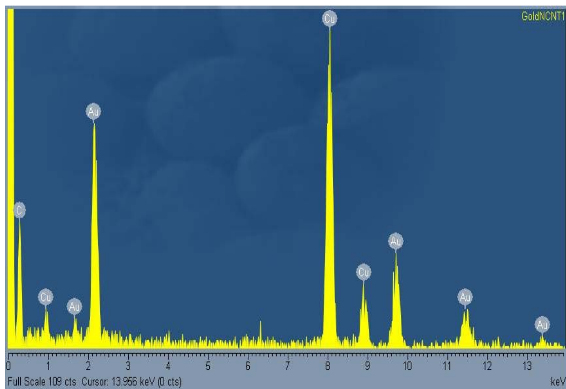
Fig. 10.4. EDX spectrum of Au/N-CNT nanostructures.
