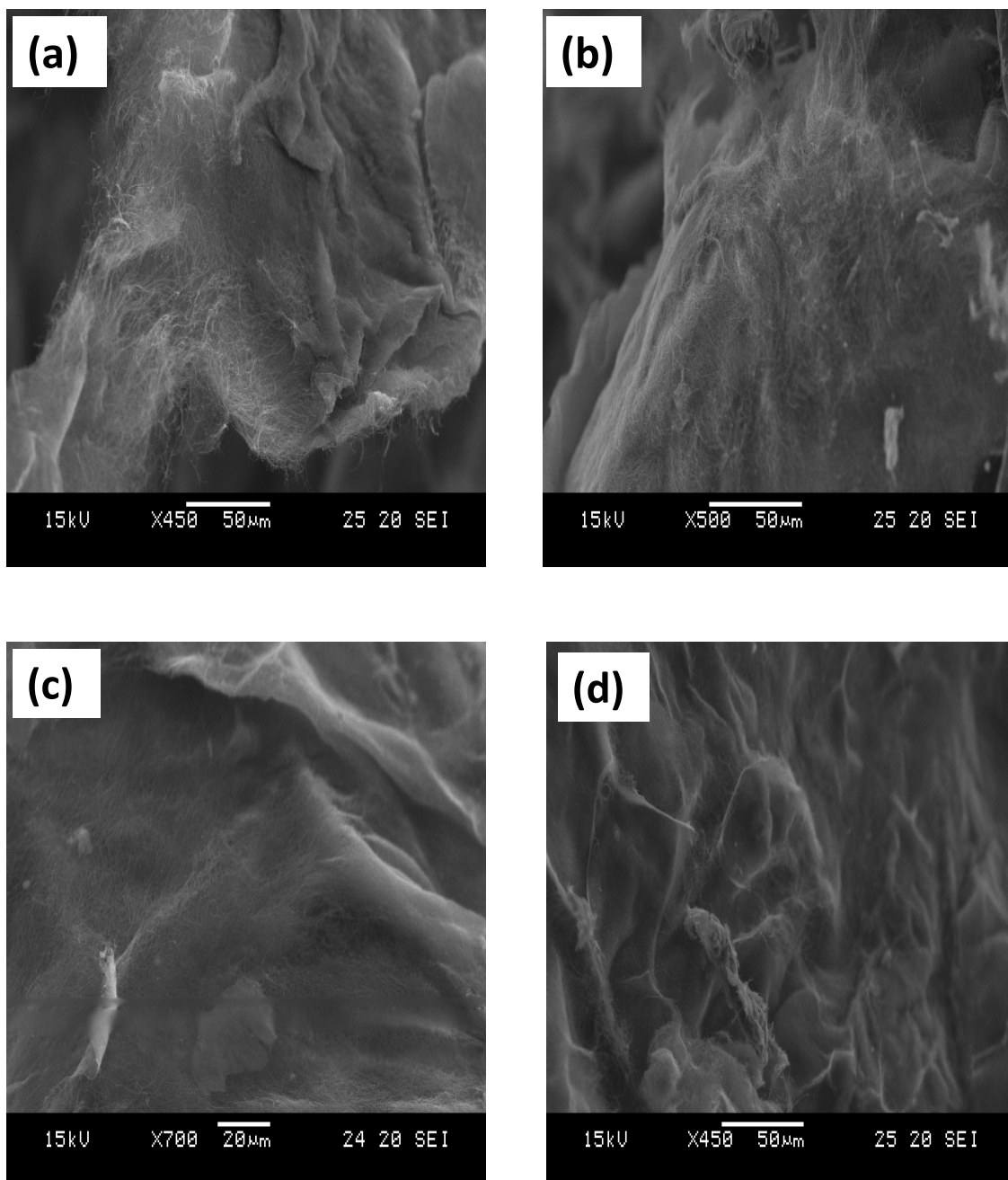
Fig. 7.8. SEM images of acid treated CNTs obtained from the pyrolysis of toluene and ferrocene in the presence of (a) 1%; and (b) 8% diethylamine; and (c) 1%; and (d) 8% hexamethylenediamine.
