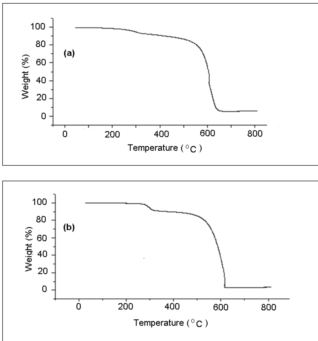
Fig. 7.9. TGA spectra of acid treated CNTs obtained from the pyrolysis of toluene and ferrocene in the presence of (a) 1%; and (b) 8% hexamethylenediamine.
