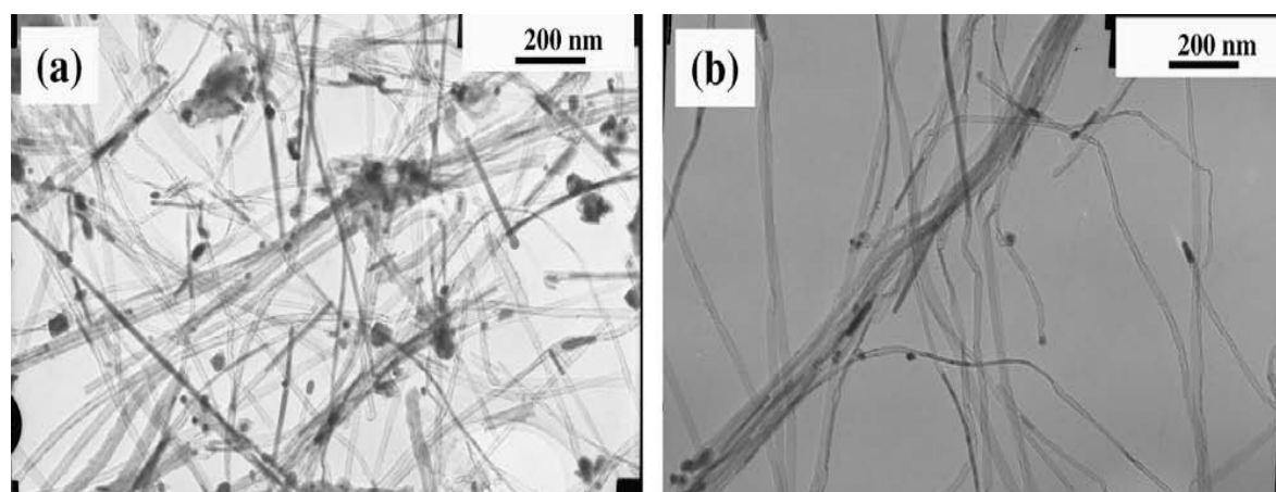
Fig. 8.3. TEM pictures of CNTs produced from the pyrolysis of FcPhBr (2.5 wt.%) at 900 °C.
