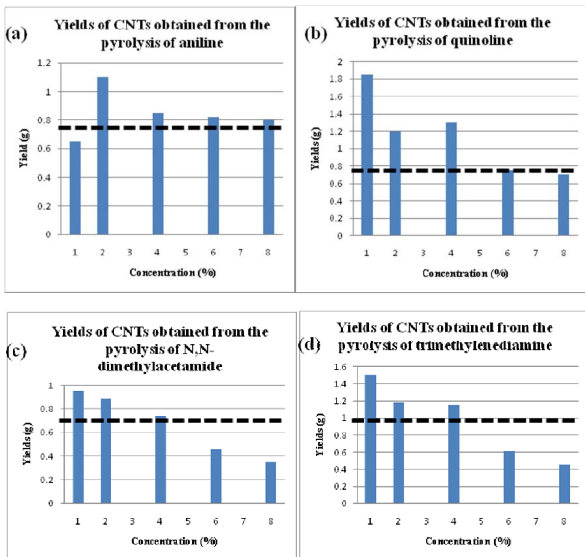
Fig. A7.2. Yield of CNTs obtained from the pyrolysis of toluene and ferrocene in the presence of (a) aniline; (b) quinoline; (c) N,N -dimethylacetamide; and (d) trimethylenediamine at different concentrations. Horizontal dotted lines indicate yields for ferrocene/toluene CNTs.
