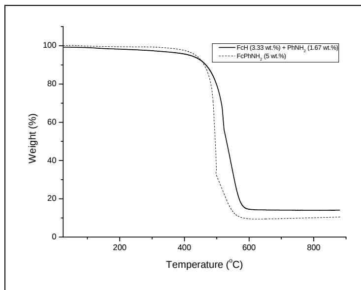
Fig. A5.2. TGA curves of CNTs grown from FcH (3.33 wt.%) /PhNH 2 (1.67 wt.%) and FcPhNH 2 (5 wt.%).
