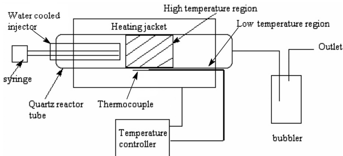
Fig. 4.1. Floating catalyst CVD reactor for the synthesis of SCNMs [8].
