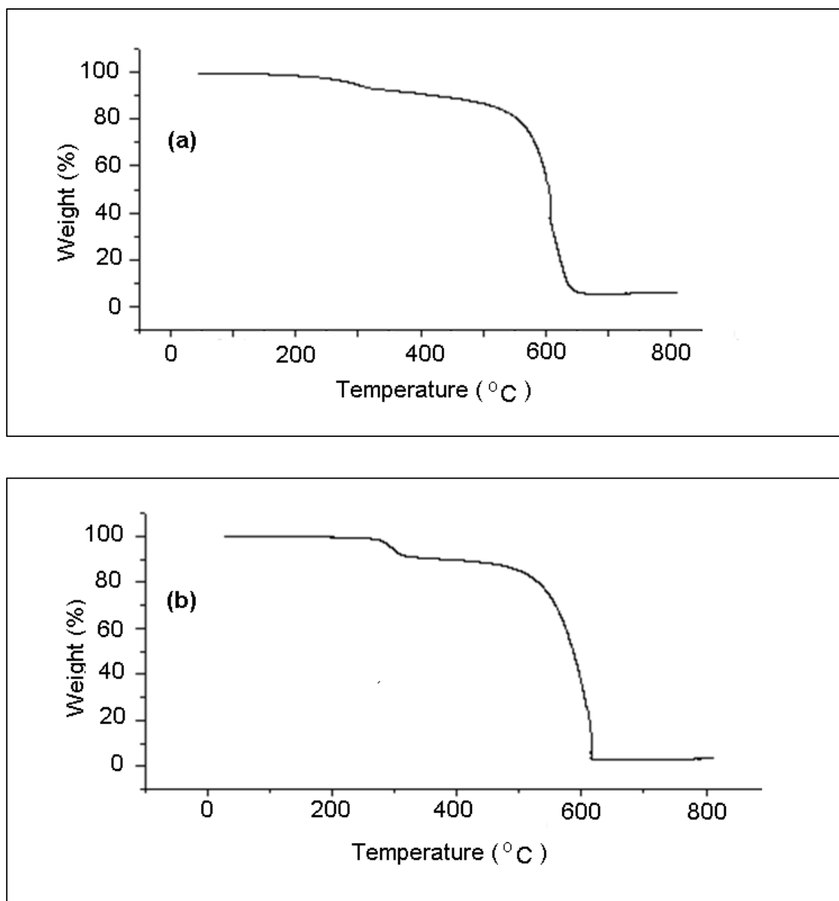
Fig. A7.8. TGA spectra of acid treated CNTs obtained from the pyrolysis of toluene and FcH in the presence of (a) 1%; and (b) 8% hexamethylenediamine.
