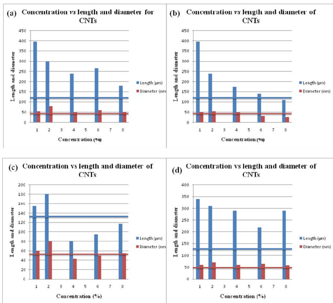
Fig. A7.6. Graph of concentration versus diameter and length of CNTs obtained from the pyrolysis of toluene and ferrocene in the presence of (a) diethylamine; (b) pyridine; (c) 1-methylpiperazine; and (d) formamide. Horizontal bar and dotted line indicate the length and diameter of the CNTs, respectively.
