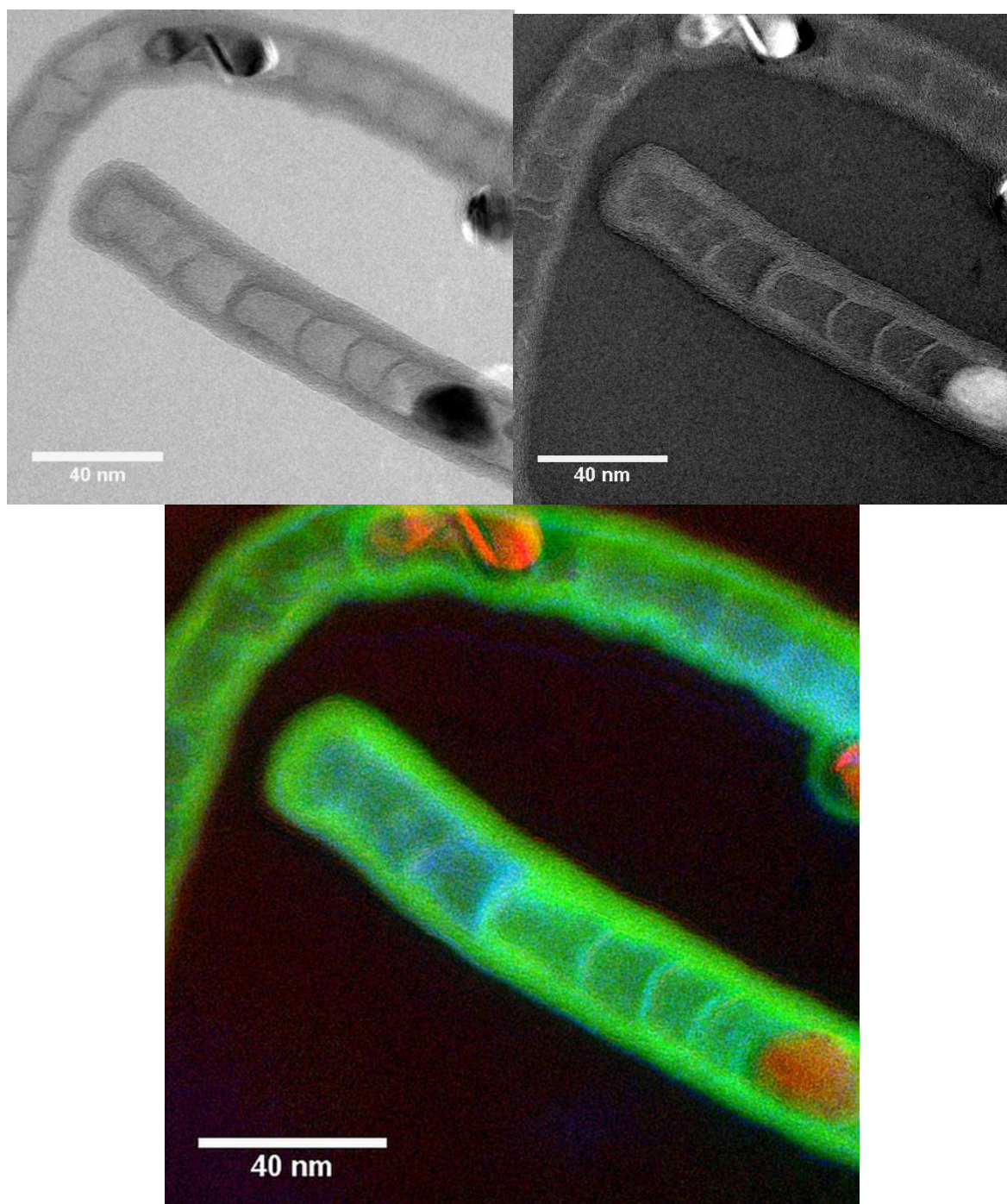
Fig. 11.4. EFTEM images of N-CNTs grown from 5 wt.% N-source; (a) bright field, (b) zero loss and (b) false colour EFTEM image with carbon (green), nitrogen (blue) and iron (red).
