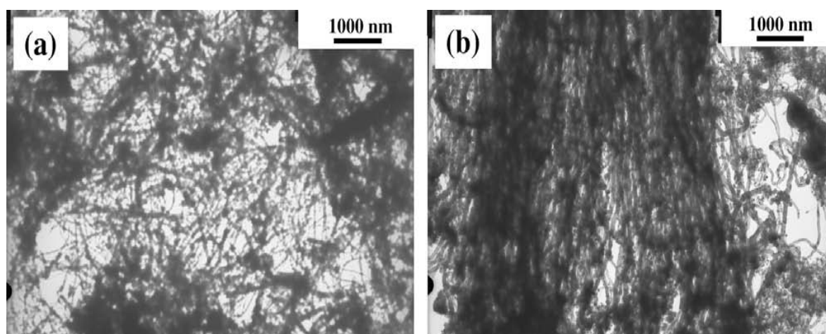
Fig. 8.2. CNTs formed from pyrolysis of (a) 2.5 wt.% FcH and (b) 2.5 wt.% FcPhH in toluene with a flow rate of 0.8 ml/min and at temperature of 800 °C.
