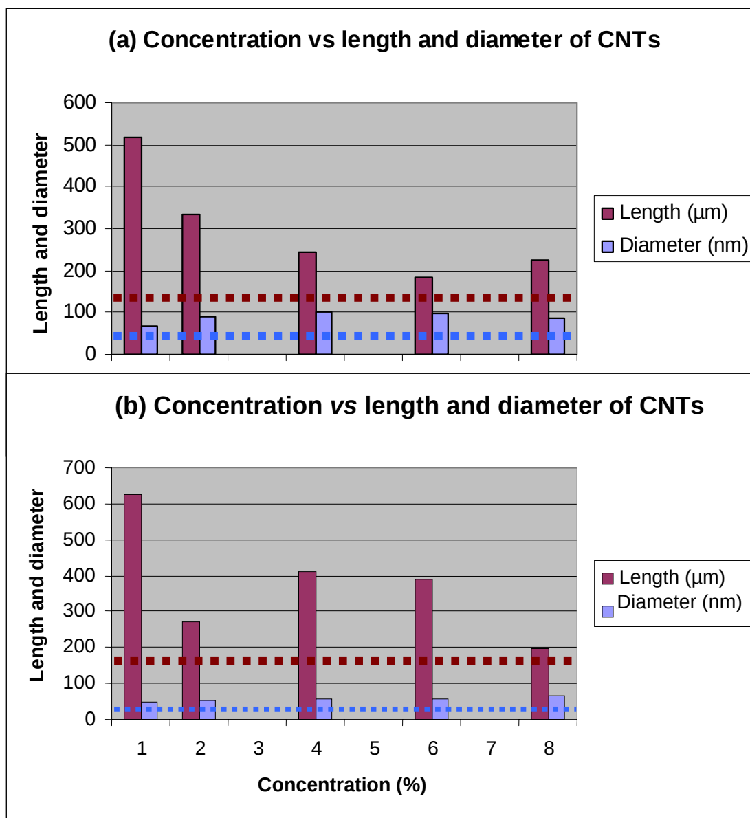
Fig. 4.7. Graph of concentration versus length and diameters of CNTs grown from (a) FcH/benzylamine; and (b) FcH/hexamethylenediamine mixtures. Horizontal dotted line indicates lengths and diameters of CNTs obtained from FcH/toluene [26].
