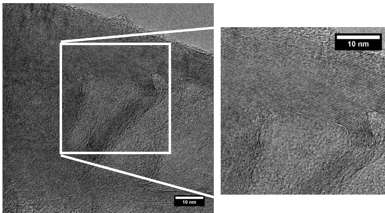
Fig. 11.3. Image showing well separated graphitic sheets in 5 wt.% N-CNTs.
