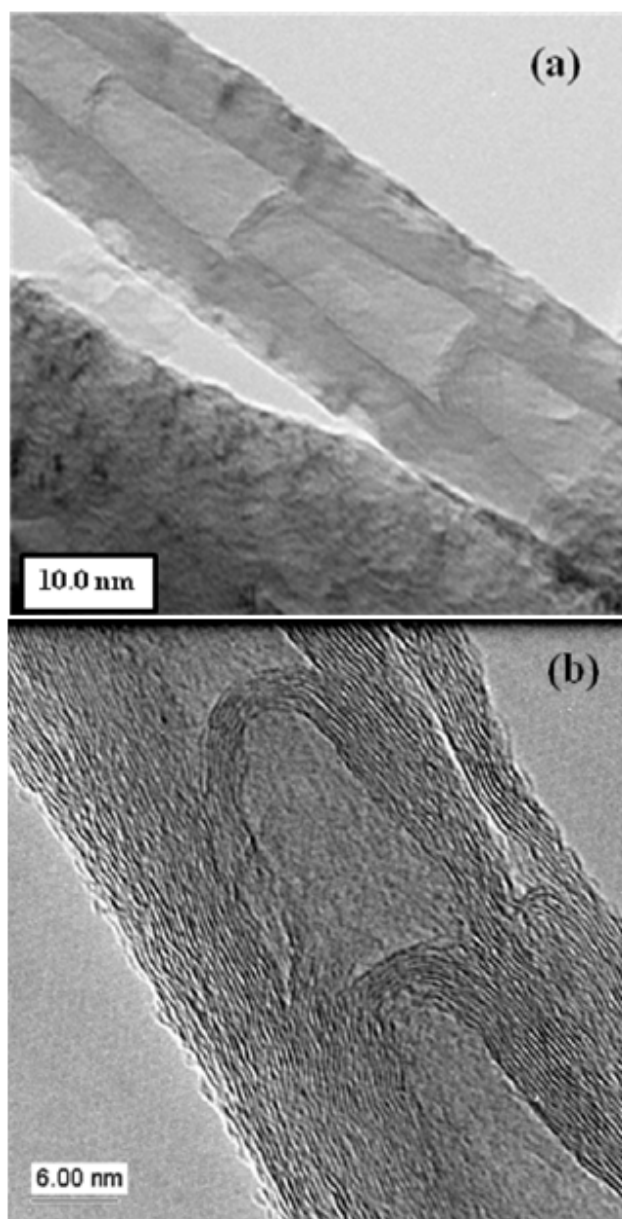
Fig. 4.3. TEM images at different magnifications (a, b) of CNTs obtained from the pyrolysis of toluene and ferrocene in the presence of 8% diethylamine [26].
