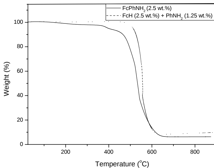
Fig. 5.6. TGA curves of CNTs grown from FcH (2.5 wt.%)/PhNH 2 (1.25 wt.%) and FcPhNH 2 (2.5 wt.%).
