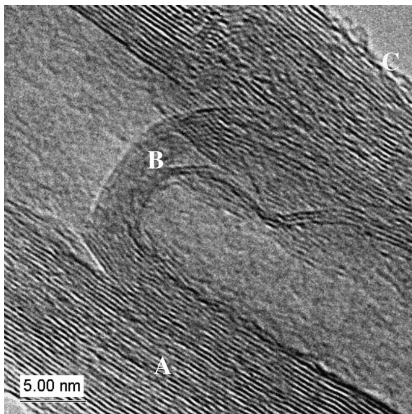
Fig. 5.5. High magnification TEM image of a N-CNT. The image clearly reveals the multi-walled nature of the tube (A), the compartment wall (B) and the rough CNT surface (C).
