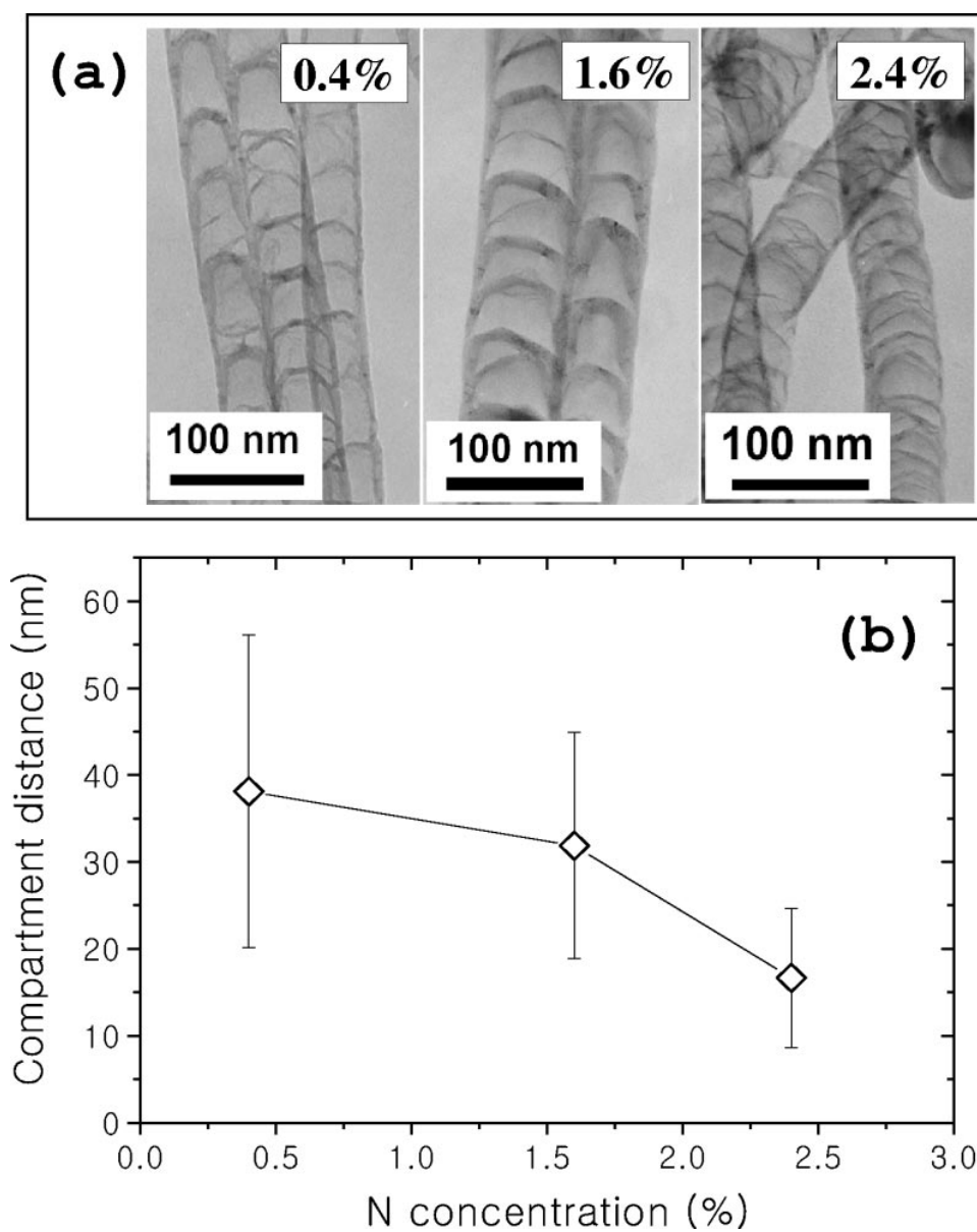
Fig. 4.4. The compartment structures for various nitrogen concentrations. (a) The TEM images of compartment layers of N doped tubes. (b) The compartment distance as a function of the nitrogen concentration. The \text{NH}_3 flow ratios of 30, 90, and 150 mL/min gave N-CNTs with N doping levels of 0.4%, 1.6%, and 2.4%. [34].
