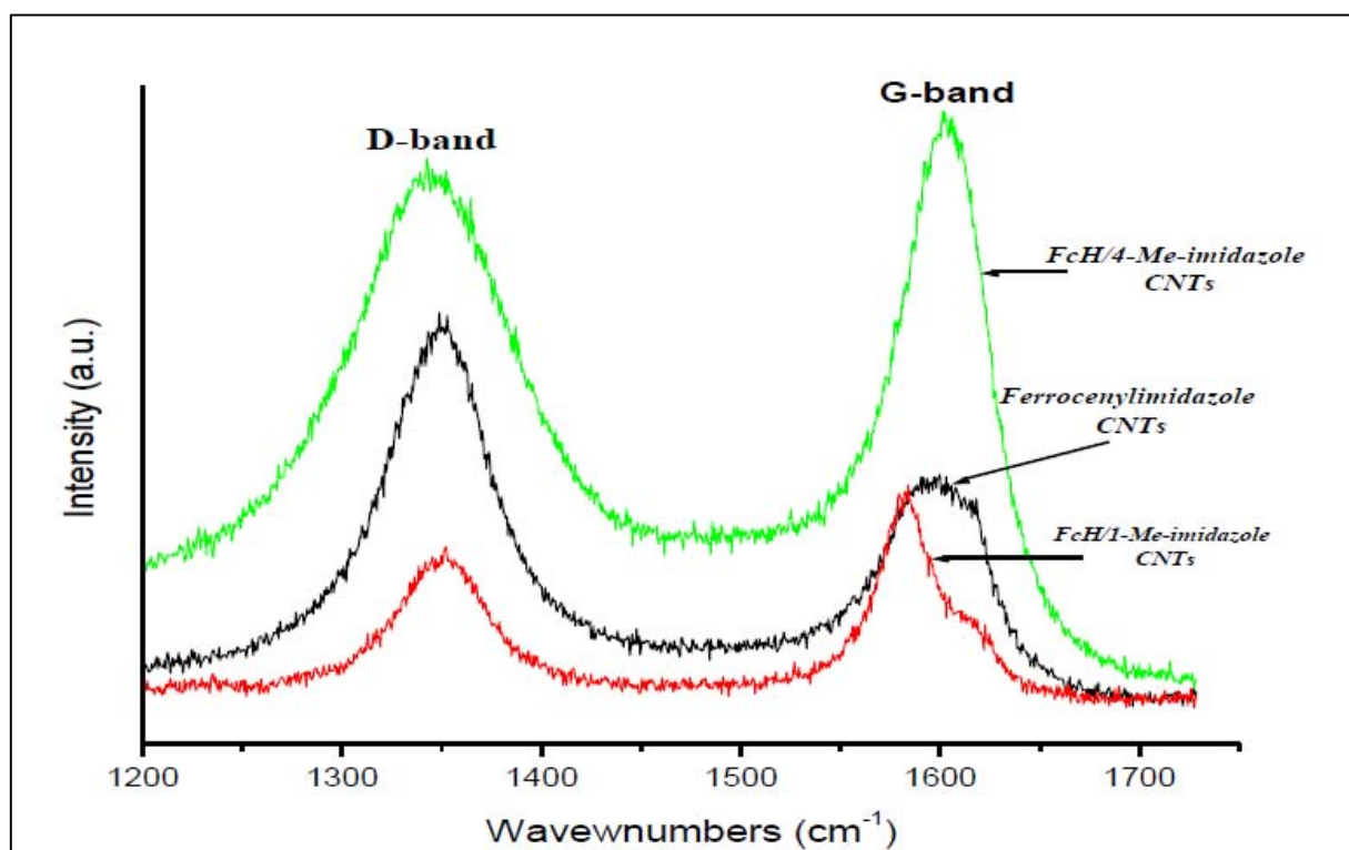
Fig. 6.8. Raman spectra of CNTs grown from ferrocenylmethylimidazole, FcH/1-methylimidazole (50:50) and FcH/4-methylimidazole (50:50).
