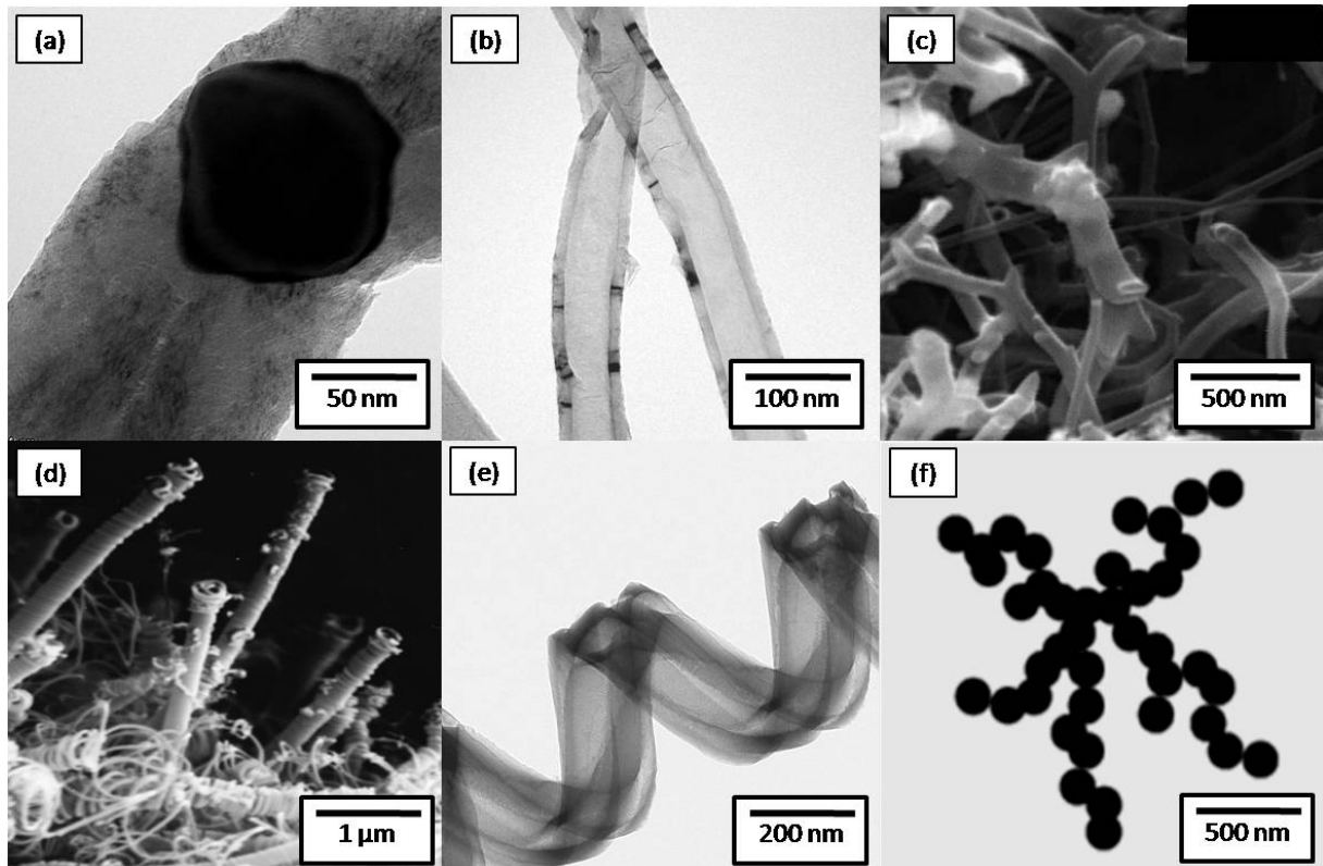
Fig. 2.3. Variety of shaped carbon materials: (a) solid fiber growing from catalyst particle, (b) tubular structure with hollow inner, (c) SEM image of branched carbon fibers, (d) SEM image of coiled carbon fibers, (e) TEM image of spring-like fiber and (f) Spherical carbon material.
