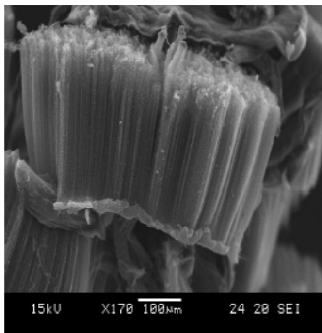
Fig. 7.7. SEM image of acid treated CNTs obtained from the pyrolysis of toluene and ferrocene.
