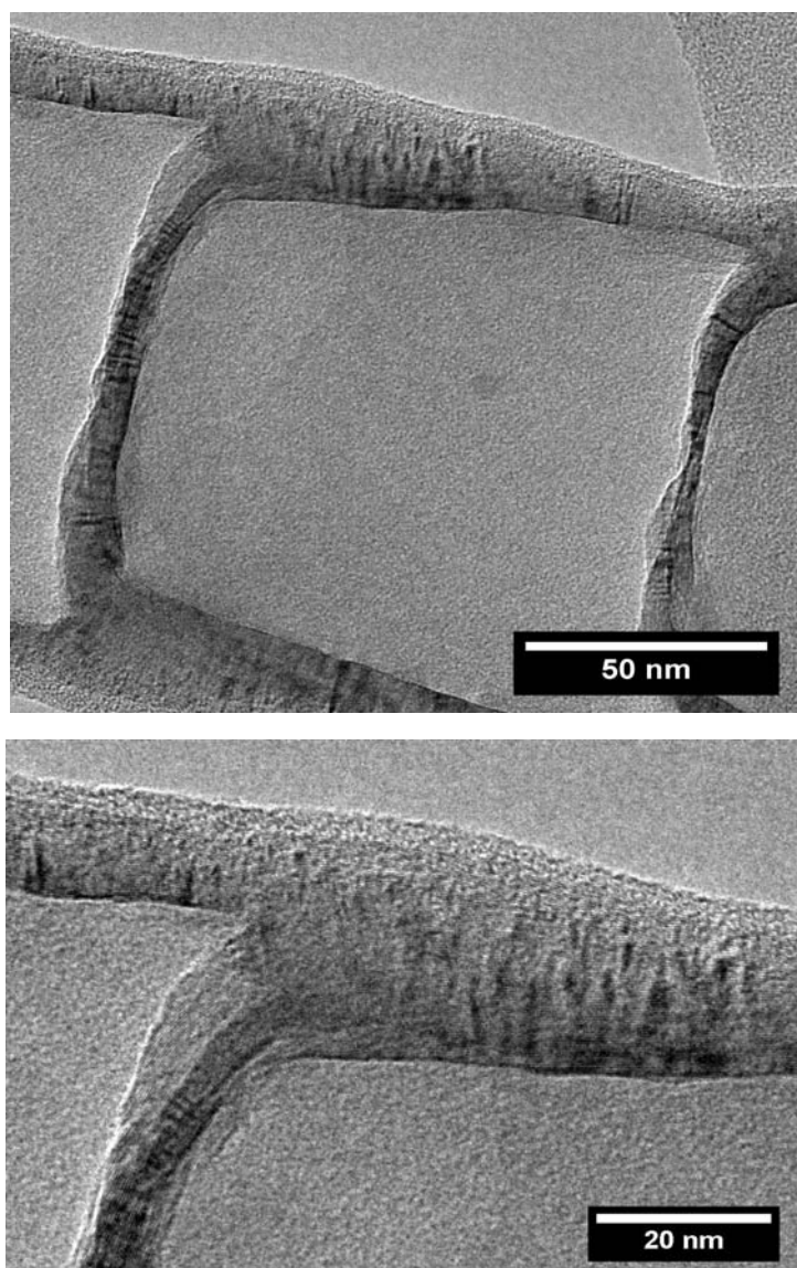
Fig. 11.2. HRTEM images for N-CNTs grown from 1 wt.% of ferrocene/diethylenetriamine mixtures. The top image shows a tube with bamboo link while the lower image is a zoomed region where lattice fringes are visible.
