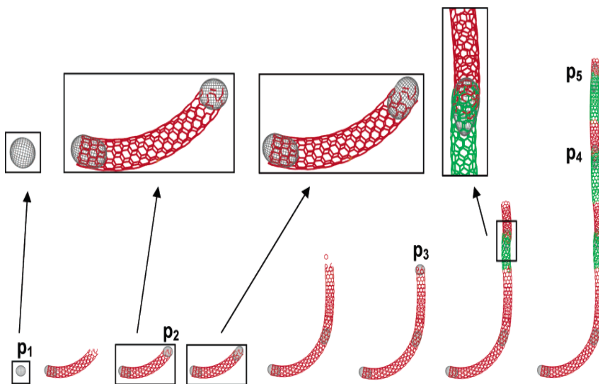
Fig. 4.6. Representation of the model of concurrent base and tip growth modes for consecutive catalyst particles [115].
