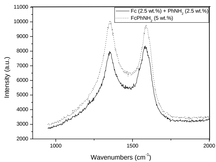
Fig. A5.4. Raman spectra of CNTs grown from FcH (2.5 wt.%) / PhNH 2 (2.5 wt.%) and FcPhNH 2 (5 wt.%).
