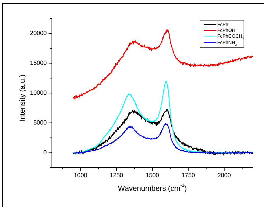
Fig. 8.5. Raman spectra of CNTs grown from different arylferrocenes (2.5 wt.%) at 900 °C.
