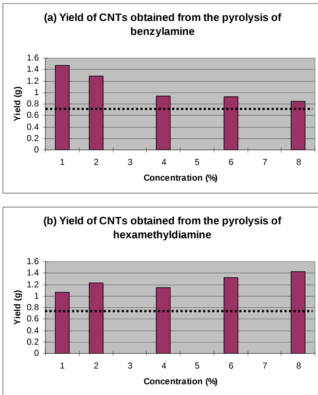
Fig. 7.1. Graphical representation of CNT yields grown from (a) benzylamine; and (b) hexamethylenediamine. Horizontal dotted line indicates yield of CNTs obtained from ferrocene/toluene.
