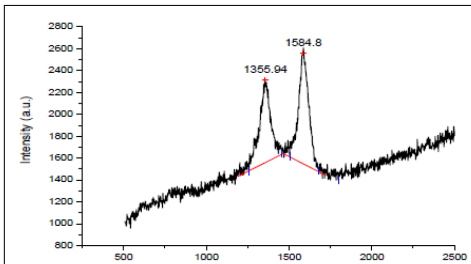
Fig. 7.6. Raman spectrum of CNTs obtained from the pyrolysis of toluene and ferrocene in the presence of 8% diethylamine.
