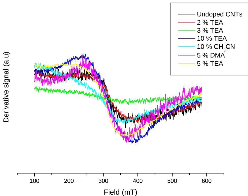
Fig. 9.3. ESR spectra of undoped and N-CNTs at 293 K. TEA = triethylamine, \text{CH}_3\text{CN} = acetonitrile, DMA = dimethylamine.
