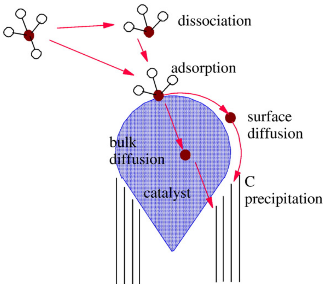
Fig. 4.5. Schematic of reactions and processes on a catalytic nano-particle during nanotube growth (tip growth illustrated) [117].
