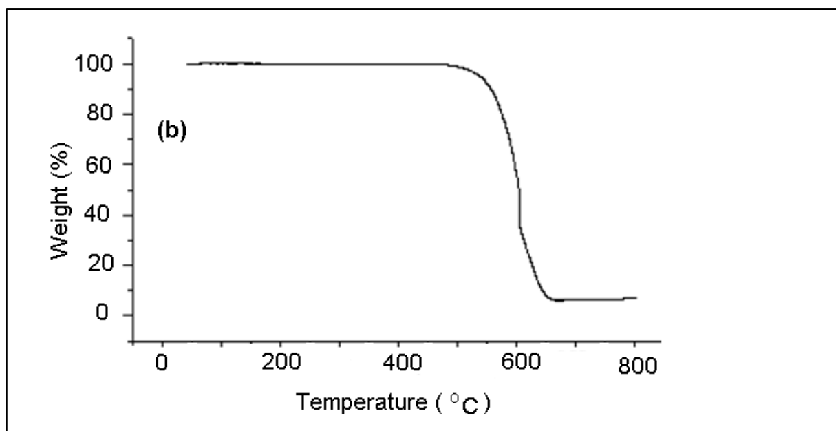
Fig. 7.5. TGA curve of CNTs obtained from the pyrolysis of (a) toluene and ferrocene; (b) toluene and ferrocene in the presence of 8% hexamethylenediamine.
