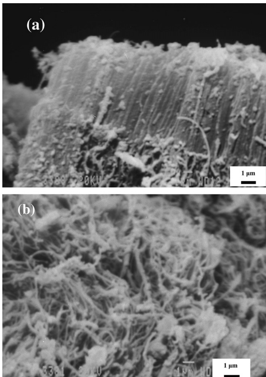
Fig. 5.3. SEM pictures of N-CNT bundles grown from; (a) FcH (2.5 wt.%) and FcH (2.5 wt.%) / PhNH 2 (15 wt.%).
