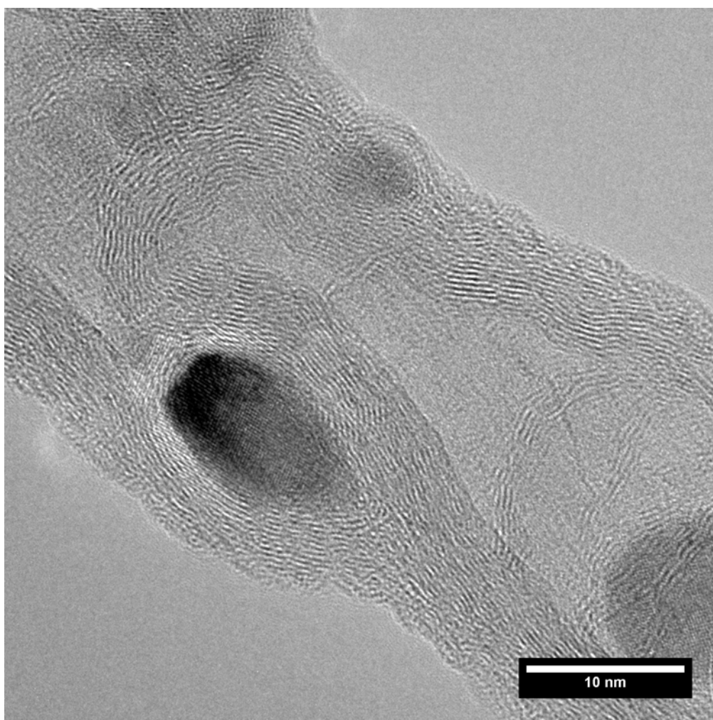
Fig. 11.5. Images of iron nanoparticles in N-CNTs.
