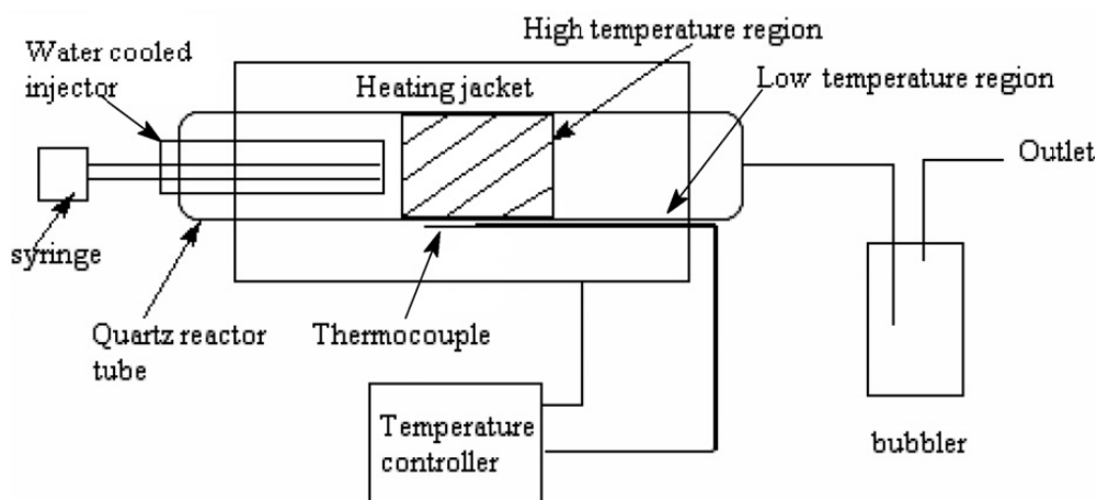
Fig. 2.7. Floating catalyst CVD reactor for the synthesis of SCNM [14].
