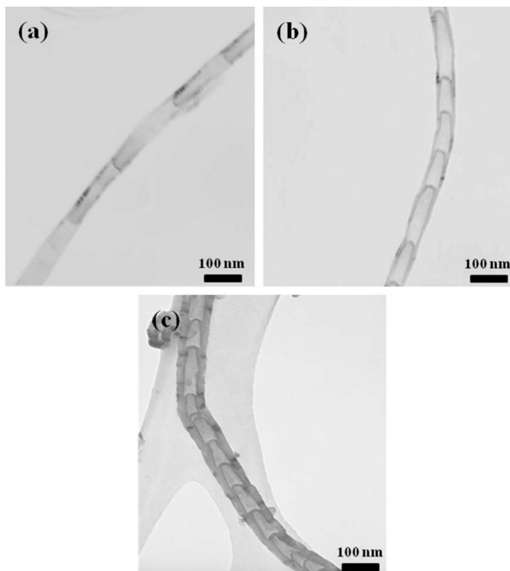
Fig. 6.4. TEM images of N-CNTs showing bamboo structures grown from the pyrolysis of (a) FcH/1-methylimidazole; (b) FcH/2-methylimidazole and (c) FcH/4-methylimidazole (50:50).
