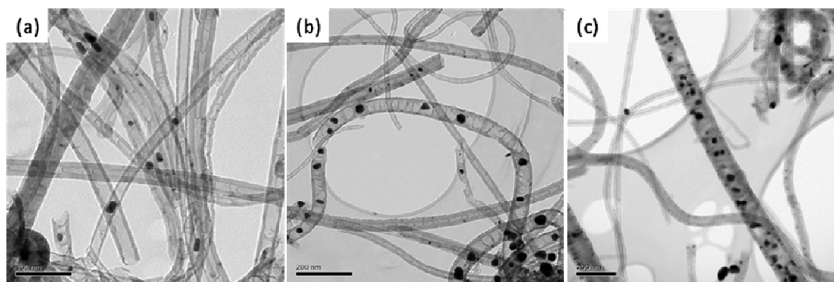
Fig. 10.2. TEM images of (a) Au/CNT; (b) 1 wt.% Au/N-CNT and (c) 3 wt.% Au/N-CNT hybrids.
