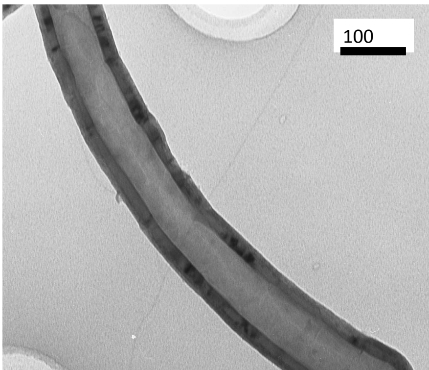
Fig. A6.1. TEM images of CNTs grown from the pyrolysis of FcH (100%).
