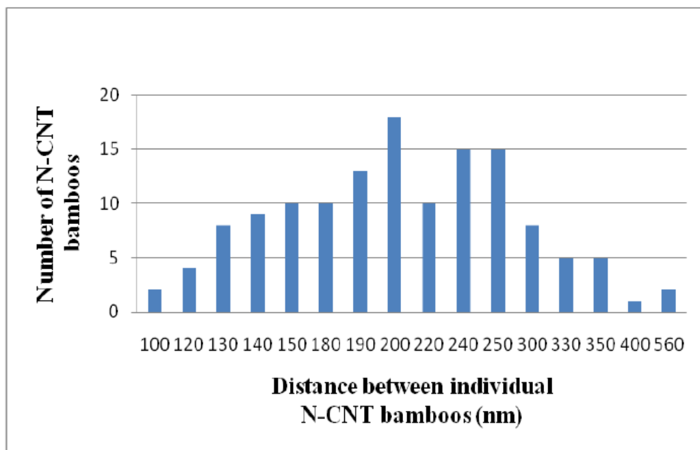
Fig. 6.5. Distance between individual bamboo compartments obtained from the pyrolysis of 1-methylimidazole (50:50).
