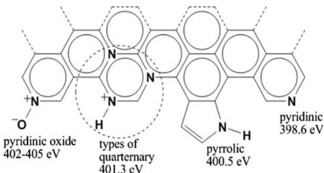
Fig. 4.2. Types of nitrogen species that can be incorporated into graphitic carbon and the XPS binding energies for each type [25].
