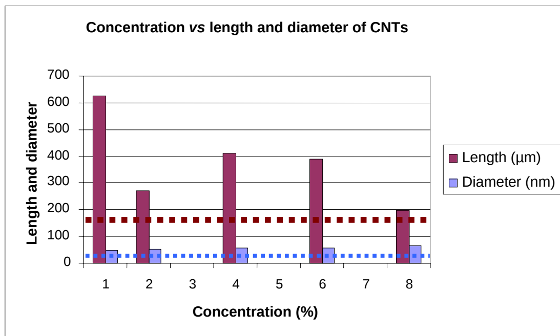
Fig. A7.5. Graph of concentration versus length and diameters of CNTs grown from hexamethylenediamine. Horizontal dotted line indicates lengths and diameters of CNTs obtained from FcH/toluene.
