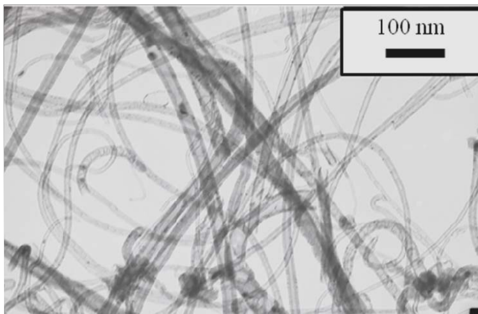
Fig. 11.1. Densely populated N-CNTs grown from 1 wt.% of N-source.
