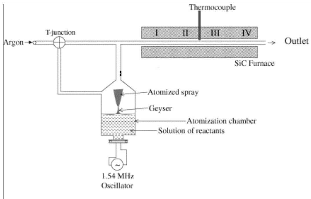
Fig. A7.1. Schematic diagram of the experimental setup for the synthesis of N-CNTs [1,2].
