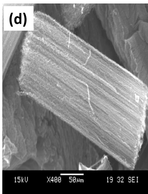
Fig. 7.2. SEM micrographs of CNT obtained from the pyrolysis of toluene and ferrocene in the presence of (a) 2%; (b) 4%; (c) 6%; and (d) 8% formamide.
