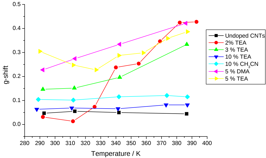
Fig. 9.4. g -shift values vs temperature of undoped and N-CNTs. TEA = triethylamine, CH 3 CN = acetonitrile, DMA = dimethylamine.
