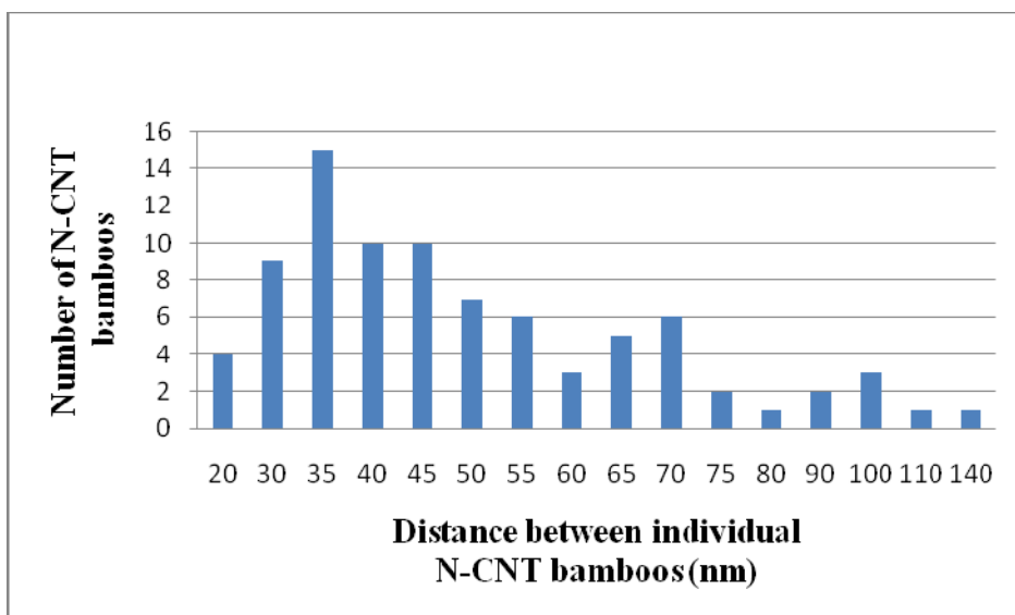
Fig. A6.3. Distance between individual bamboo compartments obtained from the pyrolysis of 4-methylimidazole (50:50).
