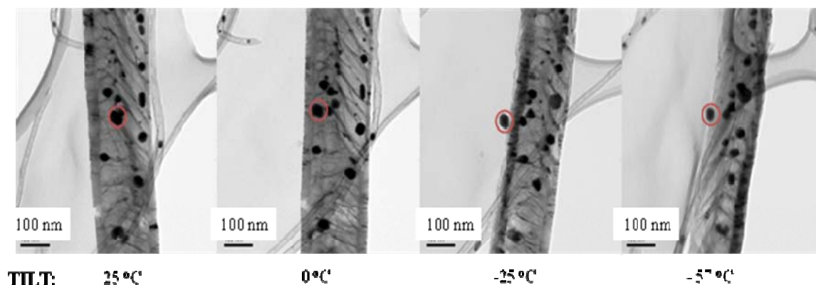
Fig. 10.3. TEM images of Au particles located on the surface of the N-CNT as the nanotube and particles are rotated through a combined orientation of \sim 82^\circ . As the nanotube is tilted, it is revealed that particles (circled) are in fact located on the surface of the nanotube.
