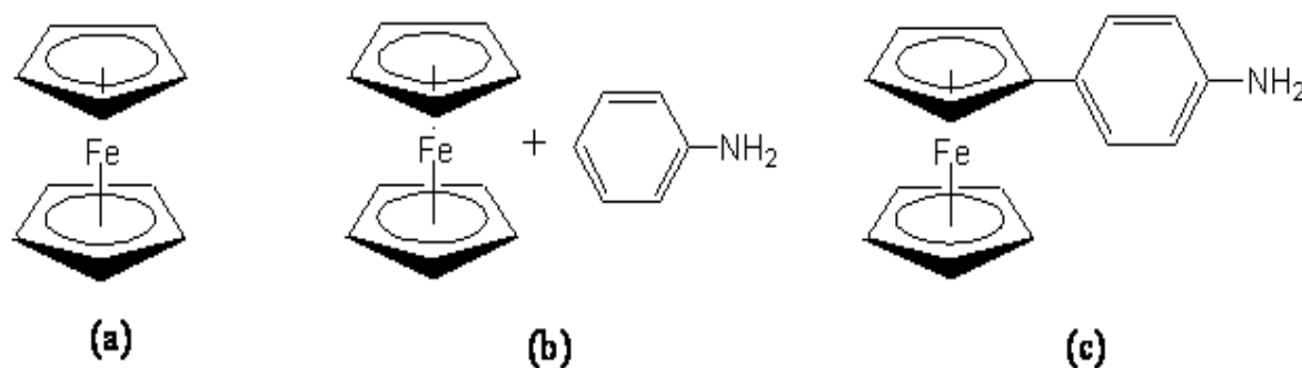
Fig. 5.2. The catalyst systems used with toluene as carbon source: (a) ferrocene (FcH); (b) ferrocene + aniline (FcH/PhNH 2 ) and (c) 4-ferrocenylaniline (FcPhNH 2 ).
