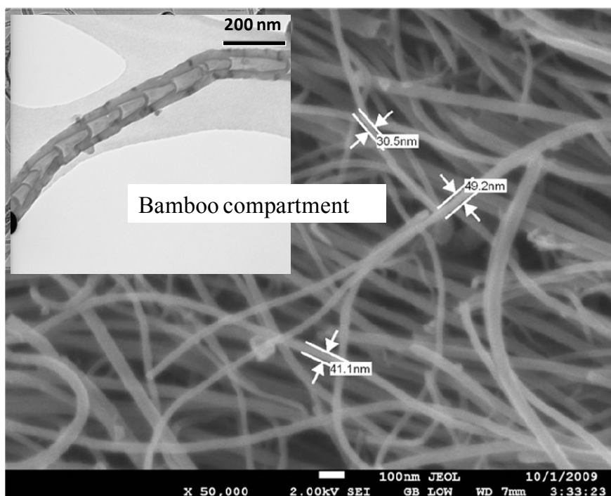
Fig. 9.1 (a). A SEM and TEM image (inset) of N-CNTs synthesized using a mixture of 10% FcH and 10% TEA in toluene.
