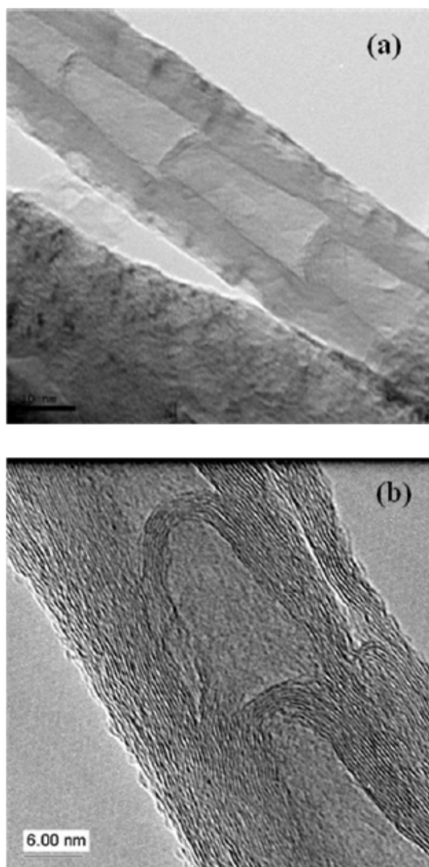
Fig. 7.4. TEM images of CNTs obtained from the pyrolysis of toluene and ferrocene in the presence of 8% diethylamine.
