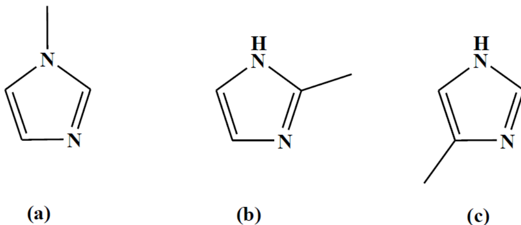
Fig. 6.1. Structures of the N sources used during the formation of SCNMs: (a) 1-methylimidazole; (b) 2-methylimidazole and (c) 4-methylimidazole.
