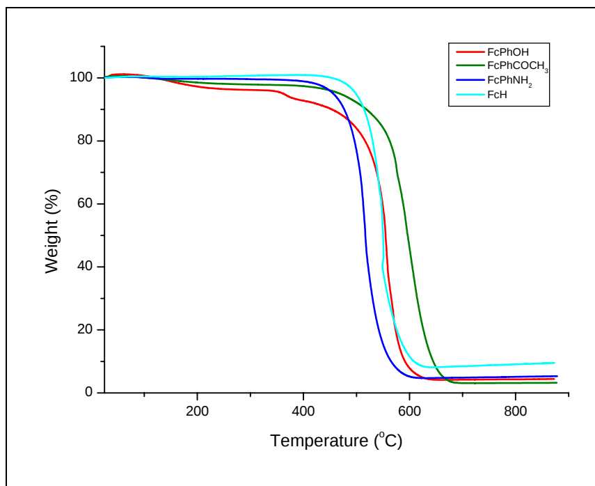
Fig. 8.4. TGA curves of CNTs grown from different arylferrocenes (2.5 wt.%) at 900 °C.
