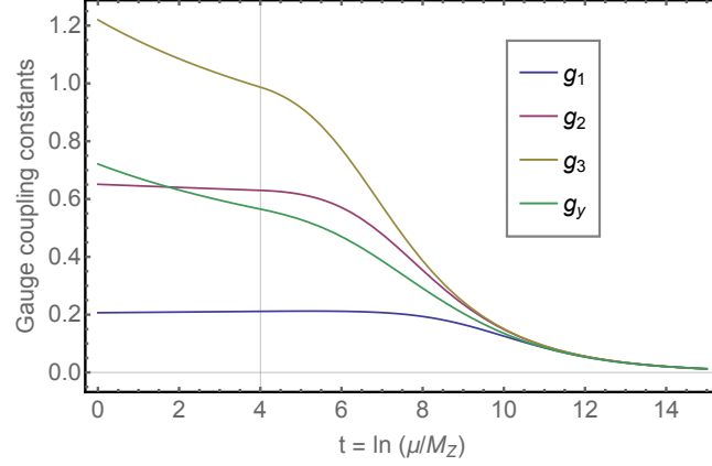
Figure 3.1: Running of the normalised gauge and Yukawa couplings for the SU(3) GHU model, for 1/R = 5 TeV. The first KK mode enters at t_{\text{KK}} \sim 4.0 .
