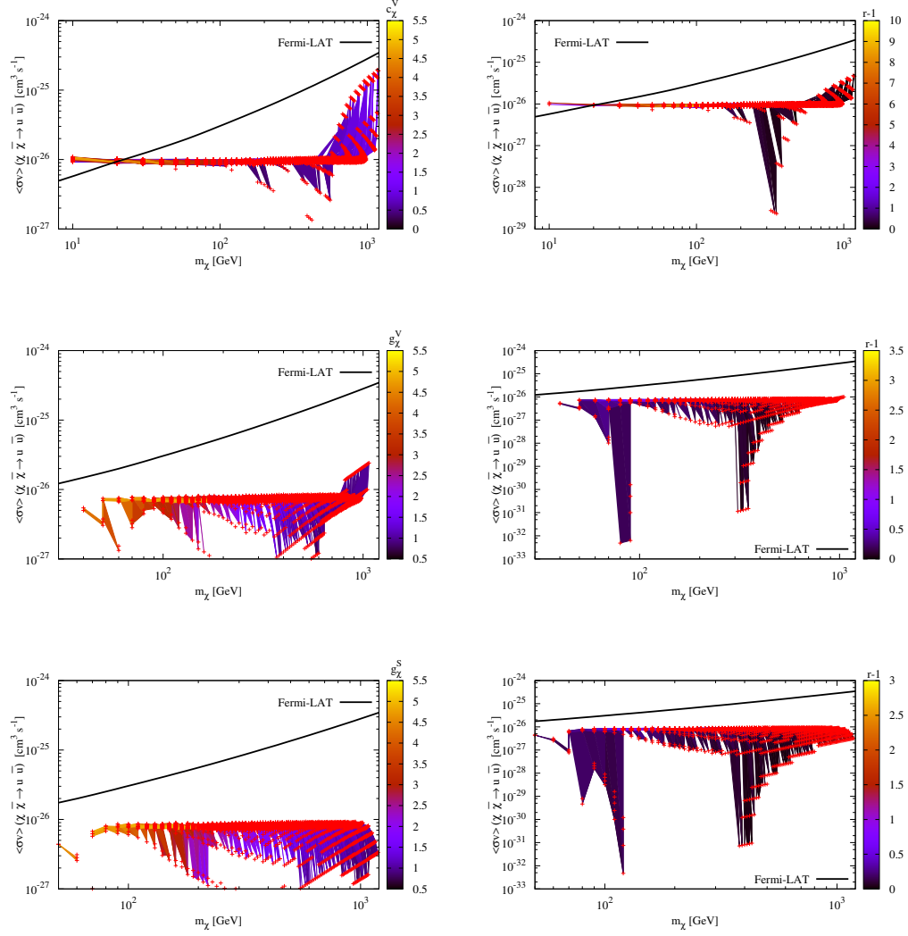
Figure 8.3: The prediction for the DM \chi\bar{\chi} annihilation rate into u\bar{u} , as a function of the DM mass m_\chi . All the parameters are chosen to be consistent with the observed relic density. The top and the middle panels are for dimension-4 and dimension-5 vector interactions respectively. The bottom panels are for the scalar interaction. The colour gradient in the left and right panels correspond to the coupling and mass splitting respectively. Bounds from the Fermi-LAT experiments are also shown [164].
