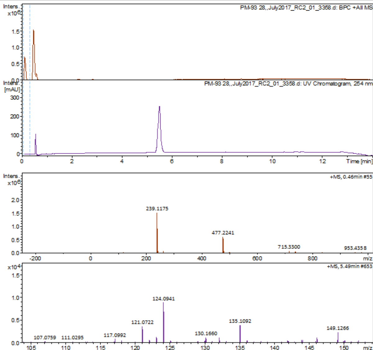
Figure A6. LC-MS analysis for Proxomix-TA018 reduction amination reaction of 58
