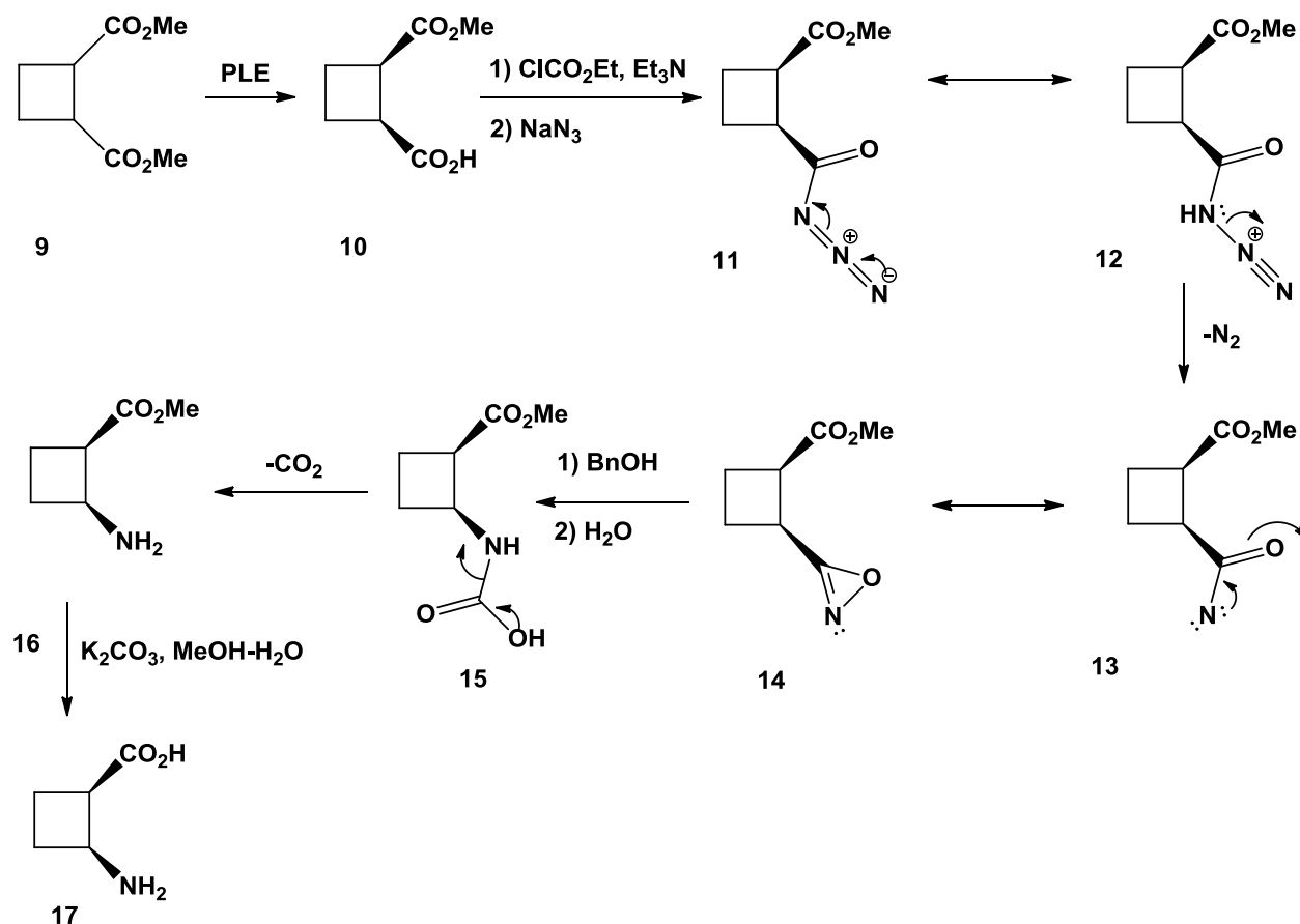
Scheme 3. A stepwise Curtius rearrangement of di-esters 9 . 64,65,66
