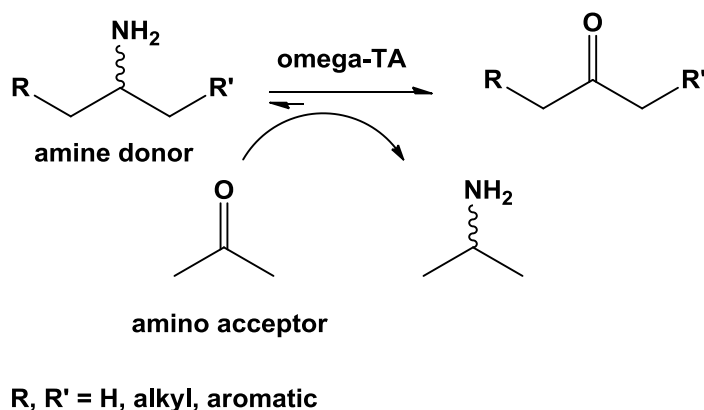
Scheme 4. Deamination of amino group involving transaminases. 78
