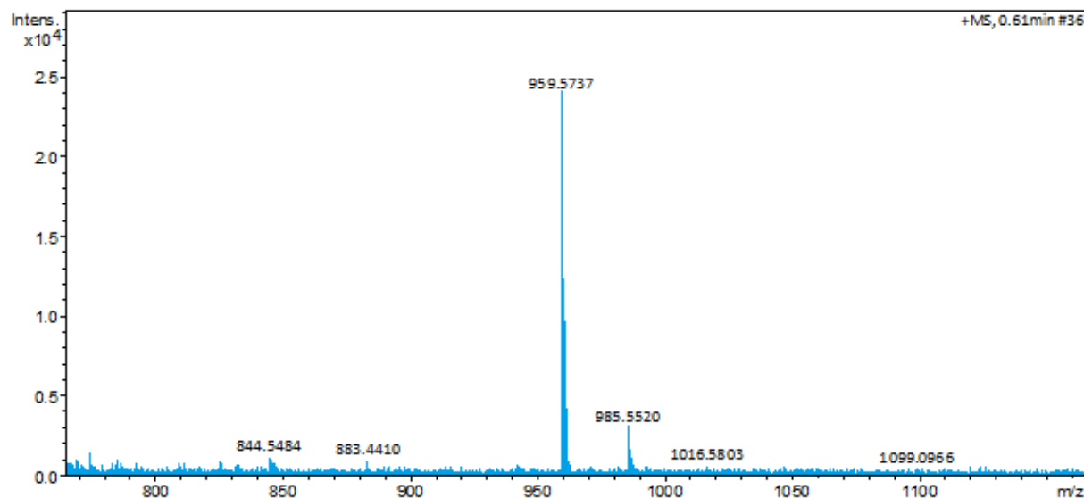
Figure A40. LC-MS analysis of GFOGRGD-Pal 60b
