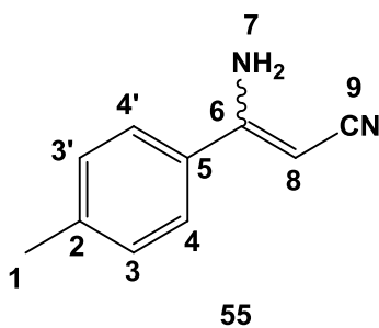
1 H NMR of 55
