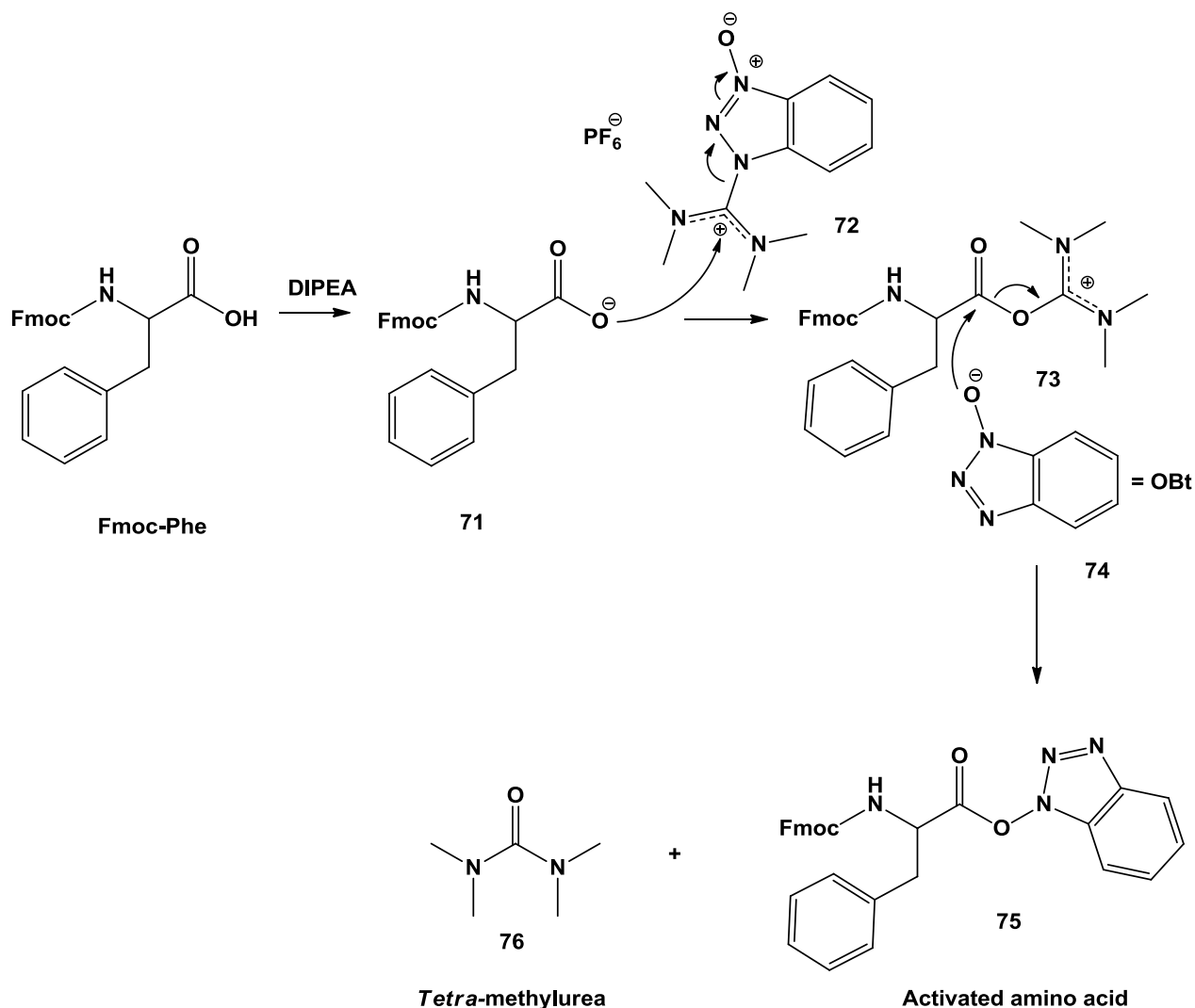
Scheme 35. The activation of amino acid using HBTU 140
