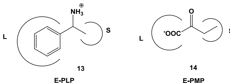
Figure 11. \omega -Transaminase substrate binding depicting the large (L) and small (S) pockets of the PLP form of the enzyme occupied by methylbenzylamine ( 13 ) and 2-oxobutylate ( 14 ). 87
