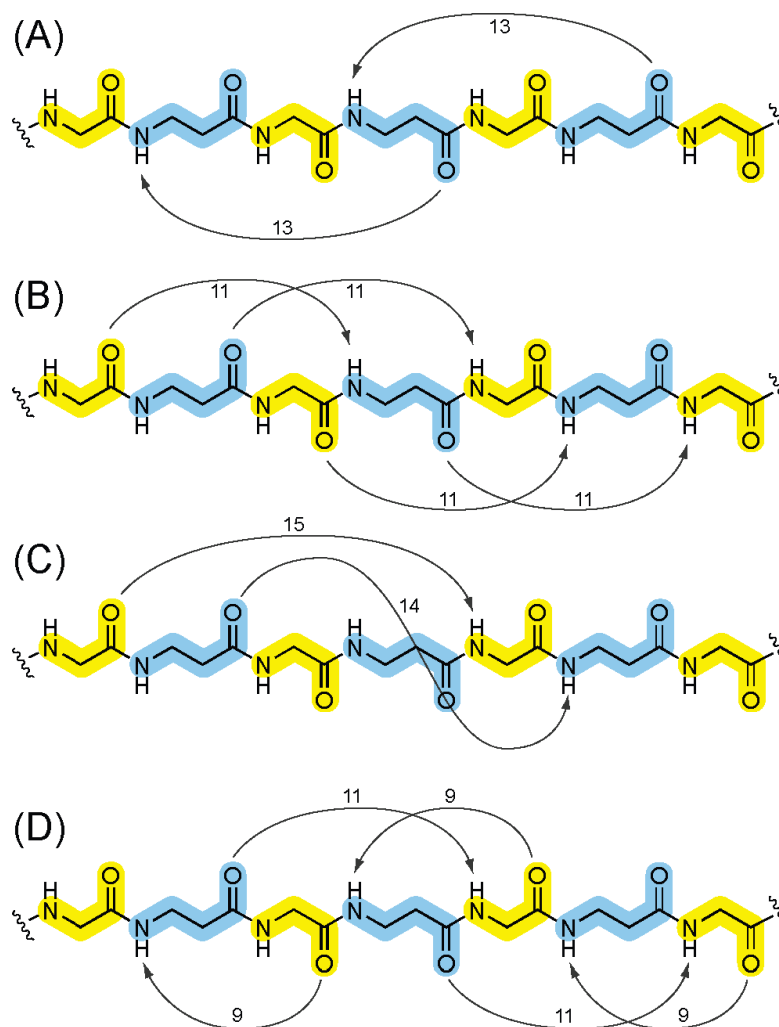
Figure 7. Intramolecular hydrogen bonding possibilities in helices of alpha and beta -amino acid containing peptides. The alpha amino acid residues are highlighted yellow while the beta -amino acid residues are highlighted blue. The hydrogen bonding is indicated by the arrows in different helices from A to D. 36 Reproduced from reference 36. 36
