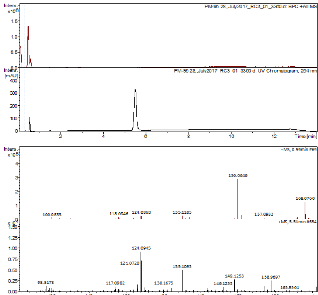
Figure A16. LC-MS analysis for reductive amination reaction involving Prozomix-TA038 at 100 mM of acetophenone
