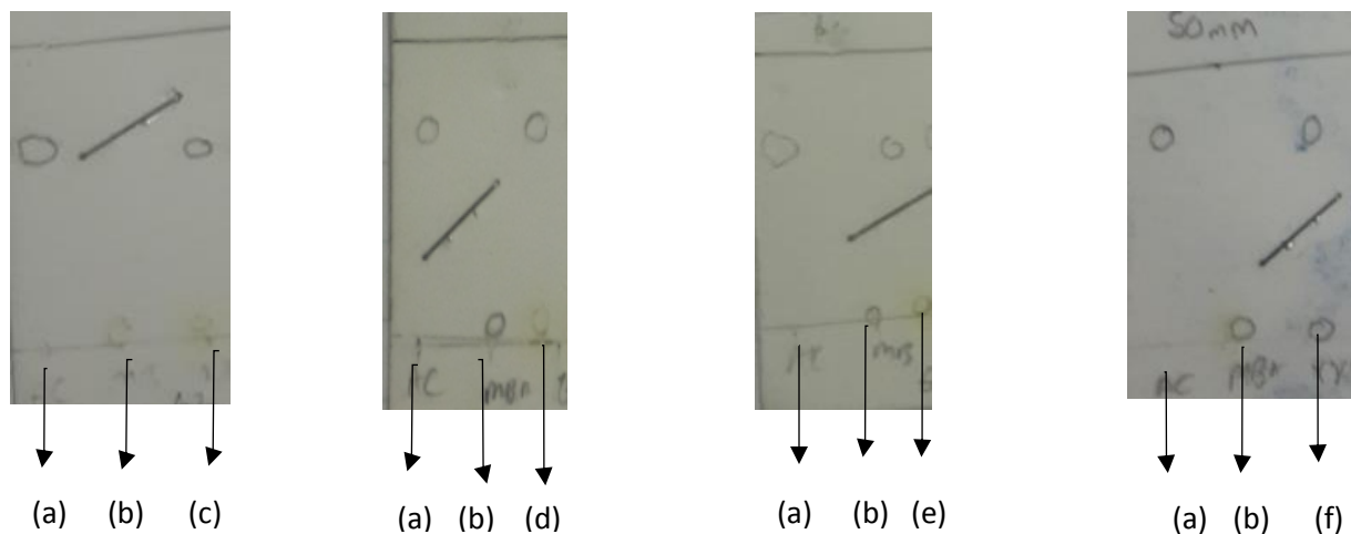
Figure A3. TLC for deamination of MBA (50 mM) (30 %EtOAc/Hexane); (a) The acetophenone standard product. (b) The MBA standard starting material. (c) Reaction involving Prozomix-TA016, (d) Reaction involving Prozomix-TA030, (e) Reaction involving Prozomix-TA037, (f) Reaction involving Prozomix-TA045.
