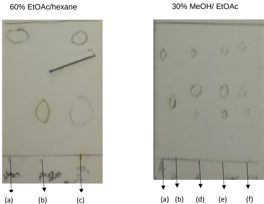
Figure A17. TLC for reductive amination of acetophenone using LDH mixture; (a) Acetophenone standard starting material. (b) MBA standard product. (c) Reaction involving ECS-TA05 with Acetophenone (50 mM). (d) Reaction involved Prozomix-TA016 with Acetophenone (50 mM). (e) Reaction involved Prozomix-TA045 with Acetophenone (50 mM). (f) Reaction involved Aspergillus fumigatus with Acetophenone (50 mM).
