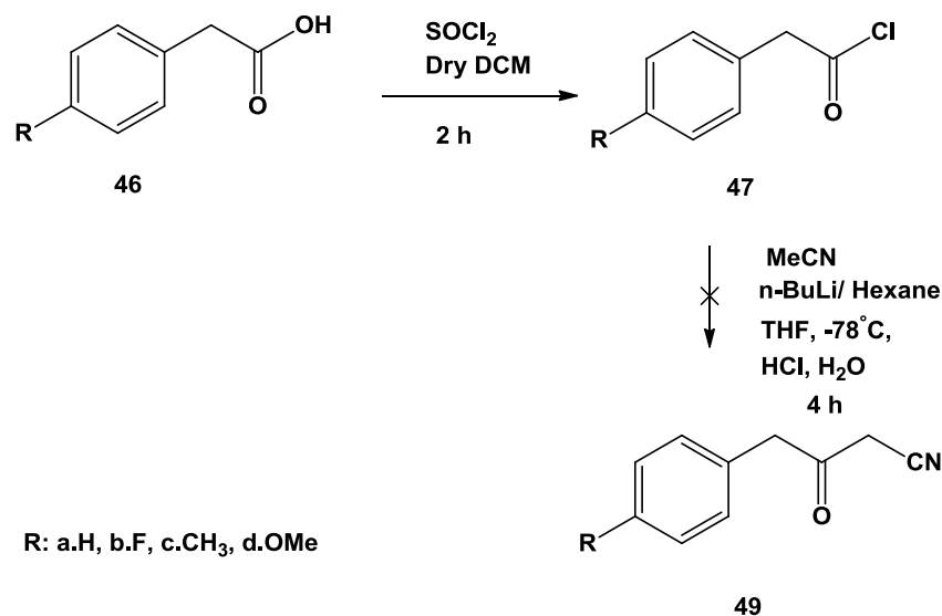
Scheme 16. Proposed synthesis of beta -ketonitriles via acyl chloride.
