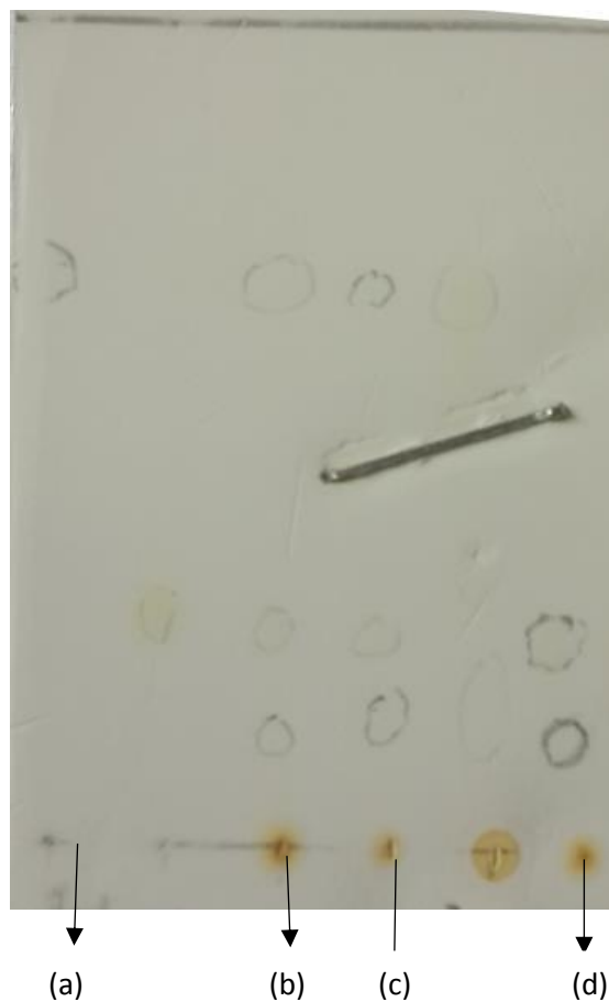
Figure A28. TLC for reductive amination of 54b using diamine donor (40% EtOAc/Hexane). (a) Standard starting material 54d . (b) Reaction involved Prozomix-TA046 . (c) Reaction involving Aspergillus fumigatus . (d) Reaction involving prozomix-TA011 .
