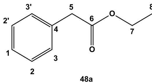
^1\text{H} NMR of 48a
