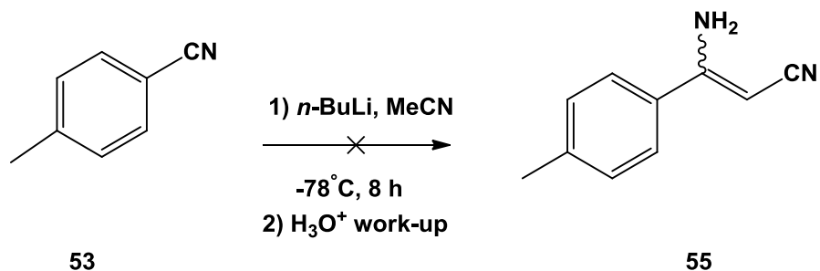
Scheme 23. Synthesis of the enamine using n -BuLi
