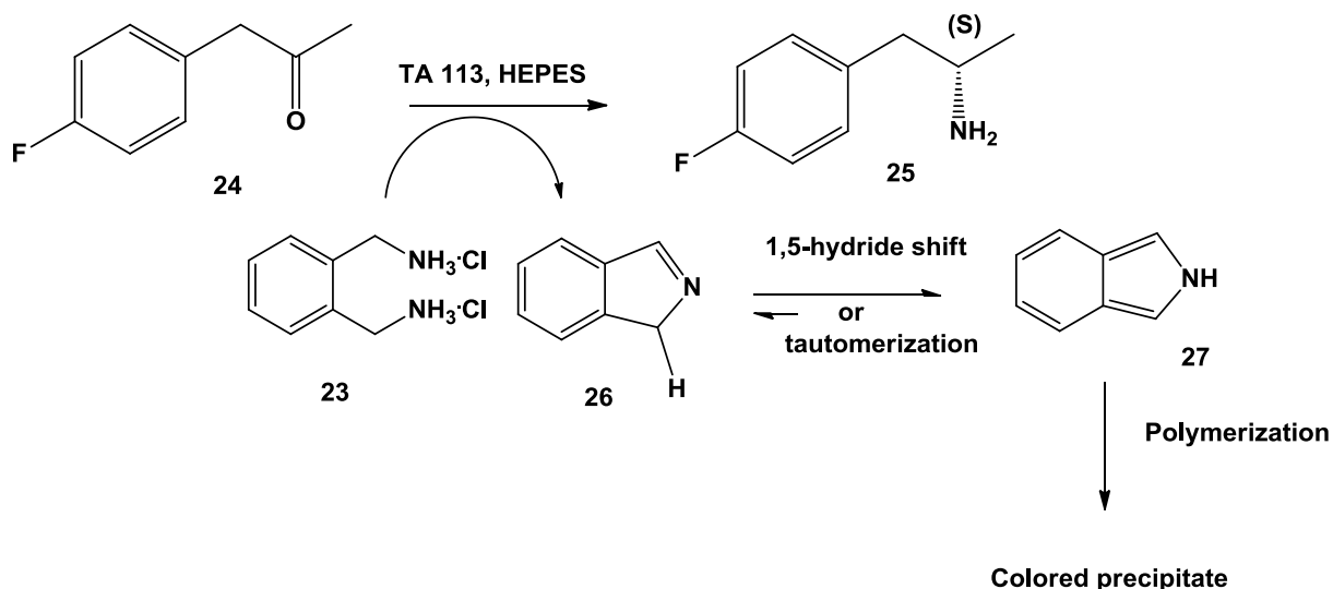
Scheme 9. Conversion of 24 into (S)- 25 using diamine donor ( 23 ) at 1.1 equivalent. HEPES = 4-(2-hydroxyethyl)-piperazine-1-ethanesulfonic acid. 99
