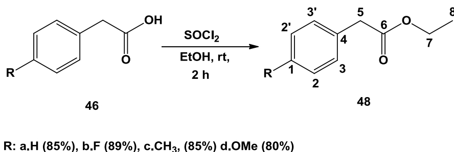
Scheme 17. Esterification of aromatic carboxylic acids using thionyl chloride/ethanol
