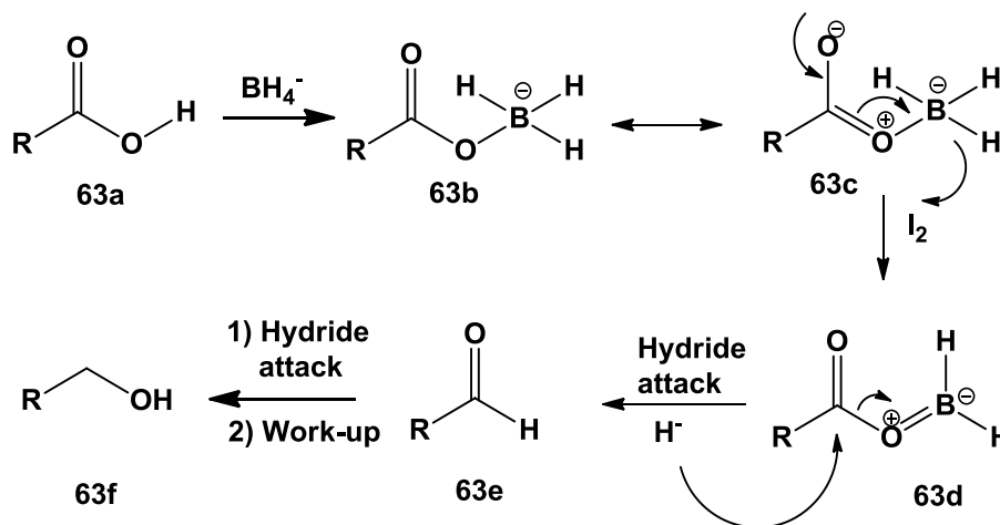
Scheme 21. Proposed mechanism involving \text{NaBH}_4\text{-I}_2
