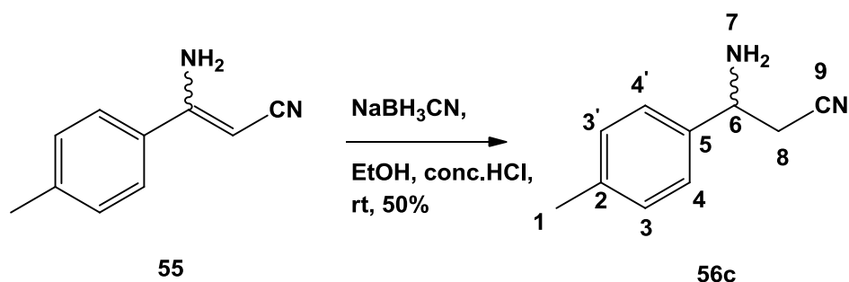
Scheme 26. Synthesis of 3-amino-3-( p -tolyl)propanenitrile 56c using \text{NaBH}_3\text{CN}
