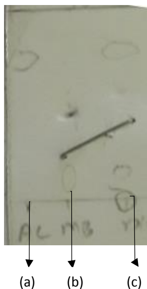
Figure A13. TLC analysis for reductive amination of 58 . (a) Acetophenone standard starting material. (b) MBA standard product. (c) Reaction involving Prozomix-TA024 at 50 mM of acetophenone
