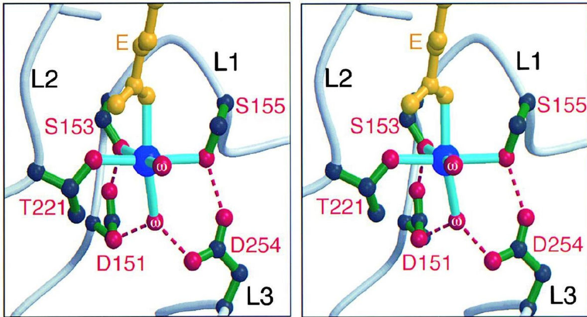
Figure 5. A stereo molecular diagram representing MIDAS. Reproduced from Ref 19. 19
