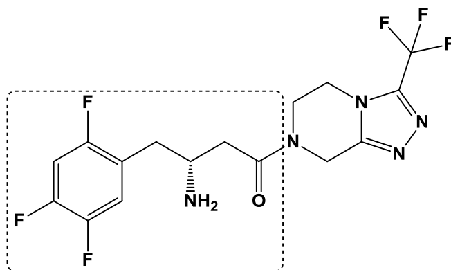
Figure 9. Structural representation of Sitagliptin.
