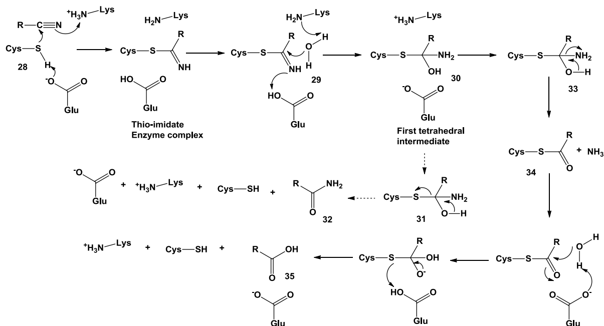
Scheme 11. Nitrilase hydrolysis mechanism for nitrile substrates. 101
