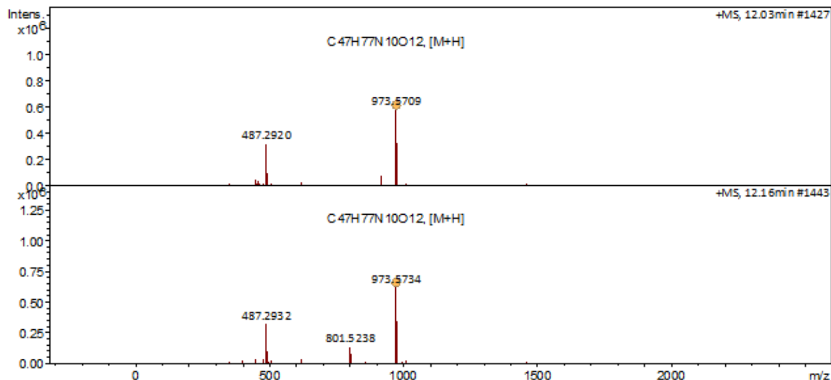
Figure A48. LC-MS analysis for 61b
