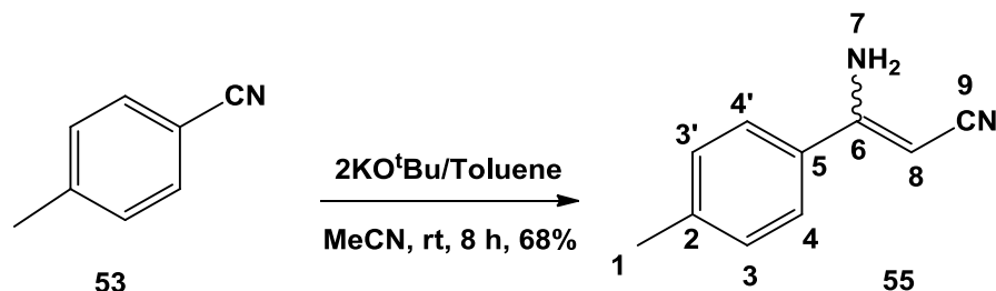
Scheme 25. Synthesis of enamine using KO t Bu/toluene
