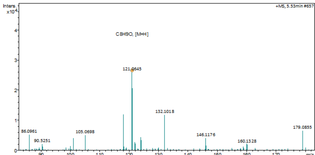
Figure A2. LC-MS data for the standard acetophenone 58
