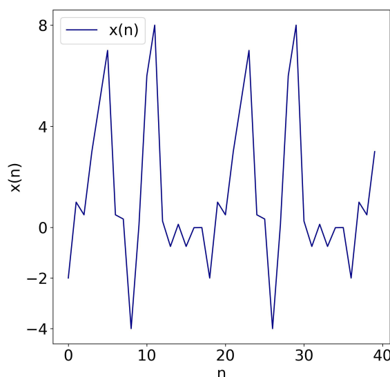
Fig. 1 Graph of x_{n+15} = \frac{x_n x_{n+6} x_{n+12}}{x_{n+3} x_{n+9} (2 + 4x_n x_{n+6} x_{n+12})} with x_0 = -2 , x_1 = 1 , x_2 = 1/2 , x_3 = 3 , x_4 = 5 , x_5 = 7 , x_6 = 1/2 , x_7 = 1/3 , x_8 = -4 , x_9 = 1/9 , x_{10} = 6 , x_{11} = 8 , x_{12} = 1/4 , x_{13} = -3/4 , x_{14} = 1/8 satisfying (1) in Theorem 3.
