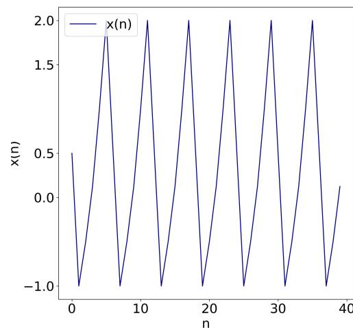
Fig. 2 Graph of x_{n+10} = \frac{x_n x_{n+4} x_{n+8}}{x_{n+2} x_{n+6} (2 + 4x_n x_{n+4} x_{n+8})} with x_0 = 1/2 , x_1 = -1 , x_2 = -1/2 , x_3 = 1/8 , x_4 = 1 , x_5 = 2 , x_6 = 1/2 , x_7 = -1 , x_8 = -1/2 , x_9 = 1/8 satisfying (2) in Theorem 3.
