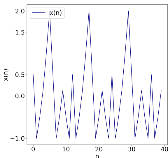
Fig. 4 Graph of x_{n+10} = \frac{x_n x_{n+4} x_{n+8}}{x_{n+2} x_{n+6} (-1 + 4x_n x_{n+4} x_{n+8})} with x_0 = 1/2, x_1 = -1, x_2 = -1/2, x_3 = 1/8, x_4 = 1, x_5 = 2, x_6 = 1/2, x_7 = -1, x_8 = -1/2, x_9 = 1/8 .
