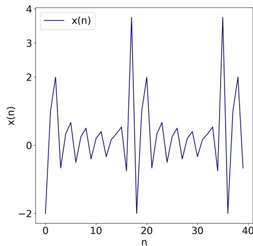
Fig. 3 Graph of x_{n+15} = \frac{x_n x_{n+6} x_{n+12}}{x_{n+3} x_{n+9} (-1 + 4x_n x_{n+6} x_{n+12})} with x_0 = -2 , x_1 = 1 , x_2 = 2 , x_3 = -2/3 , x_4 = 1/3 , x_5 = 2/3 , x_6 = -2/4 , x_7 = 1/4 , x_8 = 2/4 , x_9 = -2/5 , x_{10} = 1/5 , x_{11} = 2/5 , x_{12} = -2/6 , x_{13} = 1/6 , x_{14} = 2/6 .
