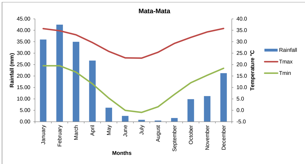
Figure 5.13: Monthly average rainfall (mm), T max and T min for Mata-Mata: 1940 - 2014.
