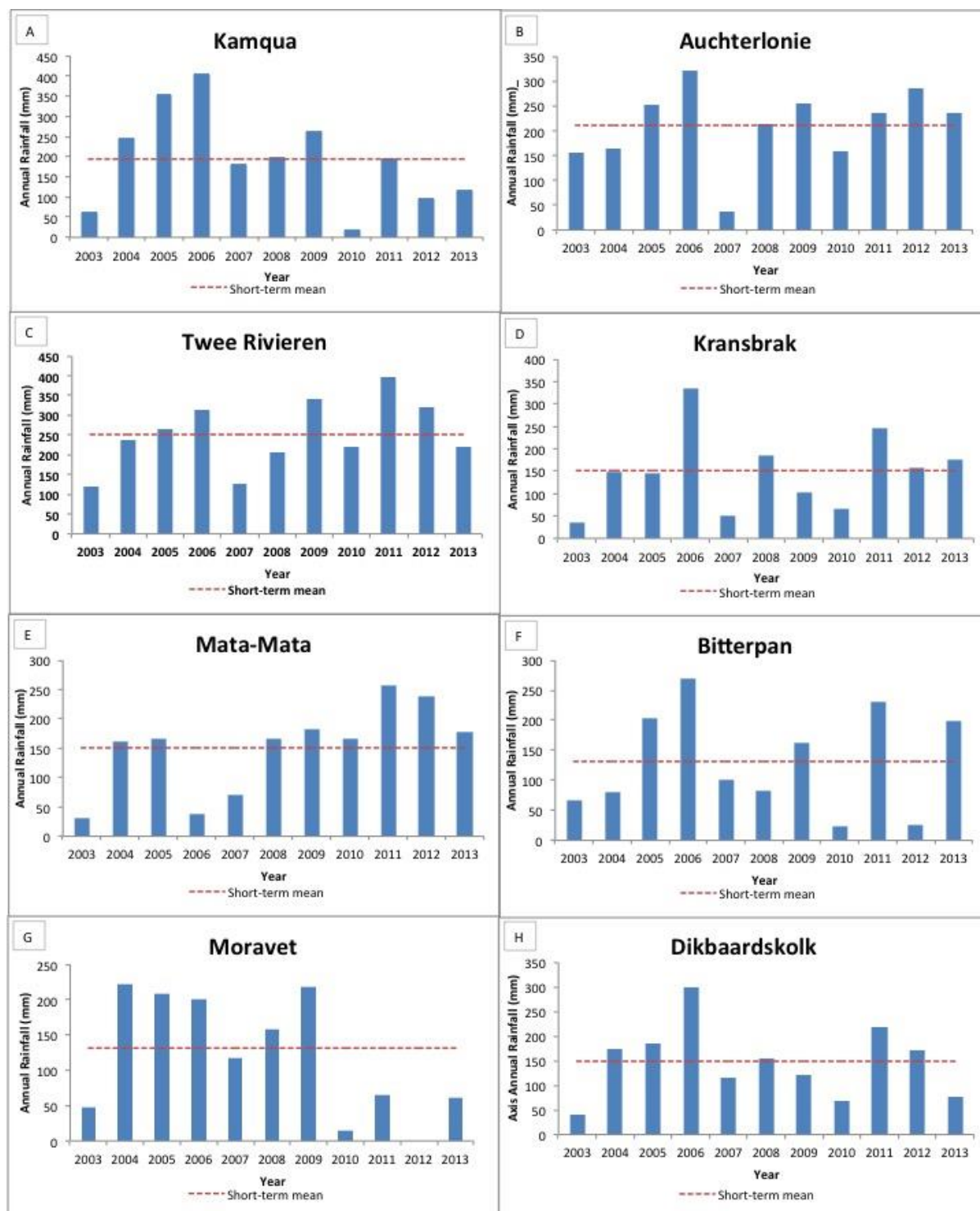
Figure 5.16: Short-term annual rainfall (mm) averages: 2003 - 2013 (A - H).
