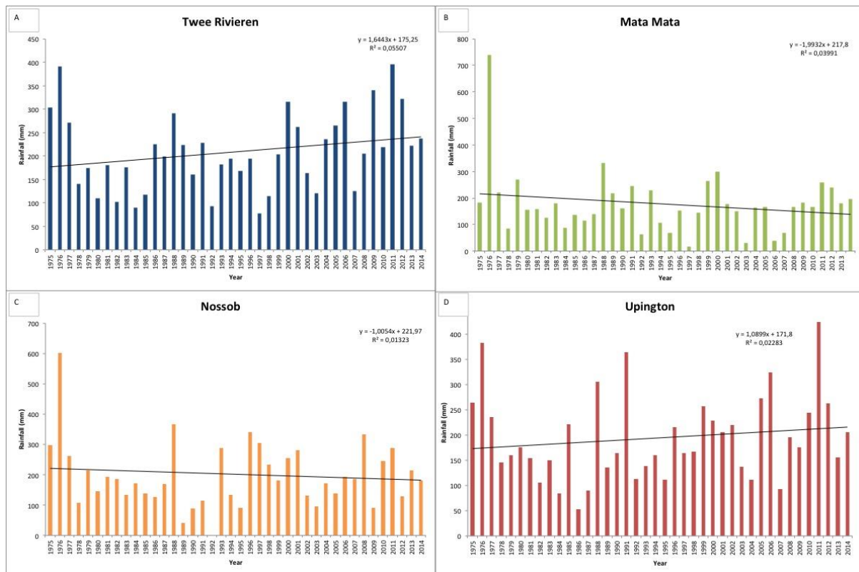
Figure 5.5: Recent rainfall trends for Twee Rivieren, Mata Mata, Nossob and Upington (1975-2014).
