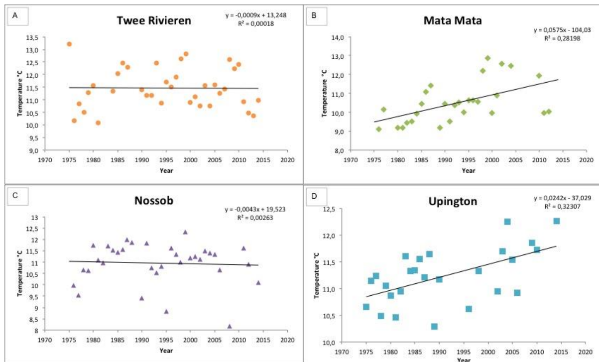
Figure 5.11: Recent temperature T_{\min} trends for Twee Rivieren: 1975 – 2014.
