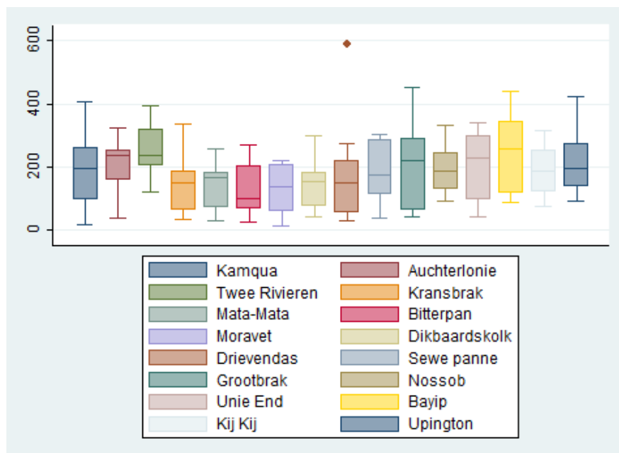
Figure 5.18: Box-and-Whisker Plot demonstrating inter-annual rainfall variability for 16 weather stations in KGNP over the period 2003 - 2013. The mid-line represents the median with the box representing quartiles and the whiskers represent the minimum and maximum. The outliers are represented by a red dot.
