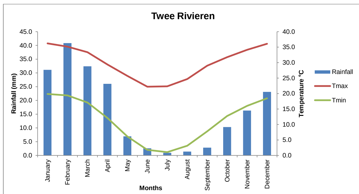
Figure 5.12: Monthly average rainfall (mm), T_{\max} and T_{\min} for Twee Rivieren: 1940 - 2014.
