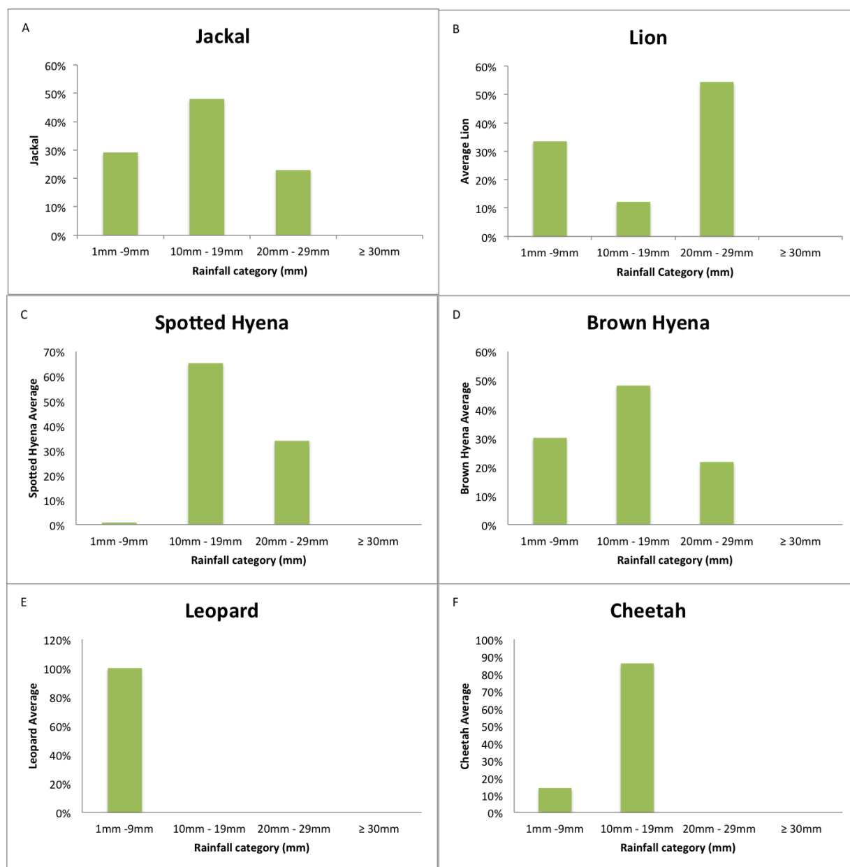
Figure 5.26: Percentage specific species water trough usage during and after specific rainfall quantities, of which four events were recorded \geq 30 mm.
