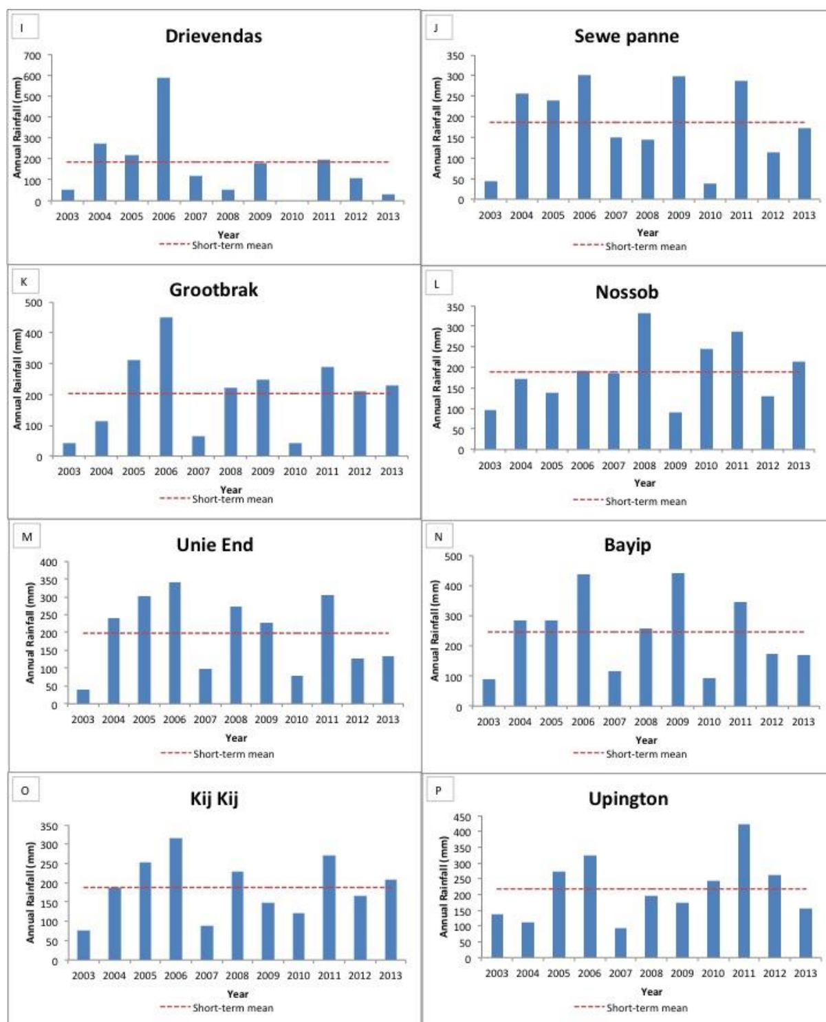
Figure 5.16 continued: continued: Short-term annual rainfall (mm) averages: 2003 - 2013 (I - P).
