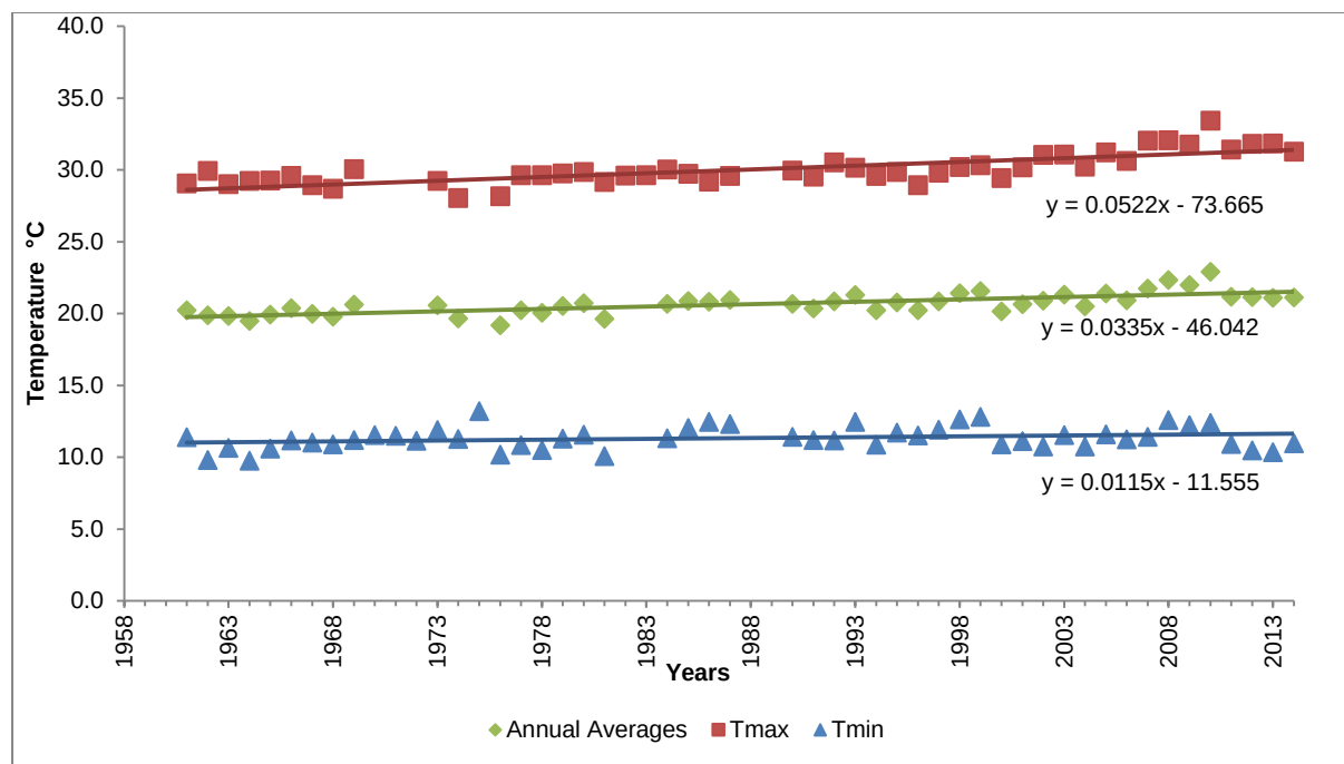
Figure 5.6: Temperature averages, T_{\max} and T_{\min} trends for Twee Rivieren: 1961 - 2014.
