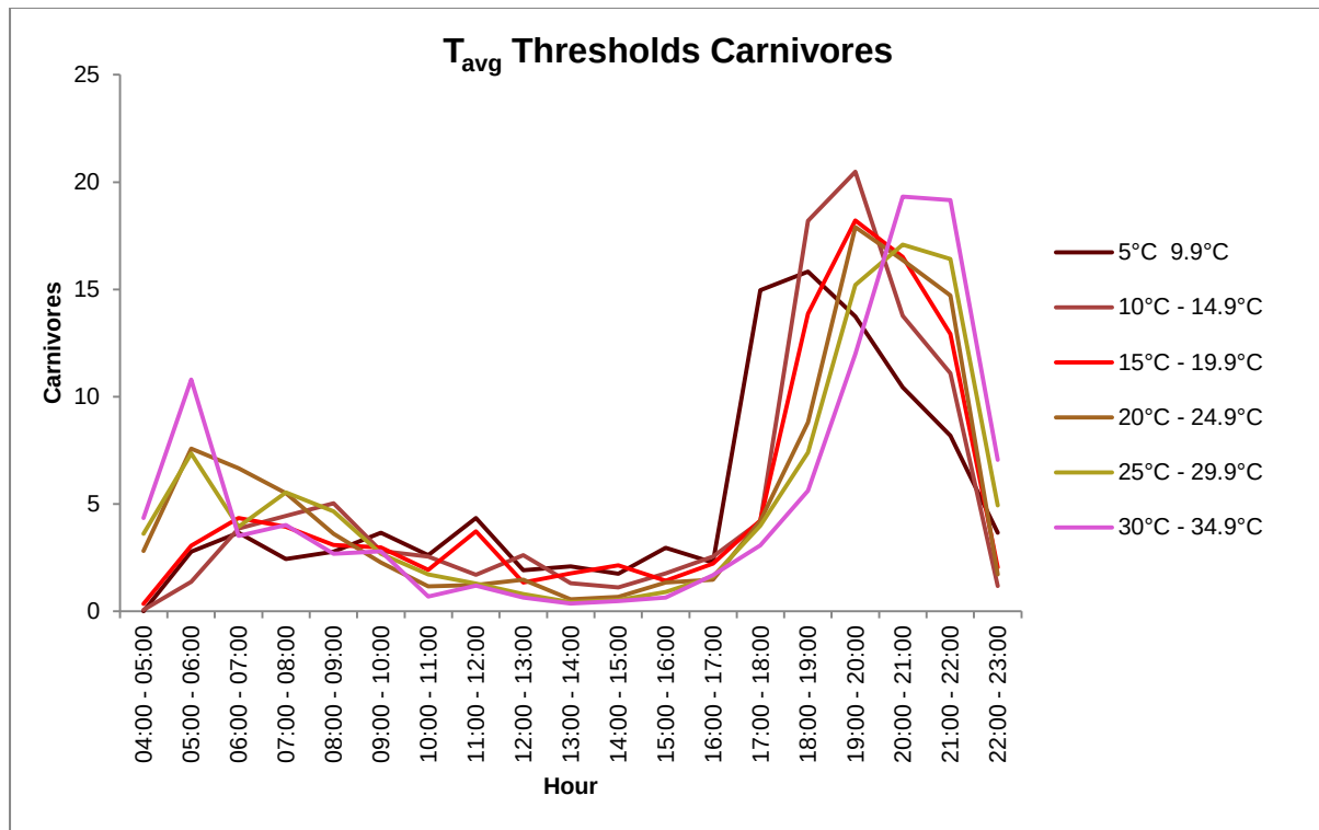
Figure 5.23: Carnivore temperature thresholds and percentage faunal water trough usage.
