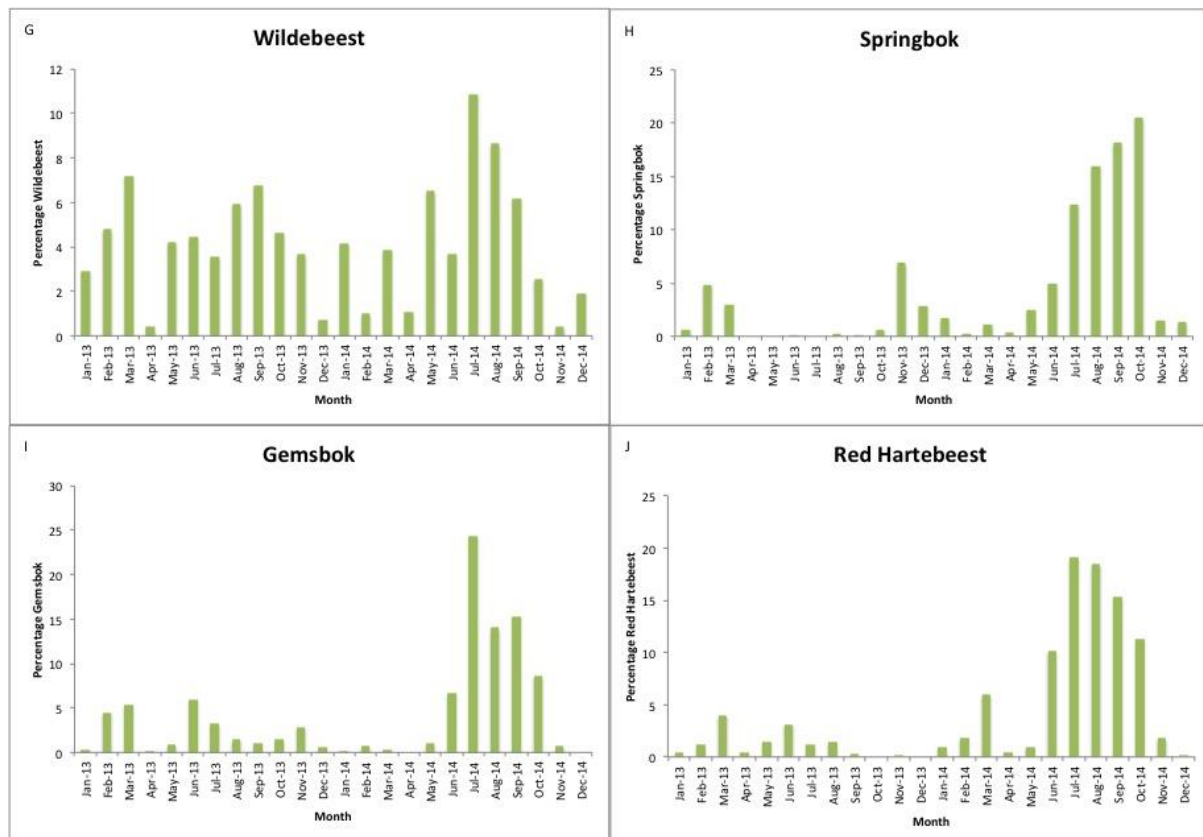
Figure 5.22 continued: Number of fauna utilising the water trough over the study period (January 2013 - December 2014).
