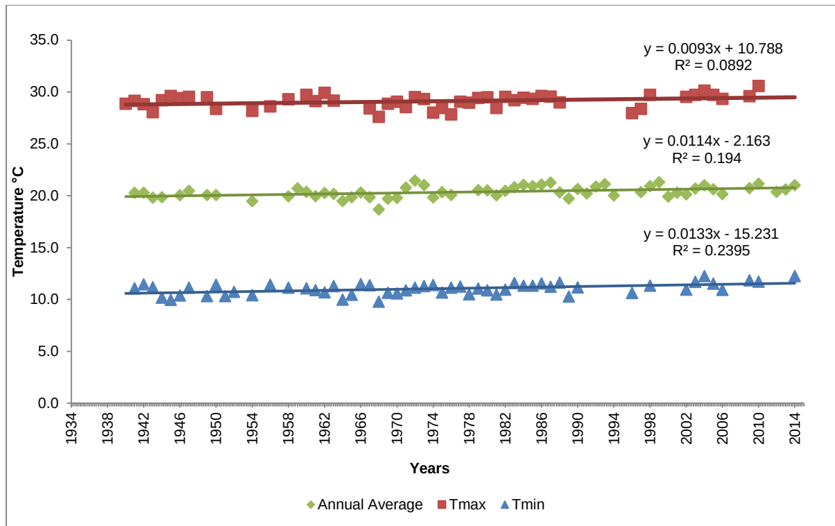
Figure 5.9: Temperature averages, T_{\max} and T_{\min} trends for Upington: 1940-2014.
