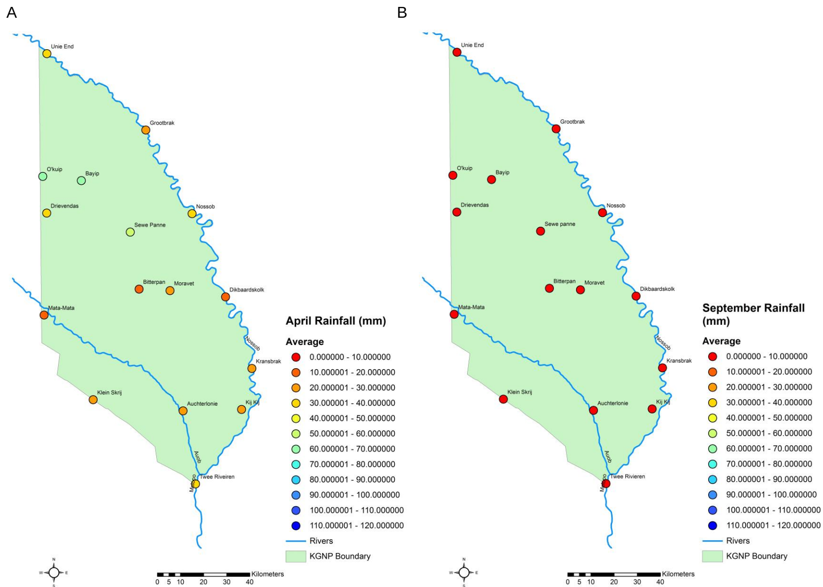
Figure 6.11: Average rainfall for April (A) and September (B) across KGNP over the period 2003 - 2014.
