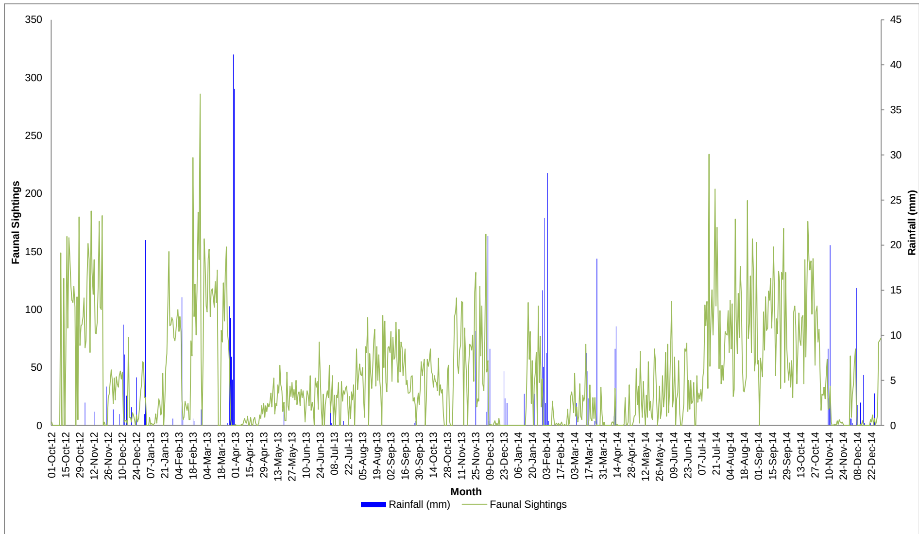
Figure 5.25: Faunal water trough usage during and after rainfall events.
