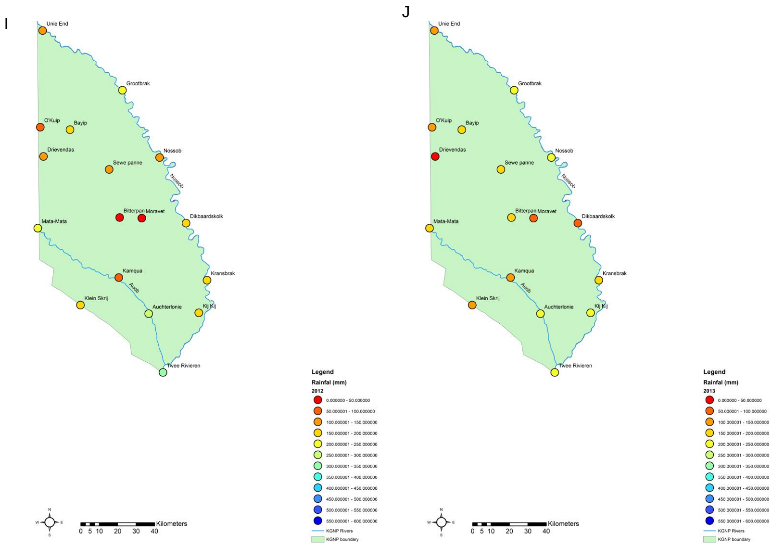
Figure 6.1: Inter-annual rainfall variability (mm) across KGNP for the period 2004-2013 (A-J).
