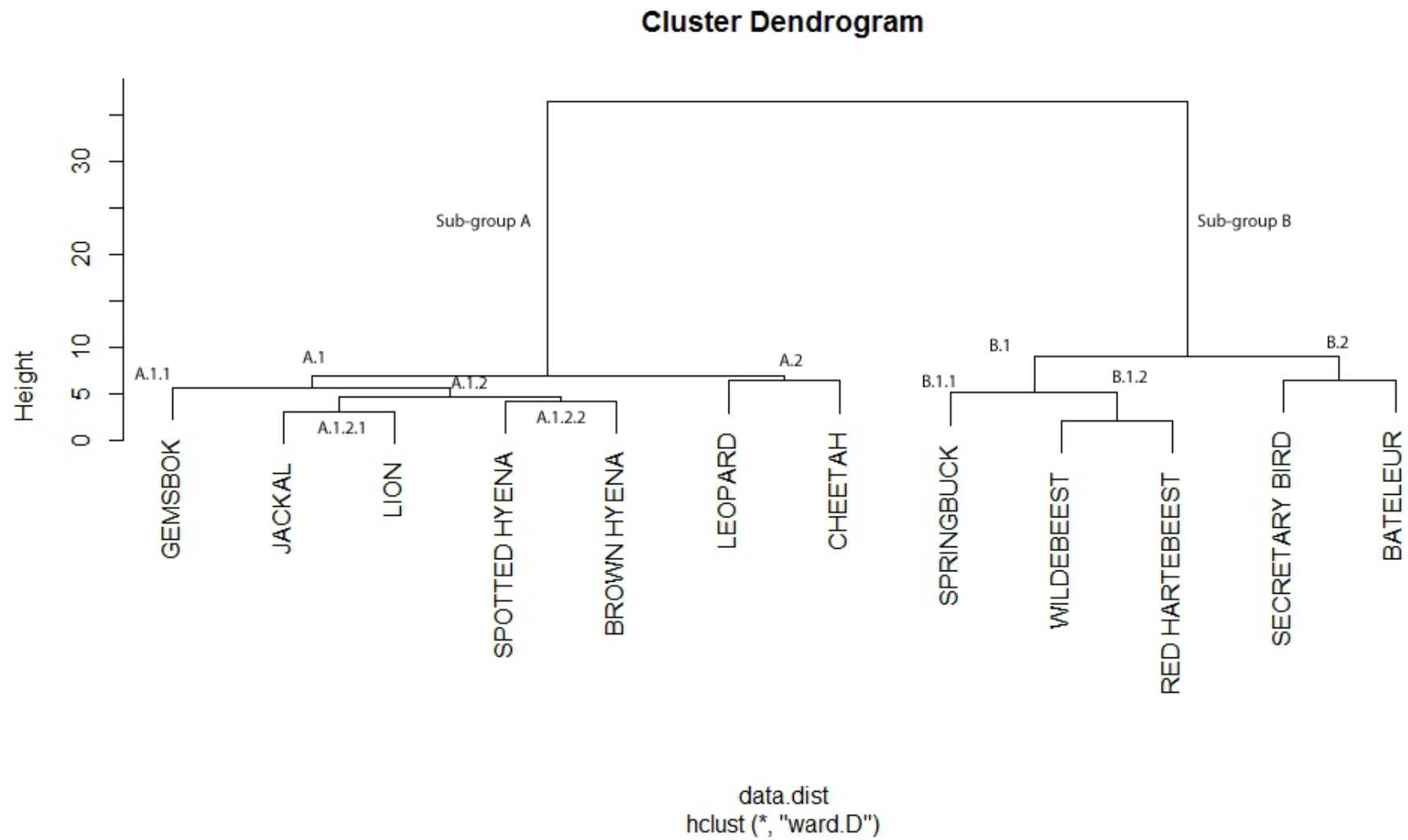
Figure 5.20: Cluster analyses of animals grouped according to the distribution of visiting times.
