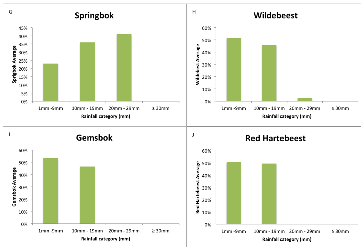
Figure 5.26 continued: Percentage specific species water trough usage during and after specific rainfall quantities, of which four events were recorded \geq 30 mm.
