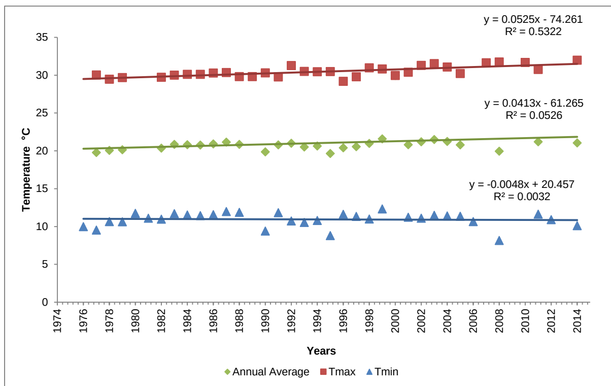
Figure 5.8: Temperature averages, T max and T min trends for Nossob: 1975-2014.
