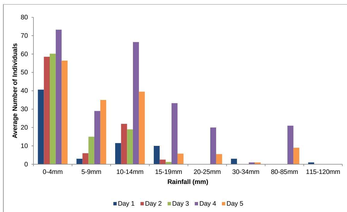
Figure 5.27: Average faunal sightings observed up to 5 days after specific rainfall events natural surface water dissipates (October 2012 - December 2014).
