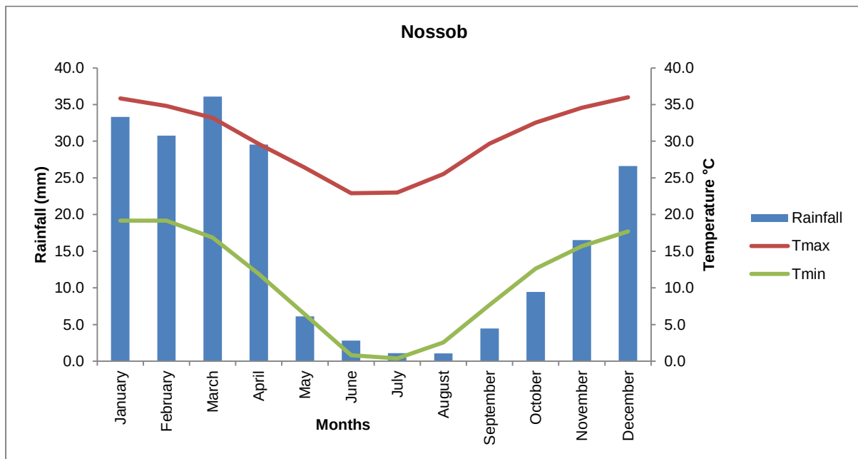
Figure 5.14: Monthly average rainfall (mm), T max and T min for Nossob: 1940 - 2014.
