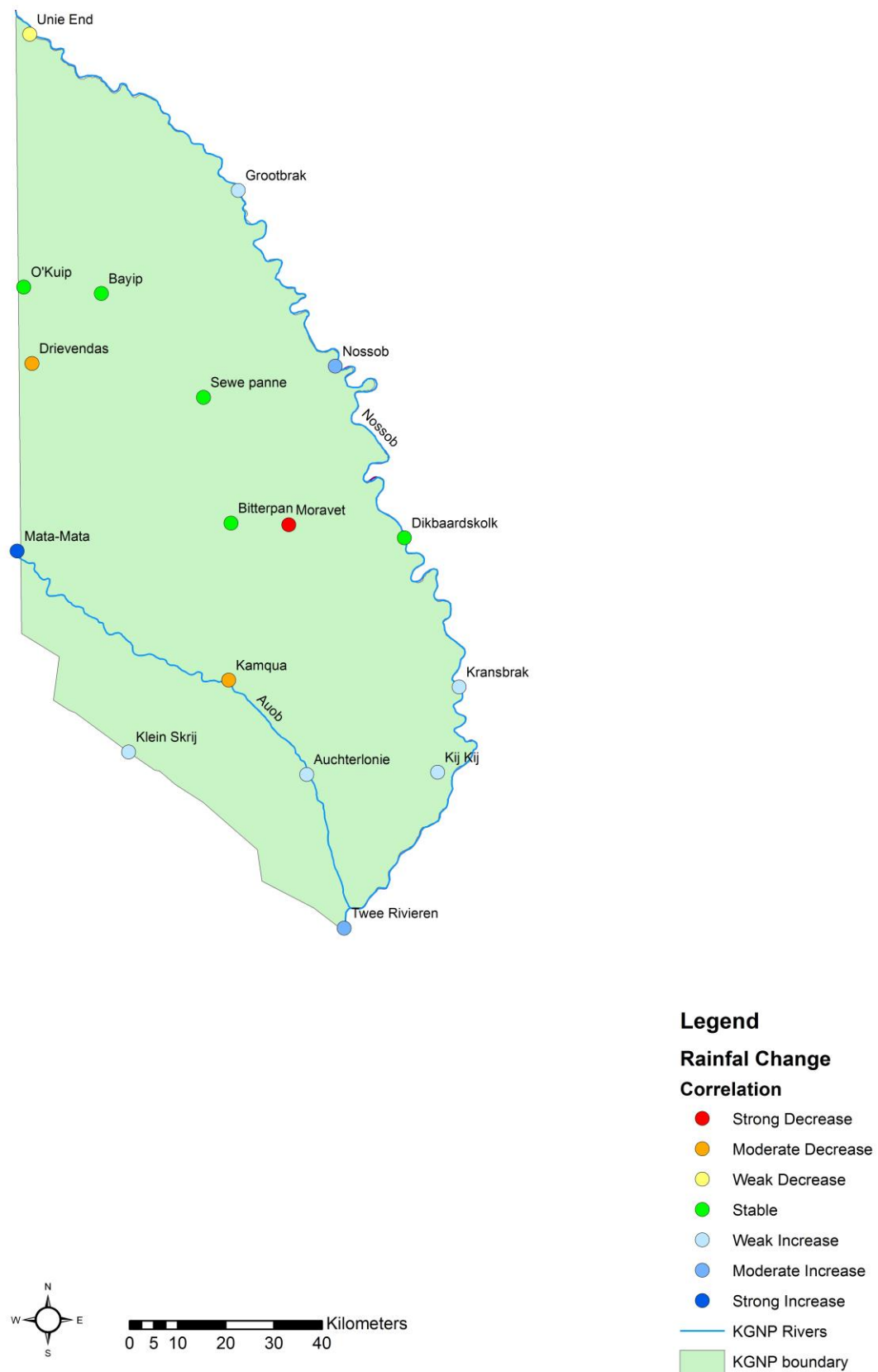
Figure 6.3: Map indicating decreasing, stable and increasing rainfall trends over the period 2003 - 2004 in KGNP.
