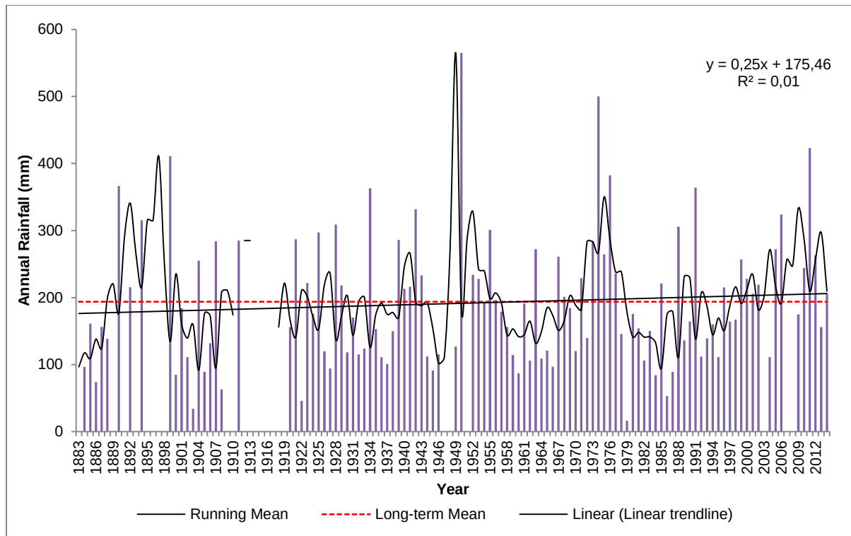
Figure 5.4: Long-term rainfall trends for Upington: 1883 - 2014.
