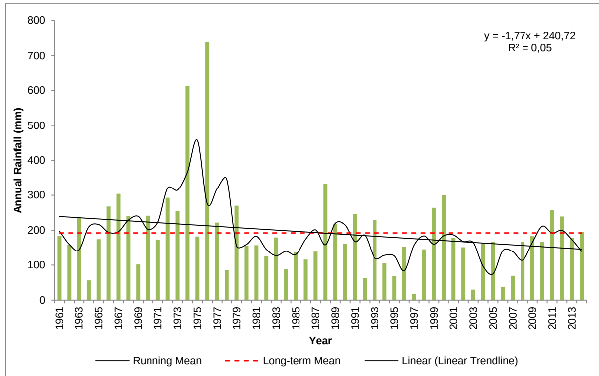
Figure 5.2: Long-term rainfall trend for Mata-Mata: 1961 - 2014.
