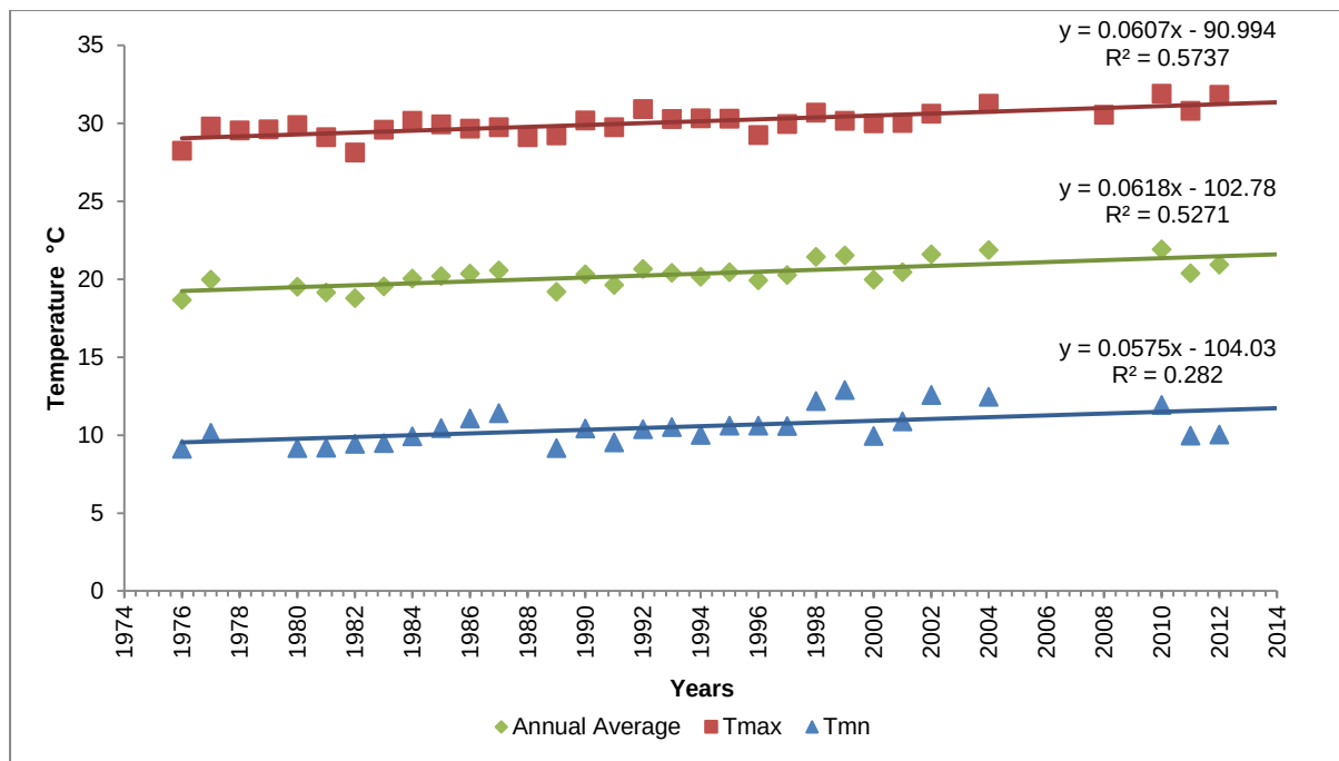
Figure 5.7: Temperature averages, T max and T min trends for Mata-Mata: 1975 - 2014.
