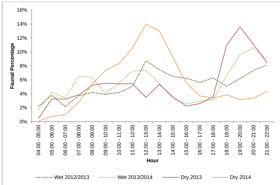
Figure 5.19: Species water trough usage during the wet and dry seasons (October 2012 - August 2014).
