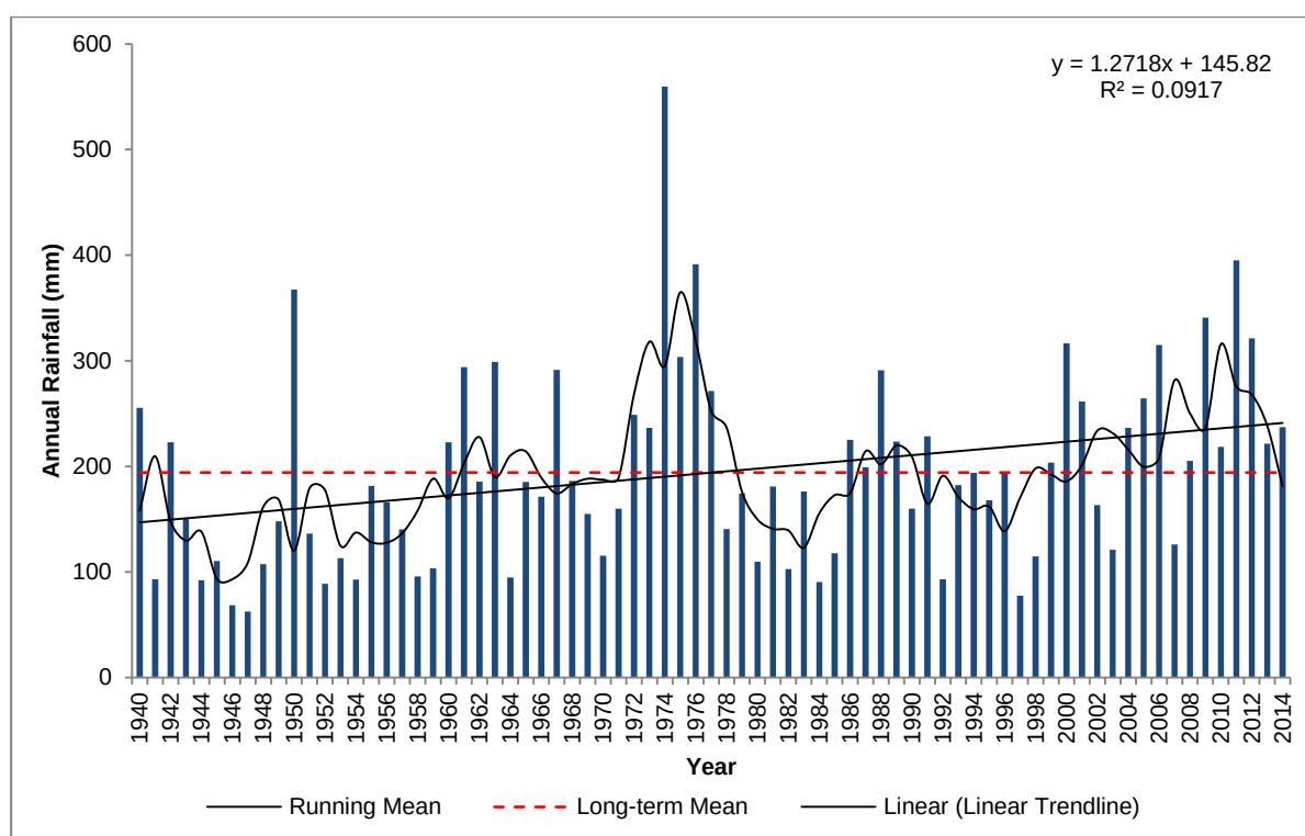
Figure 5.1: Long-term rainfall trends for Twee Rivieren: 1940 - 2014.
