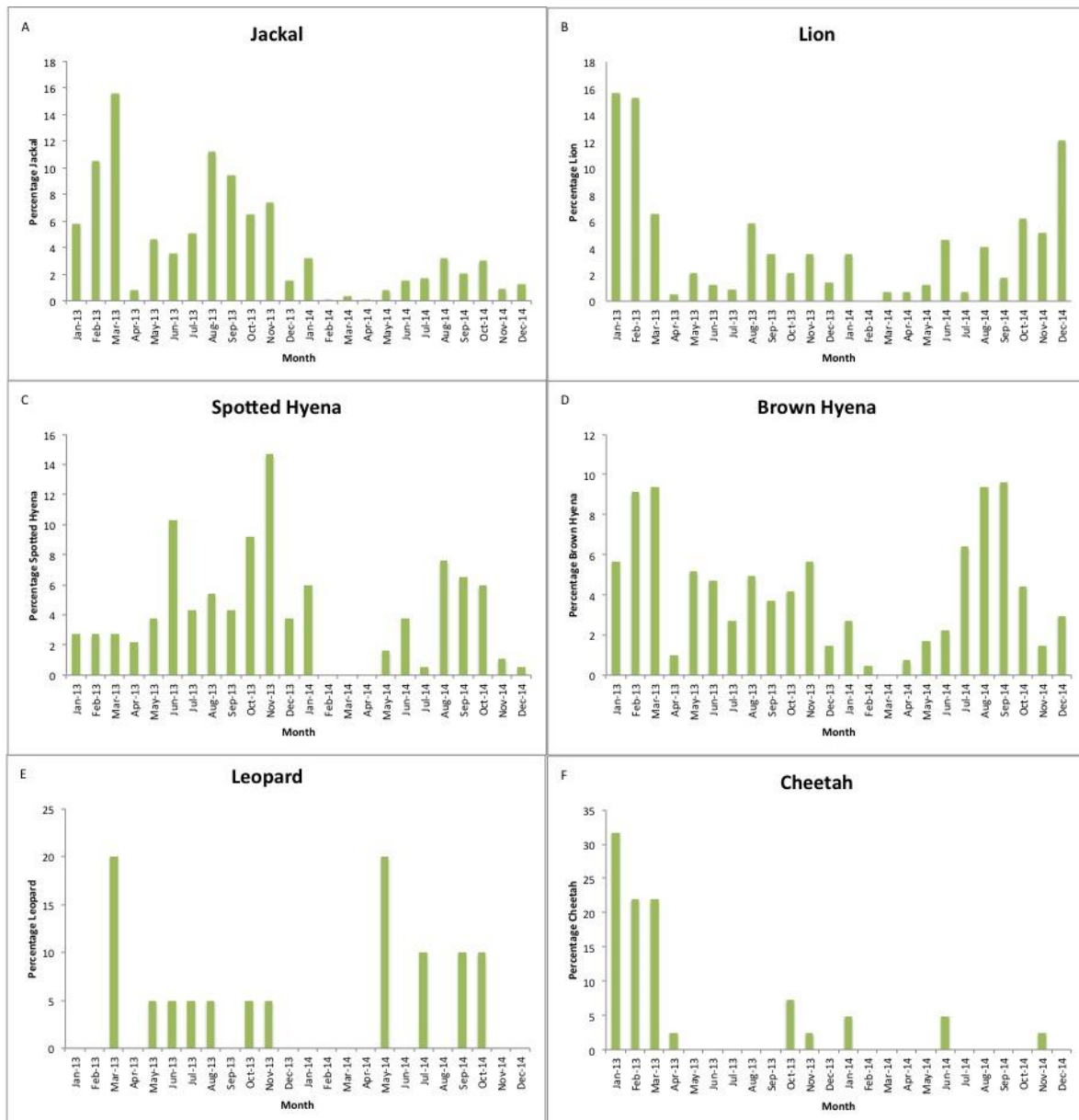
Figure 5.22: Number of fauna utilising the water trough over the study period (January 2013 - December 2014).
