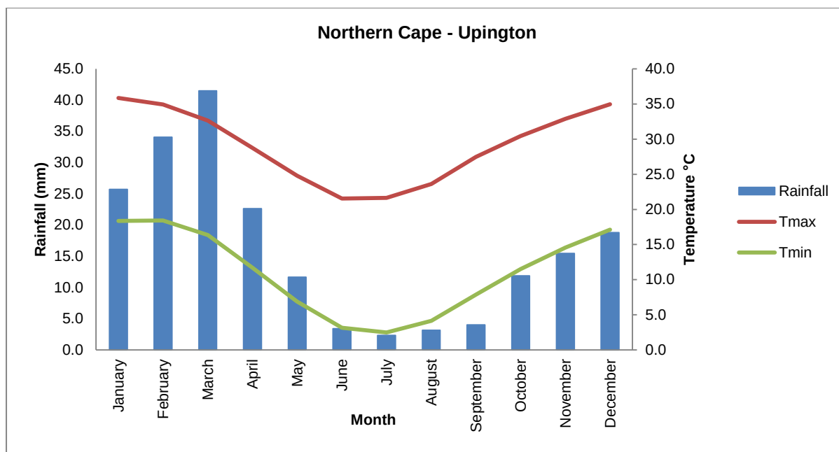
Figure 5.15: Monthly average rainfall (mm), T max and T min for Upington: 1940 - 2014.
