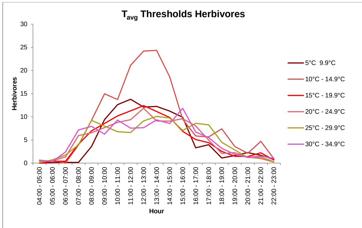
Figure 5.24: Herbivore temperature thresholds and percentage faunal water trough usage.
