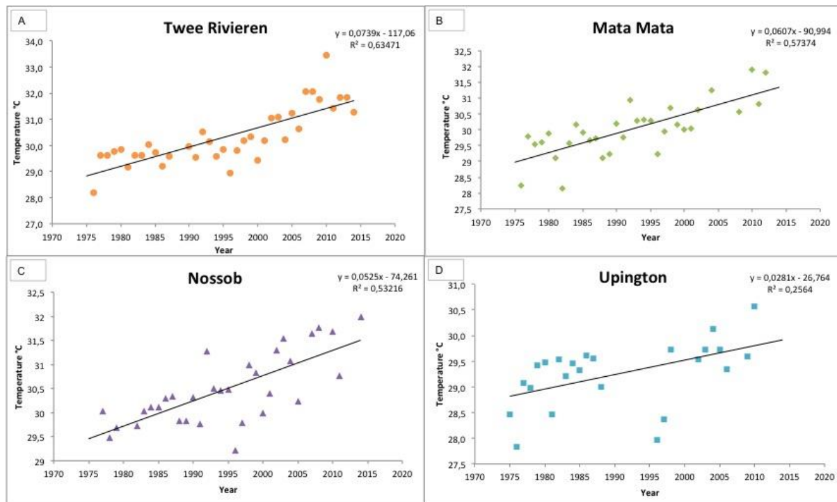
Figure 5.10: Recent temperature T_{\max} trends for Twee Rivieren: 1975 - 2014.
