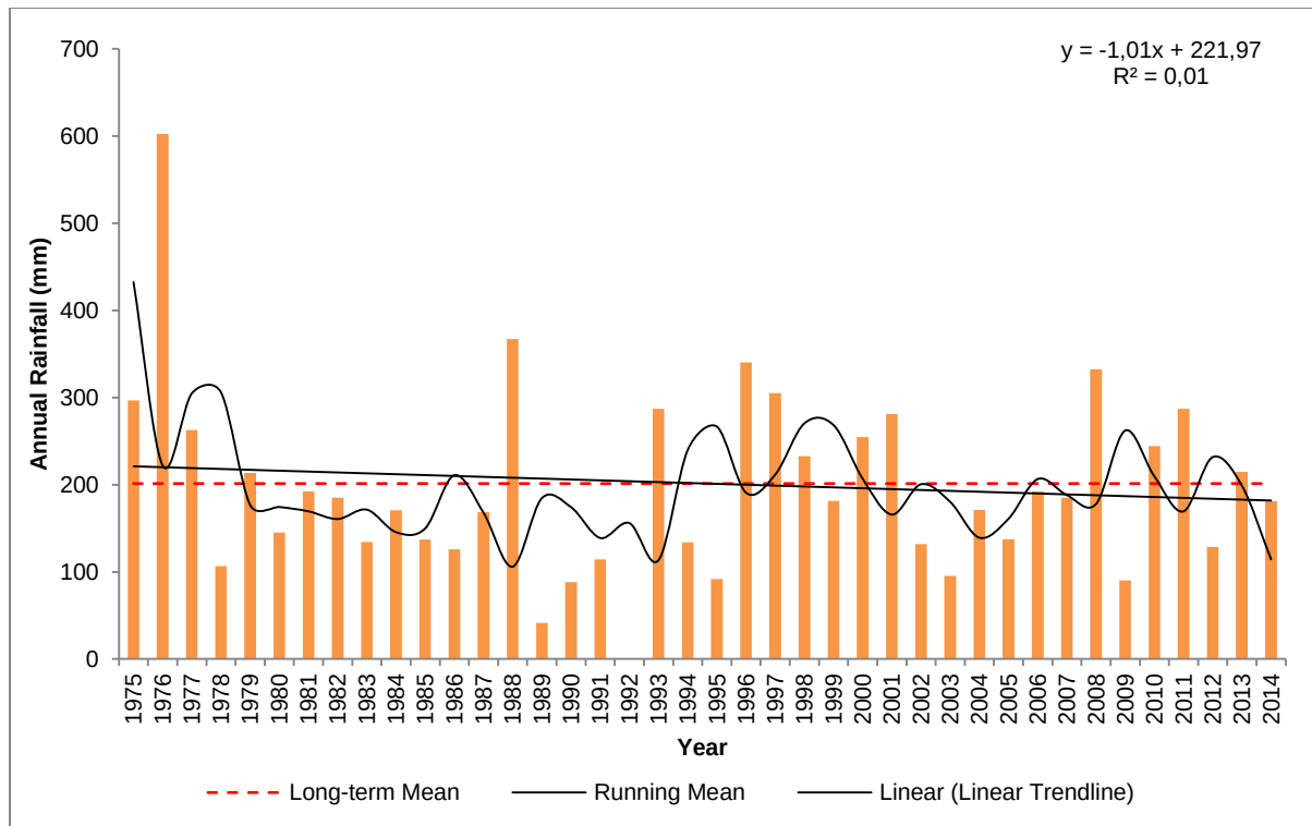
Figure 5.3: Long-term rainfall trends for Nossob: 1975 – 2014.
