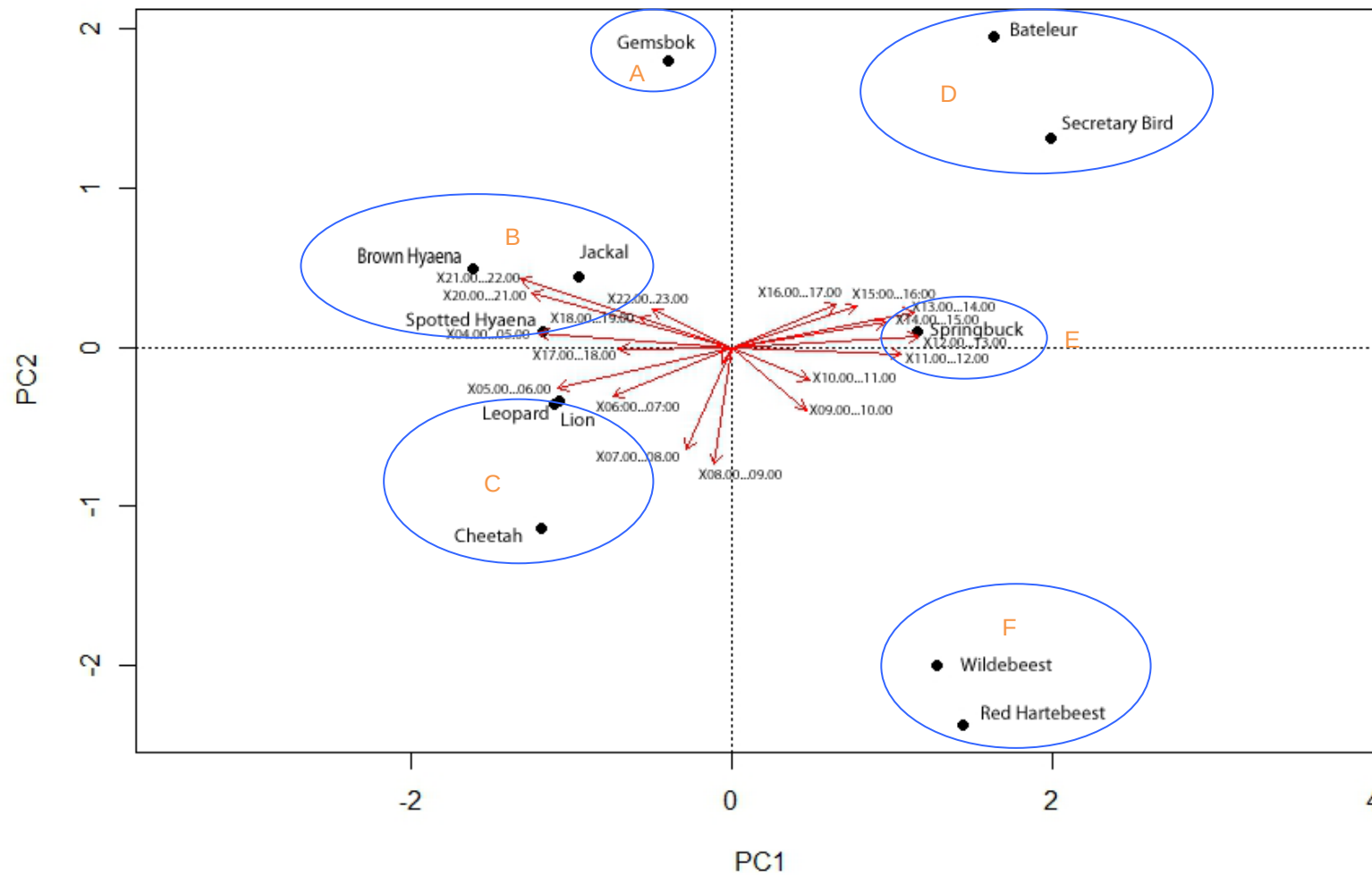
Figure 5.21: PCA analysis demonstrating the time vectors, which drive individual species water trough usage.
