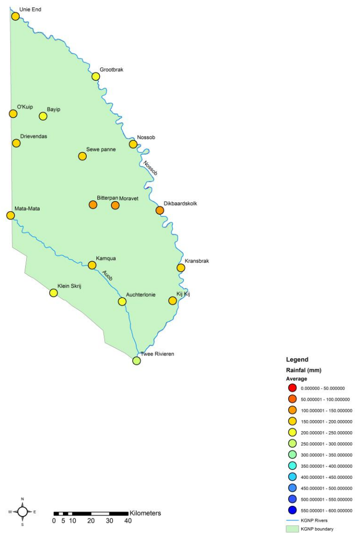
Figure 6.2: Average rainfall variability (mm) across KGNP for the period 2004-2013.
