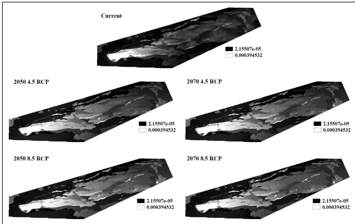
Figure C9: Suitability maps derived from Maxent for T. margaritifer . Future projections are mean ensemble maps from HadGEM2-CC, MIRCP5 and GISS-E2-R circulation models. Lighter colour indicated higher suitability.
