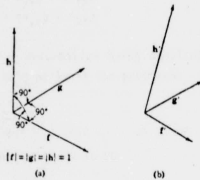
Fig. 2.1 Coordinate axes for the description of the state of strain; the orthogonal unit axes in the unstrained state (a) are deformed in the strained state (b)
