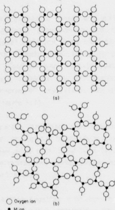
Fig. 1.1 Two-dimensional representation of an oxide M_2O_3 in (a) the crystalline form (b) the glassy form (after McMillan, 1979)
