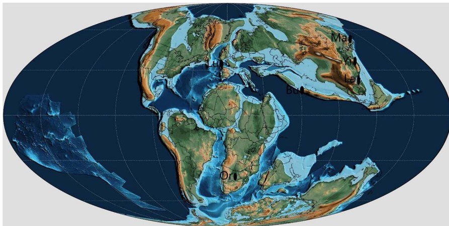
Fig. 5. Global palaeogeographic reconstruction of the mid-Cretaceous (100 Ma) showing the localities where the fossil Staphylininae have been recovered. The map in Mollweide projection was sourced from Scotese (2016, 2021; Appendix 2, Mollweide Maps.zip). The position of the localities was adapted from Rasnitsyn and Quicke (2002). Abbreviations: Bu = Burmese amber, Myanmar; La = Laiyang Formation, China; Or = Orapa Diamond Mine, Botswana; Yi = Yixian Formation, China; Ma = Magadanskaia, Russia and Lu = Lulworth Formation, Middle Purbeck.
