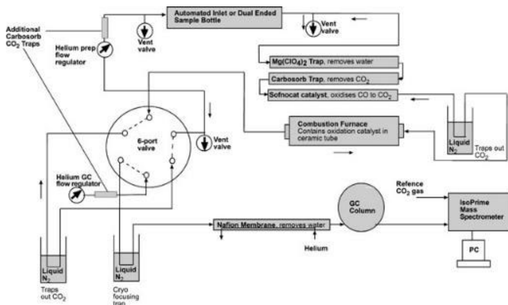
Figure 16: Diagram of the sampling equipment for CH 4 analysis set-up at RHUL. Reproduced from Fisher et al. (2006).
