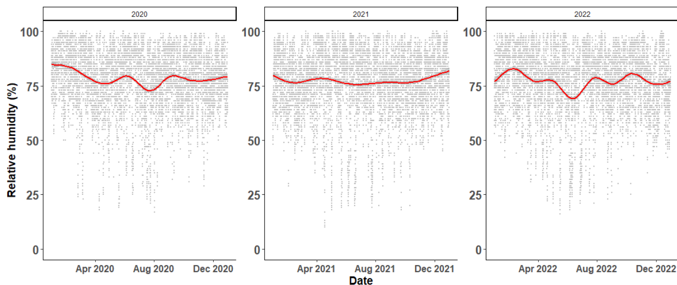
Figure 39: Seasonal/monthly relative humidity (%) patterns at Cape Point GAW station, South Africa.
