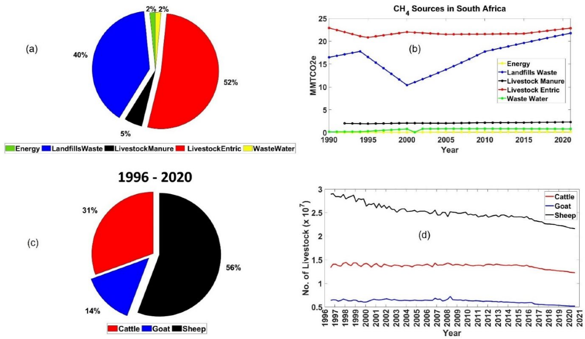
Figure 3: Sources of CH 4 by sector in South Africa (Shikwambana et al. (2022)).
