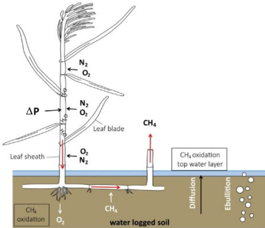
Figure 40: Diagram illustrating humidity-induced convection in Phragmites plants (van den Berg et al. , 2020). N_2 and O_2 move through stomata in the leaf sheath, driven by the diffusion gradient. Living plants generate higher pressure in the stem ( \Delta P ), causing airflow towards the rhizome, venting through old and damaged stems (red arrows). O_2 is conveyed to the soil, while CH_4 diffusing into the rhizome is transported to the atmosphere. Where O_2 and CH_4 coexist, CH_4 oxidation takes place.
