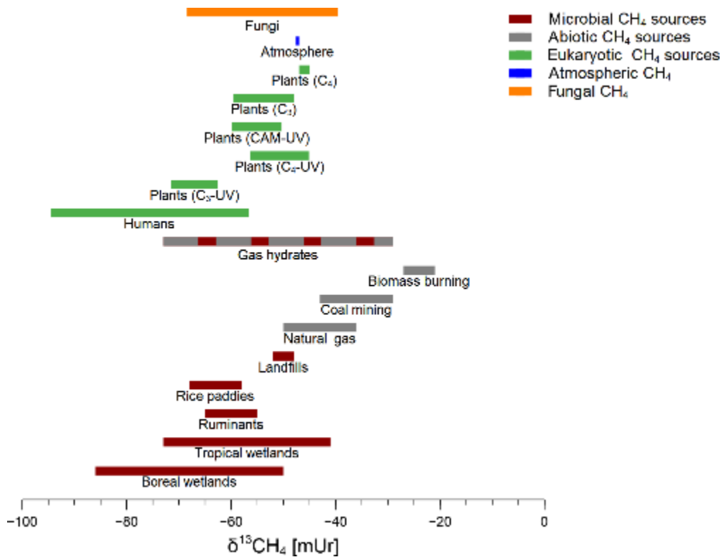
Figure 4: The range of \delta^{13}\text{CH}_4 values for various sources of methane, including microbial (red), abiotic (grey), eukaryotic (green), atmospheric (blue), and fungal (orange) origins, is presented based on findings by Schroll et al. (2020). The combination of microbial and abiotic methane formation processes for gas hydrates is indicated by the red and grey dashed bars, referring to Kvenvolden (1995). Data regarding these signatures were compiled from studies by Brownlow et al. (2017), Keppler et al. (2006, 2016), Kvenvolden (1995), Nisbet et al. (2016), Quay et al. (1999), and Vigano et al. (2009).
