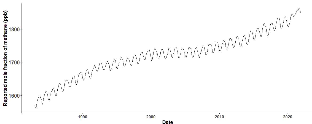
Figure 35: Reported mole fraction of methane (ppb) for each year at Cape Point for the years 1983 – 2021.
