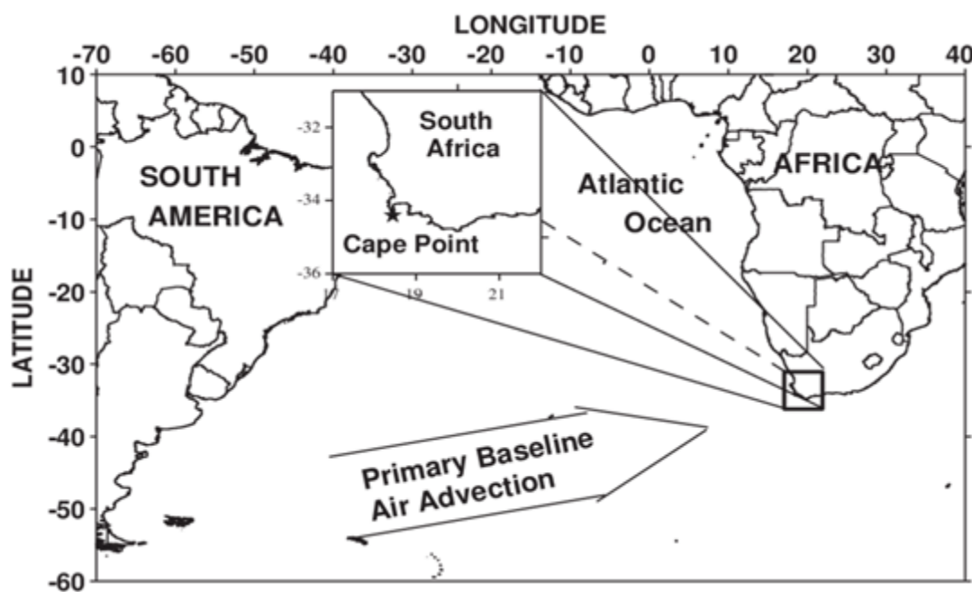
Figure 20: Map showing the location of the Cape Point GAW station (Labuschagne et al. , 2018).
