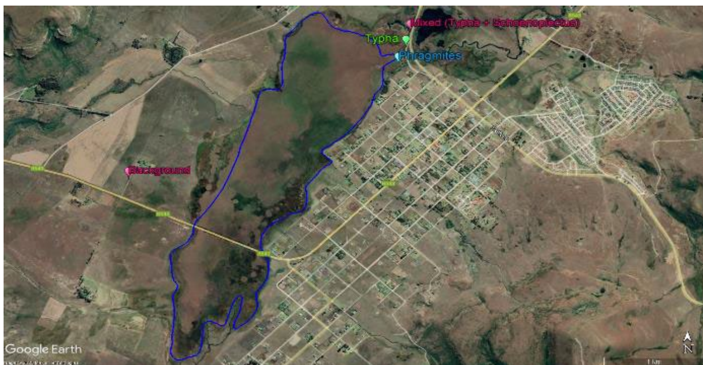
Figure 12: Google Earth image of the location of where the samples were collected for the vegetation communities along the Wakkerstroom wetland in Mpumalanga province, South Africa
