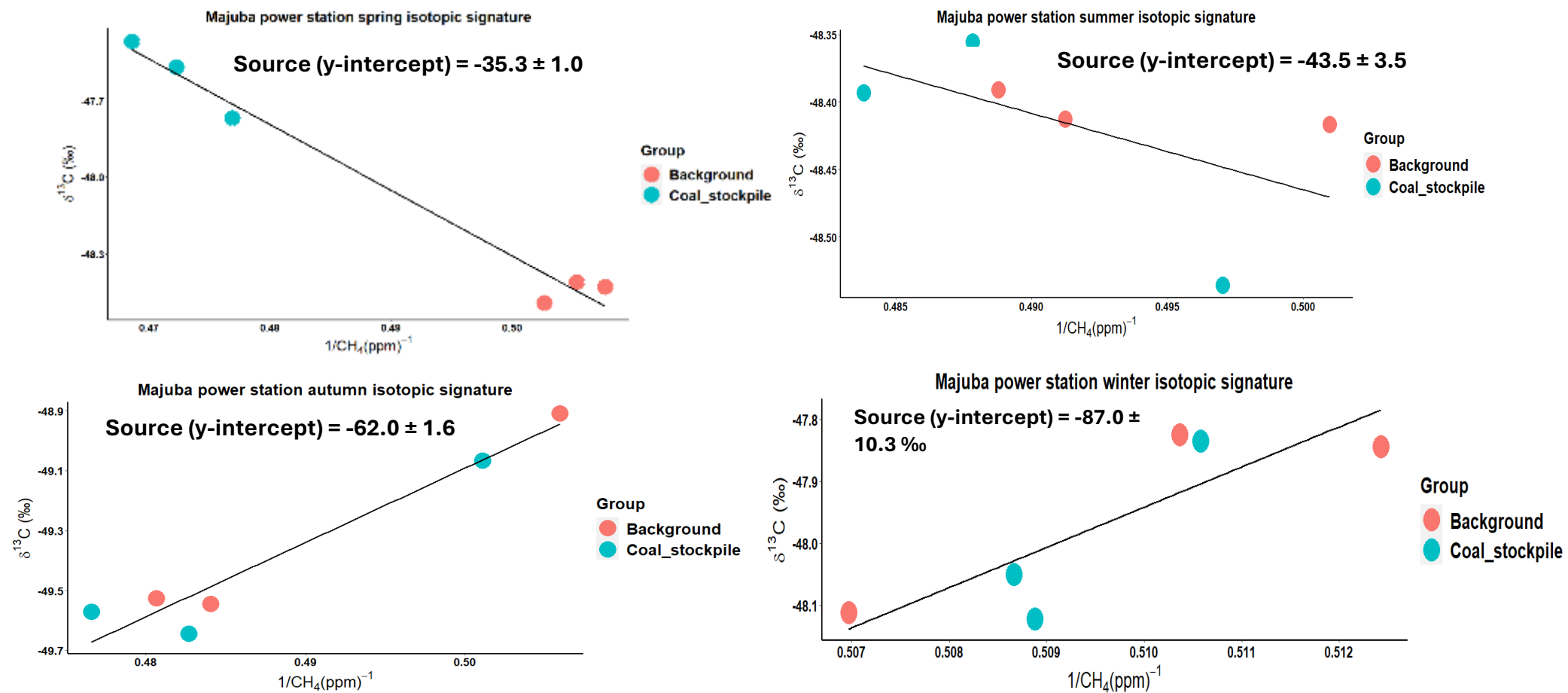
Figure 24: Keeling plots representing the carbon isotopic source signatures of the Majuba power station in the spring, summer, autumn, and winter seasons.
