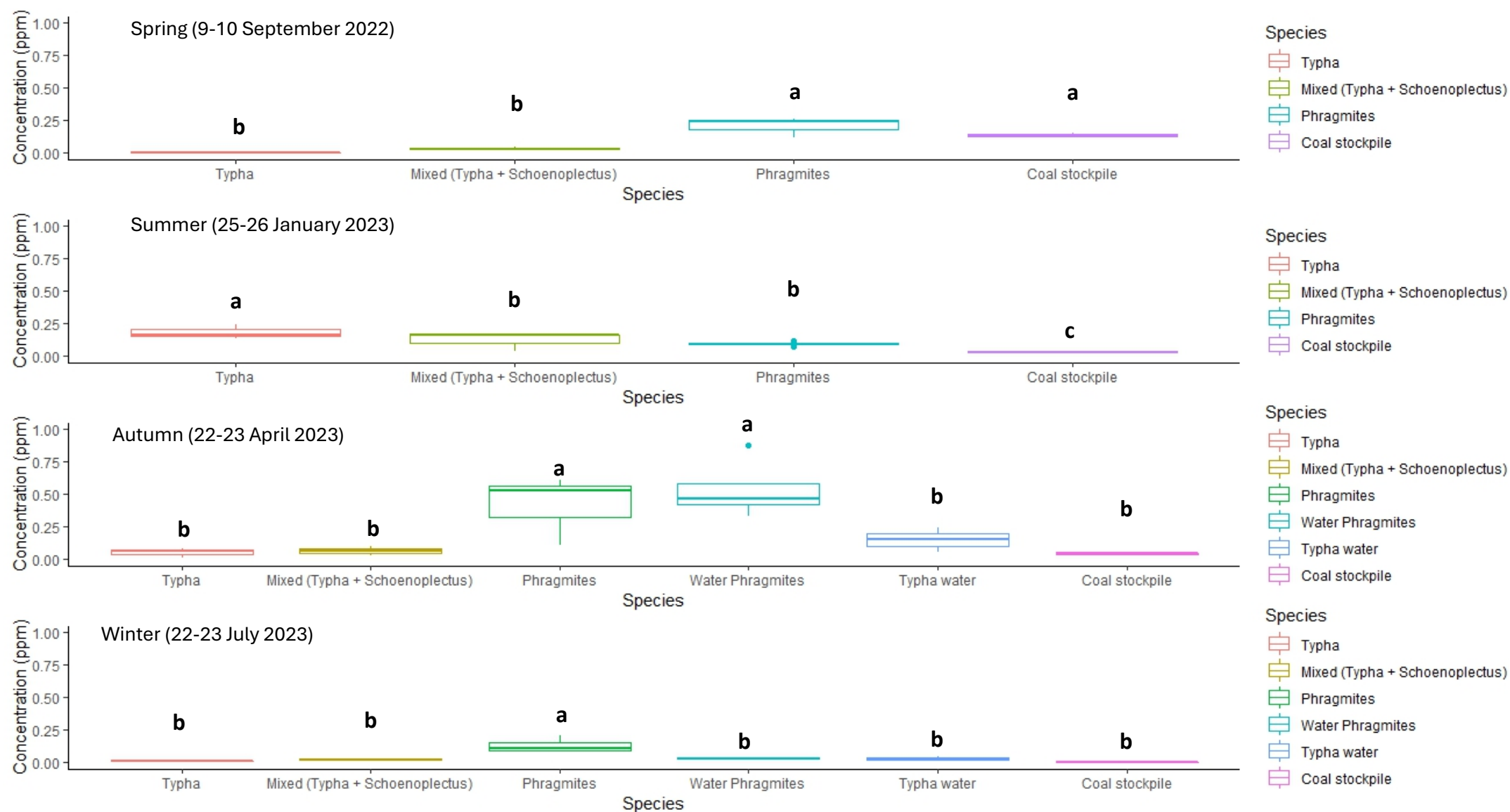
Figure 22: Concentration (ppm) measurements collected from various plant communities at the Wakkerstroom wetland and coal stockpiles at the Majuba power station in the spring (9-10 September 2022), summer (25-26 January 2023), autumn (22-23 April 2023) and winter(22-23 July 2023)
