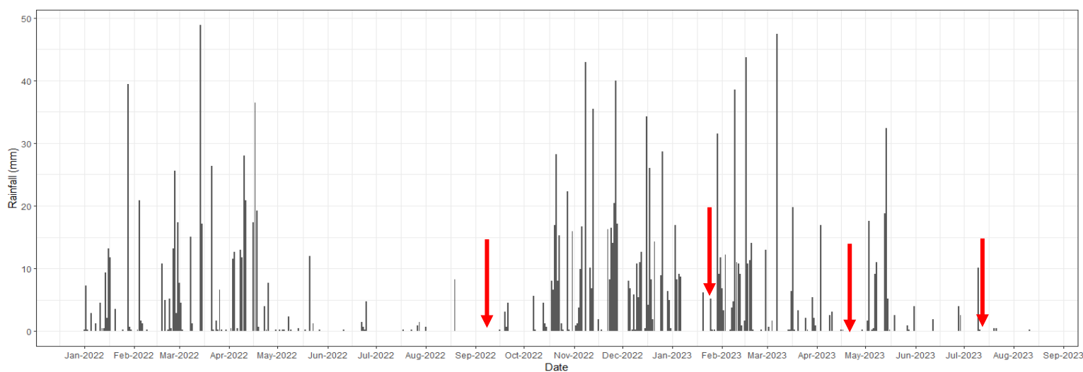
Figure 27: Seasonal rainfall pattern at Wakkerstroom, Mpumalanga from January 2022-August 2023 with red arrows indicating field sampling days in each season.
