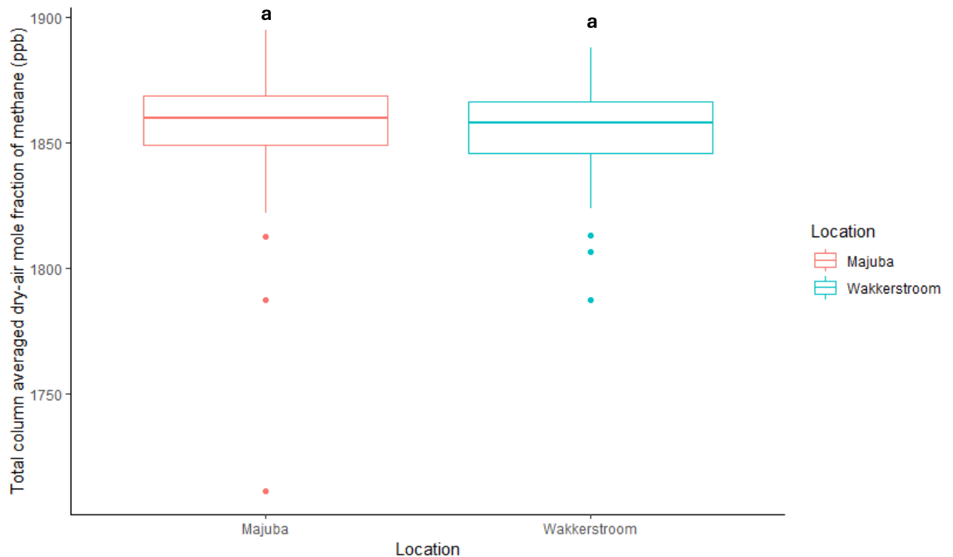
Figure 29: Boxplot showing the total column averaged dry-air mole fraction of methane at Wakkerstroom and Majuba power station in Mpumalanga province, South Africa as measured using TROPOMI.
