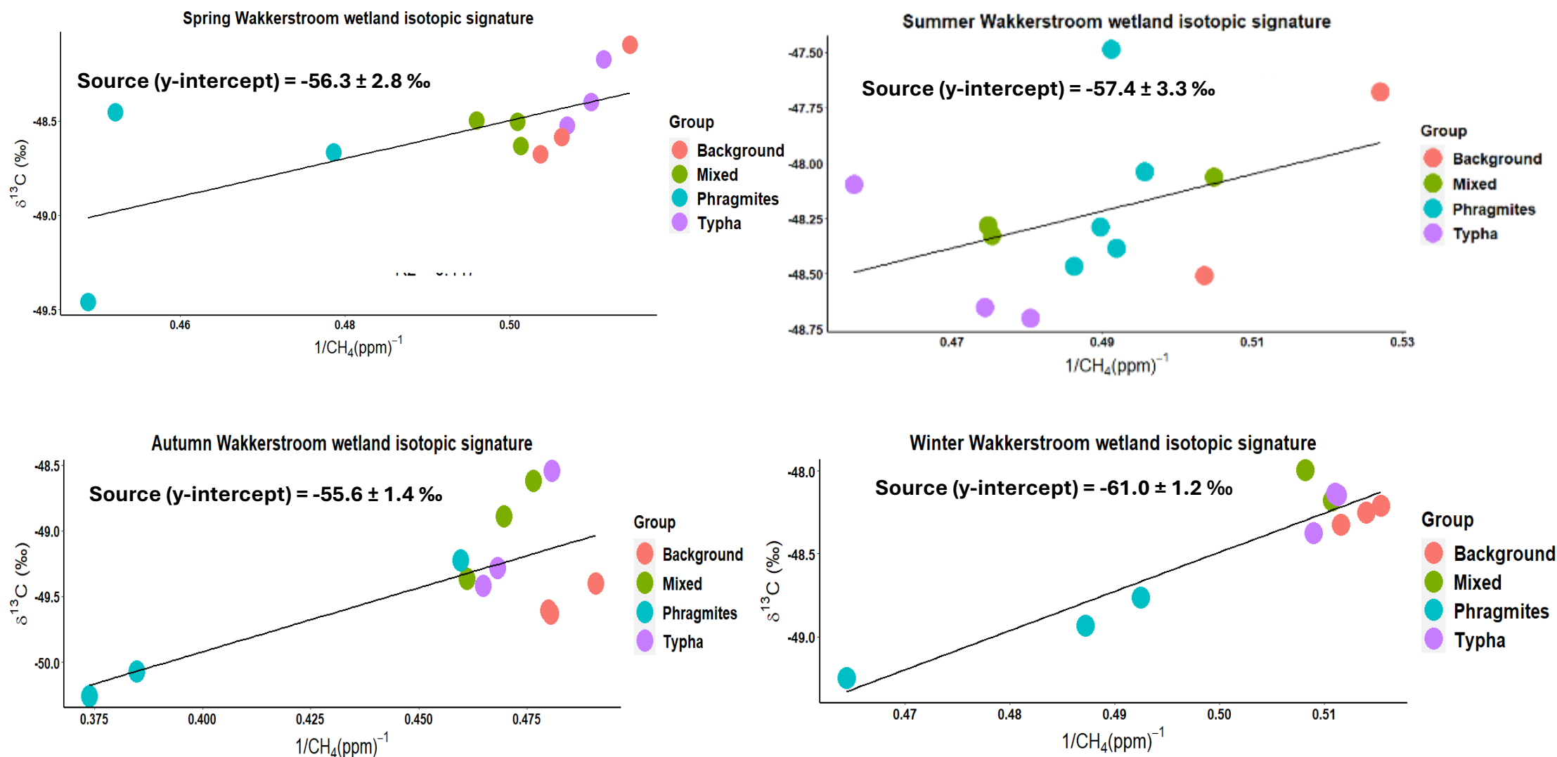
Figure 23: Keeling plots representing the source carbon isotopic source signatures of the Wakkerstroom wetland in the spring, summer, autumn, and winter seasons.
