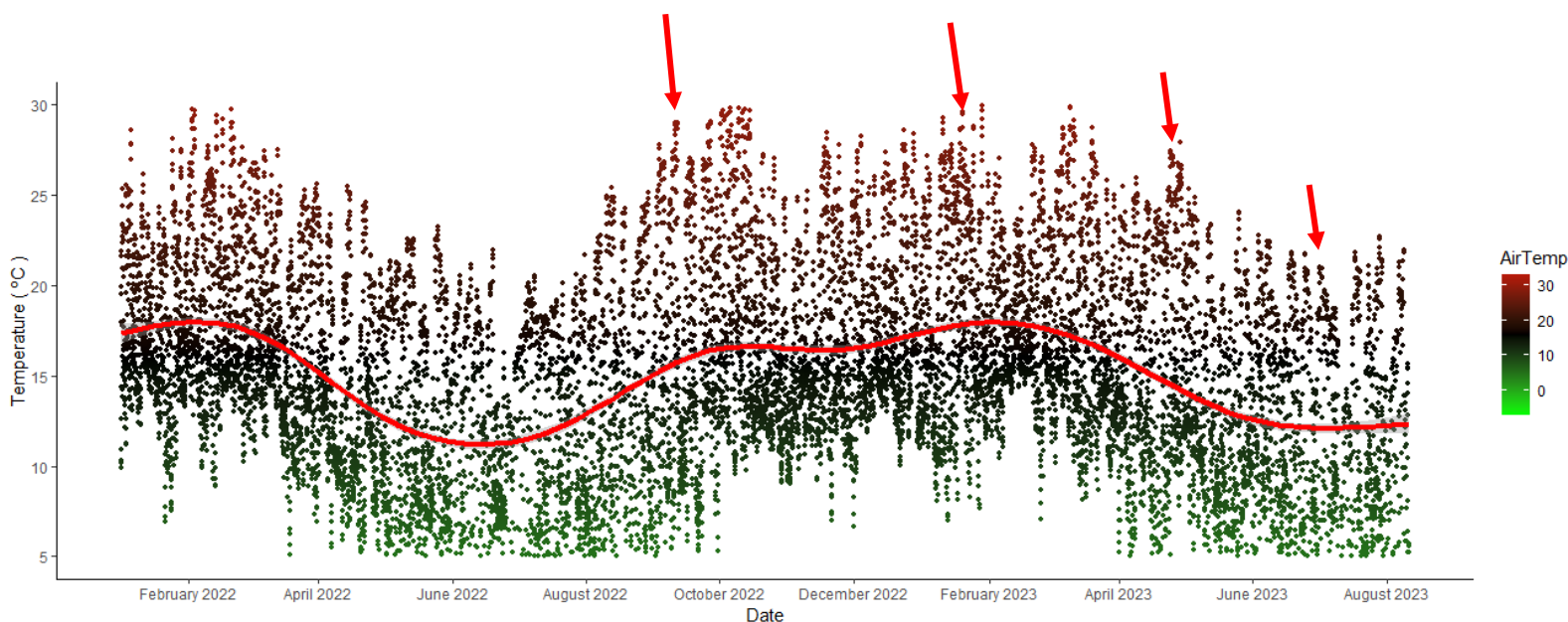
Figure 26: Seasonal temperature pattern (°C) at Wakkerstroom, Mpumalanga on January 2022 – August 2023 with red arrows indicating field sampling days in each season.
