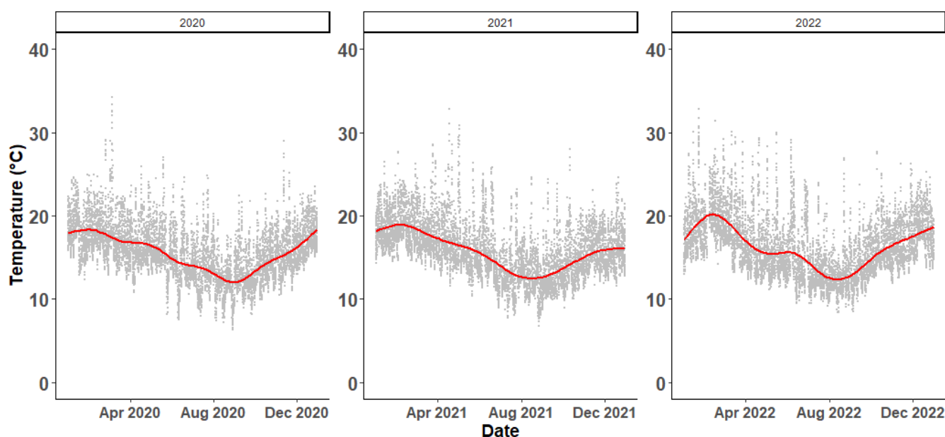
Figure 38: Seasonal air temperature graph for the Cape Point GAW station in Cape Town, South Africa for the years 2020 - 2022.
