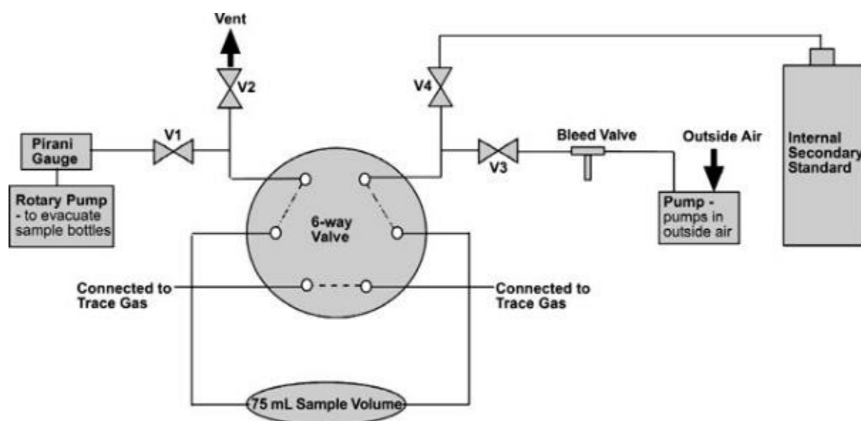
Figure 17: Diagram of the sampling equipment for CH 4 analysis set-up at RHUL. Reproduced from Fisher et al. (2006).
