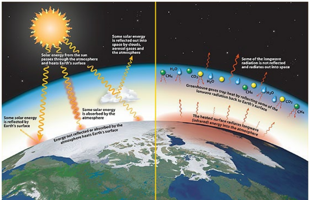
Figure 1: Diagram illustrating the greenhouse effect. Image from: https://forces.si.edu/atmosphere/02_04_07.html
