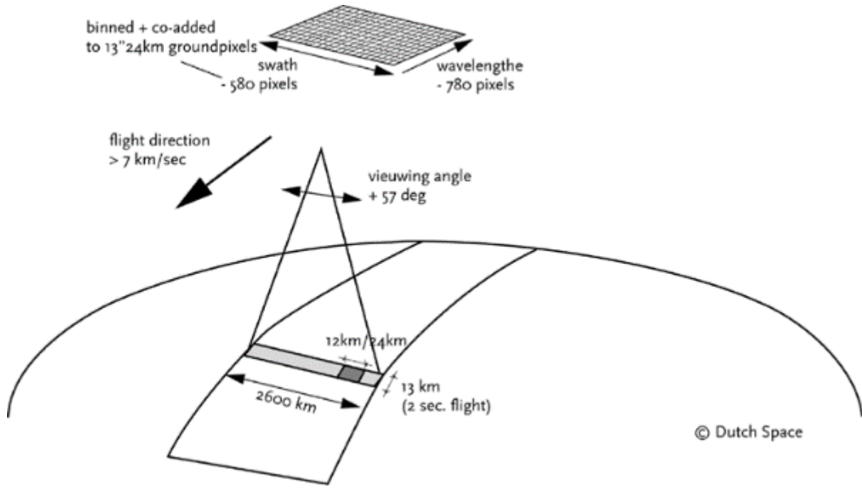
Figure 19: TROPOMI measurement principle (Apituley et al. , 2022).
