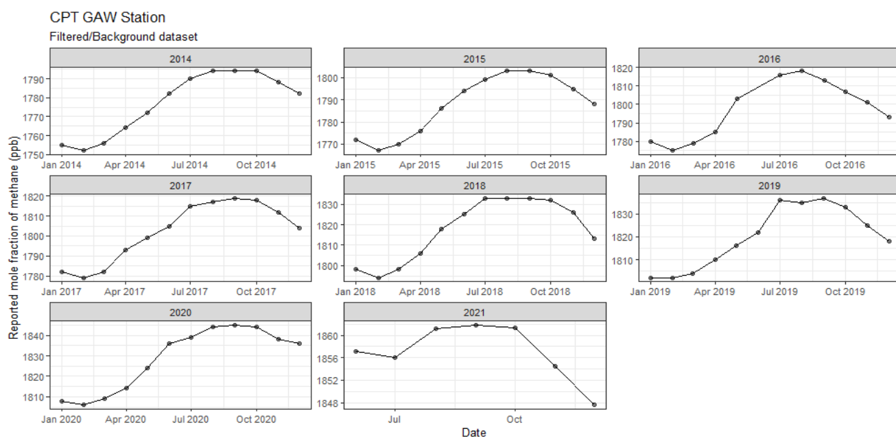
Figure 34: Mean monthly reported mole fraction of CH 4 at Cape Point GAW station during 2014-2021.
