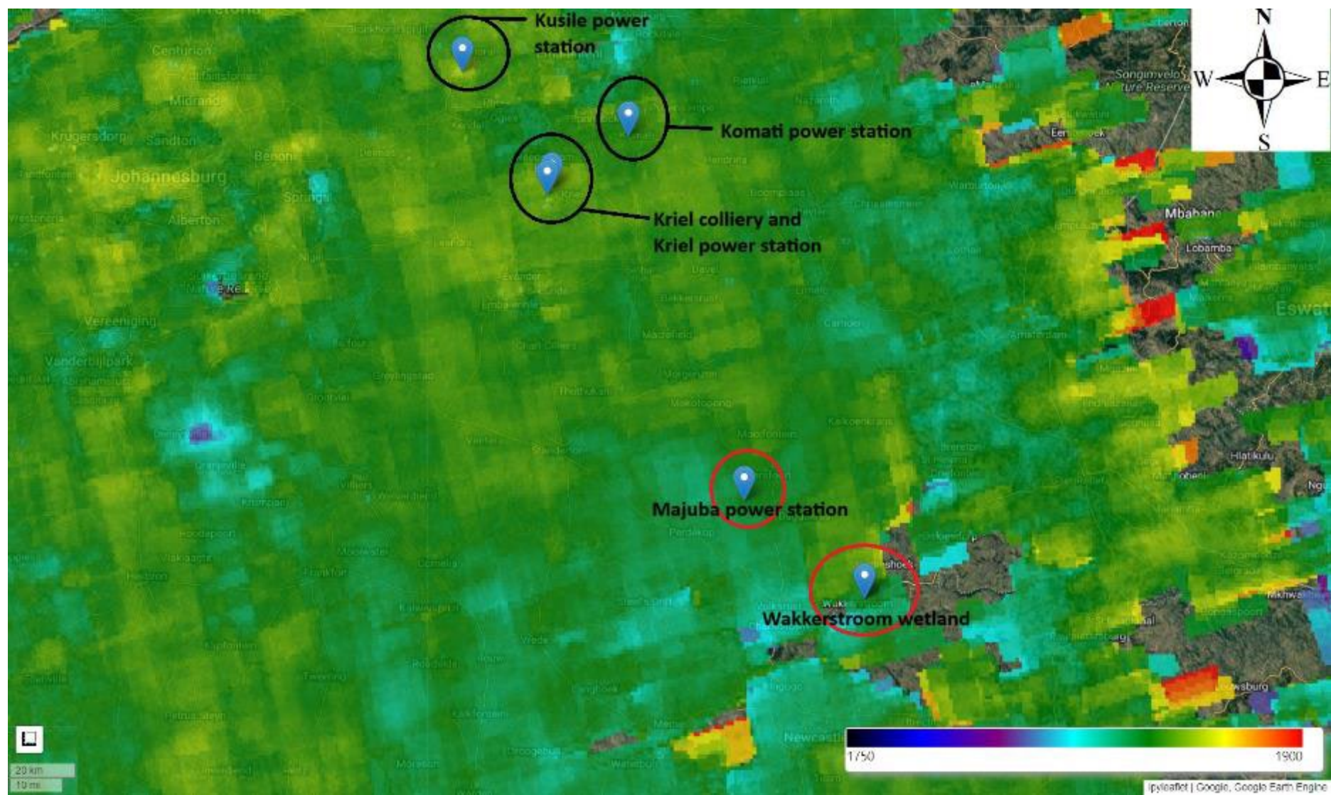
Figure 32: Map produced from TROPOMI total column averaged dry-air mole fraction of methane product (autumn 2023).
