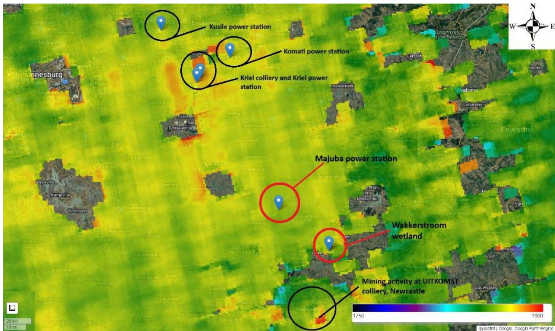
30: Map produced from TROPOMI total column averaged dry-air mole fraction of methane product (spring 2022).
