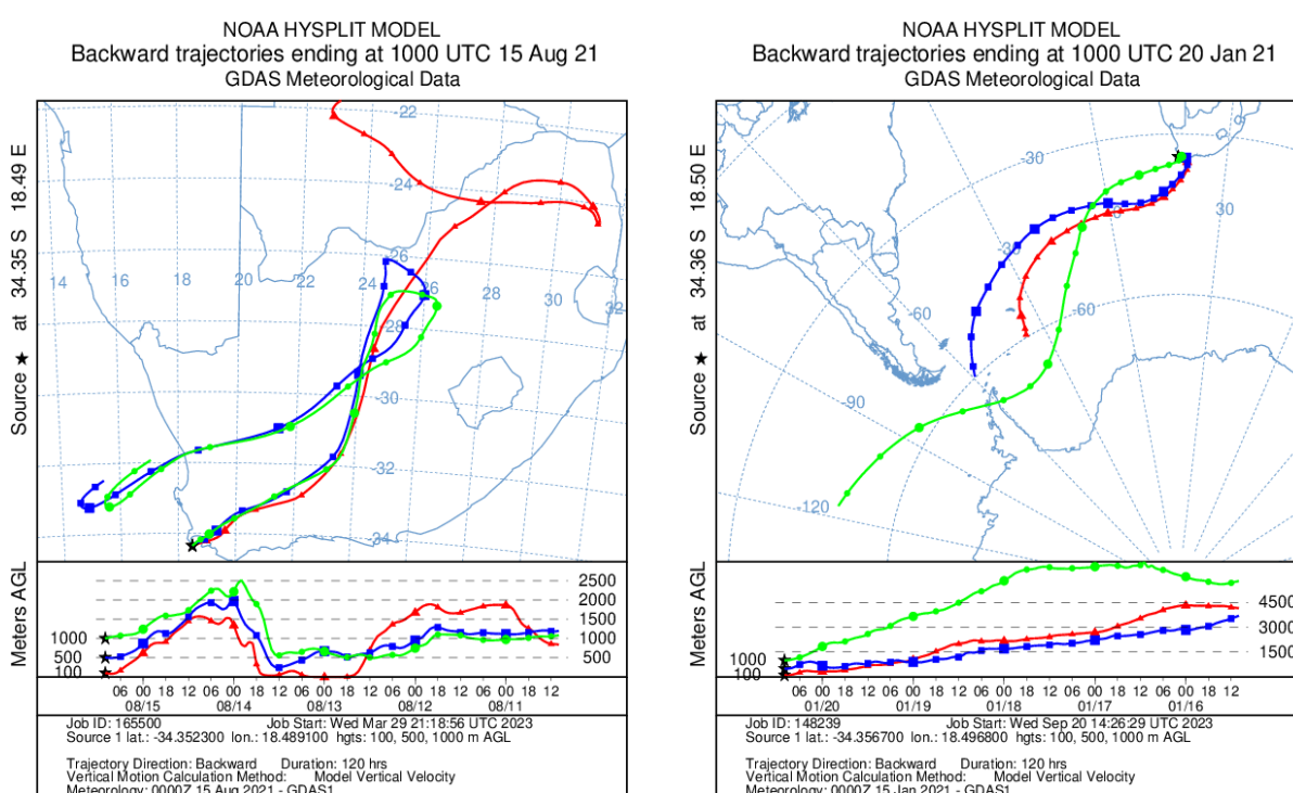
Figure 37: HYSPLIT backward trajectory analysis for the summer (20 January 2021) and winter (15 August 2021) representative days at Cape Point, South Africa.
