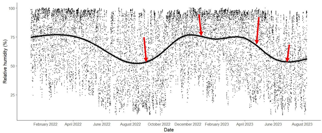
Figure 28: Relative humidity (%) at Wakkerstroom, Mpumalanga from January 2022-August 2023 with red arrows indicating field sampling days in each season.
