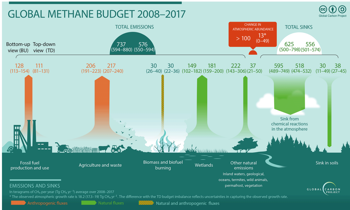
Figure 2: The global methane budget, 2008–2017, the emission range is indicated by the numbers in parenthesis, and the numbers on the left and right represent bottom-down and top-down estimations (Saunois et al. (2020)).
