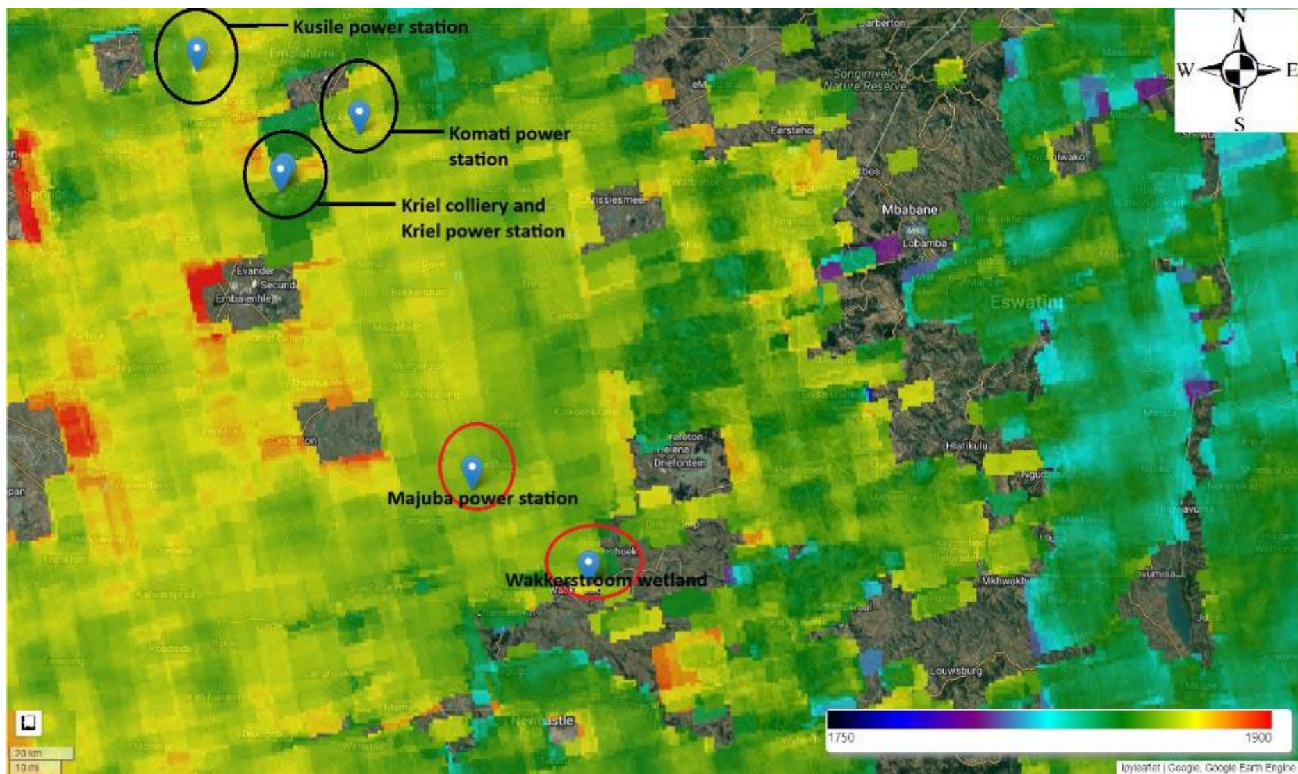
Figure 31: Map produced from TROPOMI total column averaged dry-air mole fraction of methane product (summer 2023).
