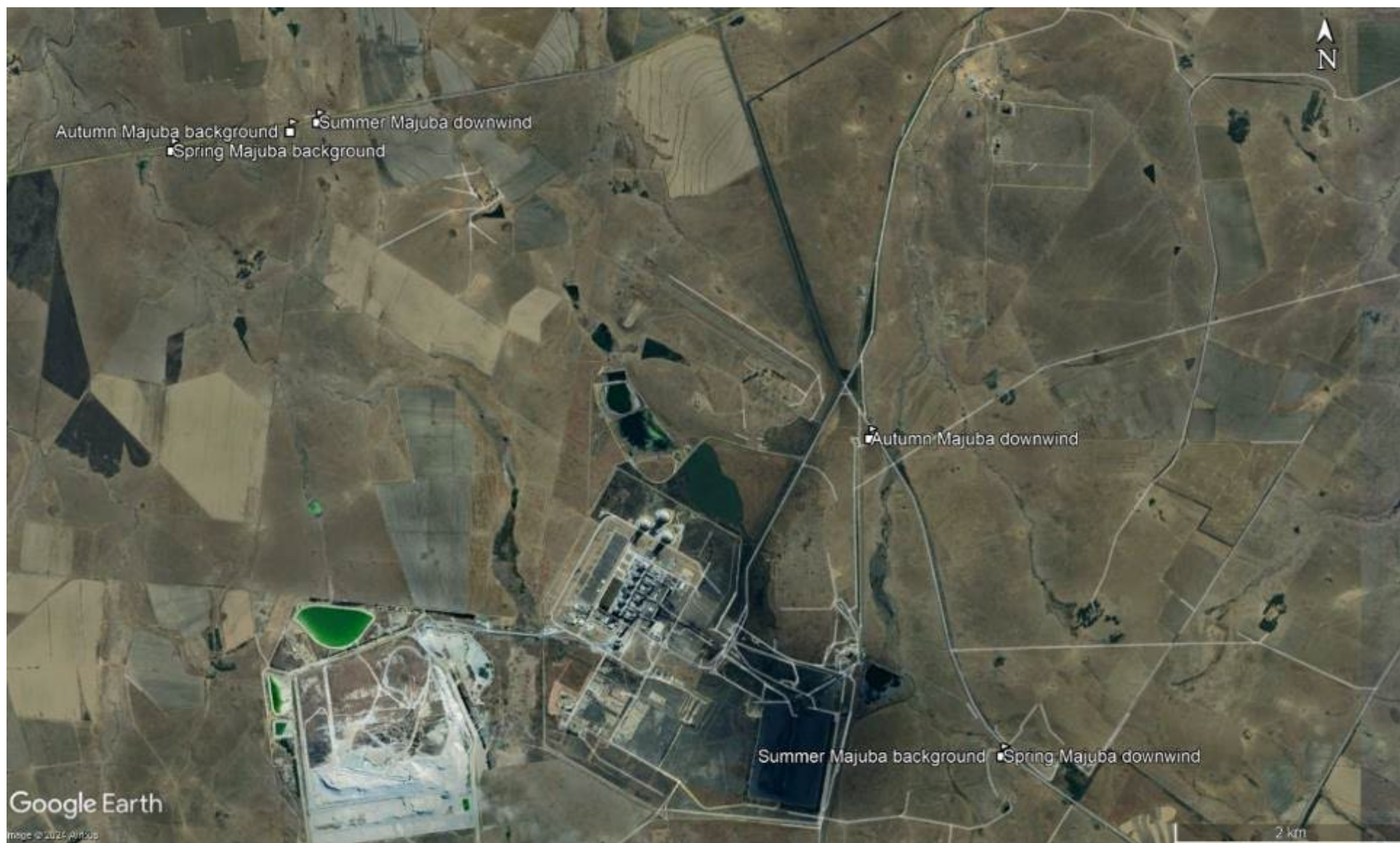
Figure 13: Location of the samples collected at Majuba power station in Mpumalanga province, South Africa.
