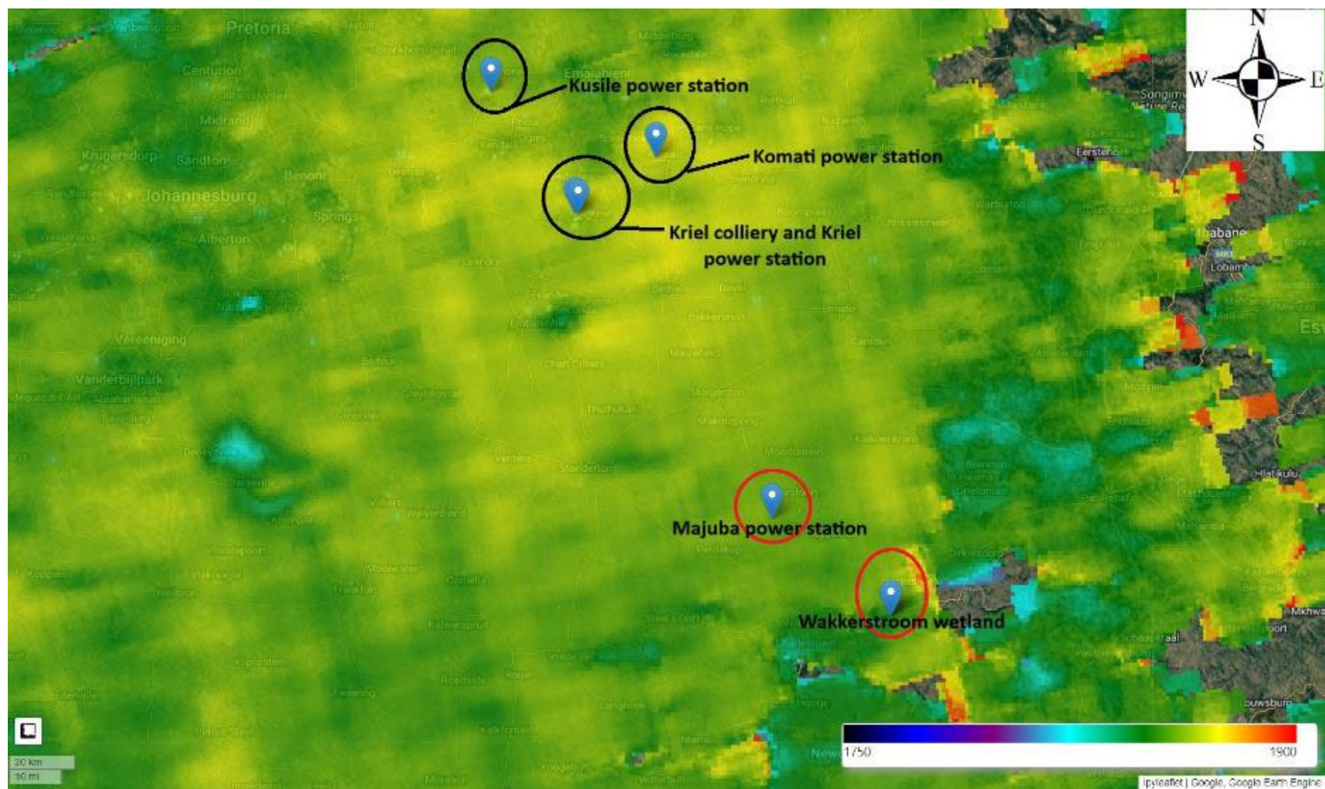
Figure 33: Map produced from TROPOMI total column averaged dry-air mole fraction of methane product (winter 2022).
