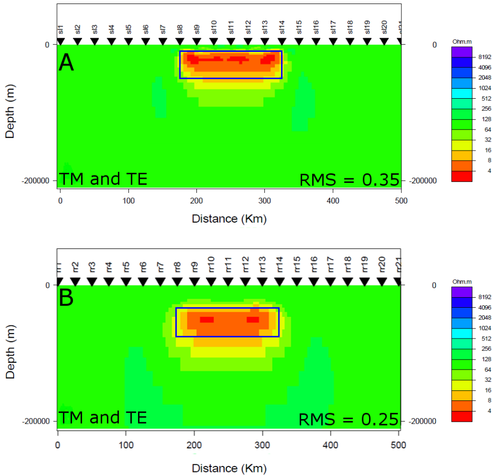
Figure 6.5: Resistivity models obtained by inversion of MT responses calculated with forward modelling, where the forward models consisted of conductive 5 \Omega.m boxes (outline shown), one with its top margin at 10 km depth (a) and the other 35 km depth (b), embedded in a homogeneous 100 \Omega.m half-space. Standard grid Laplacian regularization was selected for both inversions and the same weighting factors of; \alpha = 1 , \beta = 1.5 , H = 500 m and V = 500 m and \tau = 3 , were used.
