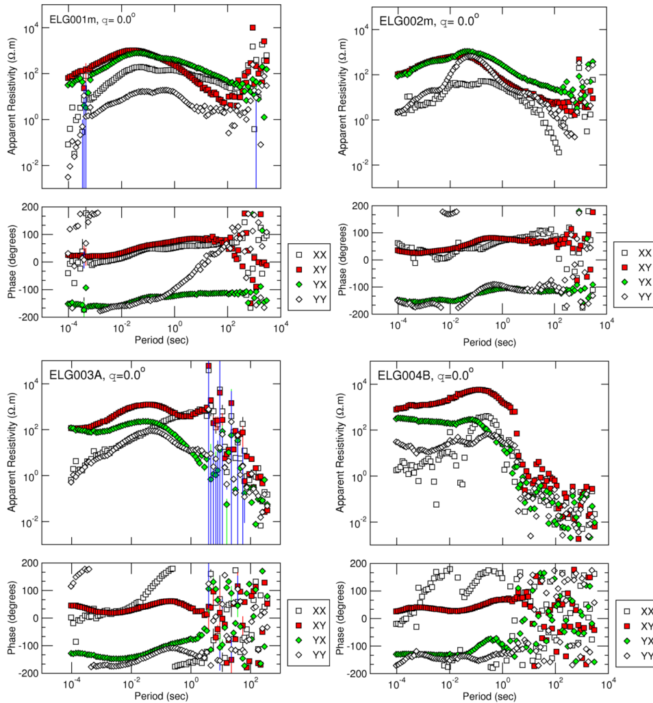
Figure B.1: MT apparent resistivity and phase curves, rotated to true north and not decomposed, for sites ELG001m, ELG002m, ELG003A and ELG004B. Sites ELG001m and ELG002m consist of merged (m) AMT and BBMT data.
