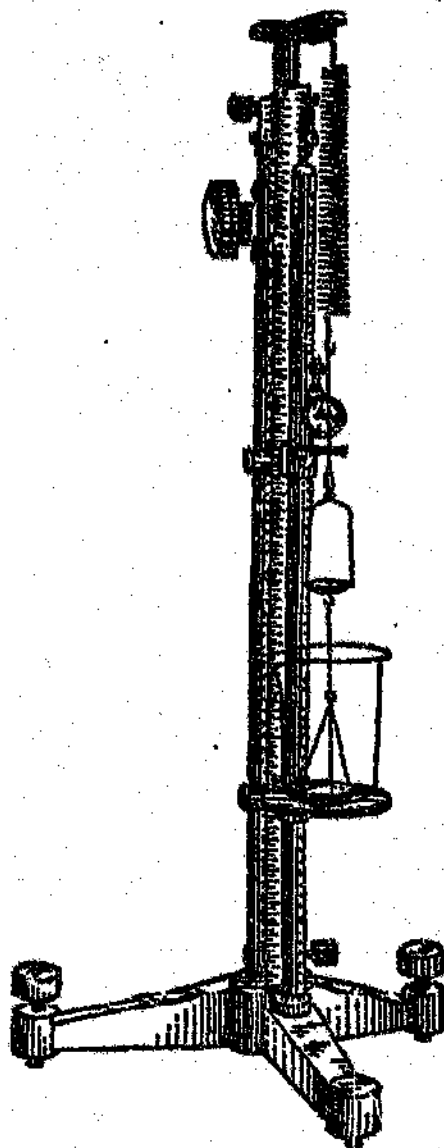
Figure 3.1 Sketch of a Jolly balance used to measure the specific gravity of samples (after Klein et al., 1985).
