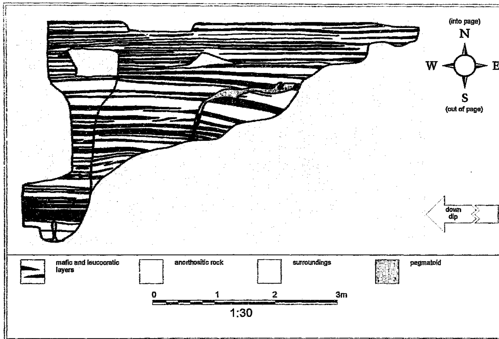
Figure 2.10 Map of the accessible portion of the vertical exposure of the Layered Marker Sequence as exposed at locality E.
