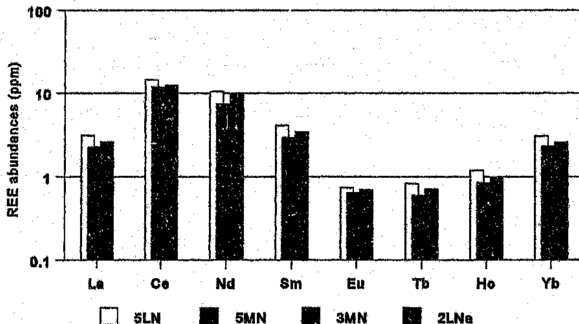
Figure 9.4 Concentration of REE's in clinopyroxene separates from the Layered Marker Sequence.
