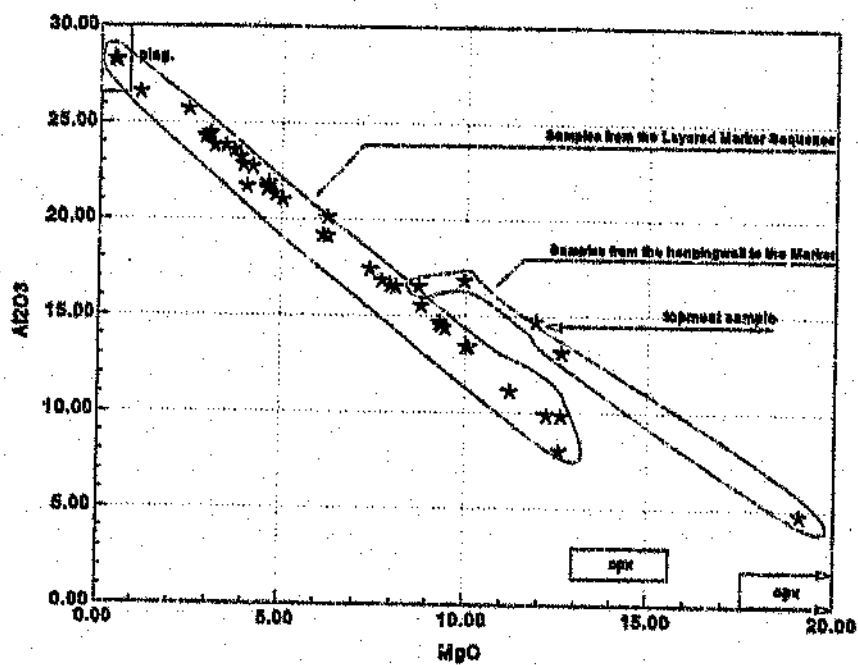
Figure 8.4 Variation of \text{Al}_2\text{O}_3 abundance with \text{MgO} .
