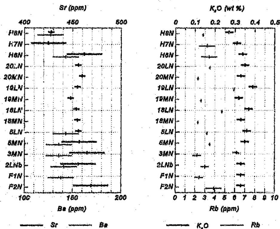
Figure 9.8 Variation in Ba, Rb, Sr and K_2O in selected plagioclase separates from profile A. Samples are in stratigraphic order but not to scale.
