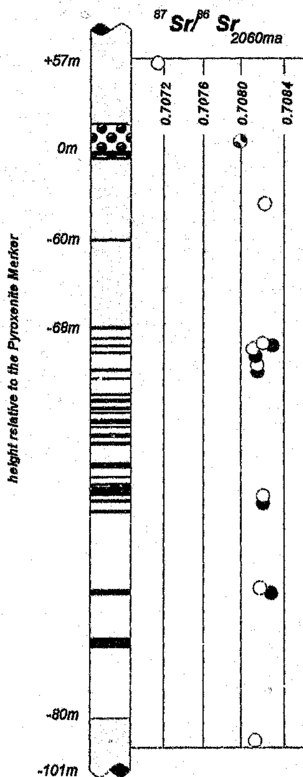
Figure 9.7 Vertical variation in the initial Sr-isotopic ratio. The symbol width reflects the approximate magnitude of analytical precision. Stippled-mafic; open-leucocratic; pale stipple-unlayered.
