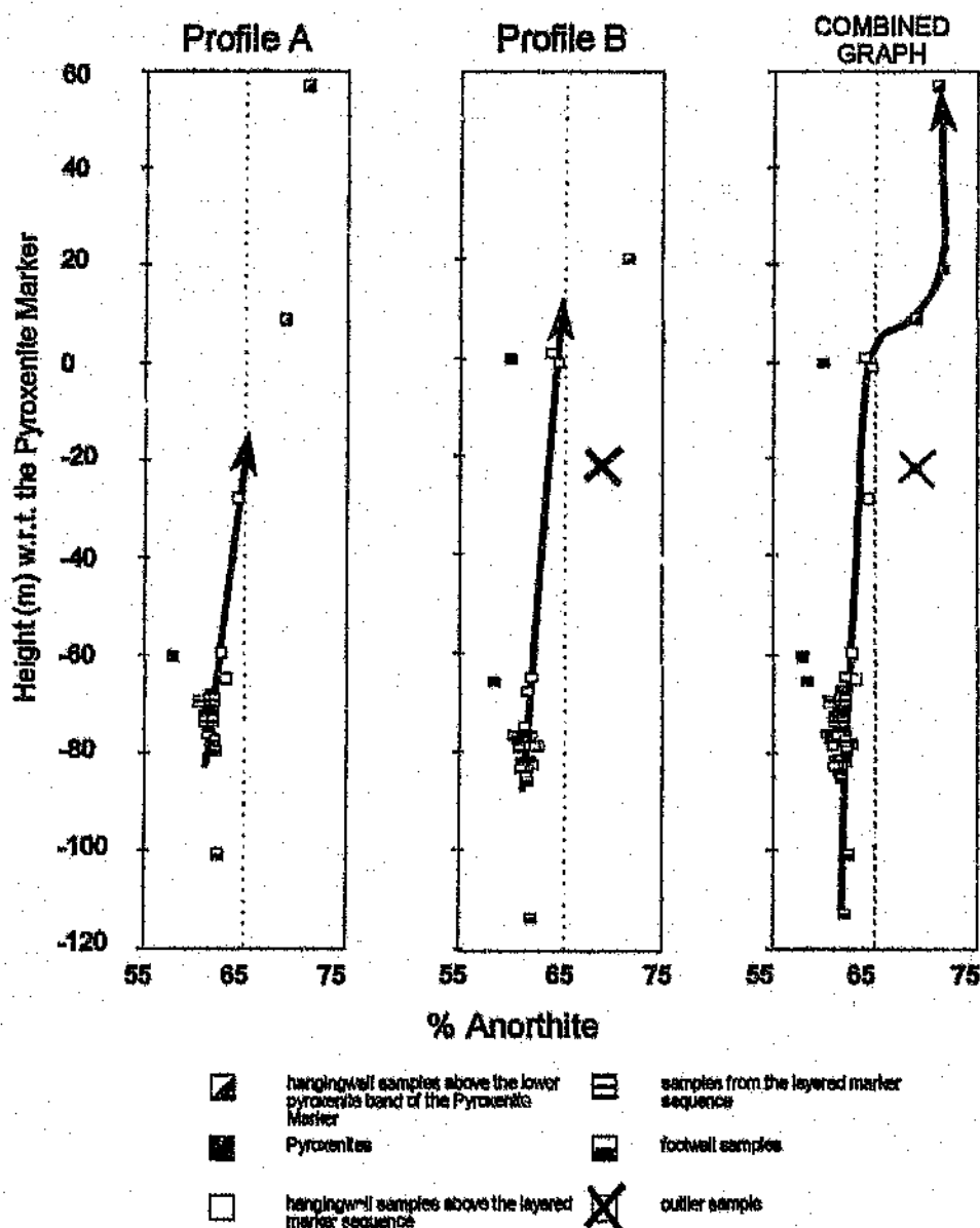
Figure 6.3 Variation in plagioclase compositions (An(2)) across the Layered Marker up to and including the Pyroxenite Marker.
