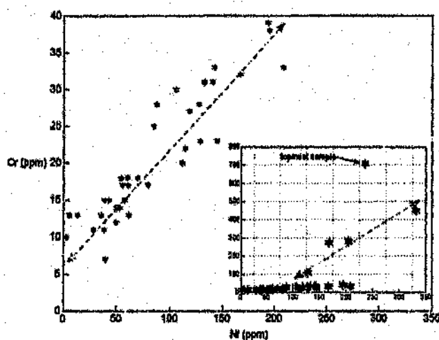
Figure 8.8 Plot of Ni versus Cr. Data points in the main graph are for samples from the layered interval. Additional sample points plotted in the inserted graph reflect the composition of hangingwall samples.
