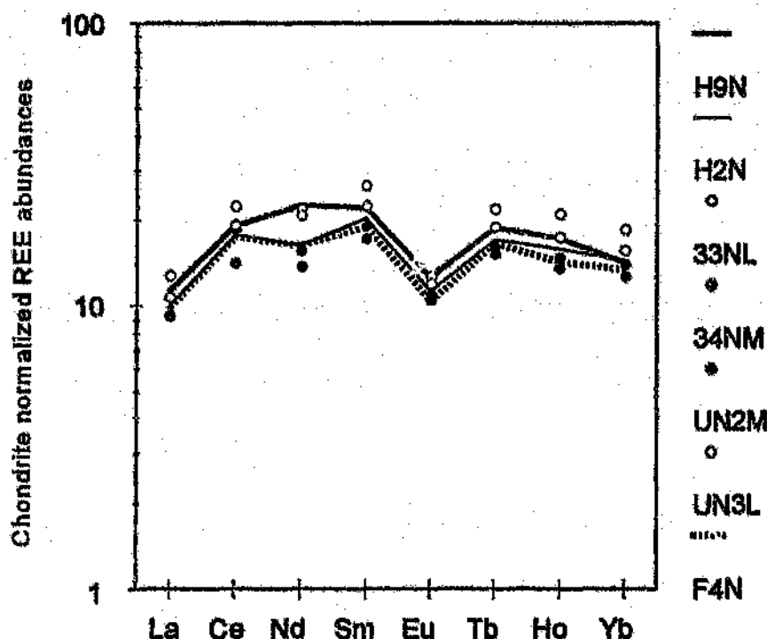
Figure 9.1 Chondrite normalized rare earth element abundances (Evenson, 1978) in clinopyroxene separates from profile A.
