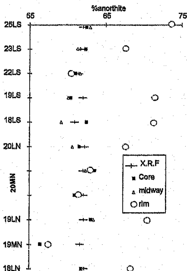
Figure 6.5 Comparison of plagioclase compositions as determined from XRF and microprobe analyses (An(2)).
