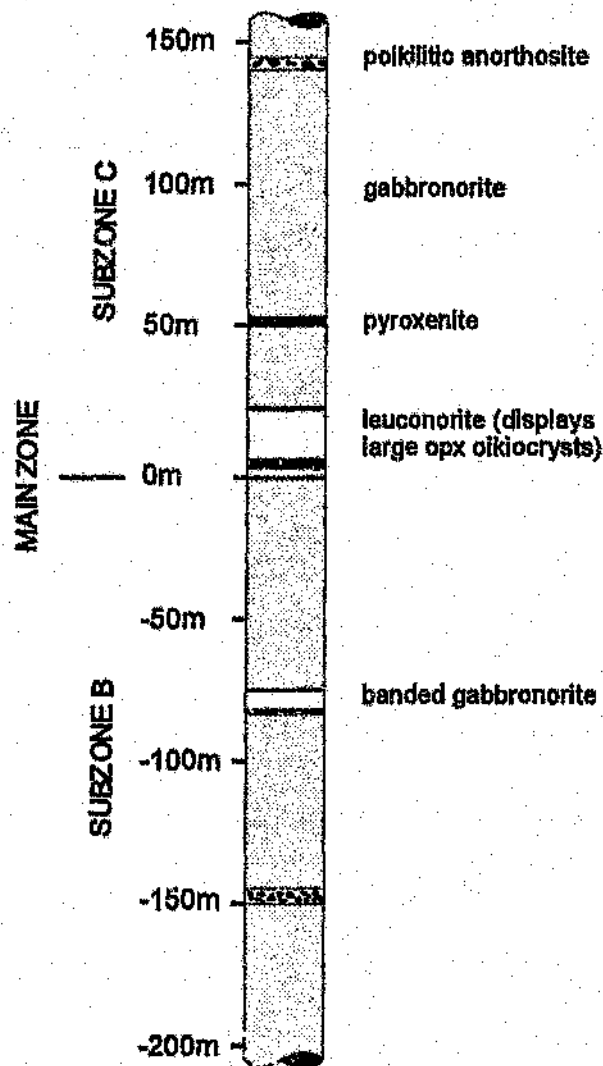
Figure 1.2 Stratigraphic position of the Layered Marker Sequence within the Main Zone of the Bushveld Complex.
