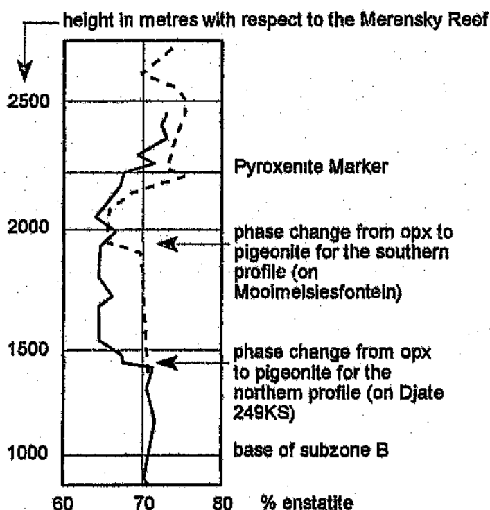
Figure 7.1 Variation in the composition of orthopyroxene, measured microscopically, across the Pyroxenite Marker (from Molyneux, 1974).
