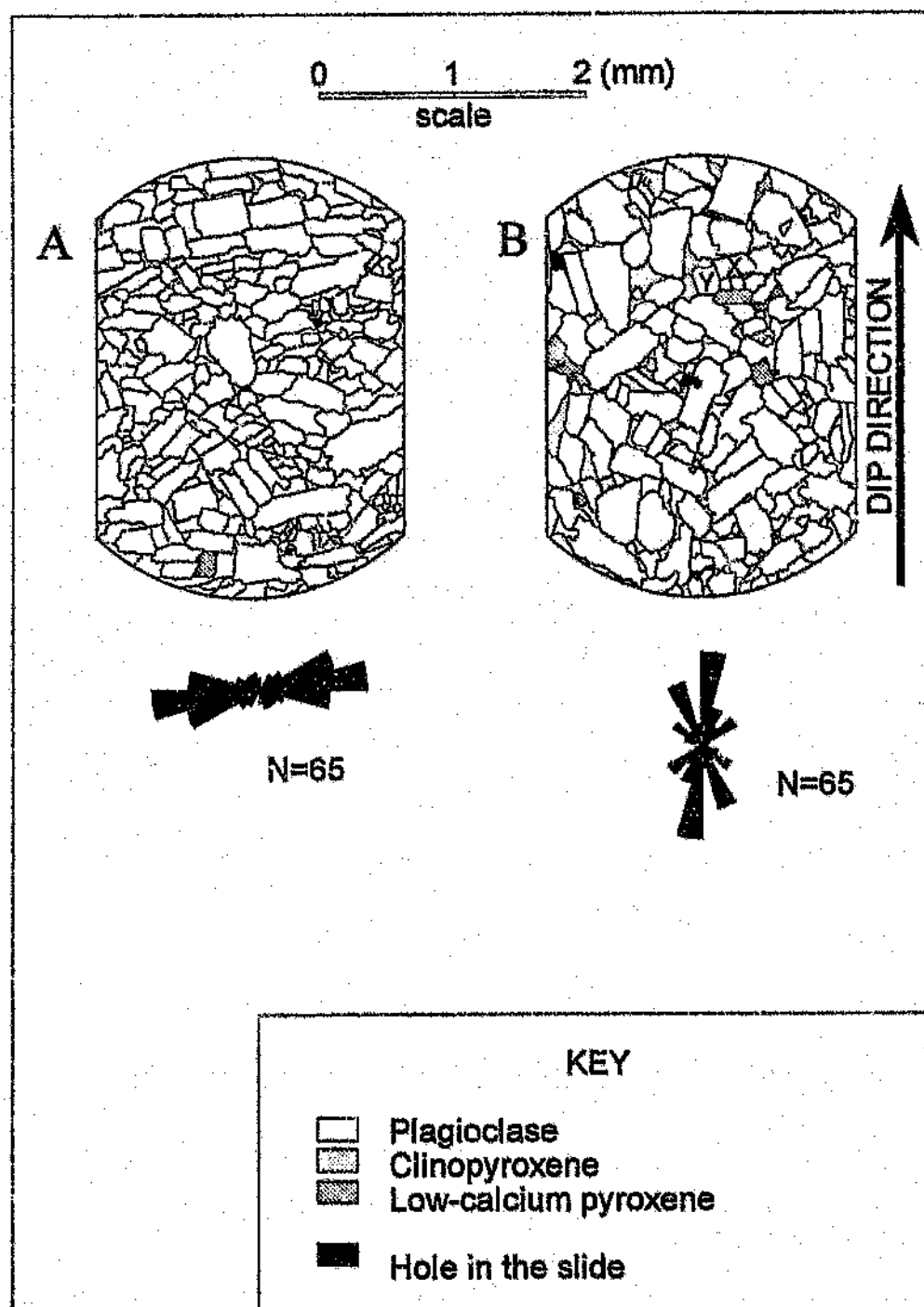
Figure 5.1 A: Sketch of a portion of a vertically orientated thin section, from a leucocratic layer. Note the well developed horizontal fabric. This is well illustrated by the attached rose diagram. B: Sketch of a portion of a thin section that was cut parallel to the plane of layering. This shows the linear habit of plagioclase within this plane. This lineation is clearly shown by the attached rose diagram.
