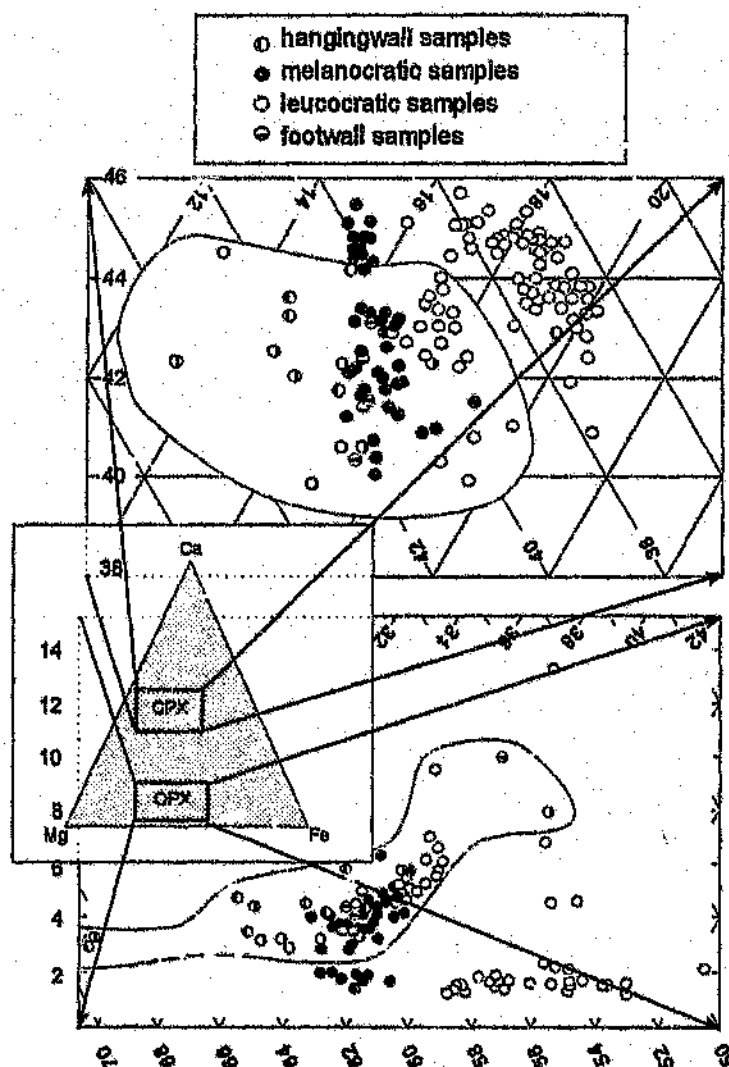
Figure 7.7 Detailed plot of the compositional variation shown by low-calcium and clinopyroxene separates as analysed in this study. The composition of those separates analysed by XRF are identified by the enclosed fields. Those data points that plot outside these fields have been analysed by microprobe.
