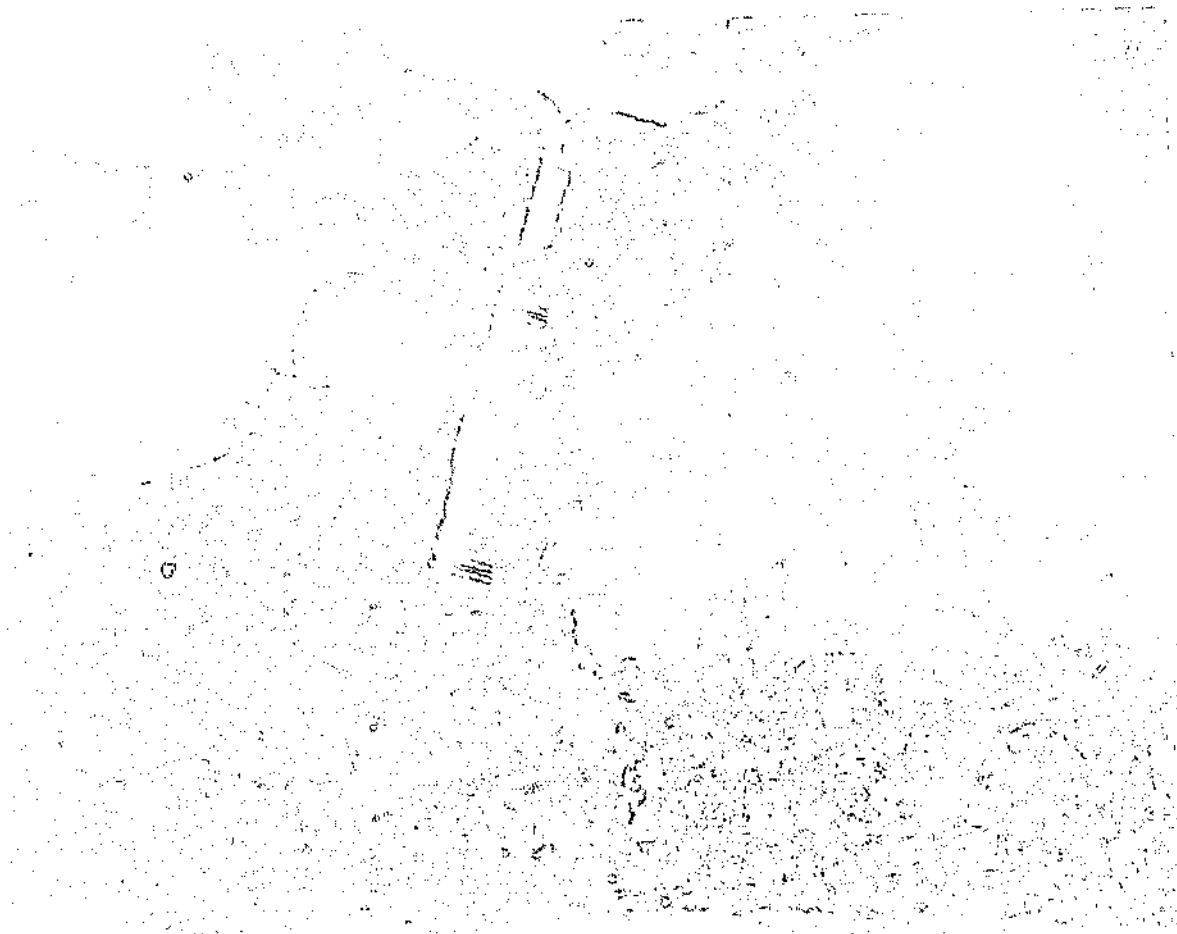
Plate 2.1. Sharp contacts and lack of grading within layers. (Photomicrograph of the ungraded character of melanocratic and leucocratic layers.)
