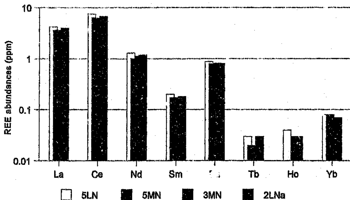
Figure 9.6 Concentration of REE's in plagioclase separates from profile A samples.
