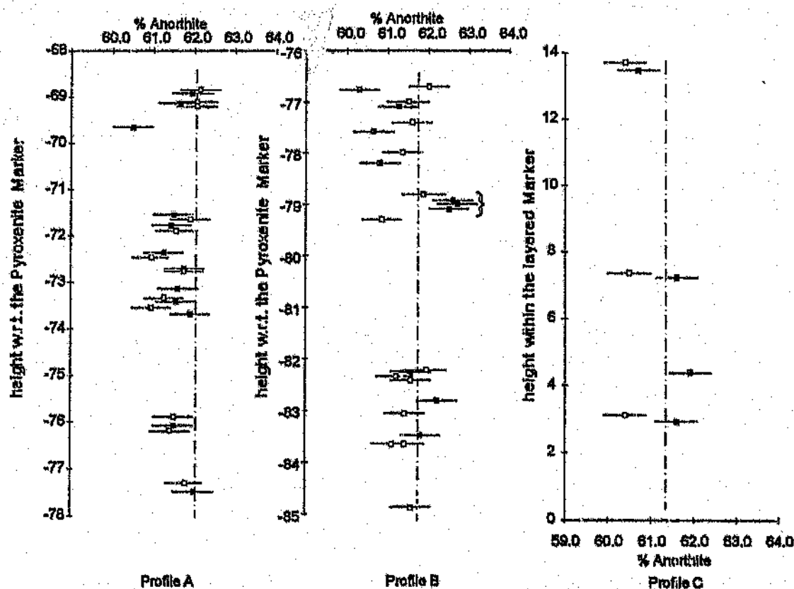
Figure 6.4 Variation in %An (An 2 ) for samples from the Layered Marker. Filled symbols refer to the mafic samples, open to the leucocratic samples. The horizontal line through each data point represents the 2σ error calculated for these analyses. The dashed lines refer to the average composition of the direct hangingwall and footwall samples.
