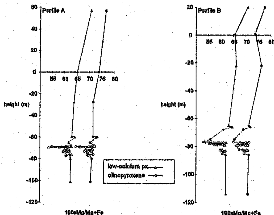
Figure 7.4 Variation in pyroxene compositions for profiles A and B. The filled symbols refer to the hangingwall and footwall samples whilst the hollow symbols refer to those samples from the Layered Marker Sequence.
