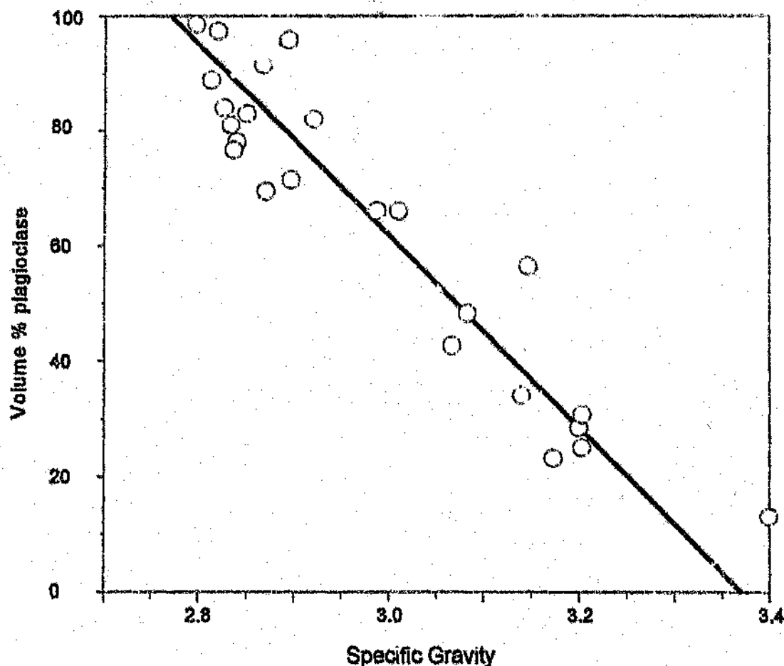
Figure 4.8 Calibration curve for the analysis of plagioclase volume % from specific gravity measurements.
