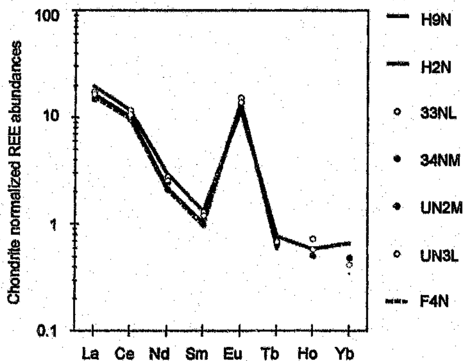
Figure 9.3 Chondrite normalized REE abundances in plagioclase separates from selected profile A samples.
