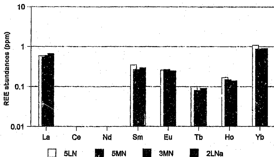
Figure 9.5 Concentration of REE's in low-calcium pyroxene separates analysed from profile A.
