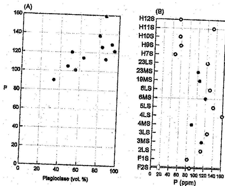
Figure 8.5 (A) Variation in P concentration with changing mode. (B) Variation in P concentrations between samples from profiles B. Samples are arranged in stratigraphic order but not to scale.
