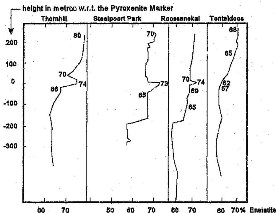
Figure 7.2 Variation in orthopyroxene composition across the Pyroxenite Marker (0m). The numbers next to each curve refer to compositions determined by X.R.F. analysis of separates (Diagram modified after Marais, 1977).
