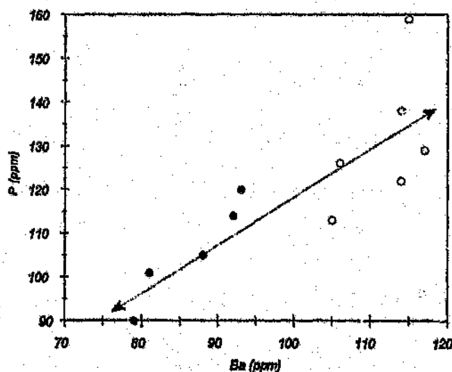
Figure 10.4 Ba versus P diagram for selected samples from profile B. The empty symbols refer to the leucocratic and the filled symbols to the melanocratic samples.
