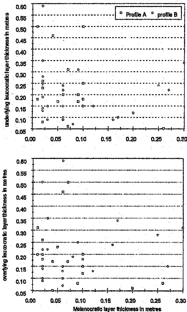
Figure 2.11 (a) Variation in underlying leucocratic layer with the overlying melanocratic layer thickness. (b) Variation in underlying melanocratic layer with the overlying leucocratic layer thickness.
