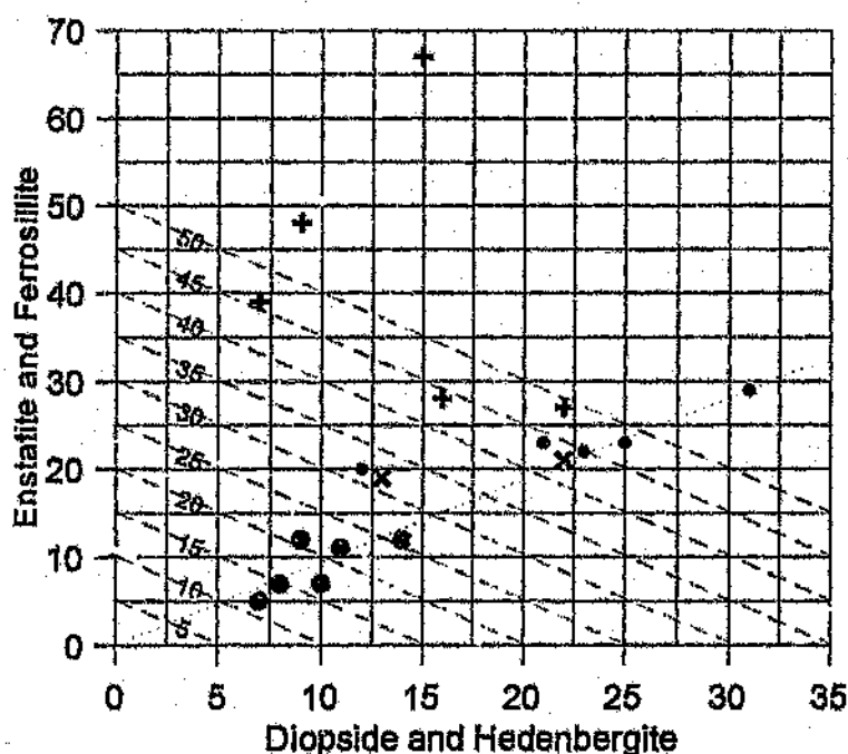
Figure 10.1 Variation in the clinopyroxene and low-calcium pyroxene abundance in selected whole rock samples as measured using a CIPW normalization calculation. The pluses refer to the hangingwall samples, crosses to the footwall samples, large filled circles to leucocratic samples and the smaller filled circles to the melanocratic samples. The weight percent of total pyroxene is shown by the numbered diagonal lines.
