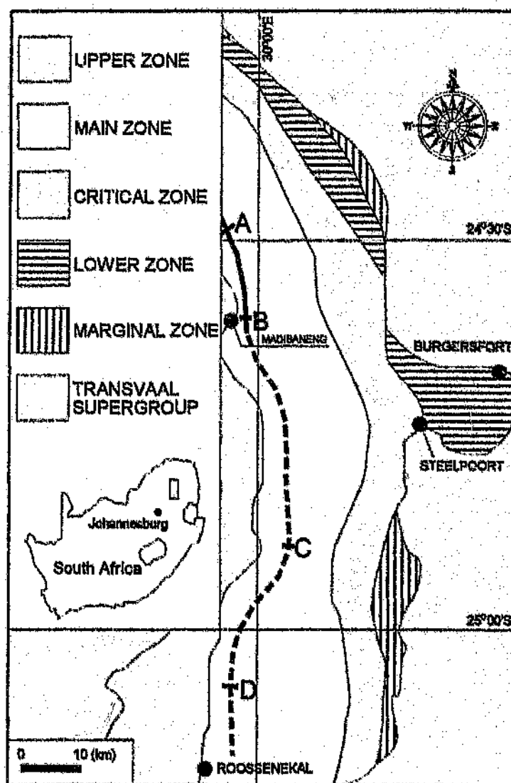
Figure 2.1 Locality map showing the approximate positions of the sample profiles
