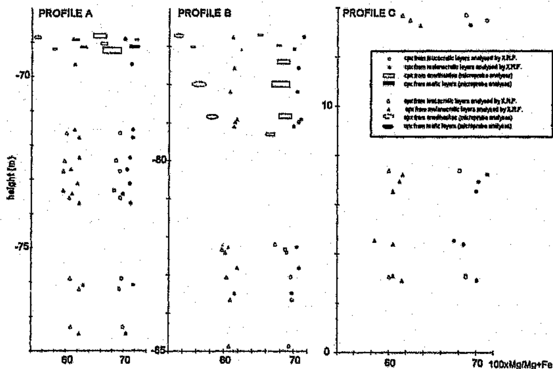
Figure 7.5 Vertical variation in pyroxene composition for samples from the Layered Marker Sequence. Symbol size is proportional to the calculated analytical error.
