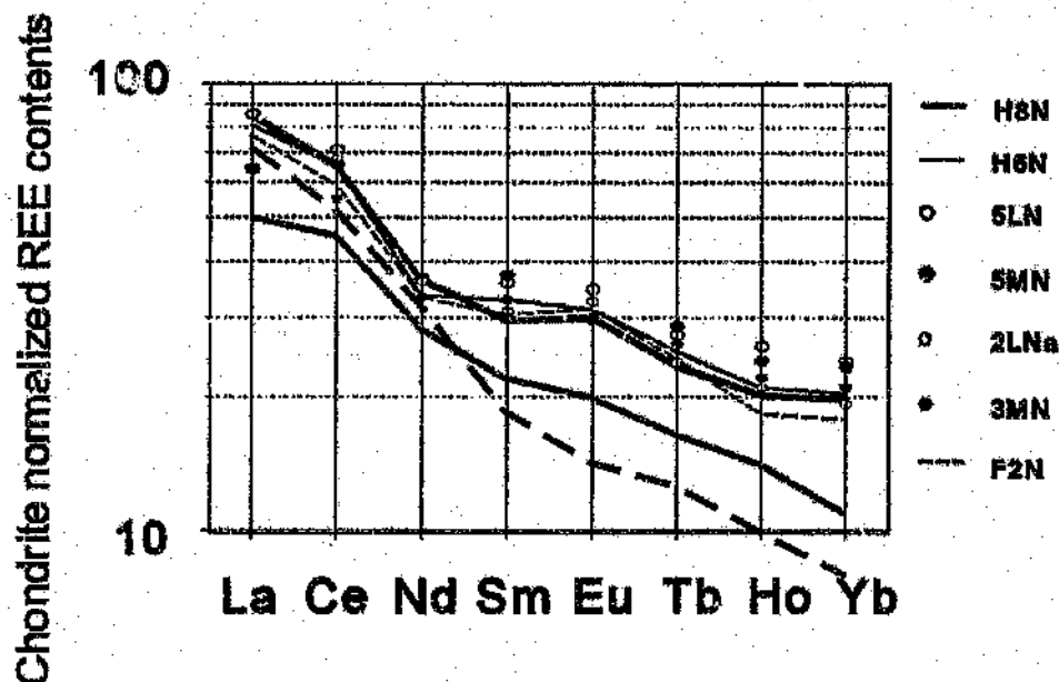
Figure 10.3 Abundance of selected REE in liquids in equilibrium with each sample. In calculating these values 10% trapped liquid has been assumed. The thick solid (green) line represents the top envelope of the compositional range for marginal rocks of the upper critical zone, as determined by Harmer and Sharpe, (1985). The thick dashed (purple) line defines the top envelope of the compositional range for 'B1-type' marginal rocks and sills, including pyroxenites and norites (Harmer and Sharpe, 1985). Note that a greater proportion of trapped liquid would push the calculated curves, for samples from the Layered Marker Sequence, to lower abundances.
