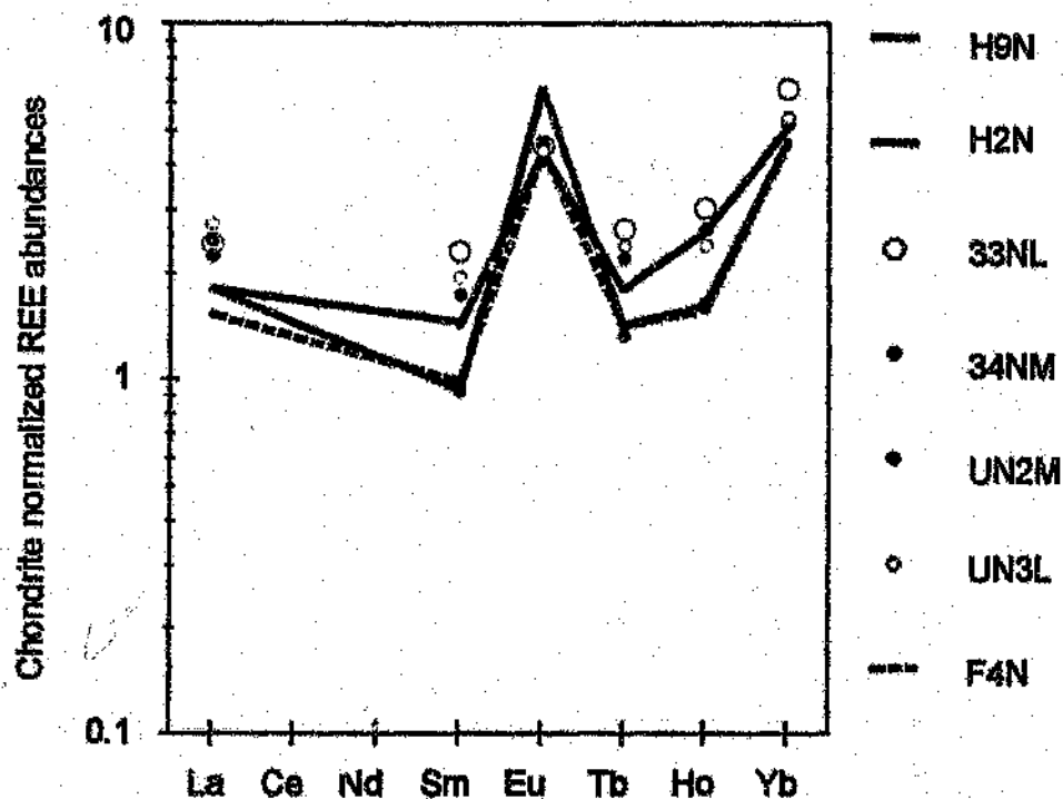
Figure 9.2 Chondrite normalized REE abundances in orthopyroxene separates from selected profile A samples.
