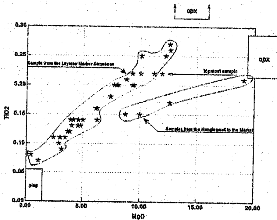
Figure 8.3 Variation of \text{TiO}_2 abundance with \text{MgO} .
