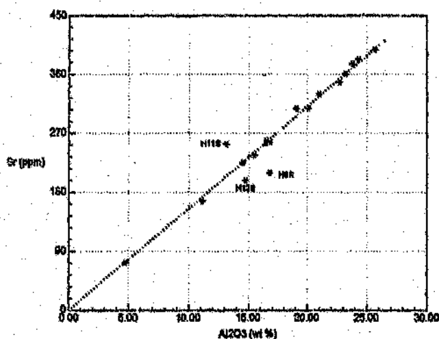
Figure 8.9 Plot of Sr versus \text{Al}_2\text{O}_3
