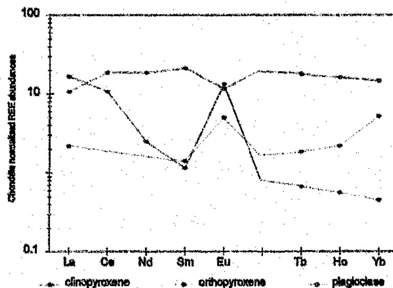
Figure A6.1 Average chondrite normalized REE abundances in plagioclase, clinopyroxene and orthopyroxene separates analysed by INAA.
