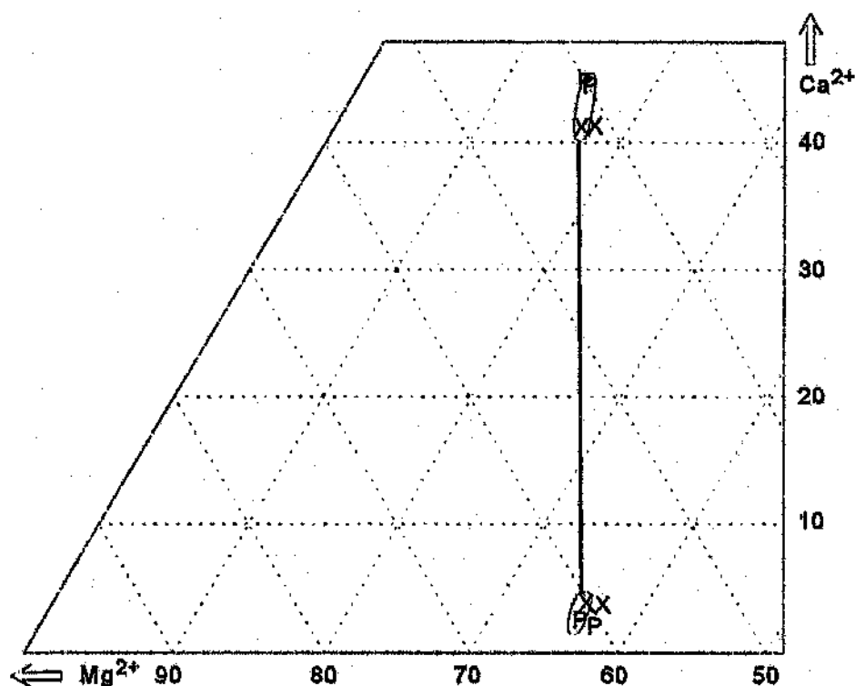
Figure 7.3 Comparison of pyroxene compositions from selected samples as determined by microprobe (p) and XRF analysis (x). Field and tie line join data points for one sample whilst the other data points refer to the other sample.
