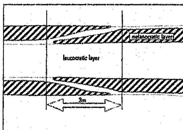
Figure 2.9 Schematic diagram showing typical layer termination morphology.
