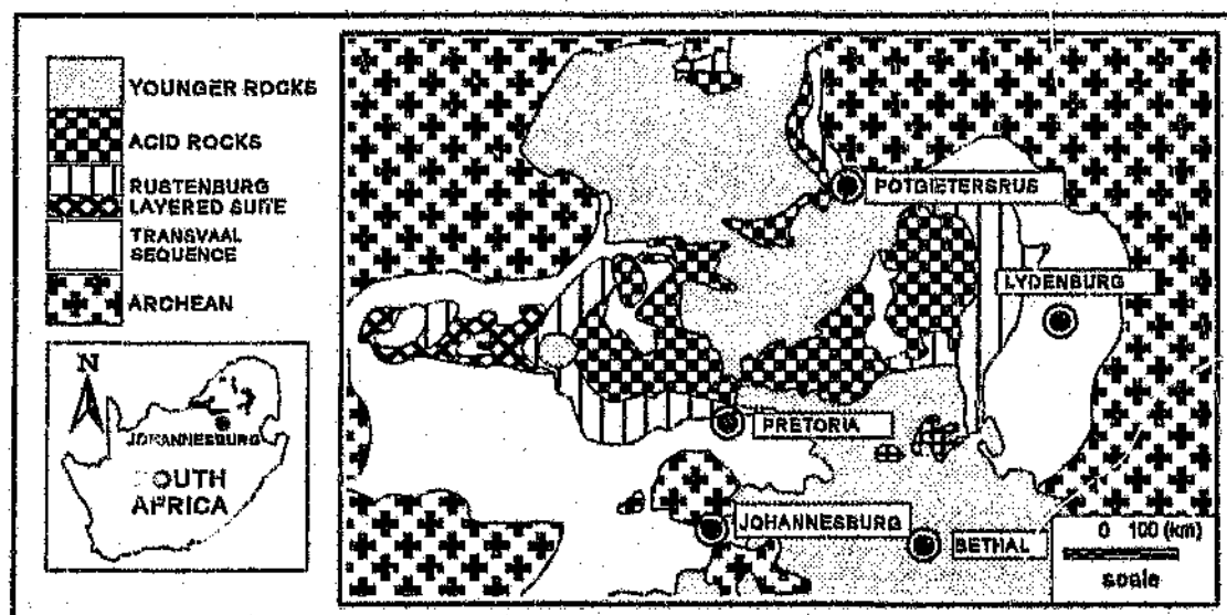
Figure 1.1 Geological map showing the lateral distribution of the Bushveld Igneous Complex rocks.
