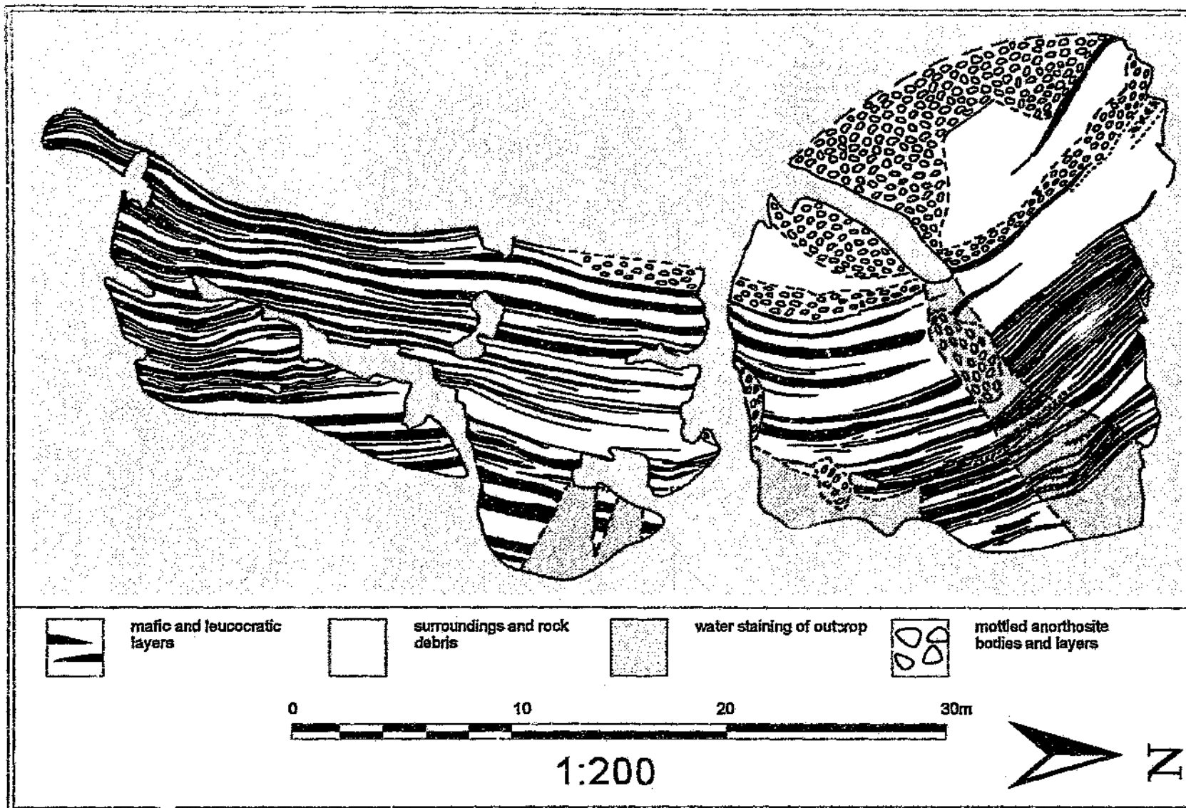
Figure 2.8 Map of a pavement exposure of the Layered Marker Sequence near locality B.
