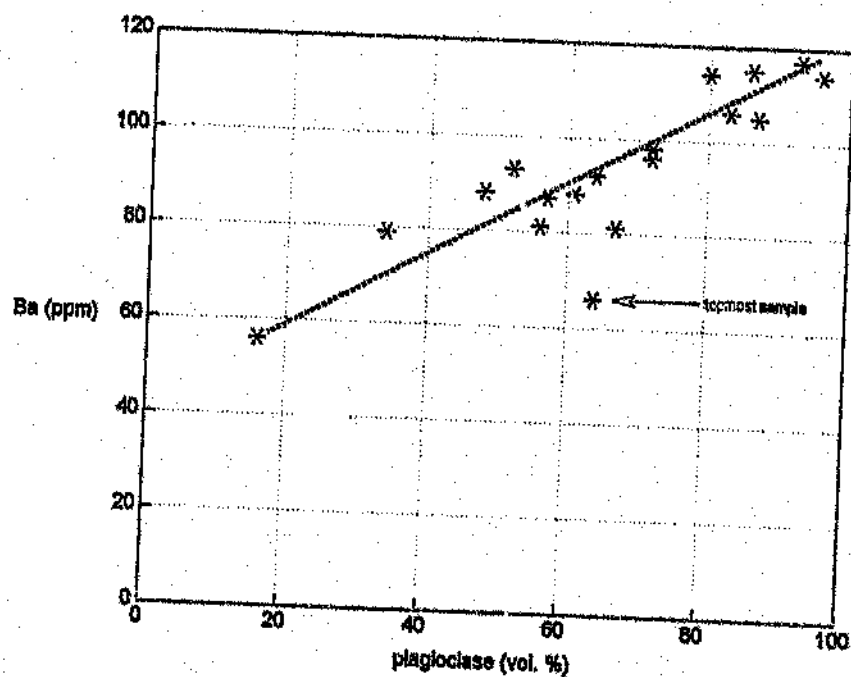
Figure 8.6 variation in Ba concentration with changing mode.
