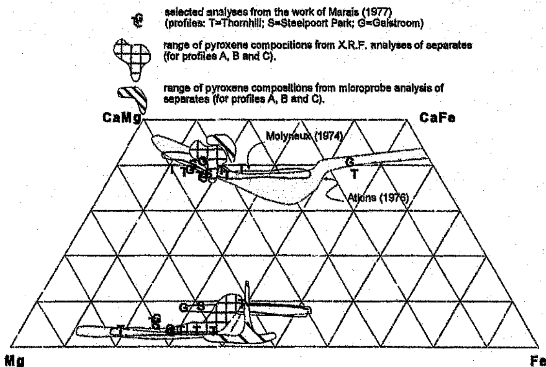
Figure 7.6 Ternary plot showing the overall range in composition of the pyroxenes analysed in the study. Also included, for comparison, is data from other studies.
