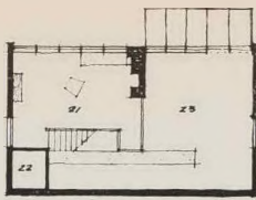
PLAN - MEZZANINE
