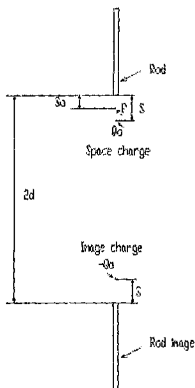
Figure 3.1 - Model of the Rod-Plane Gap
