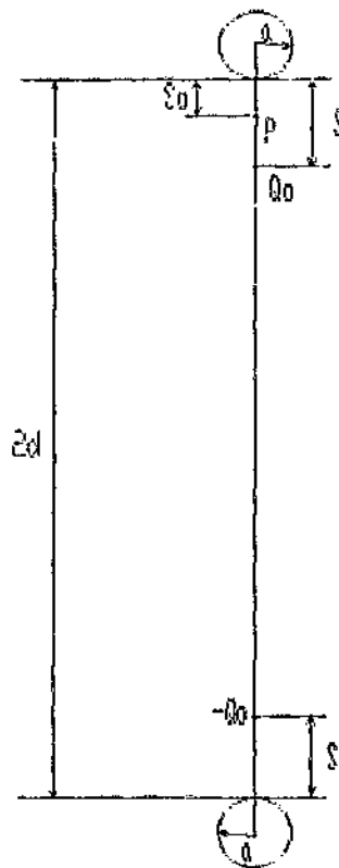
Figure B.2 - The Charge Simulation Technique
