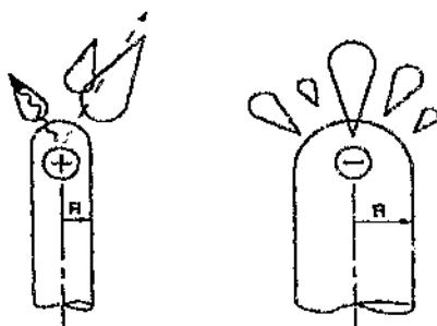
Figure 2.1 – Comparison of the Positive and Negative Streamer Channel
