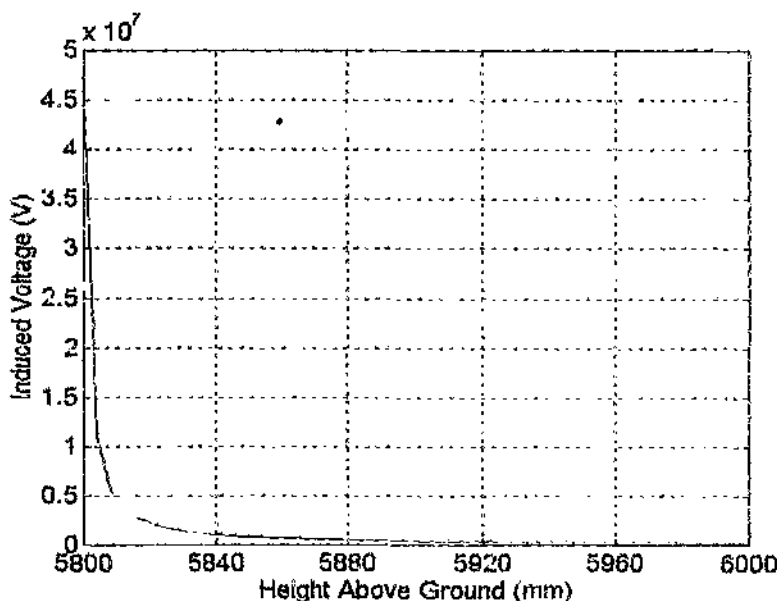
Figure 4.2 - Total Induced Voltage for the 6m Conductor-Plane Gap
