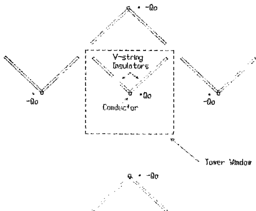
Figure 5.1 - Model for the Tower-Conductor Window Gap
