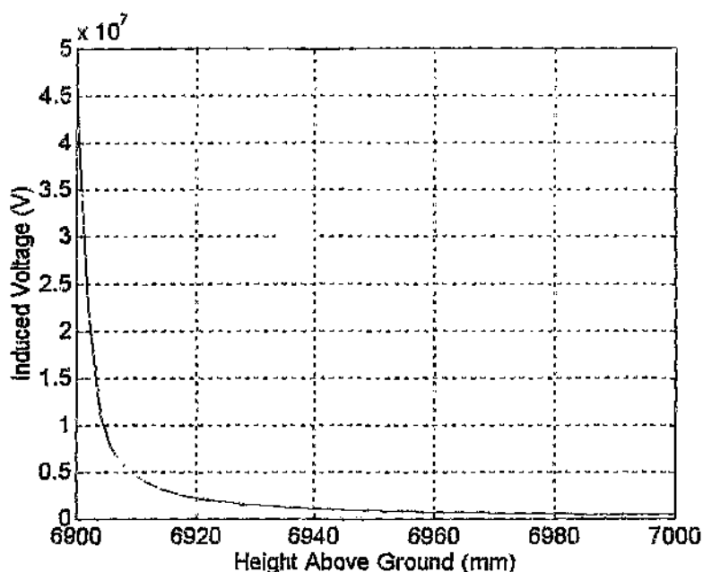
Figure 3.3 - Total Induced Voltage for the 7m Rod-Plane Gap
