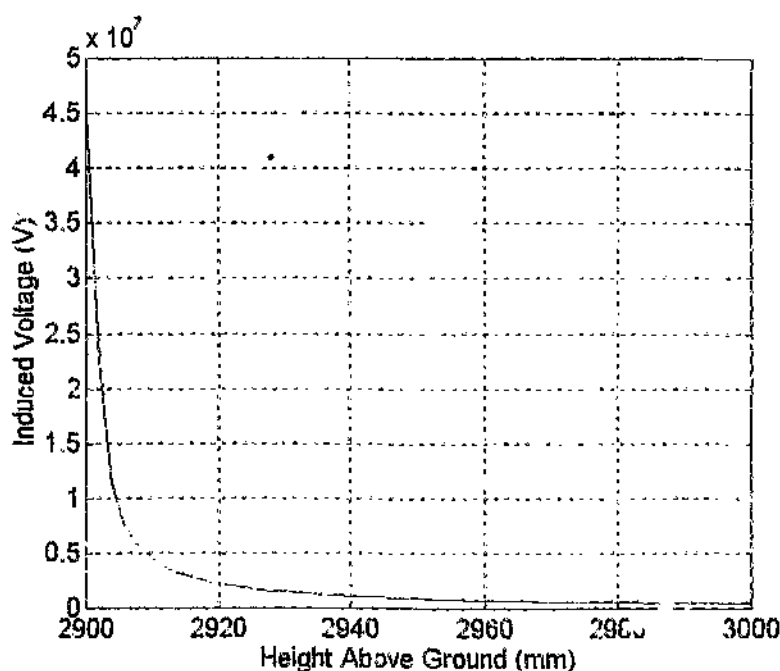
Figure 3.2 - Total Induced Voltage for the 3m Rod-Plane Gap
