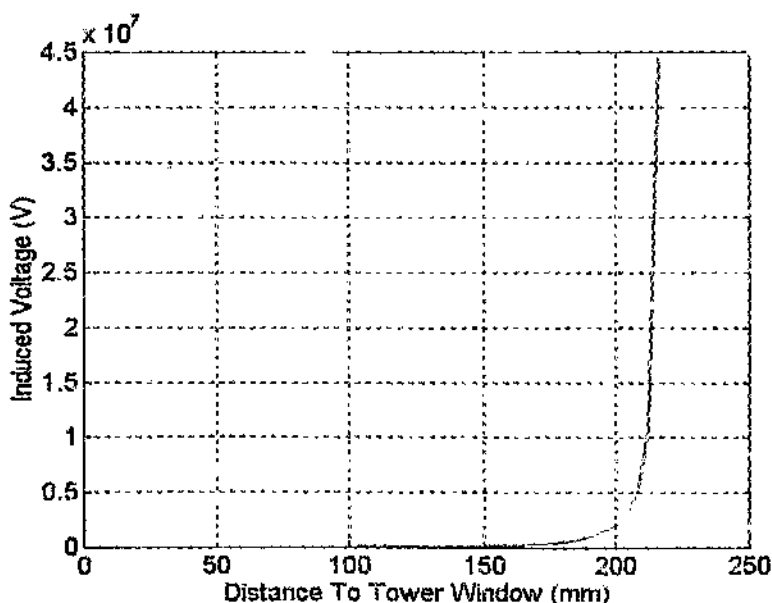
Figure 5.3 - Total Induced Voltage for the 9.3m Tower-Conductor Gap
