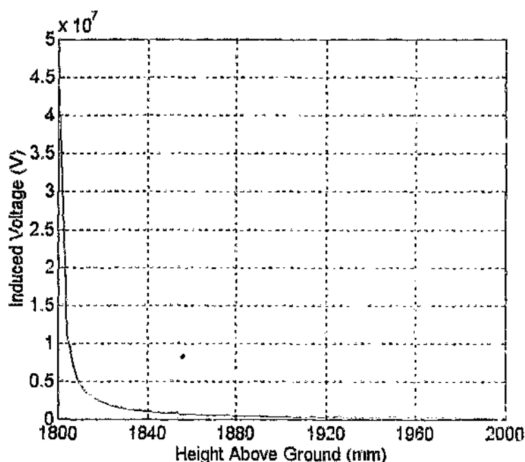
Figure 4.1 - Total Induced Voltage for the 2m Conductor-Plane Gap
