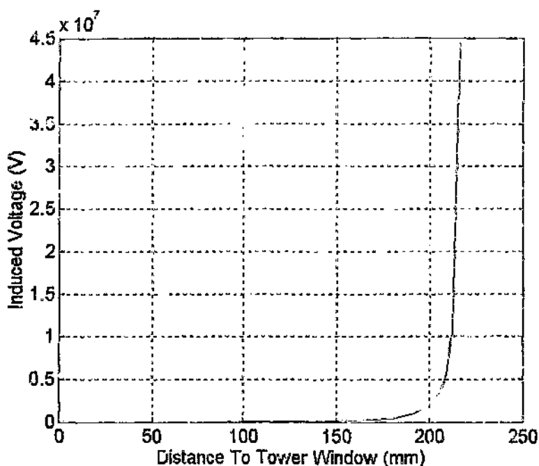
Figure 5.2 - Total Induced Voltage for the 5m Tower-Conductor Gap
