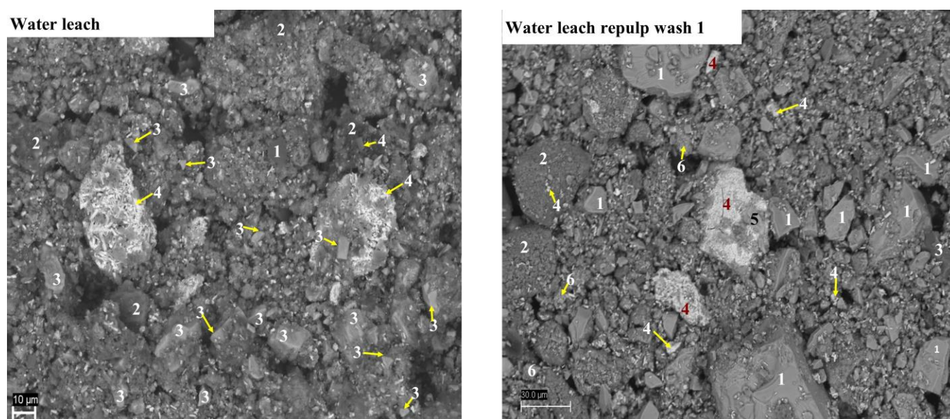
Figure 24: BSE images of residues from water leaching and washing tests; the numbered labels represent the analysed points for which average compositions are given in Table 24 .
