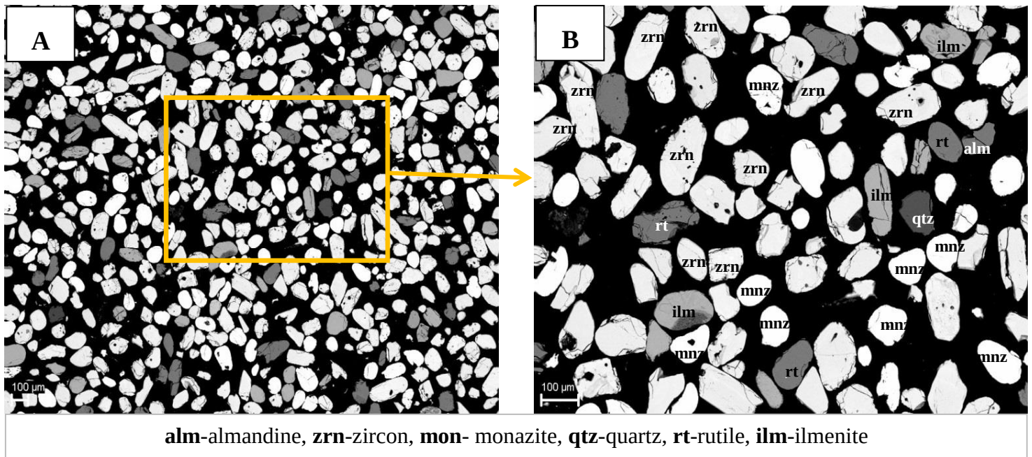
Figure 16: An overview (image A) of the –106μm size fraction illustrating the distribution of several minerals, with selected area in “yellow” presented in image B.
