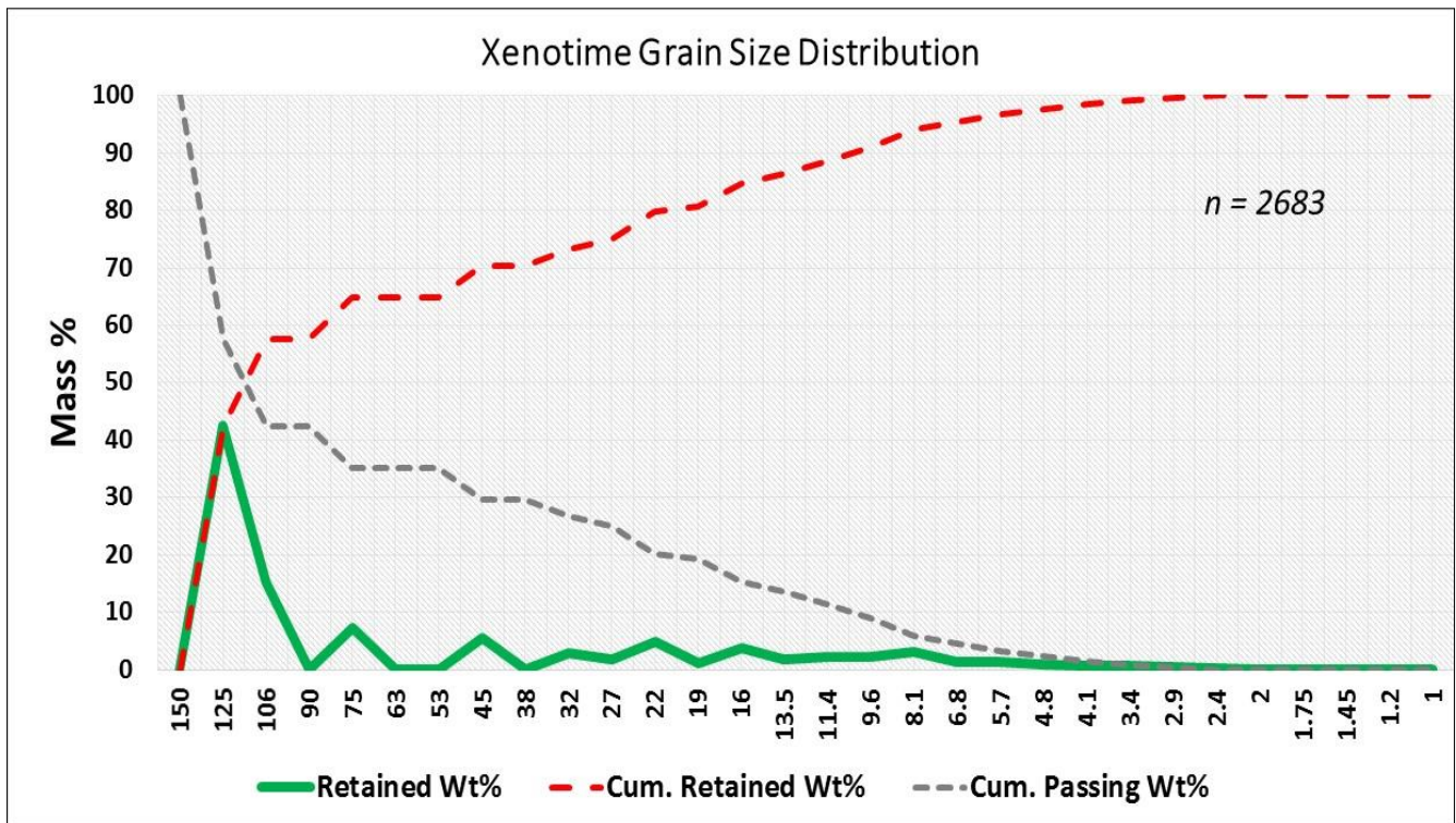
Figure 21: Xenotime grain size distribution, n = number of grains measured
