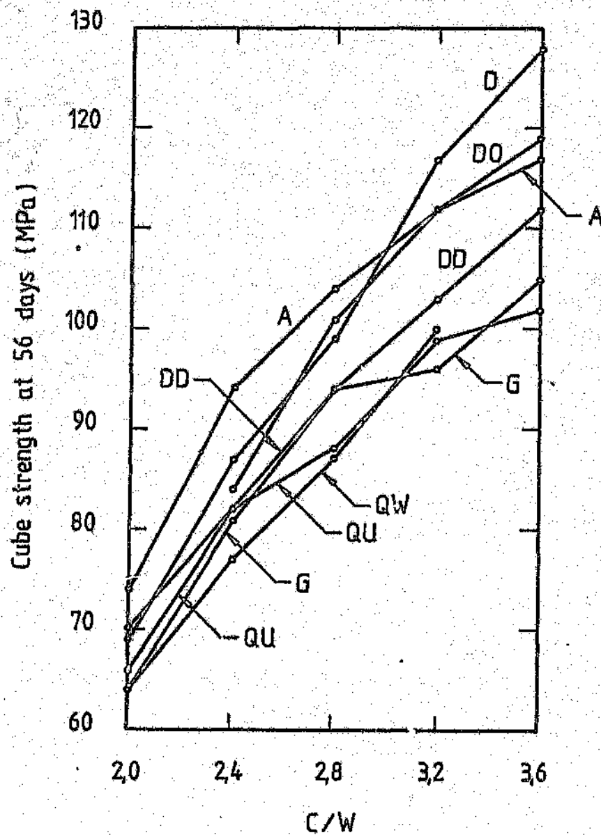
FIGURE 8.33: Cube strength at 56 days versus cement:water ratio for concretes made with aggregates of various types (see Figure 8.25 for key)
