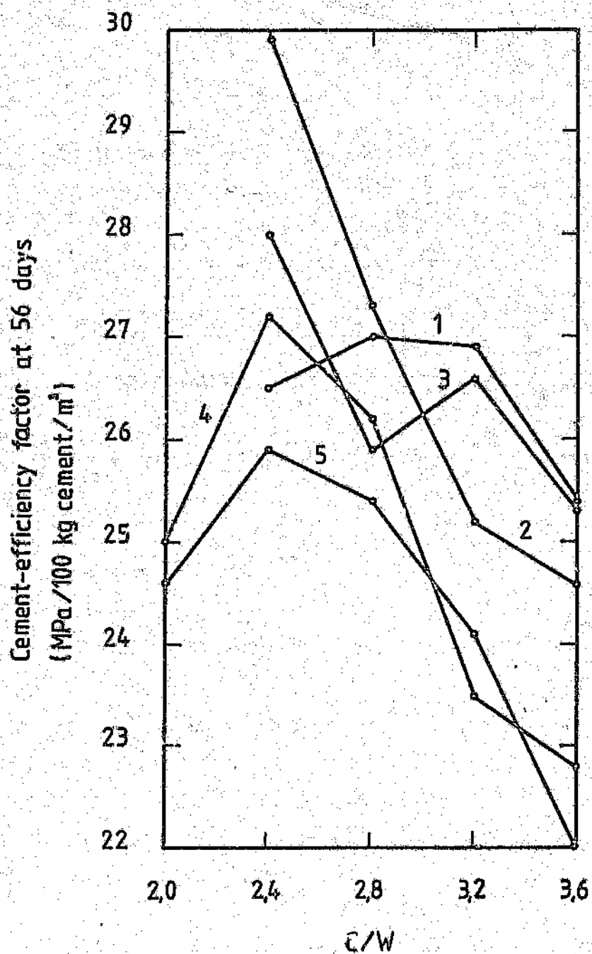
FIGURE 8.16: Cement-efficiency factor at 56 days versus cement:water ratio for concretes made with a blend of 26,5-mm and 6,7-mm stone, SNF admixture type "C" and various cementitious materials
