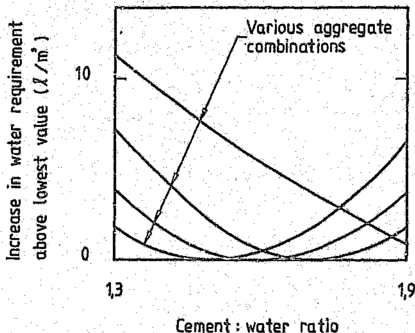
FIGURE 5.1: Increase in water requirement versus cement:water ratio for various aggregate combinations
