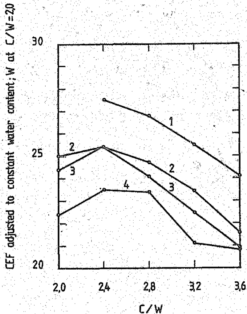
FIGURE 7.7: Cement-efficiency factor adjusted to constant water content versus cement/water ratio
