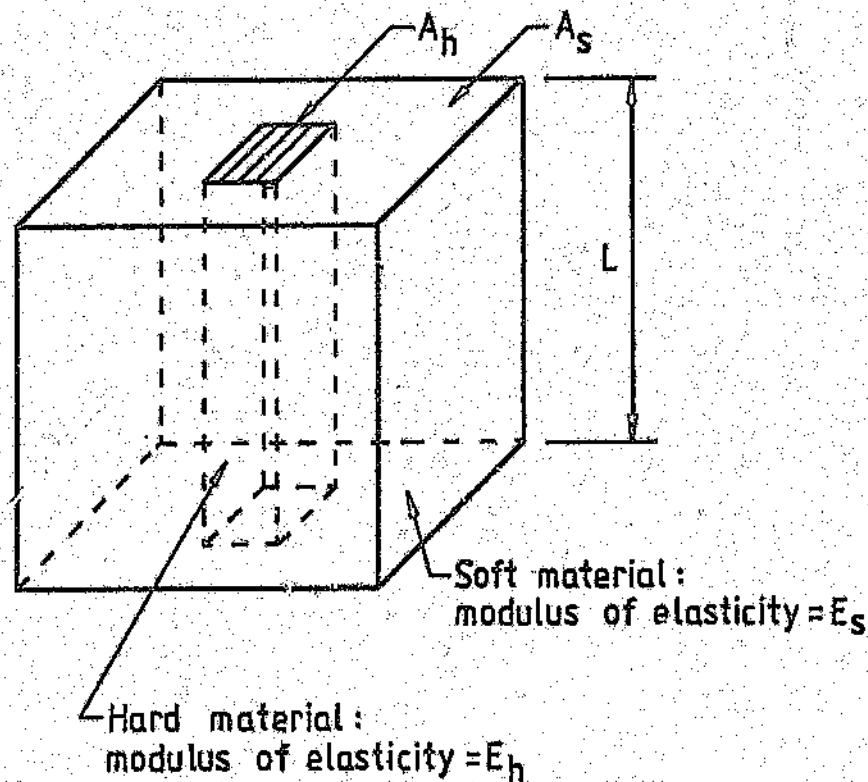
FIGURE 8.7: Isometric view of composite prism containing prisms of hard and soft phases
