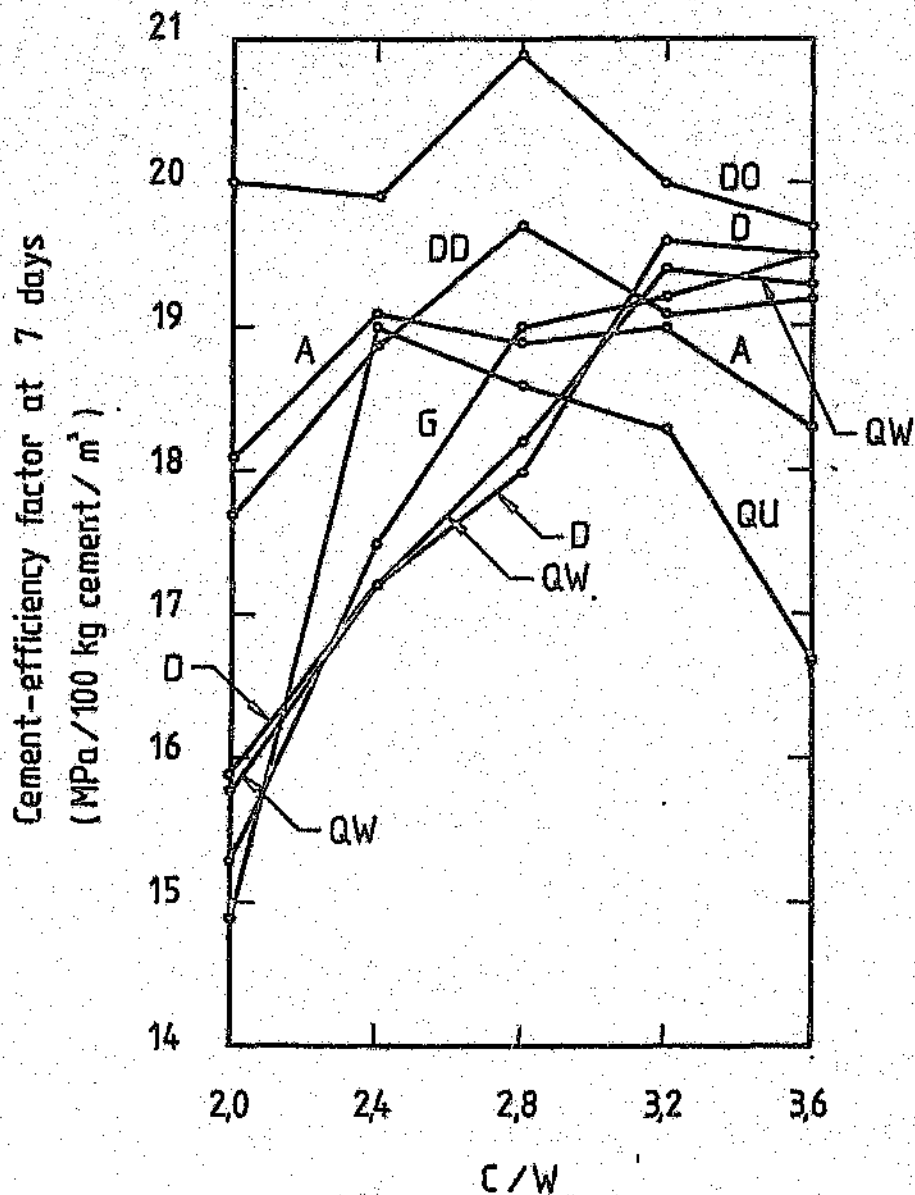
FIGURE 8.35: Cement-efficiency factor at 7 days versus cement:water ratio for concretes made with aggregates of different types (see Figure 8.25 for key)
