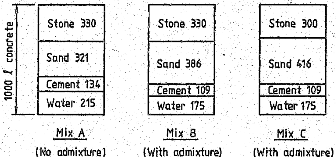
FIGURE 6.7: Solid volumes of phases of concrete in three different mixes
