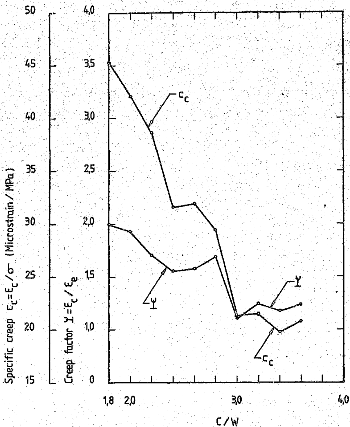
FIGURE 9.8: Specific creep and creep factor versus cement:water ratio for concretes made with andesite aggregates
