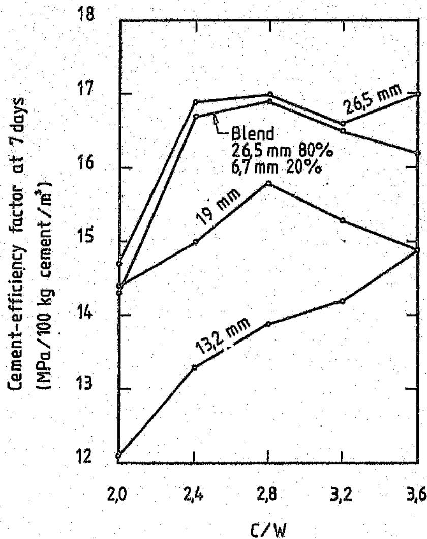
FIGURE 8.5: Cement-efficiency factor at seven days versus cement:water ratio for concrete made with stone of different sizes
