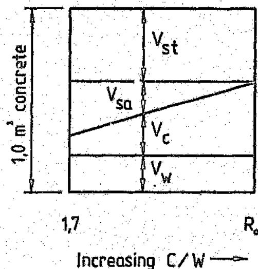
FIGURE 6.2: Solid volumes of phases of concrete versus cement:water ratio; constant stone content; constant water content
