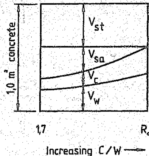
FIGURE 6.4: Solid volumes of phases of concrete versus cement:water ratio; constant stone content; water content increases at an increasing rate as C/W increases
