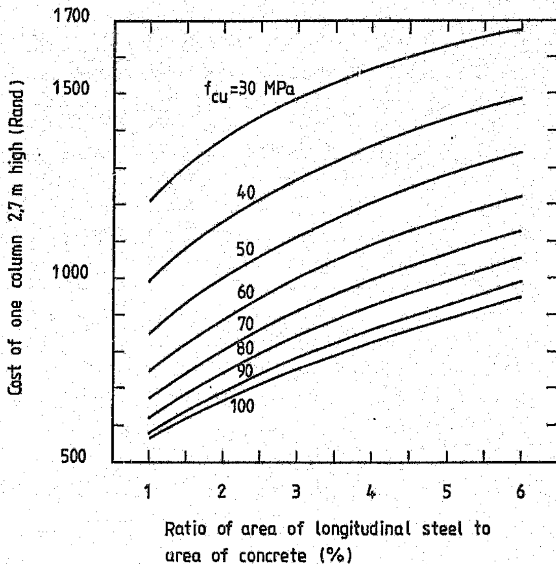
FIGURE 11.1: Building cost of one hypothetical column using local materials; based on February 1991 prices
