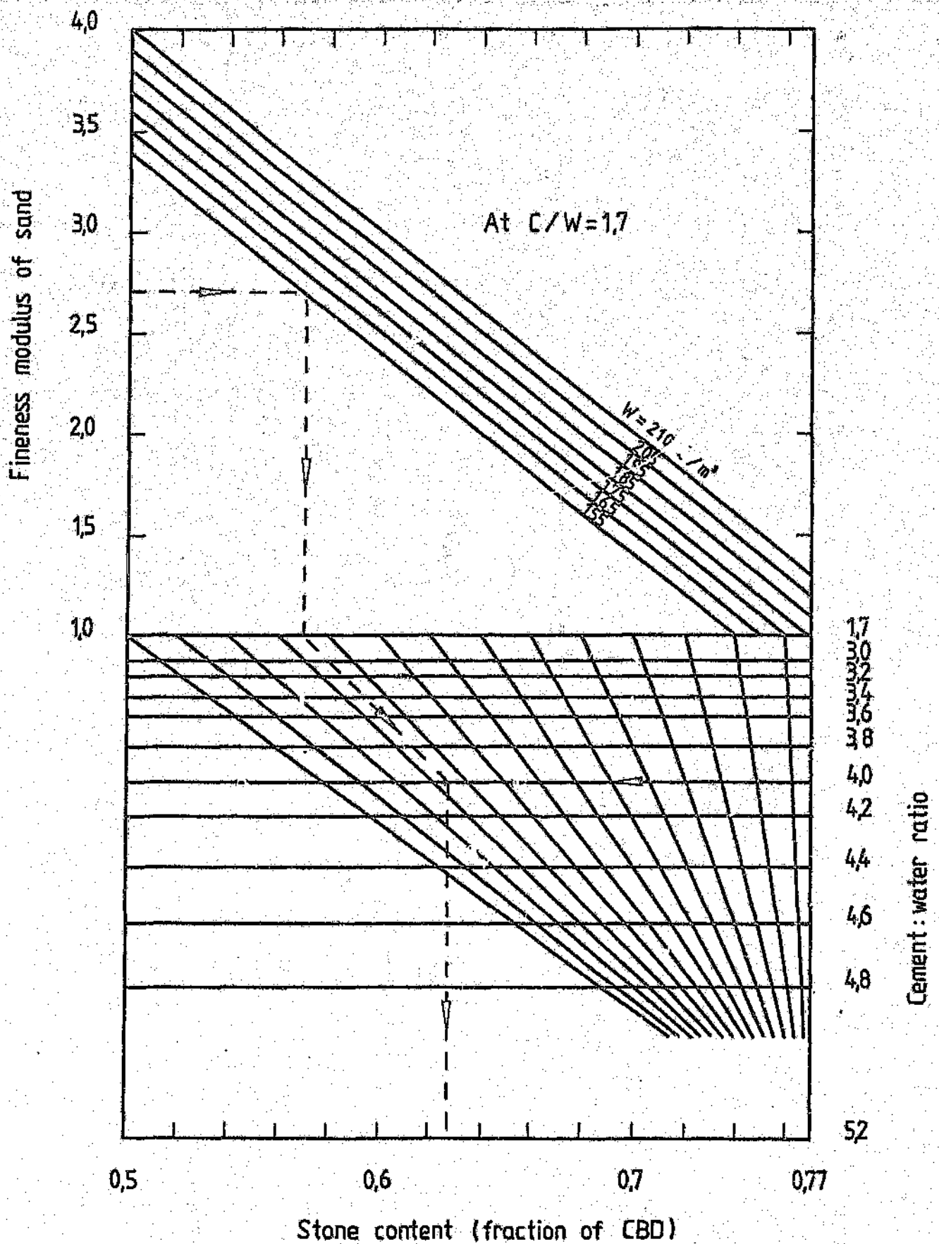
FIGURE 6.11: Chart for stone content; nominal stone size 13,2 mm ( 6,35 \leq FM of stone < 6,75 )
