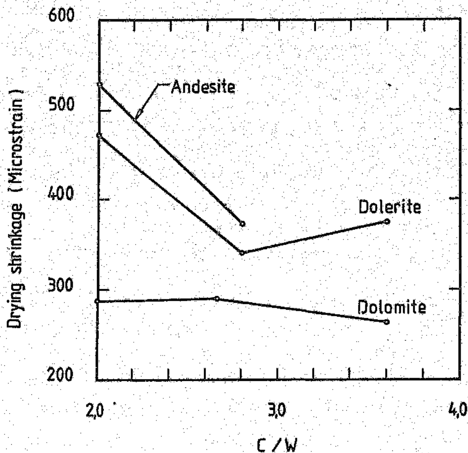
FIGURE 9.6: Shrinkage after 180 days of drying versus cement:water ratio for concretes made with three different aggregate types
