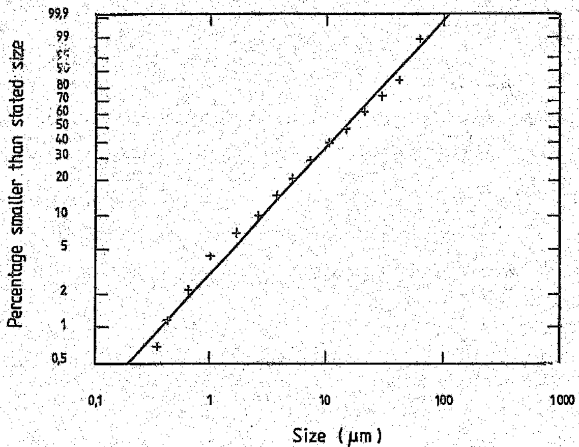
FIGURE 7.4: Particle-size distribution of cement sample
