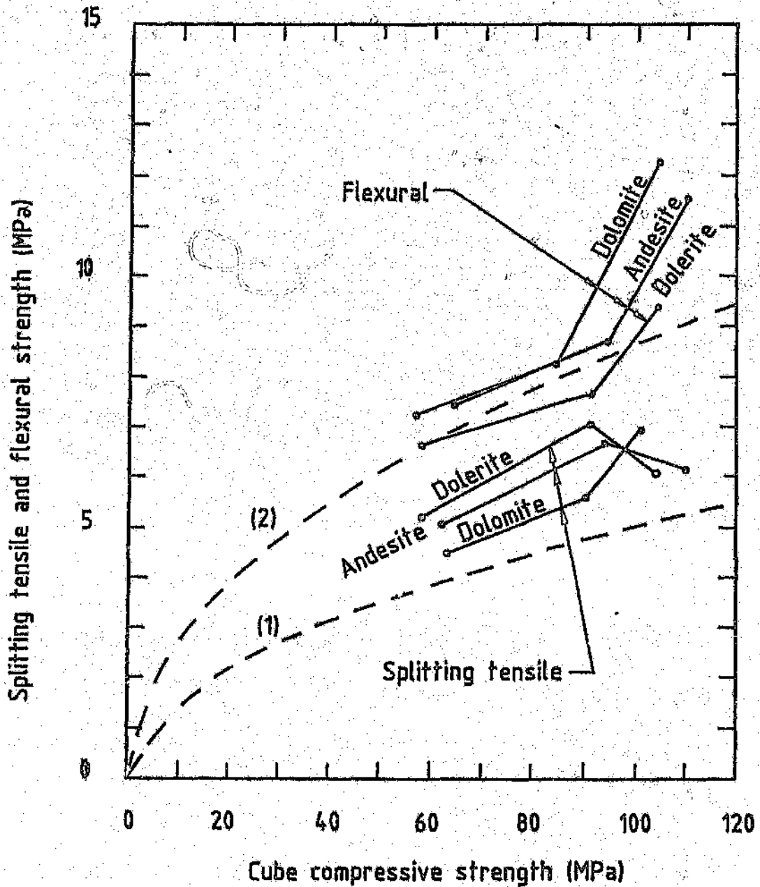
FIGURE 8.38: Splitting-tensile strength and flexural strength versus cube strength for concretes made with aggregates of various types;
