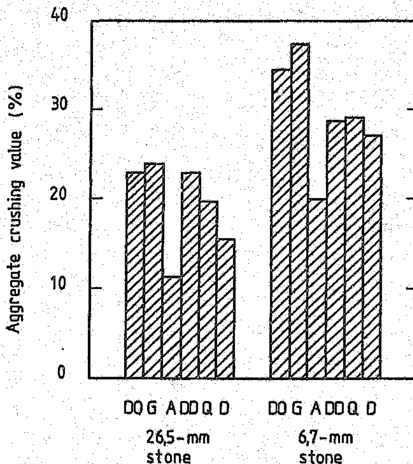
FIGURE 8.27: Aggregate crushing value for various coarse aggregates (see Figure 8.25 for key)
