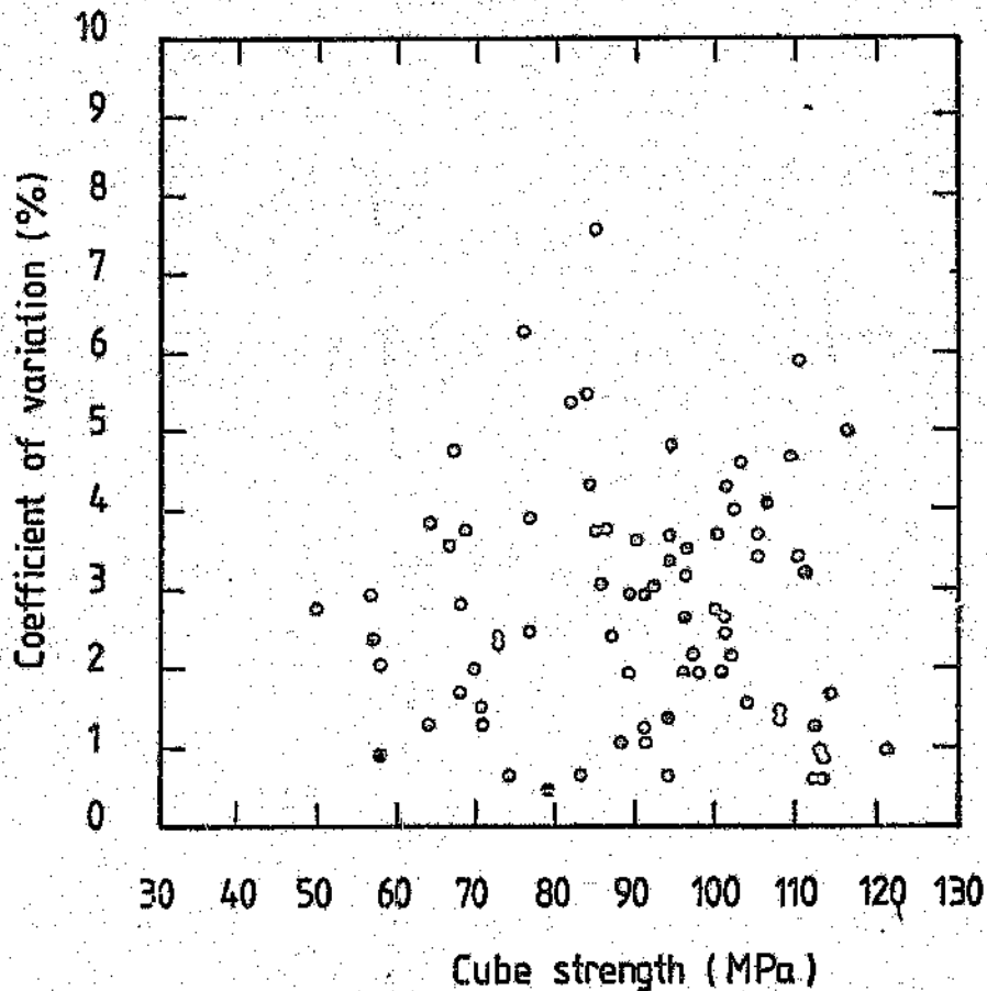
FIGURE 8.42: Coefficient of variation of individual cube strengths within batches of three versus cube strength
