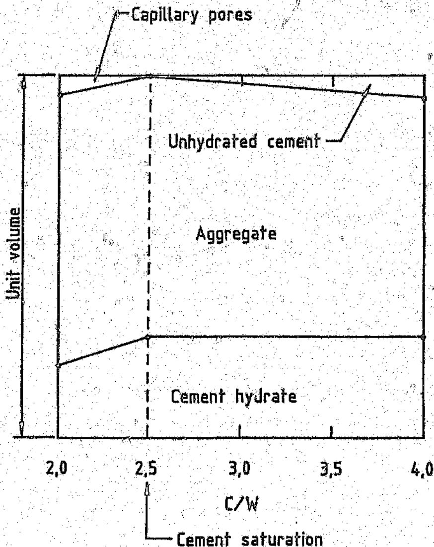
FIGURE 7.6: Volume proportions of phases of hypothetical concrete for 2 \leq C/W \leq 4 ; constant volume of mixing water 150 \text{ l/m}^3
