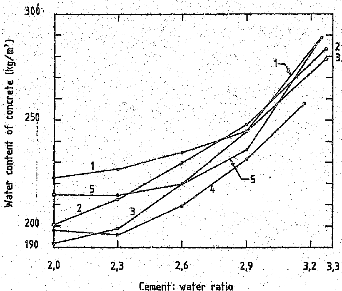
FIGURE 5.3: Water requirement versus cement:water ratio for various mixes made without admixtures; slump approximately 75 mm
