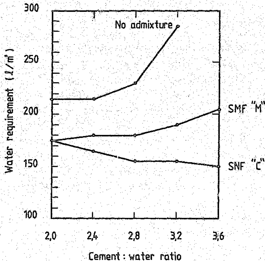
FIGURE 4.5: Water requirement of concrete versus cement:water ratio – the effect of two types of superplasticizer
