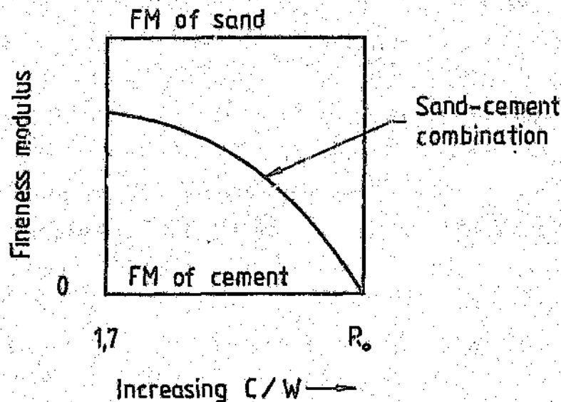
FIGURE 6.5: Fineness modulus of combination of sand and cement versus cement:water ratio; sand content is zero at C/W = R_o .
