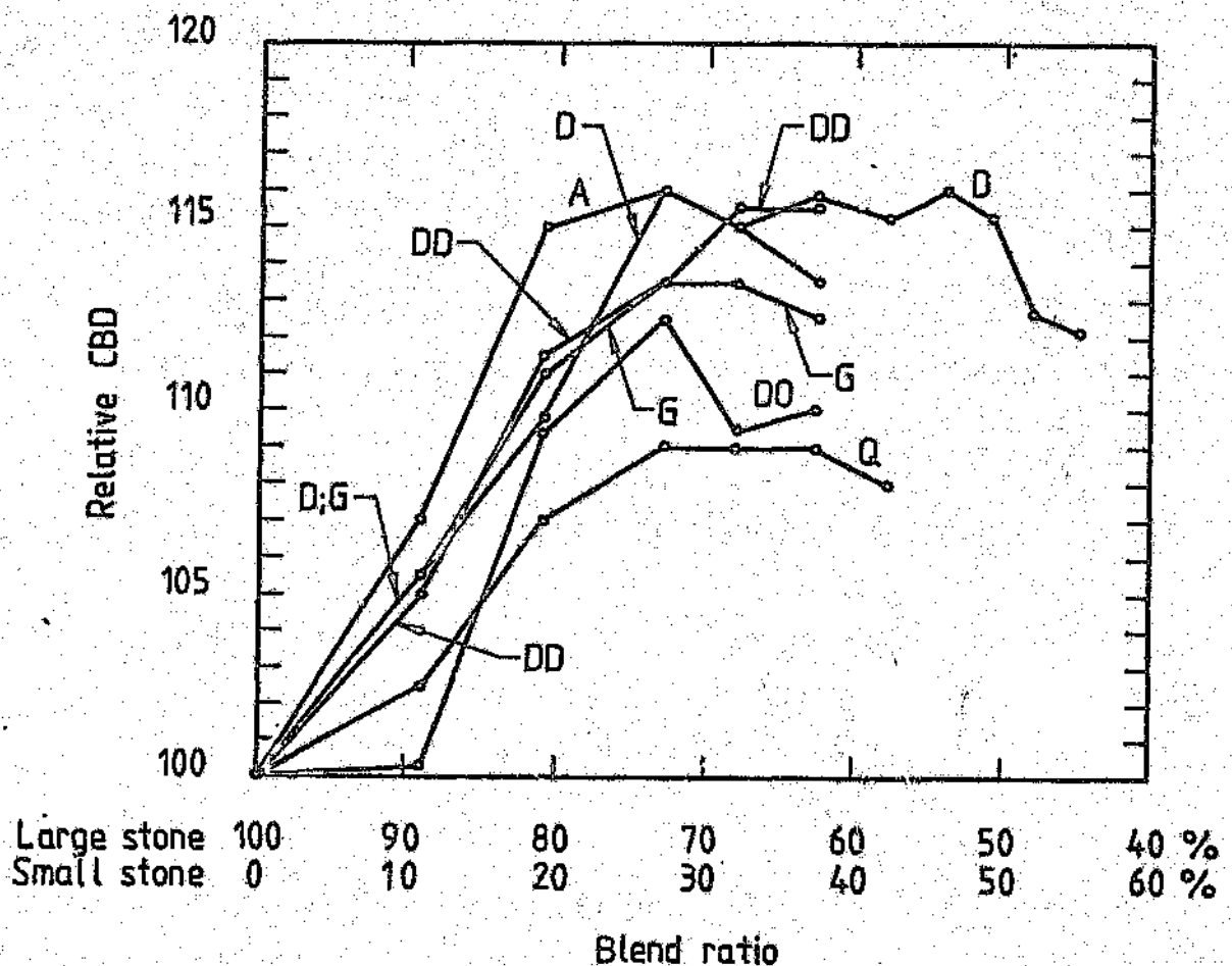
FIGURE 8.28: Relative compacted bulk density of blends of 26,5-mm and 6,7-mm stone (see Figure 8.25 for key)
