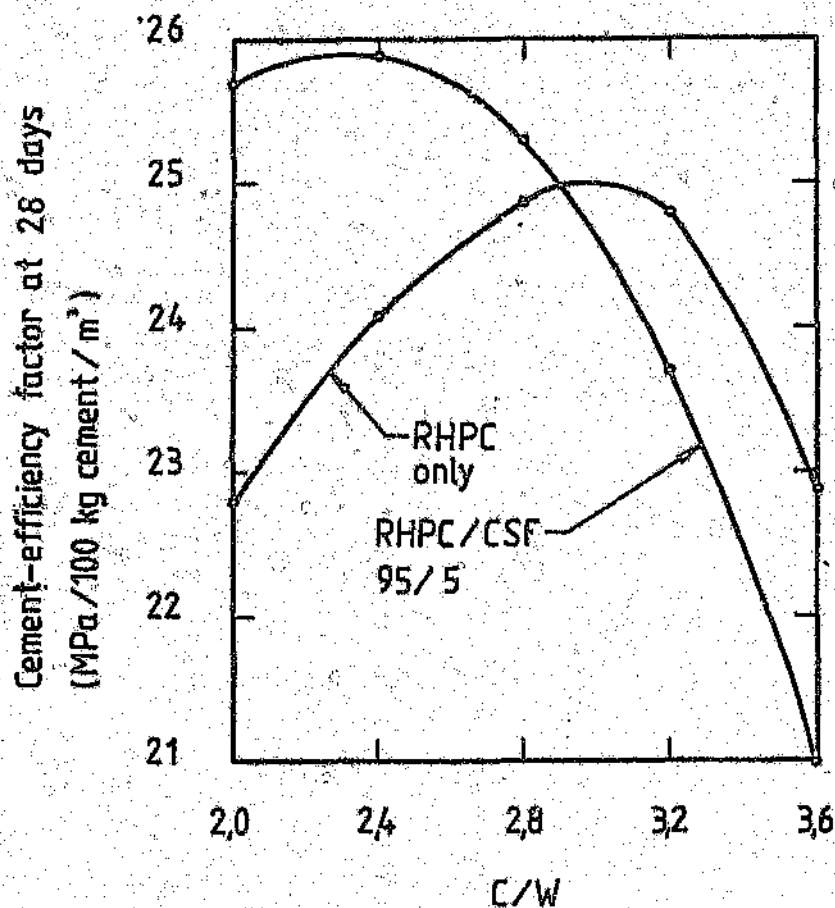
FIGURE 8.24: Cement-efficiency factor versus cement:water ratio for concretes made with RHPC only and a blend of RHPC and condensed silica fume
