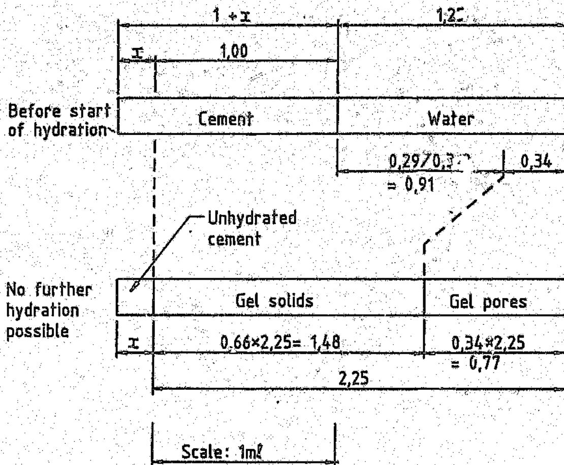
FIGURE 7.2: Absolute volumes of phases of cement paste for cement-oversaturated mix
