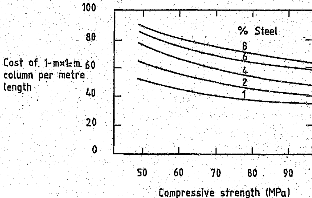
FIGURE 2.3: Cost of column versus compressive strength of concrete and for different percentages of steel [2.101]
