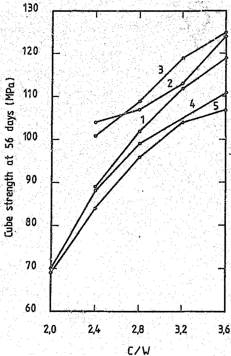
FIGURE 8.15: Cube strength at 56 days versus cement:water ratio for concretes made with a blend of 26,5-mm and 6,7-mm stone, SNF admixture type "C" and various cementitious materials
