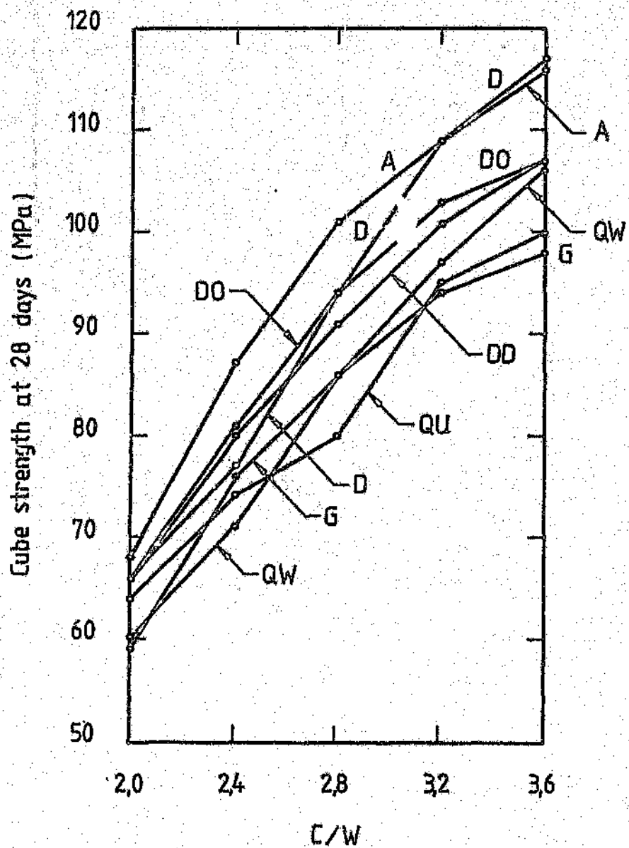
FIGURE 8.32: Cube strength at 28 days versus cement:water ratio for concretes made with aggregates of various types (see Figure 8.25 for key)
