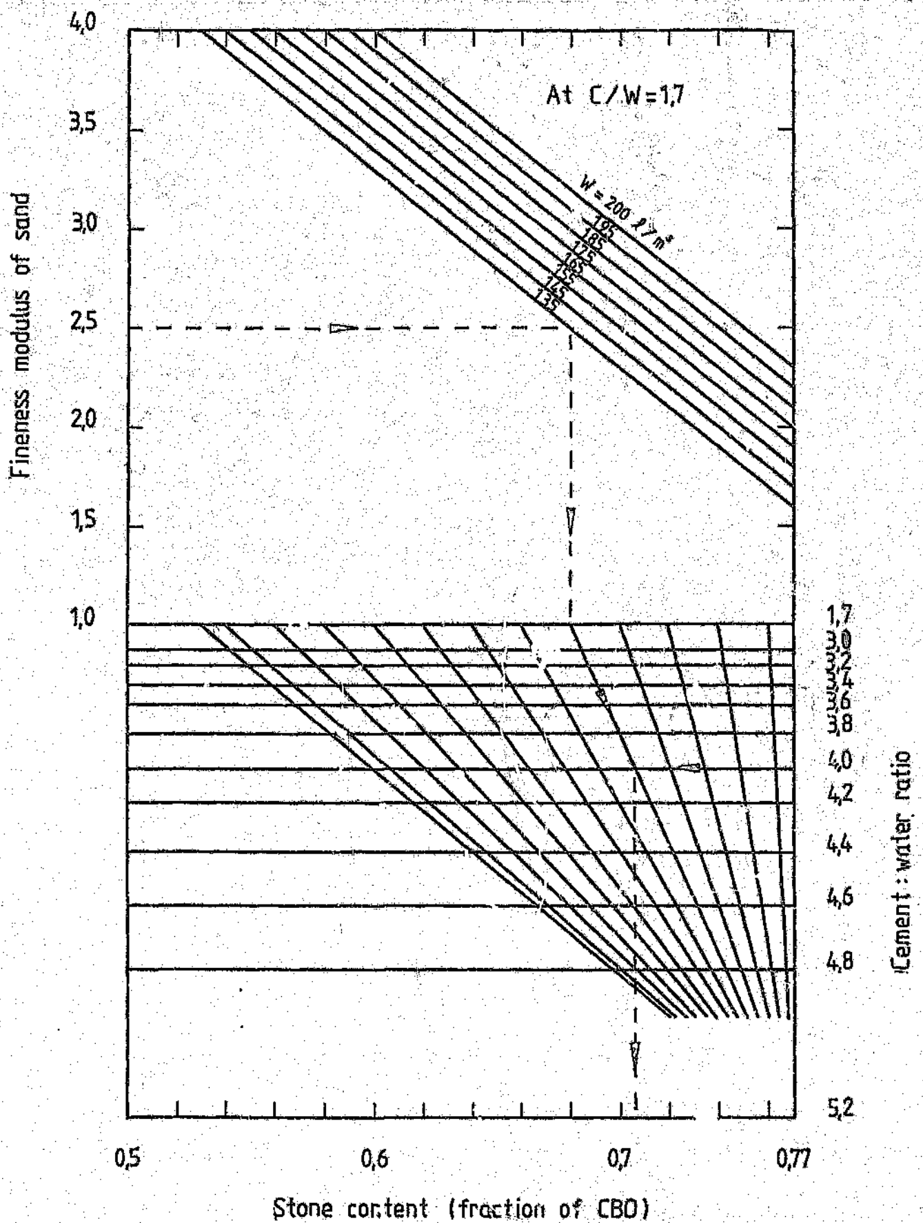
FIGURE 6.12: Chart for stone content; nominal stone size 19 mm ( 6.75 \leq \text{FM of stone} \leq 7.15 )
