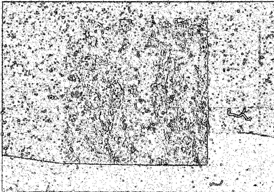
FIGURE 8.41: Photograph of fracture face; splitting-tensile test; dolomite aggregate; cube strength 101 MPa; splitting-tensile strength 7,0 MPa
