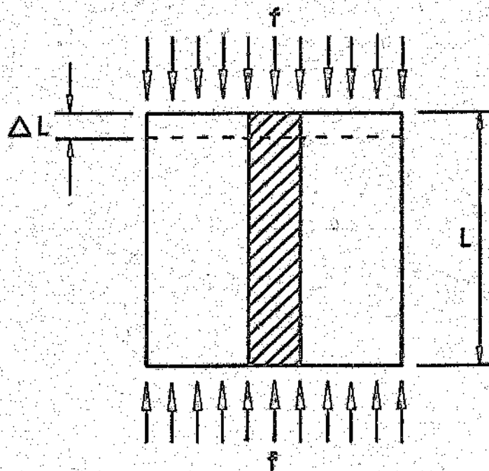
FIGURE 8.8: Shortening of composite prism under stress f
