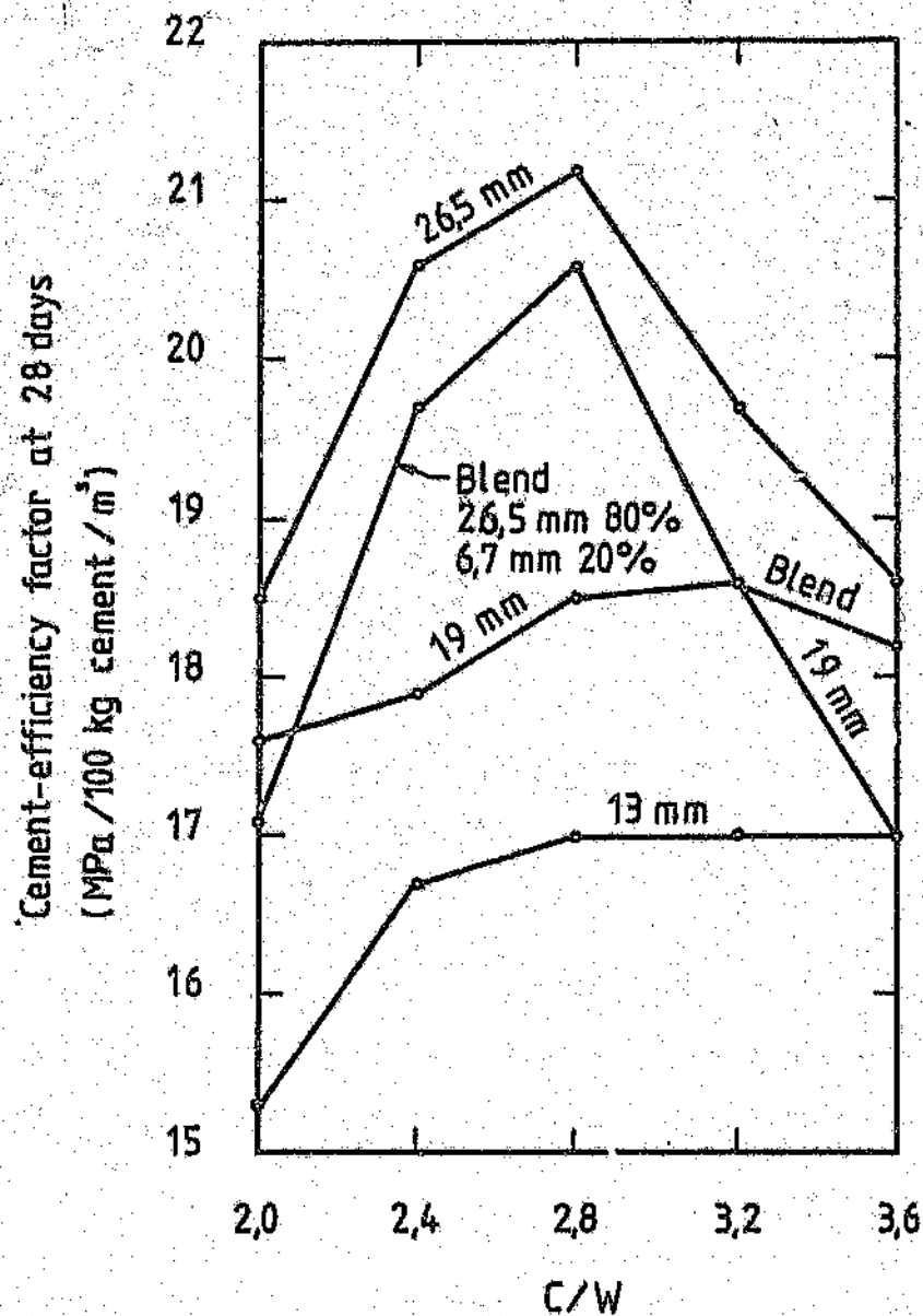
FIGURE 8.6: Cement efficiency factor at 28 days versus cement:water ratio for concrete made with stone of different sizes
