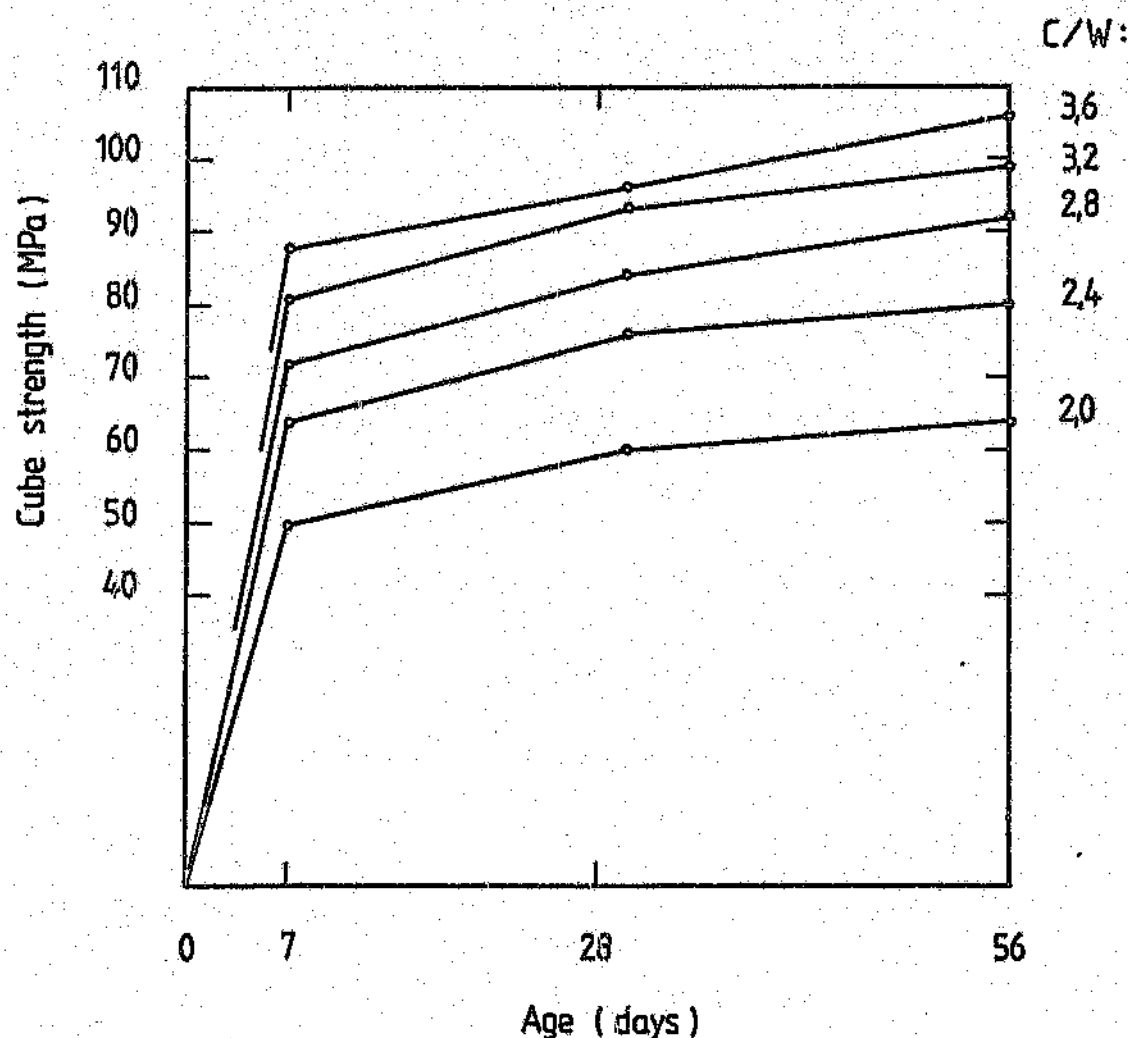
FIGURE 7.9: Strength development of actual concretes versus age; concrete made with RHPC type J, 13,2-mm dolomite stone, dolomite crusher sand, SNF admixture; specimens cured in air with 100 % RH for first 24 h then in water; testing done in wet state
