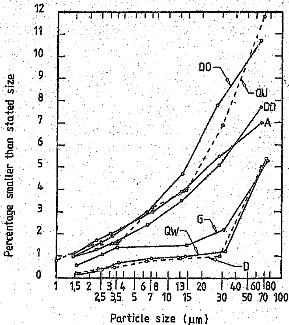
FIGURE 8.25: Fine material in sands according to hydrometer method
