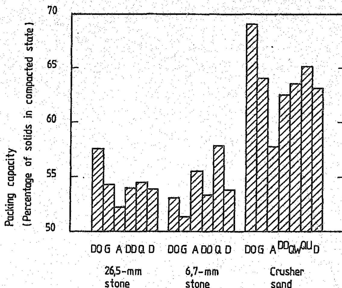
FIGURE 8.26: Packing capacity of various aggregates (see Figure 8.25 for key)
