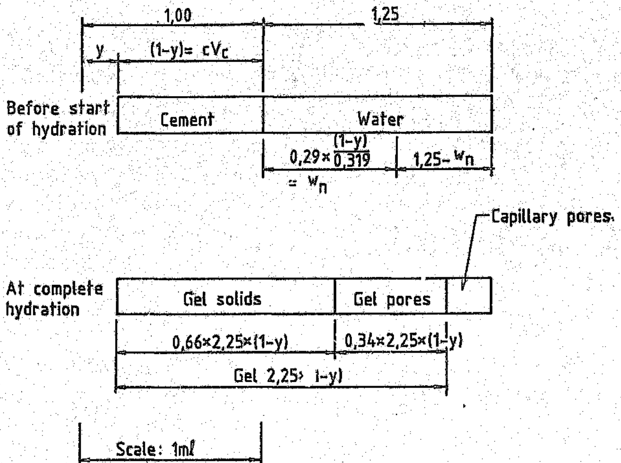
FIGURE 7.3: Absolute volumes of phases of cement paste for cement-undersaturated mix
