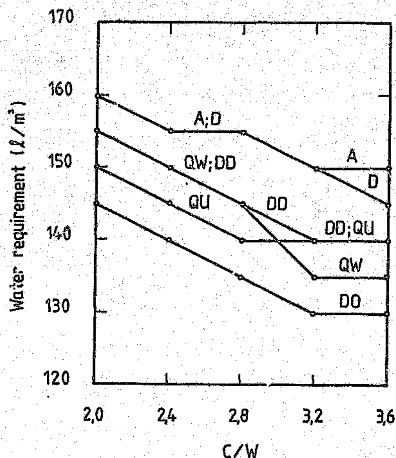
FIGURE 8.29: Water requirement (to nearest 5 l/m^3 ) for 75-mm slump versus cement:water ratio for concretes made with aggregate of various types (see Figure 8.25 for key)
