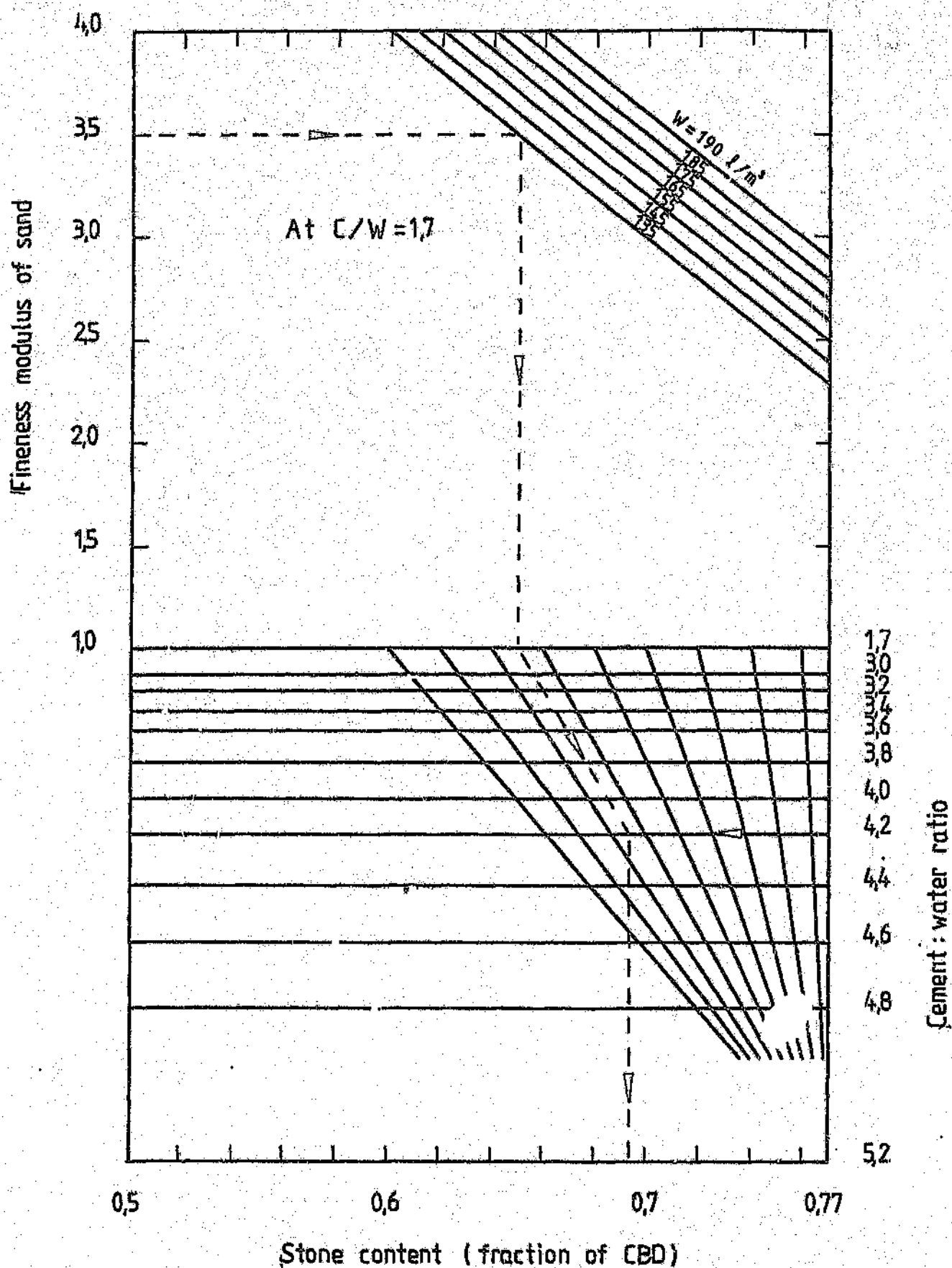
FIGURE 6.13: Chart for stone content; nominal stone size 26,5 mm ( 7,45 \leq \text{FM} of stone \leq 8,0 )
