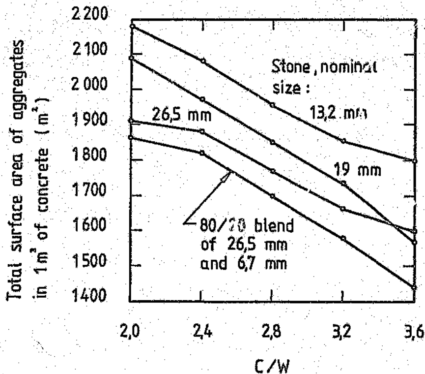
FIGURE 6.15: Total surface area of aggregates versus cement:water ratio for actual mixes; calculated on the basis of cubical particles
