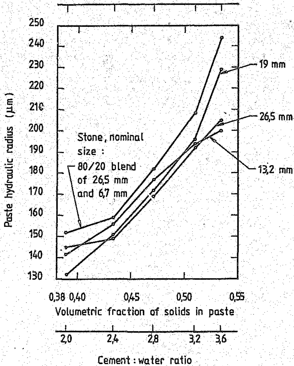
FIGURE 6.16: Paste hydraulic radius versus volumetric fraction of solids in paste for actual mixes; calculated on the basis of cubical particles
