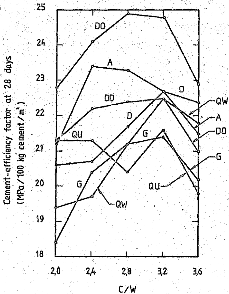
FIGURE 8.36: Cement-efficiency factor at 28 days versus cement:water ratio for concretes made with aggregates of different types (see Figure 8.25 for key)
