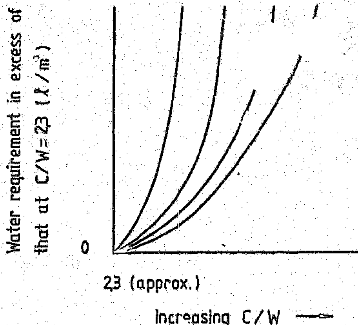
FIGURE 5.2: Shapes of typical curves for water requirement versus cement:water ratio for C/W more than about 2.3
