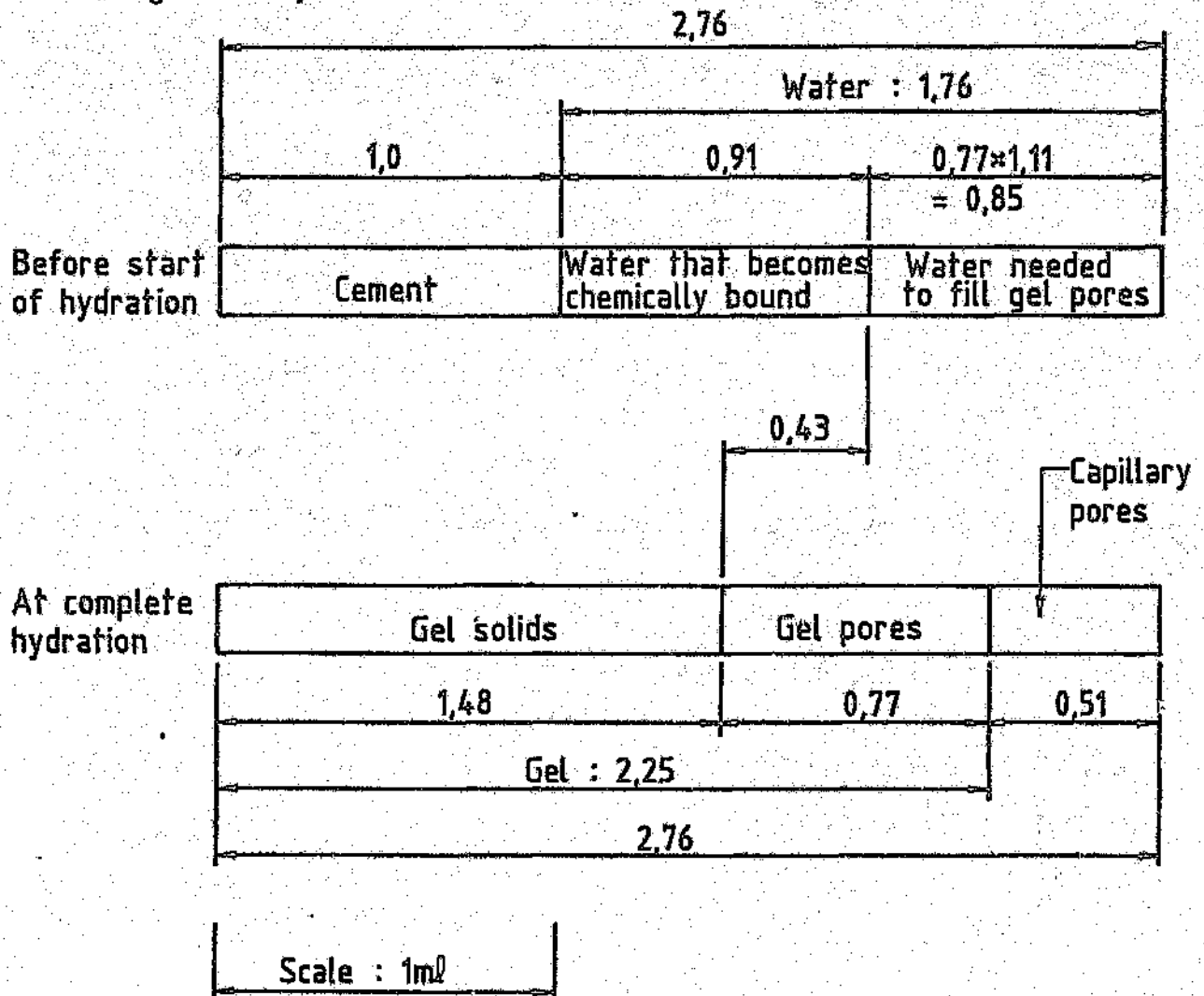
FIGURE 7.8: Calculation of critical cement:water ratio.
