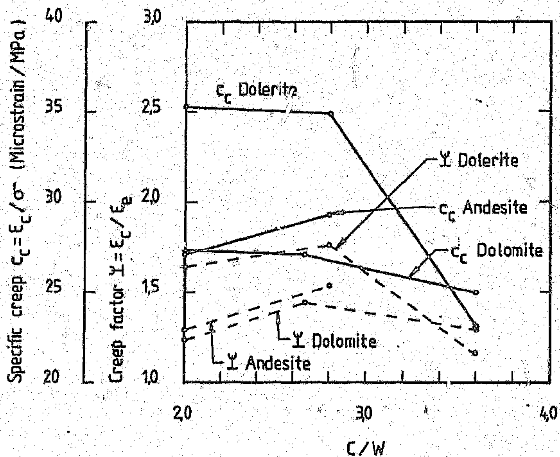
FIGURE 9.5: Specific creep and creep factor at 180 days of loading versus cement:water ratio for concretes made with three different aggregate types
