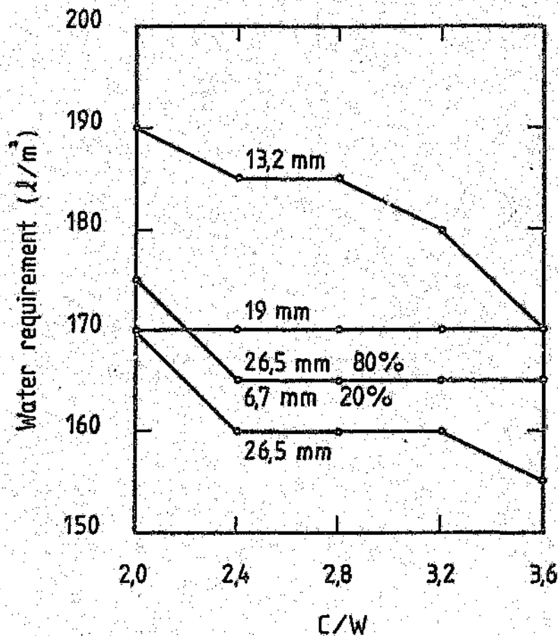
FIGURE 8.2: Water requirement versus cement:water ratio for concrete made with stone of different sizes
