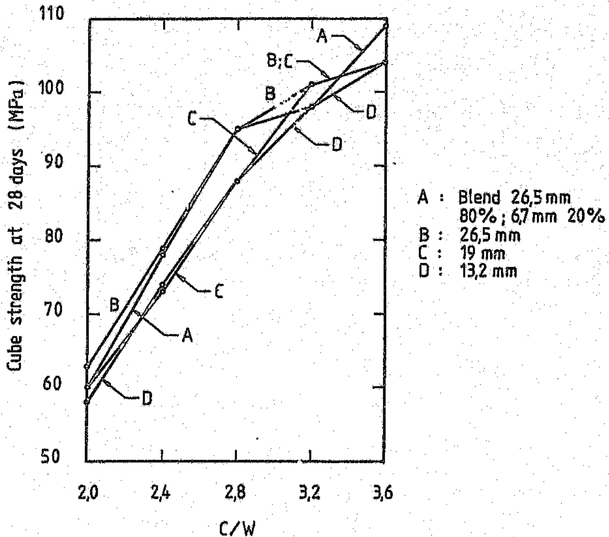
FIGURE 8.4: Cube strength at 28 days versus cement:water ratio for concrete made with stone of different sizes;
