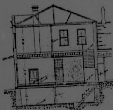
Section from working drawings of D. F. A. building which still exists. The reinforced slab carried printing presses.
