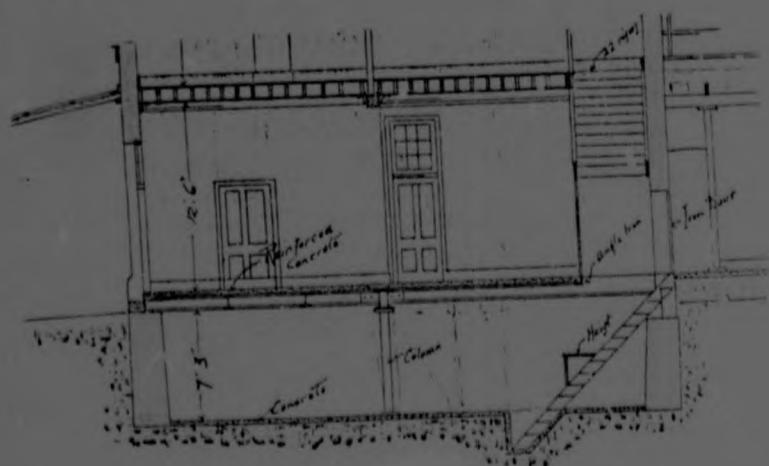
Section from working drawings of D. F. A. building which still exists. The reinforced slab carried printing presses.
