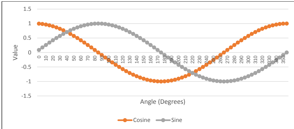
Figure 4.23 Sine – Cosine curves
