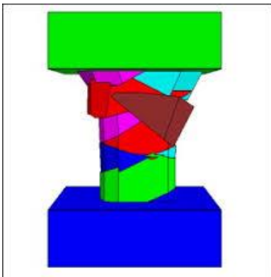
Figure 2.11 Effects of scaling, buckling and spalling on pillars (Pritchard and Hedley, 1993)
