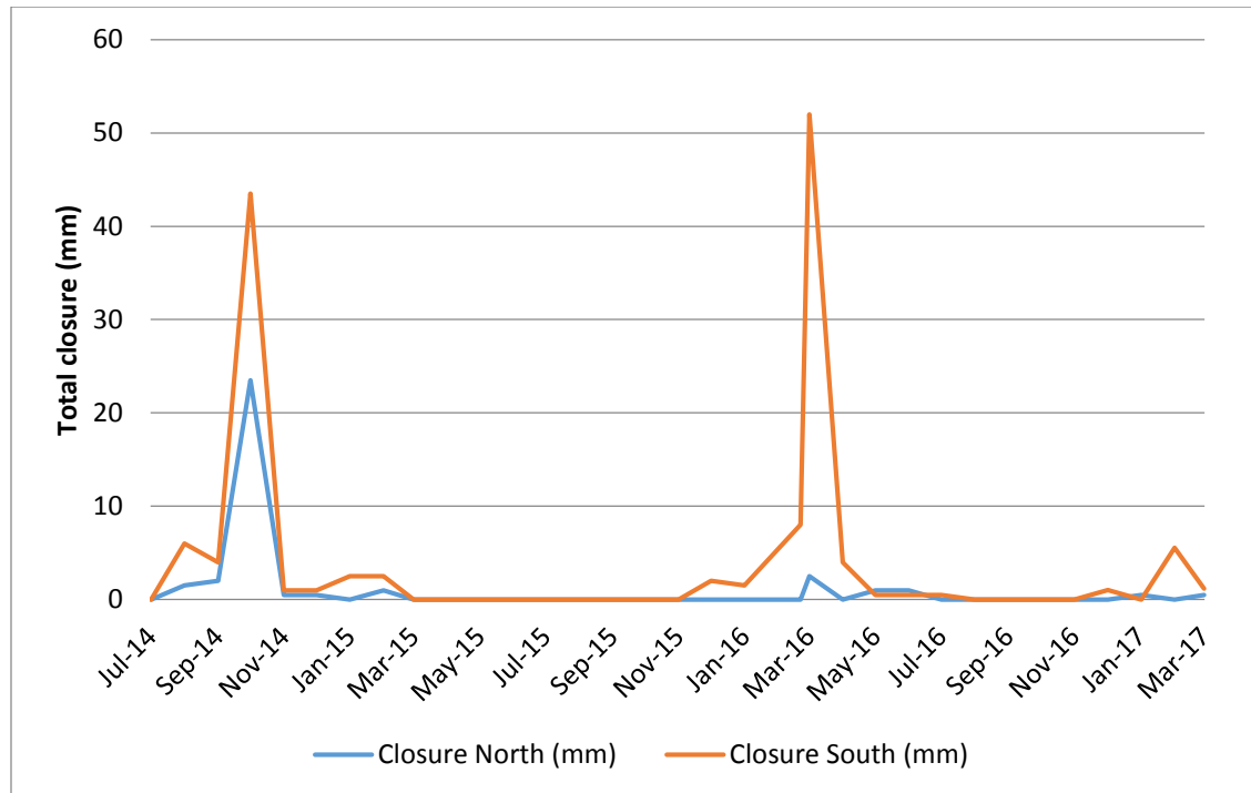
Figure 4.15 Total closure trend.
