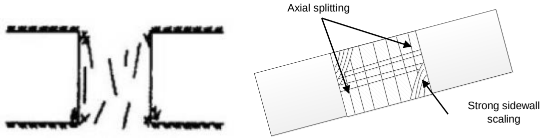
Figure 2.8 Partially failed surface spalling with isolated internal fractures (Brady & Brown, 2005)
