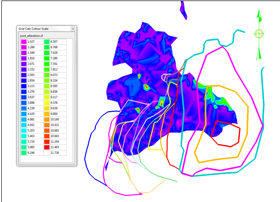
Figure 4.12 Failure migration in relation to joint alteration.
