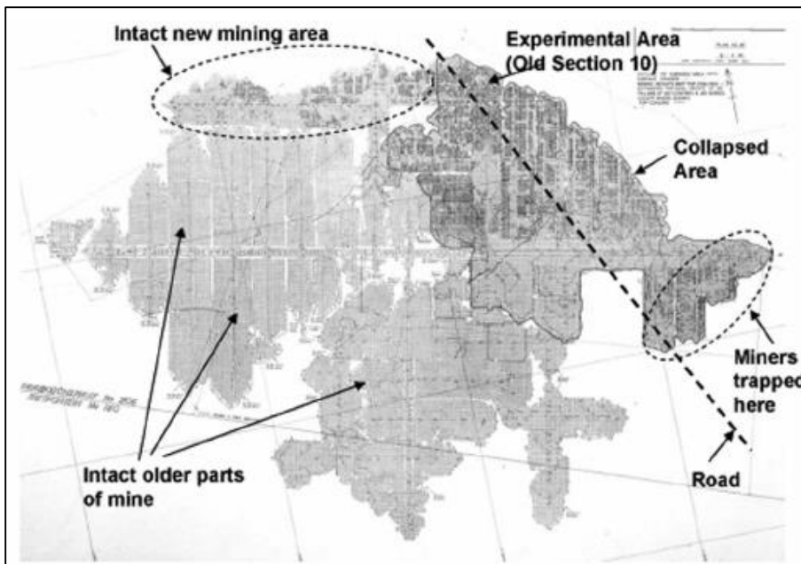
Figure 2.4 Plan of the Coalbrook mine at the time of collapse (Van Der Merwe, 2006)
