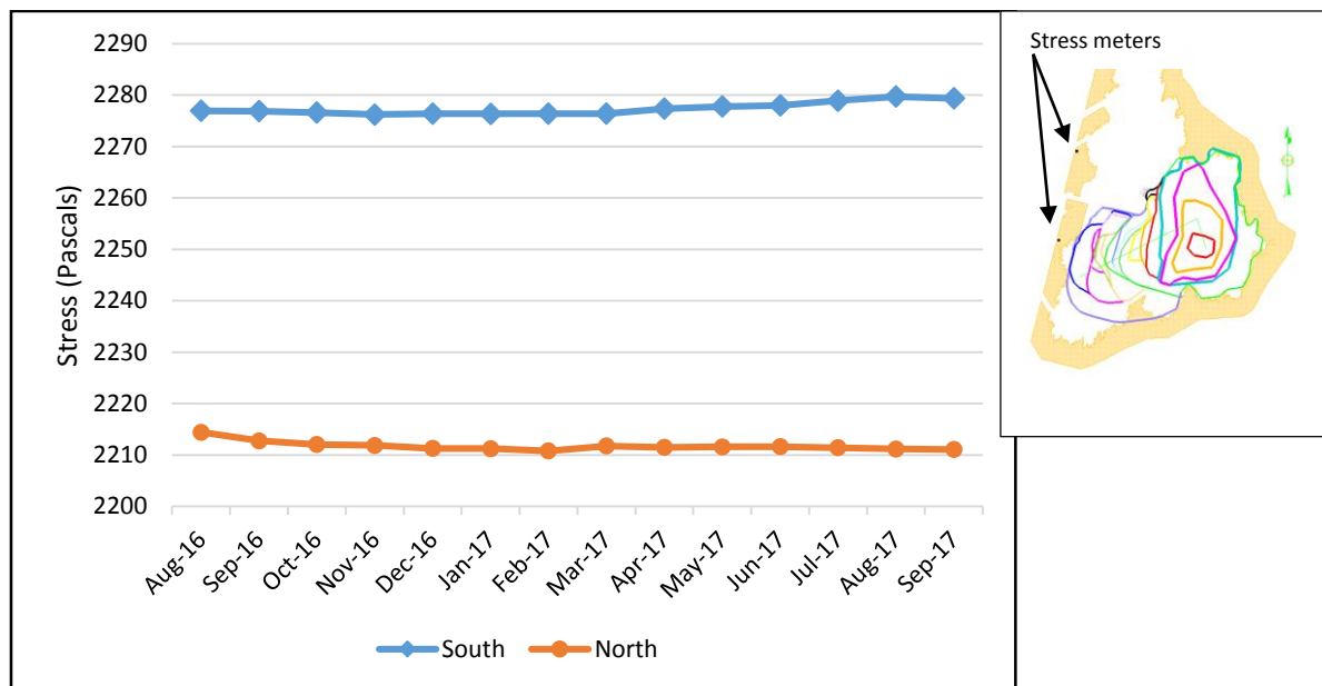
Figure 4.20 Stress meter readings and position of stress meters (insert)
