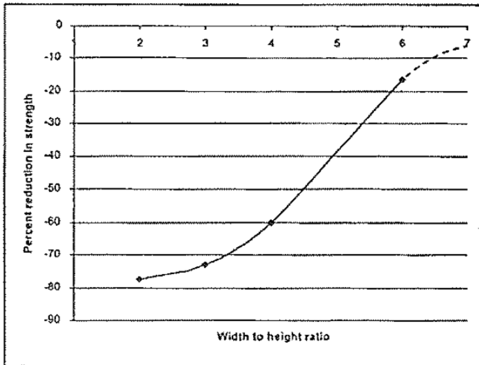
Figure 2.1 Variation of effect of jointing with pillar width to height ratio (Esterhuizen, 2000)
