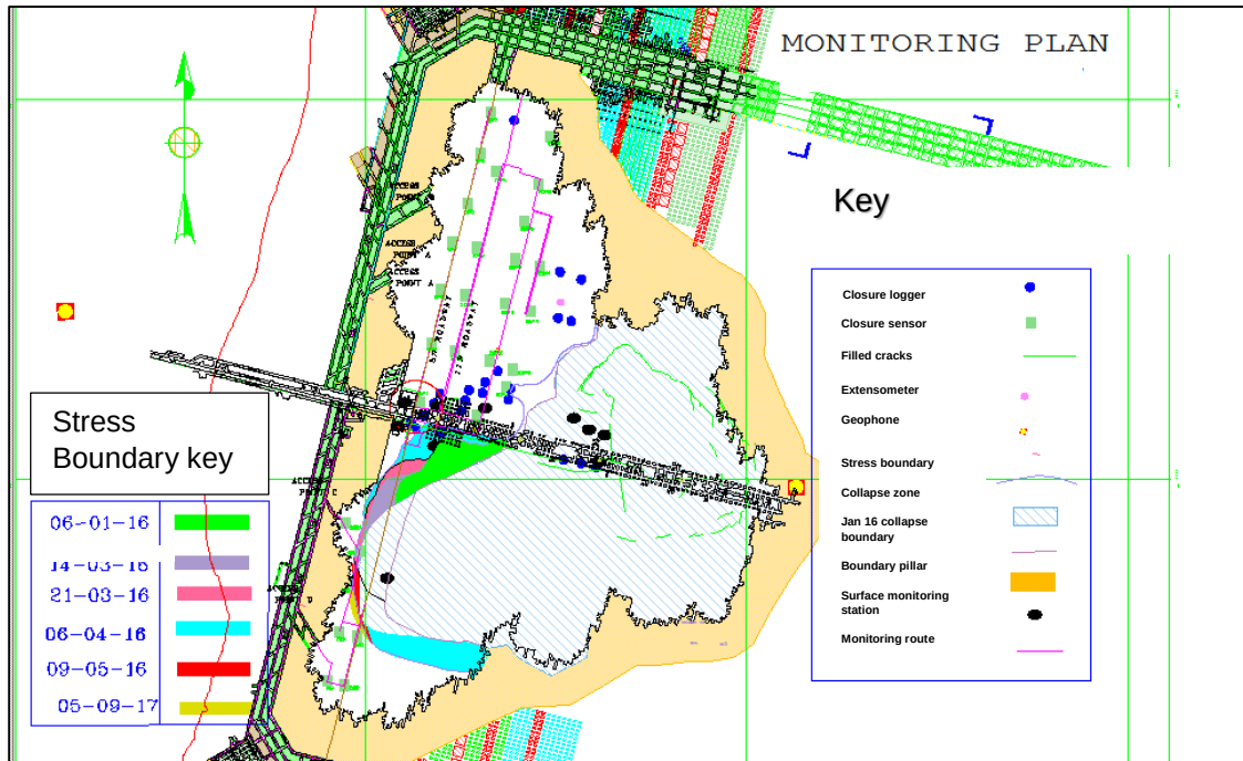
Figure 3.14 Bimha monitoring stations
