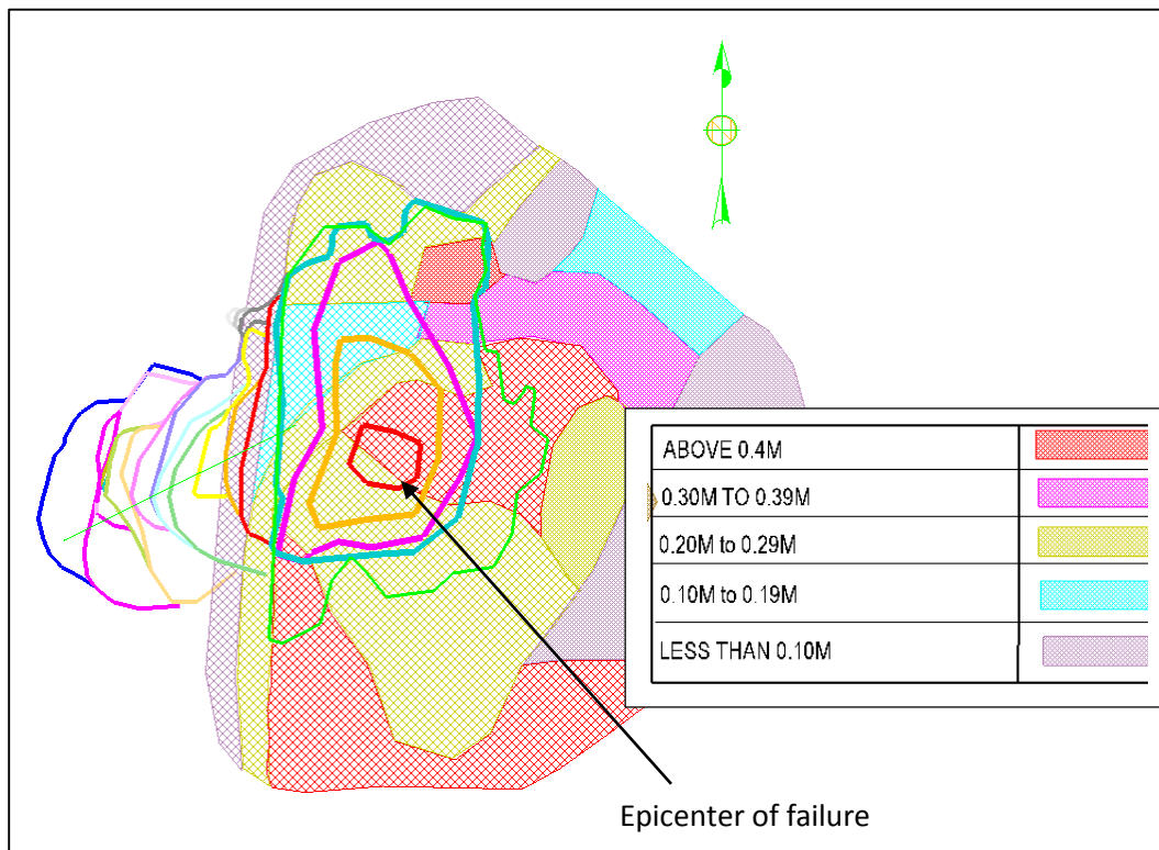
Figure 4.5 Failure migration in relation to Mutambara Shear thickness
