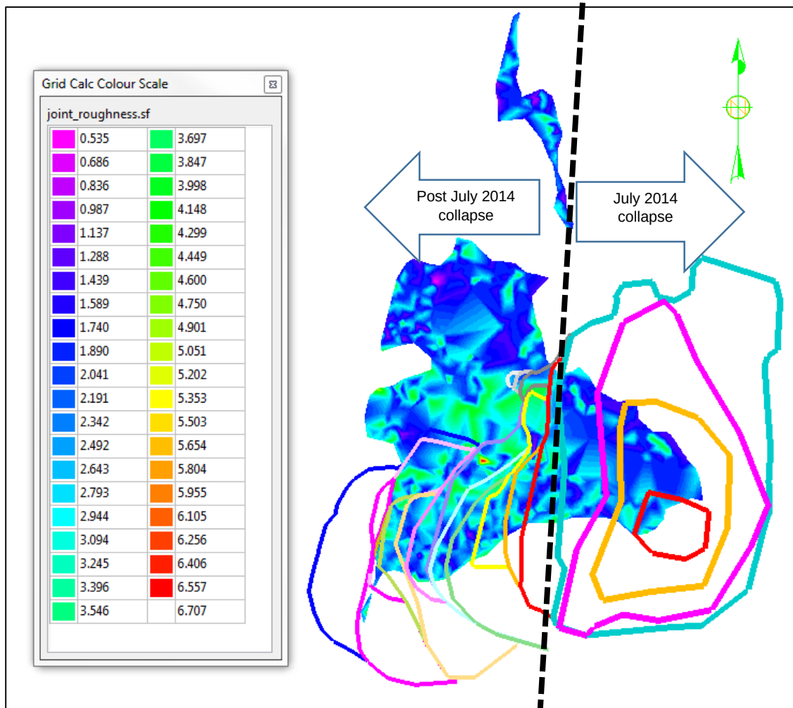
Figure 4.11 Failure migration with respect to joint roughness
