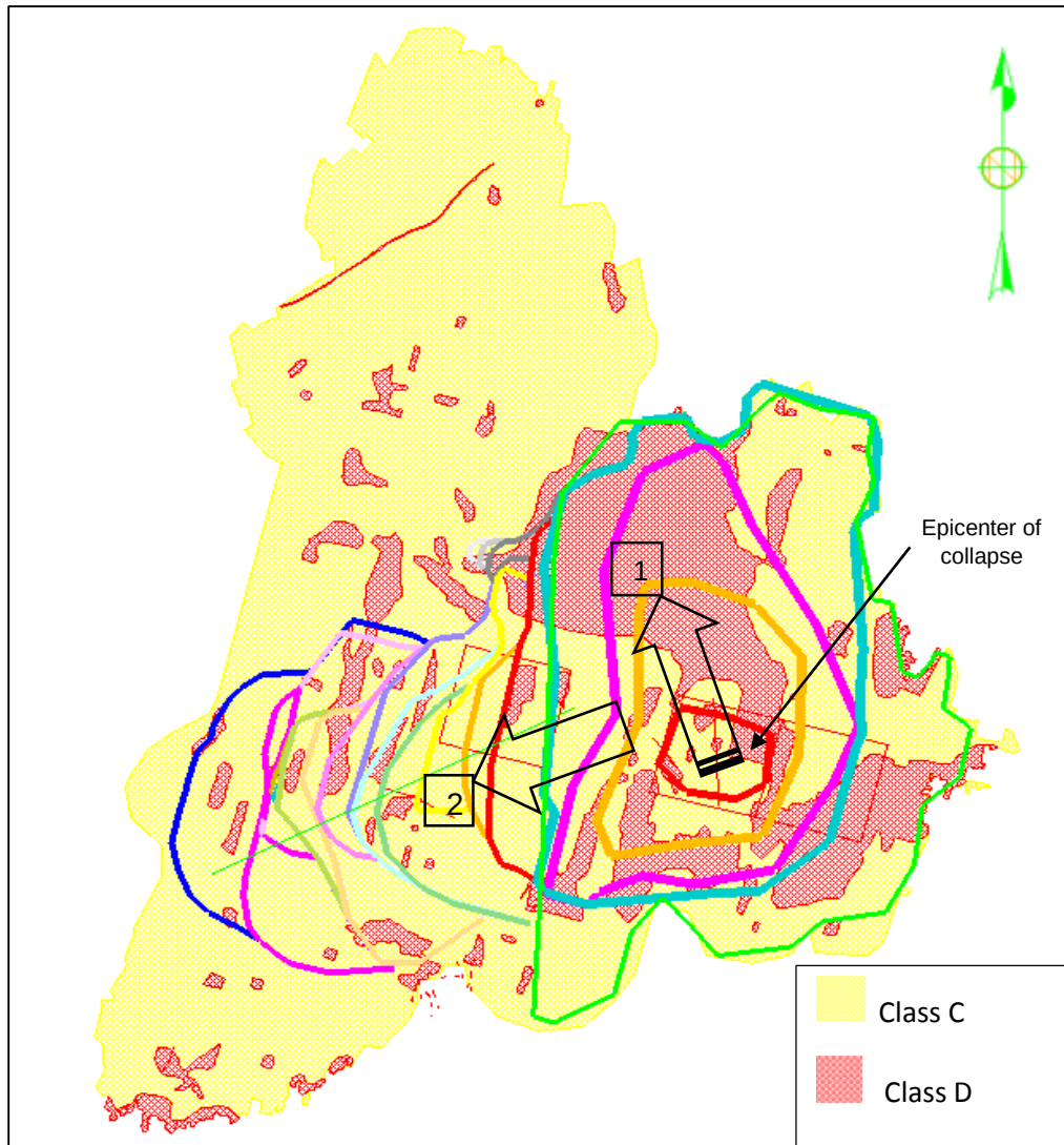
Figure 4.4 Failure migration in relation to very poor ground conditions
