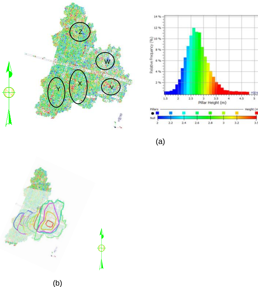
Figure 4.7 Distribution of the pillar sizes a) Distribution of pillar height, b) Pillar height compared to failure direction (Zimplats Internal report (SRK ), 2016a), (Walls & Mpunzi, 2017)
