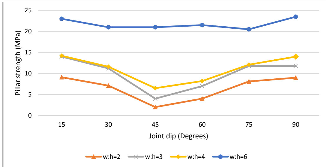
Figure 2.2 Effect of joint dip on pillar strength. (Esterhuizen, 2000)
