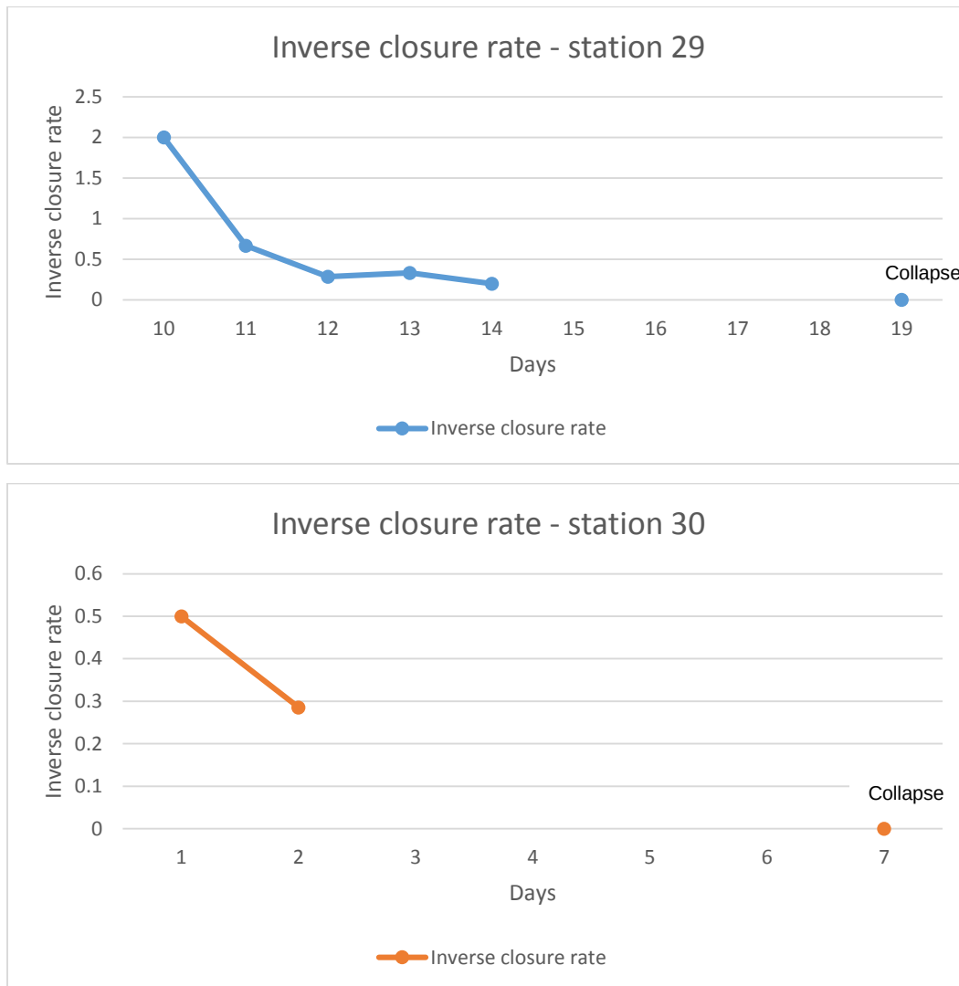
Figure 4.16 Typical inverse closure rates for stations 29 and 30
