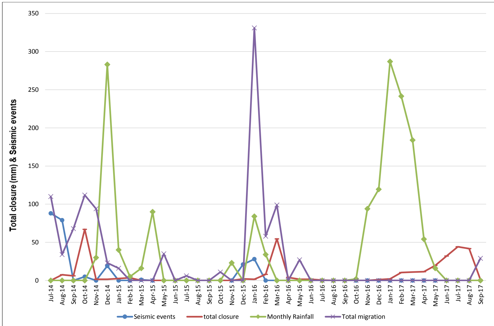
Figure 4.19 Comparison of the Monitoring trends
