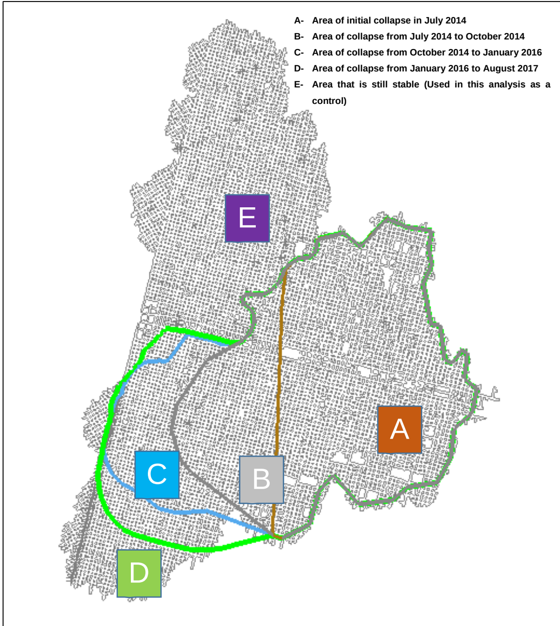
Figure 4.21 Failure areas by period
