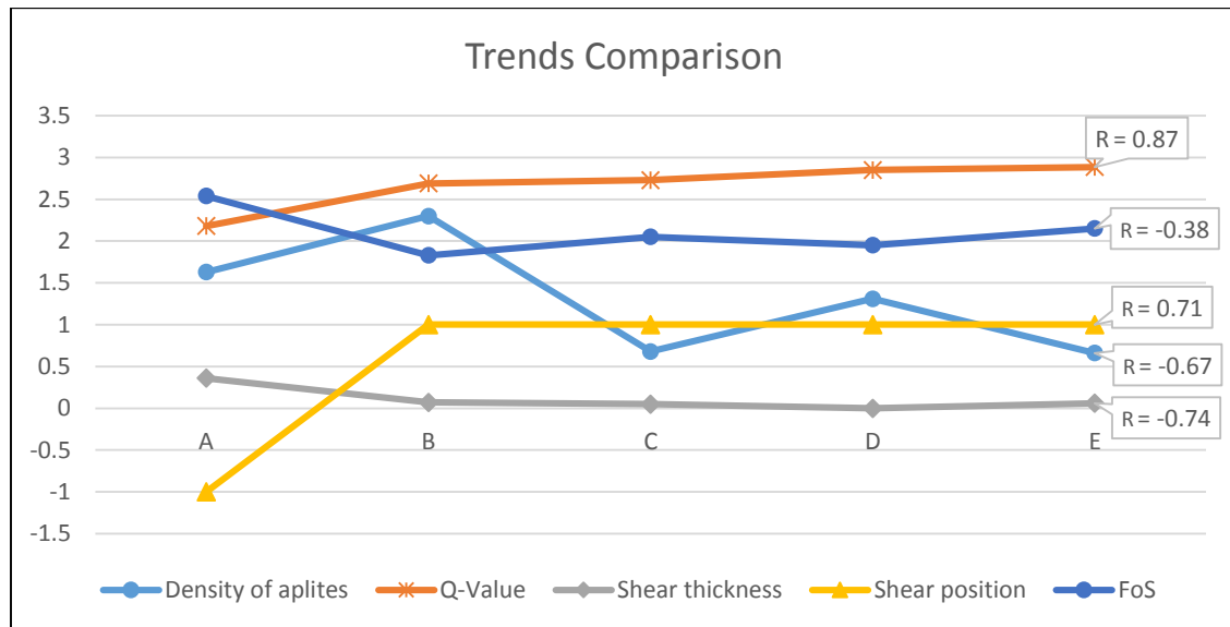
Figure 4.22 Plot of the key variables analysed with respect to the different areas. The correlations are strong except for the Factor of Safety (FoS) which has a low negative correlation of 0.38. These correlations do confirm the key variables that govern the propagation of failure as described in this analysis. Ideally if all the variables are accurately enumerated and incorporated, the FoS should have a high correlation. A low correlation for FoS could be an indication that the design did not accurately consider all the variables.
