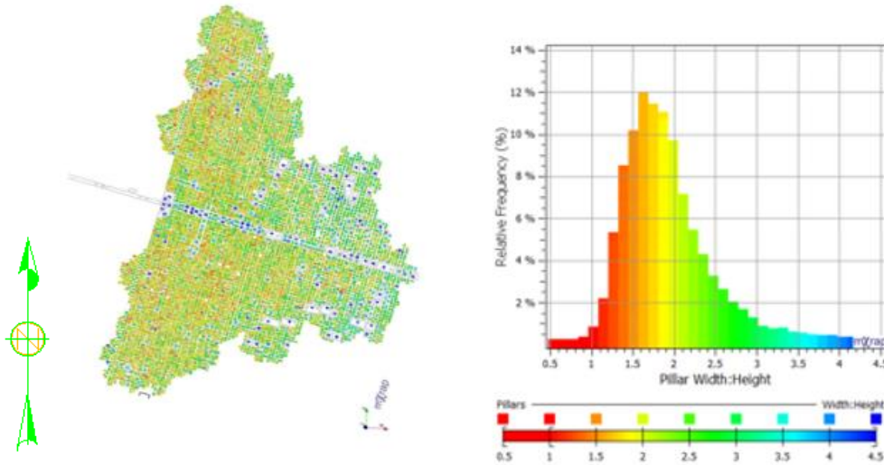
Figure 4.8 Distribution of the w/h ratio (Zimplats Internal report (SRK), 2016a), (Walls & Mpunzi, 2017)
