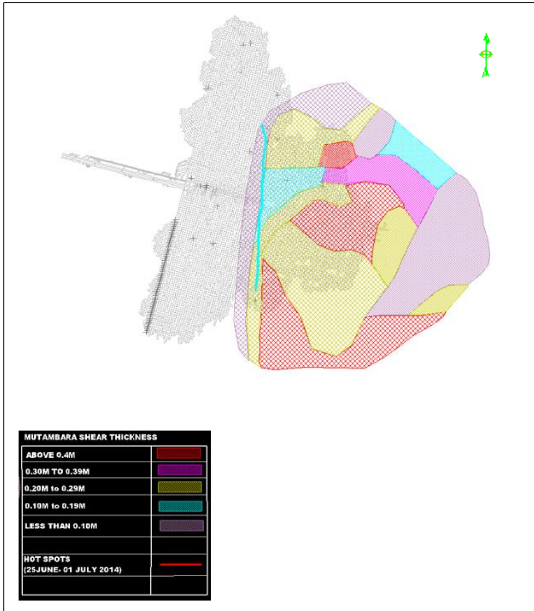
Figure 3.9 Thickness of the Mutambara shear (Zimplats Internal report, 2014)
