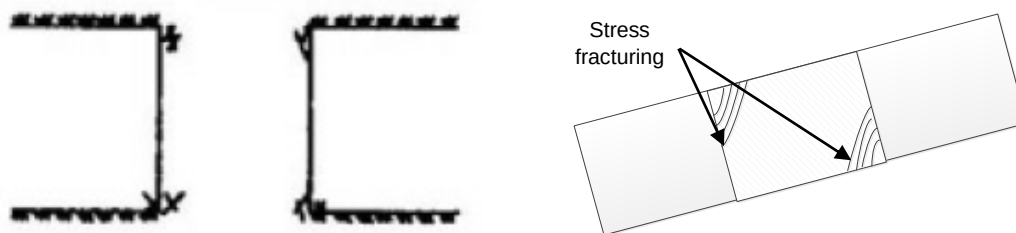
Figure 2.7 Pillar failure modes (Brady & Brown, 2005)
