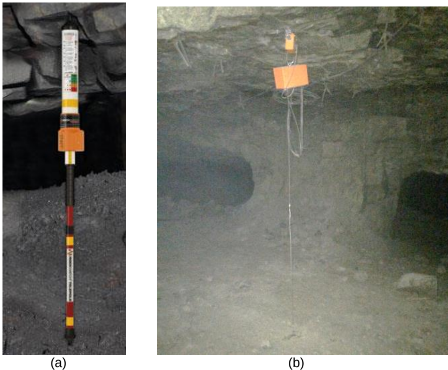
Figure 3.13 Installed closure measuring devices (a) Closure logger, (b) Online closure sensor
