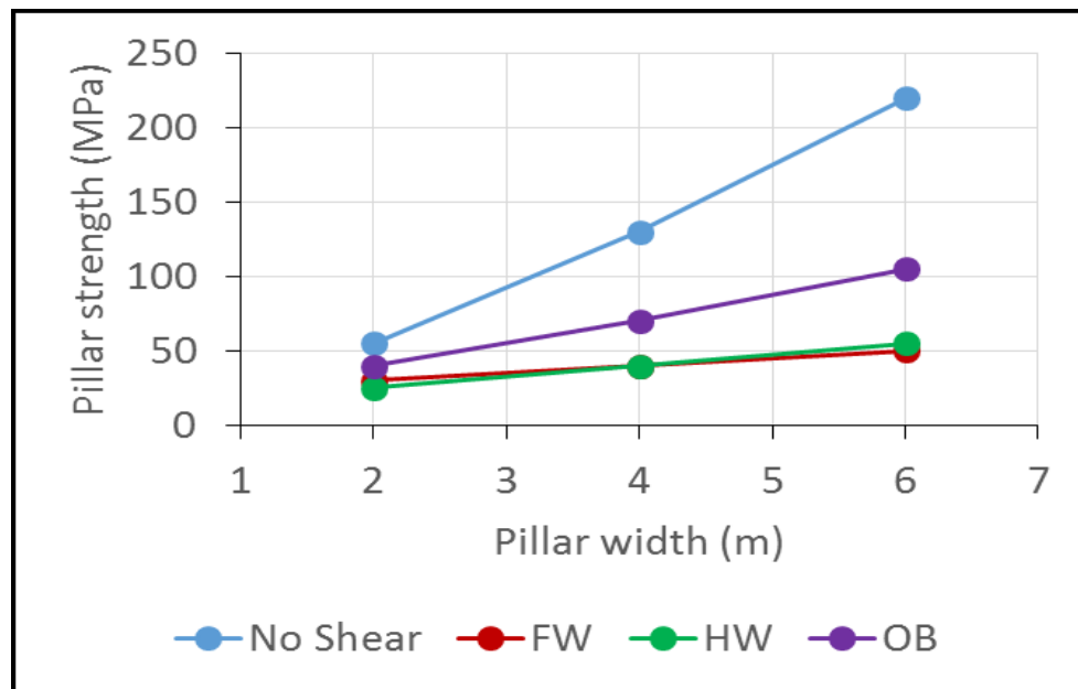
Figure 2.3 Impact of shear on strength and pillar width (Muaka, et al., 2017)
