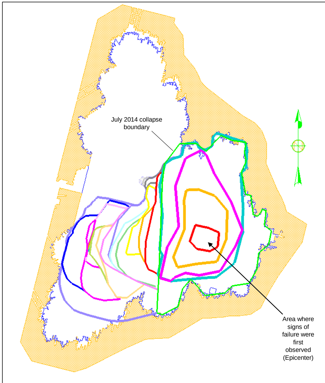
Figure 3.10 Bimha Mine plan showing failure and progression
