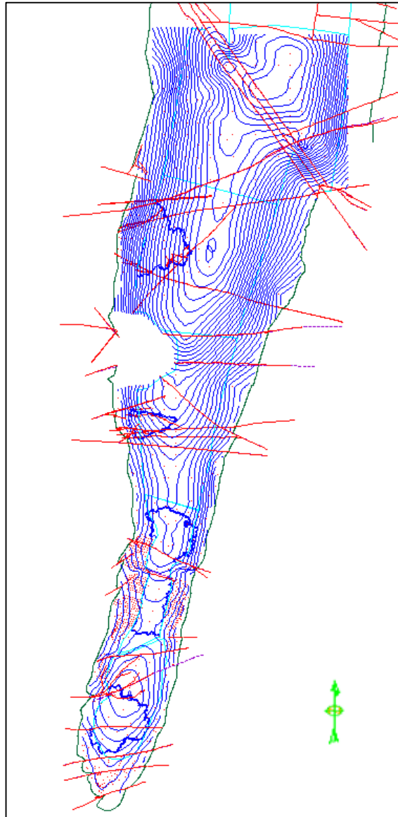
Figure 3.7 Ngezi structural model (Zimplats Internal Report (Kock S.), 2015)
