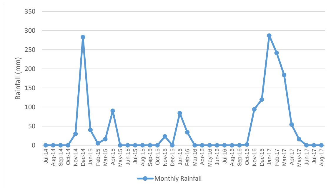
Figure 4.18 Rainfall trend
