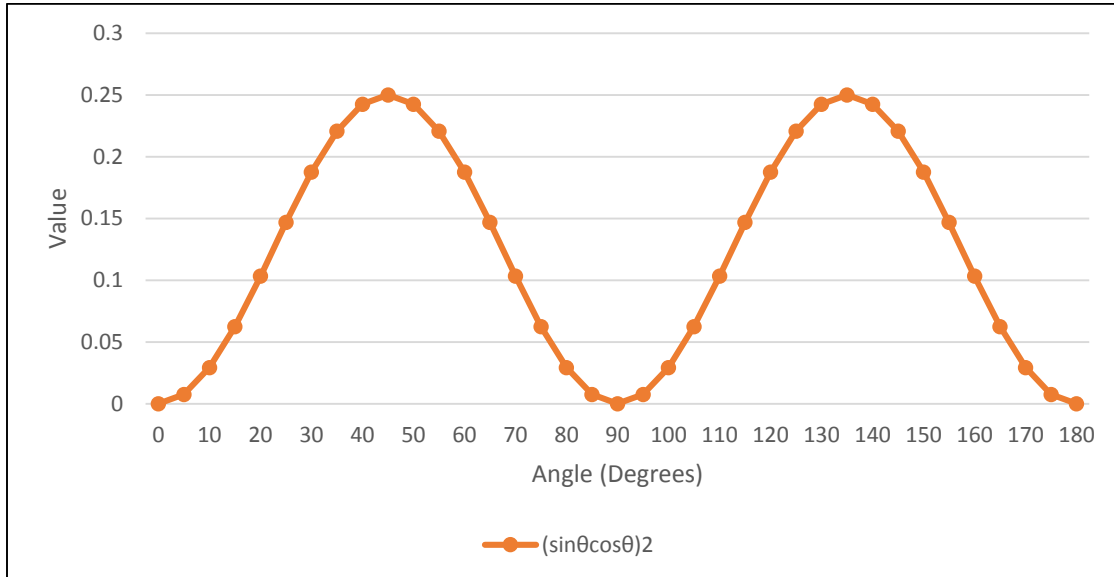
Figure 4.24 Angle difference (\sin\theta\cos\theta)^2 curve
