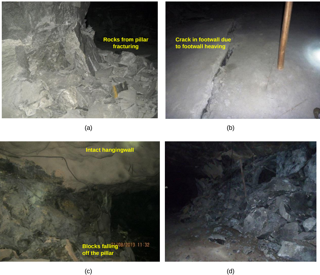
Figure 3.11 Stages of rock mass failure (a) Stress fracturing, (b) Footwall heaving, (c) Intermediate stage, (d) Hangingwall collapse stage
