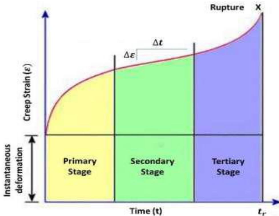
Figure 2.5 Idealised creep curve (Khoshboresh, 2013).
