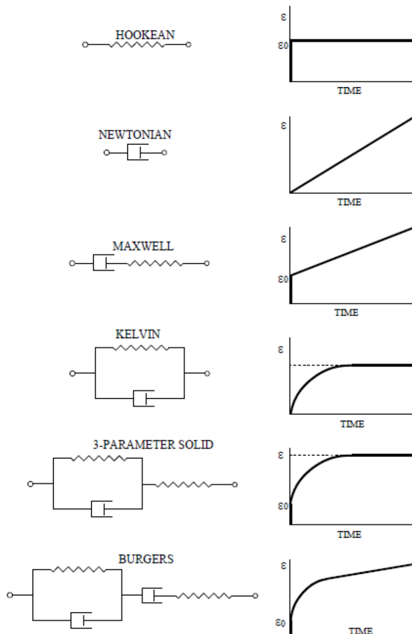
Figure 2.6 Commonly used viscoelastic models and their respective strain-time behaviour for a stepwise application of constant stress adapted from (Ryder & Jager, 2002)
