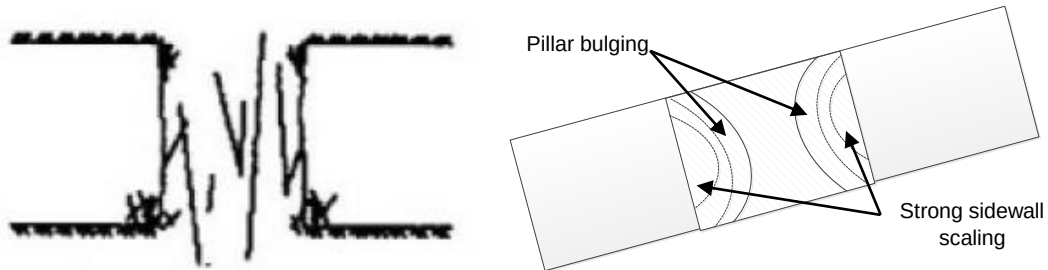
Figure 2.9 Partially failed contacts with extensive internal fractures (Brady & Brown, 2005)
