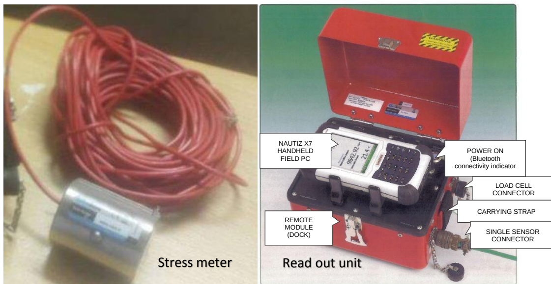
Figure 3.12 Stress meter and read out unit
