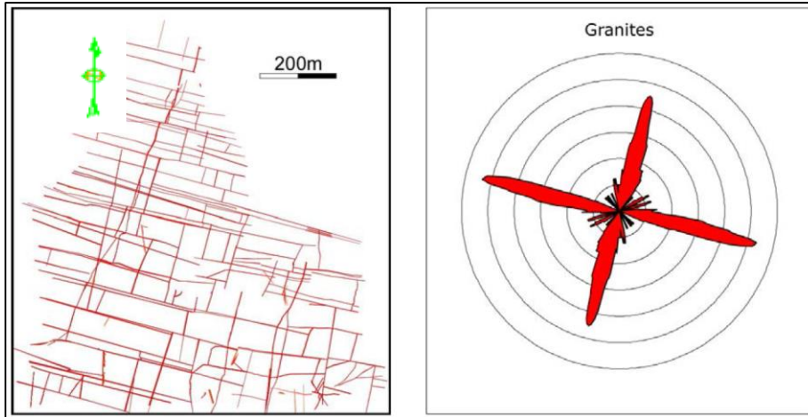
Figure 3.5 Typical orthogonal network of granite dykes as mapped in Bimha north. With the equal area rose diagram of the strikes. (Blenkinsop, 2014)
