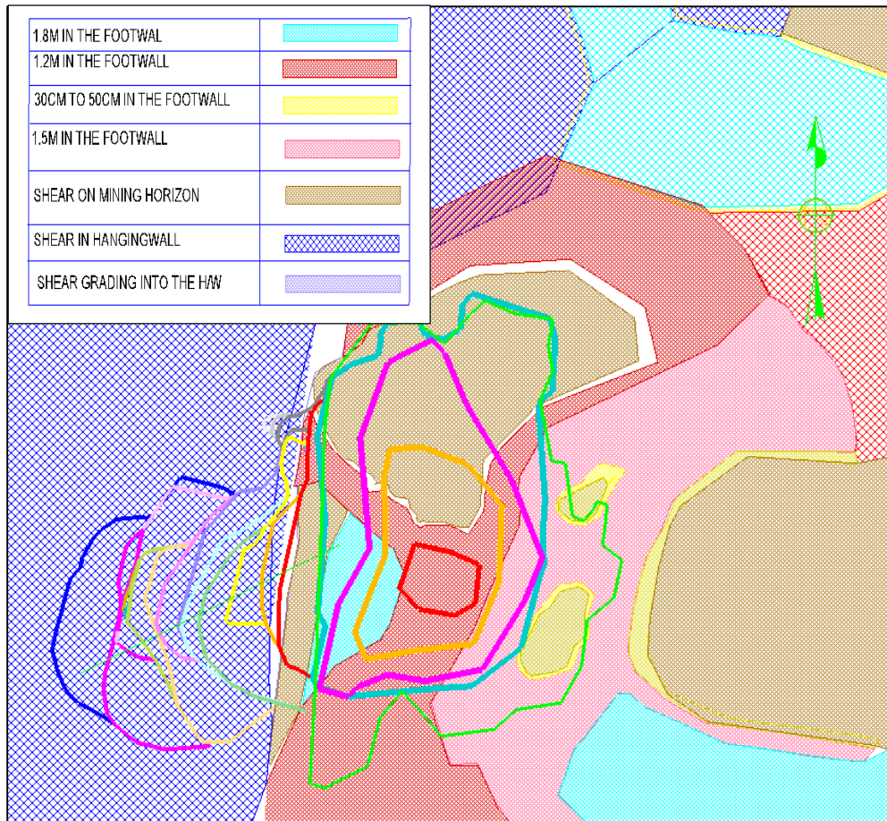
Figure 4.6 Failure migration in relation to the position of the shear
