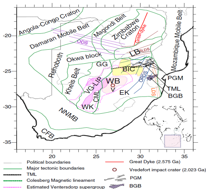
Figure 3.6 General stratigraphy of Southern Africa (Youssof et al, 2013)
