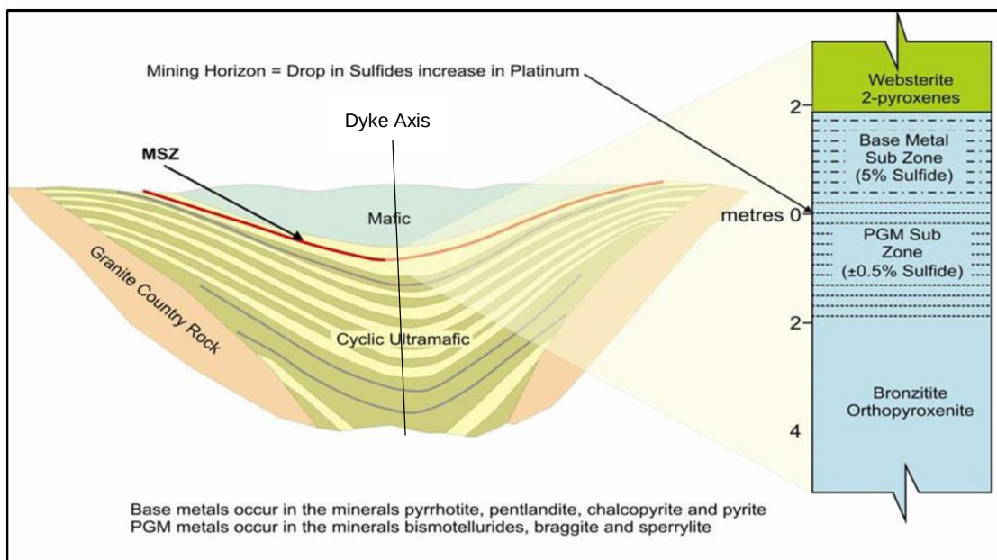
Figure 3.2 Generalised geological succession (Walls & Mpunzi, 2017)
