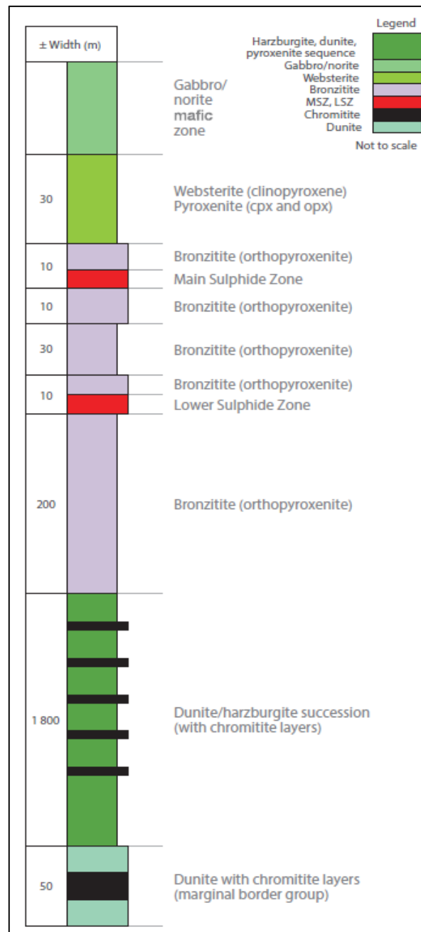
Figure 3.3 Detailed geological succession of the Great Dyke (Zimplats, 2017)
