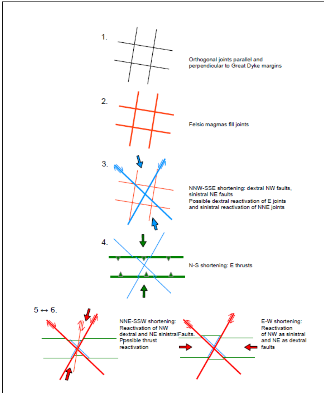
Figure 3.4 Post Great Dyke tectonic history in Ngezi area. (Blenkinsop, 2014)
