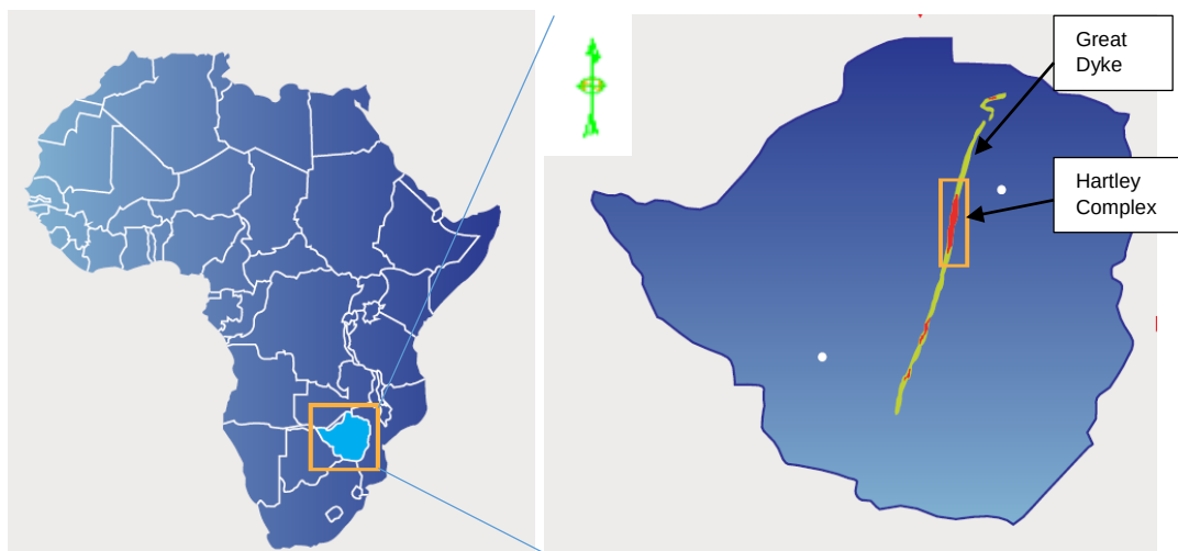
Figure 3.1 Location of the Great Dyke on the Zimbabwean craton (Zimplats, 2017).
