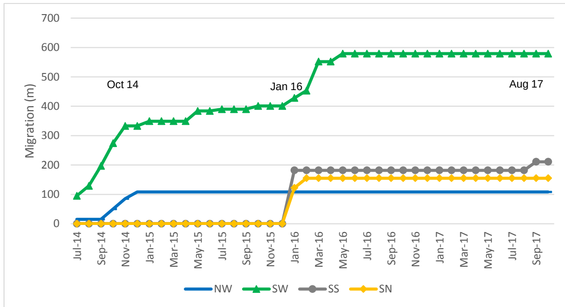
Figure 4.14 Cumulative stress migration curve
