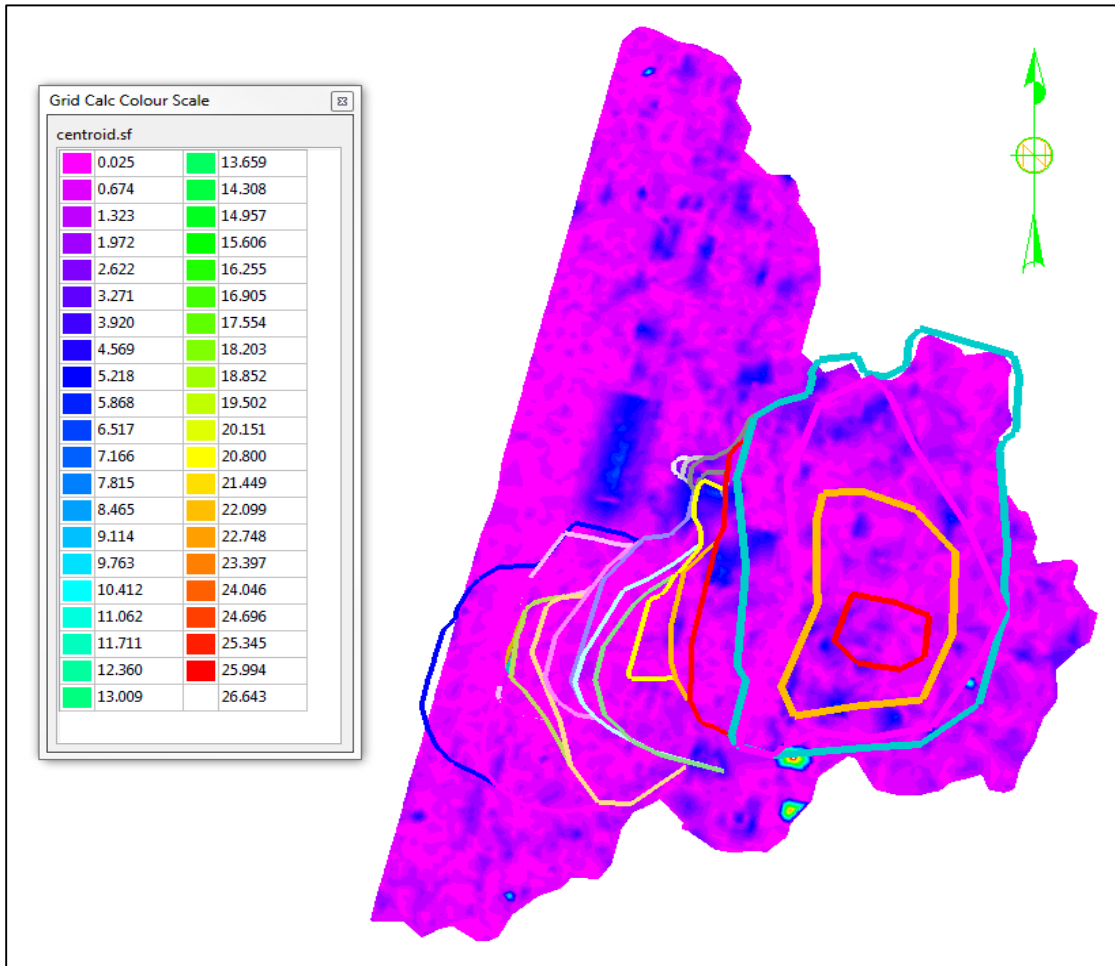
Figure 4.10 Pillar position with respect to design.
