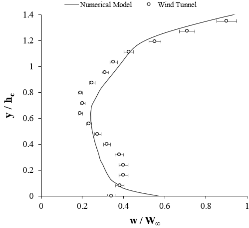
Figure 4.14: Numerical model and wind tunnel test normalised axial velocity distribution along height of car for partial wheel fairing configuration
