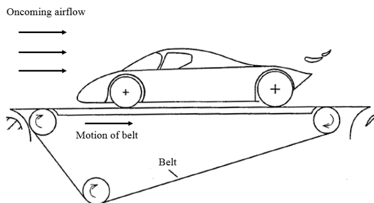
Figure 2.7: Rolling road setup in wind tunnel, illustrated by Katz [16]
