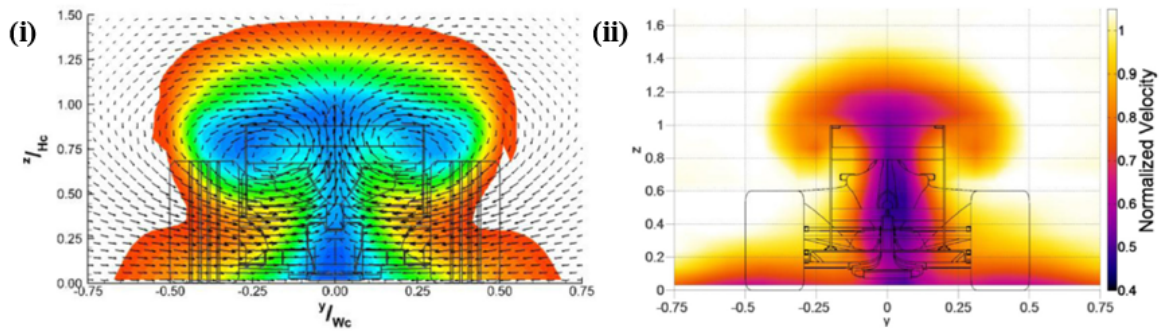
Figure 1.6: 'Mushroom-like' wake structure as found by Newbon et al. [10] (i) and Watts and Watkins [9] (ii)
