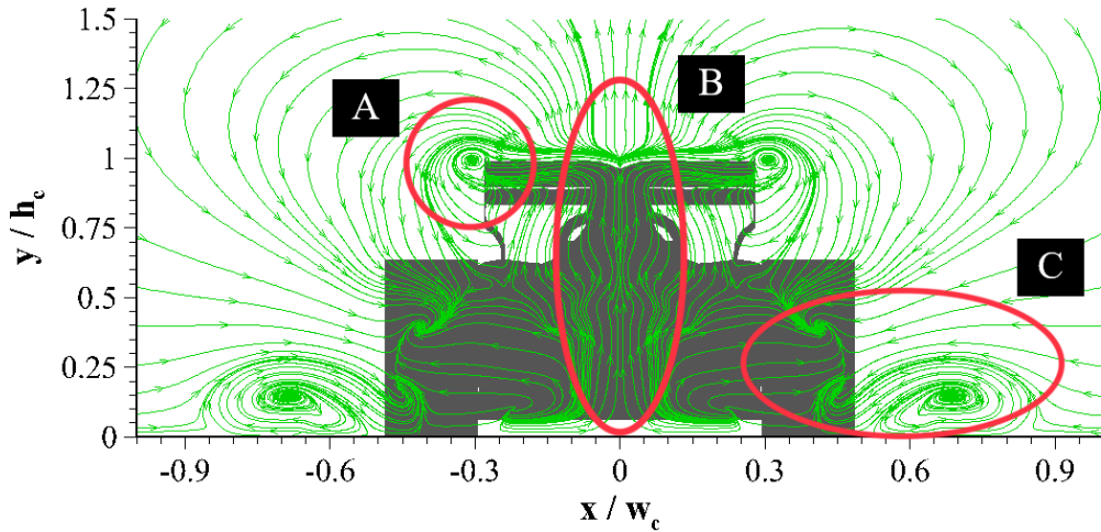
Figure 5.4: Full size planar streamtraces for no wheel fairings at z = 0.0L
