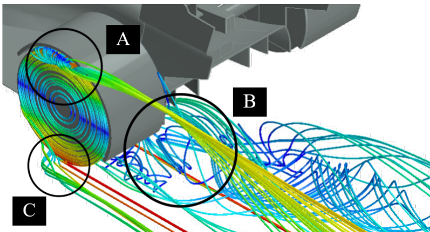
Figure 5.34: Streamlines at rear wheel for partial wheel fairings
