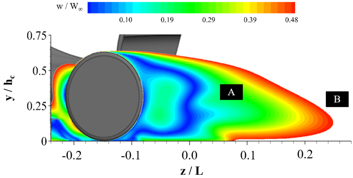
Figure 5.29: Normalised axial velocity contours in wheel midplane for no wheel fairings
