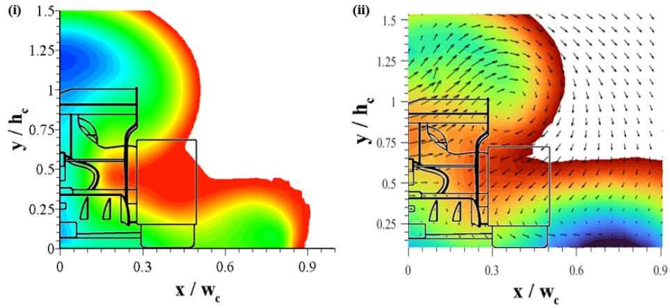
Figure A.4: Scale model normalised axial velocity contours for partial wheel fairings at z = 1.0L for CFD (i) and wind tunnel (ii) tests
