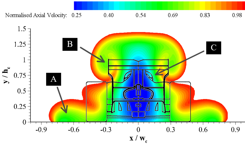
Figure 5.9: Full size normalised axial velocity contours for no wheel fairings at z = 0.5L
