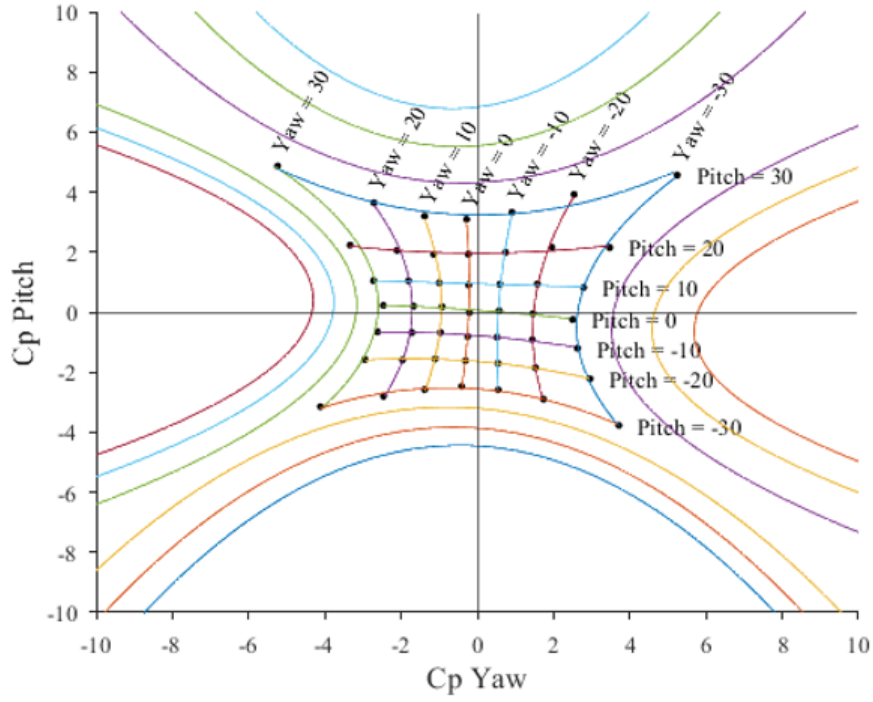
Figure 3.20: Carpet map of calibration data showing lines of constant pitch and yaws angles
