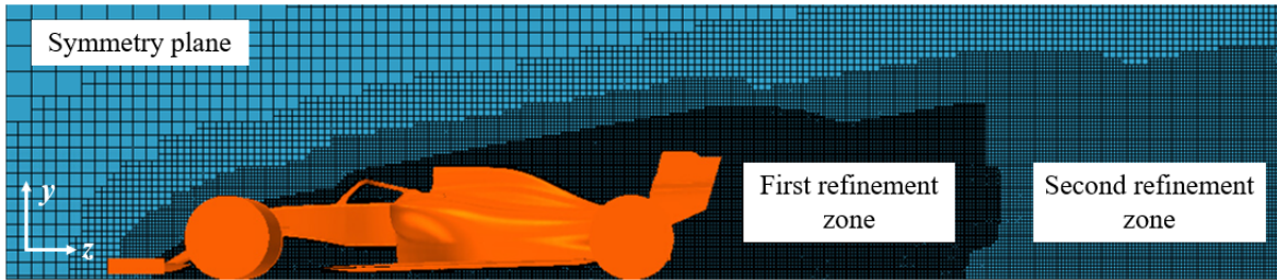
Figure 3.10: Refinement zones for volume mesh
