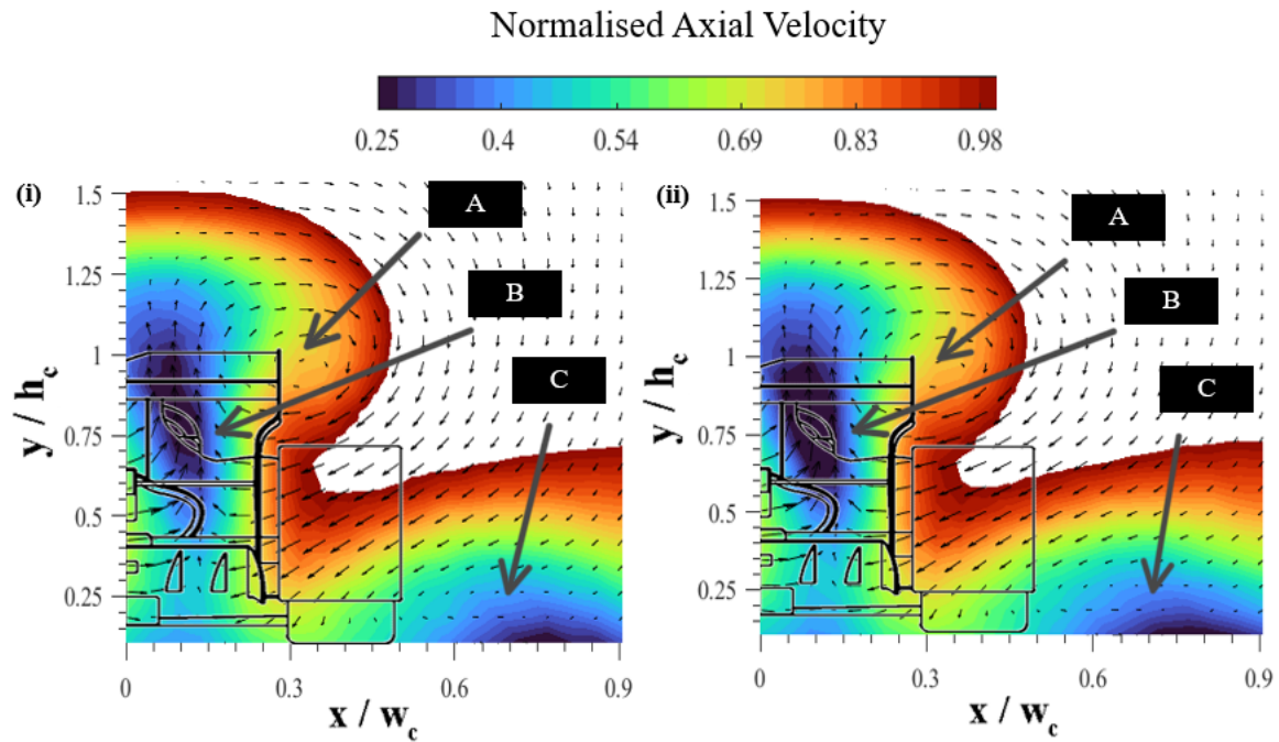
Figure 4.7: Repeatability of scale model normalised axial velocity contours for full wheel fairings at z = 0.5L for wind tunnel tests
