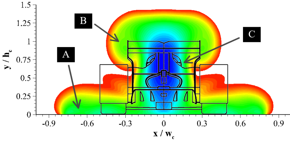
Figure 5.10: Full size normalised axial velocity contours for partial wheel fairings at z = 0.5L
