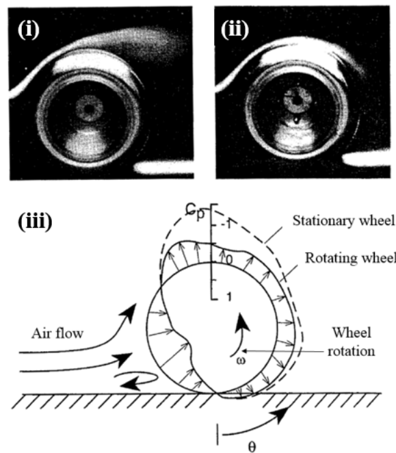
Figure 2.4: Flow visualisation showing separation over rotating (i) and non-rotating wheels (ii), with associated pressure coefficient distributions (iii) [16]
