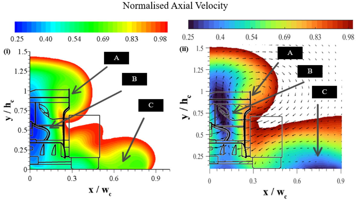
Figure 4.11: Scale model normalised axial velocity contours for partial wheel fairings at z = 0.5L for CFD (i) and wind tunnel (ii) tests
