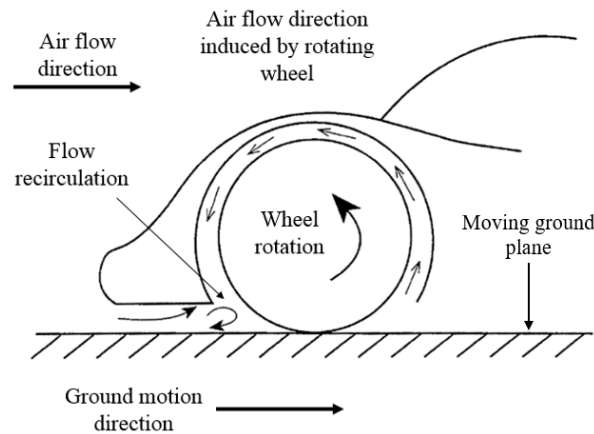
Figure 2.5: Airflow for covered wheels [16]
