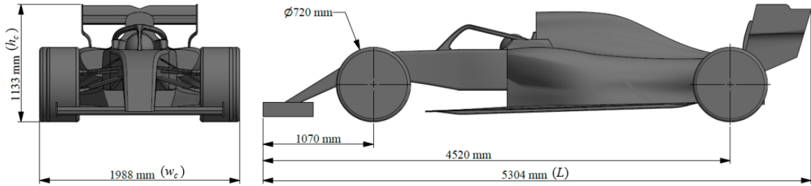
Figure 3.2: Formula One car used for study, with full size dimensions
