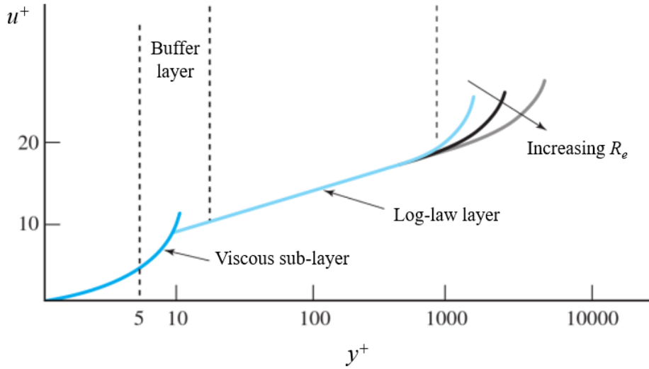
Figure 2.11: Dimensionless velocity u^+ distribution as a function of dimensionless wall distance y^+ for a turbulent boundary layer [24]
