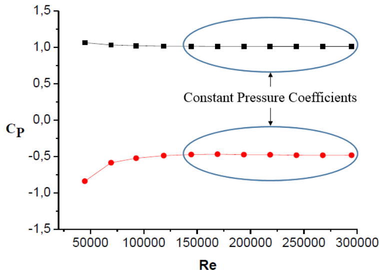
Figure 2.10: Reynolds number independence for pressure coefficients of a truck as shown by Bayındırlı [46]
