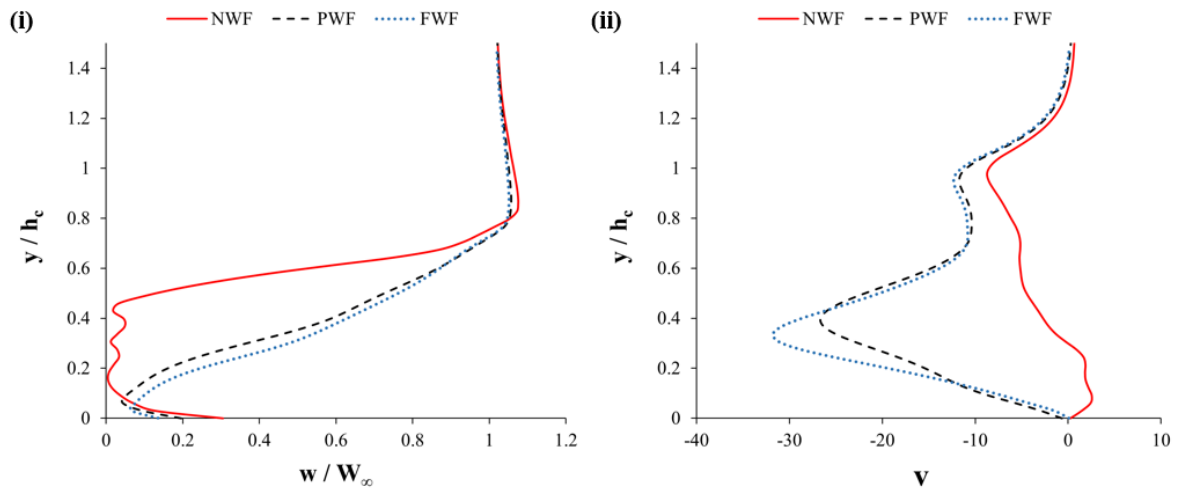
Figure 5.8: Normalised axial velocity (i) and upwash/downwash component (ii) at centreline of wheel in z = 0.0L plane
