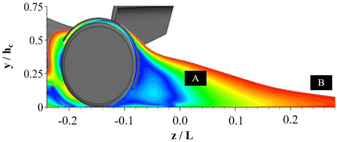
Figure 5.30: Normalised axial velocity contours in wheel midplane for partial wheel fairings
