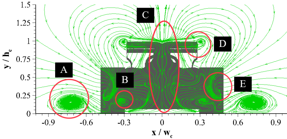
Figure 4.18: Scale model planar streamtraces for no wheel fairings at z = 0.0L for non-rotating wheels
