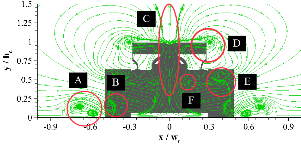
Figure 4.19: Scale model planar streamtraces for no wheel fairings at z = 0.0L for rotating wheels
