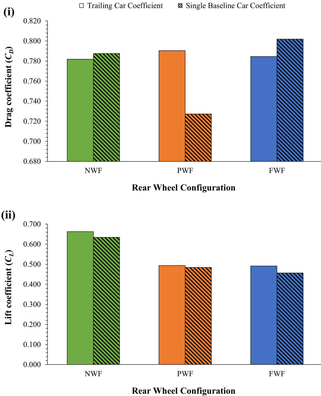
Figure 5.39: Comparison of (i) drag coefficients and (ii) lift coefficients for all configurations at trailing position D
