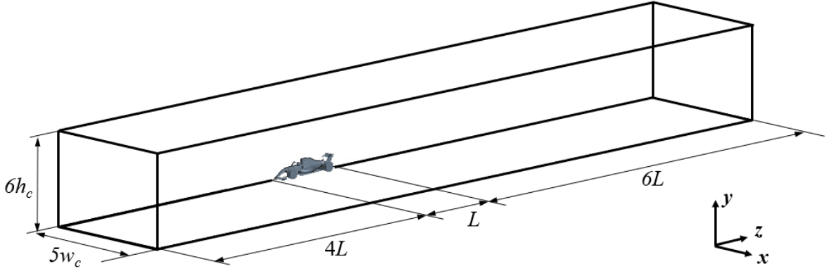
Figure 3.5: Numerical model domain dimensions
