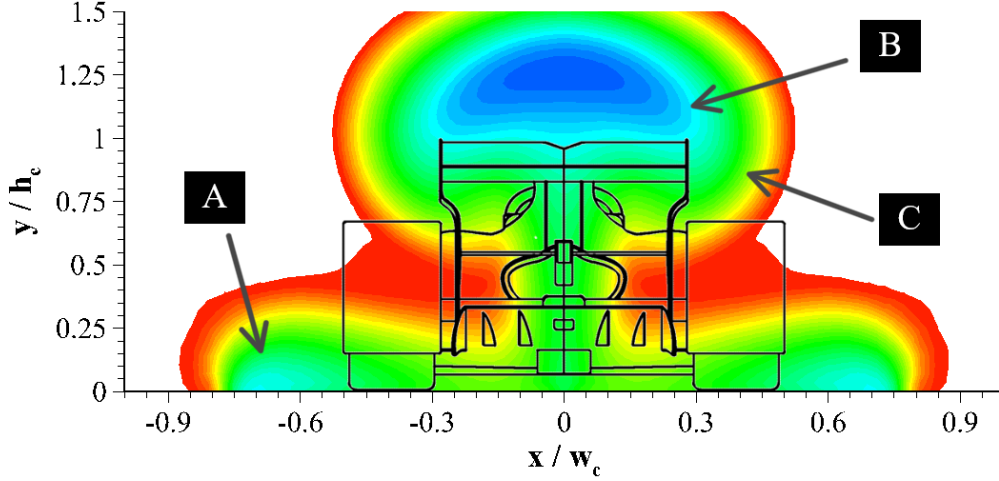
Figure 5.19: Full size normalised axial velocity contours for full wheel fairings at z = 1.0L
