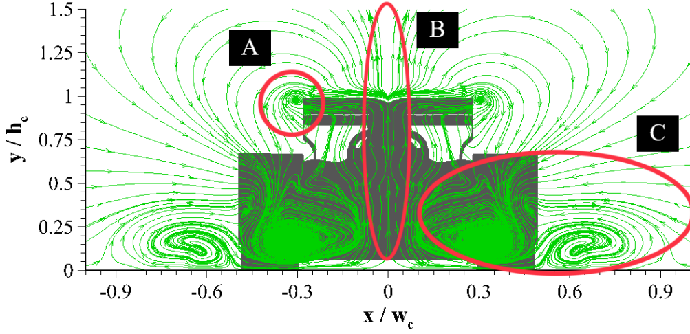
Figure 5.5: Full size planar streamtraces for partial wheel fairings at z = 0.0L
