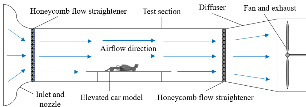
Figure 3.12: Side view of wind tunnel setup (not to scale)
