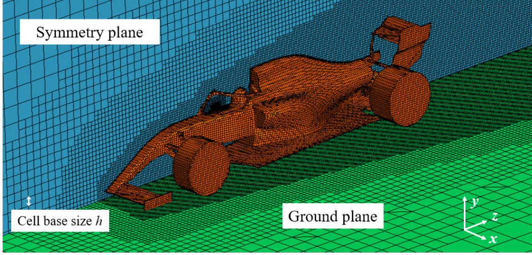
Figure 3.9: Volume mesh of numerical model composed of hexahedral cells
