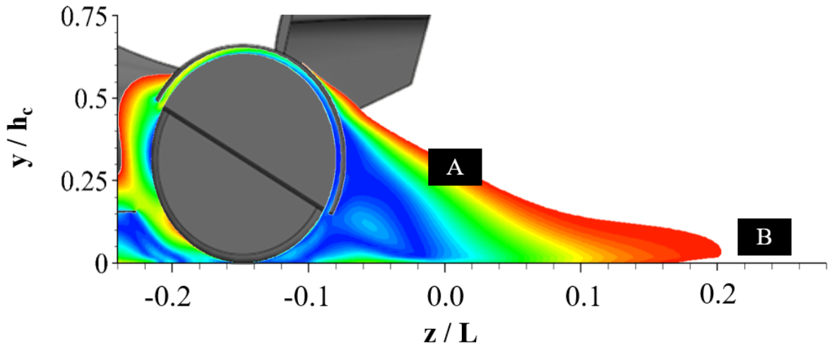
Figure 5.31: Normalised axial velocity contours in wheel midplane for full wheel fairings
