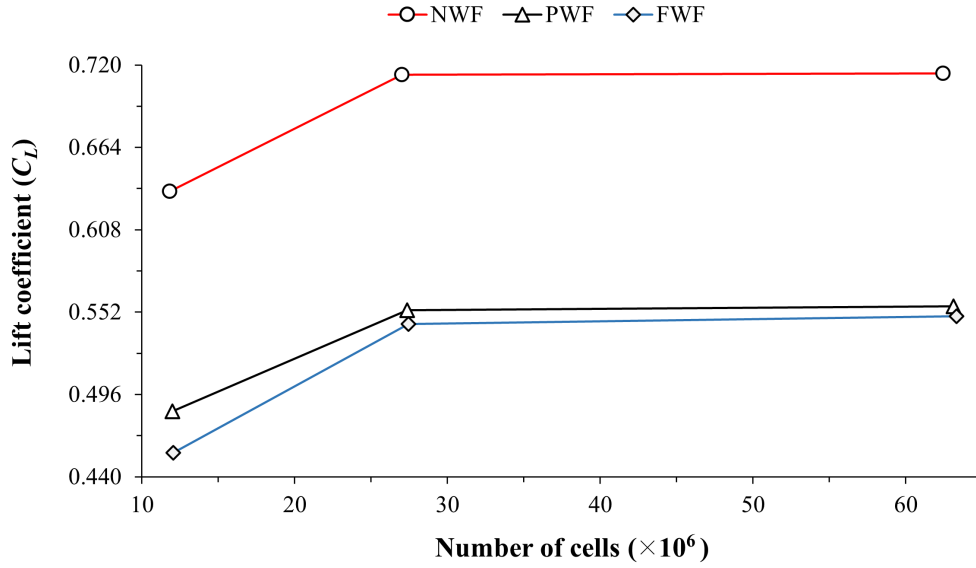
Figure 4.4: Converged lift coefficient value of car versus number of mesh cells
