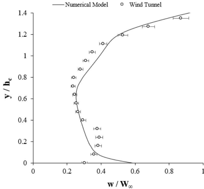
Figure 4.13: Numerical model and wind tunnel test normalised axial velocity distribution along height of car for no wheel fairing configuration
