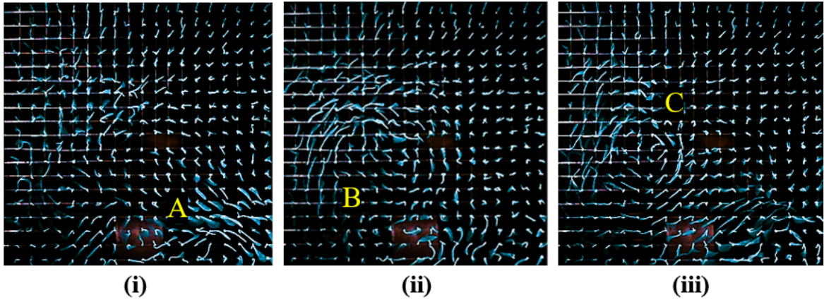
Figure A.1: Flow visualisation for partial wheel fairings at z = 0.5L
