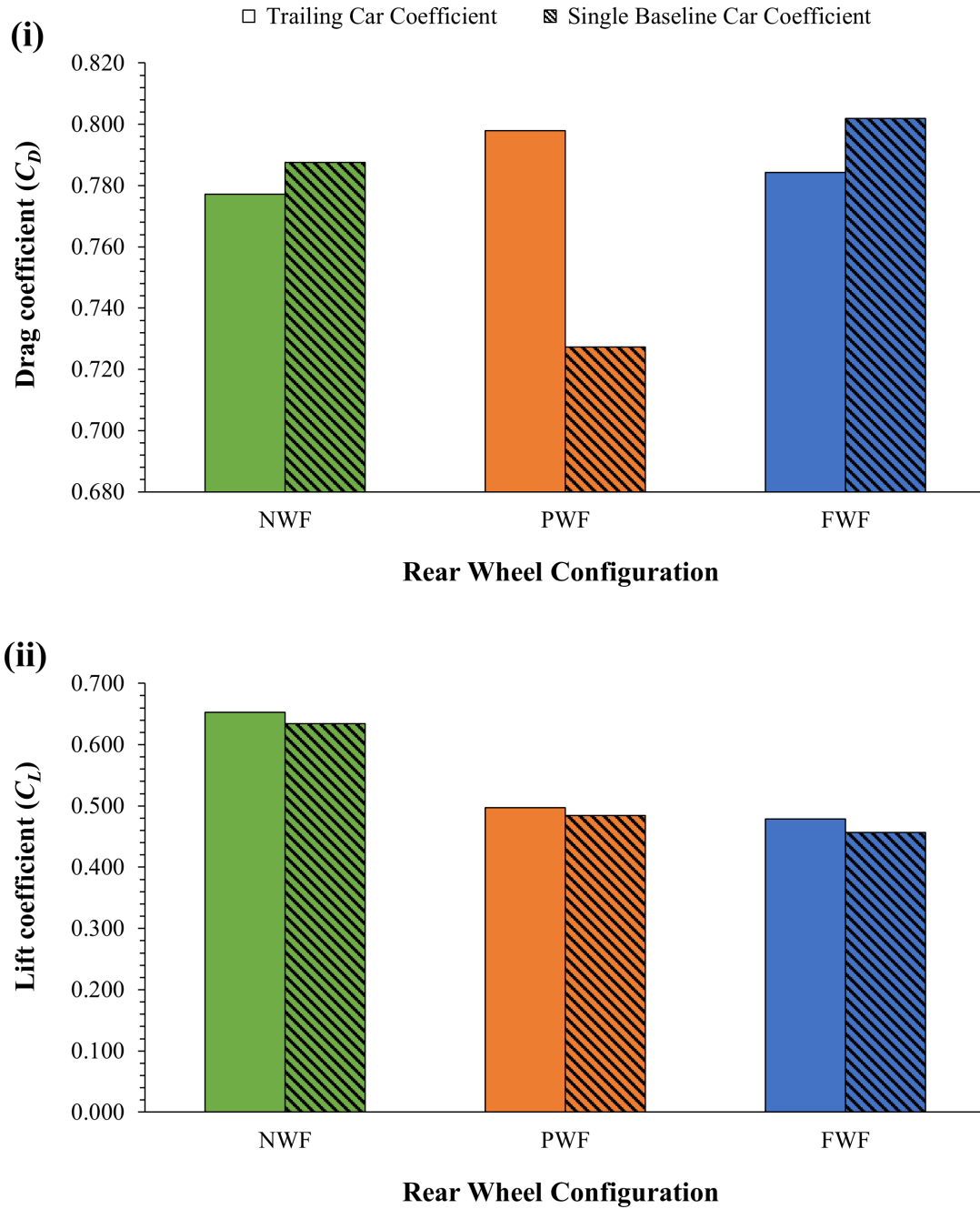
Figure 5.38: Comparison of (i) drag coefficients and (ii) lift coefficients for all configurations at trailing position C
