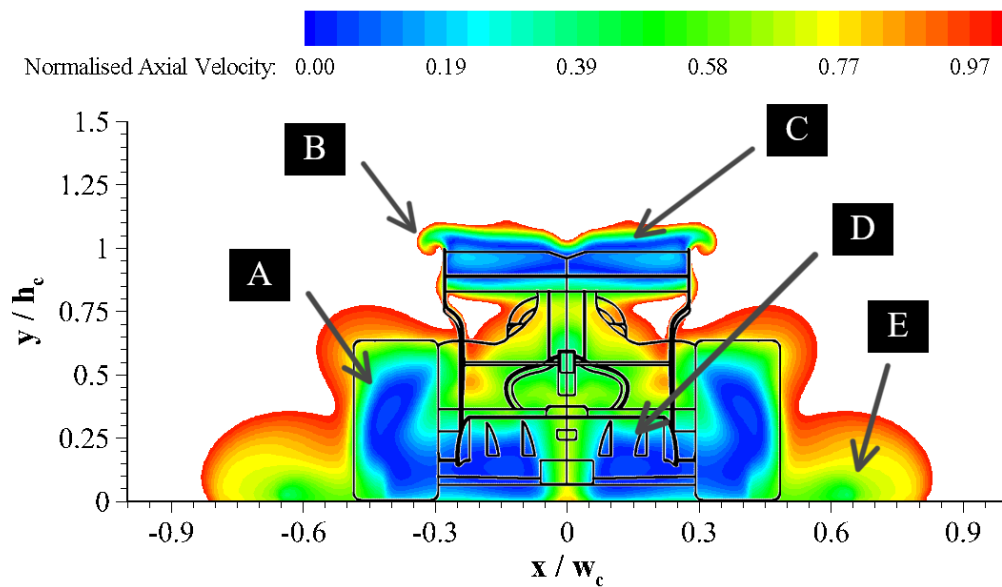
Figure 5.1: Full size normalised axial velocity contours for no wheel fairings at z = 0.0L
