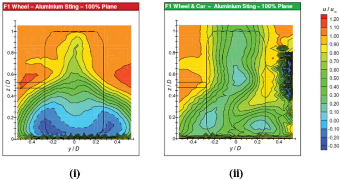
Figure 1.7: Mean u velocities in a wheel wake of an isolated wheel (i) and a wheel in the proximity to a car (ii) as found by Knowles et al. [11]
