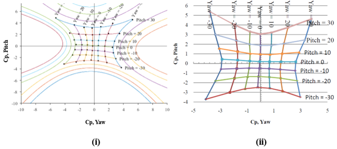
Figure 4.5: Carpet map from calibration data(i), compared to carpet map by Town and Camci (ii) [62]
