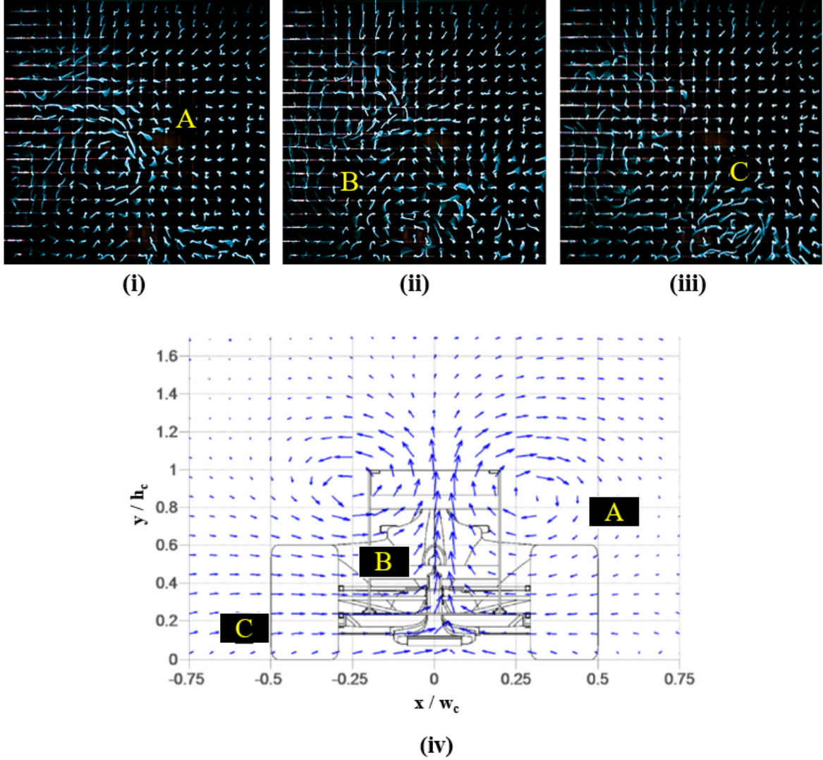
Figure 4.9: Tuft flow visualisation for no wheel fairings at z = 0.5L (i) - (iii) compared to planar velocity components by Watts and Watkins [9] (iv)
