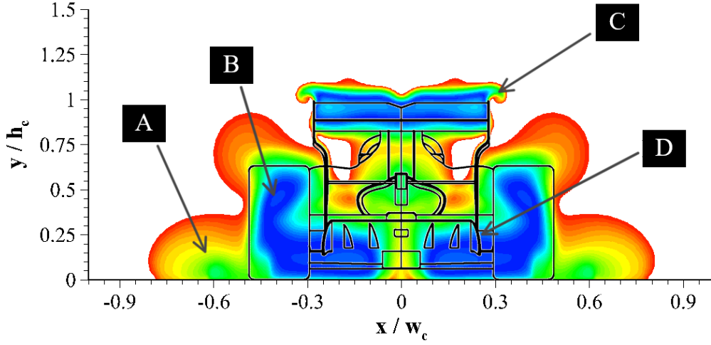
Figure 4.17: Scale model normalised axial velocity contours for no wheel fairings at z = 0.0L rotating wheels
