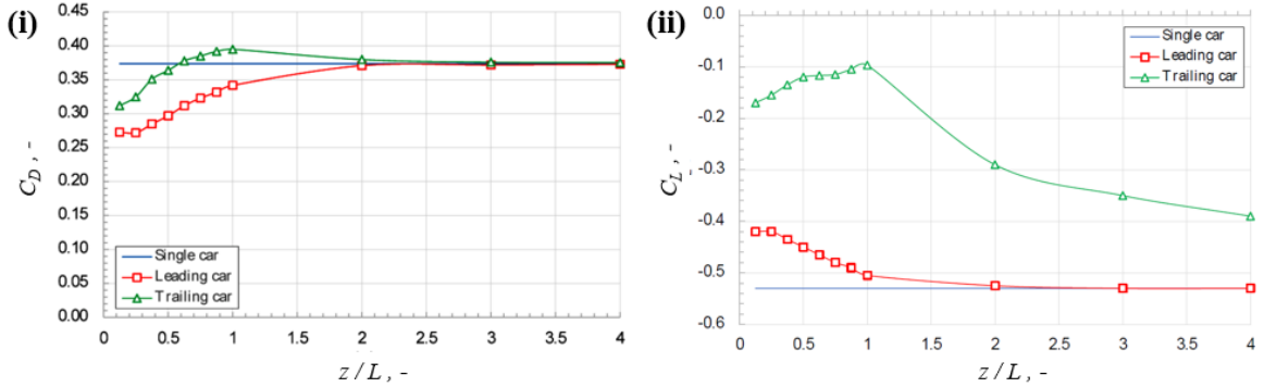
Figure 1.8: Drag (i) and lift (ii) coefficients for leading and trailing cars found by Džijan et al. [14]
