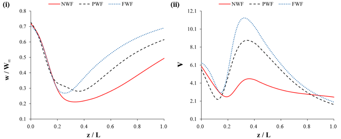
Figure 5.28: Normalised axial velocity (i) and upwash/downwash component (ii) in car symmetry plane
