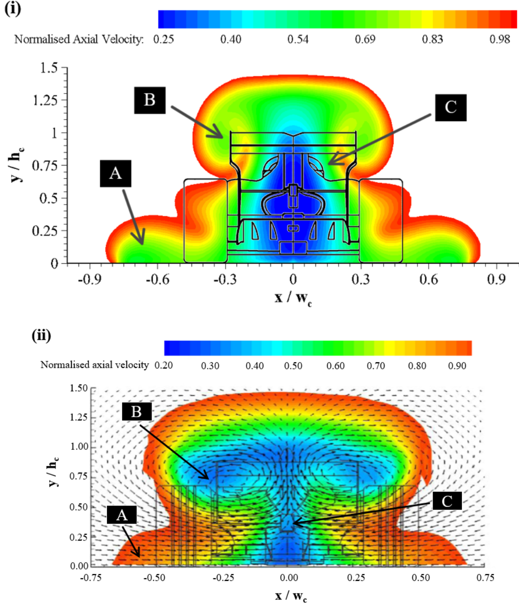
Figure 4.1: Numerical simulation velocity contours for no wheel fairings at z = 0.5L (i), compared to contours by Newbon et al. [10] (ii)
