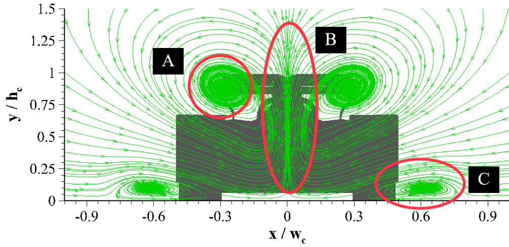
Figure 5.14: Full size planar streamtraces for full wheel fairings at z = 0.5L
