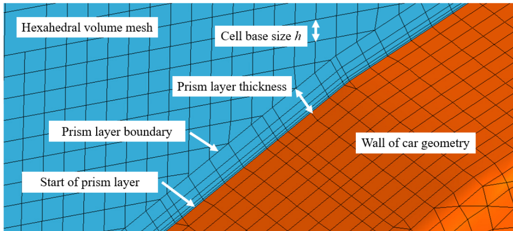
Figure 3.11: Modelling of prism layer for volume mesh
