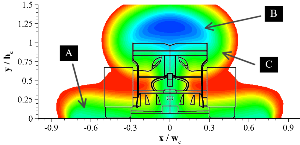
Figure 5.18: Full size normalised axial velocity contours for partial wheel fairings at z = 1.0L
