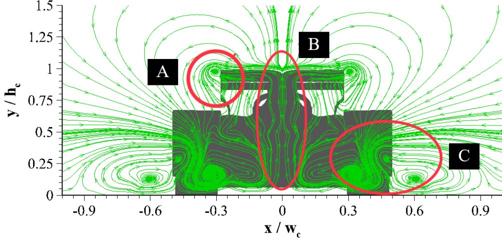
Figure 5.6: Full size planar streamtraces for full wheel fairings at z = 0.0L
