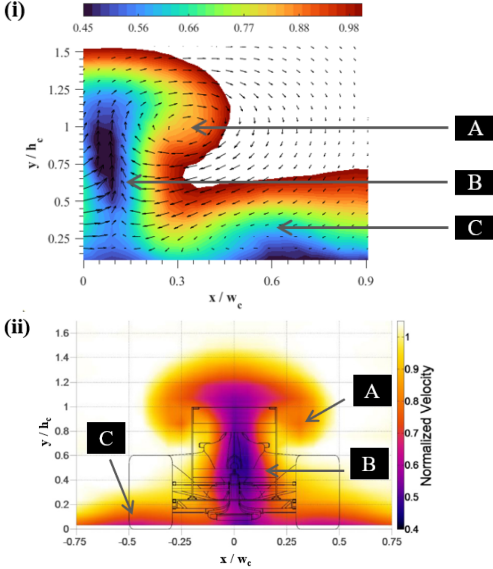
Figure 4.6: Wind tunnel velocity contours for no wheel fairings at z = 0.5L (i), compared to contours by Watts and Watkins [9] (ii)
