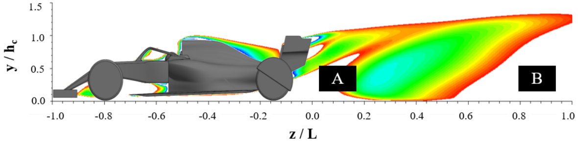
Figure 5.27: Normalised axial velocity contours in car symmetry plane for full wheel fairings
