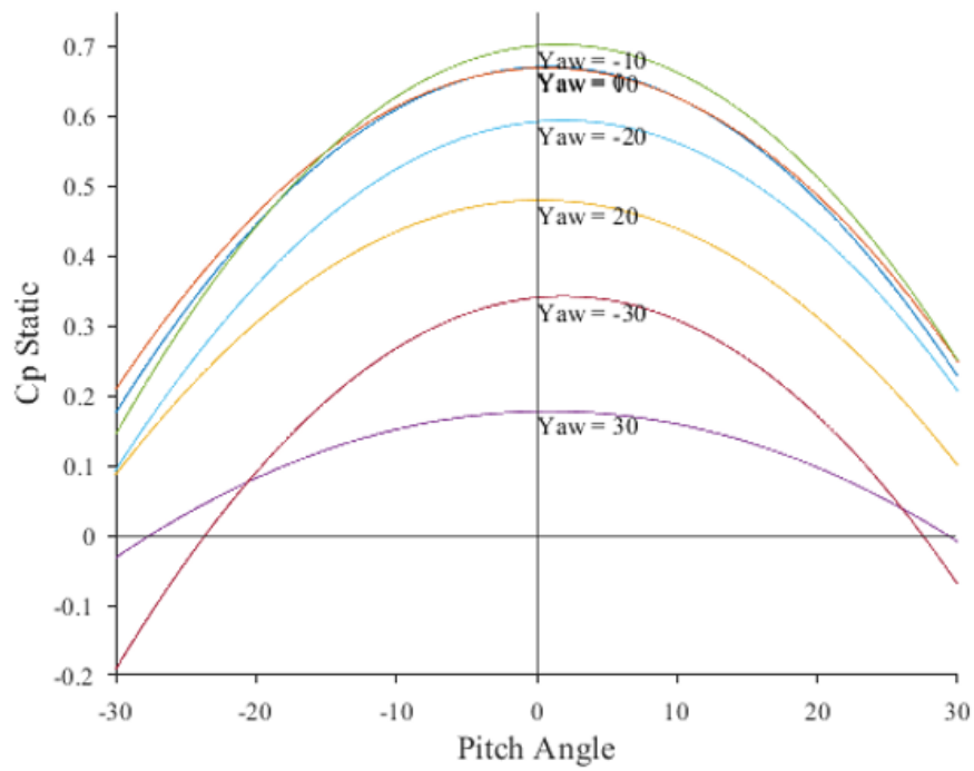
Figure 3.22: Static pressure coefficient versus pitch angles with lines of constant yaw angle for calibration data
