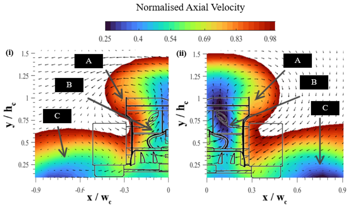
Figure 4.8: Symmetry of scale model normalised axial velocity contours for full wheel fairings at z = 0.5L for wind tunnel tests
