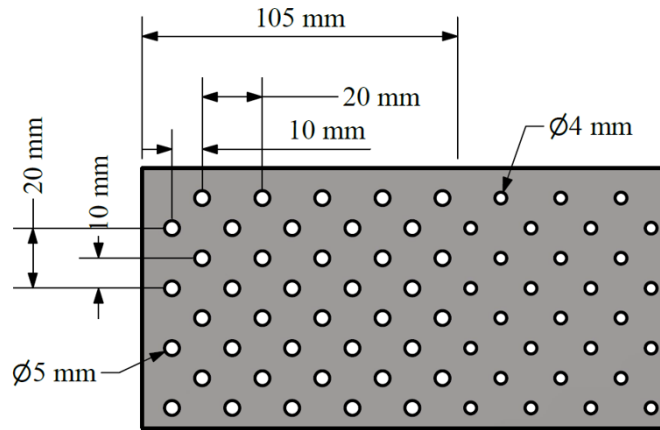
Figure 3.17: Section of boundary layer suction plate
