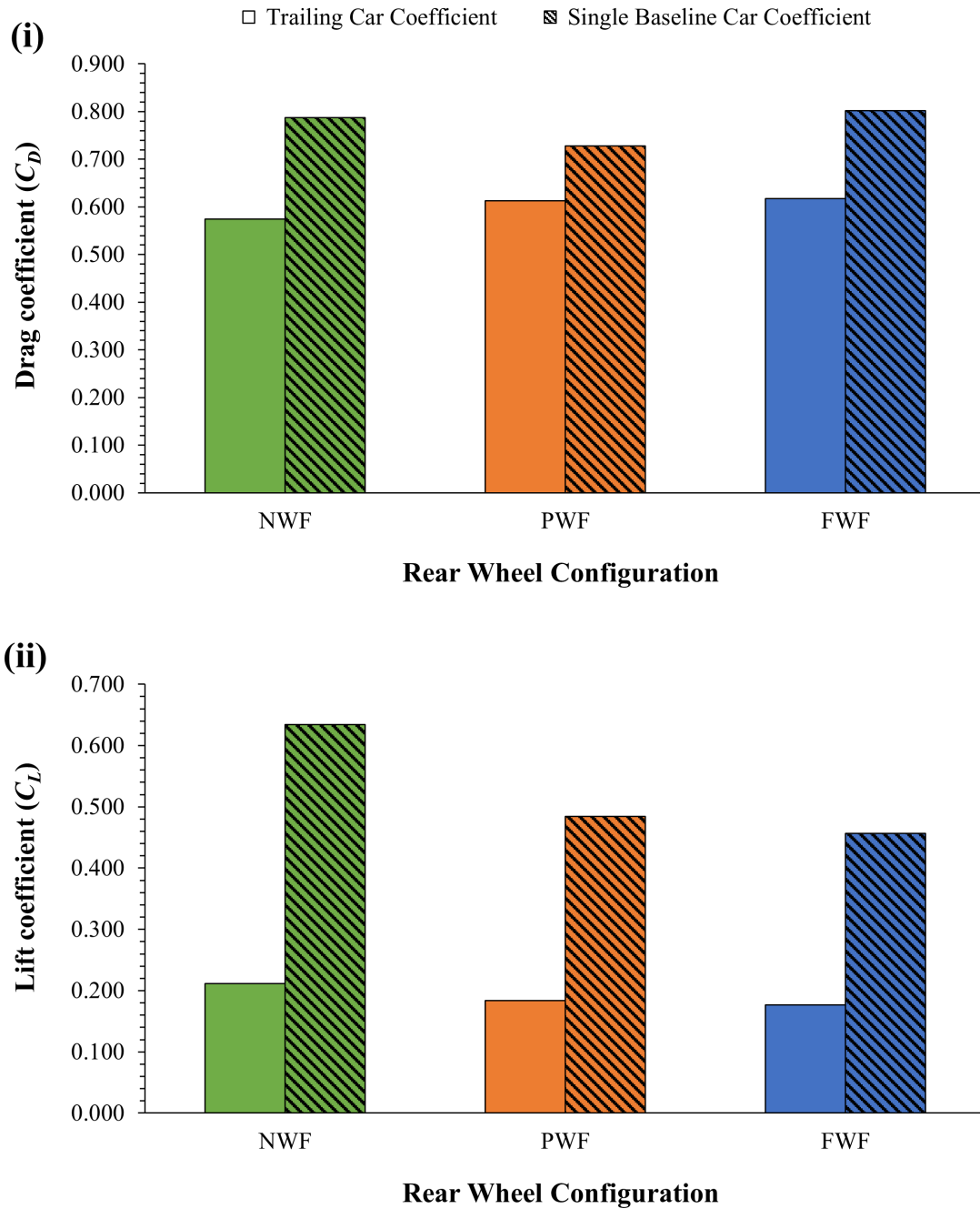
Figure 5.37: Comparison of (i) drag coefficients and (ii) lift coefficients for all configurations at trailing position B
