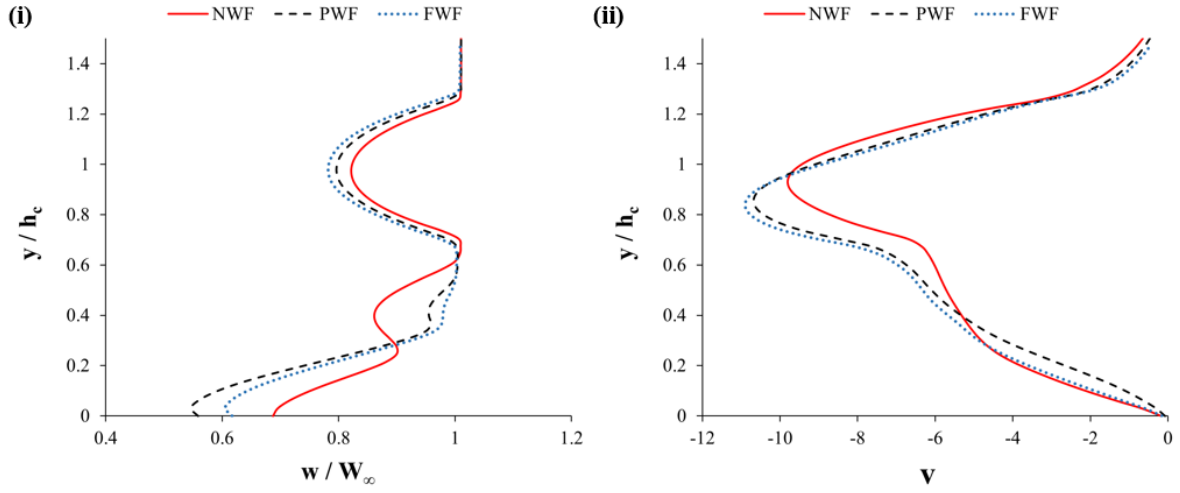
Figure 5.16: Normalised axial velocity (i) and upwash/downwash component (ii) at centreline of wheel in z = 0.5L plane
