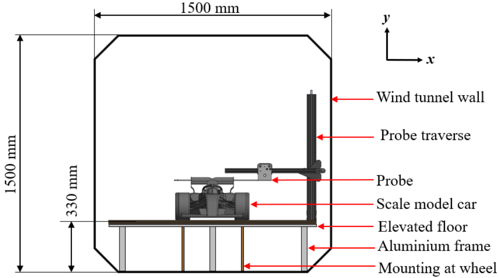
Figure 3.13: Cross sectional view of wind tunnel setup
