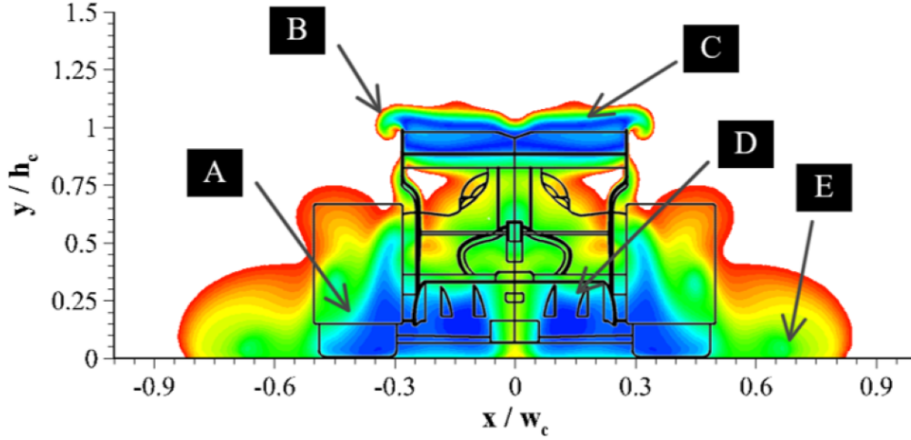
Figure 5.3: Full size normalised axial velocity contours for full wheel fairings at z = 0.0L
