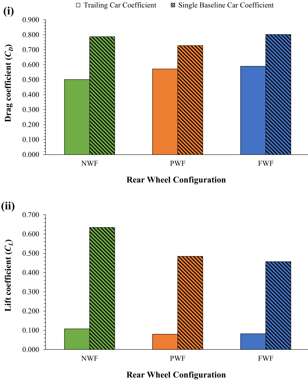
Figure 5.36: Comparison of (i) drag coefficients and (ii) lift coefficients for all configurations at trailing position A
