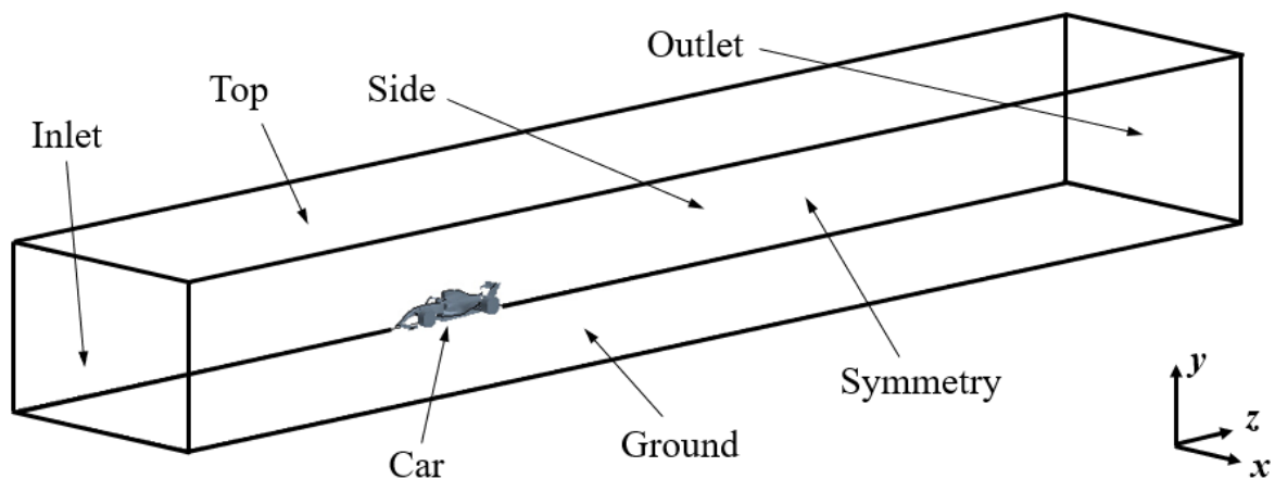
Figure 3.4: Numerical model domain boundaries
