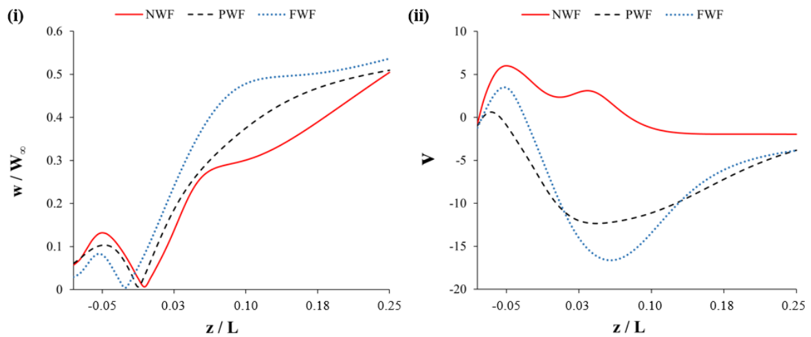
Figure 5.32: Normalised axial velocity (i) and upwash/downwash component (ii) in wheel midplane
