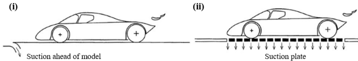
Figure 2.8: Boundary layer suction ahead (i) and distributed under (ii) model, illustrated by Katz [16]
