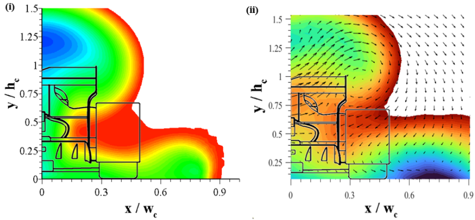
Figure A.5: Scale model normalised axial velocity contours for full wheel fairings at z = 1.0L for CFD (i) and wind tunnel (ii) tests
