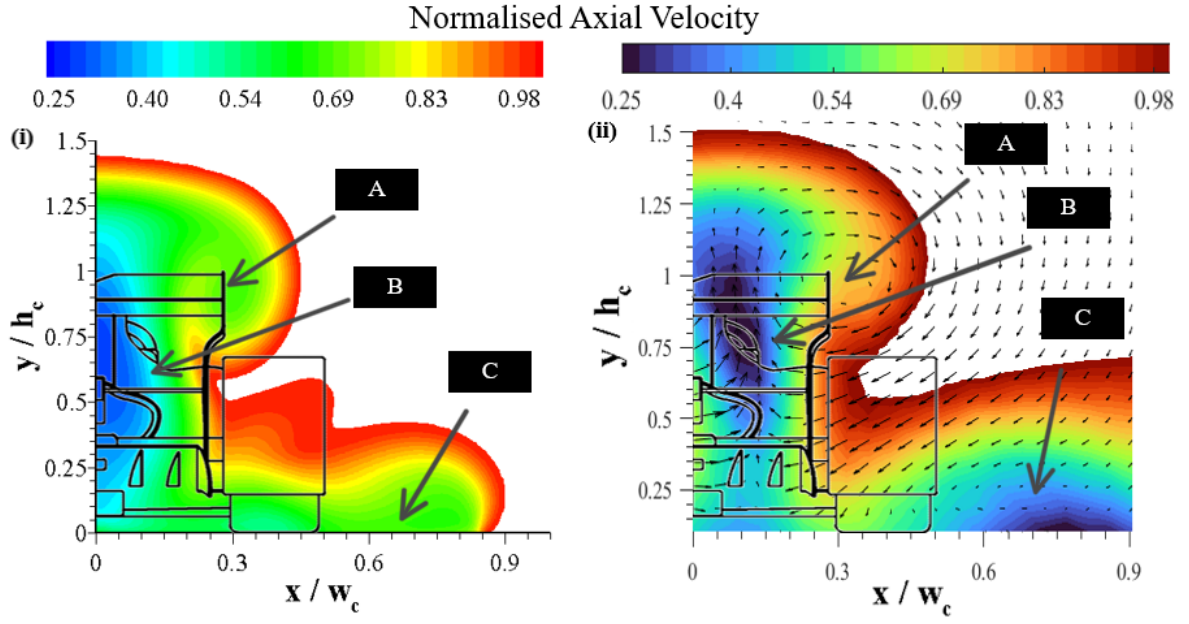
Figure 4.12: Scale model normalised axial velocity contours for full wheel fairings at z = 0.5L for CFD (i) and wind tunnel (ii) tests
