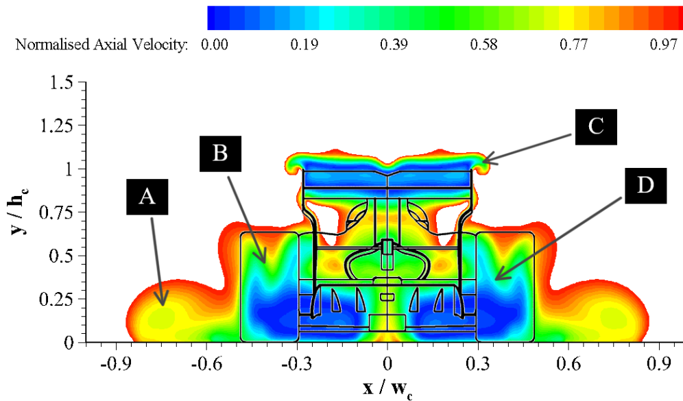
Figure 4.16: Scale model normalised axial velocity contours for no wheel fairings at z = 0.0L for non-rotating wheels
