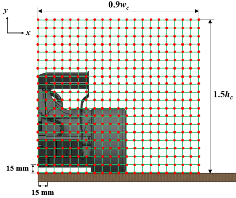
Figure 3.18: Five-hole probe traverse grid for data measurement
