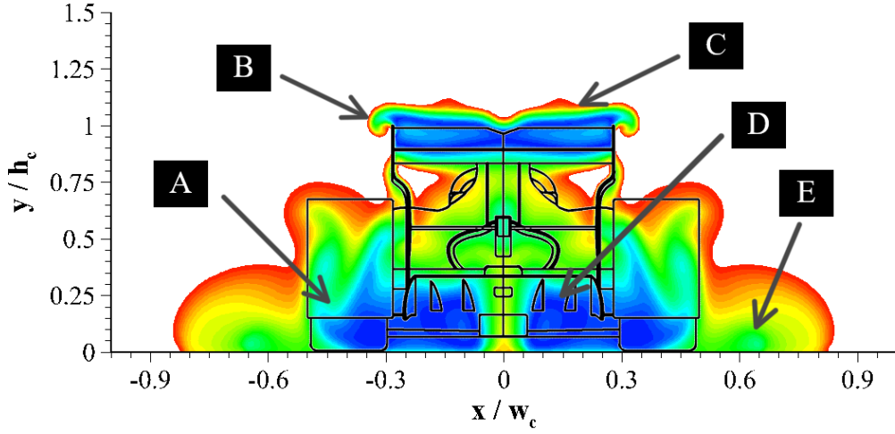
Figure 5.2: Full size normalised axial velocity contours for partial wheel fairings at z = 0.0L
