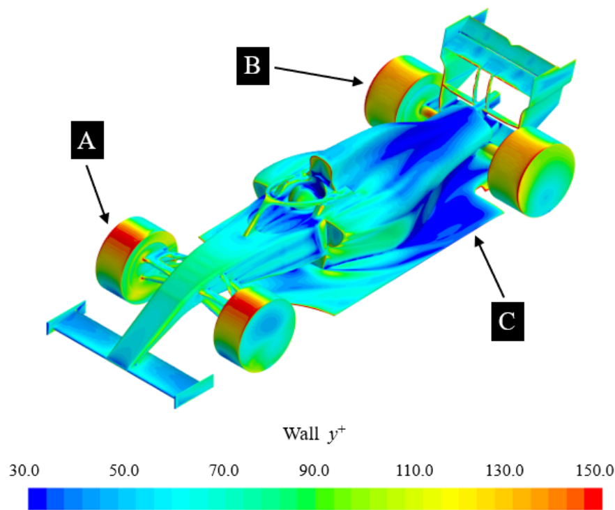
Figure 4.2: Wall y^+ distribution for no wheel fairing configuration
