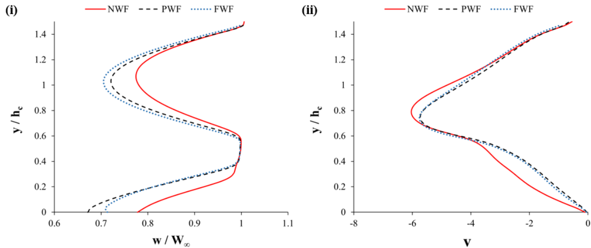
Figure 5.24: Normalised axial velocity (i) and upwash/downwash component (ii) at centreline of wheel in z = 1.0L plane
