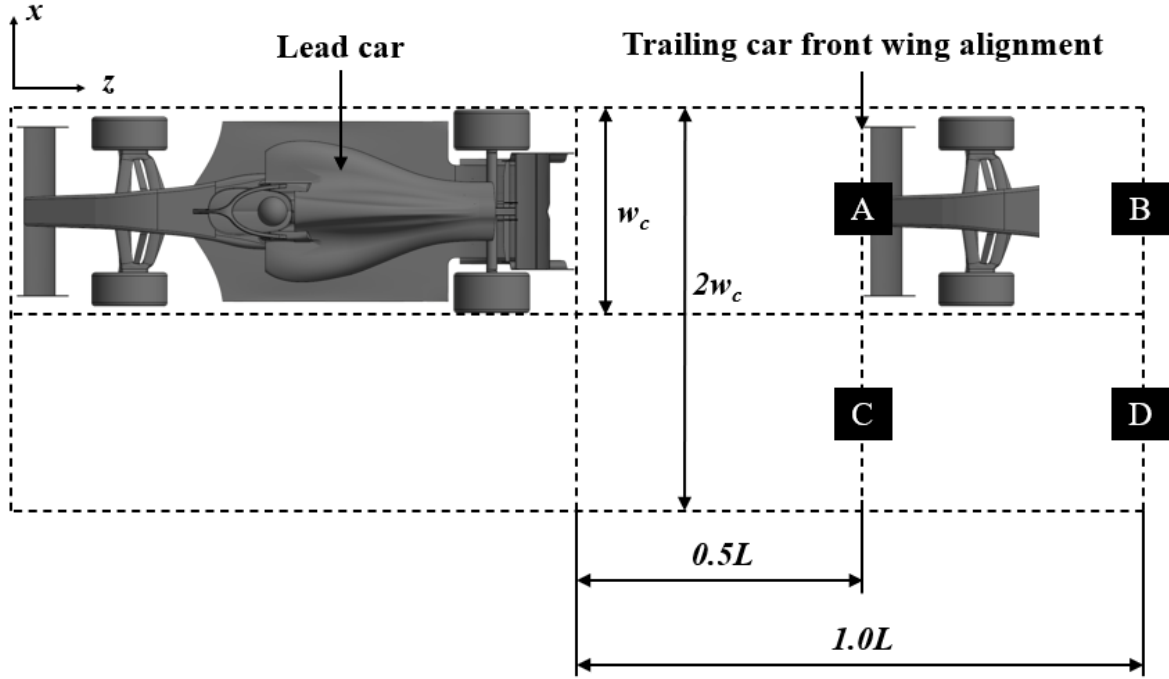
Figure 3.6: Downstream positions of trailing car for simulations
