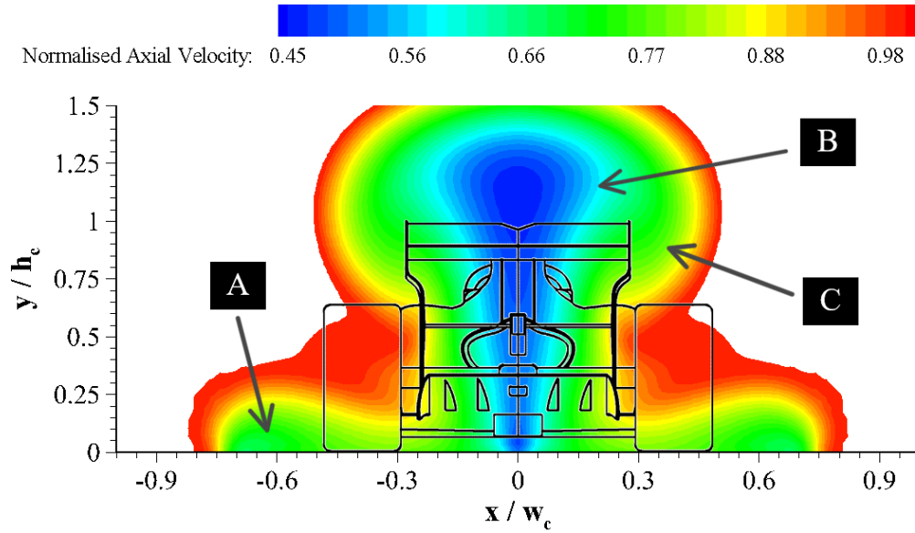
Figure 5.17: Full size normalised axial velocity contours for no wheel fairings at z = 1.0L
