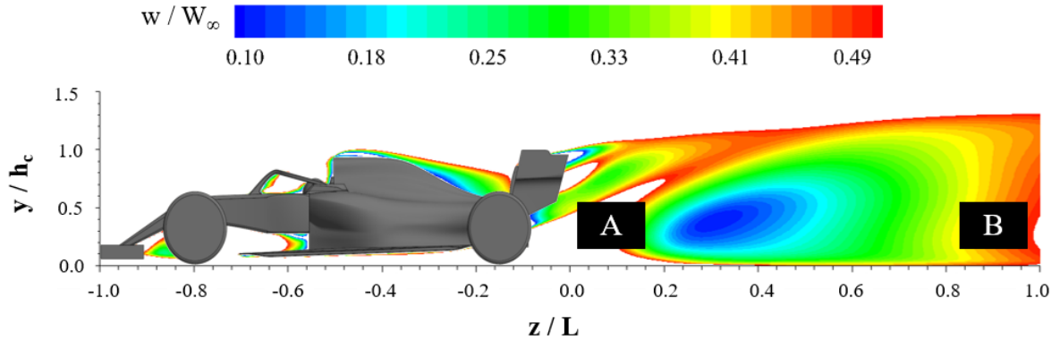
Figure 5.25: Normalised axial velocity contours in car symmetry plane for no wheel fairings
