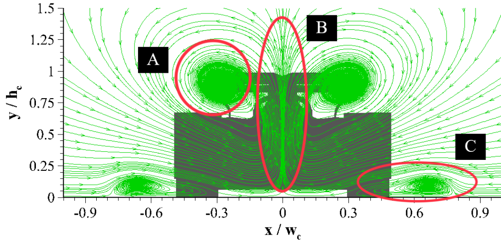
Figure 5.13: Full size planar streamtraces for partial wheel fairings at z = 0.5L
