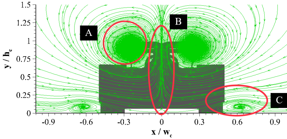
Figure 5.22: Full size planar streamtraces for full wheel fairings at z = 1.0L
