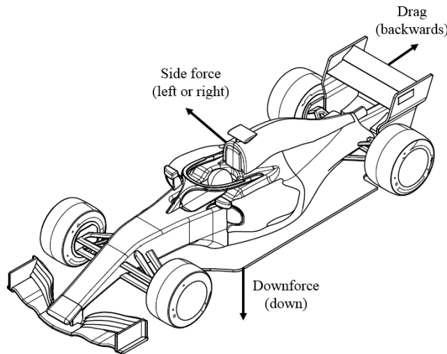
Figure 2.1: Aerodynamic forces on a Formula One car [15]
