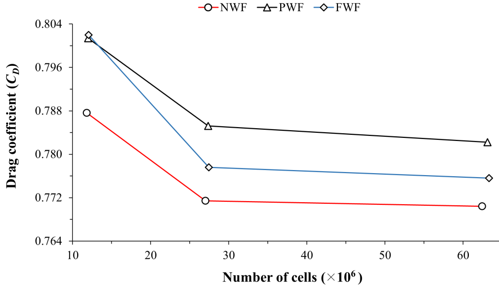
Figure 4.3: Converged drag coefficient value of car versus number of mesh cells
