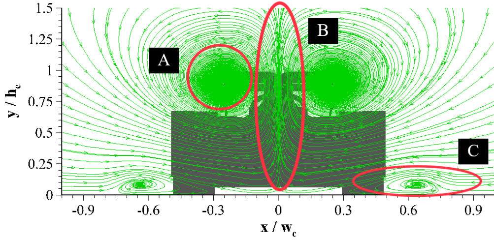
Figure 5.21: Full size planar streamtraces for partial wheel fairings at z = 1.0L
