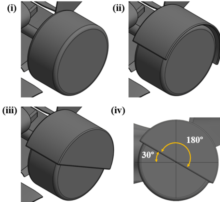
Figure 3.3: Rear wheel with (i) no wheel fairings, (ii) partial wheel fairings, and (iii) full wheel fairings, along with (iv) fairing geometry
