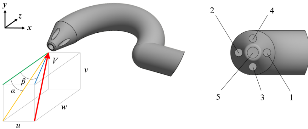
Figure 3.19: Labelled five-hole probe with velocity components and angles
