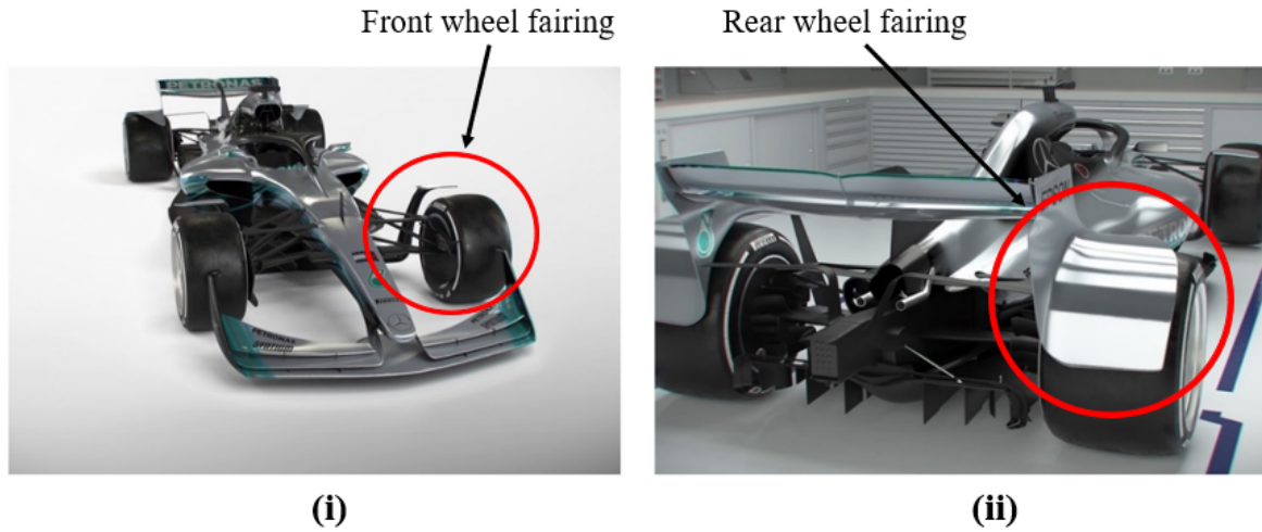
Figure 1.4: Concept car with front (i) and rear (ii) wheel fairings [7]
