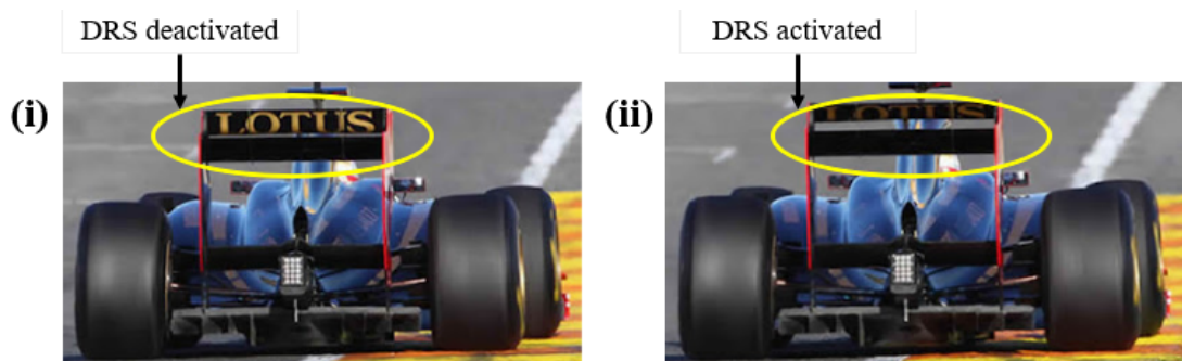
Figure 1.3: Formula One car with DRS deactivated (i) and activated (ii) [5]
