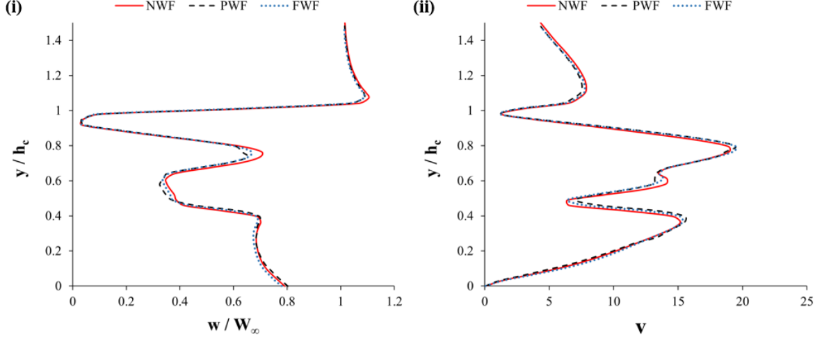
Figure 5.7: Normalised axial velocity (i) and upwash/downwash component (ii) at centreline of car in z = 0.0L plane
