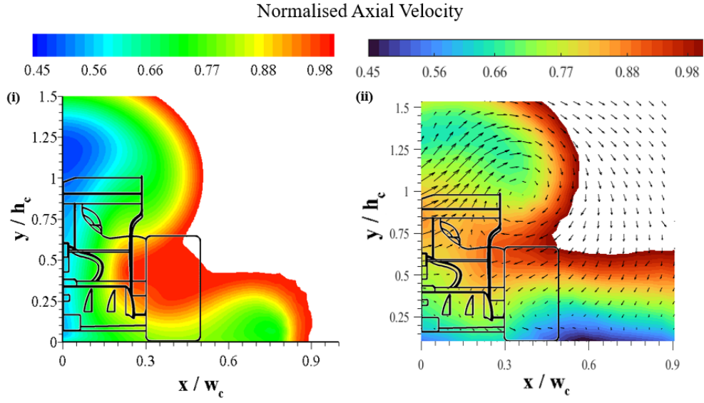
Figure A.3: Scale model normalised axial velocity contours for no wheel fairings at z = 1.0L for CFD (i) and wind tunnel (ii) tests
