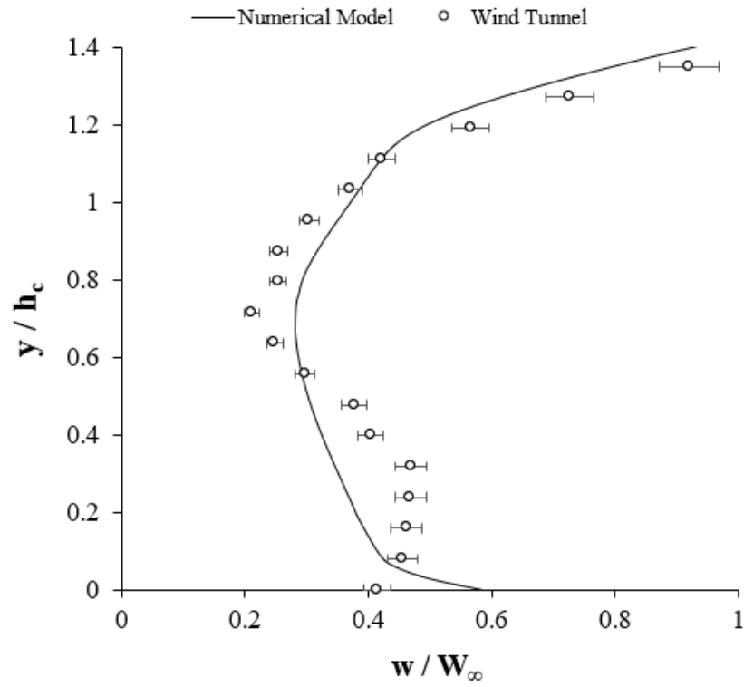
Figure 4.15: Numerical model and wind tunnel test normalised axial velocity distribution along height of car for full wheel fairing configuration
