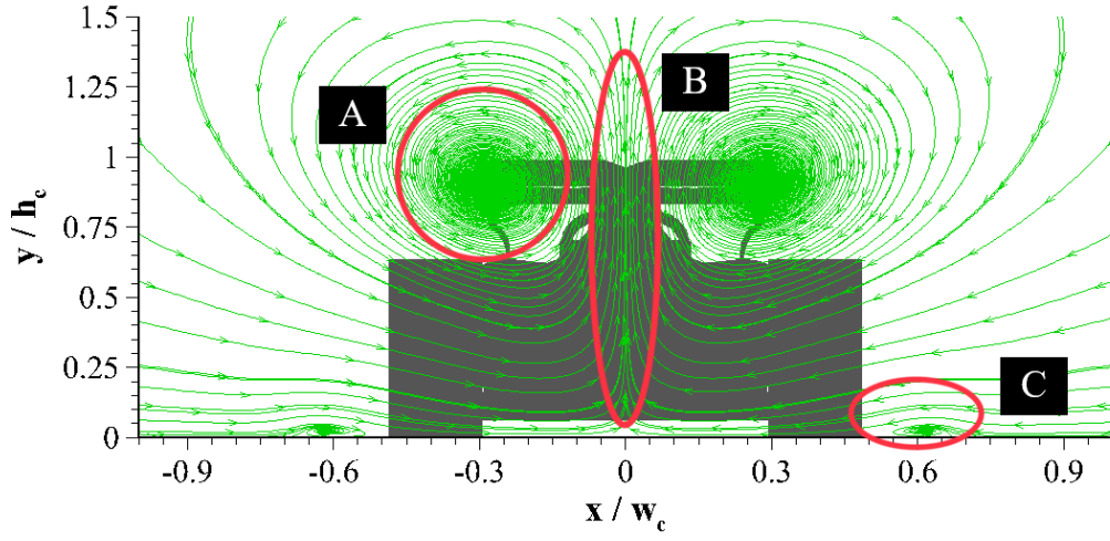
Figure 5.20: Full size planar streamtraces for no wheel fairings at z = 1.0L
