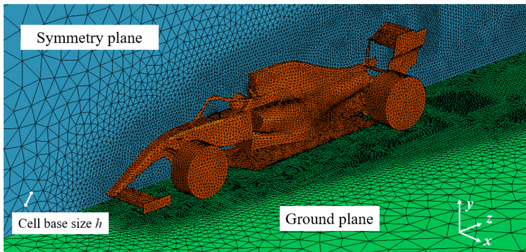
Figure 3.8: Triangulated surface mesh of numerical model
