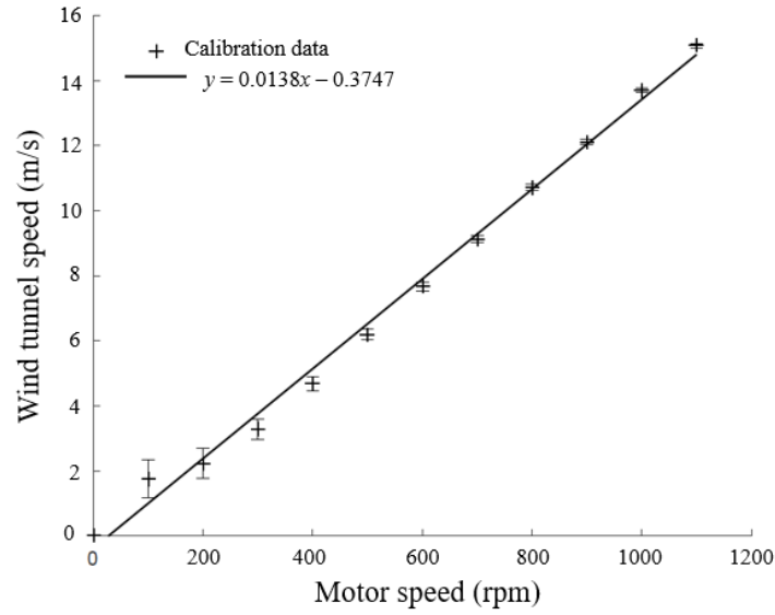
Figure 3.14: Calibration curve for draw-down wind tunnel as determined by Atherfold [60]
