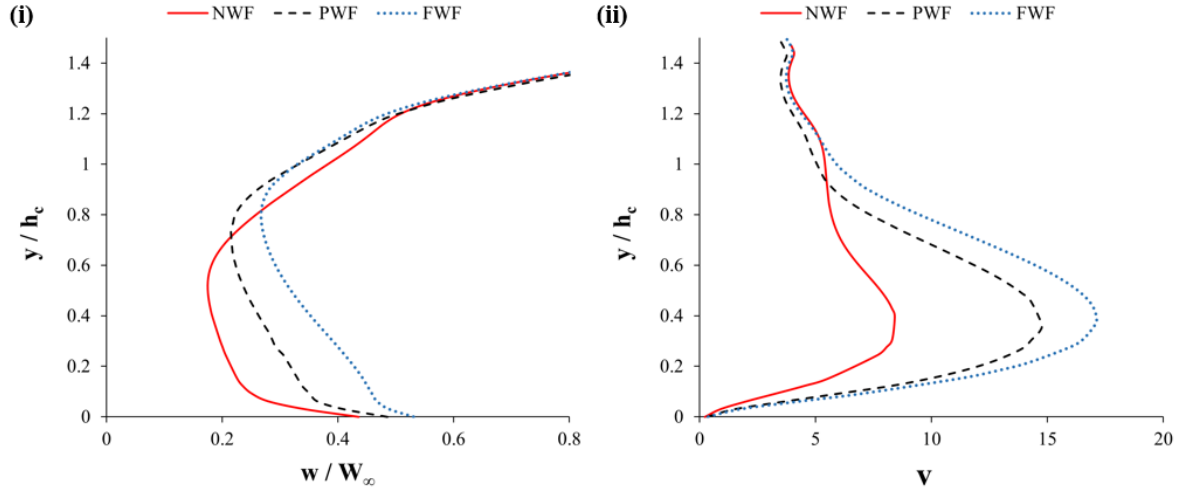
Figure 5.15: Normalised axial velocity (i) and upwash/downwash component (ii) at centreline of car in z = 0.5L plane
