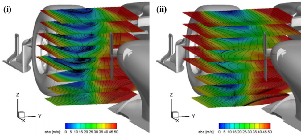
Figure 2.6: PIV measurement conducted by Nakagawa [26] on the wake behind a Formula One car wheel for geometry at the start (i) and end (ii) of a Formula One season
