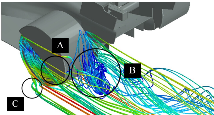
Figure 5.35: Streamlines at rear wheel for full wheel fairings
