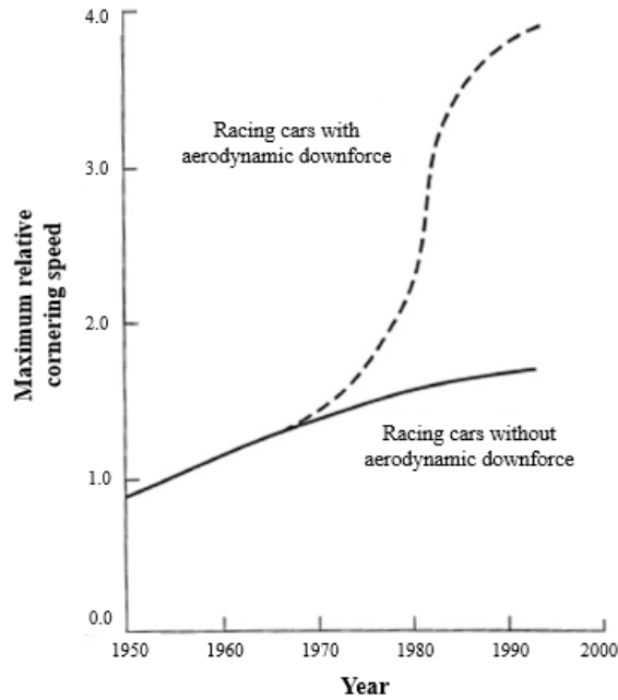
Figure 2.2: Increase in relative cornering speeds in motorsport versus year [16]
