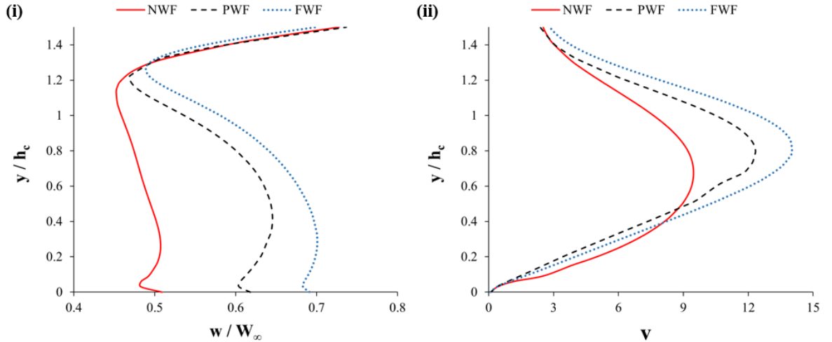
Figure 5.23: Normalised axial velocity (i) and upwash/downwash component (ii) at centreline of car in z = 1.0L plane
