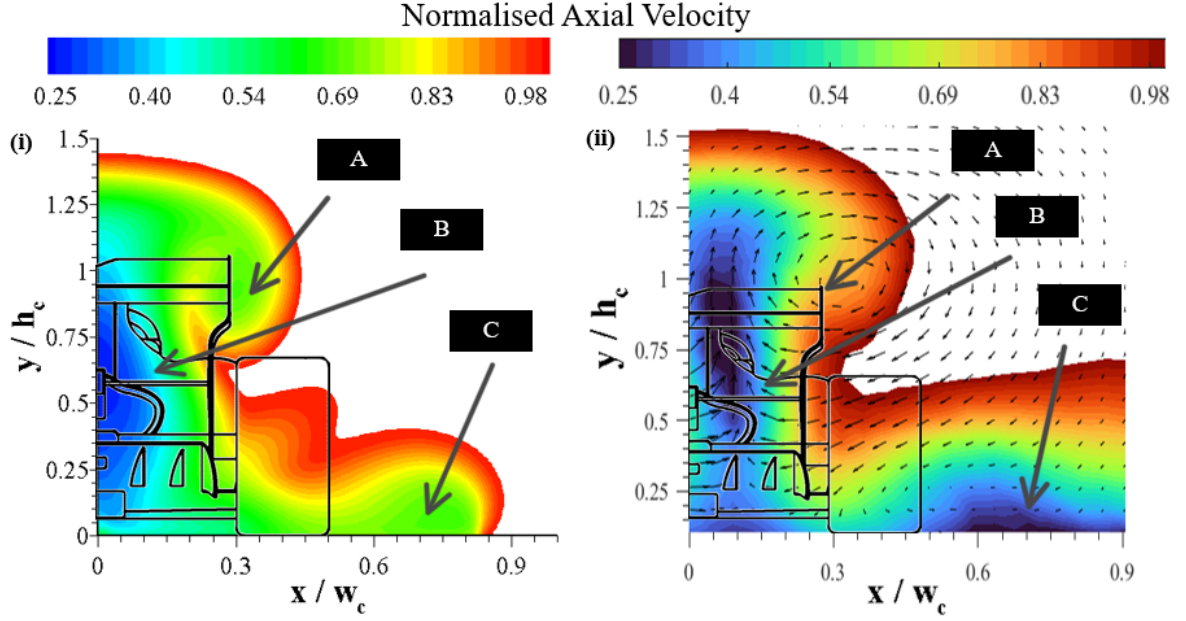
Figure 4.10: Scale model normalised axial velocity contours for no wheel fairings at z = 0.5L for CFD (i) and wind tunnel (ii) tests
