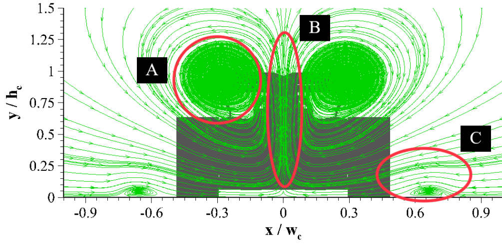
Figure 5.12: Full size planar streamtraces for no wheel fairings at z = 0.5L
