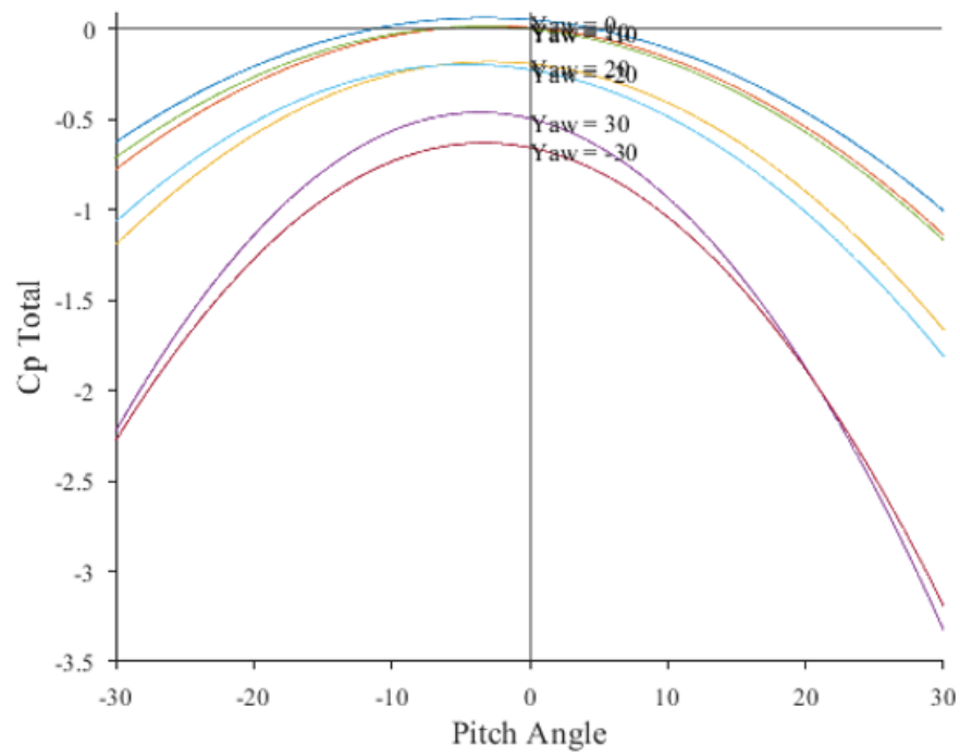
Figure 3.21: Total pressure coefficient versus pitch angles with lines of constant yaw angle for calibration data
