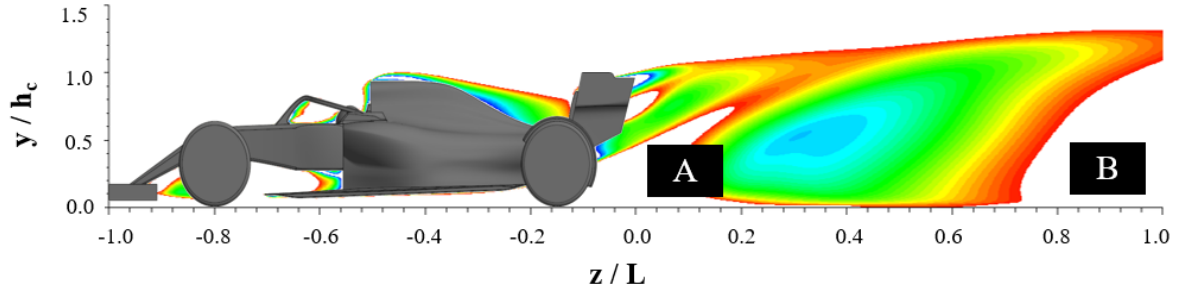
Figure 5.26: Normalised axial velocity contours in car symmetry plane for partial wheel fairings
