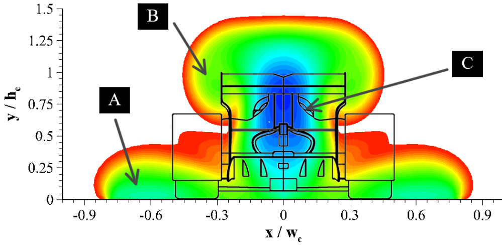
Figure 5.11: Full size normalised axial velocity contours for full wheel fairings at z = 0.5L
