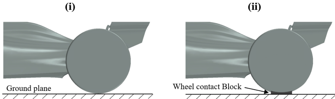
Figure 3.7: Wheel contact block for meshing
