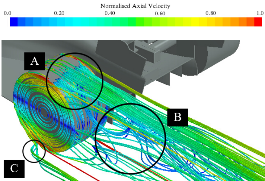
Figure 5.33: Streamlines at rear wheel for no wheel fairings
