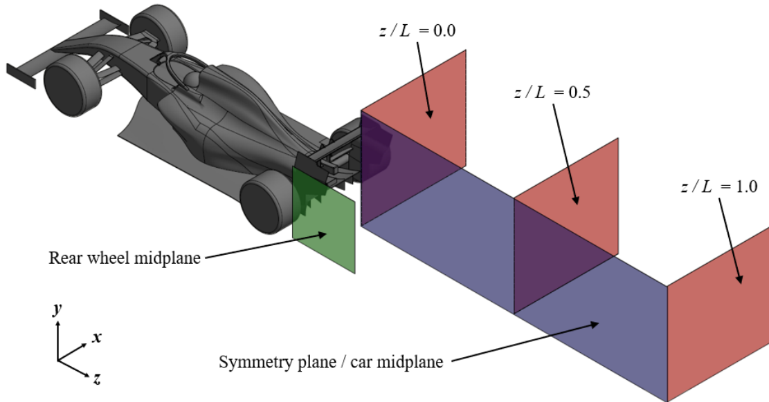
Figure 3.1: Downstream planes investigated for wake survey
