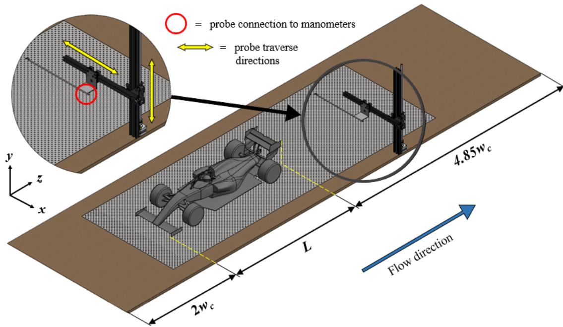
Figure 3.16: Elevated ground plane employed for wind tunnel tests
