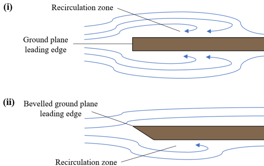
Figure 3.15: Non-bevelled (i) and bevelled (ii) ground plane leading edges
