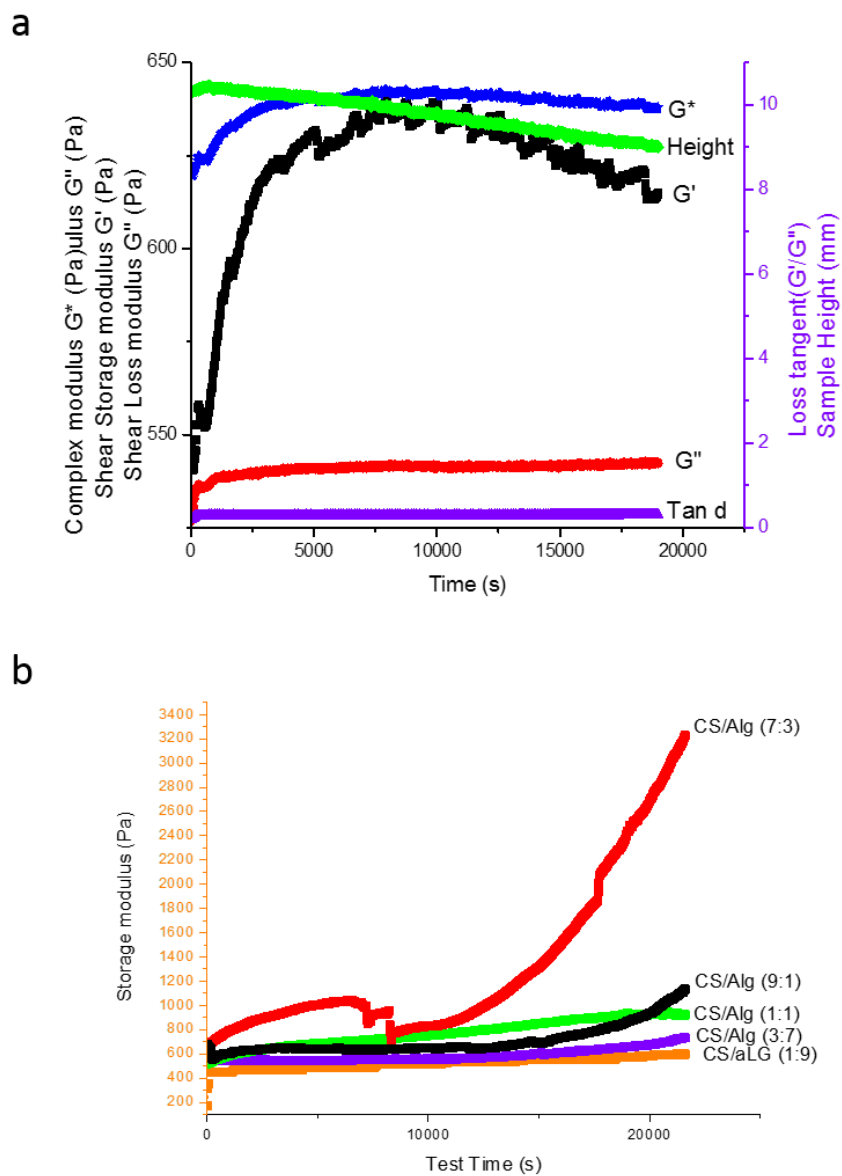
Figure 4.3. The hydrogel formation Kinetics of PC TFA-CS-Alg in simulated wound fluid (pH 7.4) at 25 °C. (a) The interpolymer complex hydrogel was formed in situ by mixing PC Alg (50 mg) and PC TFA-CS (50 mg) in 3 mL SWF. The shear storage modulus (gelling and elasticity measurements), shear loss modulus (viscosity), sample height (swelling and absorption functions), shear complex modulus and loss tangent (viscoelastic properties) were measured in real time. (b) Rate of interpolymer complexation in different bioplatfrom ratios.
