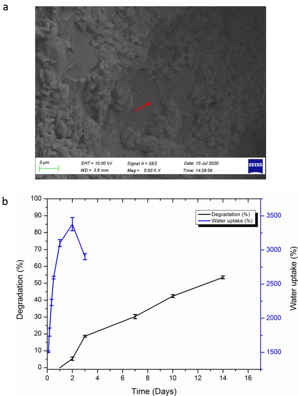
Figure 4.2. (a) Morphological evaluation via SEM and (b) fluid uptake capacity and degradation of PC TFA-CS-Alg IPC. Fluid uptake and degradation evaluation were performed in PBS (pH 7.4) solution at 37 °C at 50 rpm orbital shaker.
