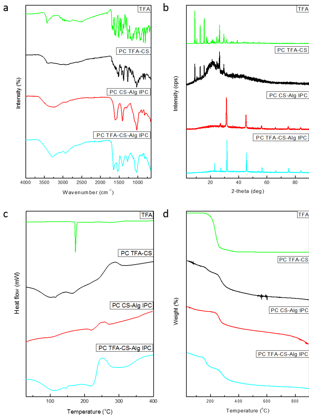
Figure 4.1. The bioplateform's functional groups, chemical composition, and phase changes induced by partial-crosslinking and TFA loading on the polymers were evaluated via the four analytical techniques (a) FTIR spectra, (b) X-Ray diffractograms, (c) DSC and (d) TGA thermograms of the bioplateforms.
