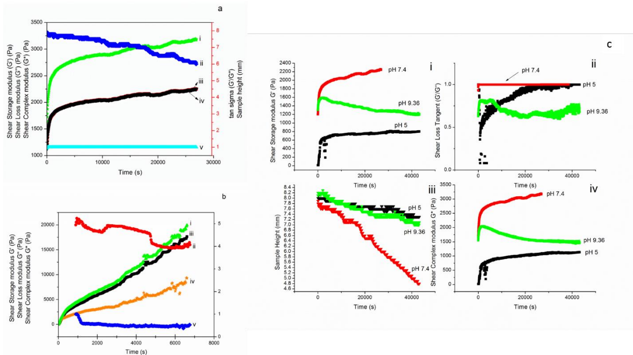
Figure 3.7. Kinetic gelation of the IPC in (a) SWF (pH 7.4) and (b) blood at 37°C. (i) represent the shear complex modulus ( G^* )(Pa), (ii) sample height (mm), (iii) shear storage modulus ( G' )(Pa), (iv) shear loss modulus ( G'' )(Pa), (v) loss tangent ( G'/G'' ). (c) The pH-dependent Kinetic gelation of the in situ forming IPC in SWF at 37°C, where (i) represent the shear storage modulus ( G' )(Pa), (ii) loss tangent ( G'/G'' ), (iii) sample height (mm), and (iv) shear complex modulus ( G^* )(Pa).
