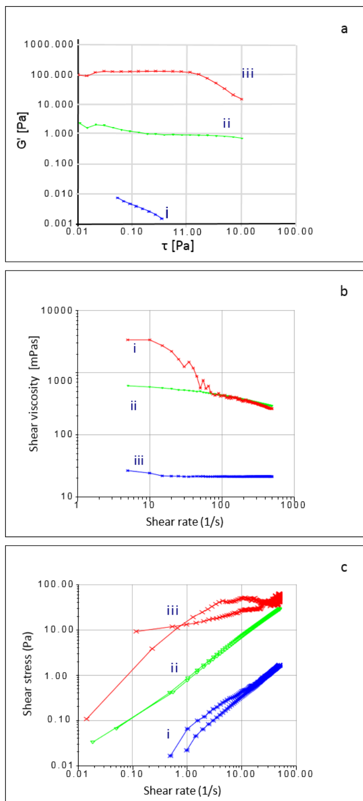
Figure 3.6. Rheological analysis of the polymers and the polyelectrolyte complex. (a) Elastic modulus as a function of shear stress for (i) alginate (2% w/v), (ii) chitosan (2% w/v), and (iii) PEC (2% w/v) performed at a frequency of 0.1 Hz. Shear viscosity (b) and (c) hysteresis loop area of the (i) alginate (2% w/v), (ii) chitosan (2% w/v) and (iii) IPC (2% w/v) platforms performed at 37°C.
