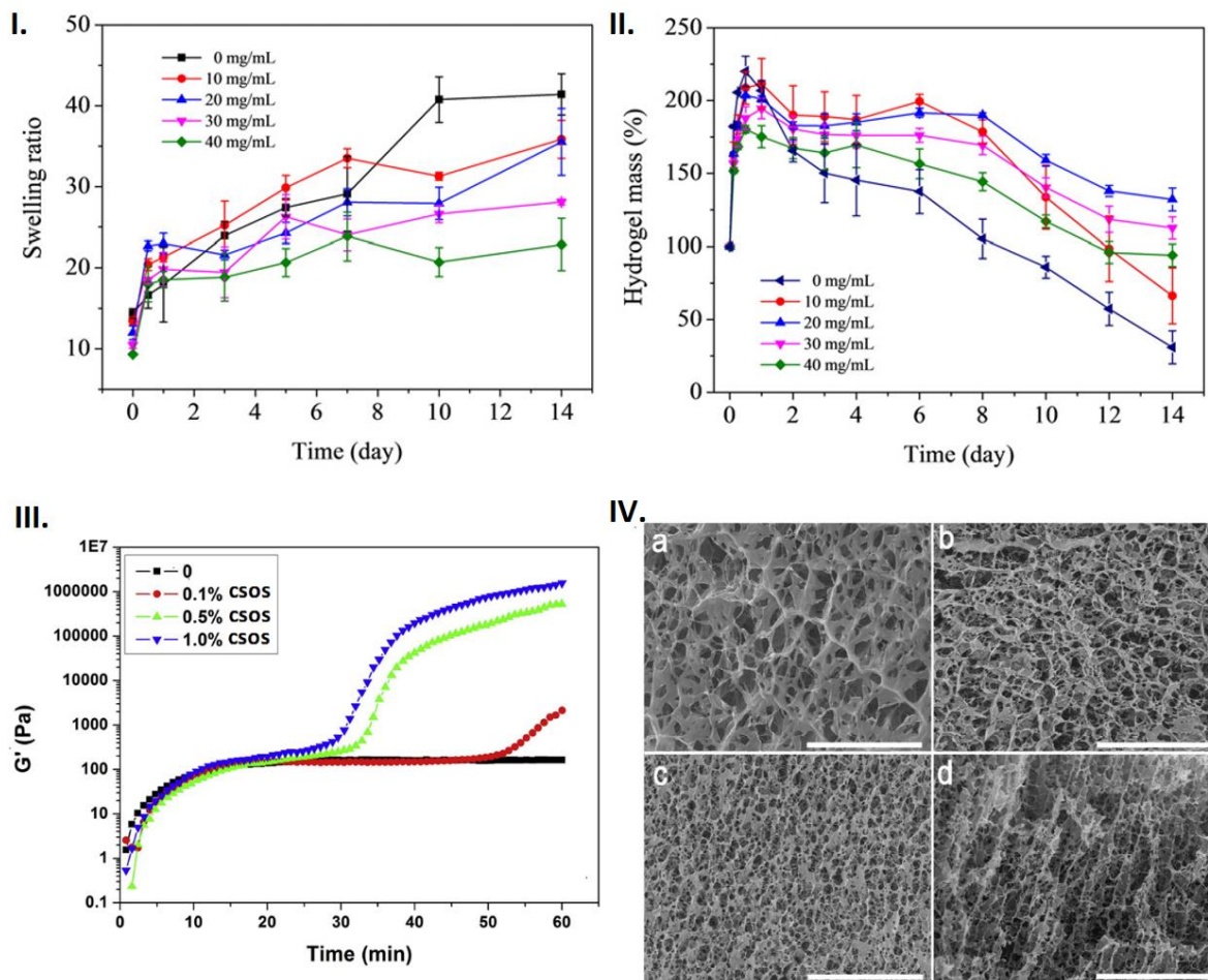
Figure 2.4. Physical and mechanical properties of chitosan-based composites: (I) Swelling and (II) degradation kinetics of tetracycline hydrochloride (TH)/oxidized alginate (OAlg)/carboxymethyl chitosan (CMCS)/gelatin microspheres (GMs) Gel with different concentration of GMs as a function of time in PBS at 37 °C. Image reproduced with permission from Chen et al. (Chen et al., 2017). (III) Gelling kinetics (of carboxymethyl chitosan (CMCS)/alginate/Chitosan oligosaccharides (CSOS) hydrogels at different CSOS concentration; (IV) Porosity observed in SEM images of CMCS/alginate (1:1) hydrogels with different concentration of CSOS: (a) no COS 0.1%, (b) CSOS, (c) 0.5% CSOS and (d) 1.0% CSOS; (scale bar=40 \mu m). Image reproduced with permission from Lv et al. (Lv et al., 2018).
