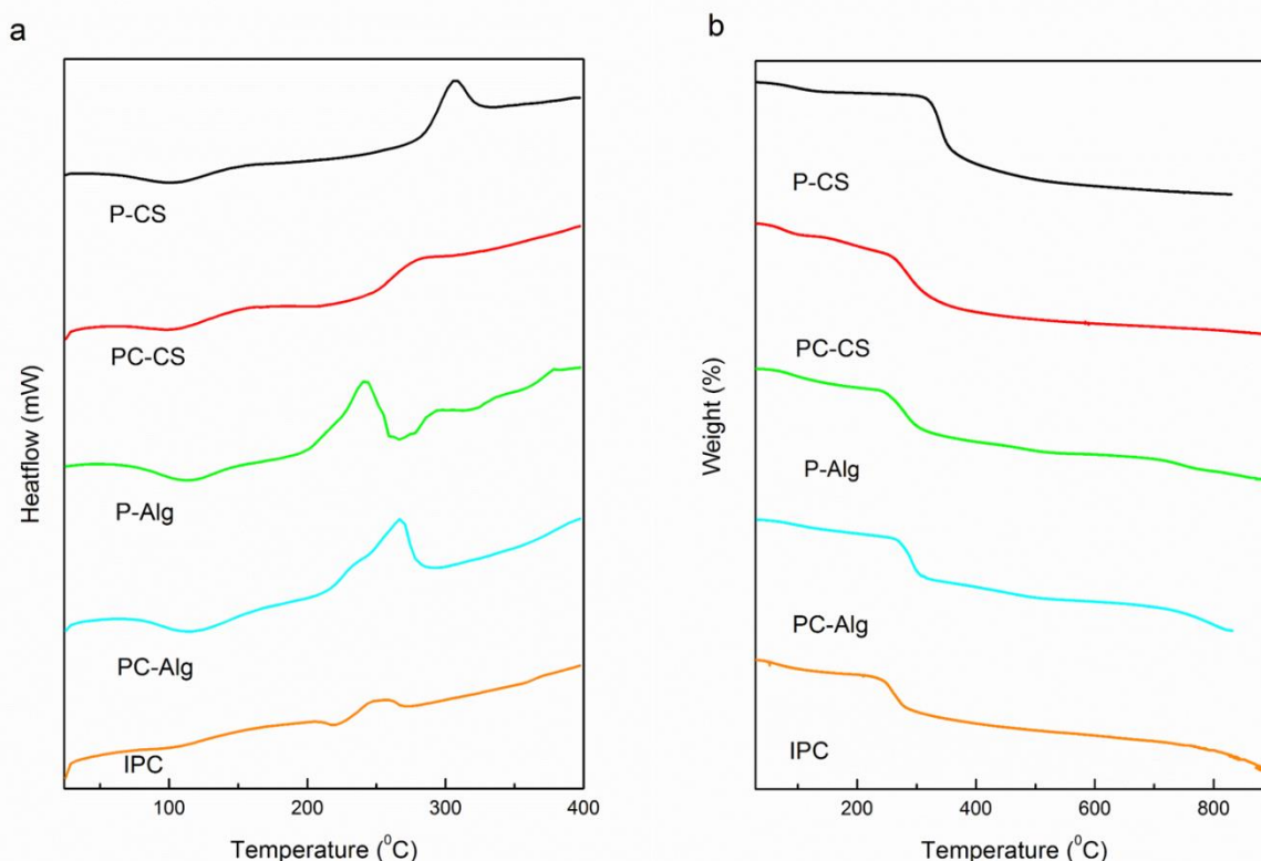
Figure 3.4. (a) Differential scanning calorimetric analyses and (b) Thermogravimetric analyses of the platforms.
