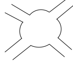
Figure 2.4: Ribbon vertex: four ribbons meet in loop.
