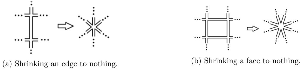
Figure 2.8: Smooth deformation in the triangulation.
