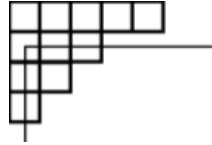
Figure 3.1: The hook associated to the first box in the second row has a length of 5 as illustrated.
