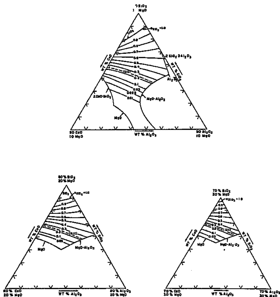
Figure 2.39. Activity of \text{SiO}_2 in \text{SiO}_2 - \text{CaO} - \text{MgO} - \text{Al}_2\text{O}_3 slags at 1600^\circ\text{C} , 10%, 20%, and 30% of \text{MgO} . After Rein and Chipman [36]
