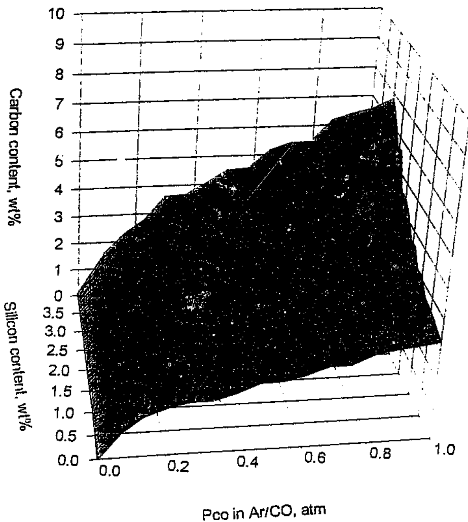
Figure 4.1.4. Relationship between carbon and silicon for alloys of 61%Cr-Fe-Si-C by mass in CO/Ar gas at 1500°C.
