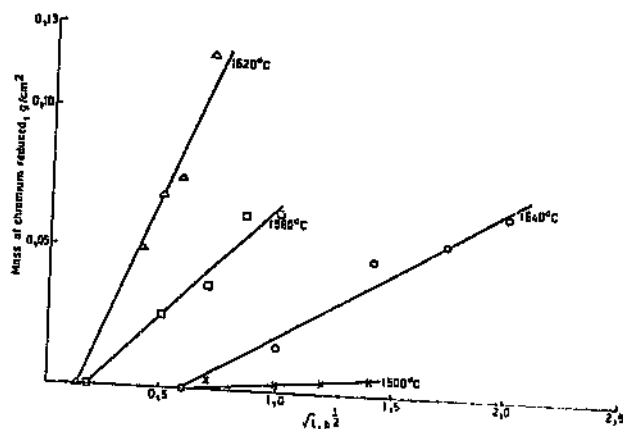
Figure 2.5. Reduction of chromium oxide from chromite-ore cube in molten slag in graphite crucible [39]
