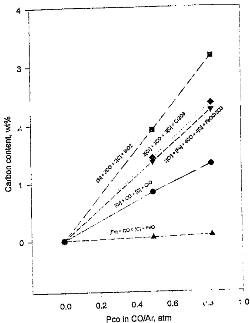
Figure 4.1.5. Calculation of carbon content picked up from CO gas at 1500°C, alloys of 63%Cr-34%Fe-3%Si-C by mass.
