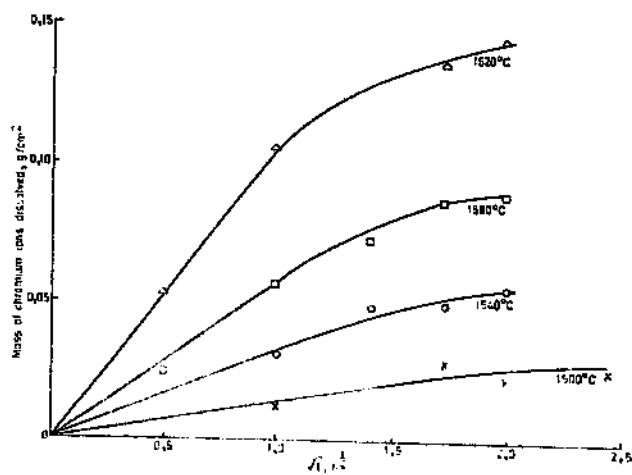
Figure 2.3. Dissolution of the chromium oxide from chromite-ore cube into the slag [39]
