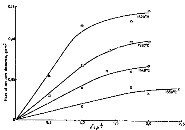
Figure 2.2. Dissolution of iron oxide from the chromite-ore cube into the slag [39]
