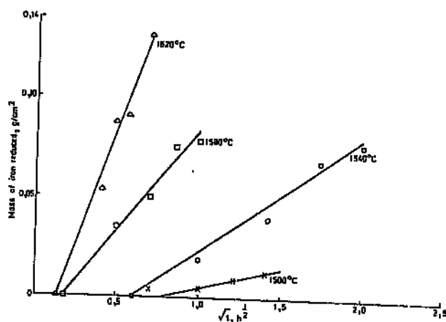
Figure 2.4. Reduction of iron oxide from chromite-ore cube in molten slag in graphite crucible [39]
