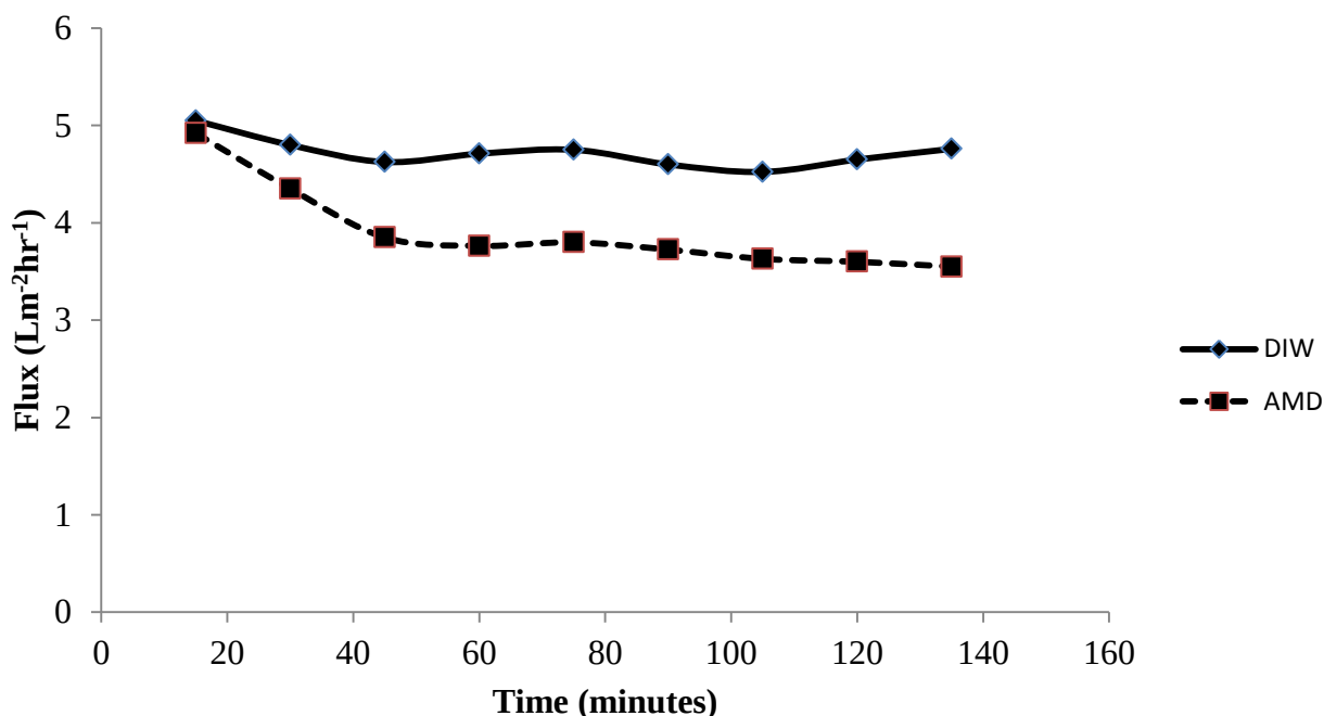
Figure 4.2: Permeate flux as a function of time at maximum flowrate
