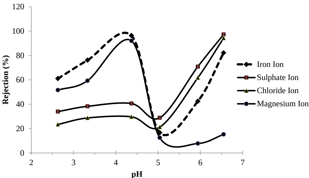
Figure 4.4: Effect of pH on rejection efficiency
