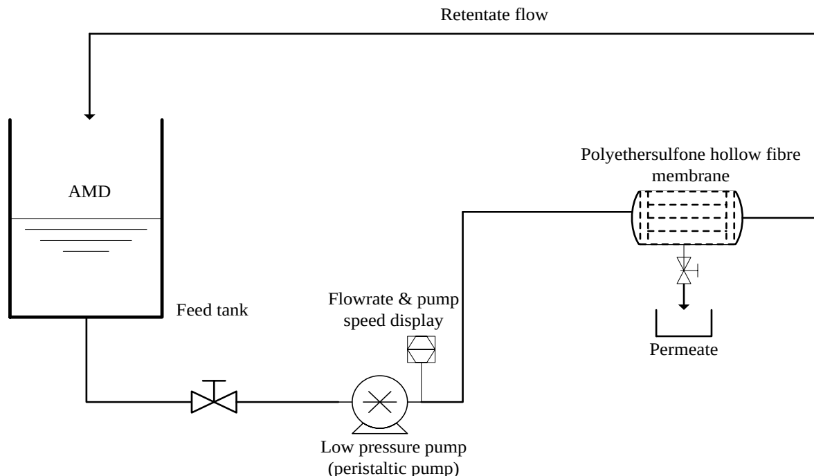
Figure 3.1: Experimental Set up
