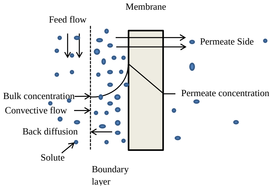
Figure 2.1: Concentration polarisation (Schafer et al., 2004)
