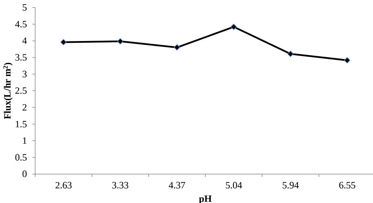
Figure 4.6: Flux as a function of pH
