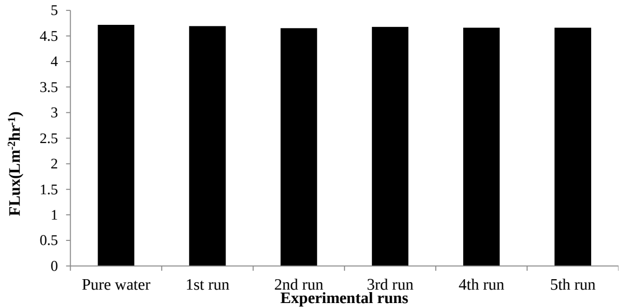
Figure 4.7: Flux of DIW in between experimental runs
