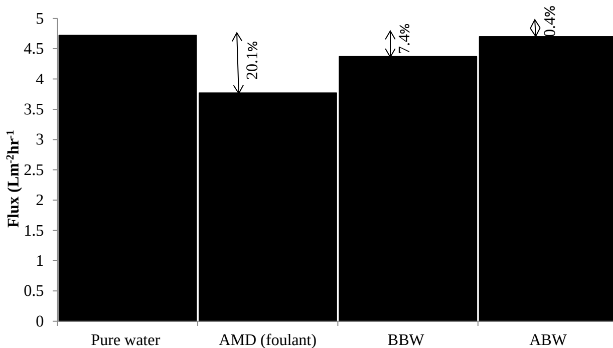
Figure 4.3: Fouling experimental results
