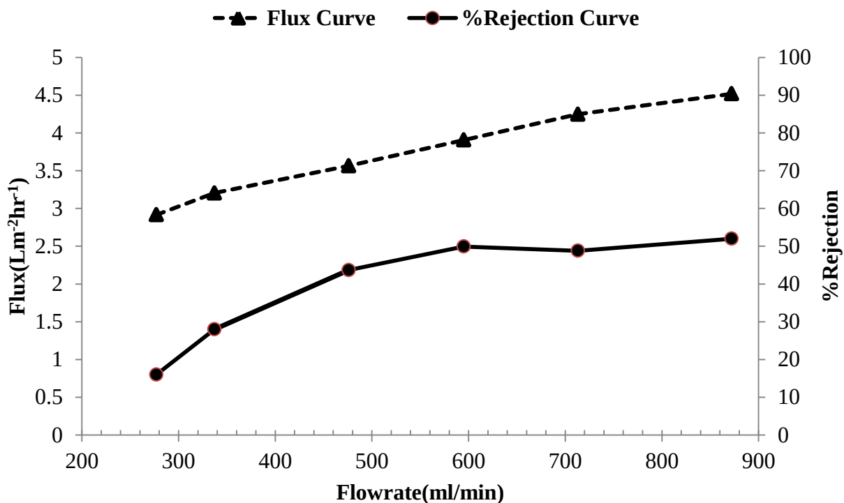
Figure 4.1: Effect of flowrate on flux and rejection efficiency of the membrane
