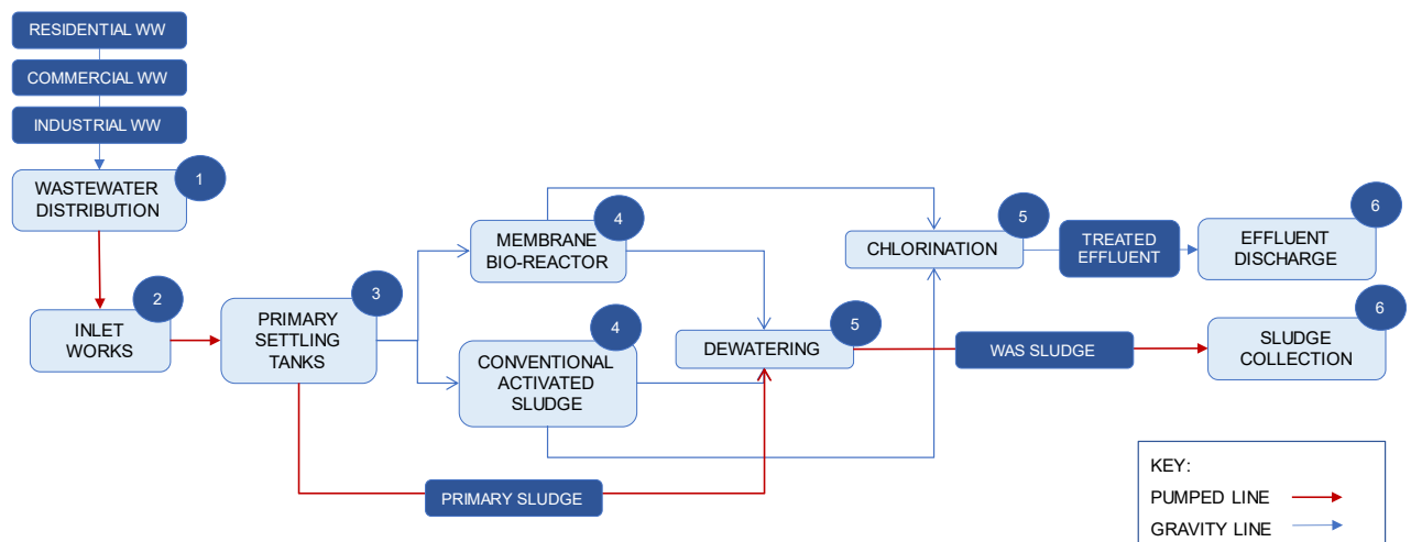
Figure 15: Process Flow Diagram for WWTP
