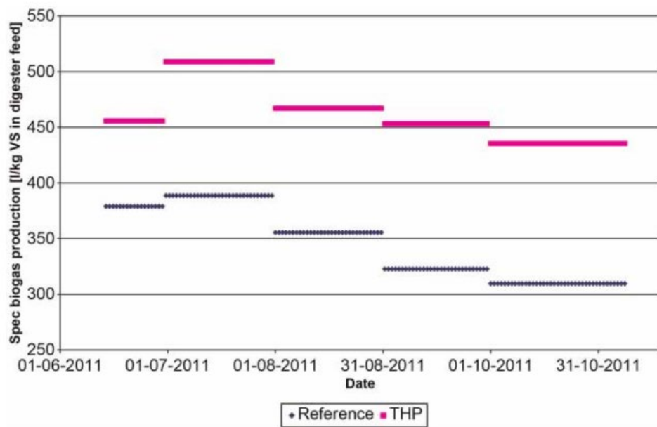
Figure 10: Experimental results of the study to show the effect of THP as a pre-treatment to anaerobic digestion on biogas production (Oosterhuis et. al., 2014)
