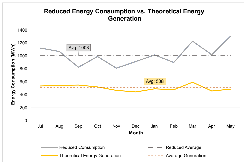
Figure 25: Reduced Energy Consumption vs. Theoretical Energy Generation from Sludge
