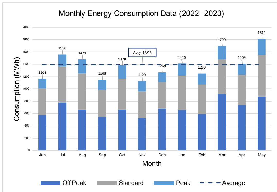
Figure 19: Monthly Energy Consumption Data (2022-2023)
