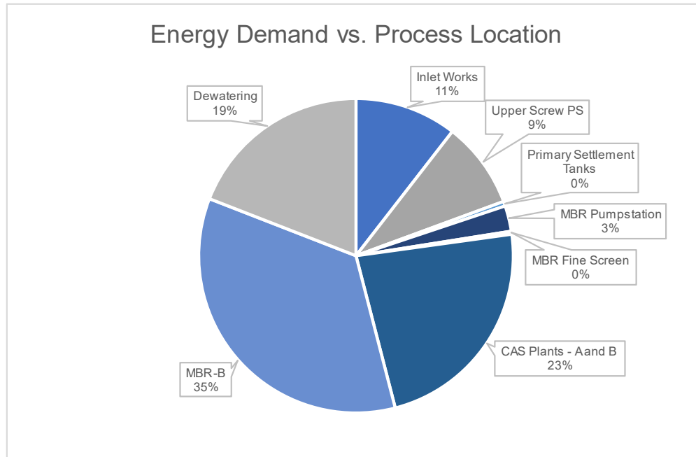
Figure 21: Energy Demand per Process Location
