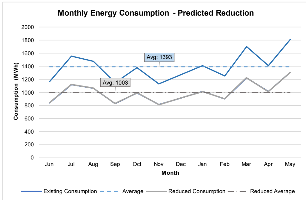
Figure 24: Baseline Energy Consumption vs. Predicted Reduced Energy Consumption
