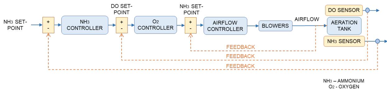
Figure 6 : DO and NH3 based control and monitoring system (adapted from Phelan, 2016)
