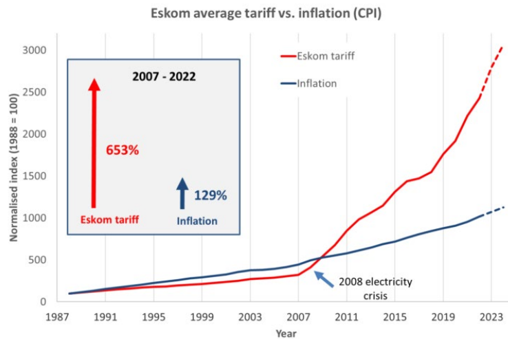
Figure 5: Graph illustrating the average Eskom tariff vs. Inflation (Power Optimal, 2022)
