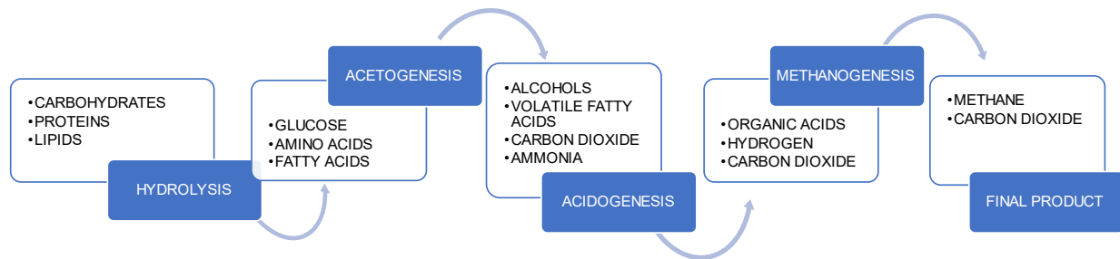
Figure 9: Summary of Anaerobic Digestion Process (adapted from Tshemese et al. , 2023).
