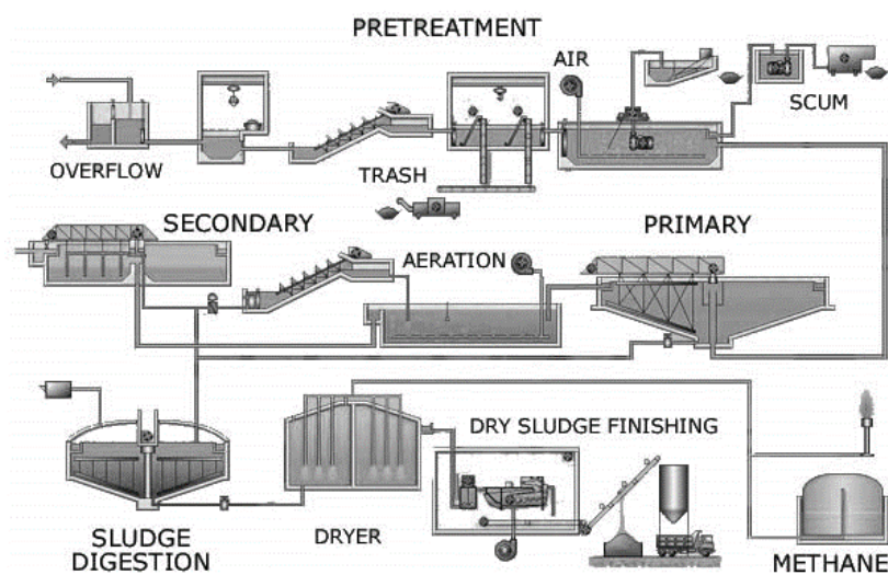
Figure 1: Wastewater Treatment Plant Process Diagram. Source: Environmental Information System (2006)
