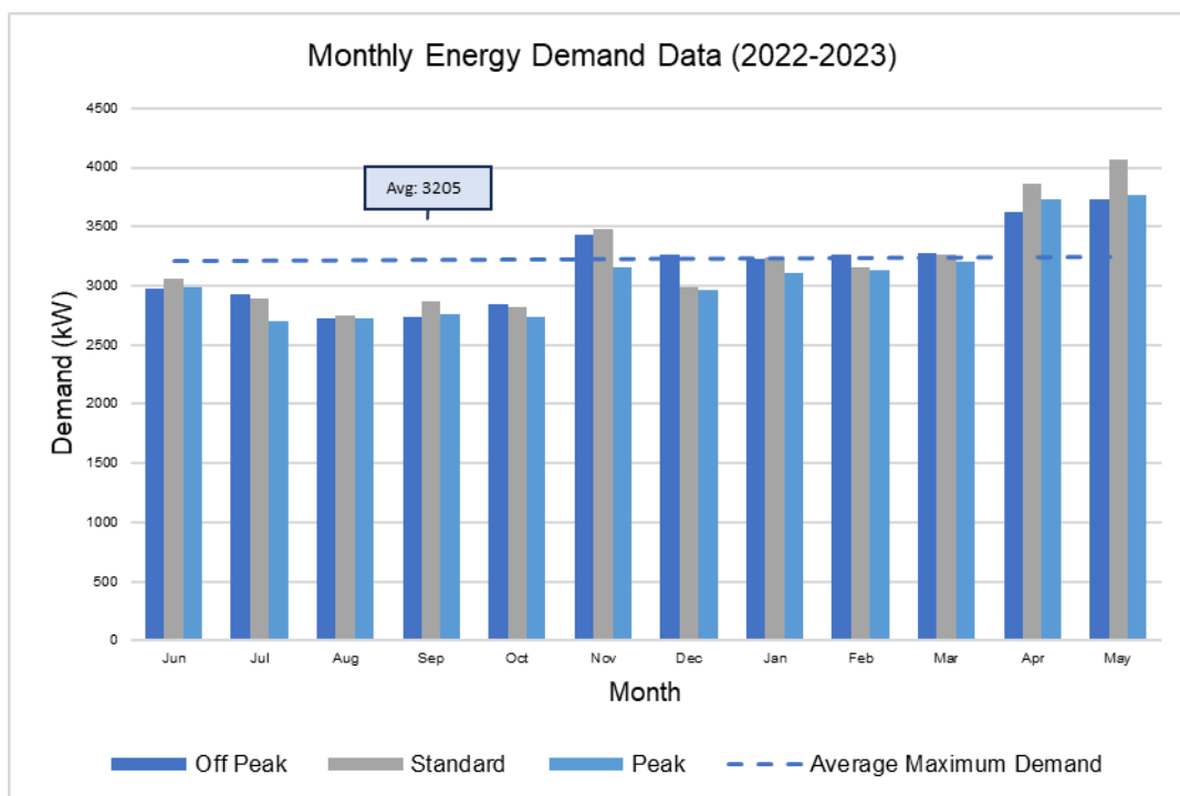
Figure 20: Month Energy Demand Data (2022-2023)
