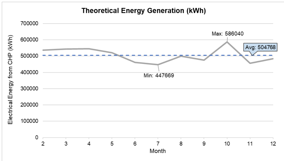
Figure 18: Theoretical Energy Generation Potential from Sludge Produced on Site
