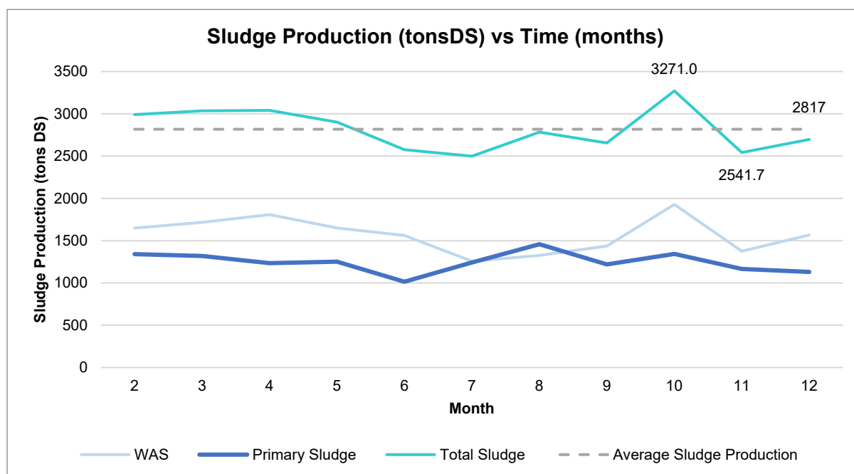
Figure 17: Graph to show the PS and WAS production over time
