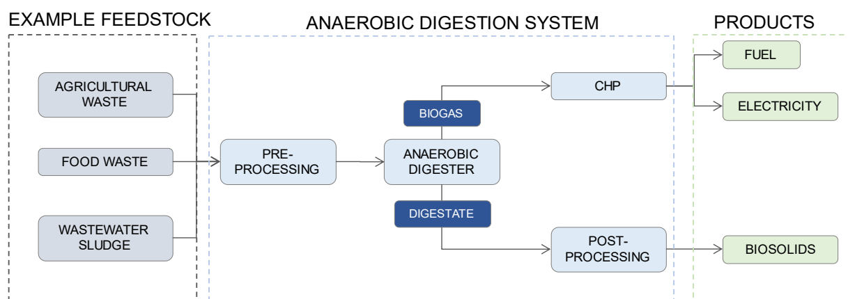
Figure 8: Process flow for AD at WWTPs (Adapted from Cambi, 2022)
