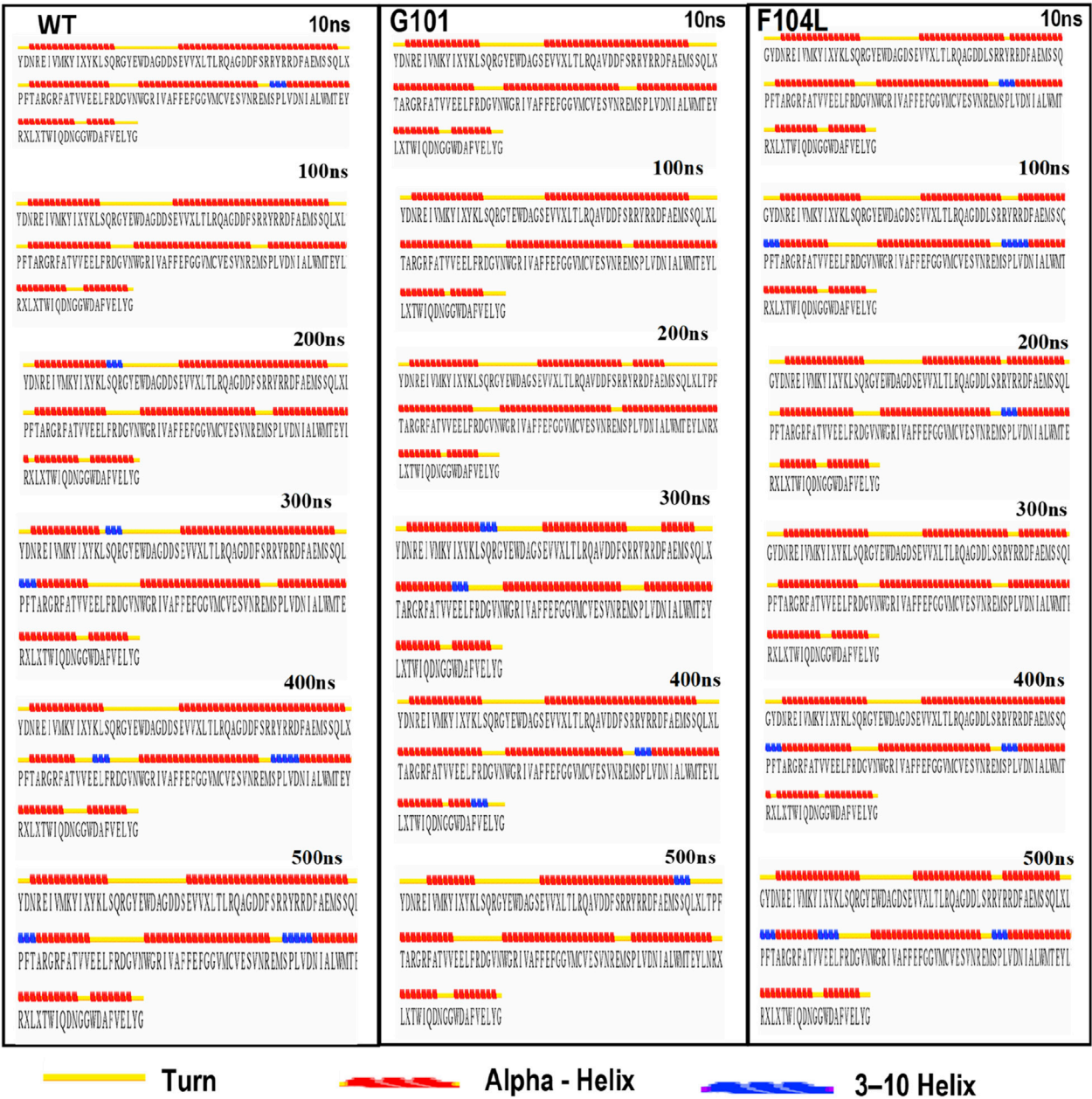
FIGURE 10 The secondary structural analysis of the Bcl-2 WT , Bcl-2 G101V , and Bcl-2 F104L at 10, 100, 200, 300, 400, and 500 ns using the STRIDE web server.
