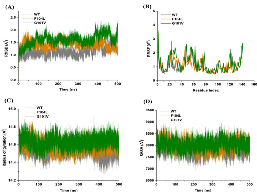
FIGURE 11 (A) RMSD, (B) RMSF, (C) Rg, and (D) SASA values across Cα of Bcl-2WT (gray), Bcl-2F104L (orange), and Bcl-2G101V (green) over 500 ns MD simulations.
