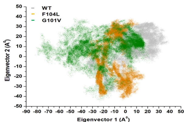
FIGURE 14 PCA for Bcl-2 WT (gray), Bcl-2 F104L (orange), and Bcl-2 G101V (green) over the 500ns MD simulations.
