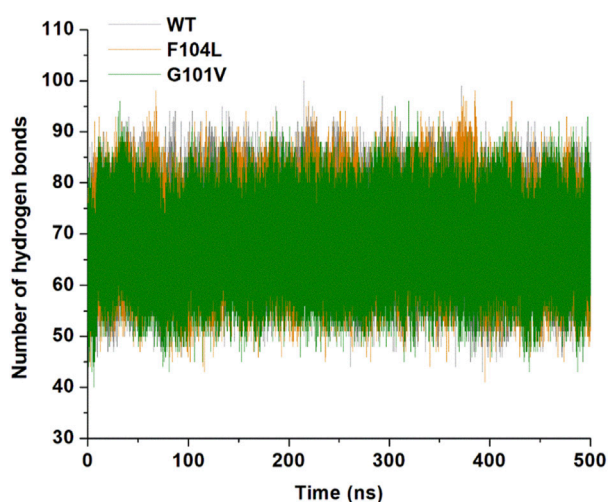
FIGURE 12 Intramolecular hydrogen bonding in Bcl-2WT (gray), Bcl-2F104L (orange), and Bcl-2G101V (green) over 500 ns MD simulations.
