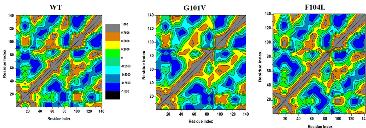
FIGURE 13 DCCM analyses for Bcl-2 WT , Bcl-2 G101V , and Bcl-2 F104L over 500 ns MD simulations.
