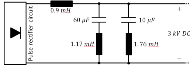
Figure 5: Diagram illustrating the equivalent circuit model of the typical harmonic filter at DC sub-stations in South Africa adapted from [2].
