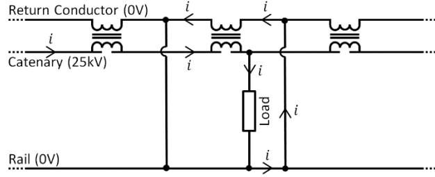
Figure 7: Diagram illustrating a simple equivalent model of a 25 kV AC traction system utilizing the booster transformer scheme.
