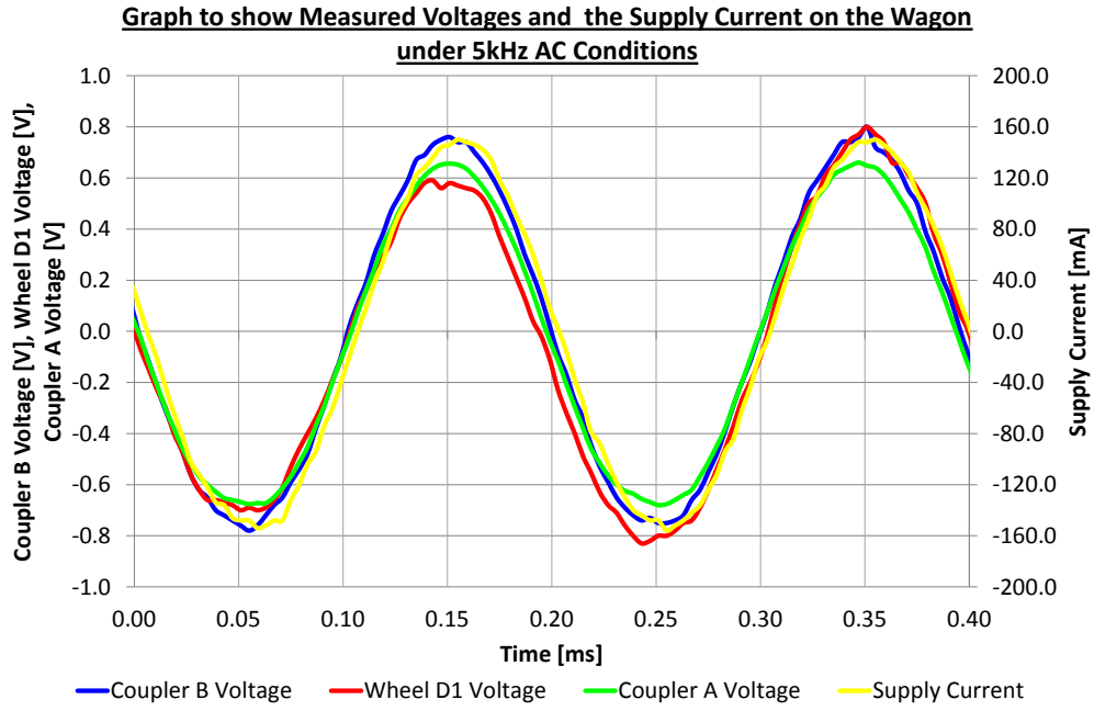
Figure 79: Graph showing wagon node voltages and supply current during measurements on the wheel D1.
