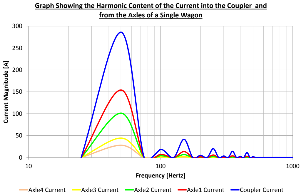
Figure 52: Graph showing the harmonic content of the current through the nodes of the 1 st wagon of the Coal Line train.
