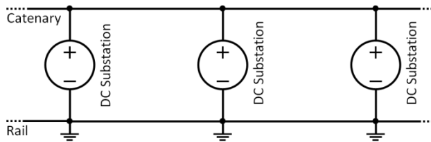
Figure 3: Diagram illustrating a simplified equivalent model of the DC traction system.
