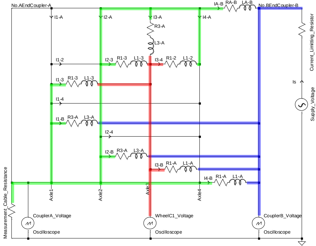
Figure 81: Circuit diagram of wagon model whilst under measurements on the wheel C1.
