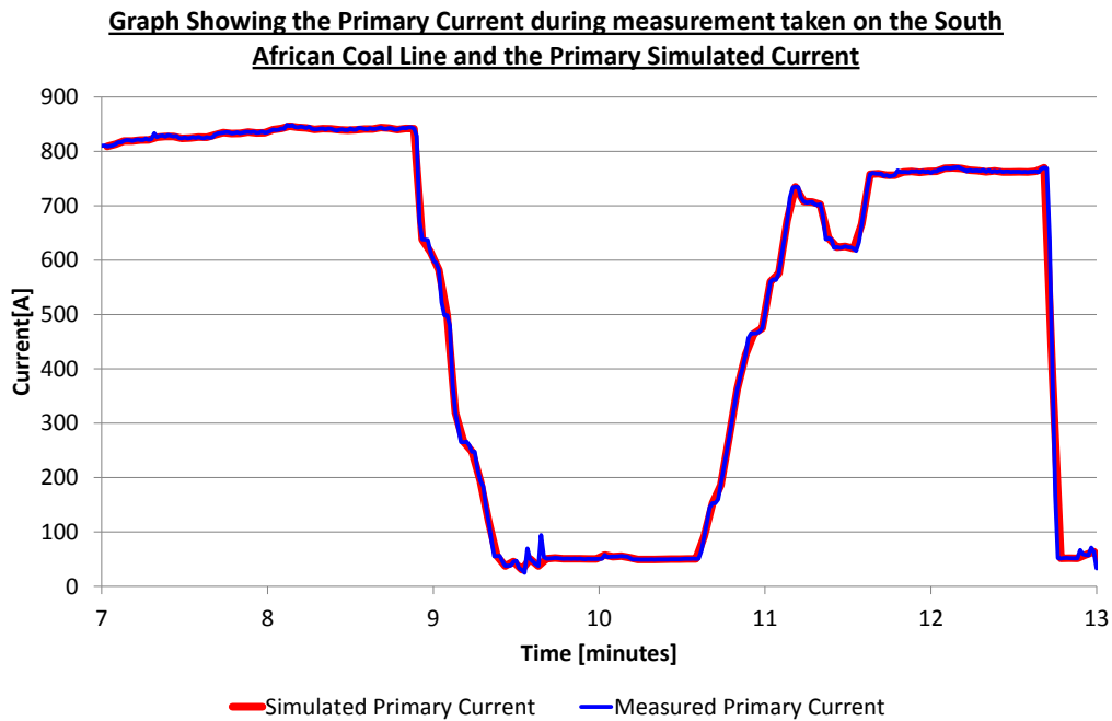
Figure 47: Graph showing the Transnet measured primary current and the simulated primary current.
