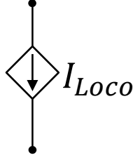
Figure 16: Diagram to show the ideal current source model of a modern locomotive utilising on-board power electronics.
