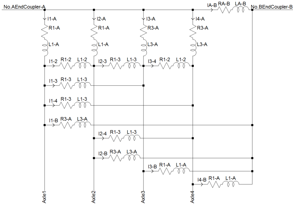
Figure 76: Diagram to show the reduced complex wagon model.
