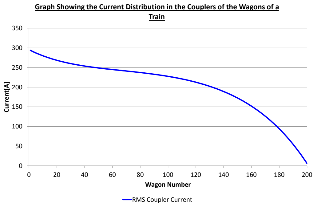
Figure 54: Graph showing current distribution in the couplers of the wagons of a Coal Line train.
