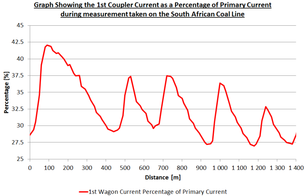
Figure 34: Graph showing the measurement results for the 1 st coupler currents against distance, obtained during measurements on the South African Coal Line.
