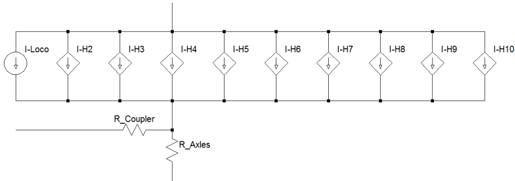
Figure 19: Diagram to show the multiple current source model of a modern locomotive utilising on-board power electronics.
