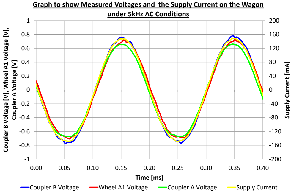
Figure 88: Graph showing wagon node voltages and supply current during measurements on the wheel A1.
