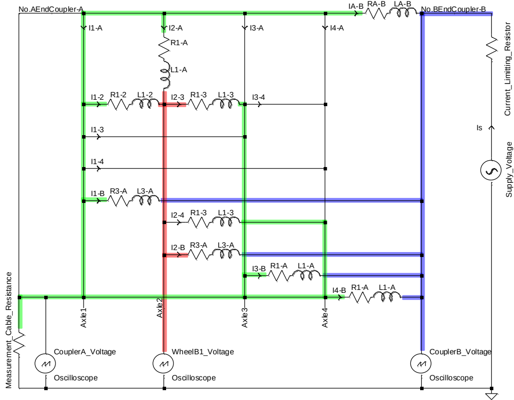
Figure 84: Circuit diagram of wagon model whilst under measurements on the wheel B1.
