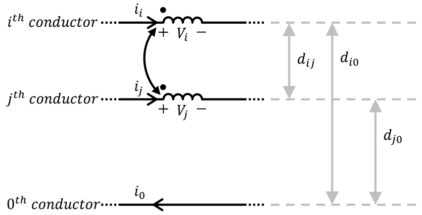
Figure 13: Diagram illustrating a 3 conductor MTL.
