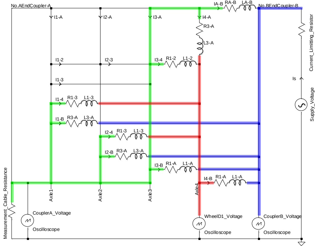
Figure 78: Circuit diagram of wagon model whilst under measurements on the wheel D1.
