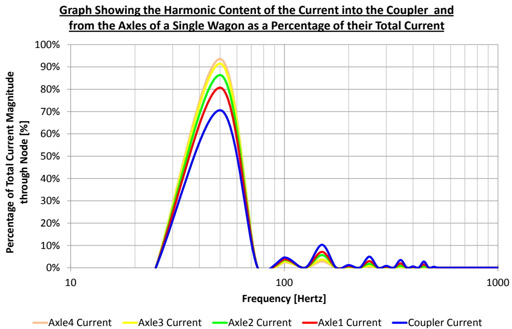
Figure 53: Graph showing the harmonic content of the current through the nodes of the 1 st wagon of the Coal Line train as a percentage of their respective total current.
