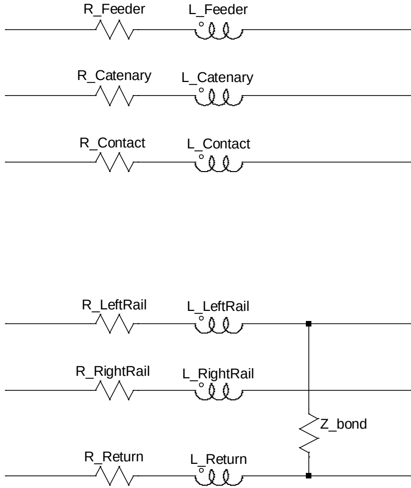
Figure 26: Diagram to show the extended lumped impedance supply model per meter inclusive of oscillating rail-to-mast bond.
