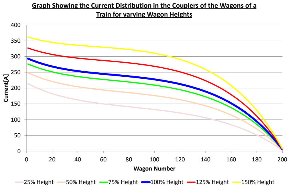
Figure 59: Graph showing current distribution in the couplers of the wagons of a Coal Line train under varying wagon heights.
