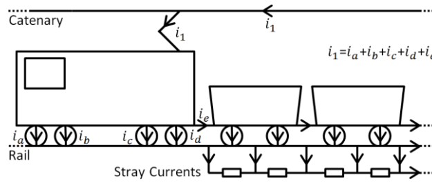
Figure 9: Diagram illustrating the possible return current paths immediately subsequent to the locomotive.
