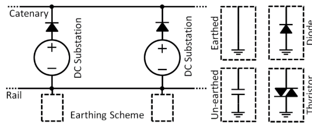
Figure 6: Diagram illustrating a simple equivalent model of the DC traction system
