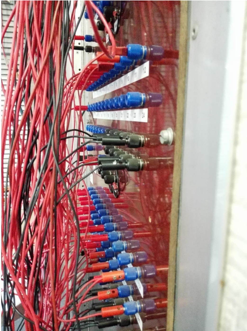
Figure 90: Photograph showing the front of the Transnet Freight Rail patch panel on one of their test coaches.
