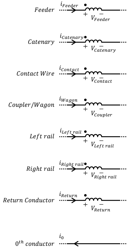
Figure 25: Diagram illustrating the typical Coal Line supply configuration with a train as a MTL.
