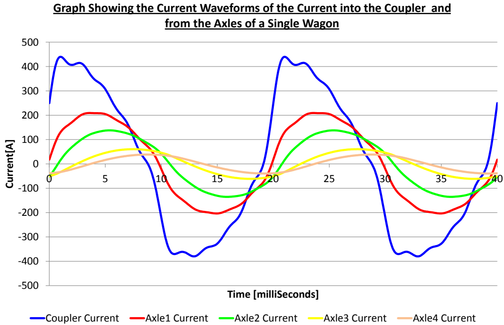
Figure 51: Graph showing the waveforms of the current through the nodes of the 1 st wagon of the Coal Line train.
