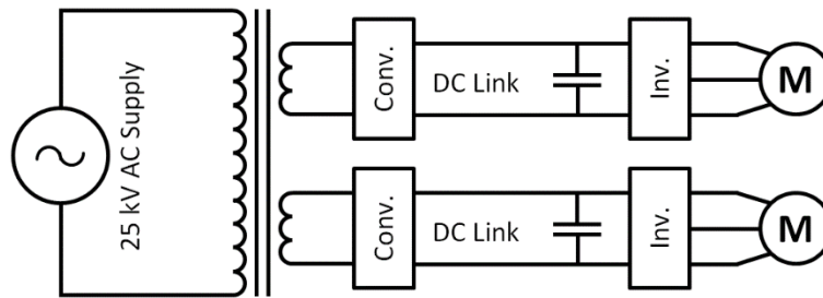
Figure 14: Diagram to show the simplified flow of power in a modern locomotive feeding from an AC supply.
