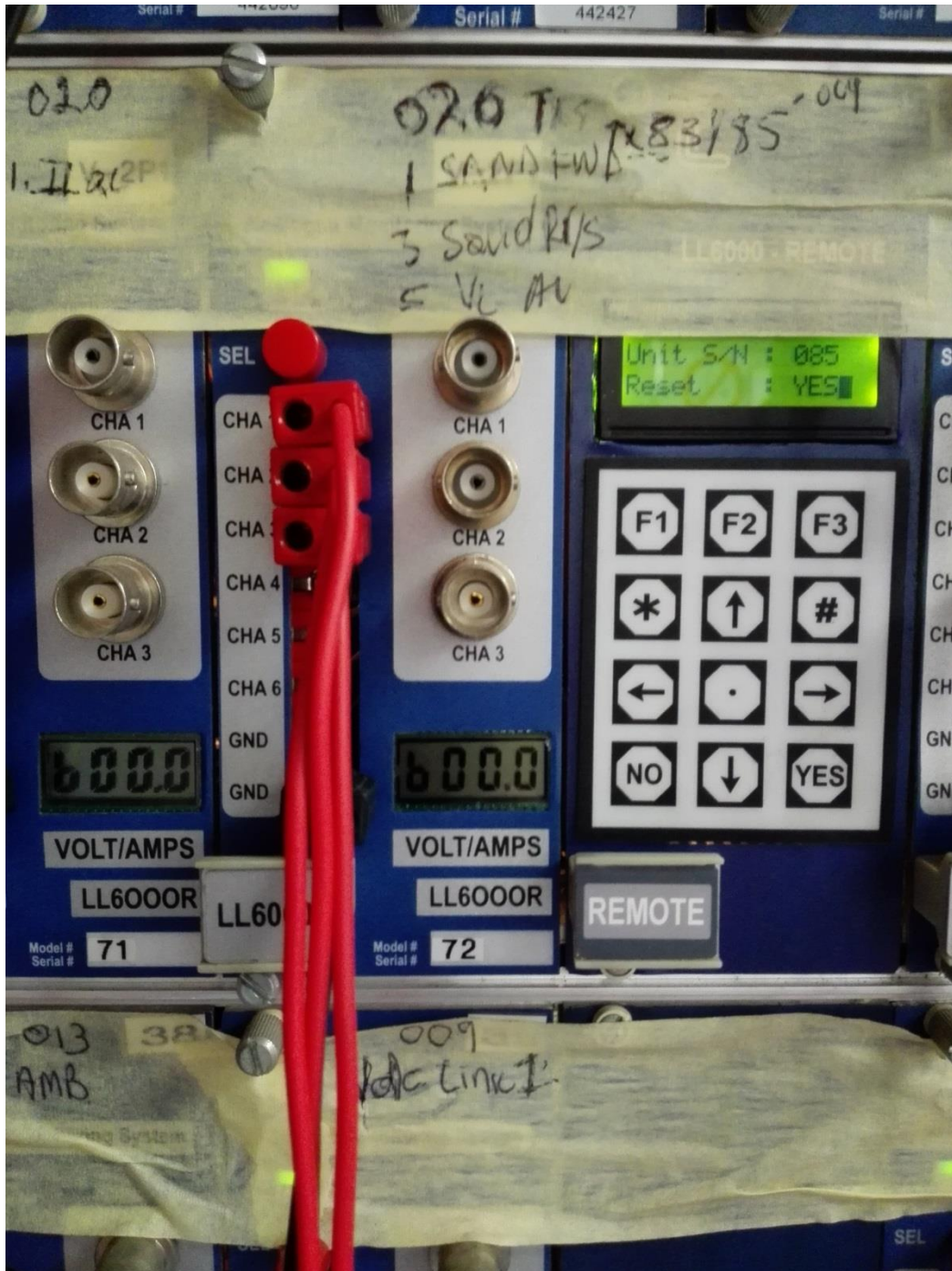
Figure 92: Photograph showing the front of the Transnet Freight Rail fiber optic receivers on one of their test coaches.
