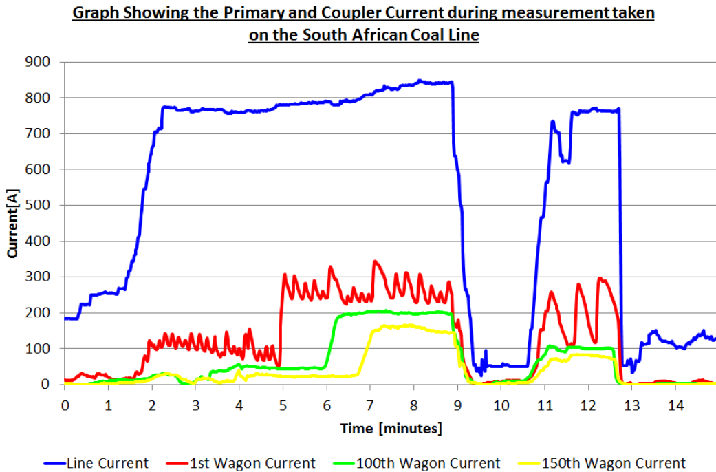
Figure 33: Graph showing the measurement results for line and coupler currents obtained during measurements on the South African Coal Line.
