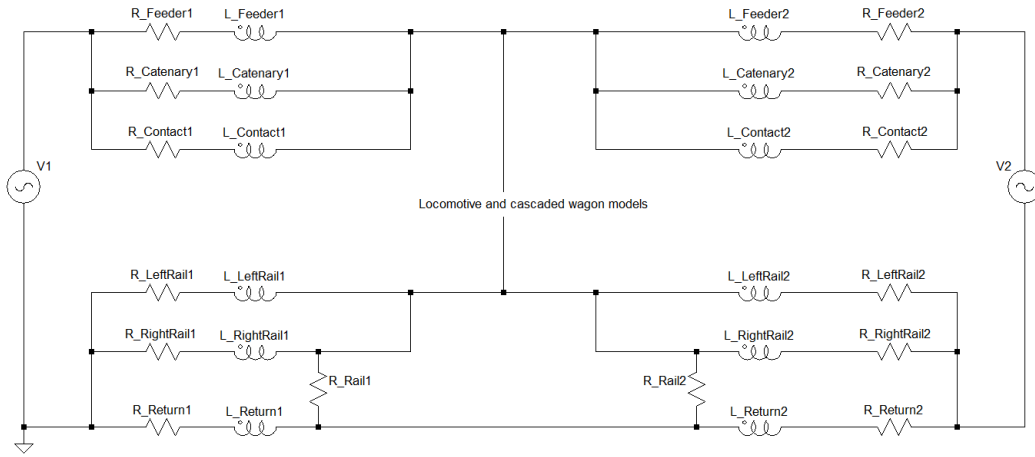
Figure 27: Diagram to show the Lumped Impedance, Parallel Supply Model.
