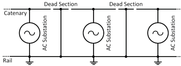
Figure 1: Diagram illustrating a simplified equivalent model of the AC traction system.
