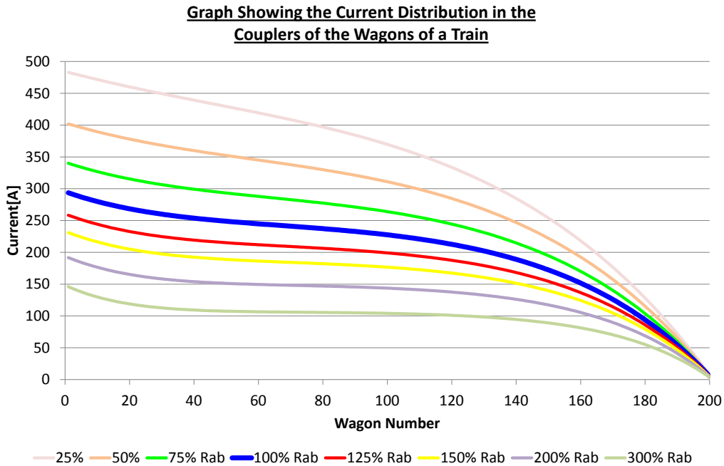
Figure 55: Graph showing current distribution in the couplers of the wagons of a Coal Line train under varying coupler to coupler resistance.
