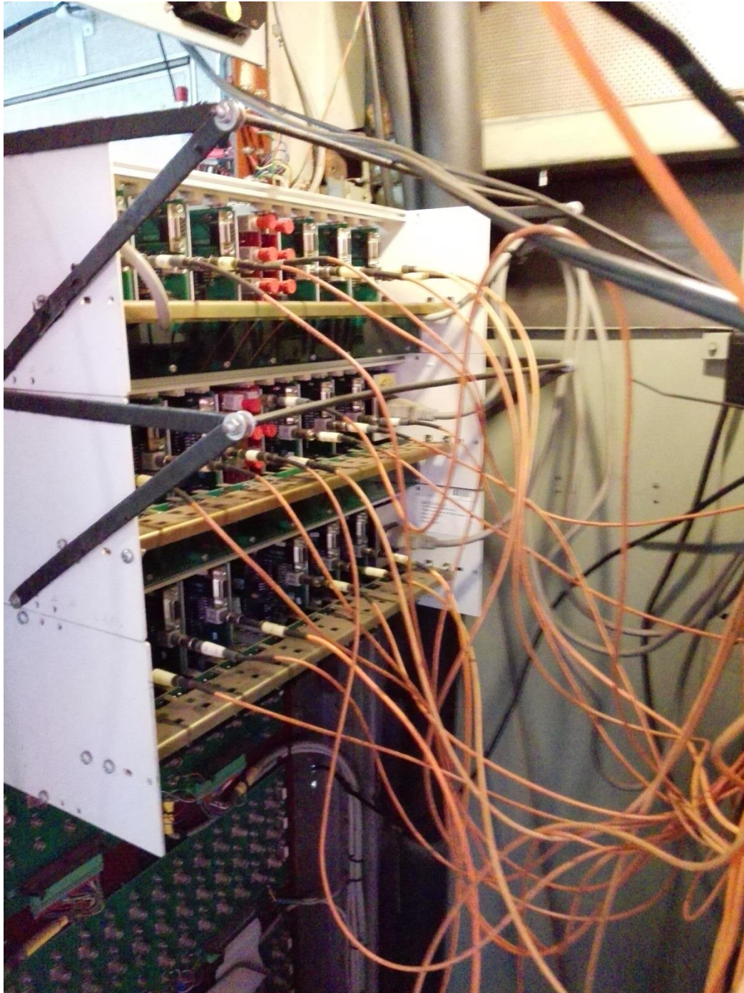
Figure 95: Photograph showing the connection of the optic cables to the receivers on one of Transnet Freight Rail's test coaches.
