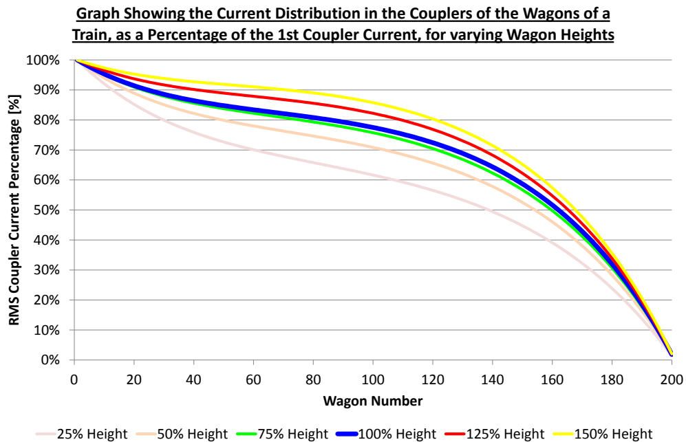
Figure 60: Graph showing current distribution in the couplers of the wagons of a Coal Line train, as a percentage of the 1 st coupler current, under varying wagon heights.
