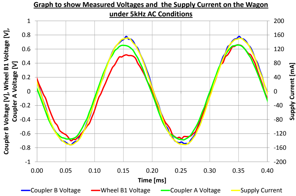
Figure 85: Graph showing wagon node voltages and supply current during measurements on the wheel B1.
