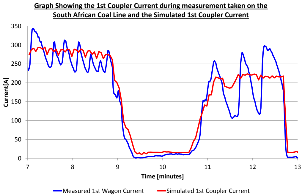
Figure 48: Graph showing the Transnet measured 1 st coupler current and the simulated 1 st coupler current.
