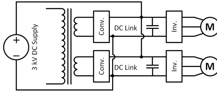
Figure 15: Diagram to show the simplified flow of power in a modern dual voltage locomotive feeding from a DC supply.
