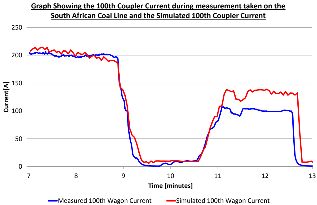
Figure 49: Graph showing the Transnet measured 100 th coupler current and the simulated 100 th coupler current.
