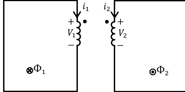
Figure 12: Diagram to 2 current carrying loops with dot convention.
