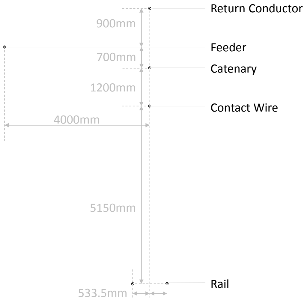
Figure 23: Diagram to show the typical supply infrastructure geometrical dimensions on the Transnet Coal Line.
