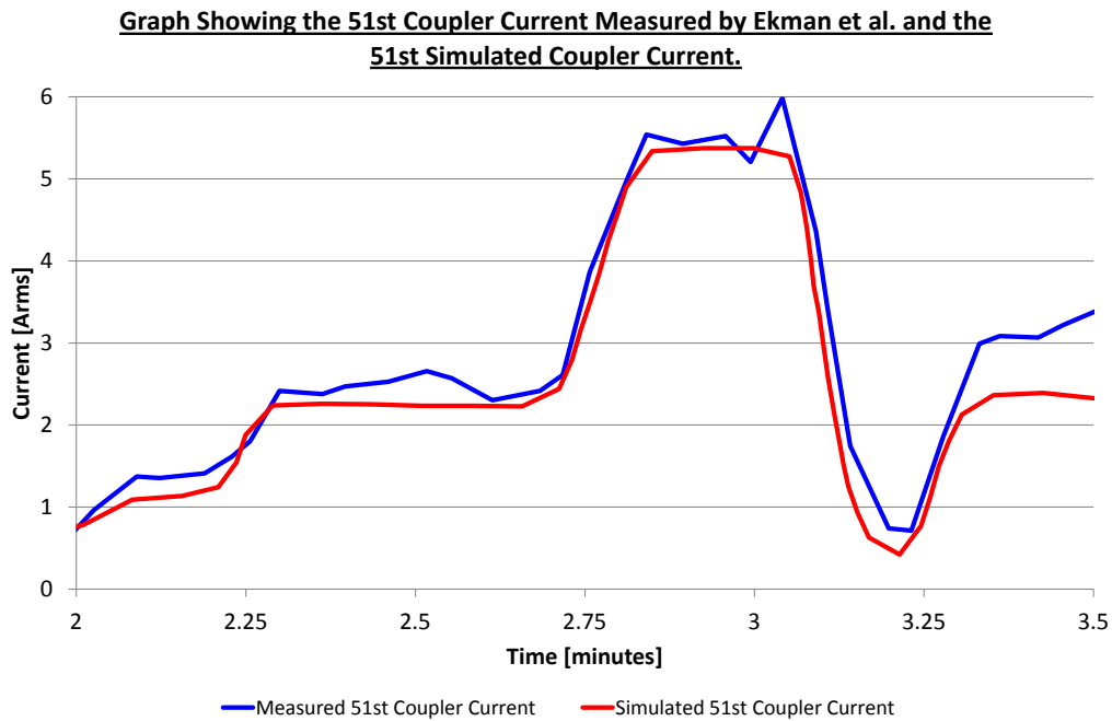
Figure 46: Graph showing the Ekman et al. measured 51 st coupler current and the simulated 51 st coupler current.
