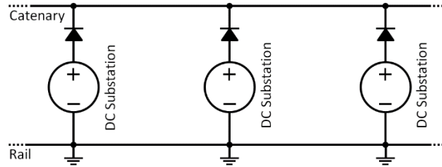
Figure 4: Diagram illustrating a simplified equivalent model of the one way DC traction supply system.
