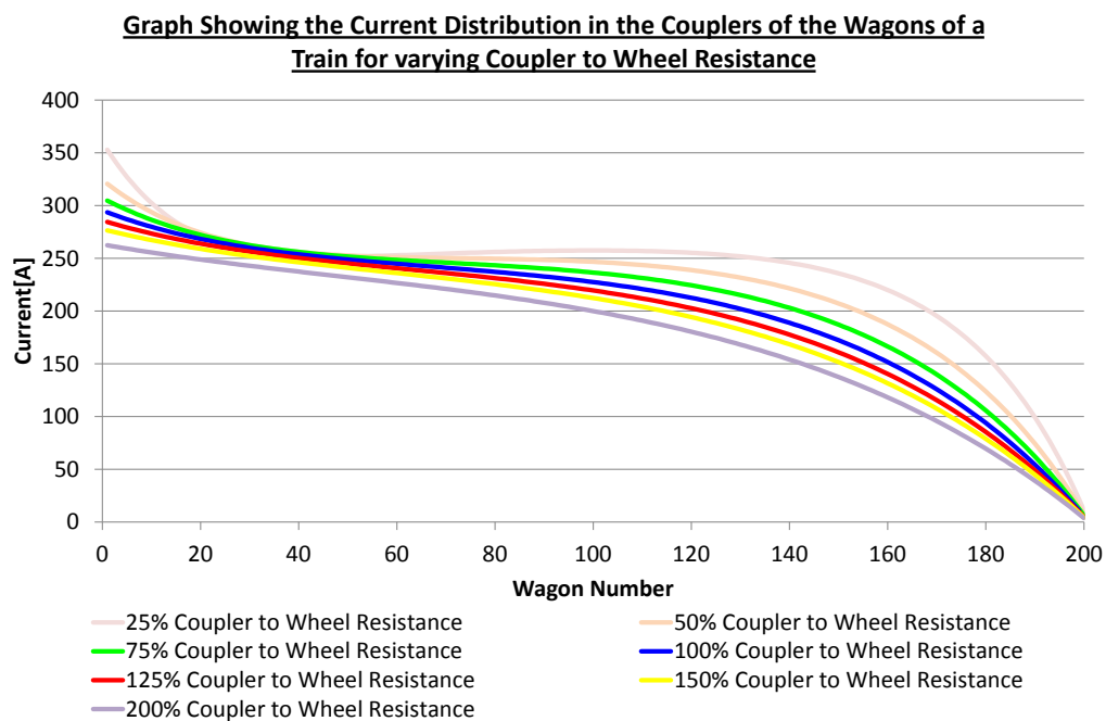
Figure 57: Graph showing current distribution in the couplers of the wagons of a Coal Line train under varying coupler to wheel resistance.
