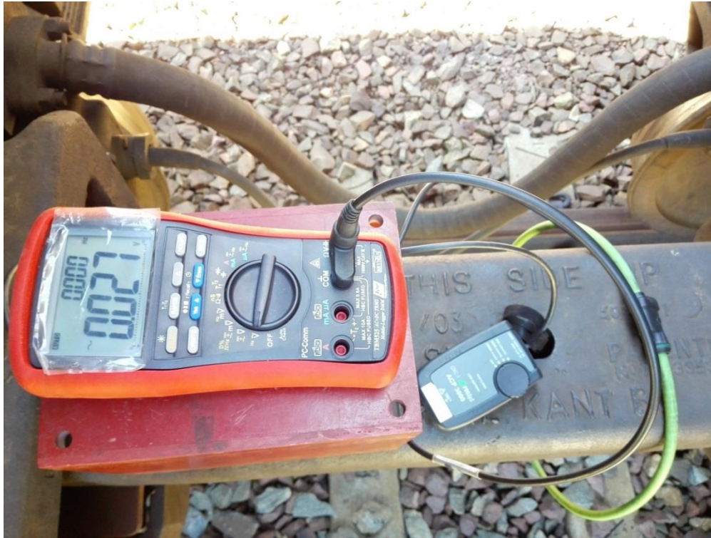
Figure 101: Photograph showing the remote logger and current clamp used to measure wagon currents at significant distance from the Transnet Freight Rail test coach.
