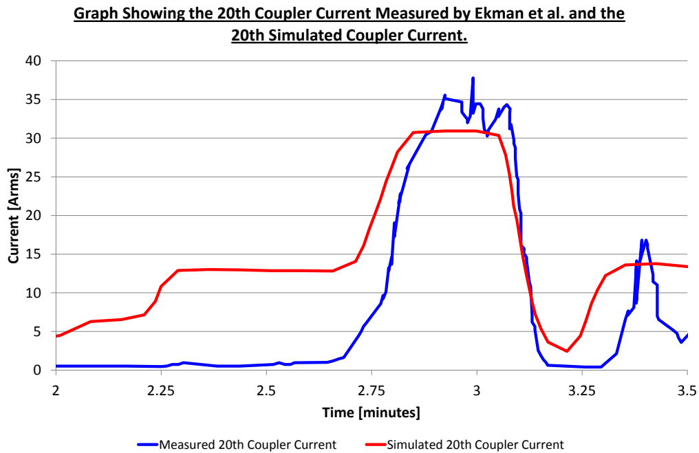
Figure 45: Graph showing the Ekman et al. measured 20 th coupler current and the simulated 20 th coupler current.
