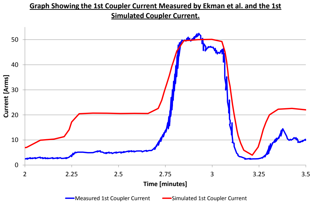
Figure 44: Graph showing the Ekman et al. measured 1 st coupler current and the simulated 1 st coupler current.
