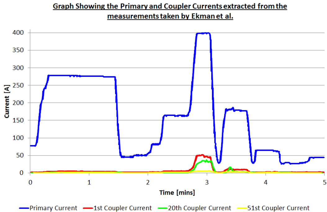
Figure 32: Graph showing the measurement results for line and coupler currents obtained by Ekman et al. during measurements in Sweden, extracted from [19].
