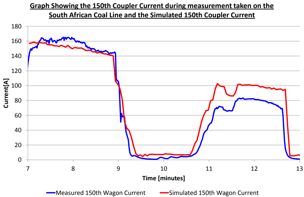
Figure 50: Graph showing the Transnet measured 150 th coupler current and the simulated 150 th coupler current.
