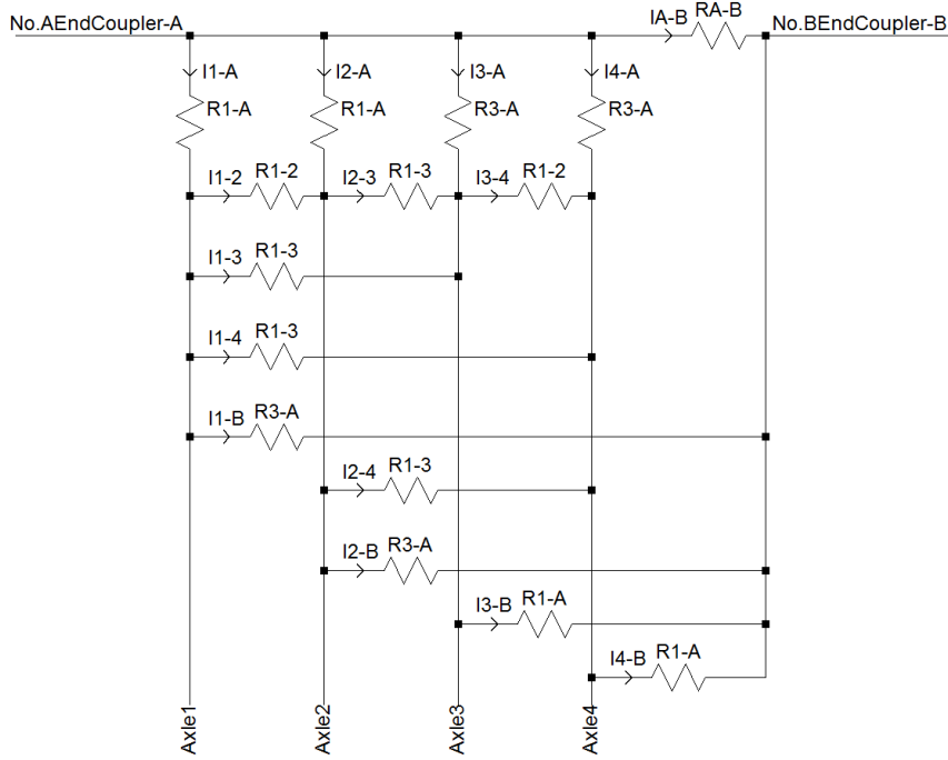
Figure 30: Diagram to show the reduced ideal wagon model from physical wagon symmetries.
