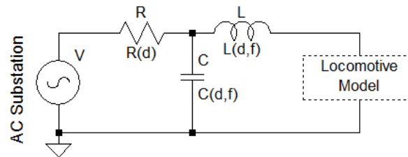
Figure 21: Diagram to show the lumped impedance supply model.
