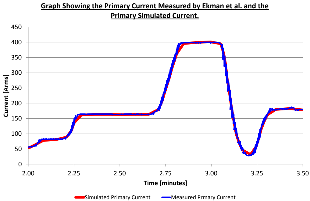
Figure 43: Graph showing the Ekman et al. measured primary current and the simulated primary current.
