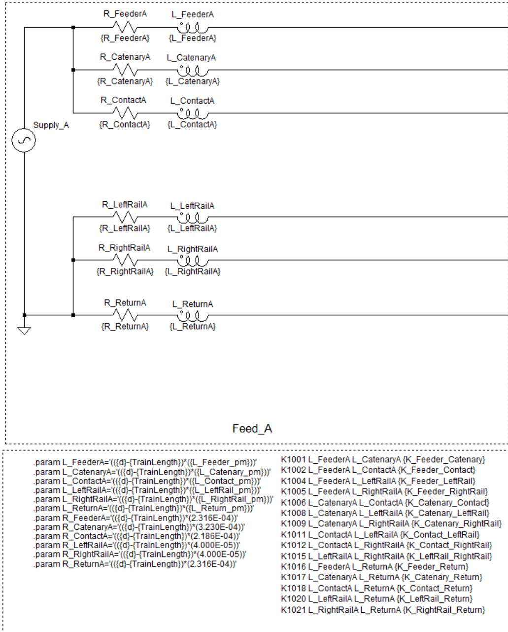
Figure 38: Figure showing the supply feed subsequent to the train for the main simulation circuit, extracted from Figure 35.
