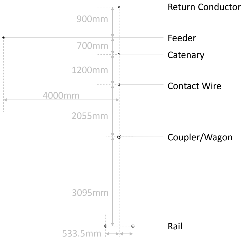
Figure 24: Diagram to show the typical supply infrastructure geometrical dimensions on the Transnet Coal Line inclusive of wagons modelled as a continuous drawbar.
