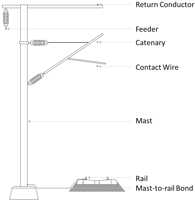
Figure 22: Diagram to show the typical supply infrastructure layout on the Transnet Coal Line.
