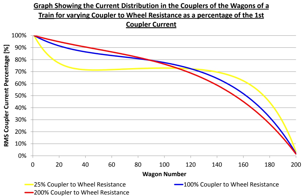
Figure 58: Graph showing current distribution in the couplers of the wagons of a Coal Line train under varying coupler to wheel resistance, as a percentage of the 1 st coupler current.
