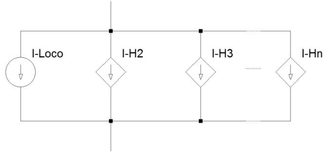
Figure 18: Diagram to show the multiple current source model of a modern locomotive utilising on-board power electronics.
