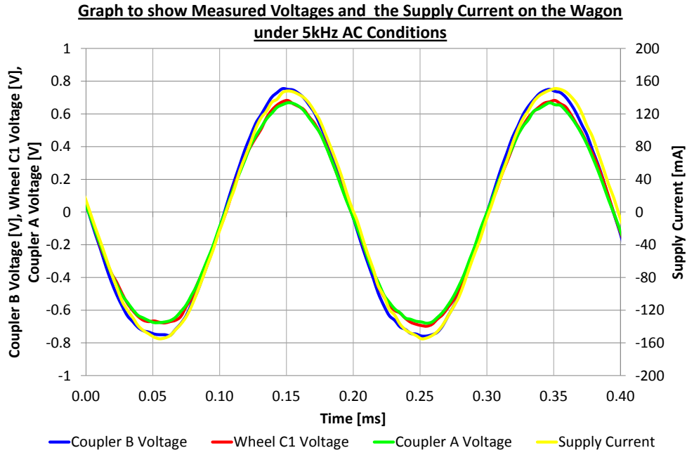
Figure 82: Graph showing wagon node voltages and supply current during measurements on the wheel C1.
