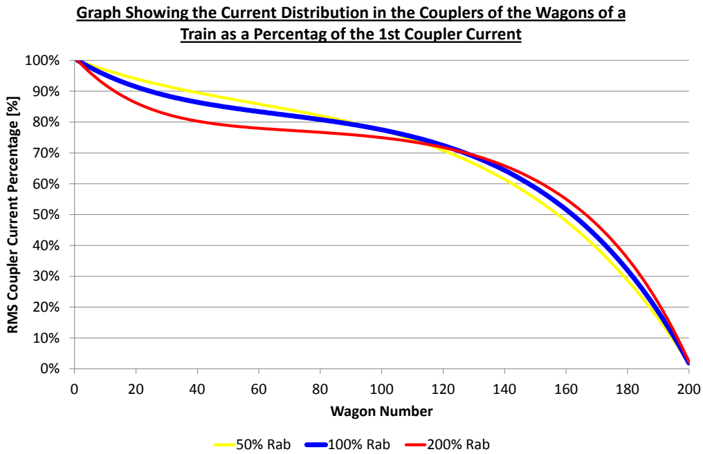
Figure 56: Graph showing current distribution in the couplers of the wagons of a Coal Line train under varying coupler to coupler resistance, as a percentage of the 1 st coupler current.
