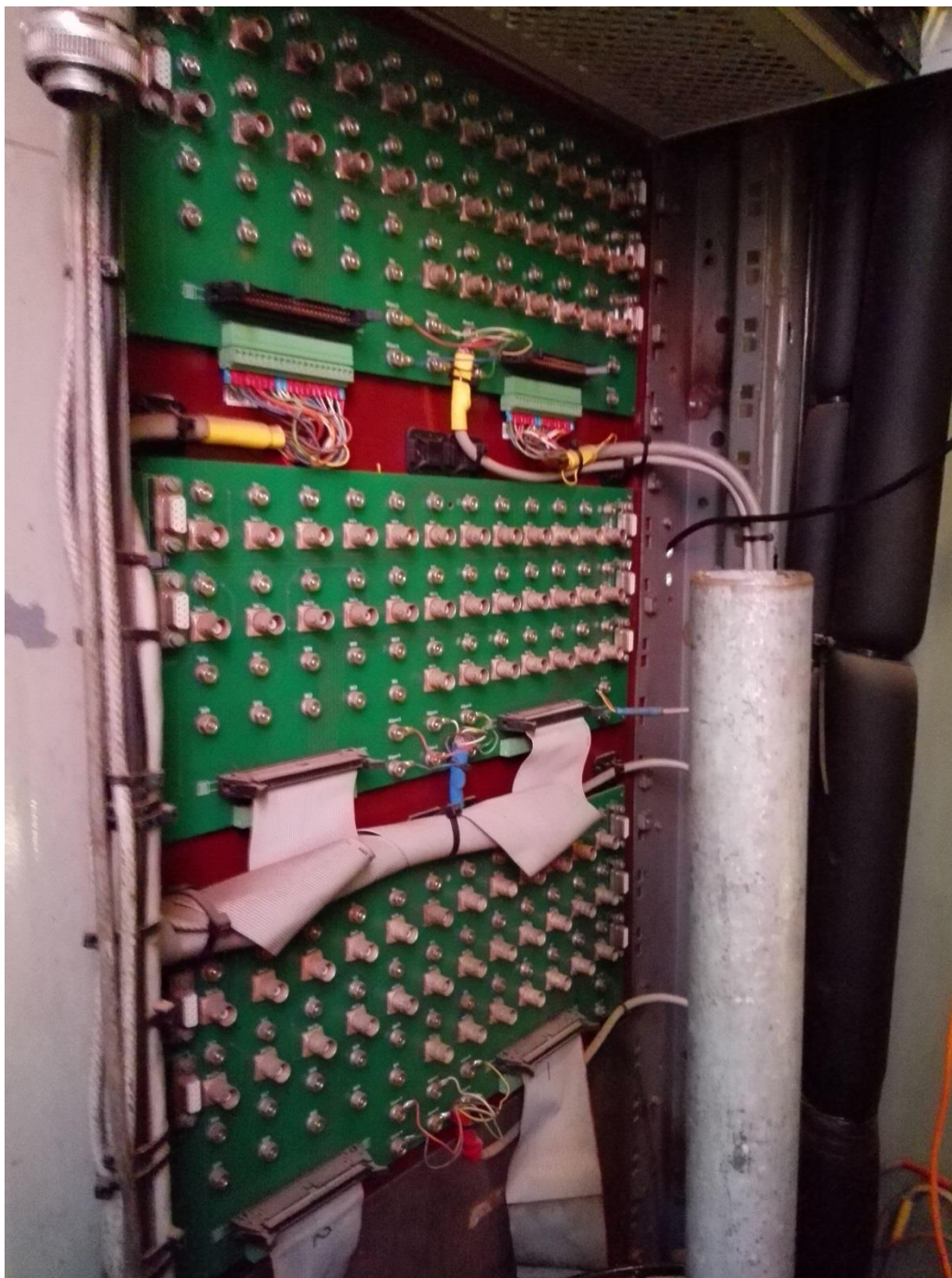
Figure 91: Photograph showing the back of the Transnet Freight Rail patch panel on one of their test coaches.
