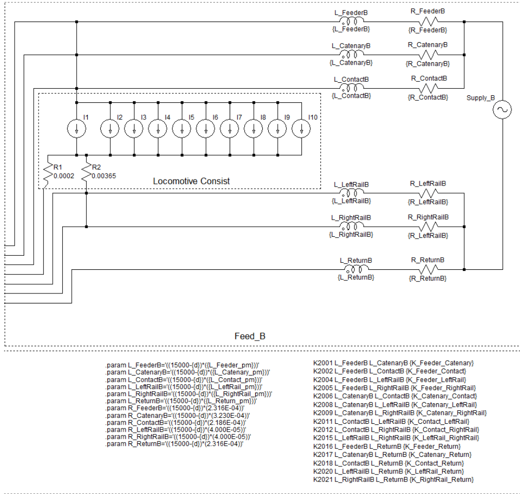
Figure 39: Figure showing the supply feed preceding the train as well as the locomotive consist for the main simulation circuit, extracted from Figure 35.
