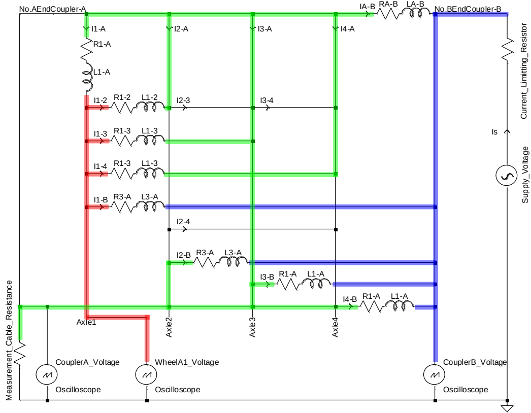
Figure 87: Circuit diagram of wagon model whilst under measurements on the wheel A1.
