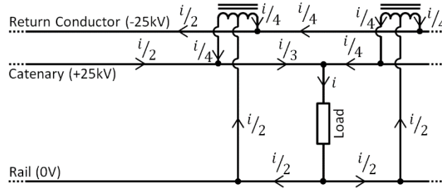
Figure 8: Diagram illustrating a simple equivalent model of a 2 x 25 kV AC traction system utilizing the auto transformer scheme.
