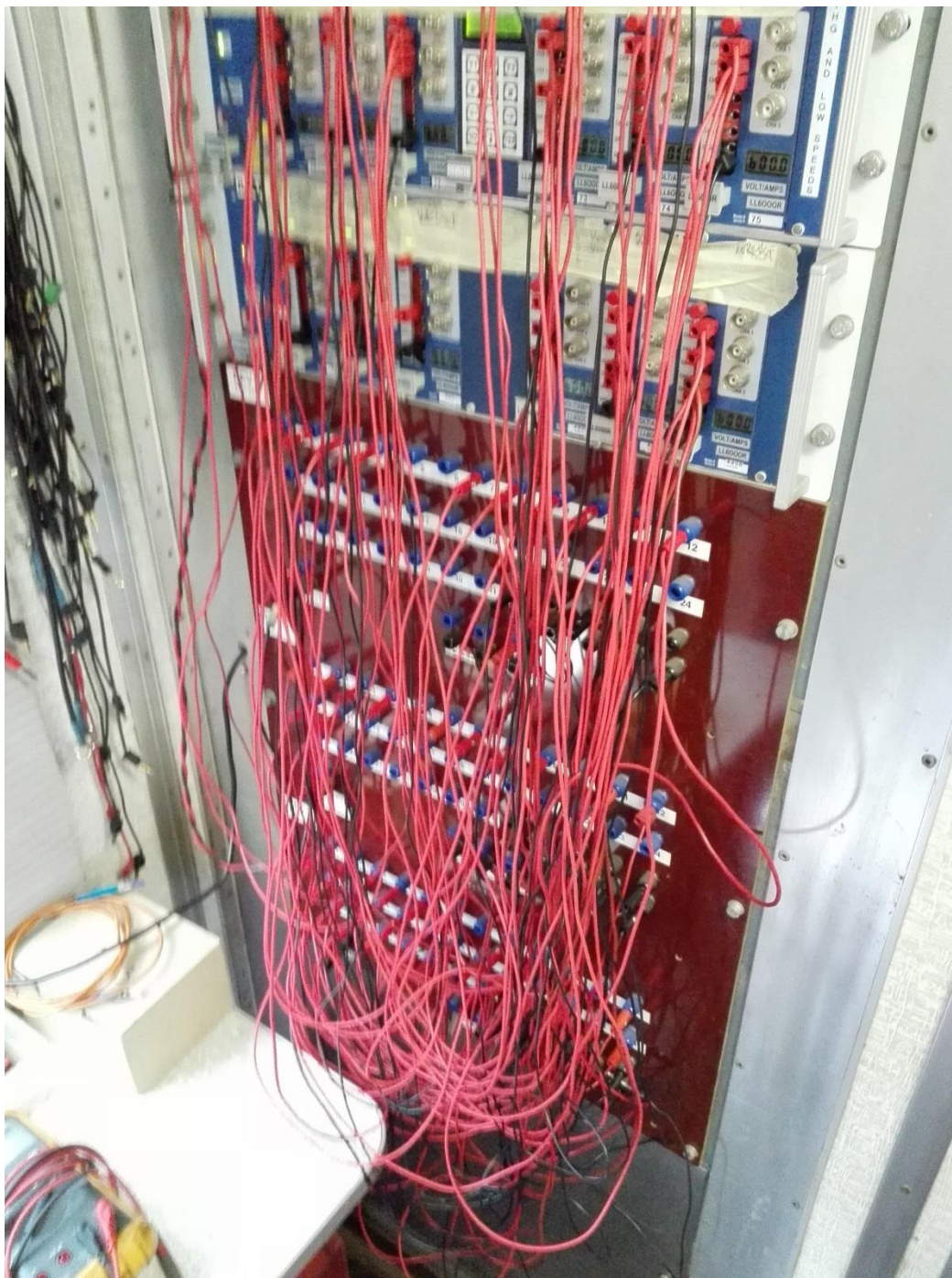
Figure 93: Photograph showing the connection from the optic receivers to the patch panel on one of Transnet Freight Rail's test coaches.
