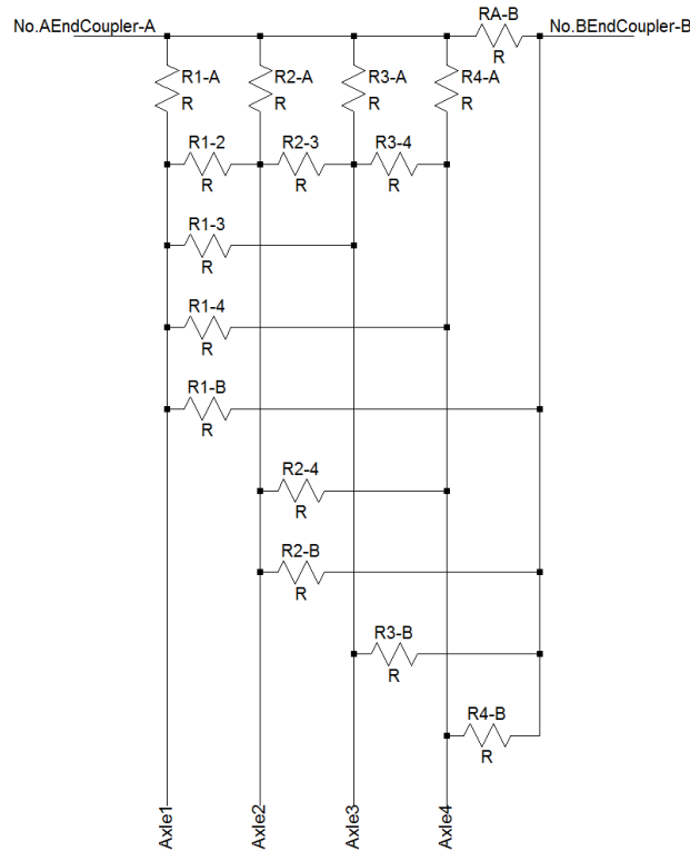
Figure 29: Diagram to show the reduced ideal wagon model from axle symmetries.
