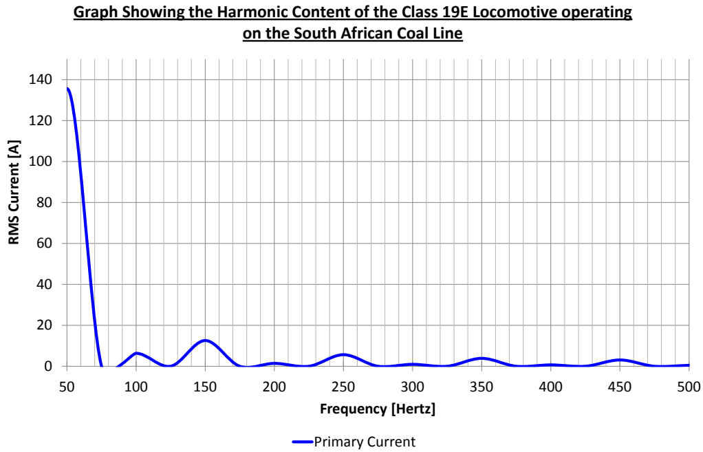
Figure 17: Diagram to show the harmonic content found in a typical modern locomotive utilising power electronics, extracted from [25].
