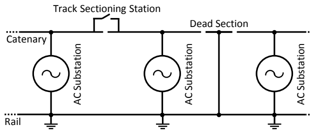
Figure 2: Diagram illustrating a simplified equivalent model of the dual feed AC traction system.
