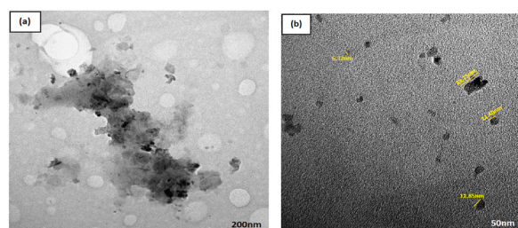
Fig. 1. TEM analysis of \text{TiO}_2 -DI water Nanofluid.
