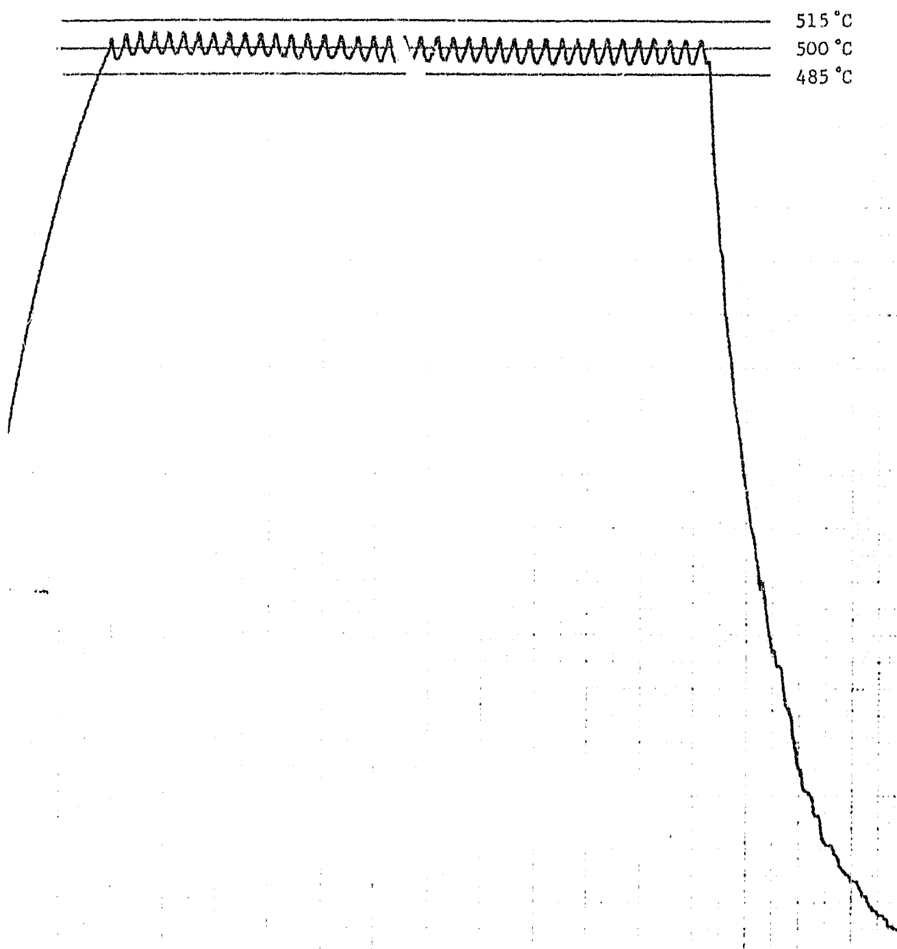
Figure 4.17 The ON-OFF controller does not maintain a constant temperature but the variation is small, \sim 15^{\circ}\text{C} at 500^{\circ}\text{C} .
