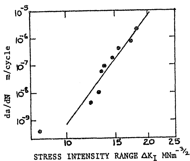
Figure 2.23 Fatigue crack growth rate in WC-11Co. 111
