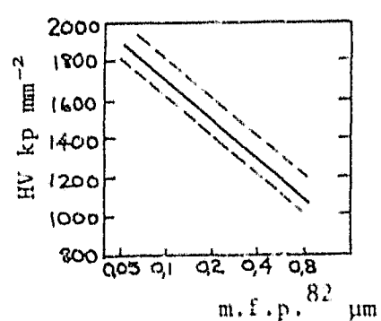
(c) Variation in hardness with mean free path of the cobalt binder. 57,82
