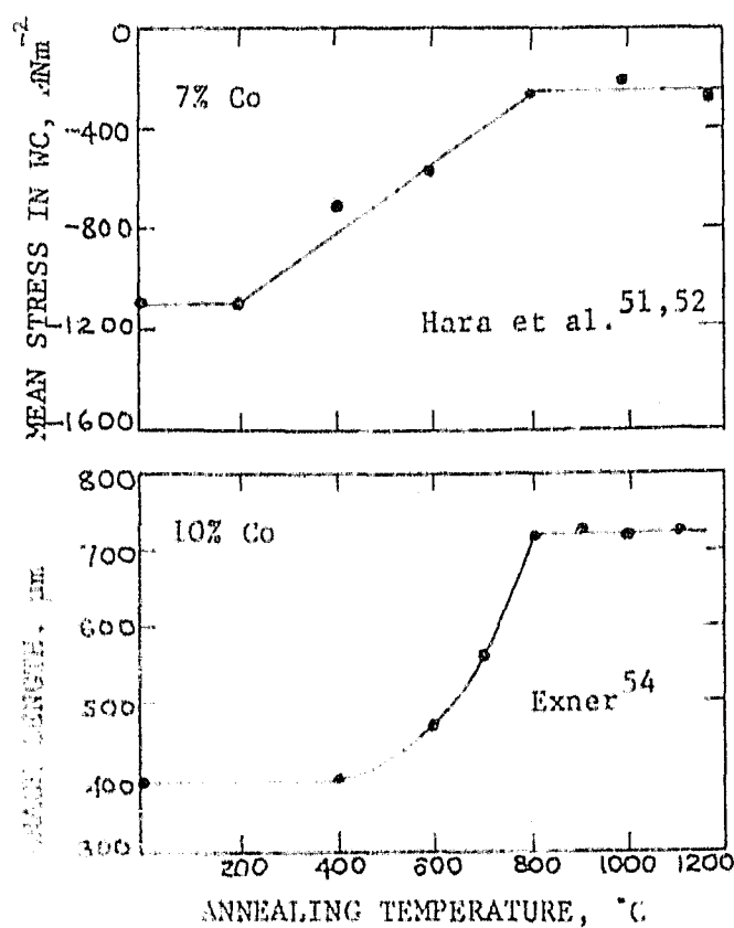
Figure 2.3 Residual stresses and crack length at Vickers indentations as a function of annealing temperature. 51,52,54
