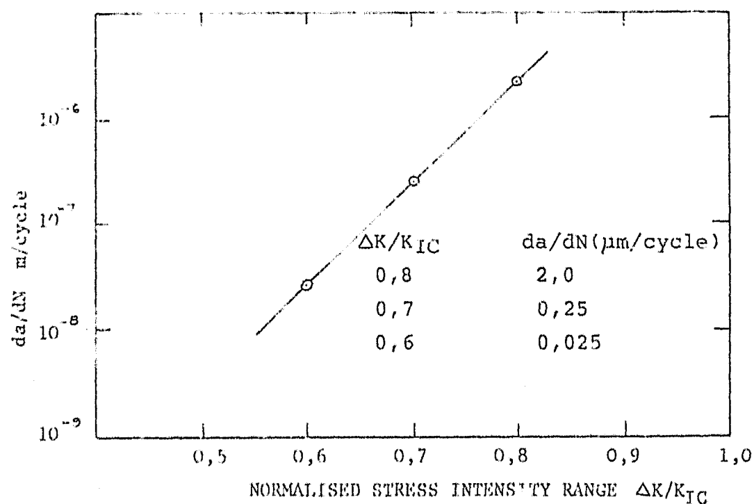
Figure 2.25 Normalised fatigue crack growth rate in WC-Co having K_{IC} \approx 17 \text{ MNm}^{-3/2} .
