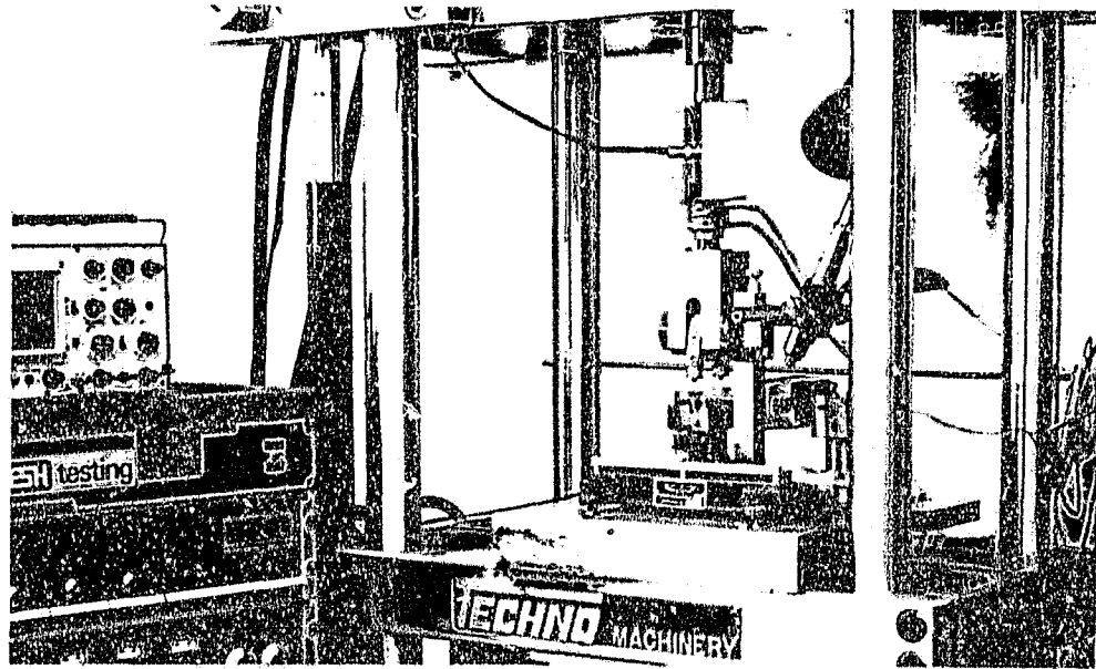
Figure 4.7 General view of test system.
