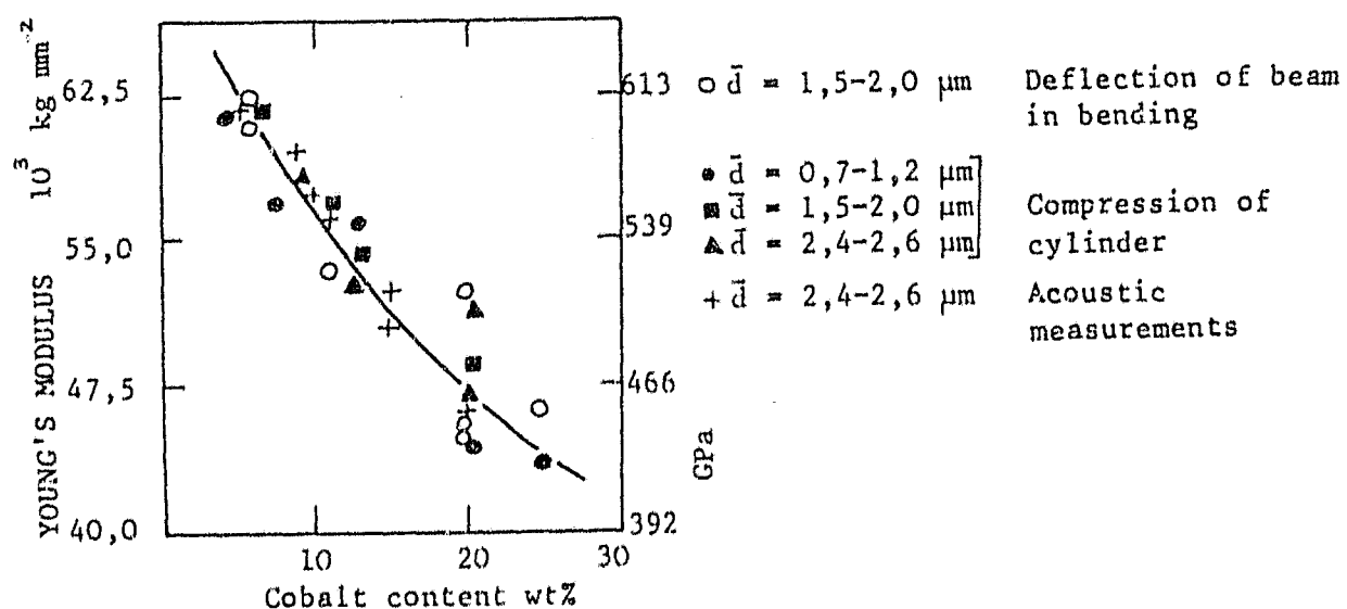
Figure 2.14 Variation in Young's modulus with cobalt content. 8
