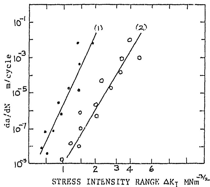
Figure 2.22 Fatigue crack growth rates measured by load relaxation in WC-6Co. 109
