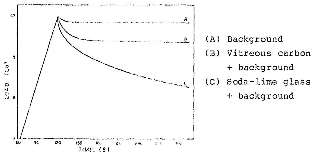
Figure 3.16 Typical load relaxation graph. 143
