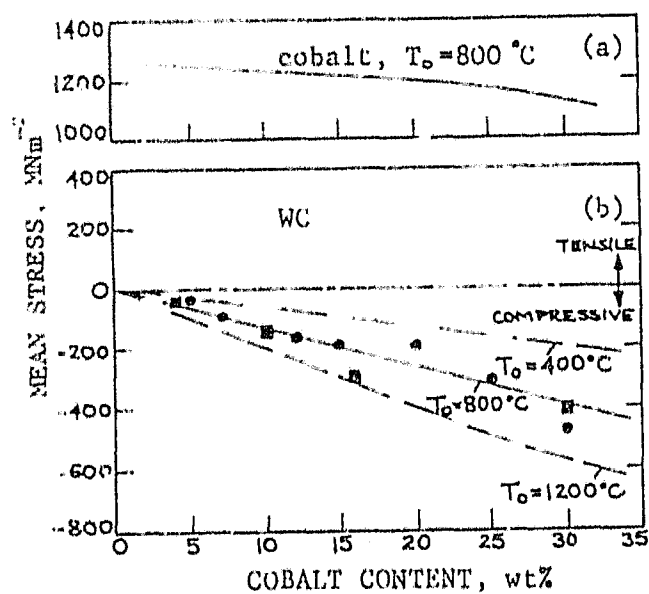
Figure 2.4 (a) Tensile stresses in cobalt, calculated. 3 (b) Compressive stresses in WC, data points from double X-ray exposure results of: ■ Öhman et al. 44 • Hara et al. 51,52 Theoretical curves after: Amberg 53 and Öhman 44
