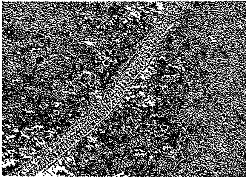
Figure 4.18 Electric pencil mark on fracture surface used to demarcate zones of different fatigue levels and fast fracture.
