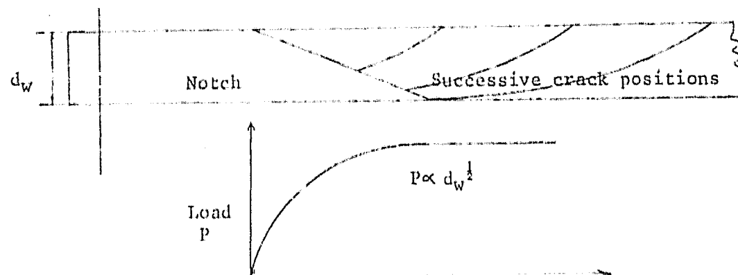
Figure 3.13 Sketch of load required for fracture using tapered starter notch.
