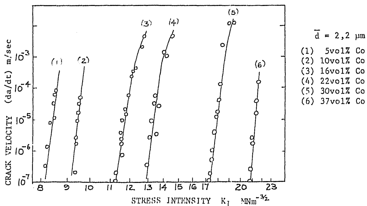
Figure 2.15 Static crack growth rates in WC-Co alloys 104
