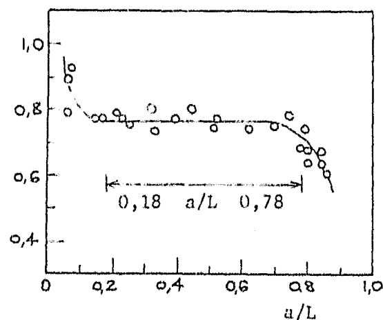
Experimental results of Pletka et al. 123 for crack length, a , in the range 0,05L to 0,85L . Validity limits predicted by Trantina 123 also shown.
