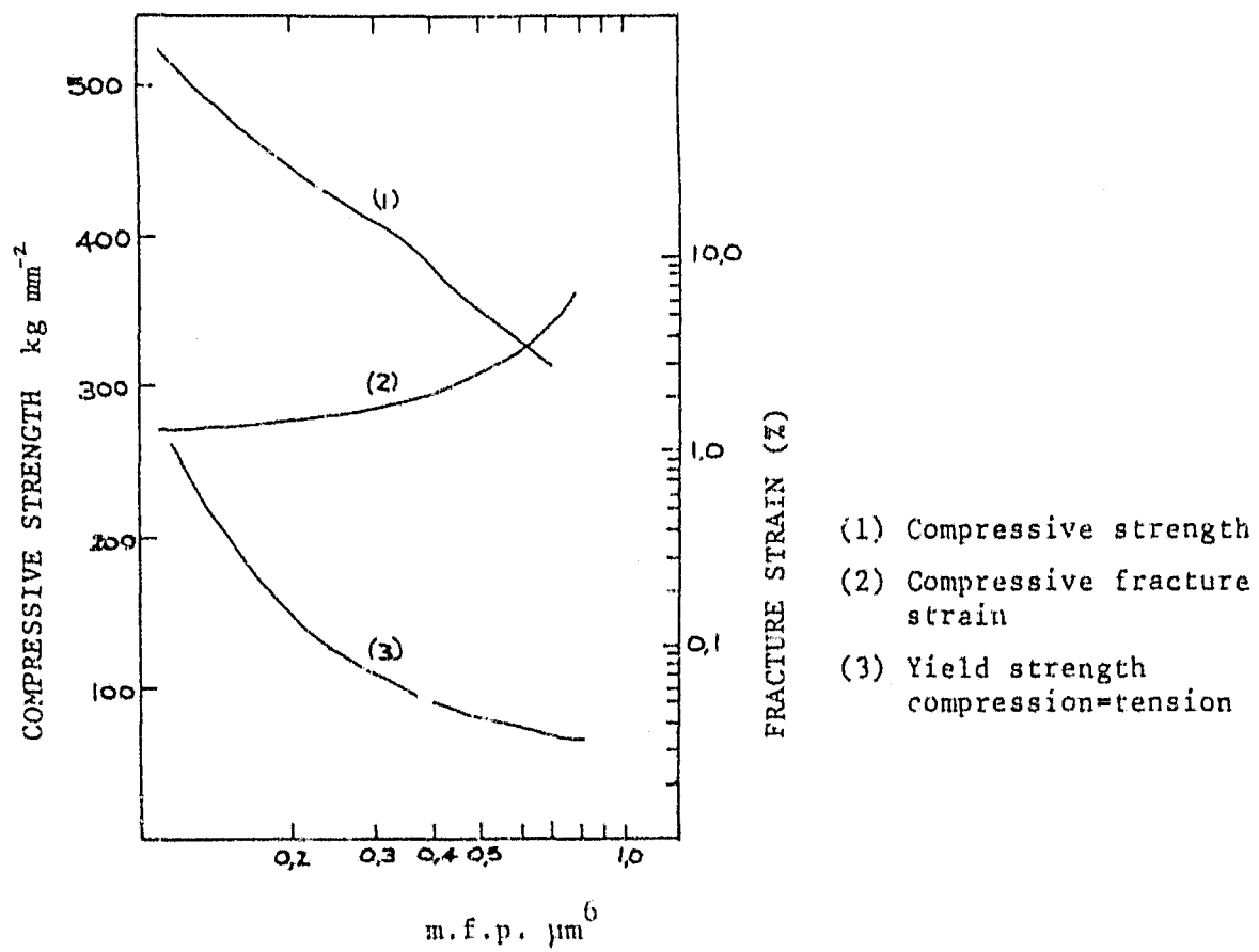
(c) Variation in compressive strength with mean free path of the cobalt binder. 6
