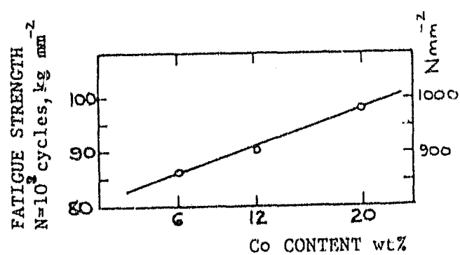
Figure 2.16 Effect of cobalt content on fatigue life using rotating beam test. 104
