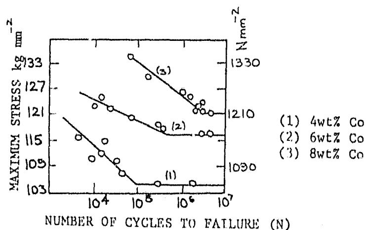
Figure 2.18 Effect of cobalt content on fatigue life using 3-point bend test. 107
