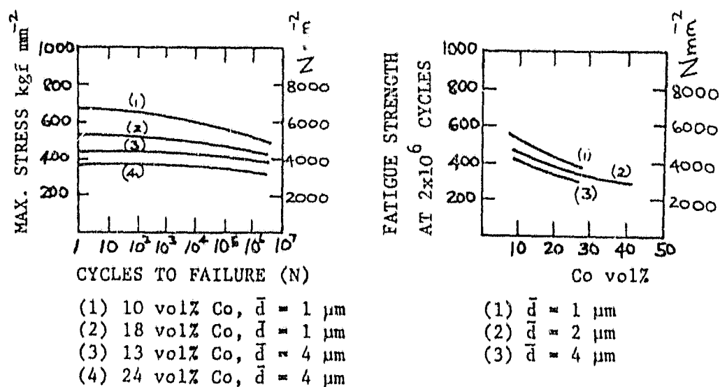
Figure 2.20 Effect of cobalt content on fatigue life in compression. 108
