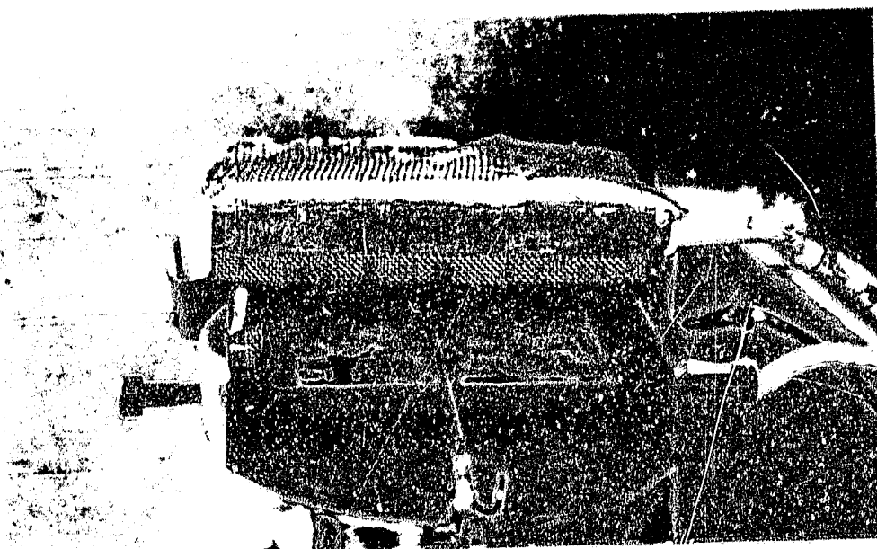
(a) Photograph showing heating unit in position around specimen.
