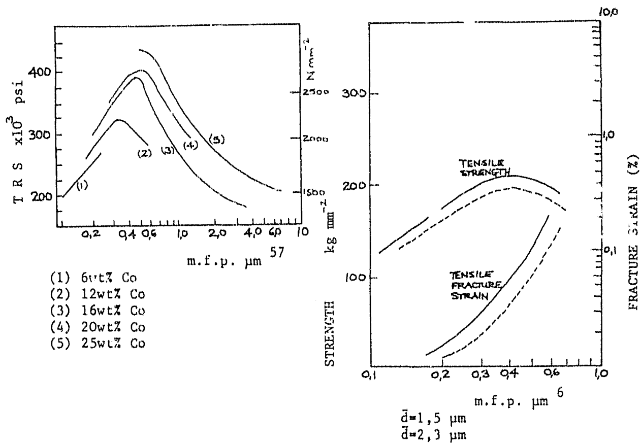
(c) Variation in the transverse rupture strength with mean free path of the cobalt binder. 6,57
