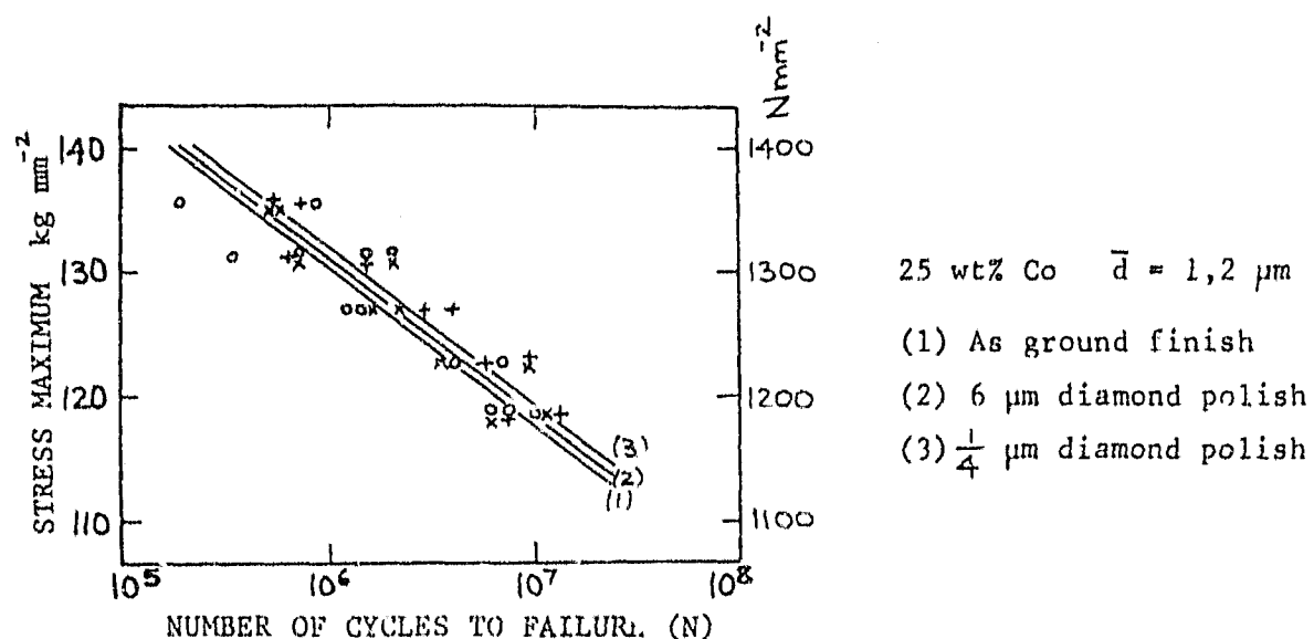
Figure 2.17 Effect of surface finish on fatigue life. 105
