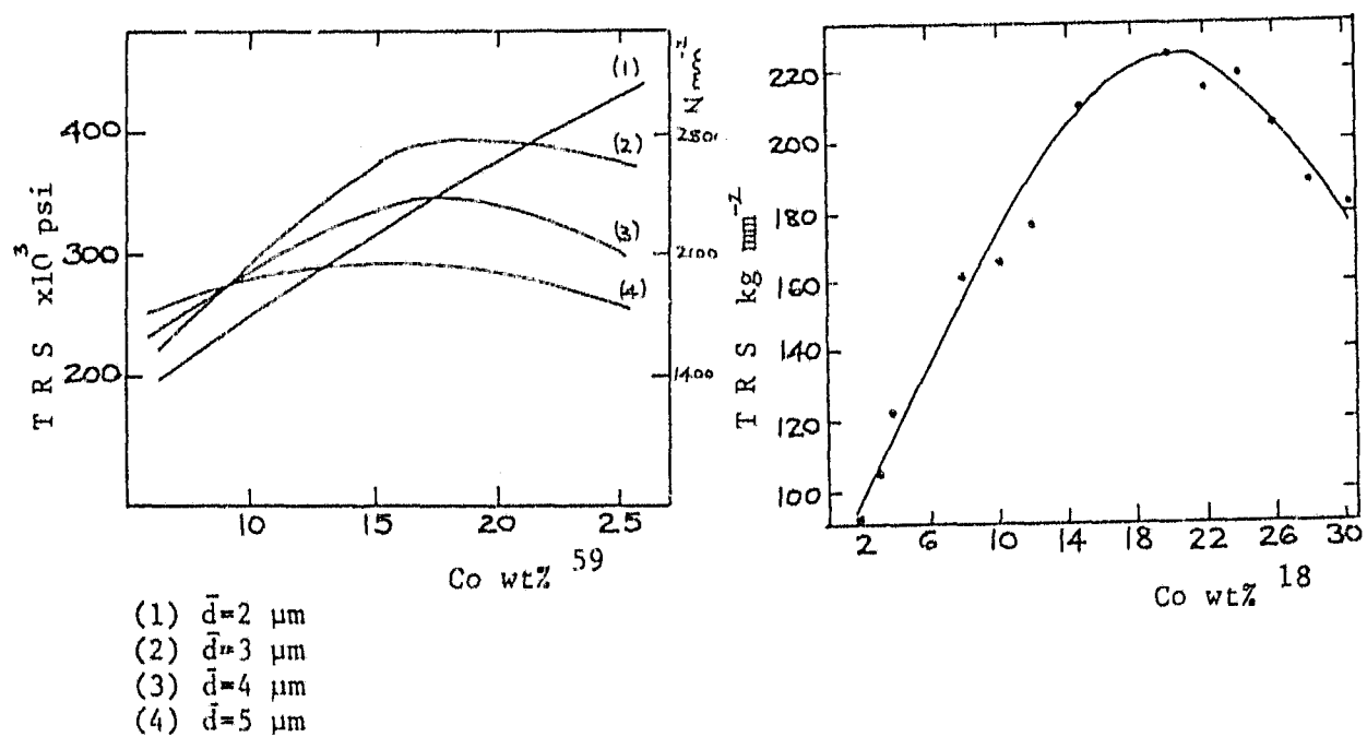
(a) Variation in transverse rupture strength with cobalt content. 18,59
