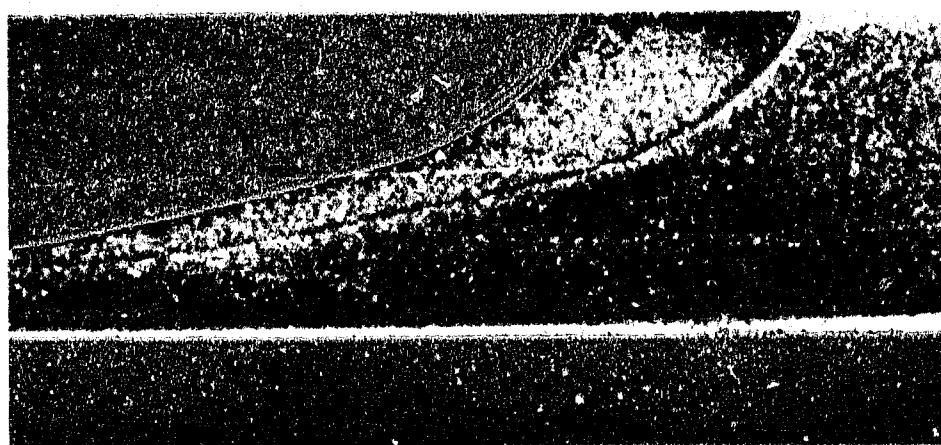
Figure 4.6 Crack front shape, in alloy S10, successive positions revealed by heat tinting.
