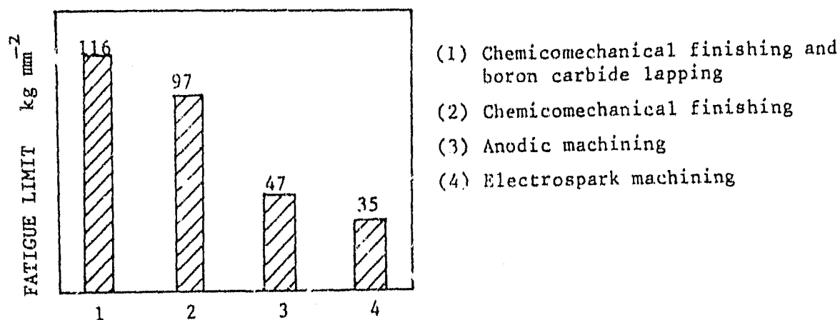
Figure 2.19 Effect of surface finish on fatigue life. 106
