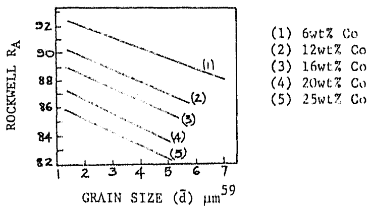
(b) Variation in hardness with WC grain size. 59
