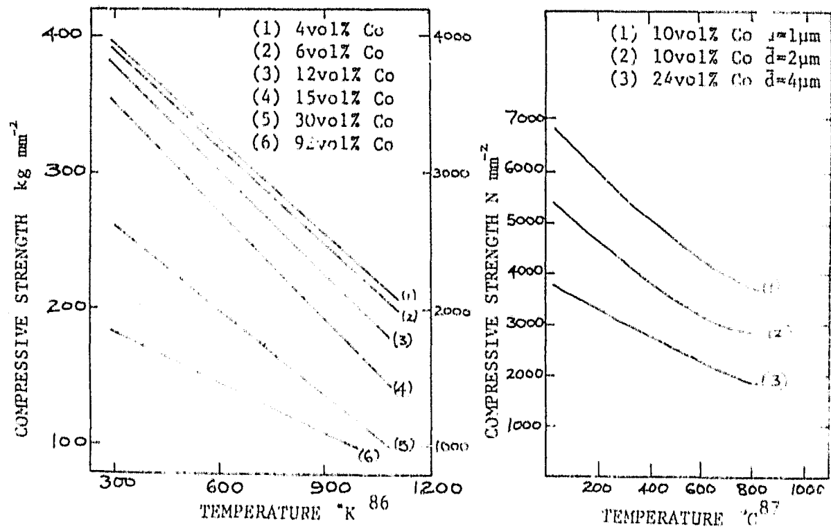
(d) Variation in compressive strength with temperature. 86, 87
