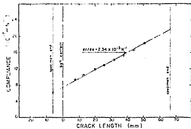
Compliance plot obtained by cutting specimen along crack line.
