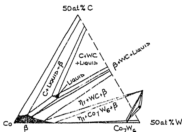
Figure 2.2 Isothermal section at 1260°C of cobalt rich part of W-C-Co ternary phase diagram.
