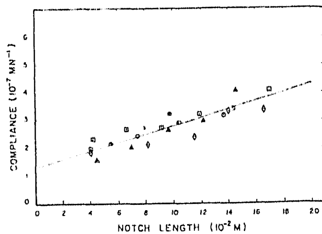
Compliance curve for notched cement-paste specimens. Data from 7 specimens.
