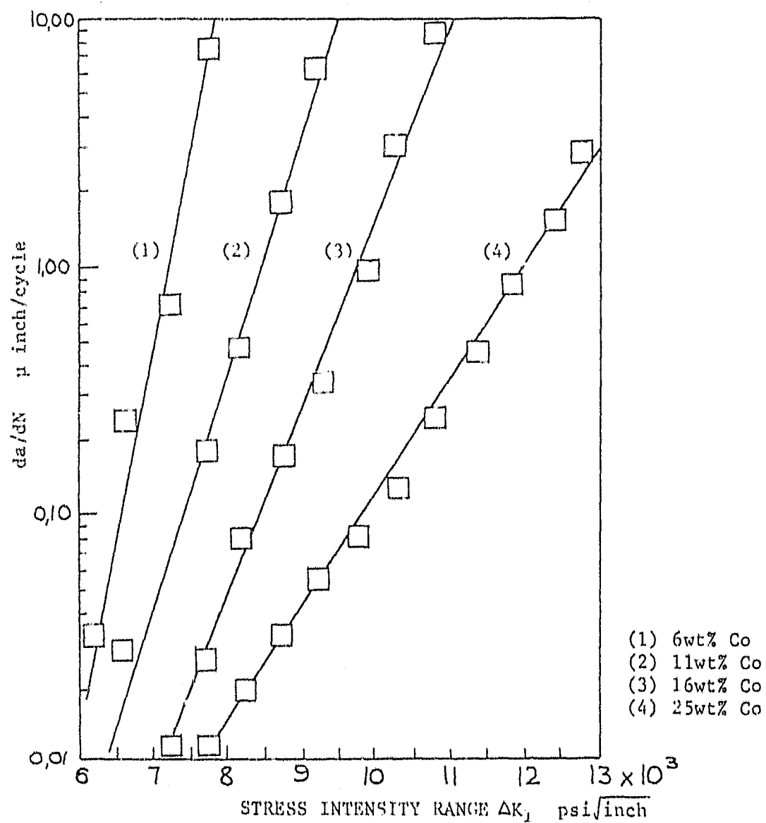
Figure 2.24 Fatigue crack growth rates measured using the DT geometry for a range of alloys.110
