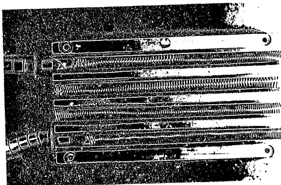
(b) Photograph showing heating coils and ceramic insulator.
