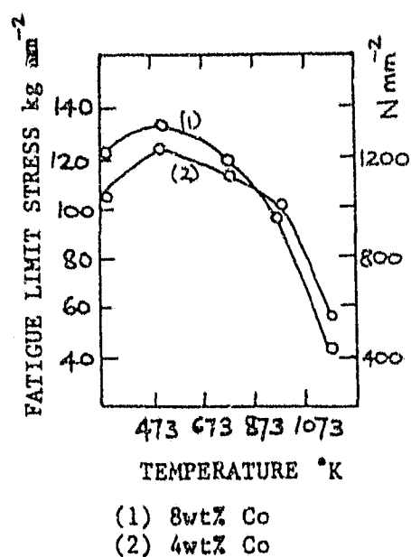
Figure 2.21 Effect of temperature on fatigue life. 107
