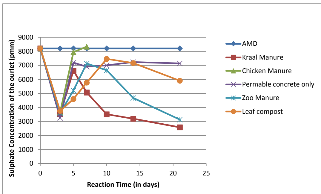
Figure 8: Effect of reaction time on sulfate removal for all feed stocks
