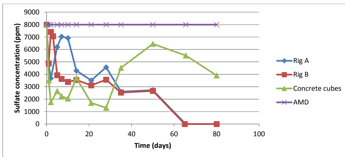
Figure 9 : Sulfate reduction over 80 days for manure and sawdust based PRBs.
