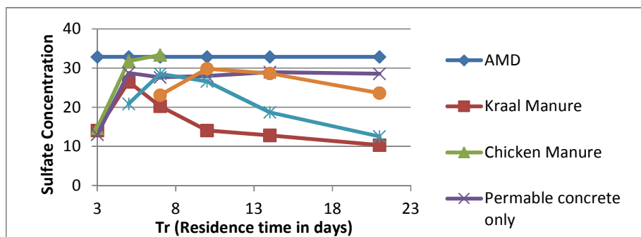
Figure 3. Effect of residence time on sulfate reduction
