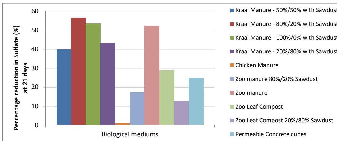
Figure 7 : Sulfate removal after 21 days for different substrates
