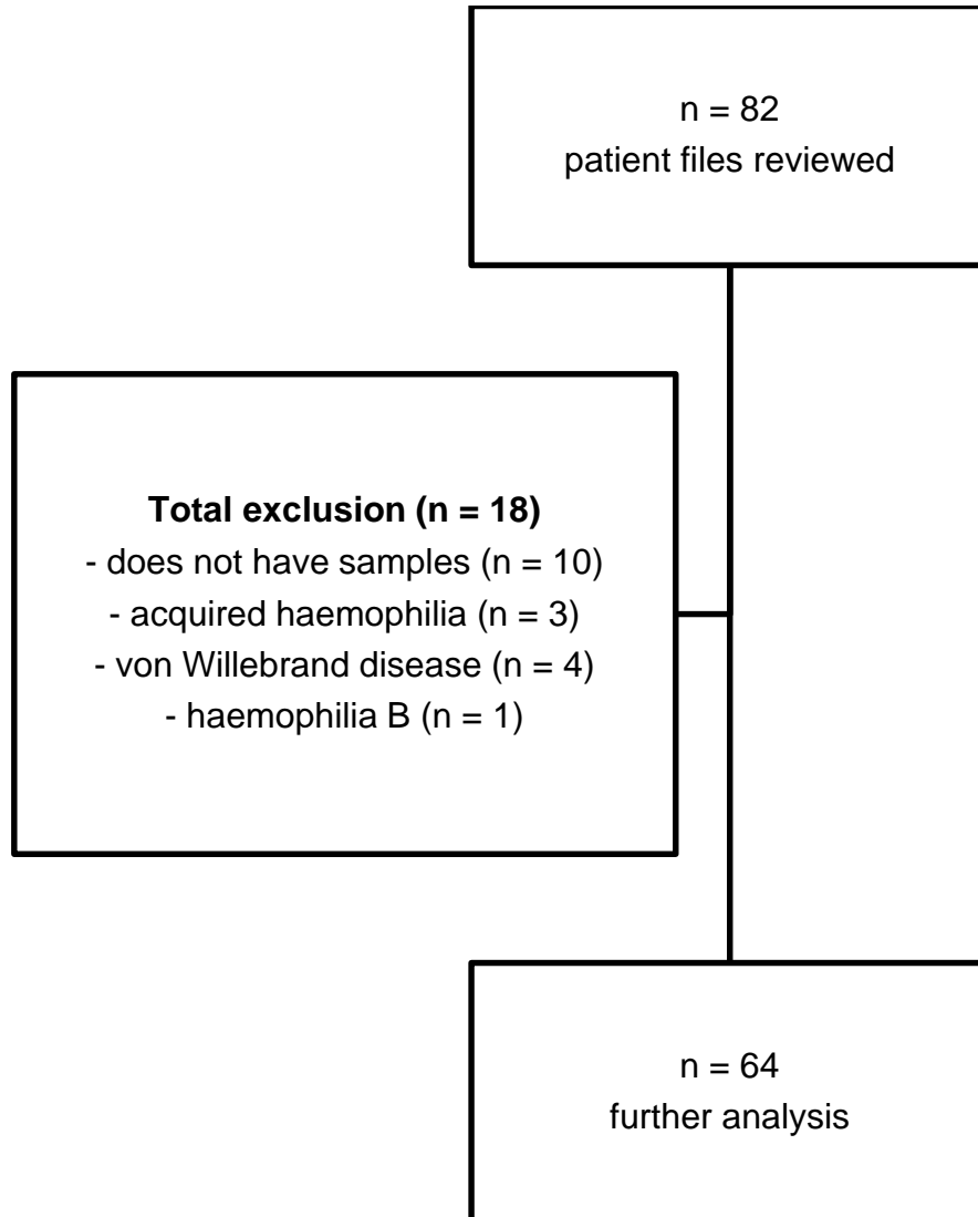
Figure 3.7. Flow diagram indicating the number of patient files reviewed, exclusion criteria and total number analyzed.
