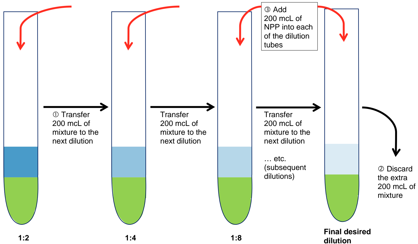
Figure 2.2. Flow chart demonstrating the setup of doubling dilutions.
