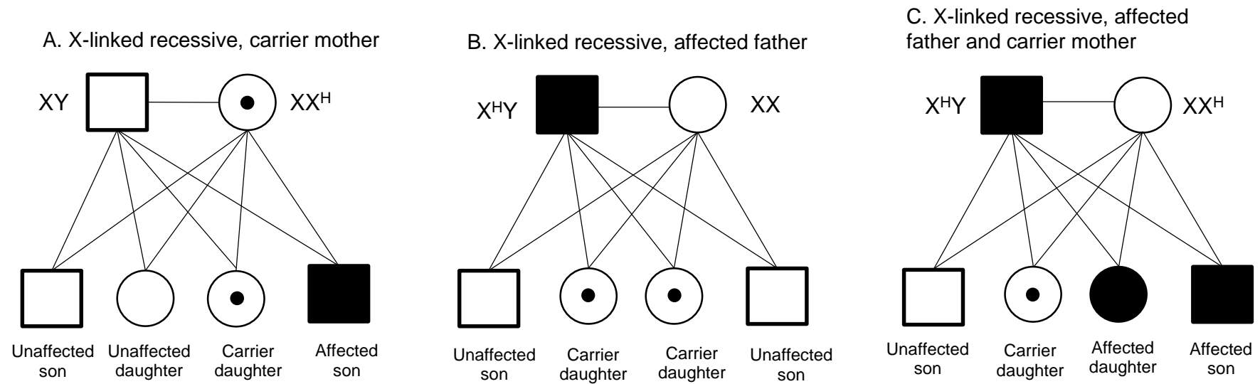
Figure 1.1. Inheritance pattern of Haemophilia.
