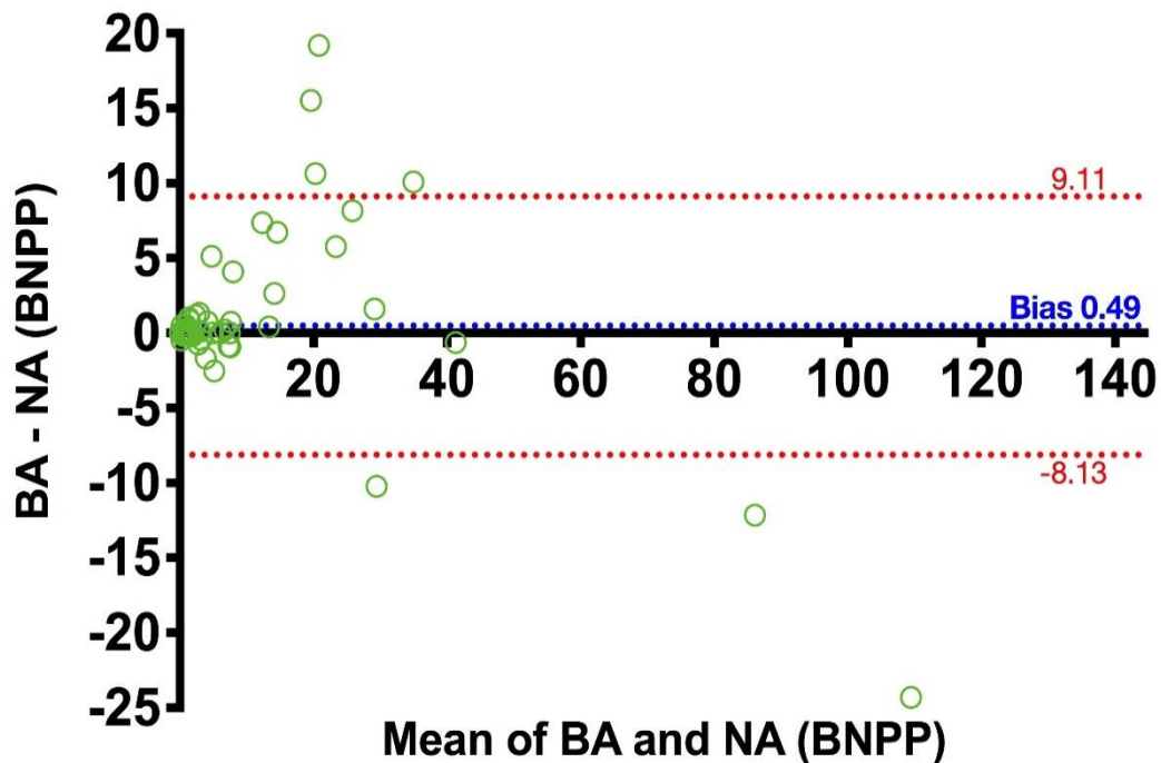
Figure 3.2. Bland-Altman plot demonstrating accuracy between BA and NA with BNPP.
