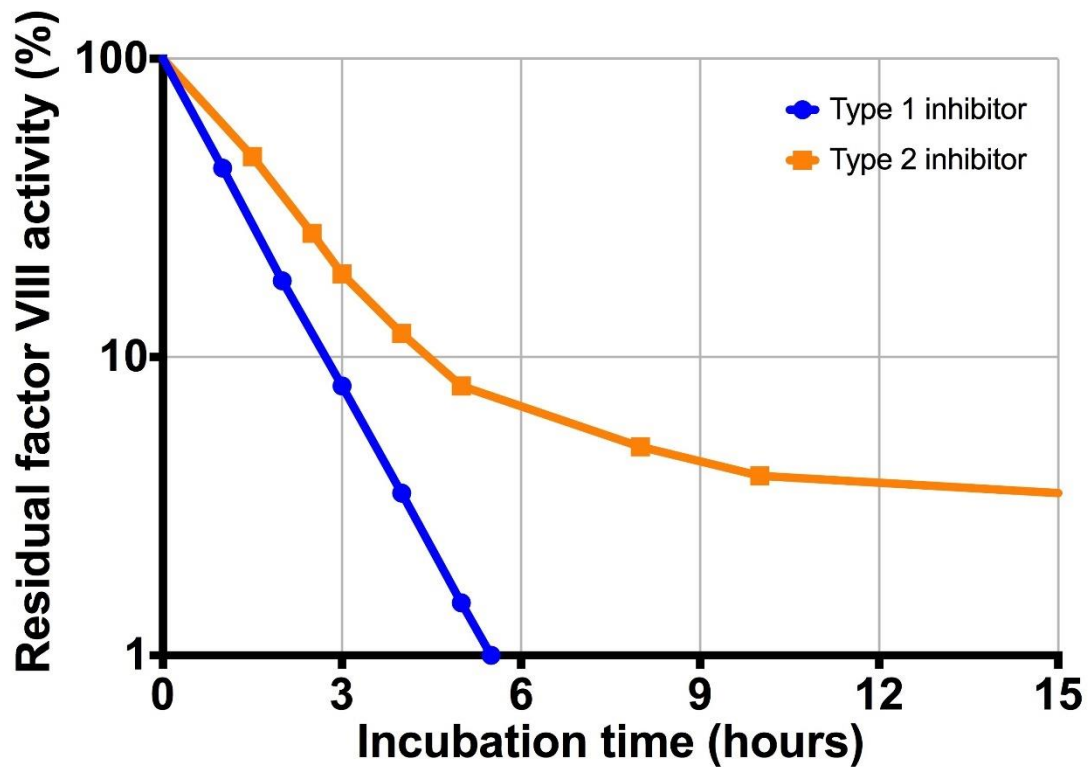
Figure 1.2. Kinetics of type 1 and type 2 inhibitors against Factor VIII.
