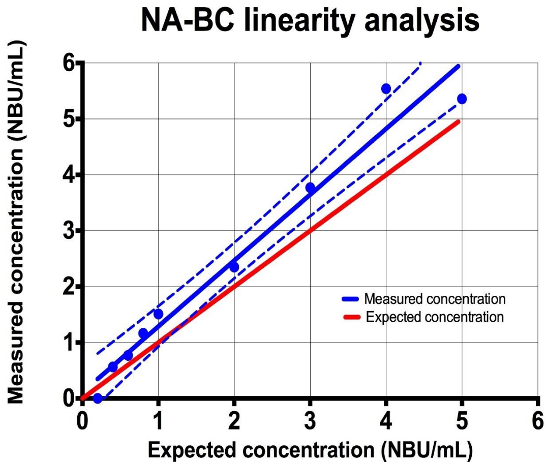
Figure 3.6. Linearity analysis of NA with BC.
