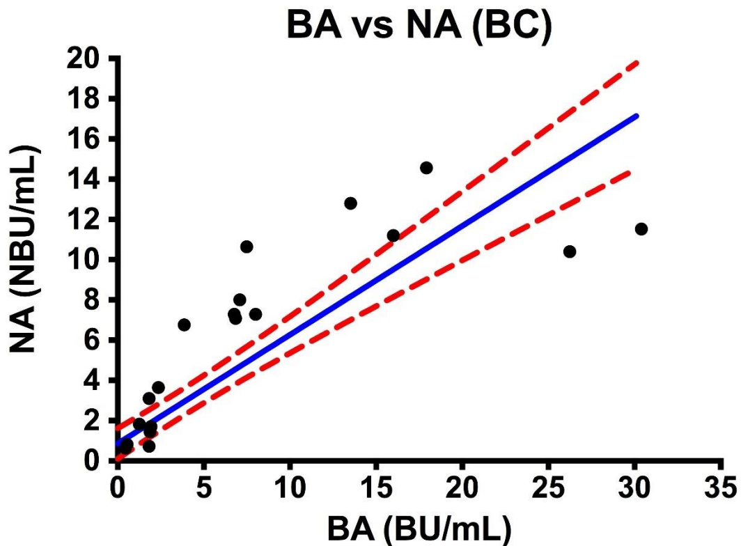
Figure 3.4. Linear regression graph demonstrating NA using BC against BA.
