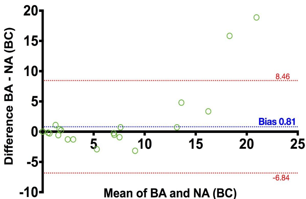
Figure 3.5. Bland-Altman plot demonstrating accuracy between BA and NA with BC.
