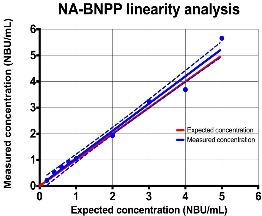
Figure 3.3. Linearity analysis of NA with BNPP.
