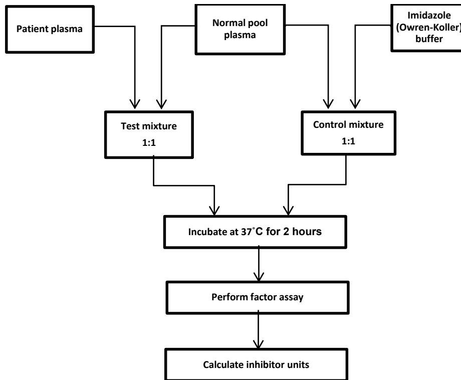
Figure 1.3. Flow diagram of Bethesda Assay 81 .
