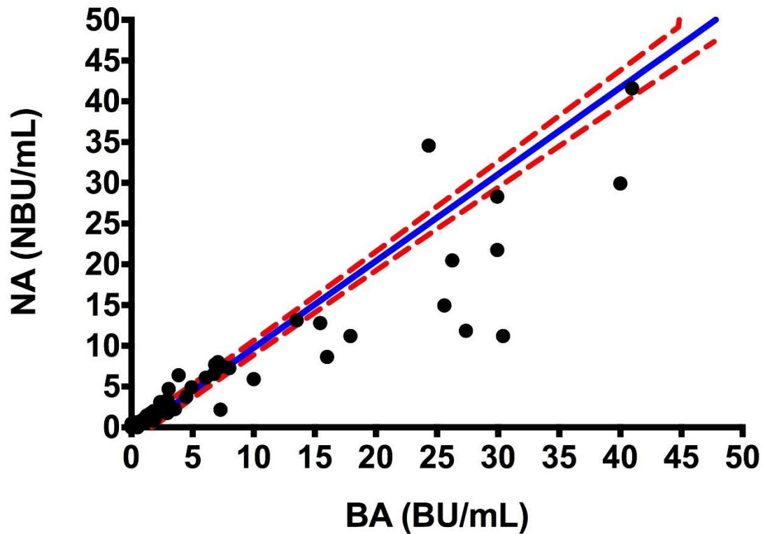
Figure 3.1. Linear regression graph demonstrating NA using BNPP against BA.
