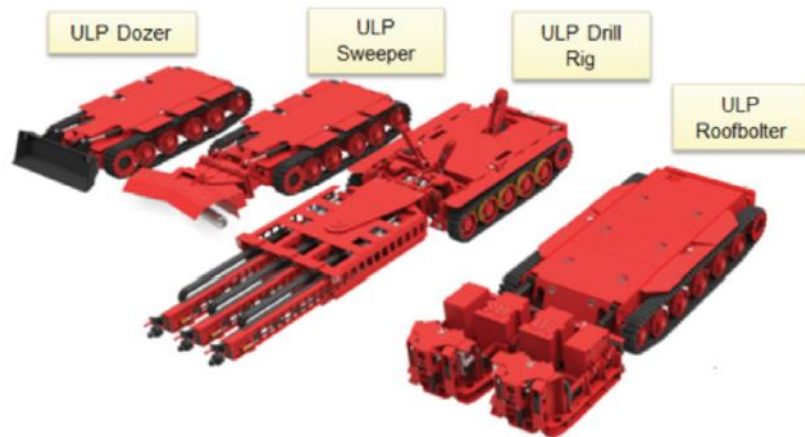
Figure 2.2: Ultra Low Profile trackless equipment fleet at Anglo American Platinum (Fourie et al. 2014)
