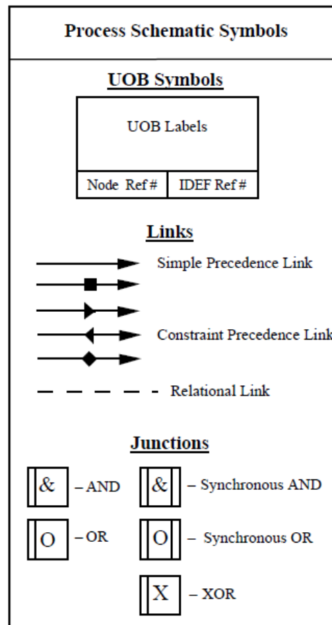
Figure 3.6: Symbols used for IDEF3 diagrams (Mayer et al. 1995)
