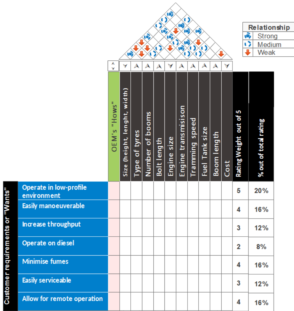
Figure 4.9: Correlations matrix between technical parameters
