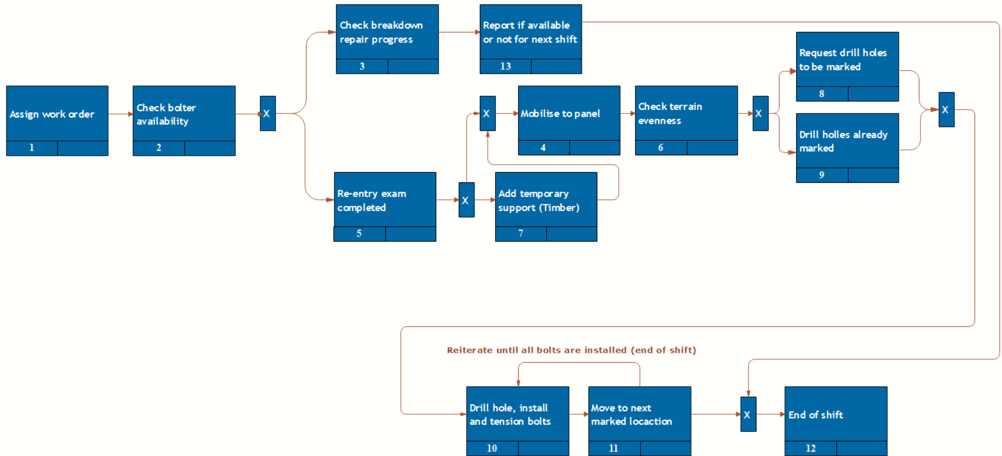
Figure 4.13: IDEF3 diagram of roofbolt installation scenario
