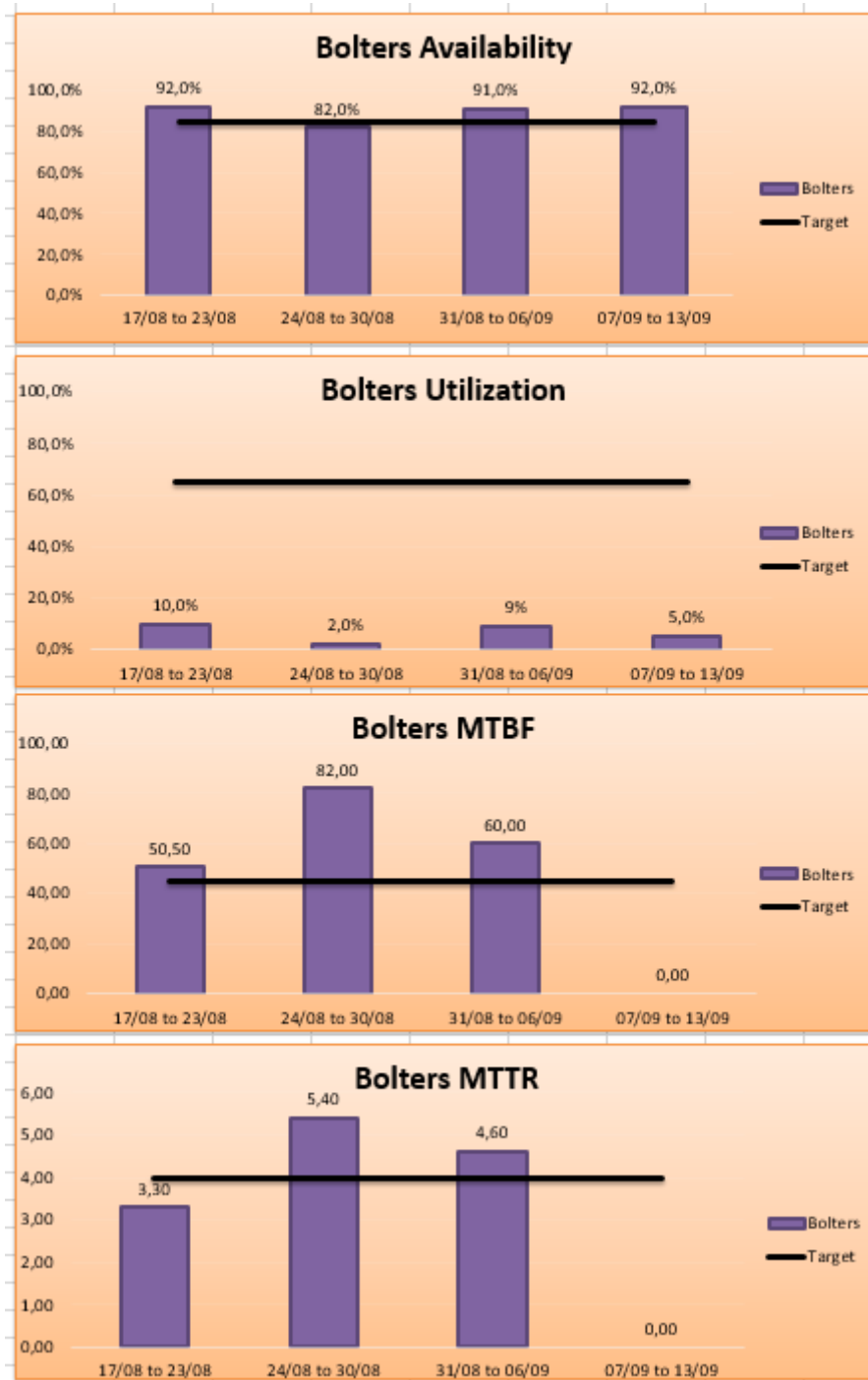
Figure 5.3: Availability, utilisation, MTBF and MTTR sample data
