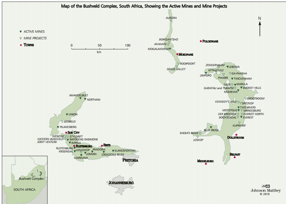
Figure 4.1: The Bushveld Complex showing the northern, eastern and western limbs as well as active mines, mine projects and towns in the area (Cawthorn 2010).
