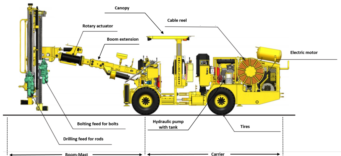
Figure 4.6: Single boom roof-bolter rig for mechanised roof support (Resemin 2015).
