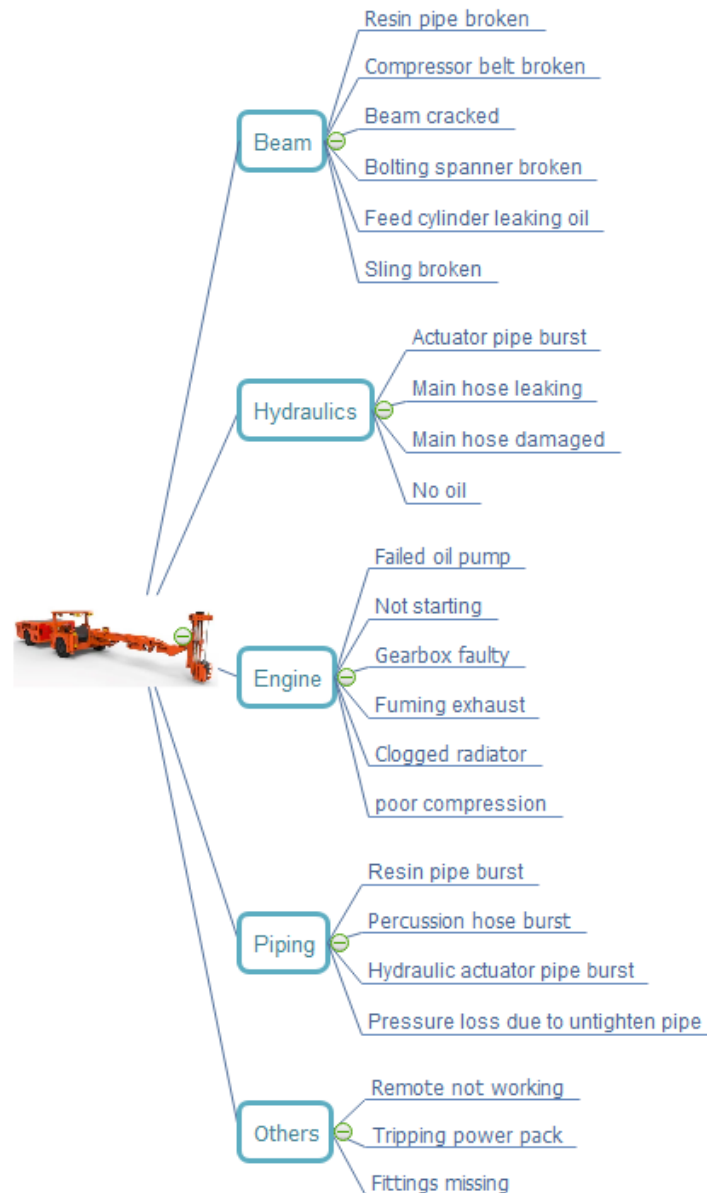
Figure 5.4: Mind map presenting group of common breakdowns on the roof-bolter
