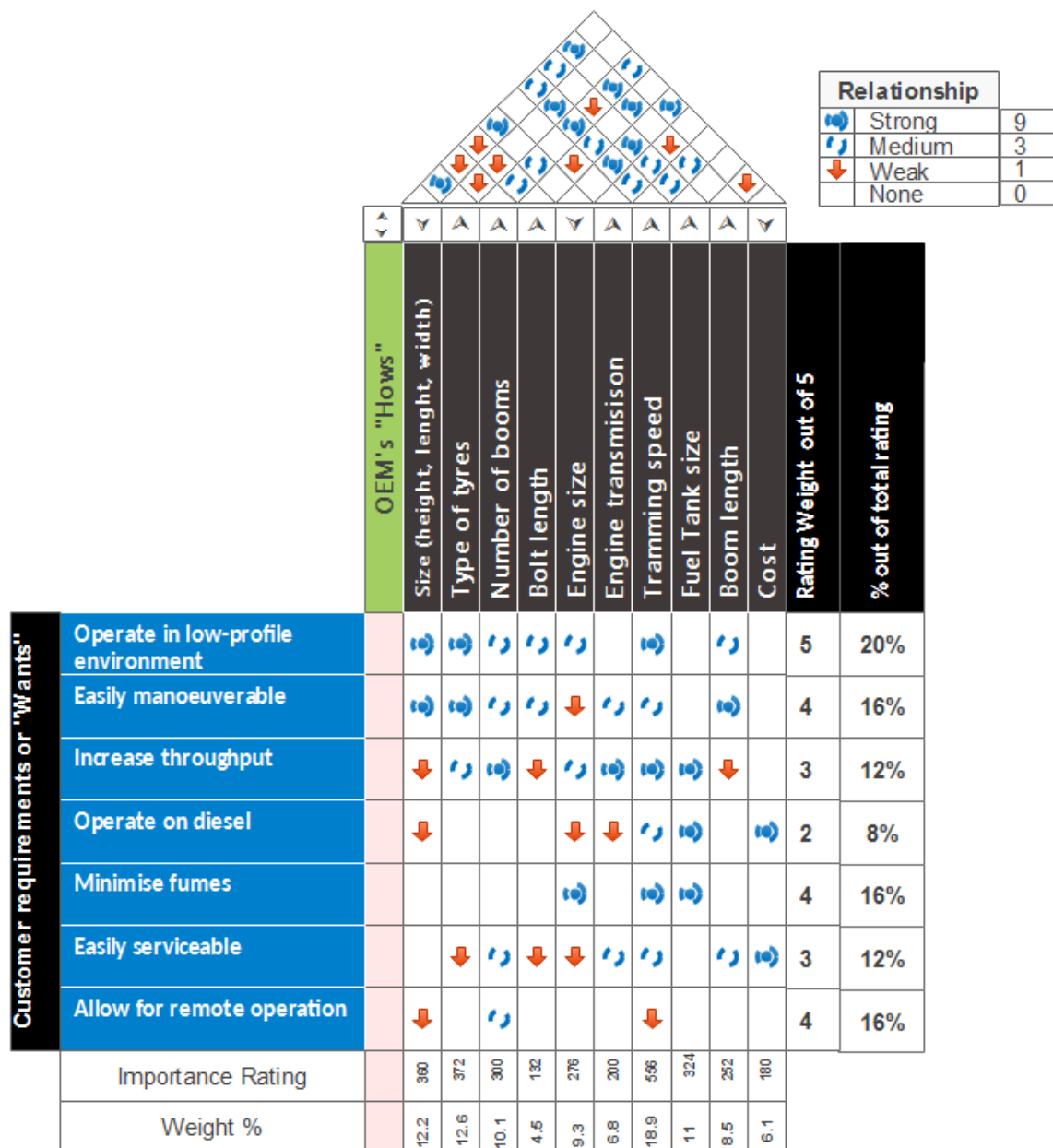
Figure 4.10: Whats and Hows relationship matrix and importance ratings
