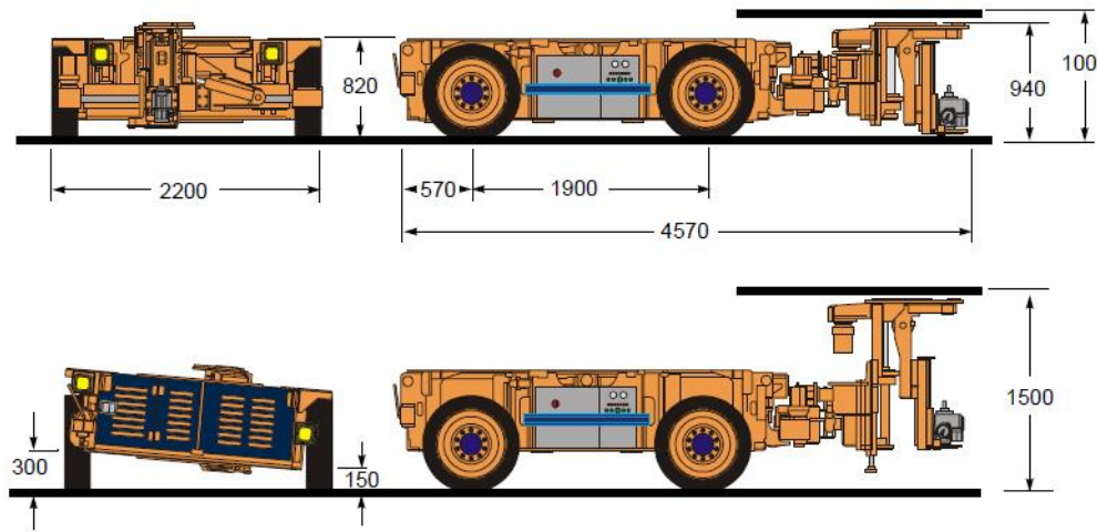
Figure 2.3: Sandvik’s ROBOLT XLP roof-bolting machine (SANDVIK 2006)
