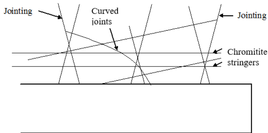
Figure 4.2: Stratified and blocky nature of UG2 reef type. Also shown are jointing, curved joints and chromite stringers. (Sellers et al. 2016)
