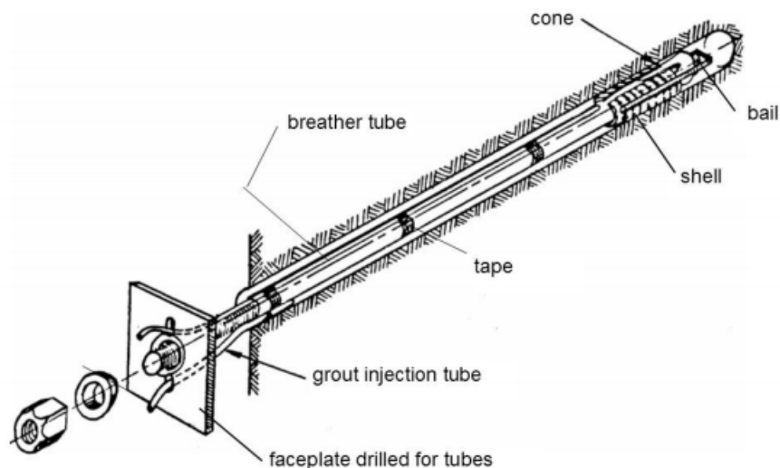
Figure 4.5: Mechanically anchored roof-bolt showing the different components (Cawthorn 2010).
