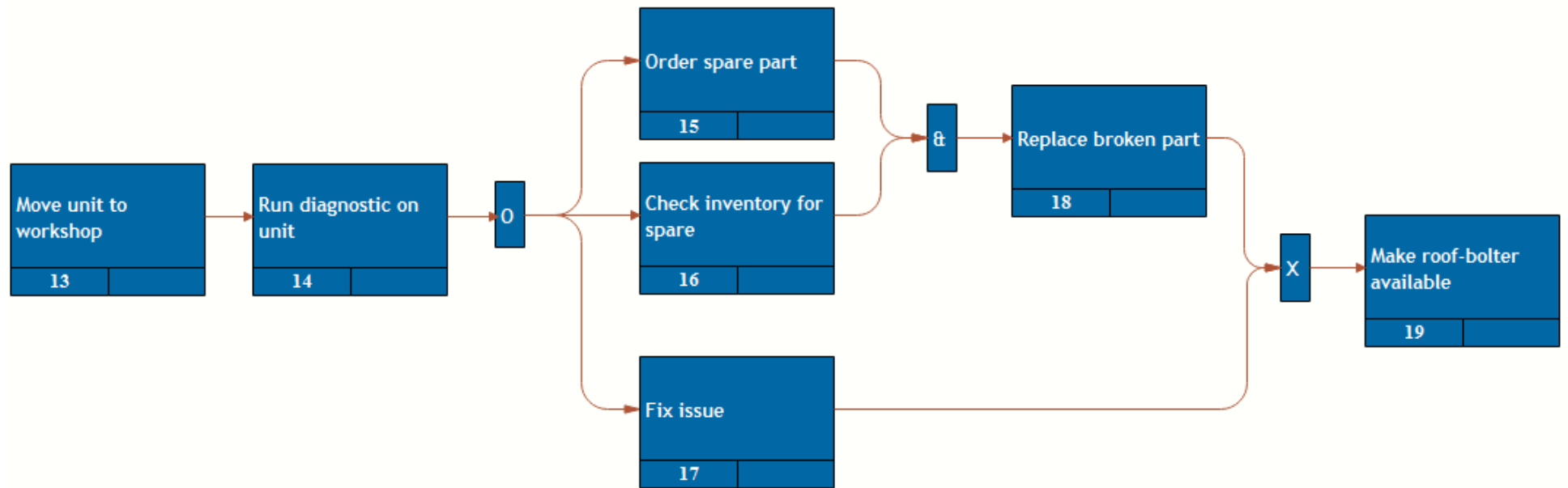
Figure 4.14: IDEF3 diagram of breakdown scenario
