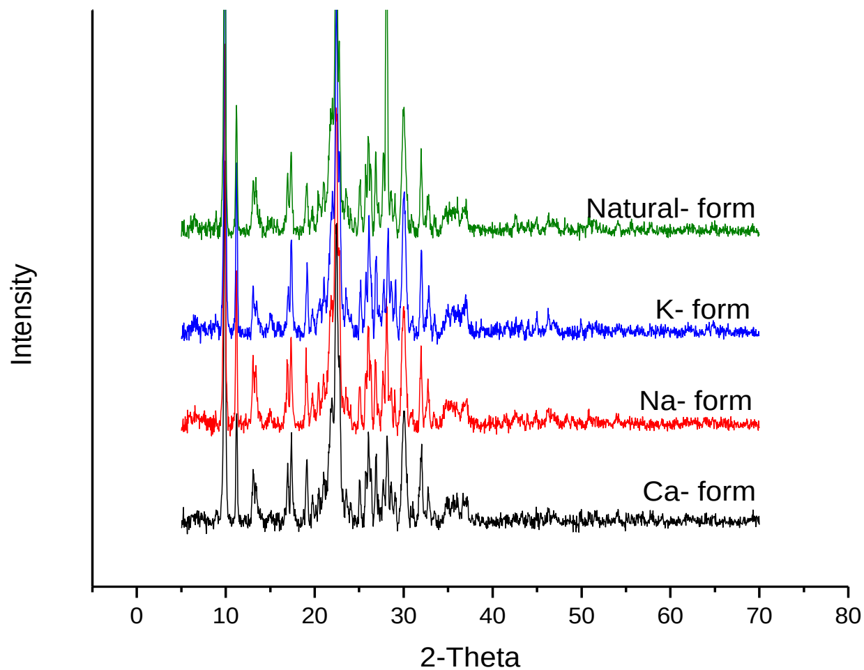
Figure 4. 7: X-ray diffraction (XRD) pattern of natural and pretreated forms of clinoptilolite. The patterns were determined with a Siemens D500 x-ray diffractometer.
