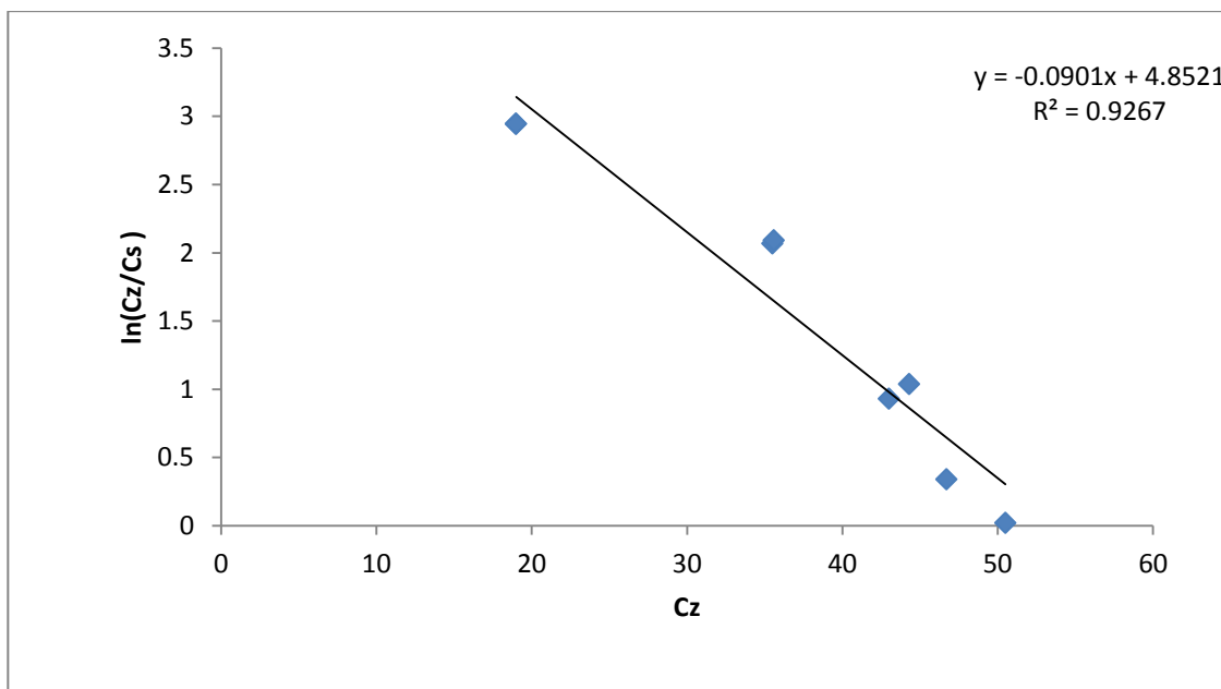
Figure D-3: Plot of \ln(C_z/C_s) versus C_z (For Na-form at 50°C).
