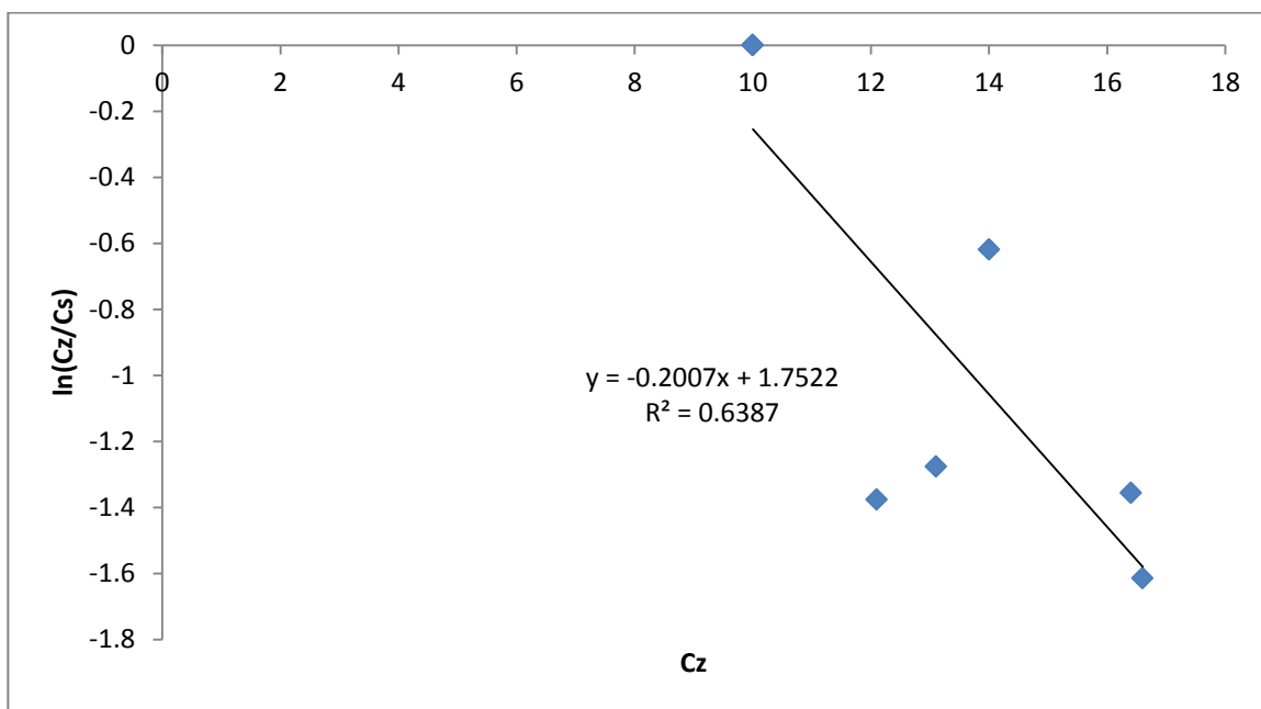
Figure D-6: Plot of \ln(C_z/C_s) versus C_z (For K-form at 25°C).
