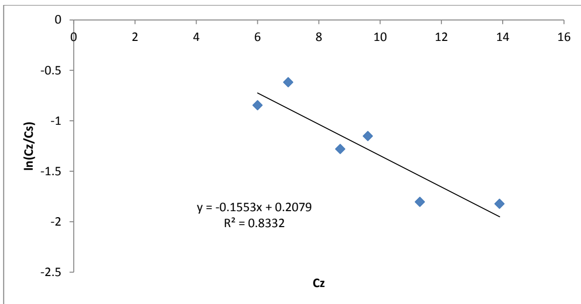
Figure D-13: Plot of \ln(C_z/C_s) versus C_z (For Ca-form at 50°C)
