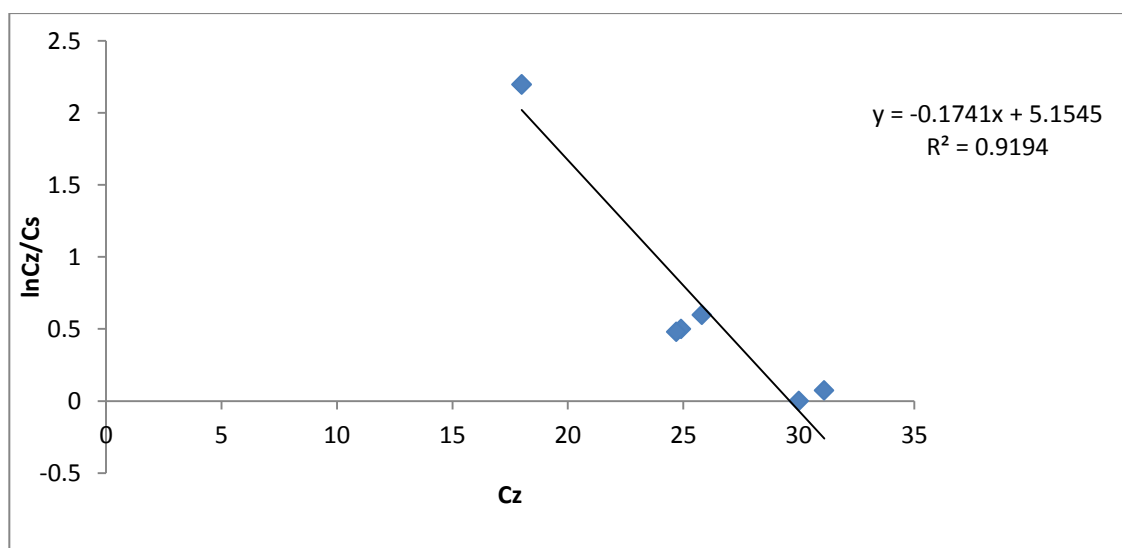
Figure D-1: Plot of \ln(C_z/C_s) versus C_z (For Na-form at 25°C).
