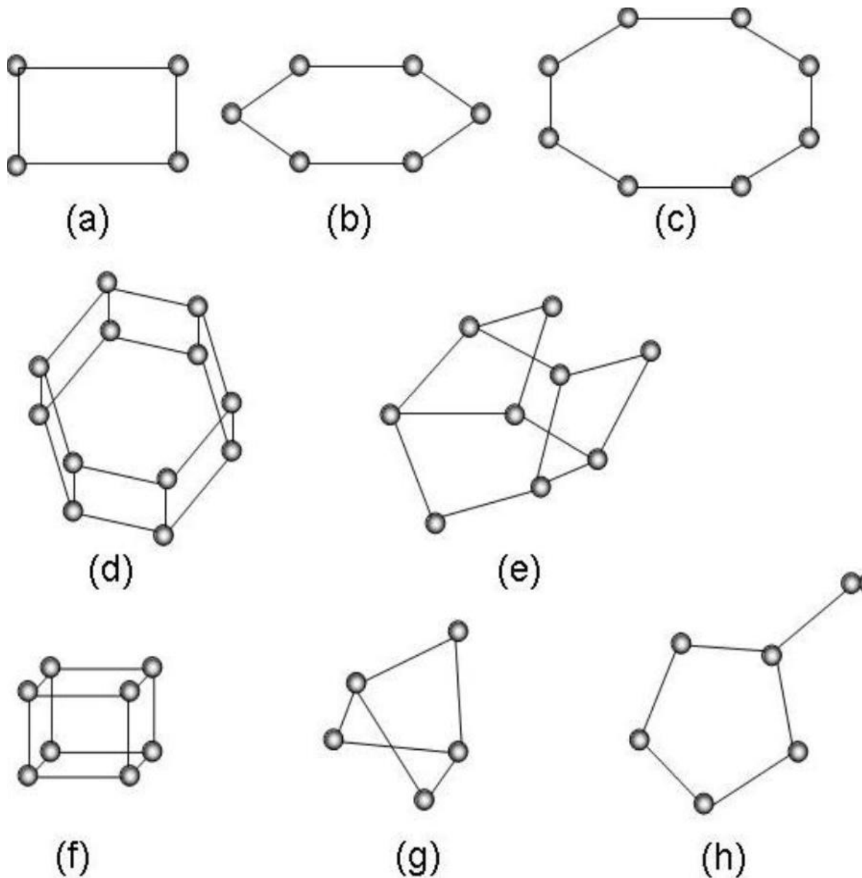
Figure 2.1: Secondary building units in zeolite frameworks; (a) single four ring (S4R), (b) single six ring (S6R), (c) single eight ring (S8R), (d) double six ring (D6R), (e) complex 4-4-1 (f) double four ring (D4R), (g) complex 4-1 and (h) complex 5-1 (Ruthven, 1984; Dyer, 1988).
