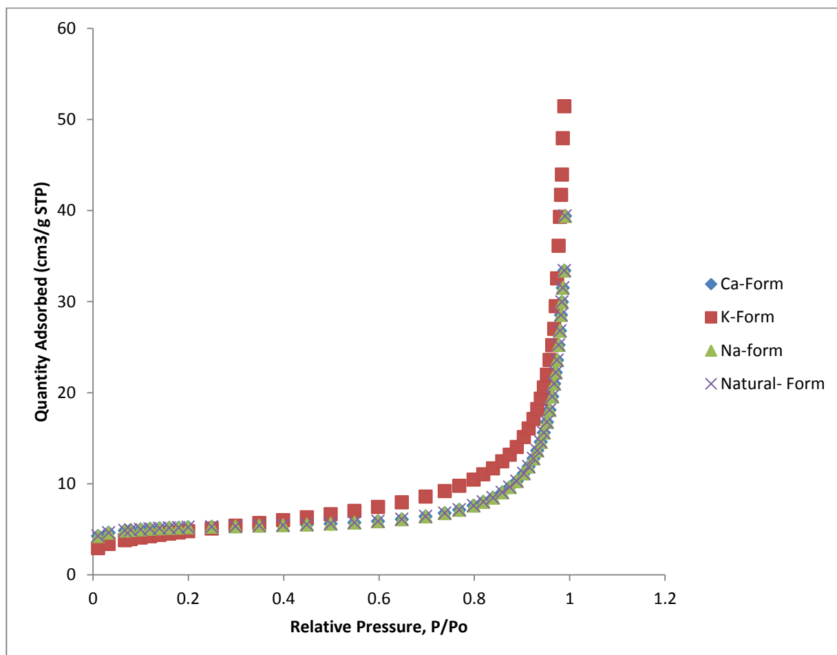
Figure 4.1. Adsorption isotherms of nitrogen on different forms of clinoptilolite.
