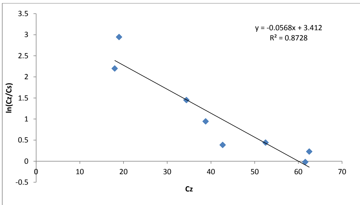
Figure D-19: Plot of \ln(C_z/C_s) versus C_z (For Natural-form at 60°C).
