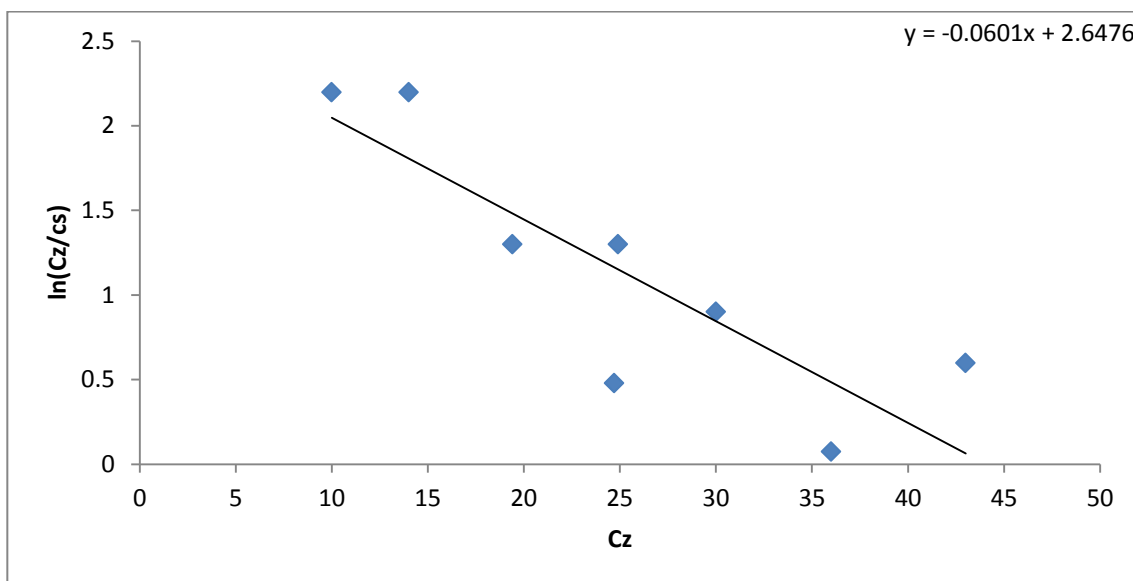
Figure D-2: Plot of \ln(C_z/C_s) versus C_z (For Na-form at 35°C).
