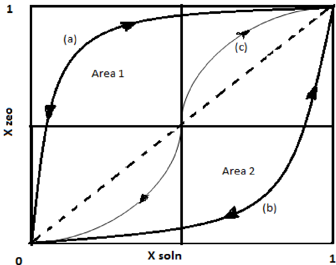
Figure 2. 4 : Idealised cation exchange isotherms.
