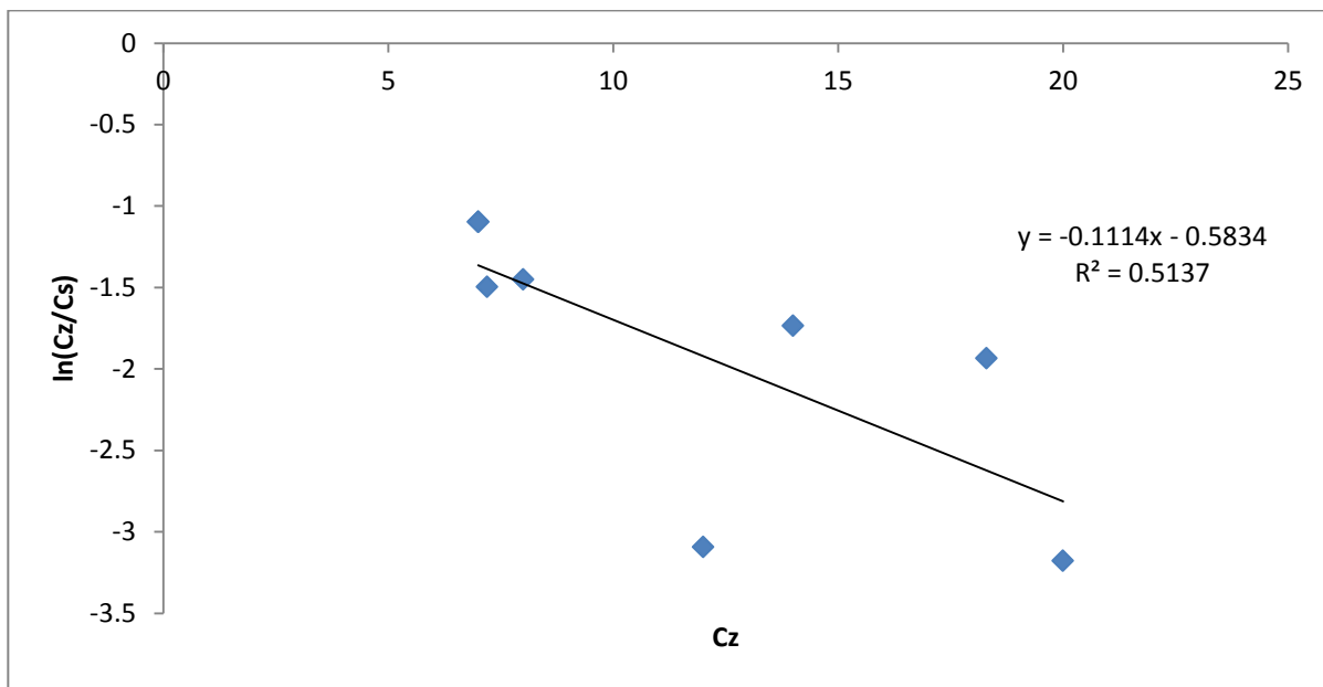
Figure D-12: Plot of \ln(C_z/C_s) versus C_z (For Ca-form at 35°C).
