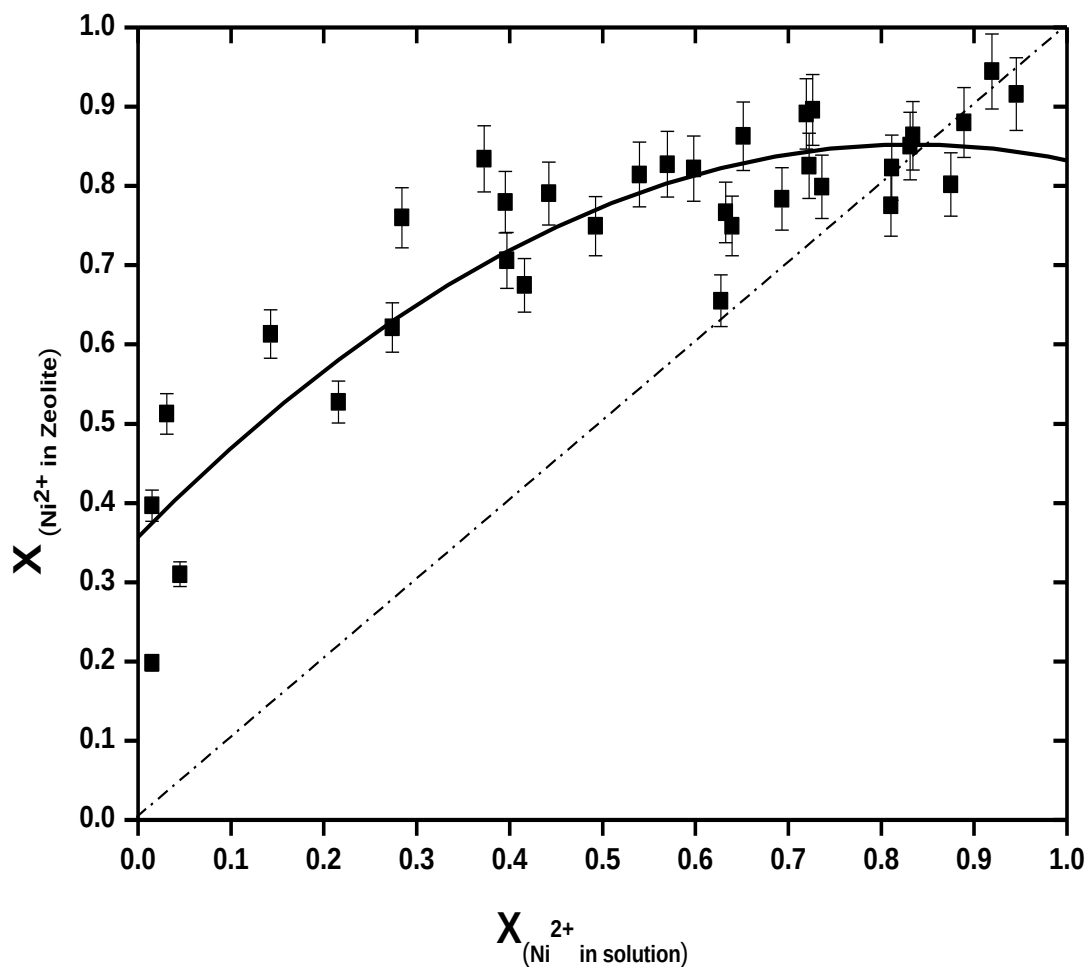
Figure 4.12: The \text{Na}^+ \text{-Ni}^{2+} isotherm at 25^\circ\text{C} . X_{(\text{Ni}^{2+} \text{ in soln})} : equivalent fraction of ingoing nickel in the liquid phase; X_{(\text{Ni}^{2+} \text{ in Zeo})} : equivalent fraction of nickel cation in the solid phase. Error bars for all points are indicated.
