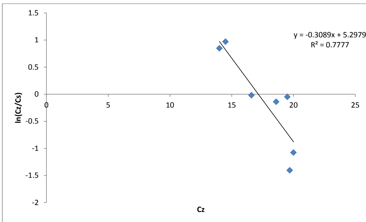
Figure D-8: Plot of \ln(C_z/C_s) versus C_z (For K-form at 50°C).
