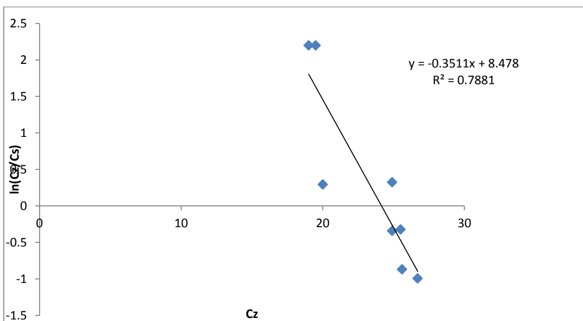
Figure D-17: Plot of \ln(C_z/C_s) versus C_z (For Natural-form at 35°C).
