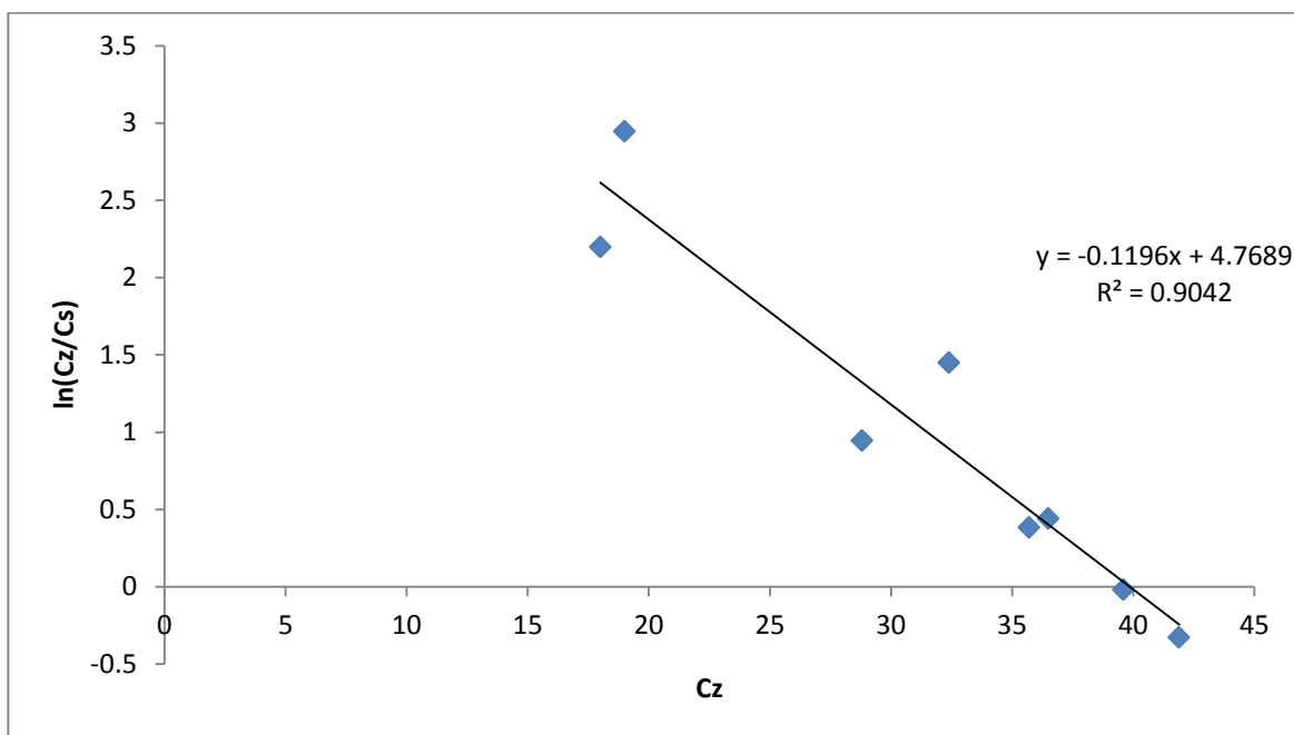
Figure D-18: Plot of \ln(C_z/C_s) versus C_z (For Natural-form at 50°C).
