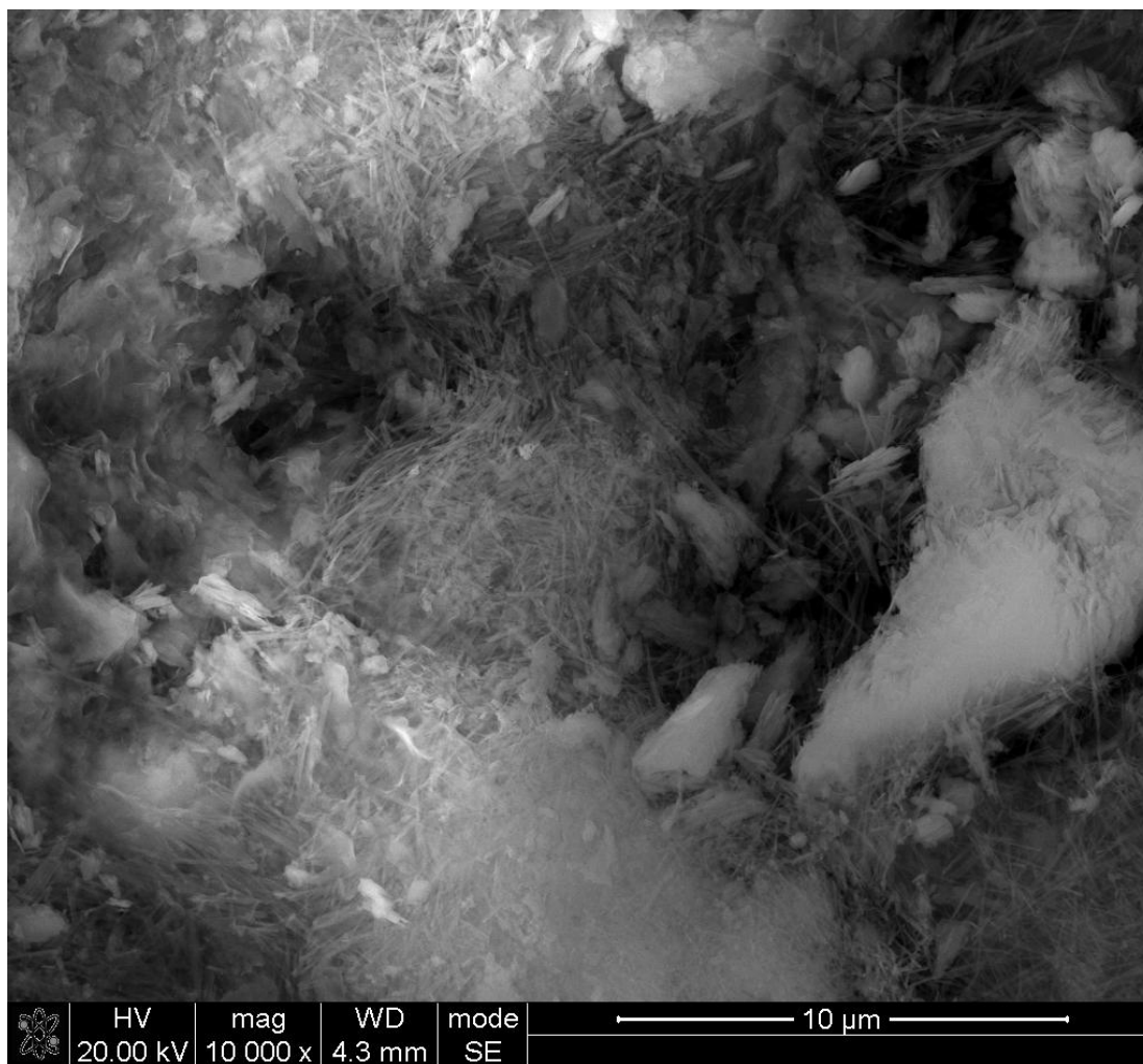
Figure 4.8: Micrograph of natural clinoptilolite showing surface and pores covered by extraneous material.
