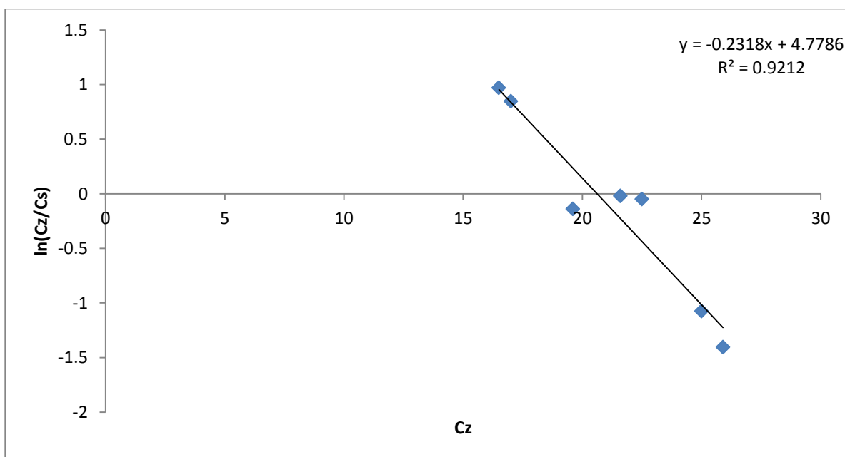
Figure D-9: Plot of \ln(C_z/C_s) versus C_z (For K-form at 60°C).
