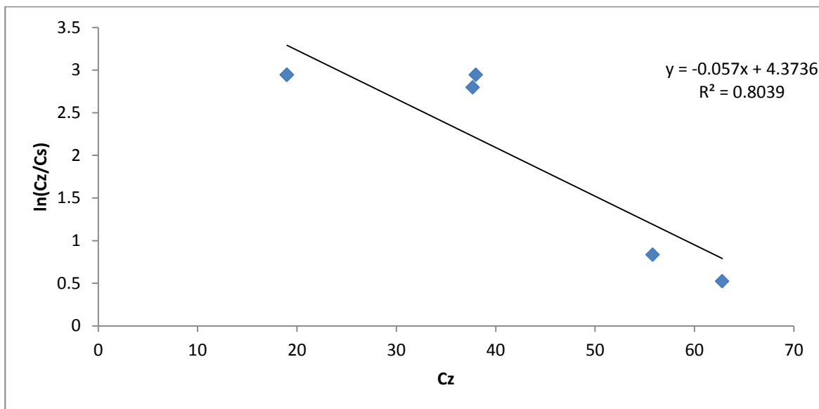
Figure D-20: Plot of \ln(C_z/C_s) versus C_z (For Natural-form at 75°C).
