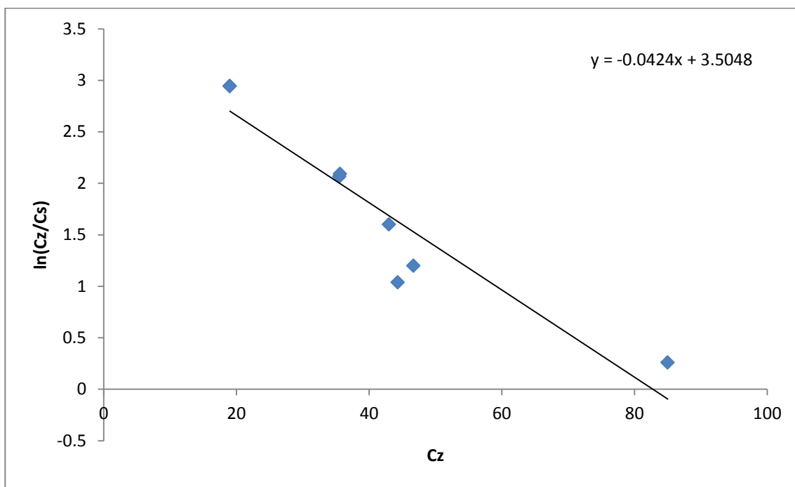
Figure D-4: Plot of \ln(C_z/C_s) versus C_z (For Na-form at 60°C).
