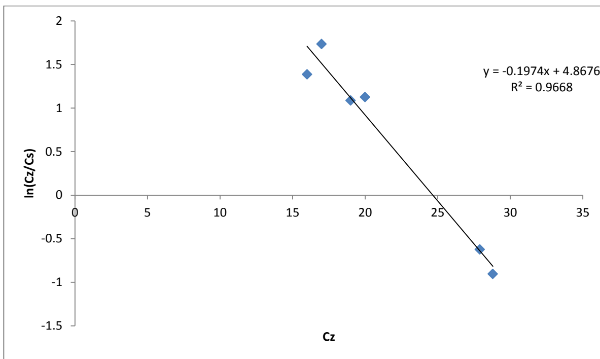
Figure D-10: Plot of \ln(C_z/C_s) versus C_z (For K-form at 75°C).
