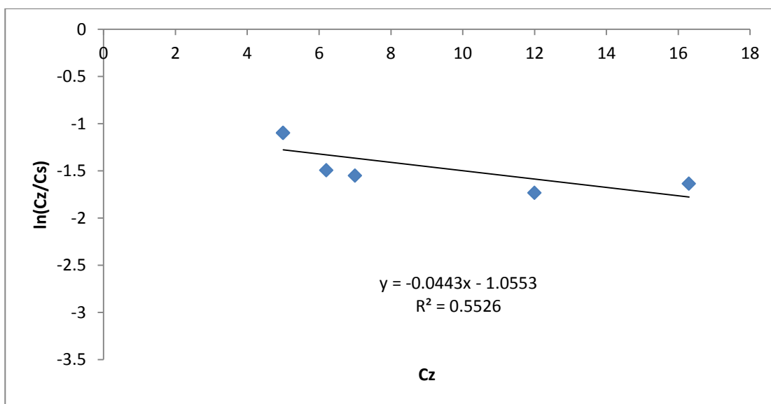
Figure D-11: Plot of \ln(C_z/C_s) versus C_z (For Ca-form at 25°C)
