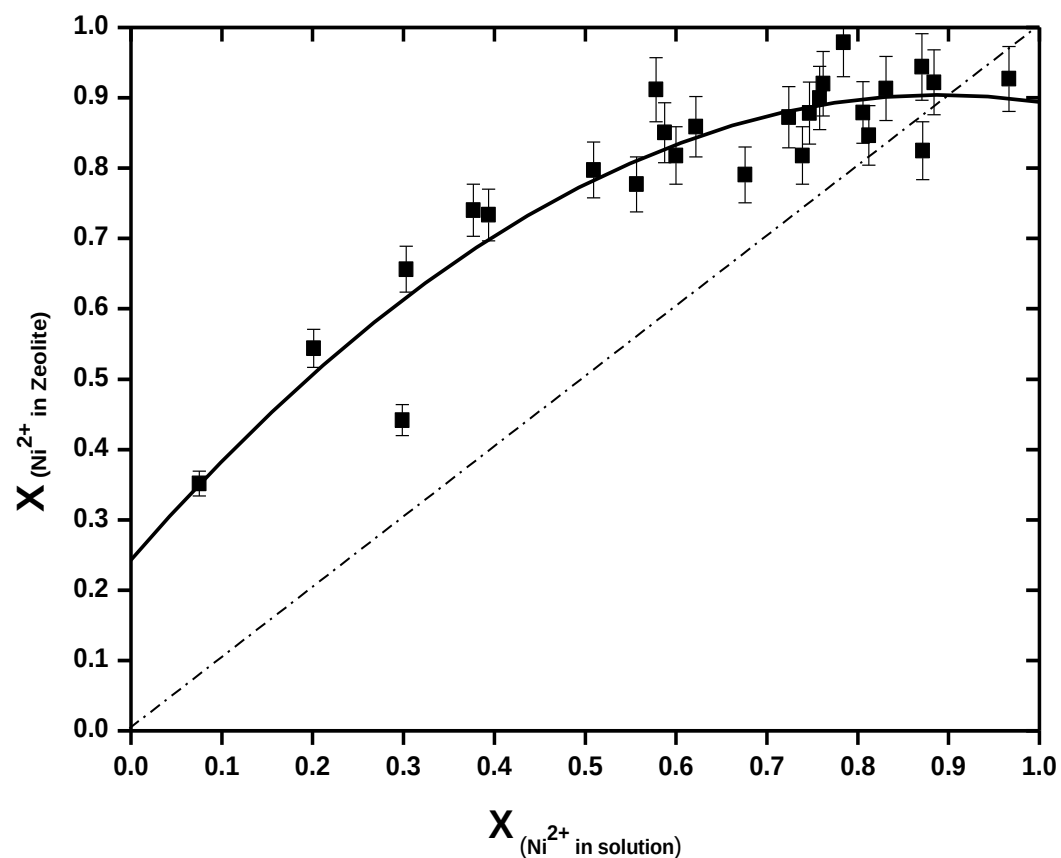
Figure 4.13: The \text{K}^+ - \text{Ni}^{2+} isotherm at 25^\circ\text{C} . X_{(\text{Ni}^{2+} \text{ in soln})} : equivalent fraction of ingoing nickel in the liquid phase. X_{(\text{Ni}^{2+} \text{ in Zeo})} : equivalent fraction of nickel cation in the solid phase. Error bars for all points are indicated.
