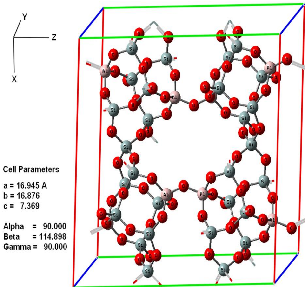
Figure 2. 2: The crystallographic unit cell of clinoptilolite, \text{Na} [\text{SiAlO}] structure generated by Gauss View 1998.
