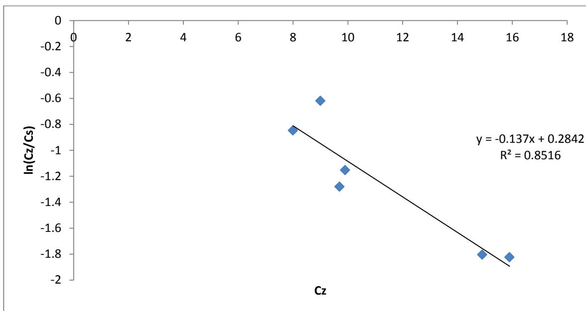
Figure D-14: Plot of \ln(C_z/C_s) versus C_z (For Ca-form at 60°C).
