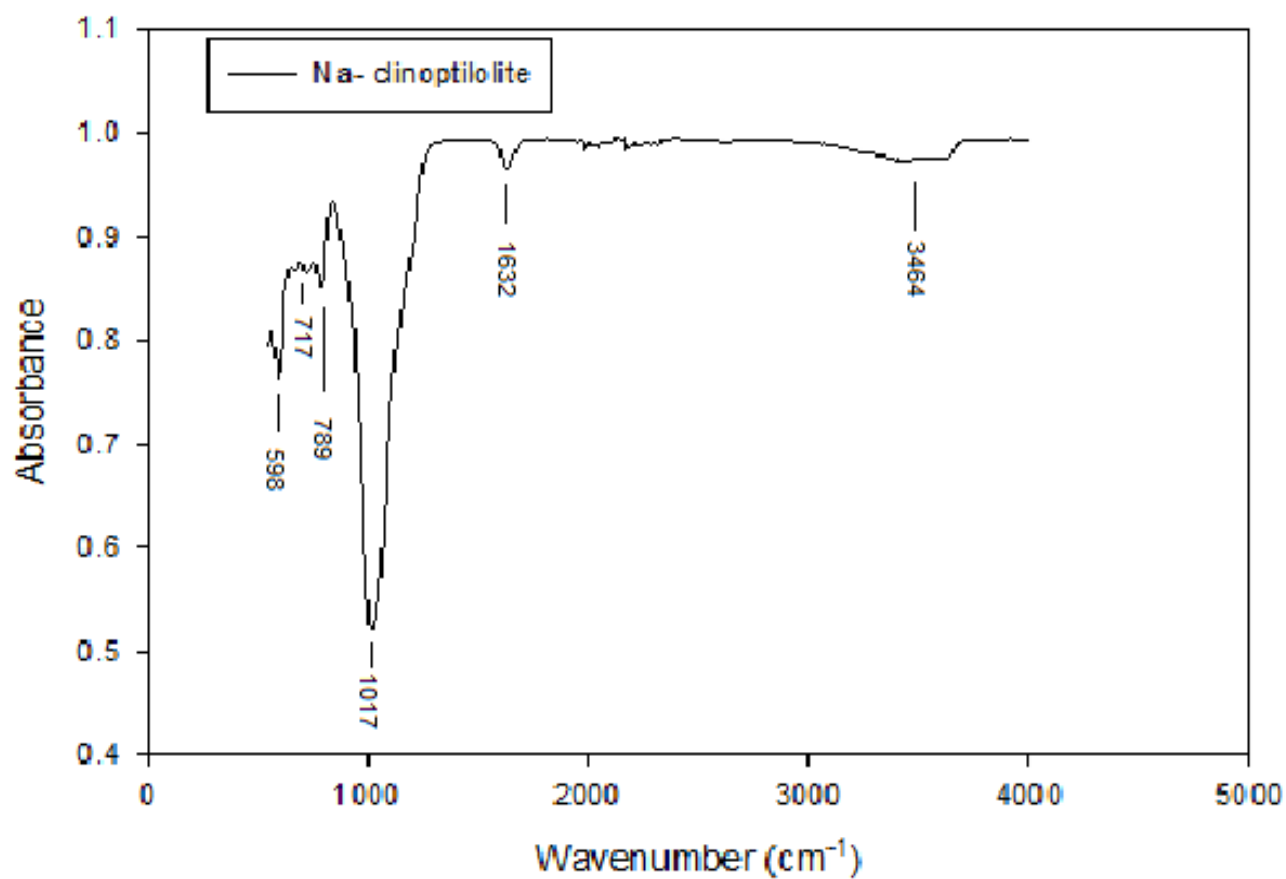
Figure 4. 4: The FTIR spectrum for Na- Clinoptilolite.
