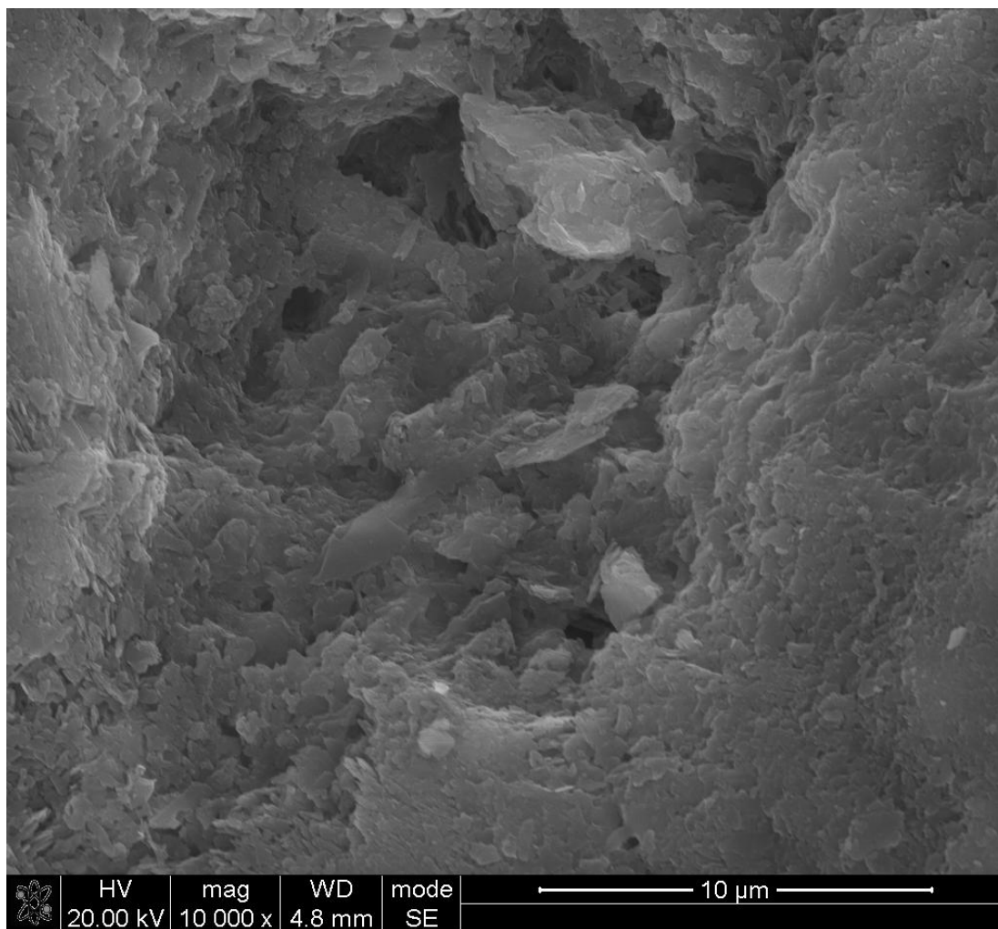
Figure 4.10: Electron micrograph of K- form of clinoptilolite.
