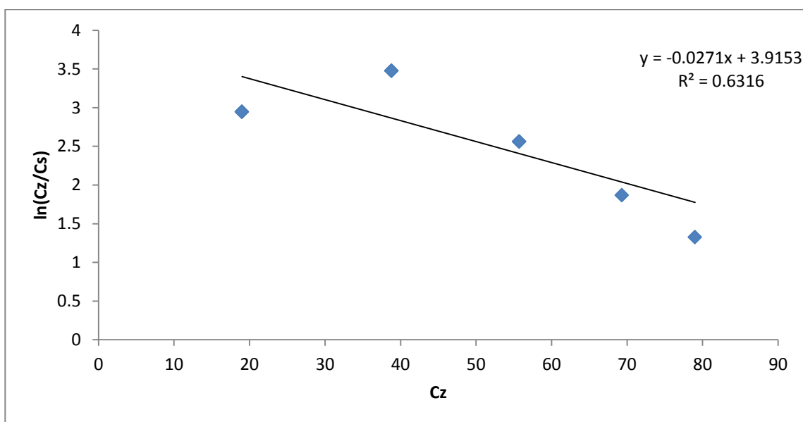
Figure D-5: Plot of \ln(C_z/C_s) versus C_z (For Na-form at 75°C).
