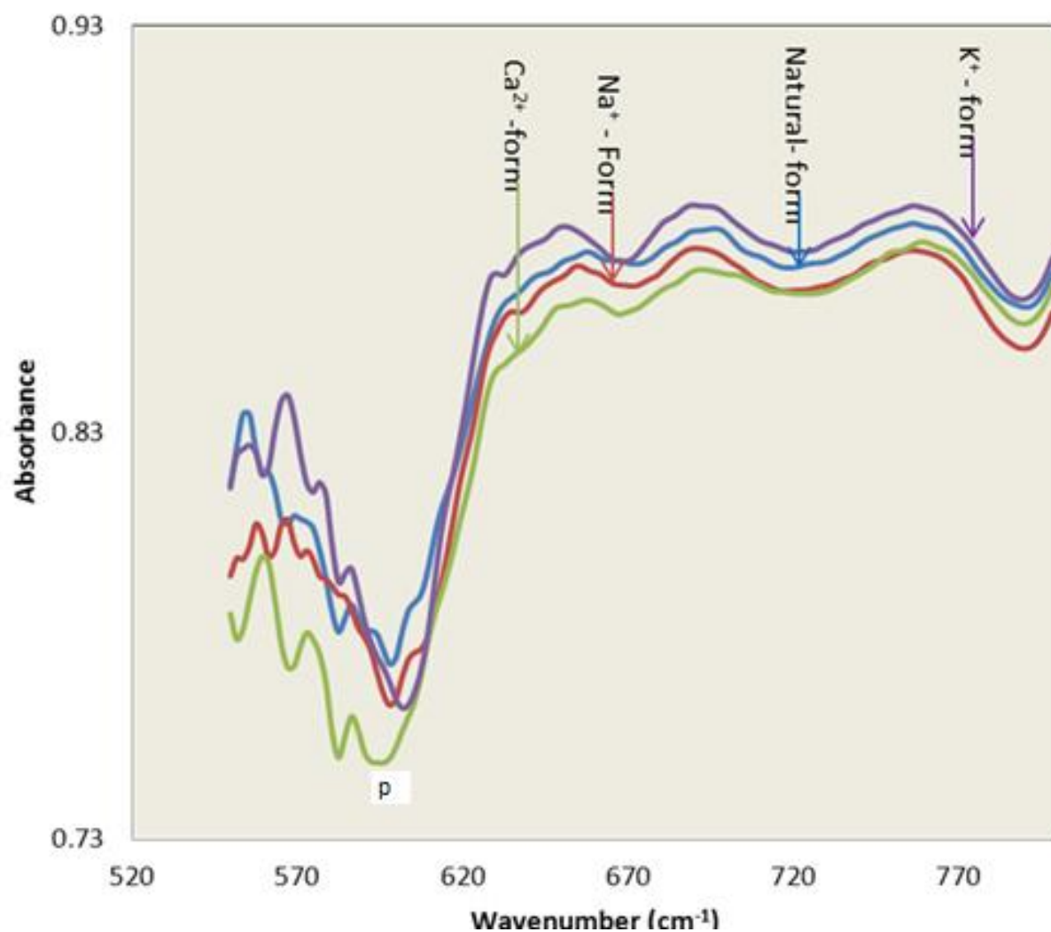
Figure 4. 6: The FTIR spectra for natural and pretreated clinoptilolite. A comparison of the band at 584\text{cm}^{-1} (point marked P) shows a particular trend in intensity for different forms of clinoptilolite.
