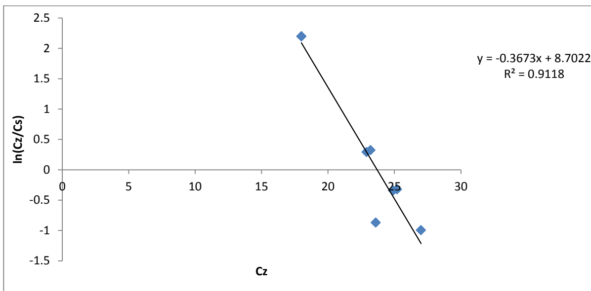
Figure D-16: Plot of \ln(C_z/C_s) versus C_z (For Natural-form at 25°C).
