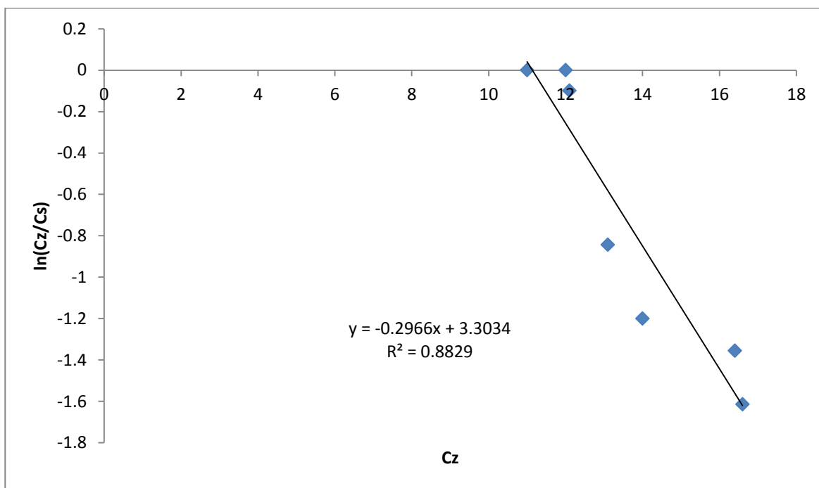
Figure D-7: Plot of \ln(C_z/C_s) versus C_z (For K-form at 35°C).
