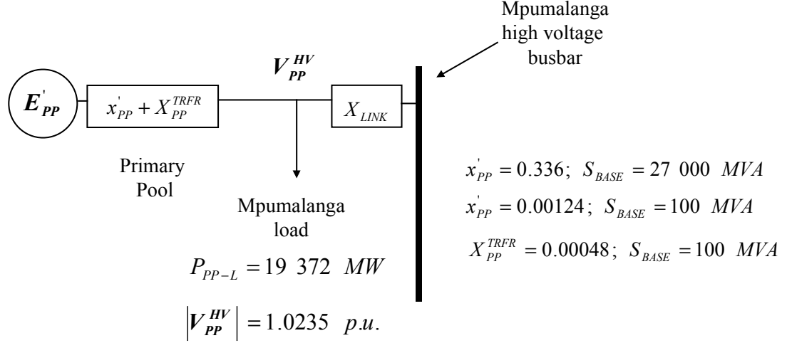
FIGURE E.1 Parameters of the electric circuit used to model the Primary Pool
