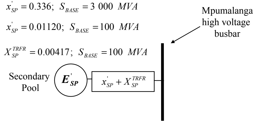
FIGURE E.2 Parameters of the Secondary Pool generator
