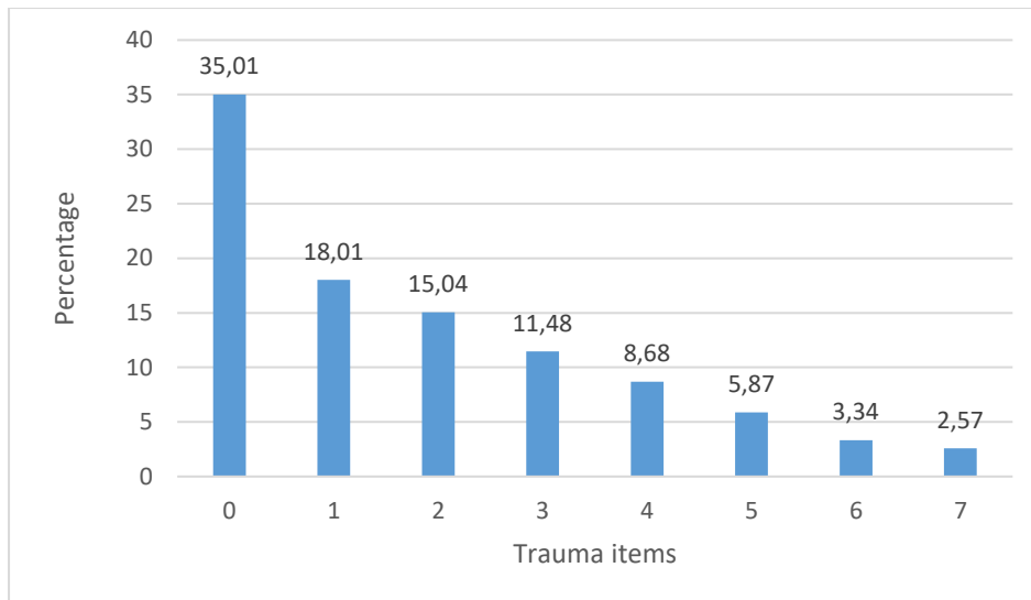
Figure 5: Distribution of the numbers of TE experienced
