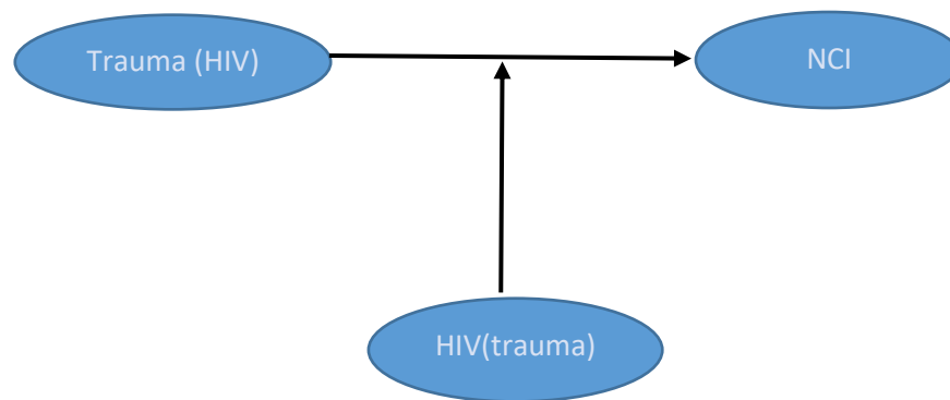
Figure 4 Directed Acyclic Graph (DAG) of variables conceptualized for examining causal relationships
