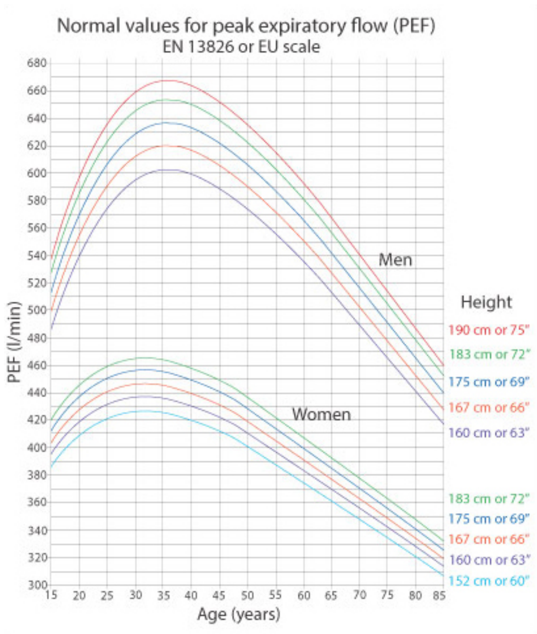
Figure 2-1: Nunn and Gregg nomogram for determining predicted PEF.(5)
