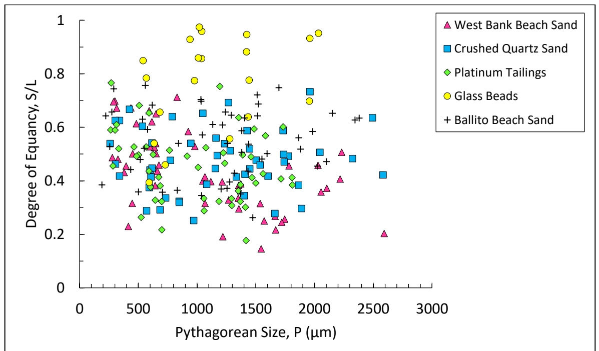
Figure 4-21: Degree of equancy, S/L , plotted against Pythagorean size,
