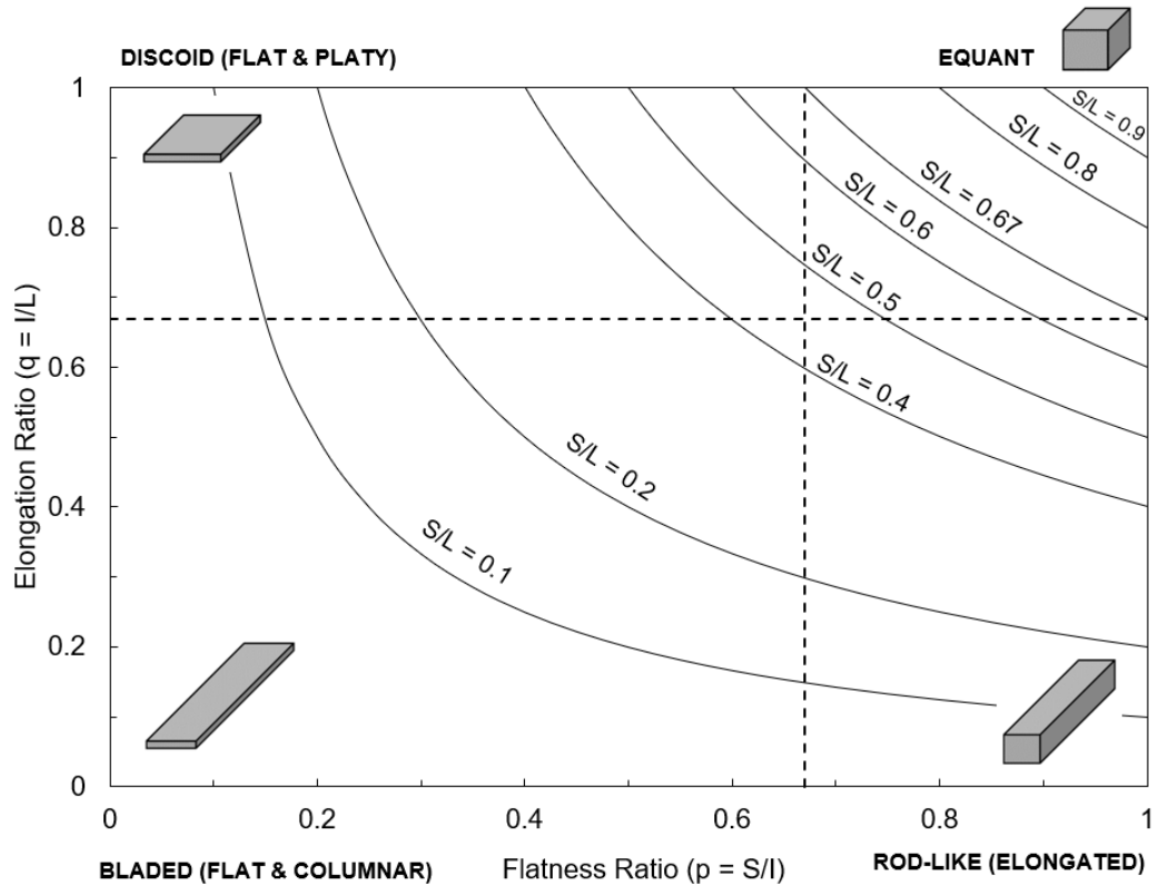
Figure 2-9: Isolines of S/L plotted on the Zingg diagram (drawn by the author).
