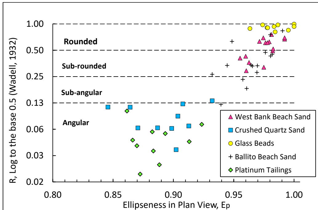
Figure 4-26: E_p plotted against R , including a roundness classification scheme proposed by Blott & Pye (2008).
