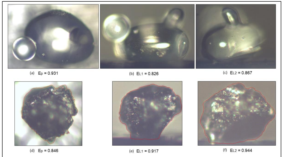
Figure 4-24: Comparison of E_p , E_{L1} , and E_{L2} : (a) to (c) glass bead, (d) to (f) platinum tailings particle.
