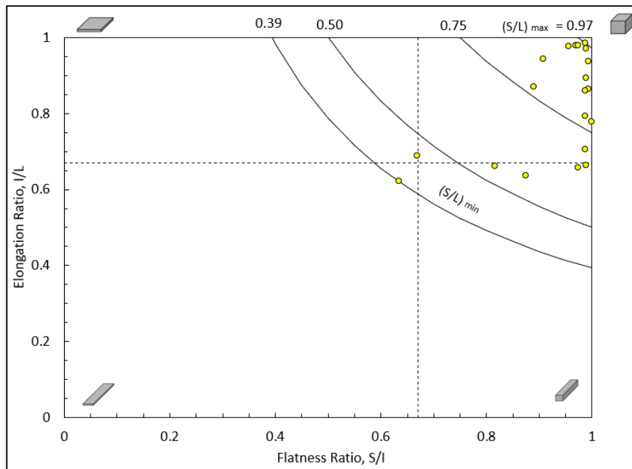
Figure 4-17: Plot of form parameters showing spherical glass beads.
