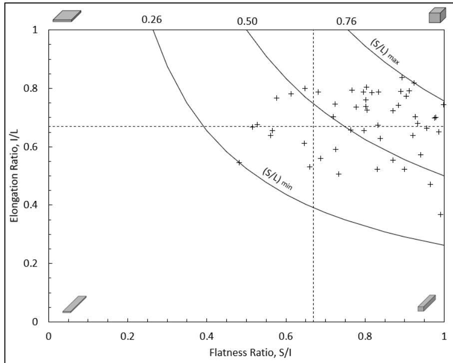
Figure 4-18: Plot of form parameters showing Ballito beach sand.
