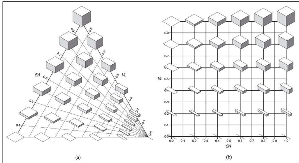
Figure 2-11: 36 Forms plotted at regular geometric intervals to ensure even distribution of elongation and flatness ratios (a) Sneed & Folk diagram, (b) Zingg diagram (Blott & Pye, 2008).
