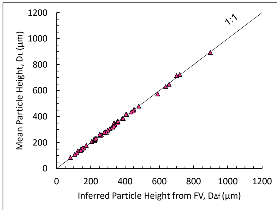
Figure 4-1: Relationship between D_L and D_{\Delta f} for West Bank beach sand.
