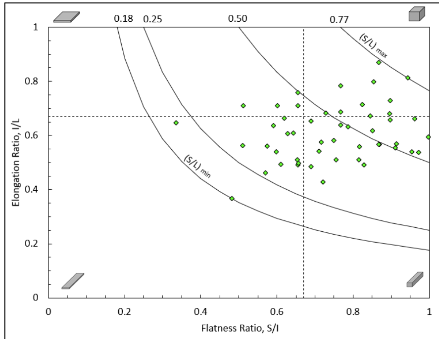
Figure 4-16: Plot of form parameters showing platinum tailings sand.
