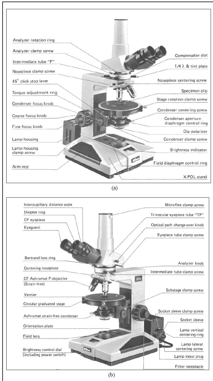
Figure 3-8: Illustration of Nikon Opti-phot Pol optical microscope, without epi-illumination system, (a) left view; (b) right view (OPTIPHOT-POL Instruction Manual).
