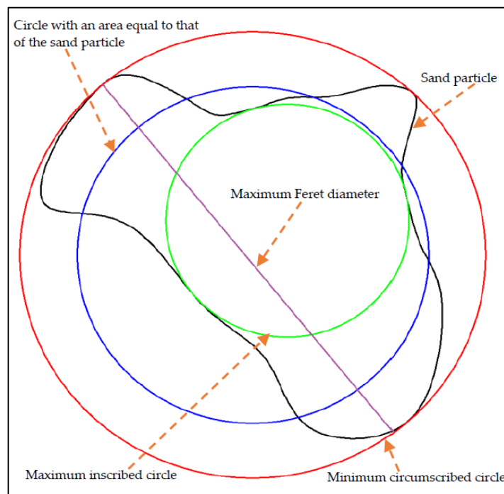
Figure 2-2: Plan view of the basic size parameters of an irregular sand particle (Wang et al., 2020).
