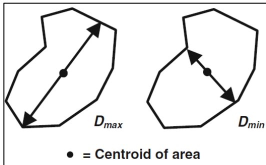
Figure 2-5: Definitions of D_{max} and D_{min} (Le Pen et al., 2013).
