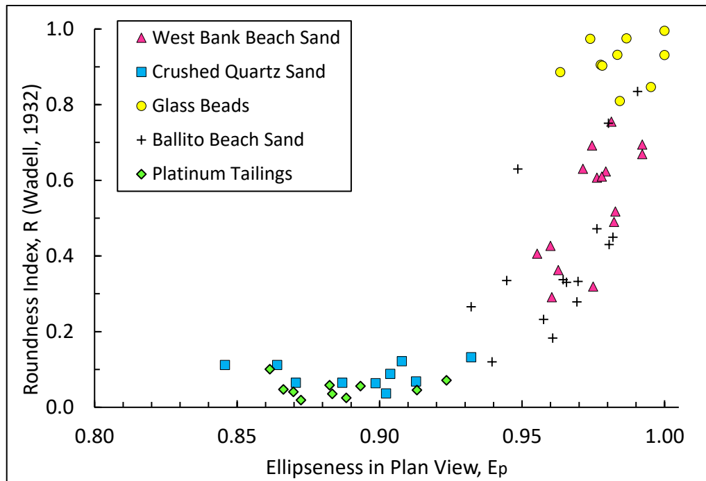
Figure 4-25: Evaluation of E_p against Wadell's (1932) roundness, R .
