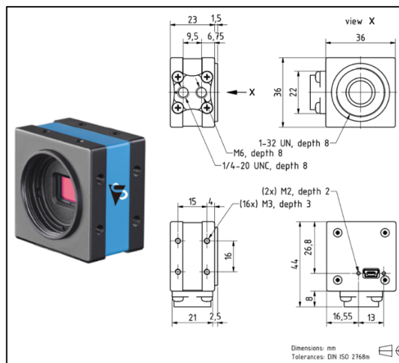
Figure 3-10: DFK 72AUC02 CMOS Sensor ( https://www.theimagingsource.com/products/industrial-cameras/usb-2.0-color/dfk72buc02/ ).
