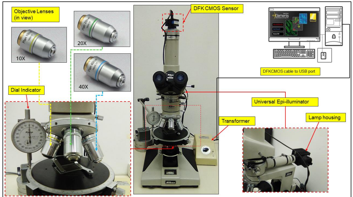
Figure 3-12: Establishment of the focus variation instrument.
