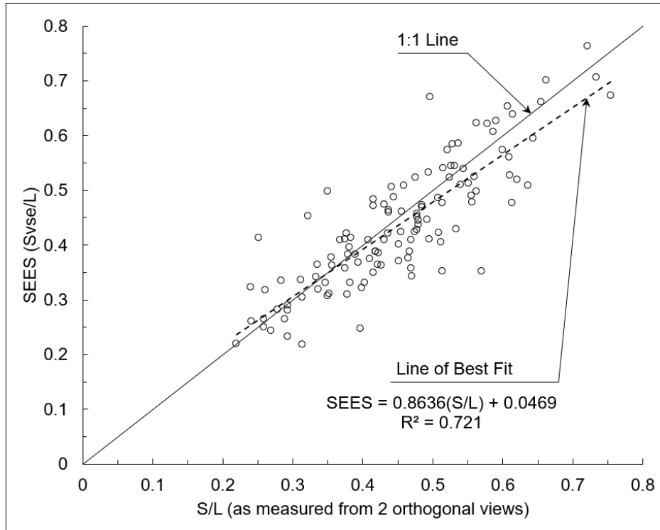
Figure 2-6: Comparison of S/L ratio using two methods (redrawn after Le Pen et al., 2013).
