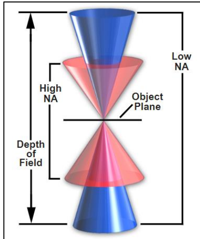
Figure 3-7: Depth of field ranges, where NA = numerical aperture ( https:// www.microscopyu.com/microscopy-basics/depth-of-field-and-depth-of-focus ).
