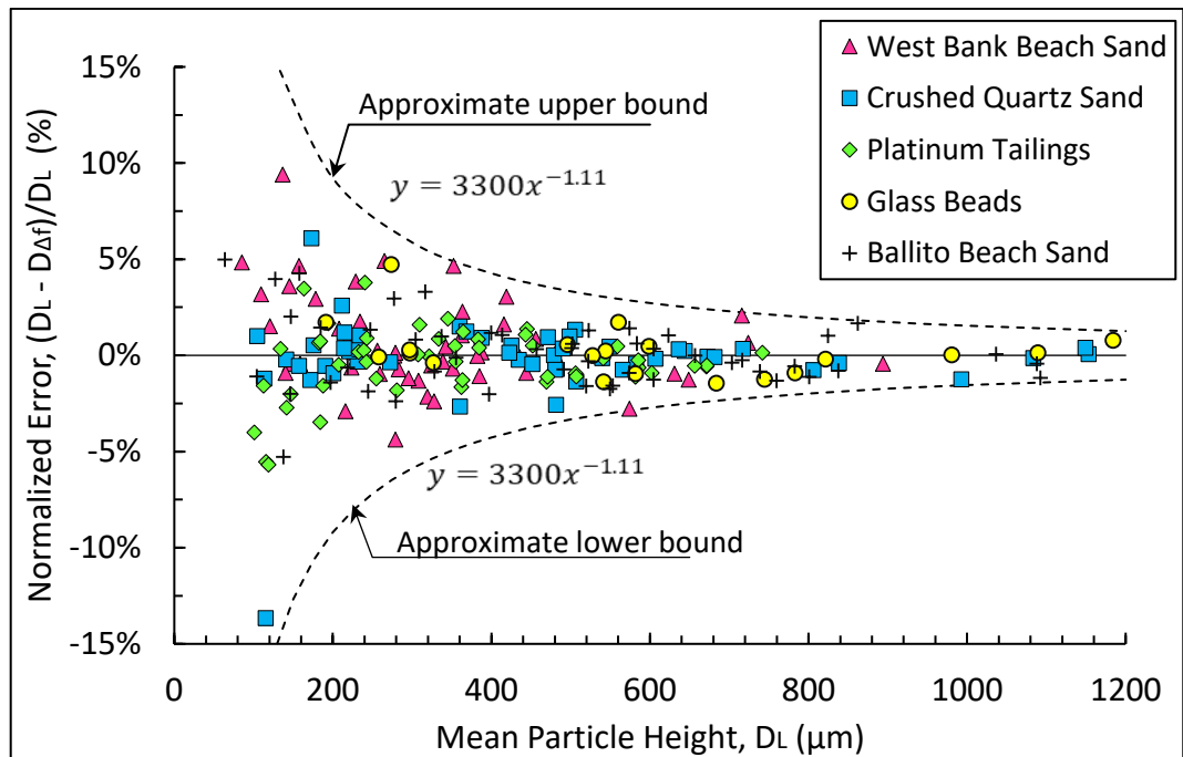
Figure 4-11: Relationship between the normalized error and D_L .
