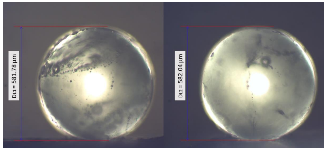
Figure 3-13: Measurement of particle height from two lateral views, on a glass bead particle.
