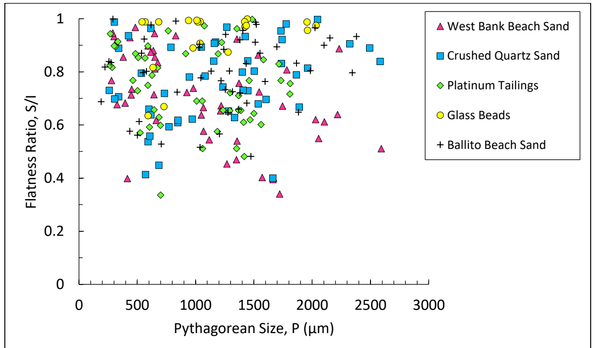
Figure 4-19: Flatness ratio, S/I , plotted against Pythagorean size, P .
