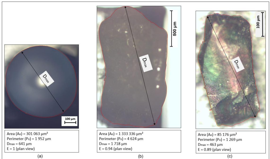
Figure 3-17: Parameters used to compute ellipseness in plan-view: (a) glass bead, (b) Ballito beach sand, and (c) tailings sand.
