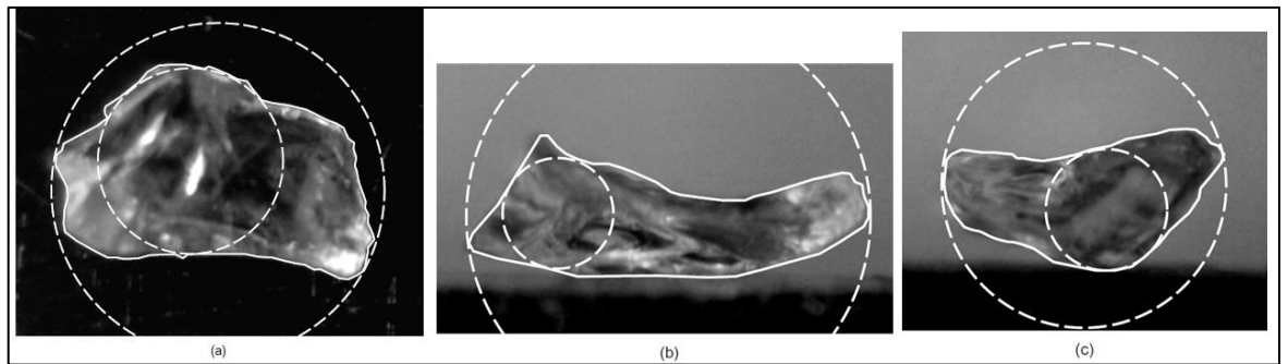
Figure 2-3: Example of the measurement of individual grain dimensions: (a) plan view, x-y plane; (b) elevation, y-z plane; (c) elevation, x-z plane. Dashed lines show minimum circumscribed circles and maximum inscribed circles for each view (Clayton et al., 2009).
