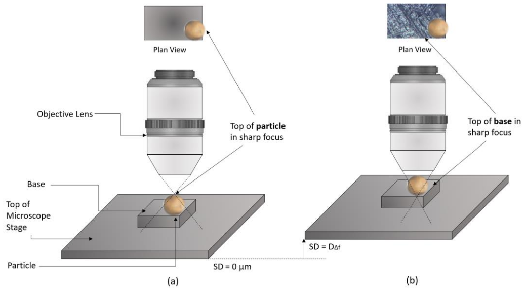
Figure 3-14: (a) start of FV procedure, (b) end of FV procedure.
