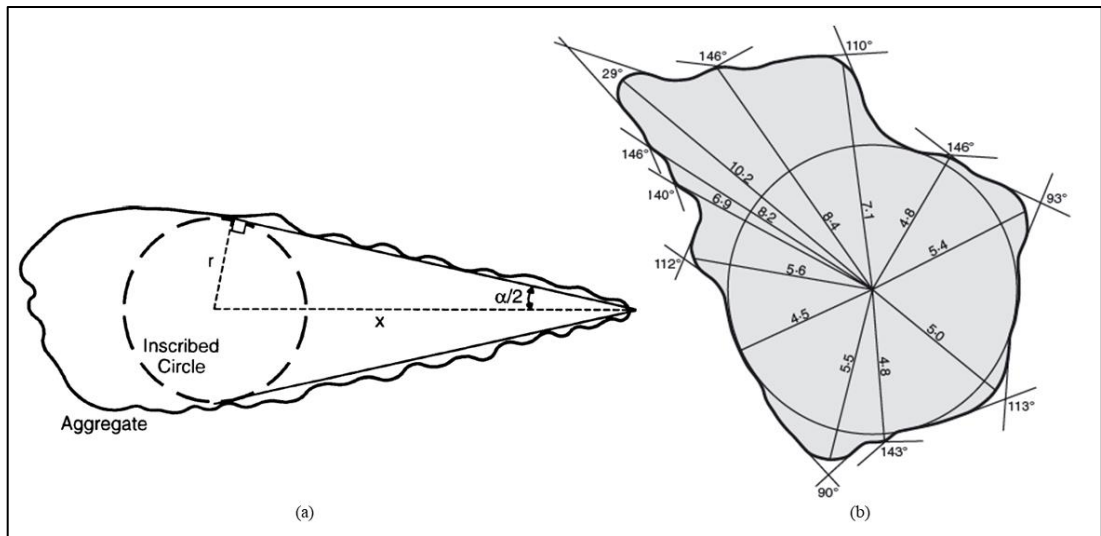
Figure 2-13: (a) Parameters for determining the degree of angularity (After Lees, 1964), (b) Schematic indicating the measure of angularity of each corner on a projected plane (Blott & Pye, 2008).
