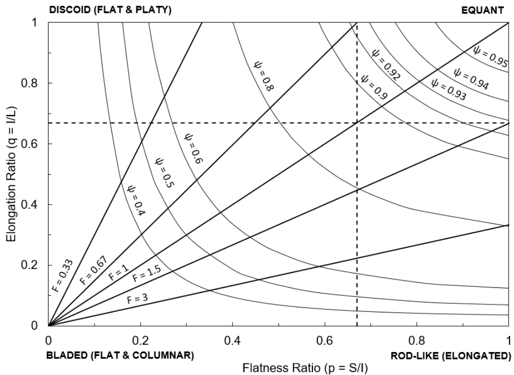
Figure 2-8: Isolines of working sphericity and shape factor plotted on the Zingg diagram (drawn by the author).
