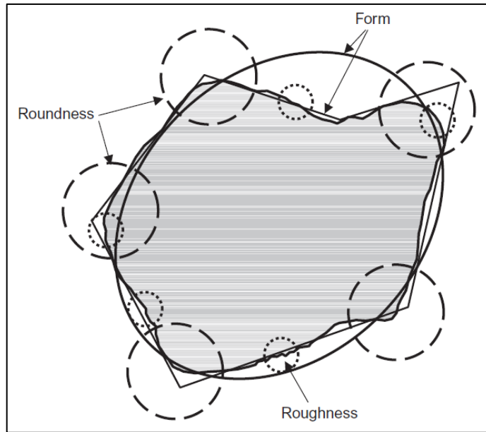
Figure 2-1: Elements of particle shape (after Clayton et al., 2009).
