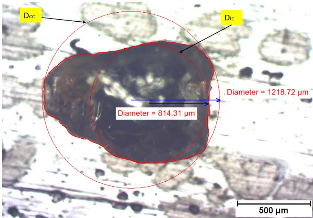
Figure 3-16: Measurement of D_{ic} and D_{cc} , in plan view at 50x magnification on a Ballito beach sand particle.
