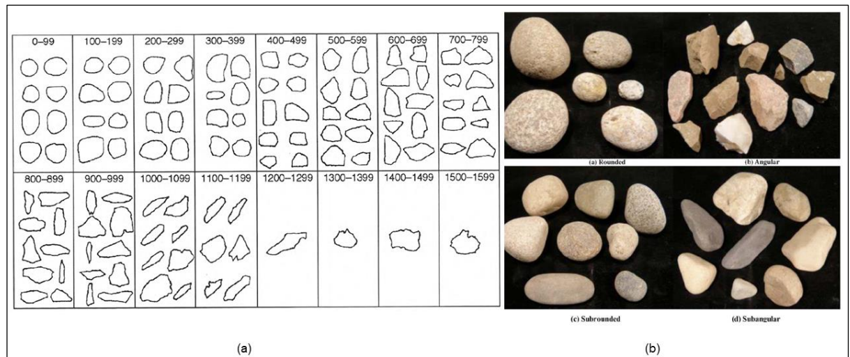
Figure 2-14: Visual description for particle angularity, (a) Degree of angularity (After Lees, 1964), and (b) Visual identification of aggregate angularity (after ASTM D 2488-17E01, 2017).
