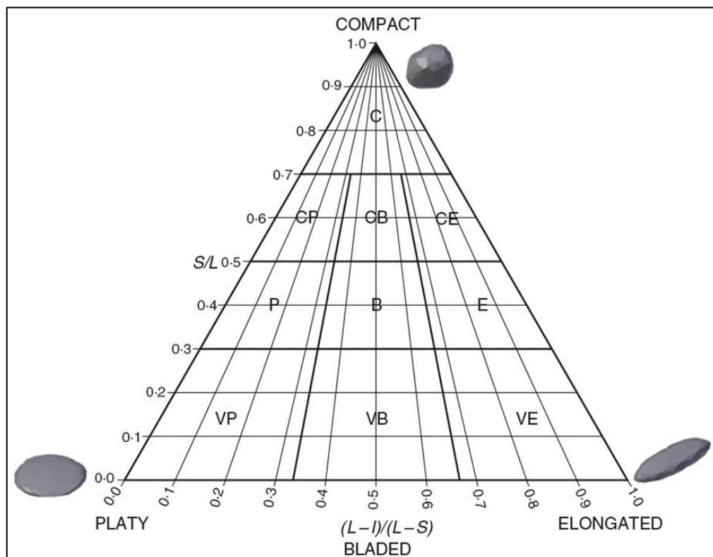
Figure 2-10: Sneed & Folk (1958) ternary diagram comprising ten classes of form: C (compact), CP (compact-platy), CB (compact-bladed), CE (compact-elongated), P (platy), B (bladed), E (elongated), VP (very platy), VB (very bladed), VE (very elongated) (redrawn after Blott & Pye, 2008).
