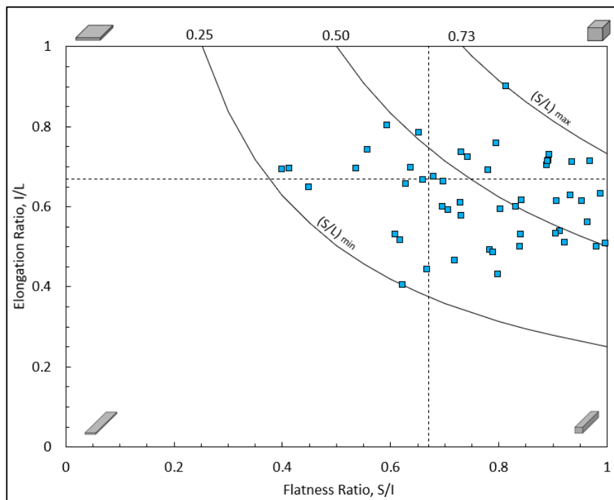
Figure 4-15: Plot of form parameters showing crushed quartz sand.
