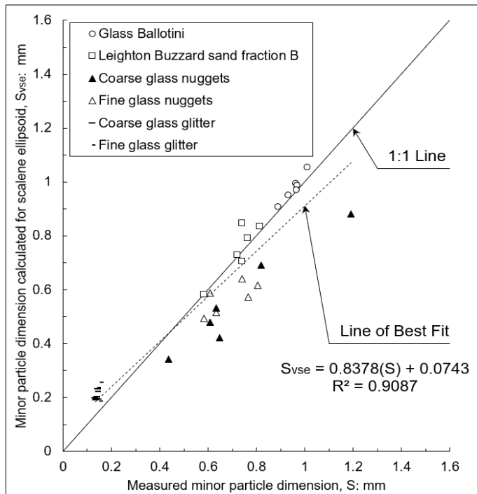
Figure 2-4: Comparison of S and S_{vse} (redrawn after Clayton et al., 2009).
