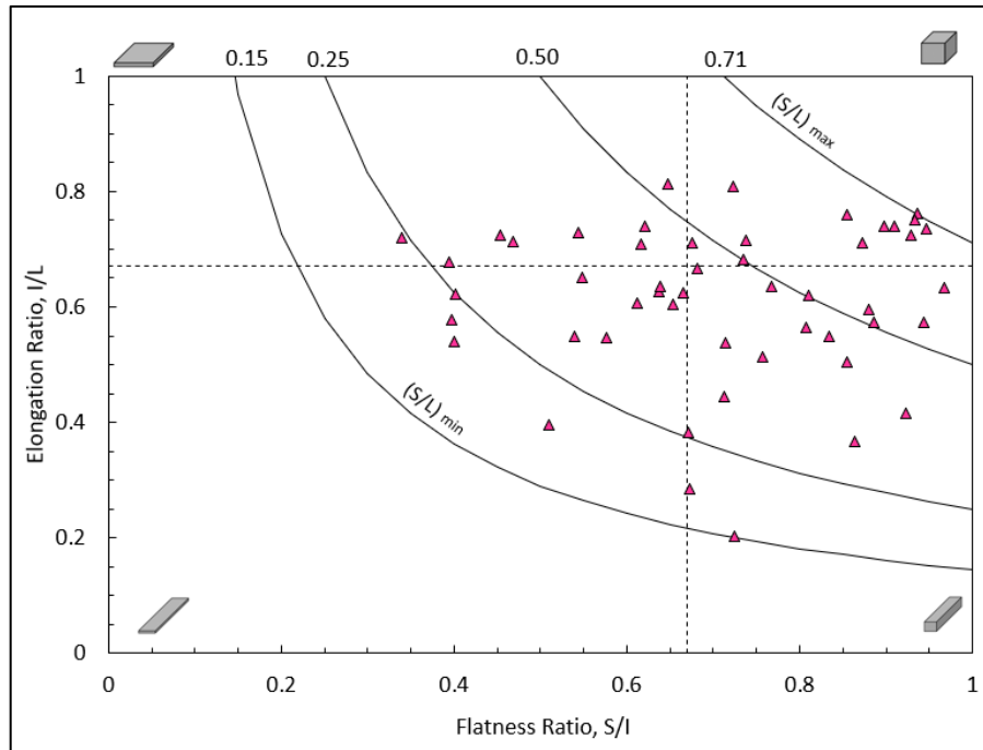
Figure 4-14: Plot of form parameters showing West Bank beach sand.
