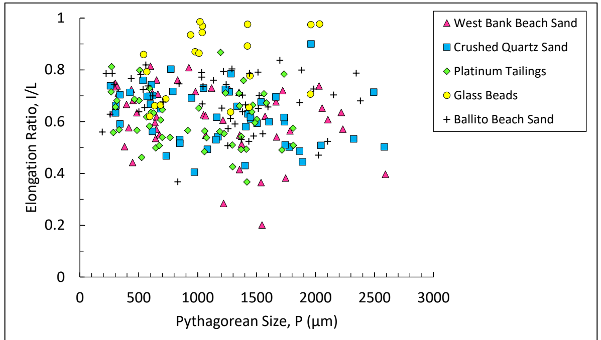
Figure 4-20: Elongation ratio, I/L , plotted against Pythagorean size, P .
