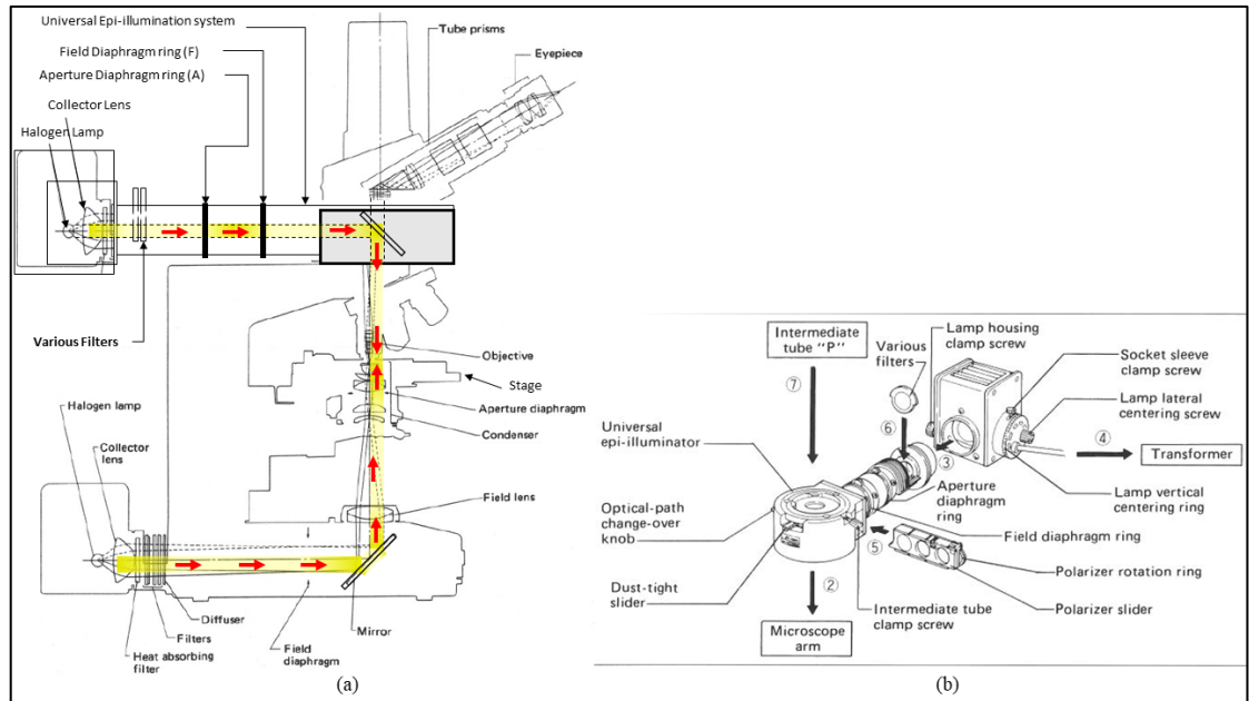
Figure 3-9: (a) Optical path of the Nikon Opti-phot Pol optical microscope; (b) Universal epi-illuminator (OPTIPHOT-POL Instruction Manual).
