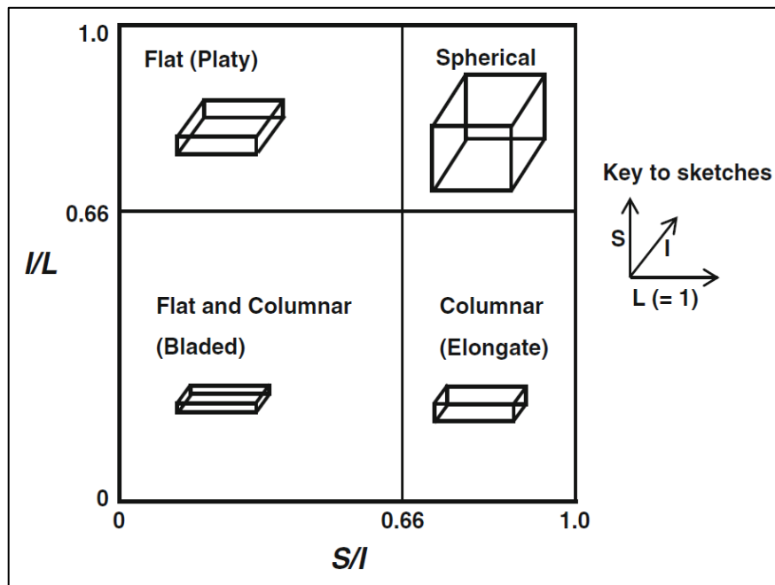
Figure 2-7: Zingg (1935) diagram (After Le Pen et al., 2013).
