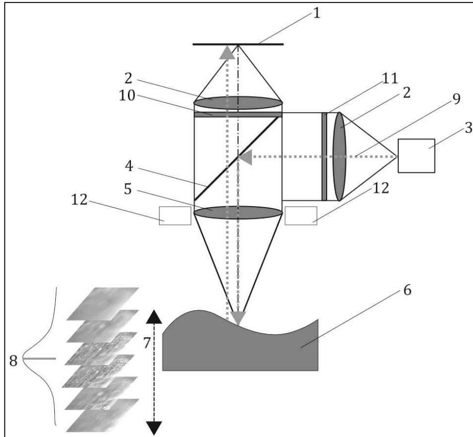
Figure 3-6: Schematic diagram of a typical measurement device based on focus variation: (1) CCD sensor, (2) lenses, (3) white light source, (4) semi-transparent mirror, (5) objective lens with limited depth of field, (6) sample, (7) vertical movement with driving unit, (8) contrast curve calculated from the local window, (9) light rays from the white light source, (10) optional analyser, (11) optional polarizer and (12) optional ring light (from Helmli, 2011).
