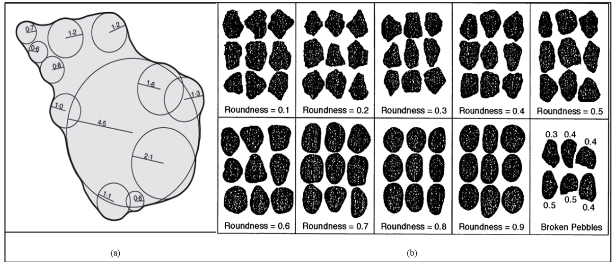
Figure 2-12: (a) Schematic demonstrating the measure of roundness proposed by Wadell (1932), (from Blott & Pye, 2008). (b) Roundness chart for 16 – 32 mm aggregate, Krumbein (1941).
