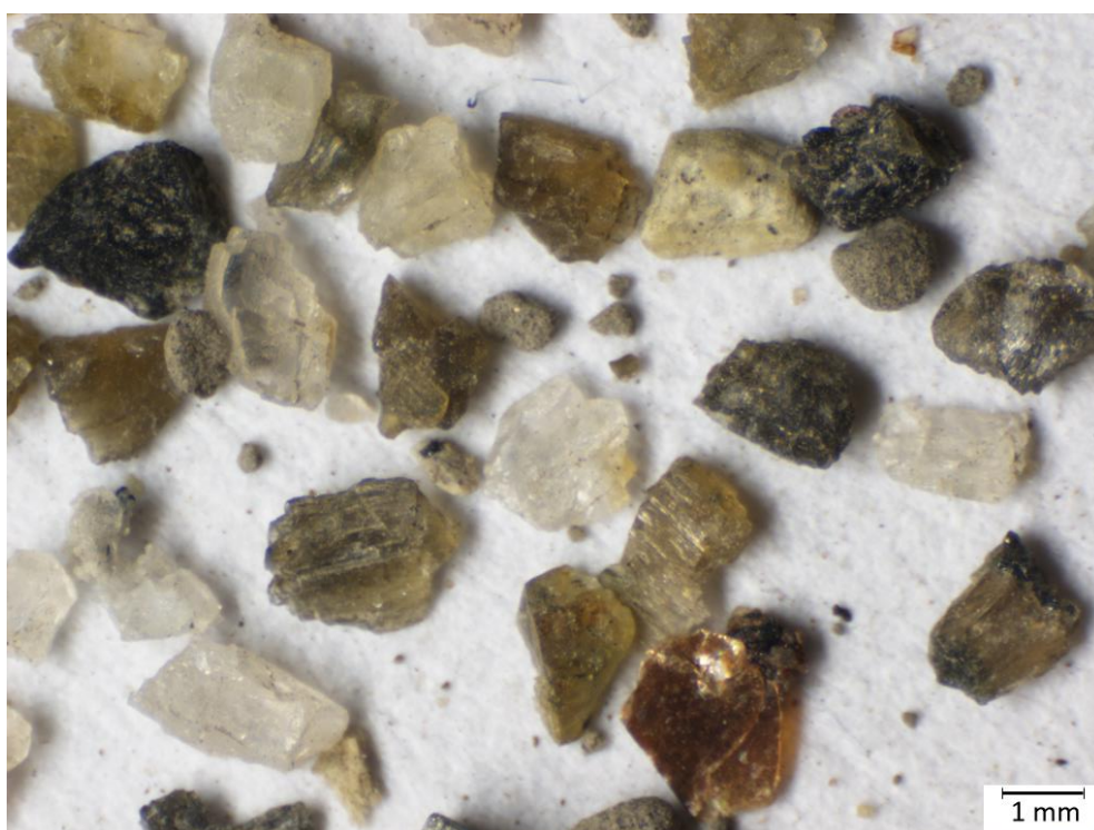
Figure 3-4: Photomicrograph of platinum tailings sand.
