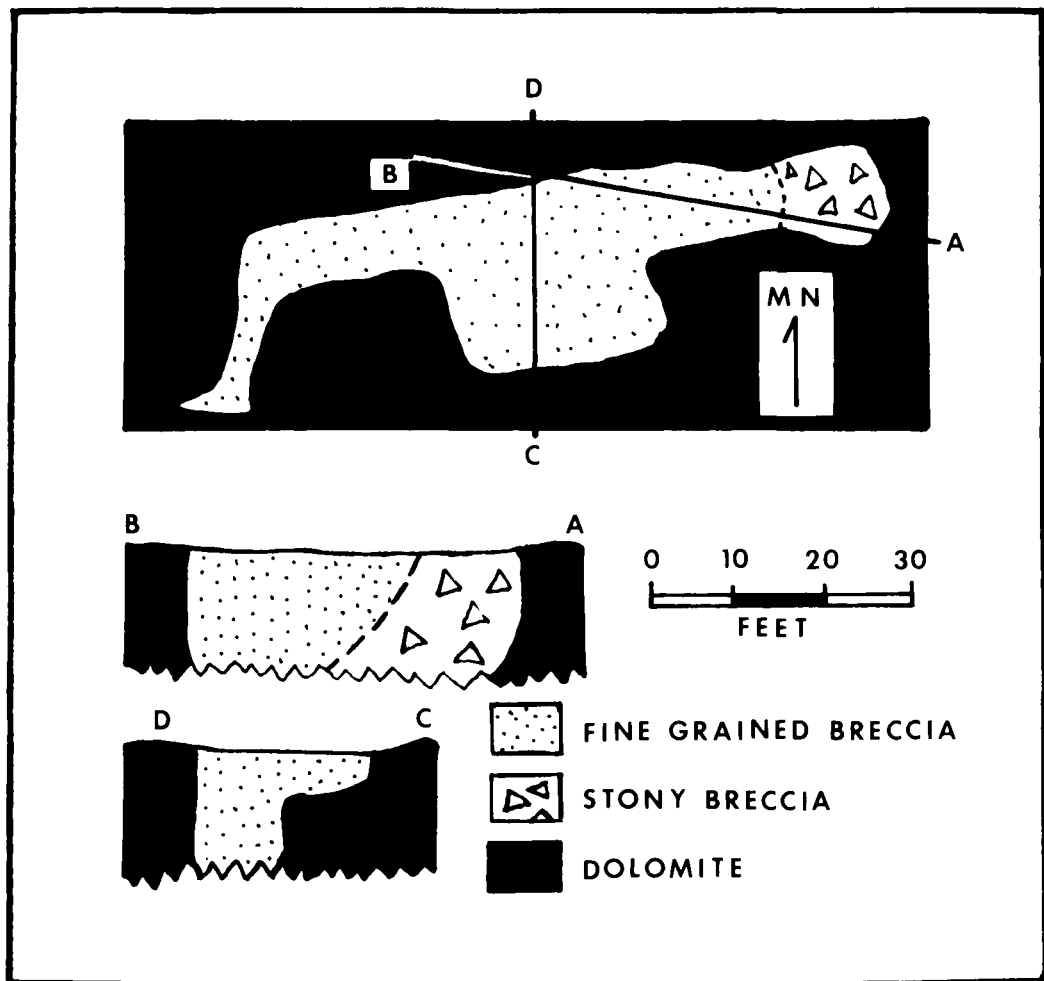
Fig. 23 A plan and vertical sections through the Kromdraai A cave. (after Brain 1958 )
