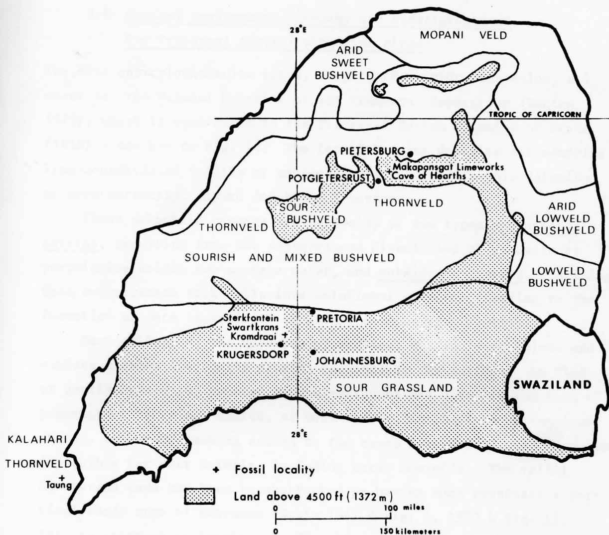
Fig. 2 Map of the Transvaal showing the principal vegetation zones and the location of the five South African australopithecine sites and the Cave of Hearths.
