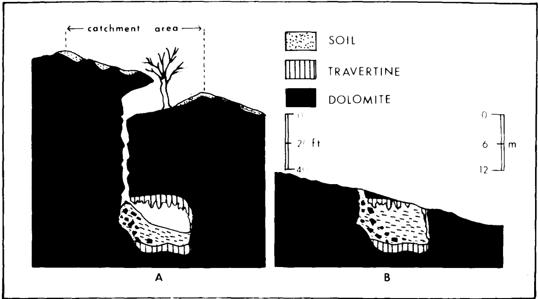
Fig. 21 Diagrammatic N-S vertical section through the Swartkrans hillside: A: reconstructed original rockshelter and shaft and B: with the shaft removed by erosion as it is today. after Brain 1967d and 1970b
