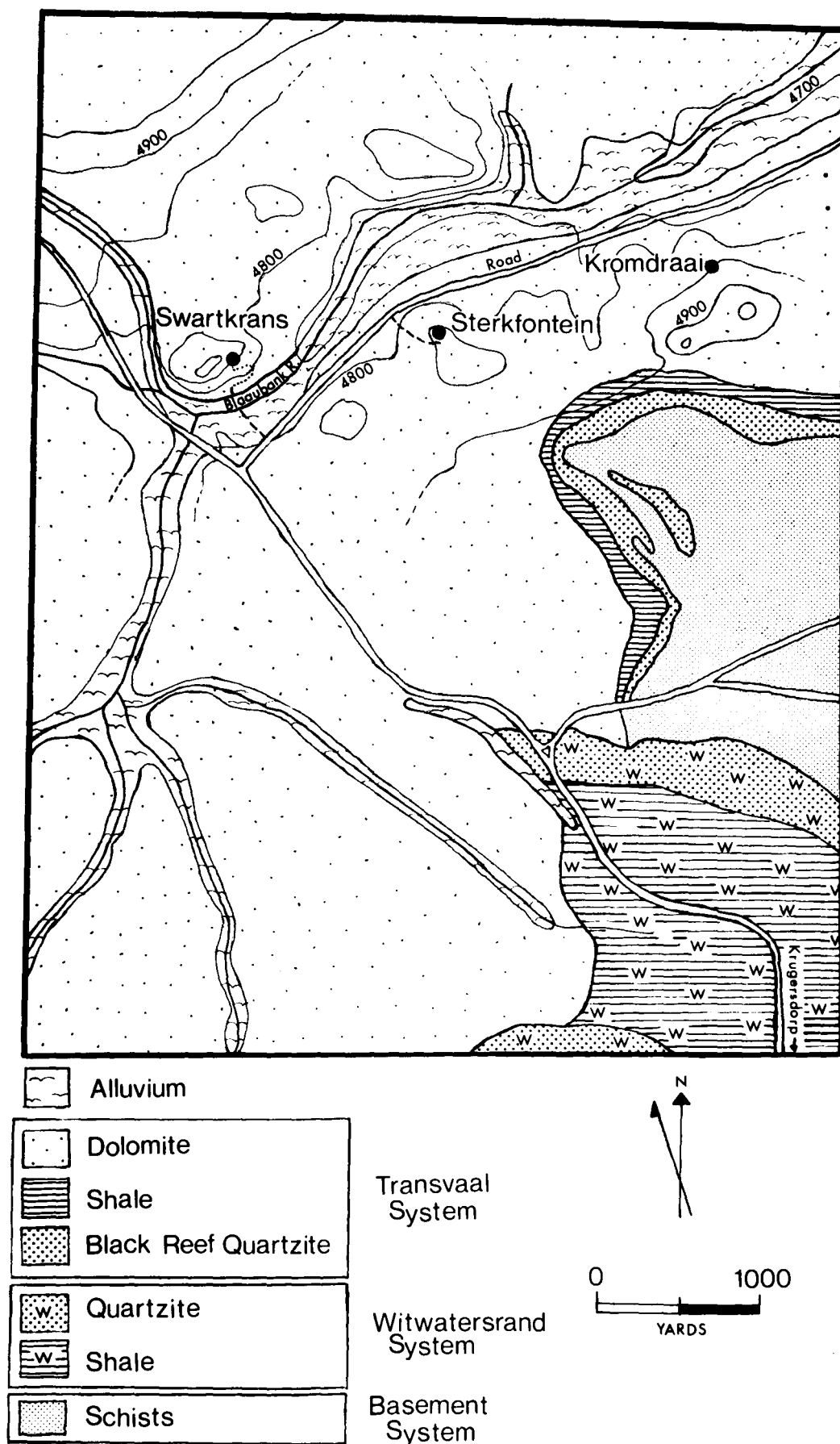
Fig.16 Map of the Sterkfontein area, showing geology and altitude and the positions of Swartkrans, Sterkfontein and Kromdraai relative to roads and to the Blaauwbank stream. (after Brain 1958. figs. 37 and 38.)
