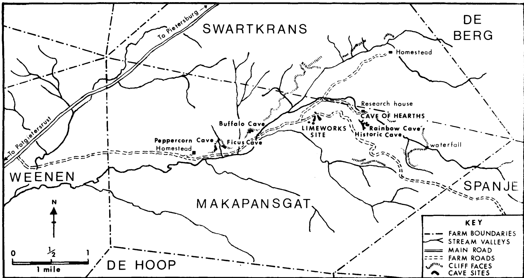
Fig. 3 Plan of the Makapansgat valley showing the location of the Limeworks and Cave of Hearths and other caves of palaeontological or archaeological interest. ( after Wells and Cooke 1956 )
