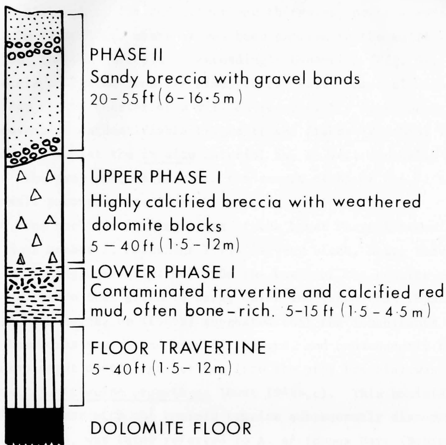
Fig. 8 Composite stratigraphic profile for the whole of the Limeworks deposit. (after Brain 1958)
