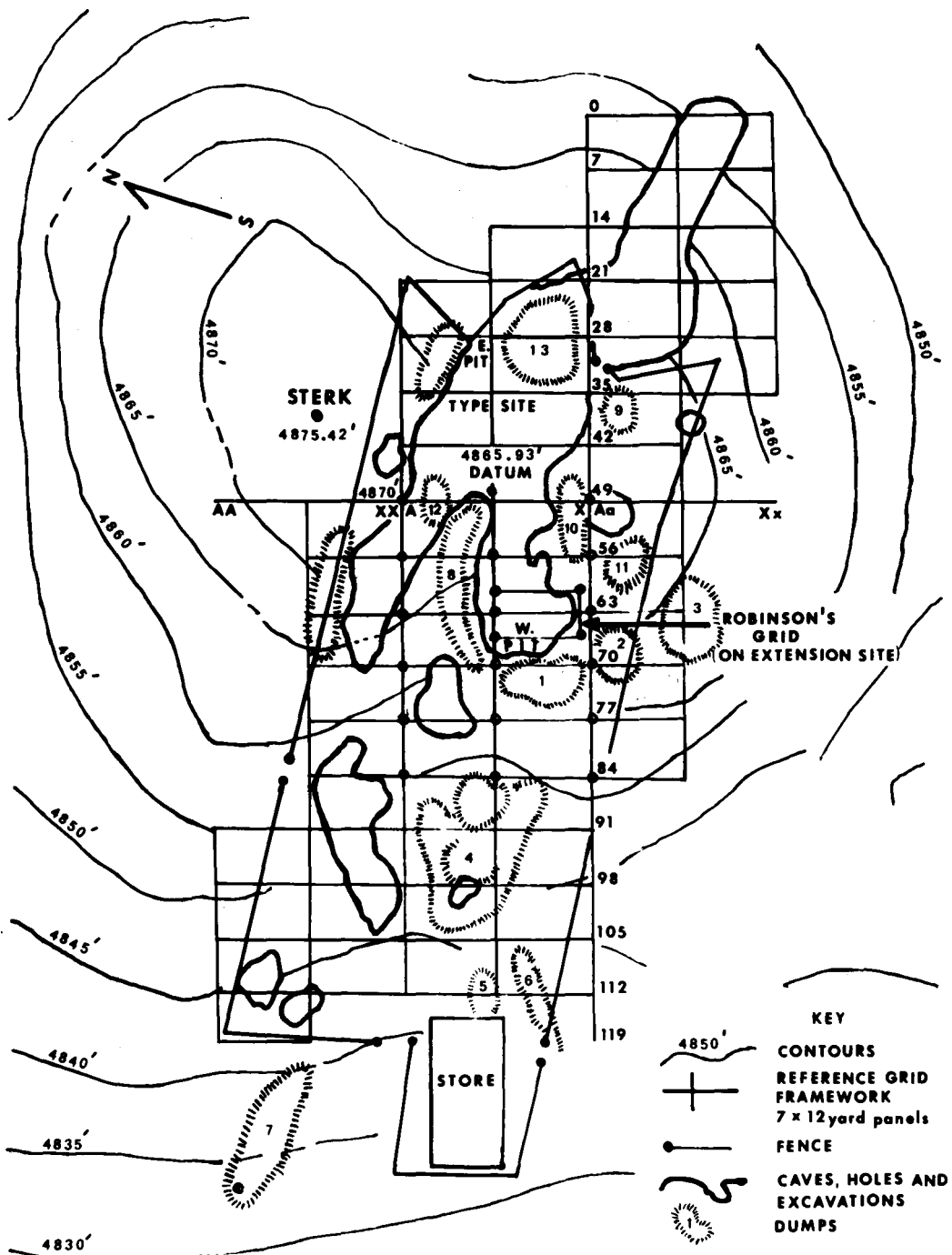
Fig.18 Contour plan of the Sterkfontein koppie showing excavations and the present grid framework. (after Watt, I.B. in Tobias and Hughes 1969 )
