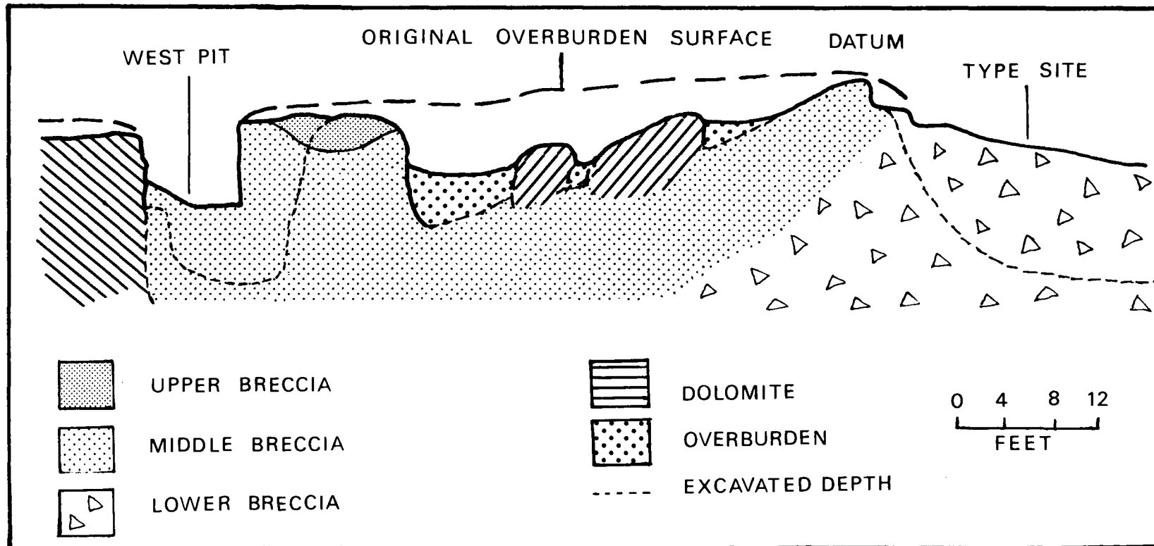
Fig. 19 E-W section through the Extension Site and portion of the Type Site showing breccias. ( after Robinson 1962 )
