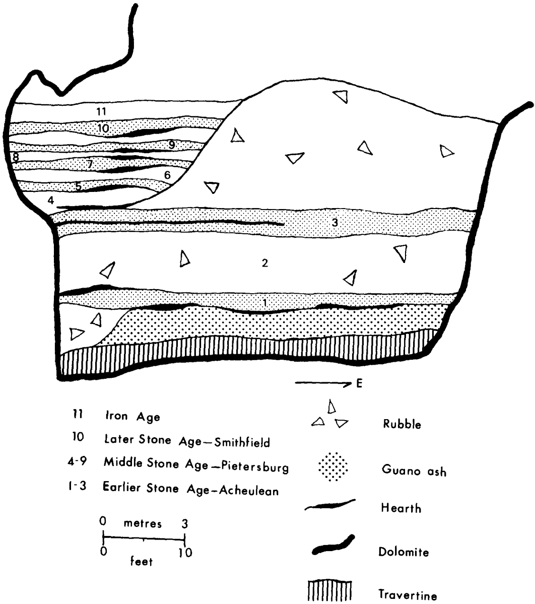
Fig. 15 Mason's 1962 stratigraphic profile of the Cave of Hearths. (Mason 1962 fig. 51)
