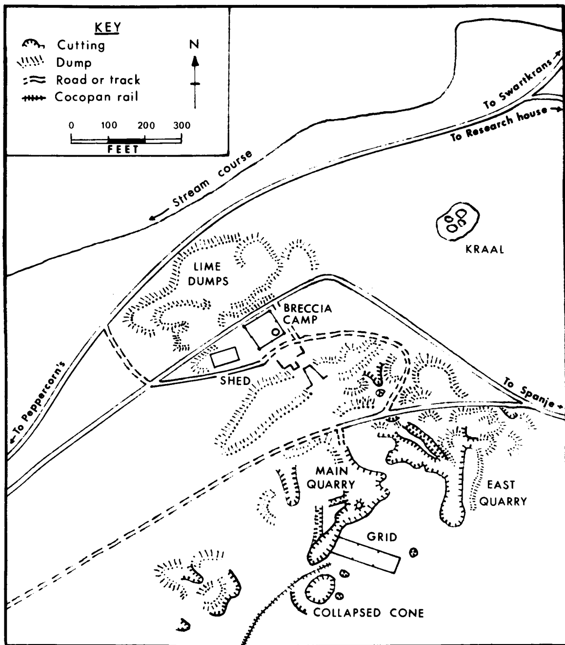
Fig. 6 Map showing the surface features of the area surrounding the Limeworks site. (after Brain 1958, modified by Maguire, pers. comm.)
