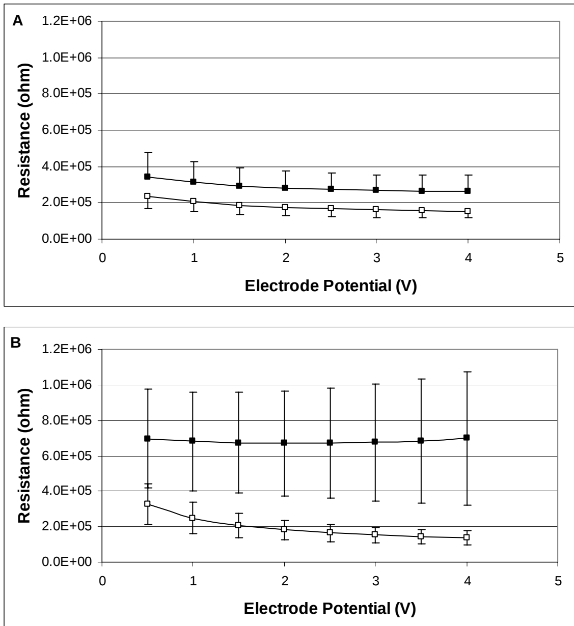
Fig. 3.5 Skin resistance versus voltage after the 'breakthrough effect':
