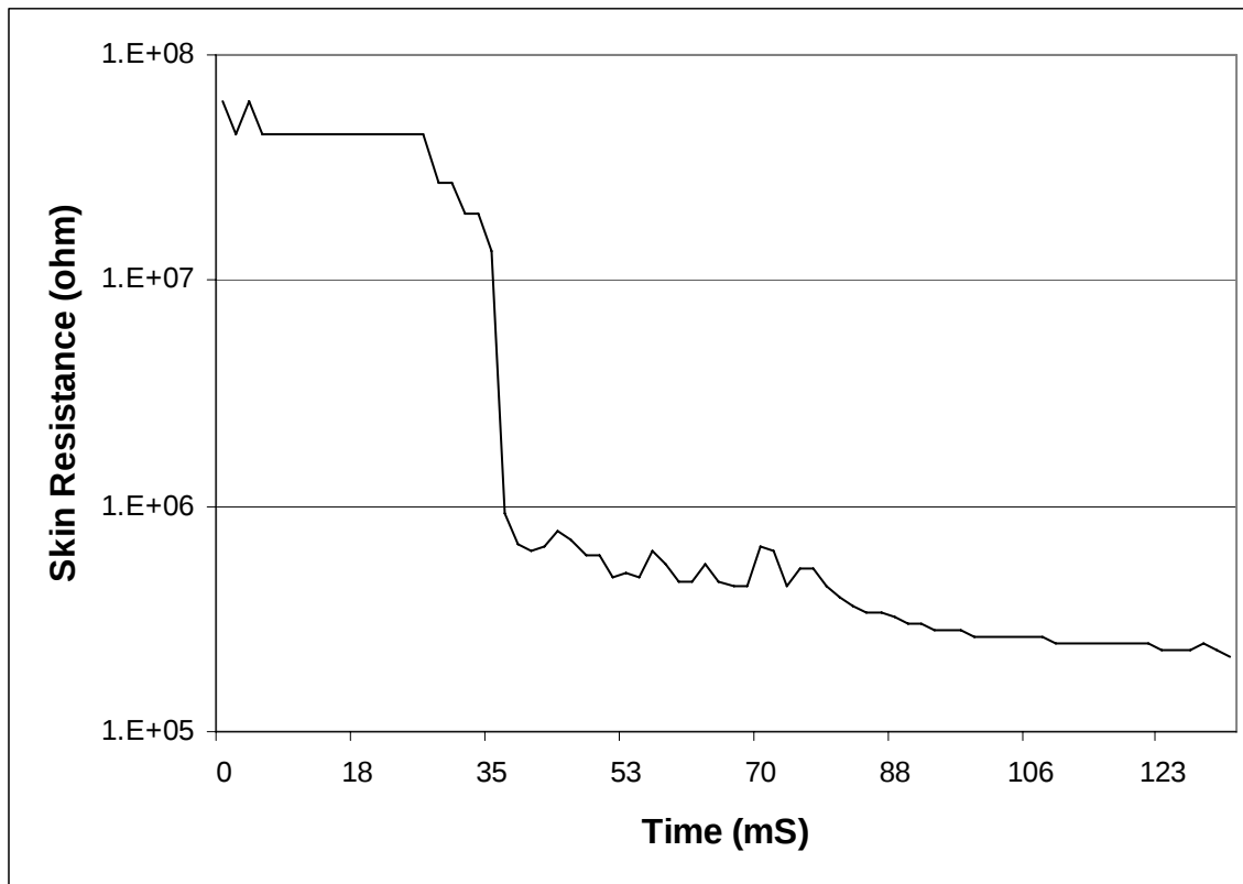
Fig.3.4 Example of reversible skin resistance ‘breakthrough’ under constant voltage stimulation.
