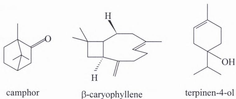
Figure 51: Chemical structures for major compounds detected in the essential oil of Salvia namaensis .
