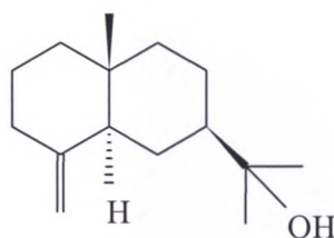
\beta -eudesmol
