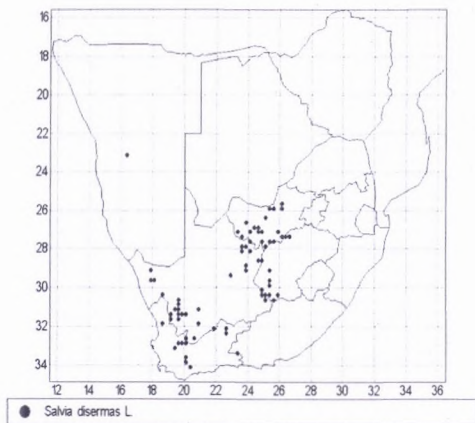
Figure 36: Geographical distribution of Salvia disermas .
