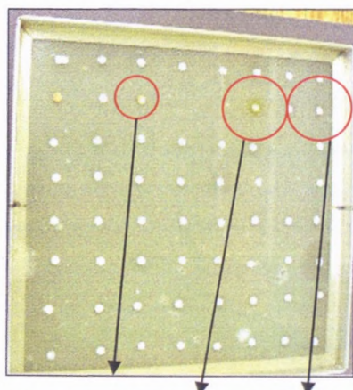
Figure 60: Agar plate ( C. albicans ) showing zones of inhibition by the oils tested.
