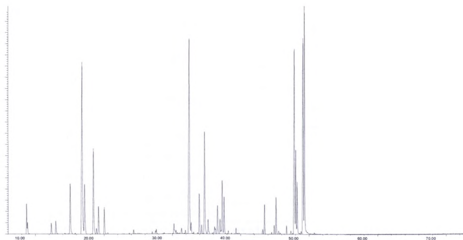
Figure 34: GC-MS profile of the hydro-distilled essential oil obtained from Salvia africana-lutea .
