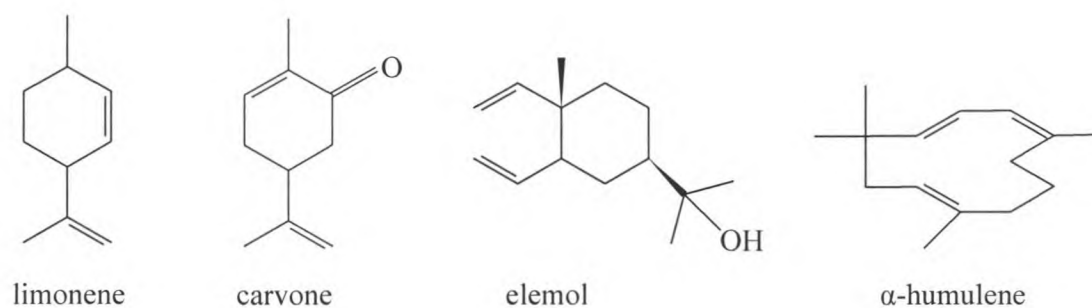
Figure 29: Chemical structures for major compounds detected in the essential oil of Ocimum americanum .
