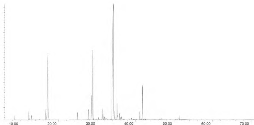
Figure 25: GC-MS profile of the hydro-distilled essential oil obtained from Mentha longifolia .
