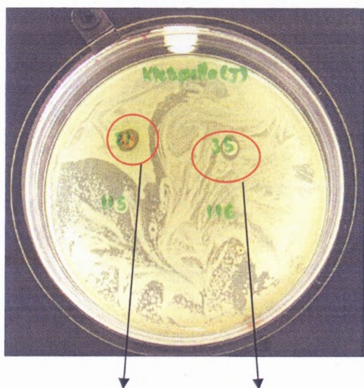
Figure 59: Zones of inhibition caused by Mentha longifolia against K. pneumoniae .
