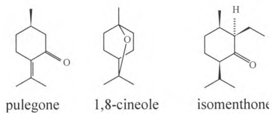
Figure 26: Chemical structures for major compounds detected in the essential oil of Mentha longifolia .
