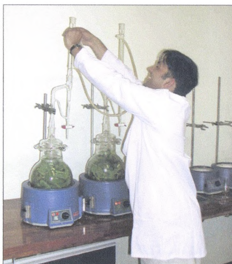
Figure 2: Distilling of plant material using the Clevenger apparatus.
