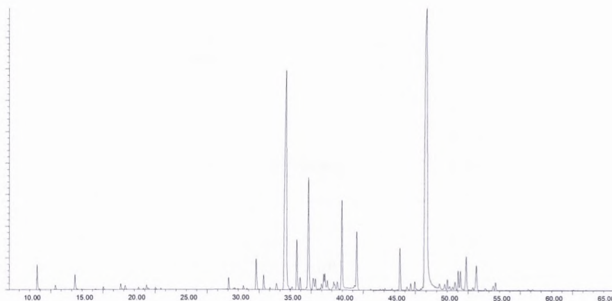
Figure 56: GC-MS profile of the hydro-distilled essential oil obtained from Salvia runcinata .
