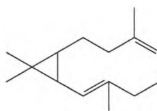
bicyclogermacrene
