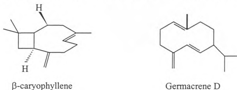
Figure 20: Chemical structures for major compounds detected in the essential oil of Leonotis leonurus .
