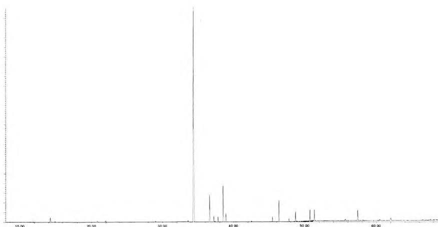
Figure 14: GC-MS profile of the hydro-distilled essential oil obtained from Hemizygia pretoriae .
