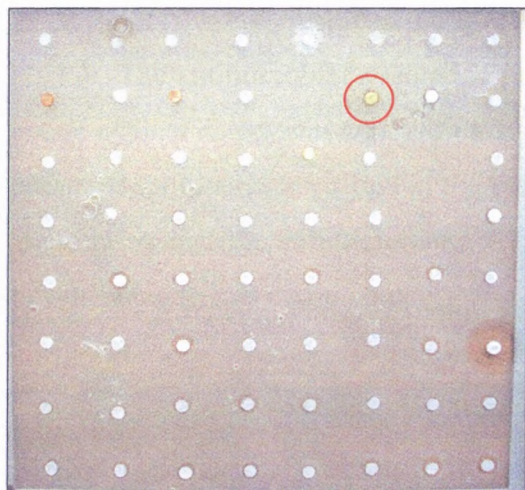
Figure 58: Zone of inhibition (indicated by the red circle) caused by Mentha longifolia against S. aureus .
