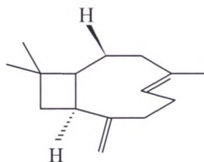
\beta -caryophyllene
