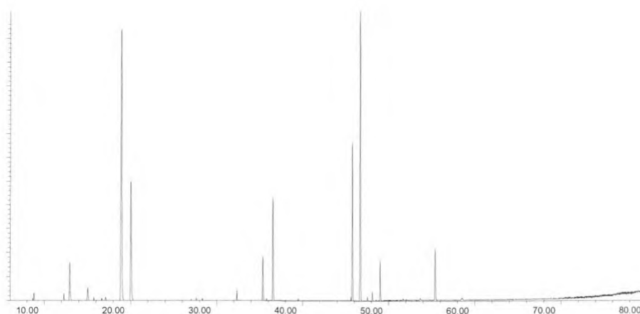
Figure 8: GC-MS profile of the hydro-distilled essential oil obtained from Hemizygia modesta .
