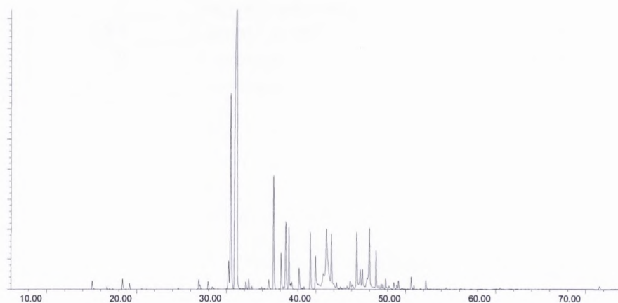
Figure 40: GC-MS profile of the hydro-distilled essential oil obtained from Salvia disermas .
