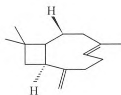
\beta -caryophyllene
