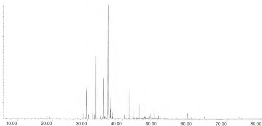
Figure 19: GC-MS profile of the hydro-distilled essential oil obtained from Leonotis leonurus .
