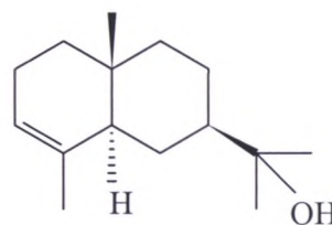
\alpha -eudesmol
