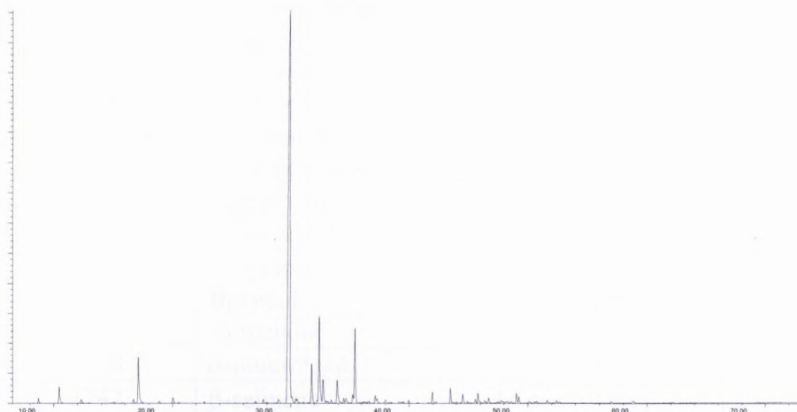
Figure 50: GC-MS profile of the hydro-distilled essential oil obtained from Salvia namaensis .
