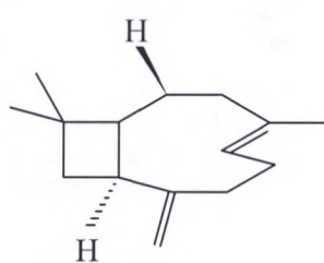
\beta -caryophyllene
