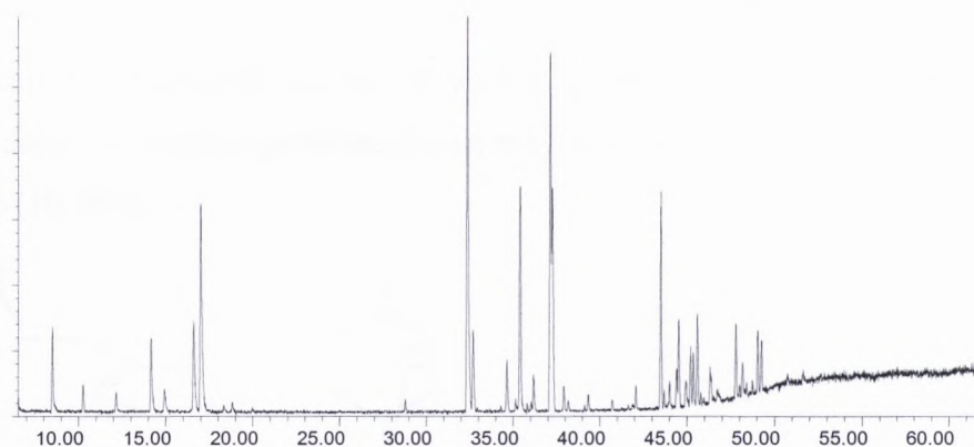
Figure 46: GC-MS profile of the hydro-distilled essential oil obtained from Salvia dolomitica .
