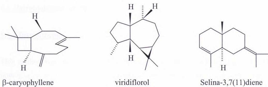
Figures 57: Chemical structures for major compounds detected in the essential oil of Salvia runcinata .
