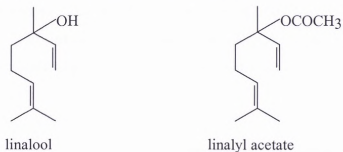
Figure 41: Chemical structures for major compounds detected in the essential oil of Salvia disermas .
