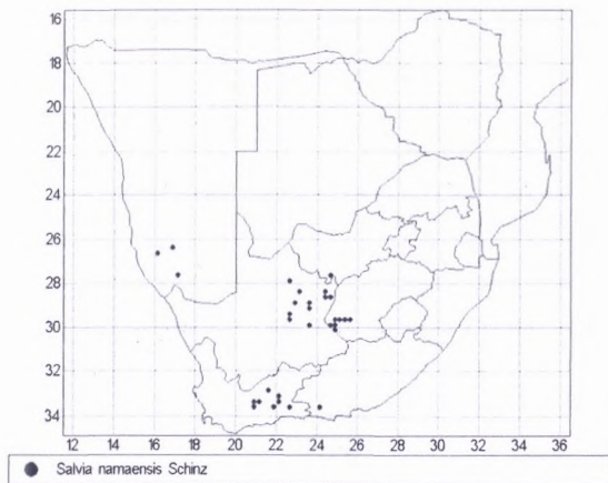
Figure 48: Geographical distribution of Salvia namaensis .
