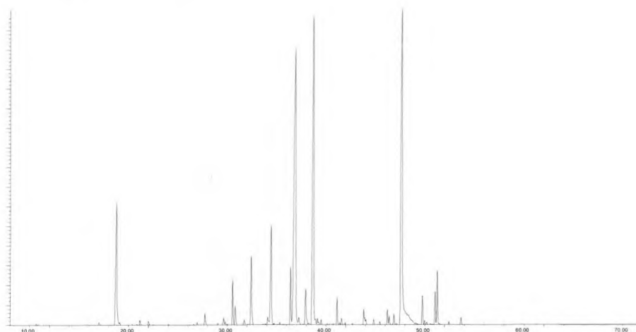
Figure 28: GC-MS profile of the hydro-distilled essential oil obtained from Ocimum americanum .
