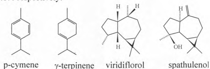
Figure 9: Chemical structures for major compounds detected in the essential oil of Hemizygia modesta .
