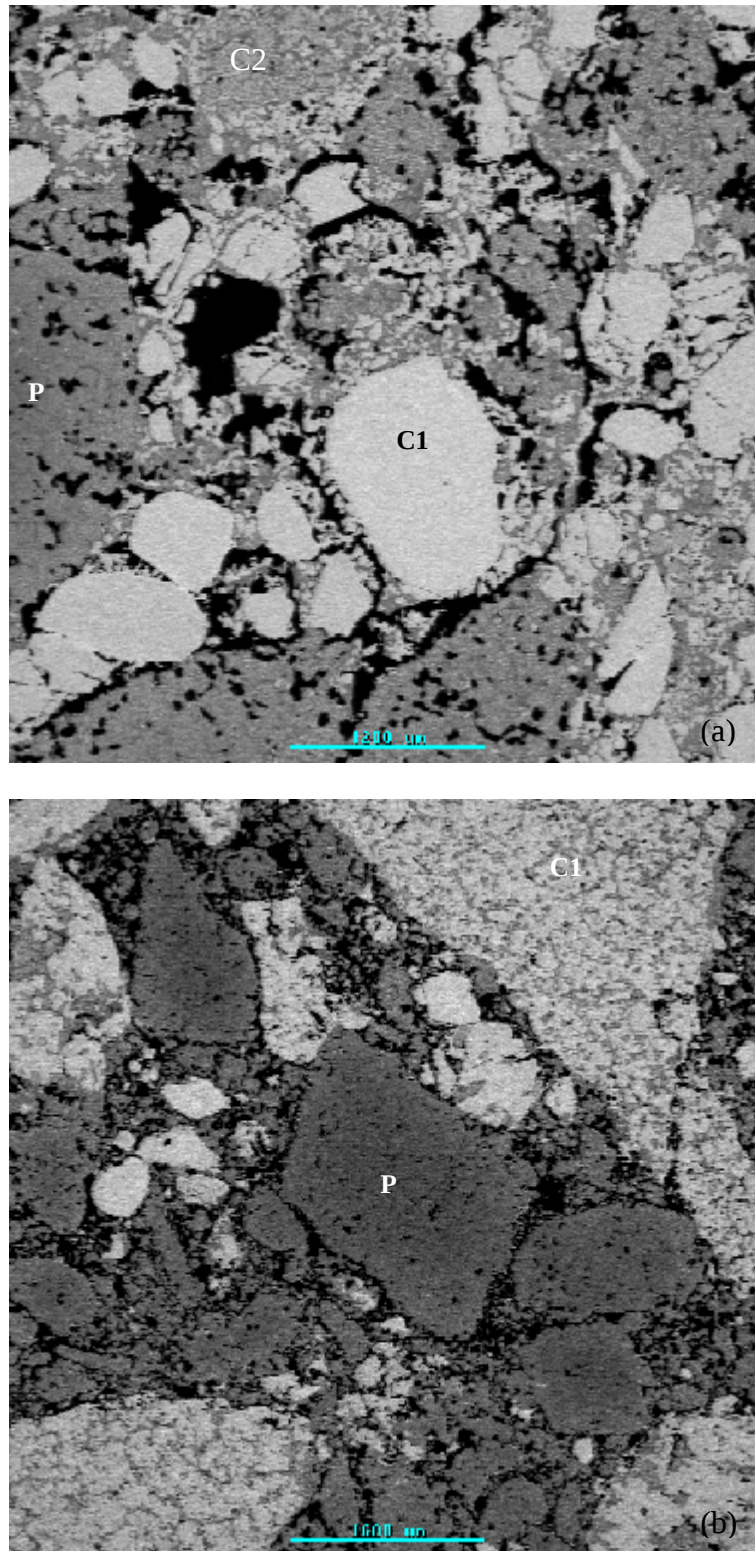
Figure 4.18. SEM-BSE micrographs of (a) Chrome-magnesite A reacted in \text{SO}_2\text{-O}_2 gas mixture at 1350C, showing gray phase = magnesia (periclase P), black= pores. Intragranular precipitate chromites =C2. (b) Chrome-magnesite D50-C5 showing bright phase= chromite (C1) with discontinuous magnesium spinel pockets, gray phase = magnesia (periclase P), black= pores.
