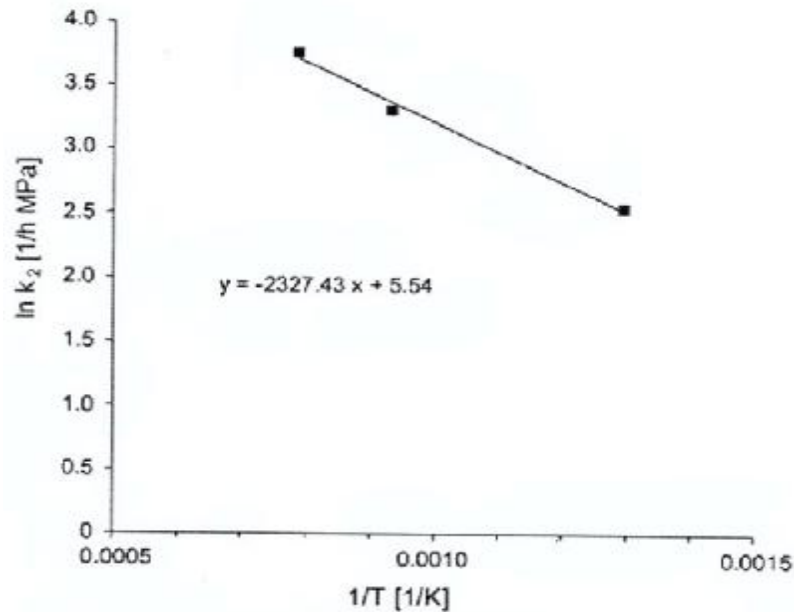
Figure 2.4. Reaction rate constant k_2 of MgO in \text{SO}_2\text{-O}_2 system between 500°C and 1000°C (Reference Podwórny, Piotrowski and Wojsa 78 ).
