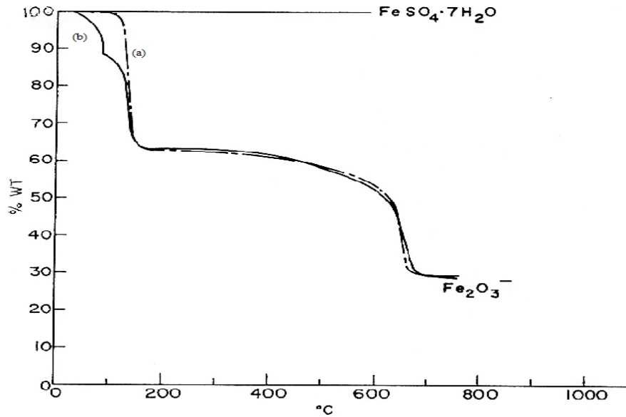
Figure 2.2. Decomposition curves of iron (II) sulfate during heating: (a) in air; (b) in oxygen atmosphere (Reference Gallagher, Johnson and Schrey 81 ).
