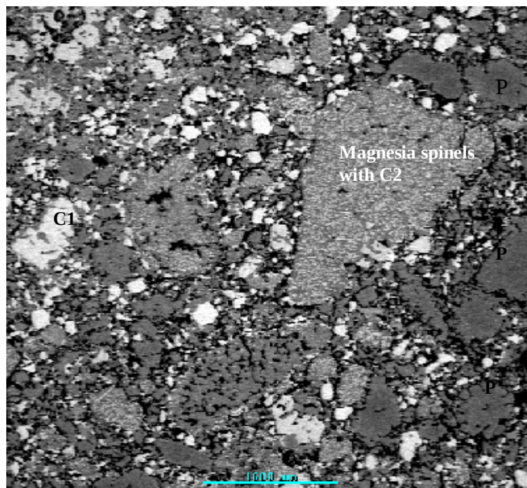
Figure 4.20. SEM-BSE micrograph of Magnesite-chrome brick 1 reacted in \text{SO}_2\text{-O}_2 gas mixture at 1350C, showing bright phase= chromite (C1), intragranular precipitate chromites =C2, gray phase = magnesia (periclase P), black= pores. .
