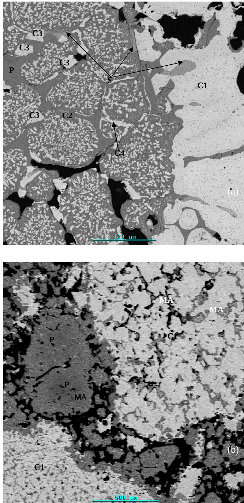
Figure 4.3: SEM-BSE micrographs of unreacted (a) Chrome-Magnesite A showing bright phase= chromite (C1), gray phase = magnesia (periclase P), light-gray phase = silicate (S), black= pores. Intragranular precipitate chromites =C2 and intergranular precipitate chromites = C3 and C4. (b) Chrome-magnesite D50-C5 showing bright phase= chromite (C1), gray phase = magnesia (periclase P), and black= pores.
