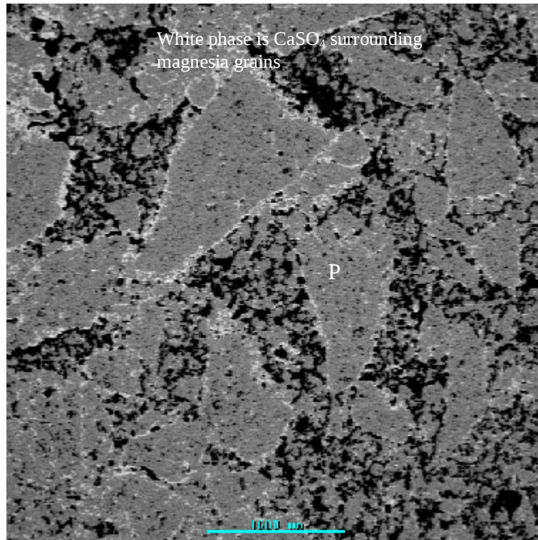
Figure 4.19. SEM-BSE micrograph of the (a) magnesite reacted in \text{SO}_2\text{-O}_2 gas mixture at 1350C, showing calcium sulfate forming at the grain boundaries. The gray phase = magnesia (periclase P), black= pores and white phase = \text{CaSO}_4 .
