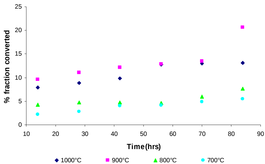
Figure 4.36. Chrome-magnesite D50-C5 conversion fractions in \text{SO}_2\text{-O}_2 gas mixtures at different temperatures as a function of time.
