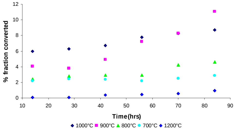
Figure 4.38. Magnesite-chrome D60/100 conversion fractions in \text{SO}_2\text{-O}_2 gas mixtures at different temperatures as a function of time.
