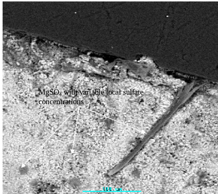
Figure 4.23. SEM-BSE micrographs of (a) laboratory magnesium oxide powdered pellet reacted in \text{SO}_2\text{-N}_2 gas mixtures at 700^\circ\text{C} , showing a collective mass of particles of a continuous spongy sulfate structure. The dark grey phase = magnesium sulfate high in \text{SO}_3 concentration, light grey phase = magnesia sulfate, white precipitates = \text{MgO} , black = pores.
