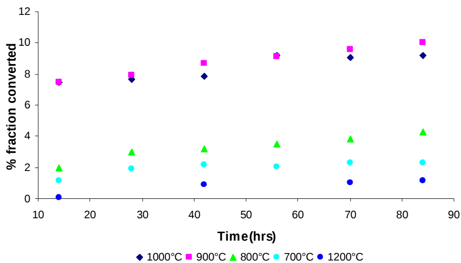
Figure 4.35. Chrome-magnesite A conversion fractions in \text{SO}_2\text{-O}_2 gas mixtures at different temperatures as a function of time.
