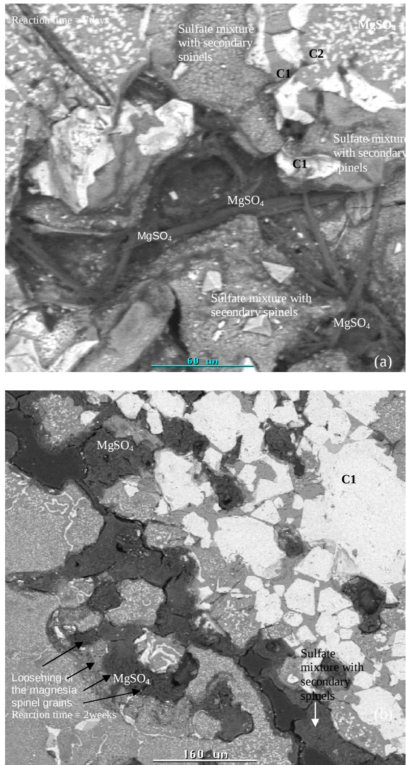
Figure 4.28. SEM-BSE micrographs of chrome-magnesite A refractory reacted in SO 2 -O 2 gas mixture at 700°C where, (a) after 7 days, showing chemical reaction with the magnesia matrix. The dark gray phase = magnesium sulfate, bright phase = chromite (C1), intragranular precipitate chromites = C2. (b) shows reaction after 2 weeks. The bright phase = chromite (C1), gray phase = magnesia sulfate, grey phase with light precipitates = sulfate mixture with secondary spinels.
