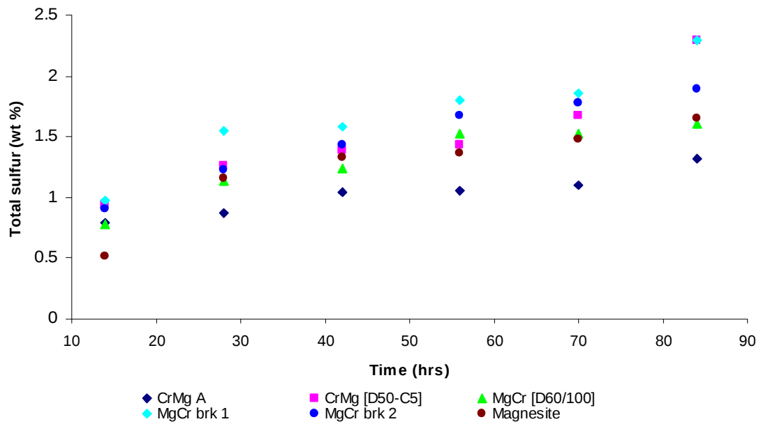
Figure 4.34. Total sulfur (wt %) in basic refractories as a function of time in SO 2 -O 2 mixture at 700°C.
