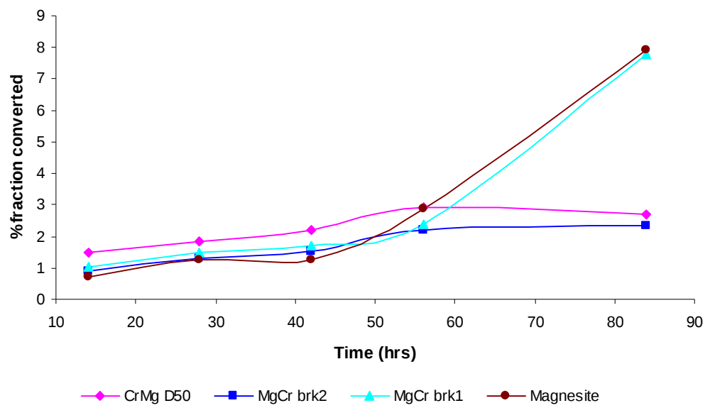
Figure 4.43. Comparison of conversion fractions of basic refractories in \text{SO}_2 gas atmosphere at 800^\circ\text{C} as the function time.
