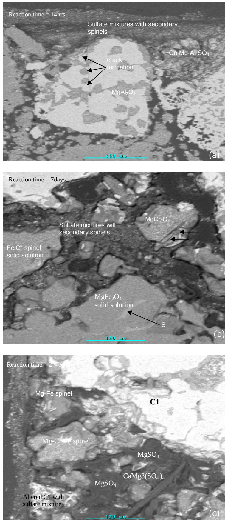
Figure 4.29. SEM-BSE micrographs of chrome-magnesite D50-C5 reacted in SO 2 -O 2 gas mixture at 700°C where, (a) after 14 hrs, showing low gas infiltration and reactions forming at the boundaries, (b) after 7days, showing formation of magnesia spinel solid solutions and high gas infiltration. (c) after 2 weeks, showing elongated sulfate structure and spongy sulfate mixtures with secondary spinels.
