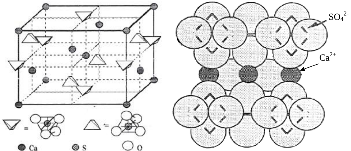
Figure 5.2. The schematic illustration of CaSO 4 crystal structure (a), and CaSO 4 lattice showing the [SO 4 2- ] tetrahedra in light grey and dark grey Ca 2+ cations in-between (Reference, Hasi, Pierre and Raghunathan 98–99 ).
