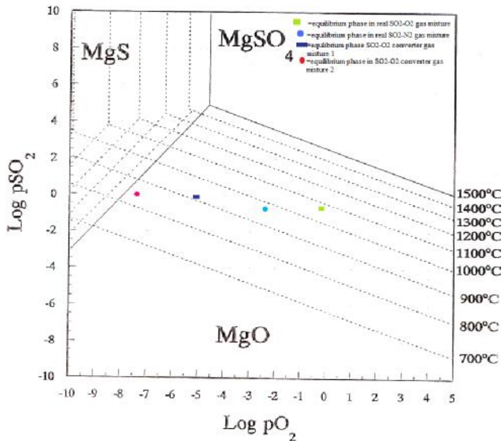
Figure 2.5. Predominance area diagram of magnesium, sulfur and oxygen at varying temperatures, and partial pressure of oxygen and sulfur dioxide (reference, Liouw, Tsikiris and Gray 22 ).
