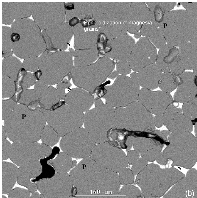
Figure 4.6. SEM-BSE micrographs of (a) Magnesite reacted at 700°C showing uneven texture of magnesia grains with dihedral contact angles. (b) Magnesite reacted at 1350 showing smooth texture of magnesia grains and spheroidization achieved by the magnesia grains at the triple points. The gray phase = magnesia (periclase, P), bright phase = silicate (S) and black = pores.
