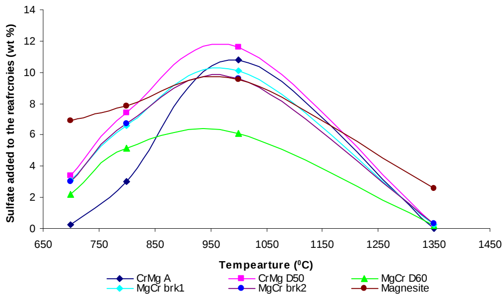
Figure 4.46: Sulfate (wt %) added after 7 days of reaction as a function of temperature at 1atm of \text{SO}_2\text{-O}_2 gas mixture
