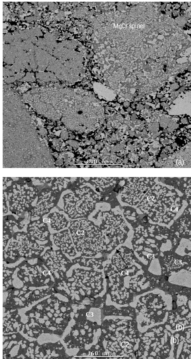
Figure 4.7. SEM-BSE micrographs of (a) Magnesite-chrome D60/100 reacted in O_2 gas at 1350^\circ C , showing distribution of chromite grains and increasing volume of magnesia-chromite spinel at low magnification (b) Magnesite-chrome D60/100 at high magnification, showing angular to subherdal blocky intergranular chromites, continuous intergranular chromites and intragranular chromites. The gray phase = magnesia (periclase P), black = pores, bright phase = intragranular chromites precipitate = C2 and intergranular precipitate chromites = C3 and C4.
