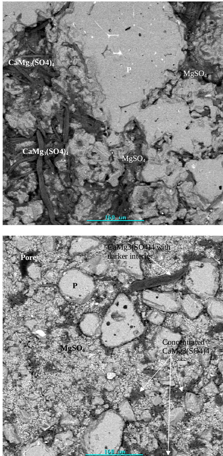
Figure 4.22. SEM-BSE micrographs of (a) magnesite refractory reacted in \text{SO}_2\text{-N}_2 gas mixture at 700^\circ\text{C} , showing magnesium sulfate forming along the grain boundaries. (b) Refractory powdered pellet of magnesite showing heterogeneous reaction of magnesia. The grey phase = magnesium sulfate, light grey phase = magnesia (periclase P), black = pores and bright phase = silicate.
