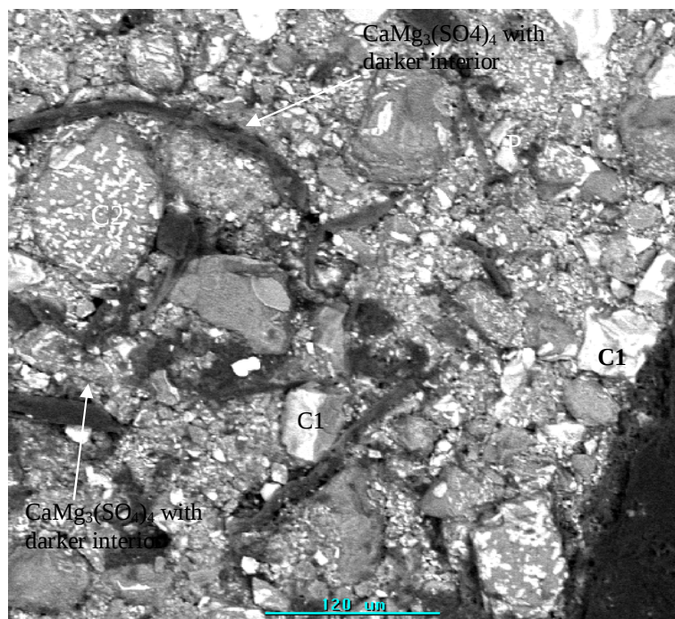
Figure 4.24. SEM-BSE micrographs of (a) Refractory powdered pellet of magnesite-chrome refractory reacted in \text{SO}_2\text{-N}_2 gas mixtures at 700^\circ\text{C} , showing the sulfate phase. The dark grey phase (needles) = calcium magnesium sulfate, black = pores, bright phase = chromite (C1), intragranular precipitate chromites = C2, grey phase = magnesia.
