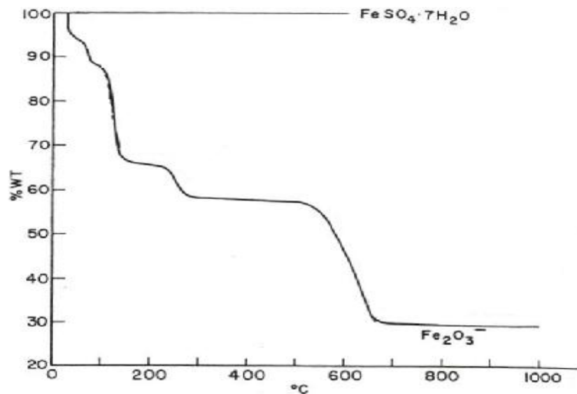
Figure 2.3. Decomposition curves of iron (II) sulfate during heating in nitrogen atmosphere (Reference Gallagher, Johnson and Schrey 81 ).
