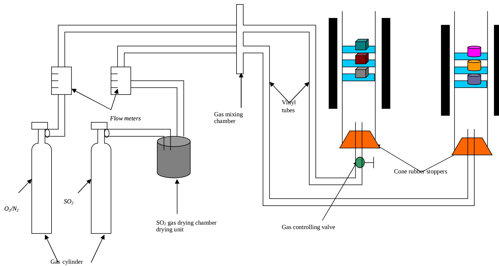
Figure 3.2. Schematic gas flow chart of the gas systems and furnace
