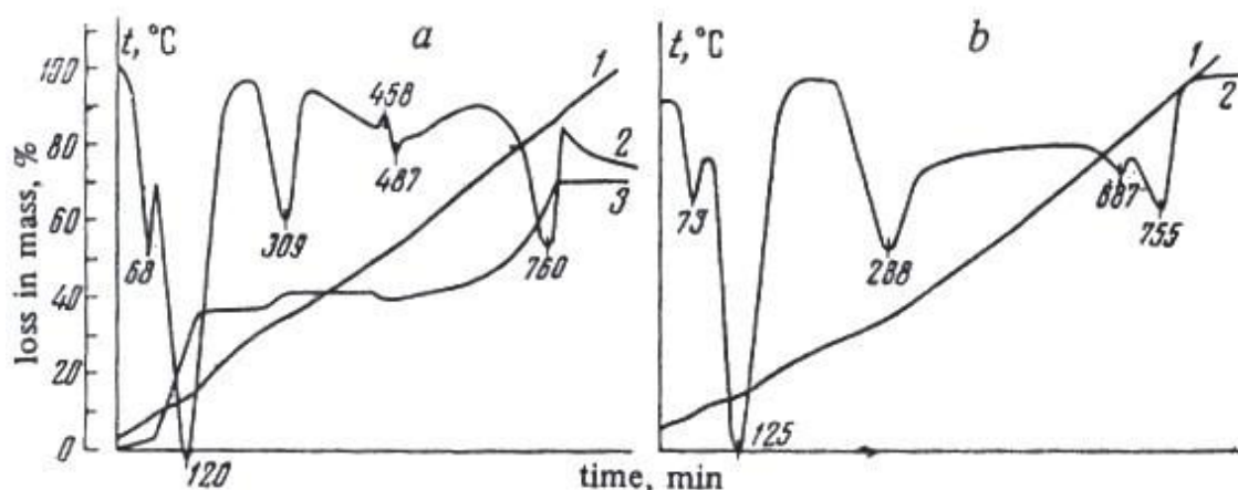
Figure 2.1. Decomposition curves of iron (II) sulfate during heating: (a) in air; (b) in argon atmosphere. 1) temperature record; 2) differential record and 3) loss in mass of specimen (Reference Safiullin, Gitis and Panasenکو 80 ).
