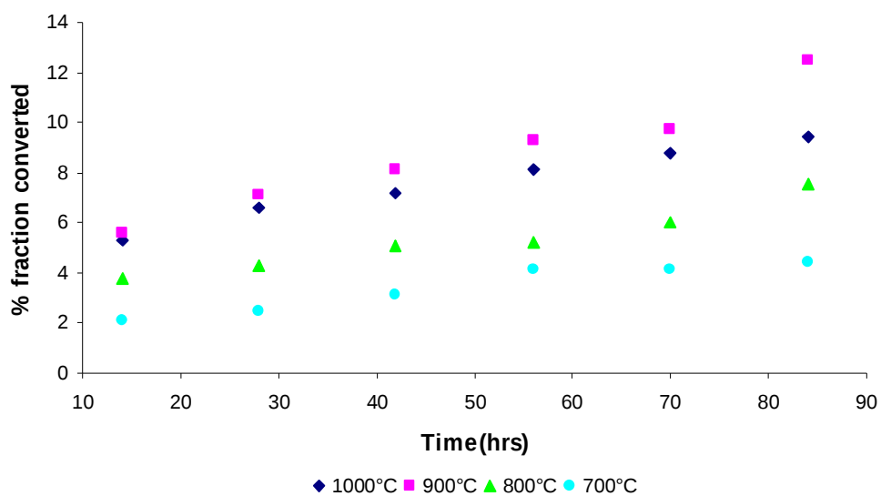
Figure 4.39. Magnesite-chrome brick 2 conversion fractions in \text{SO}_2\text{-O}_2 gas mixtures at different temperatures as a function of time.
