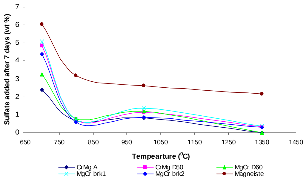
Figure 4.48: Sulfate (wt %) added after 7 days of reaction as a function of temperature at 1atm of \text{SO}_2\text{-N}_2 gas mixture.
