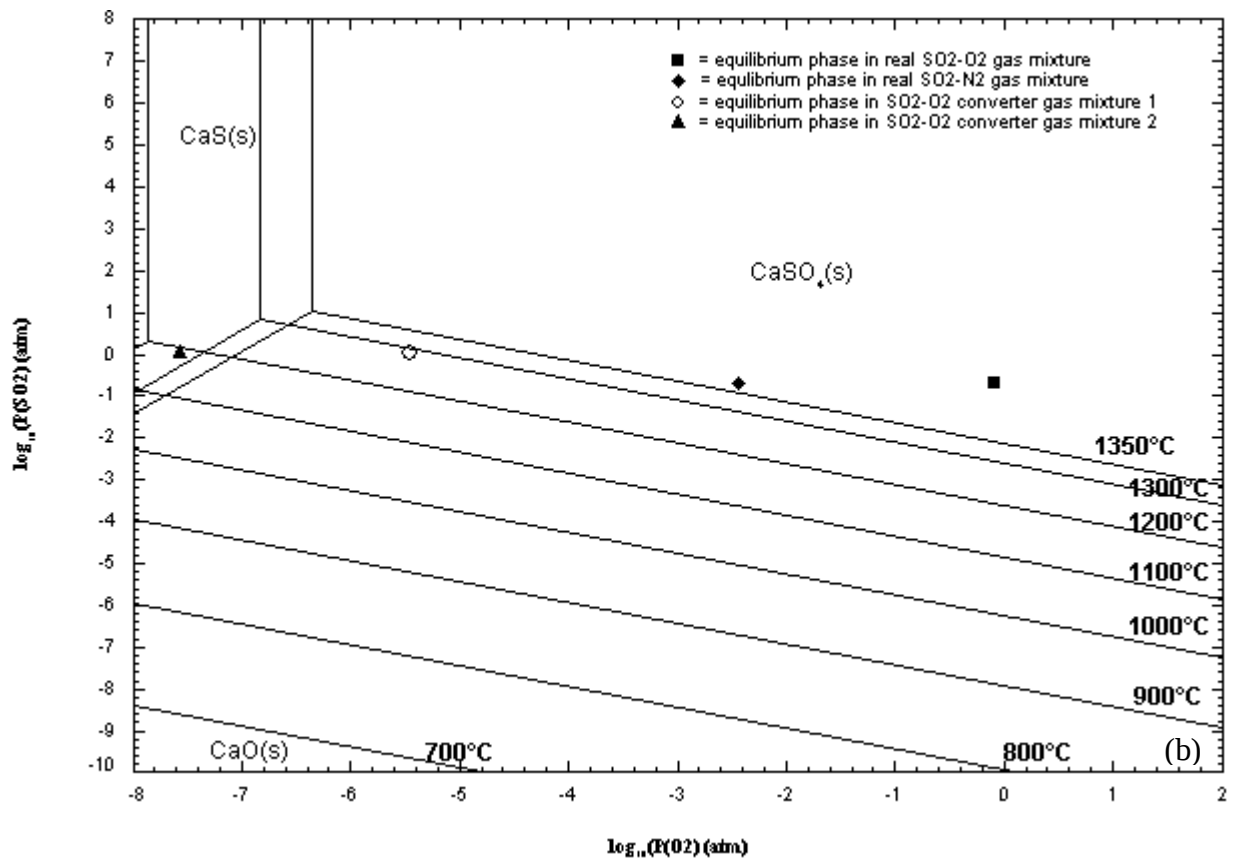
Figure 4.11: Predominance area diagrams for Ca-S-O at 700°C to 1350°C, and varying partial pressures of oxygen and sulfur dioxide using FactSage software programme 121-122 .
