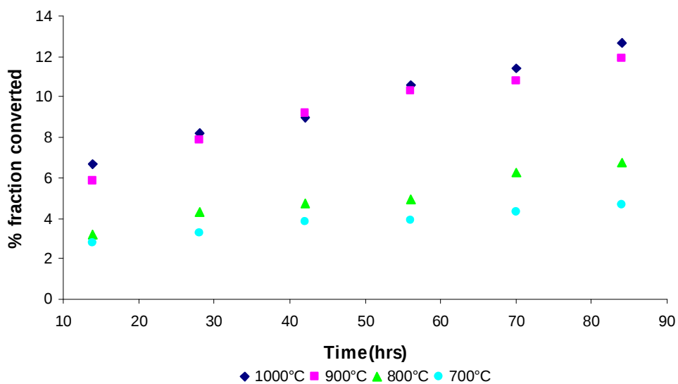
Figure 4.40. Magnesite-chrome brick 1 conversion fractions in \text{SO}_2\text{-O}_2 gas mixtures at different temperatures as a function of time.
