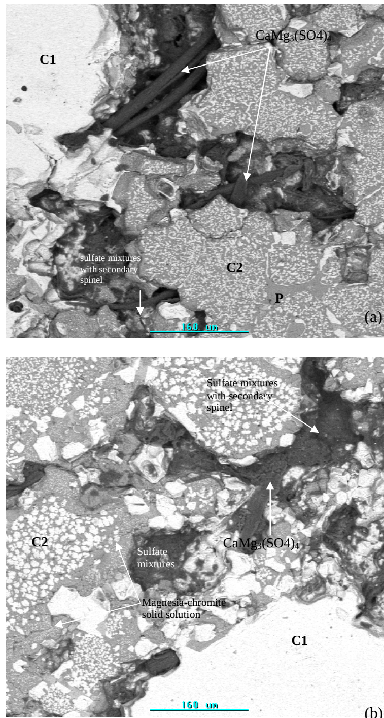
Figure 4.25. SEM-BSE micrographs of (a) magnesite-chrome D60/100 reacted in \text{SO}_2\text{-N}_2 gas mixture at 700^\circ\text{C} , showing reaction of magnesite matrix with sulfur-bearing gases. The gray phase = magnesia (periclase P), bright phase = chromite (C1), intragranular precipitate chromites = C2, black = pores. (b) magnesite-chrome D60/100 showing development of sulfate mixtures with secondary spinels along the magnesite spinel grain boundaries. The bright phase = chromite (C1), gray phase = magnesia (periclase P), black = pores.
