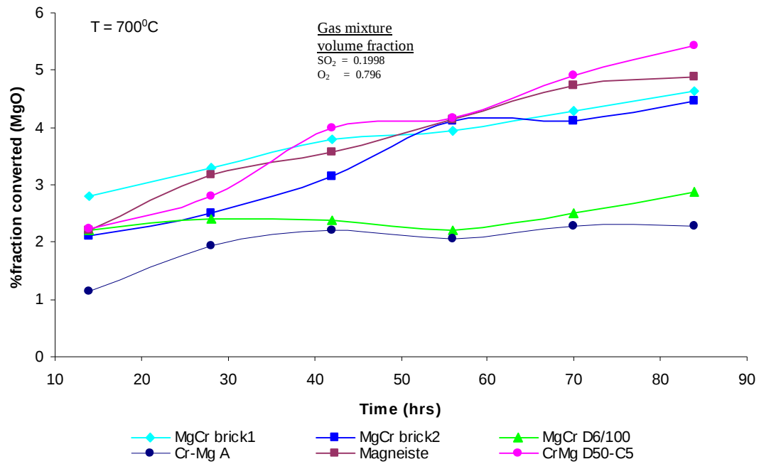
Figure 4.33. Effect of time on sulfation conversions of MgO in basic refractories in SO 2 -O 2 mixture at 700°C.
