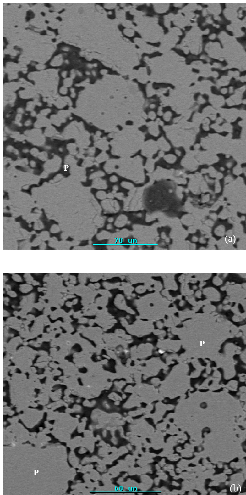
Figure 4.15. SEM-BSE micrographs of (a) laboratory magnesium oxide powdered pellets, reacted in \text{SO}_2\text{-N}_2 gas mixtures at 1350^\circ\text{C} , showing formation of magnesia grains with some direct bonding between grains. (b) Refractory powdered pellet of magnesite showing magnesia grains with a skeletal structure. The gray phase = magnesia (periclase P), black = pores.
