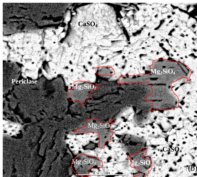
Figure 4.14. SEM-BSE micrographs of (a) Magnesite reacted in \text{SO}_2\text{-N}_2 gas mixture at 1350^\circ\text{C} , showing formation of calcium sulfate at grain boundaries. (b) Magnesite showing formation of silicate and intragranular porosity. The gray phase = magnesia (periclase P), light-gray phase = silicate (S), black = pores and white phase = \text{CaSO}_4
