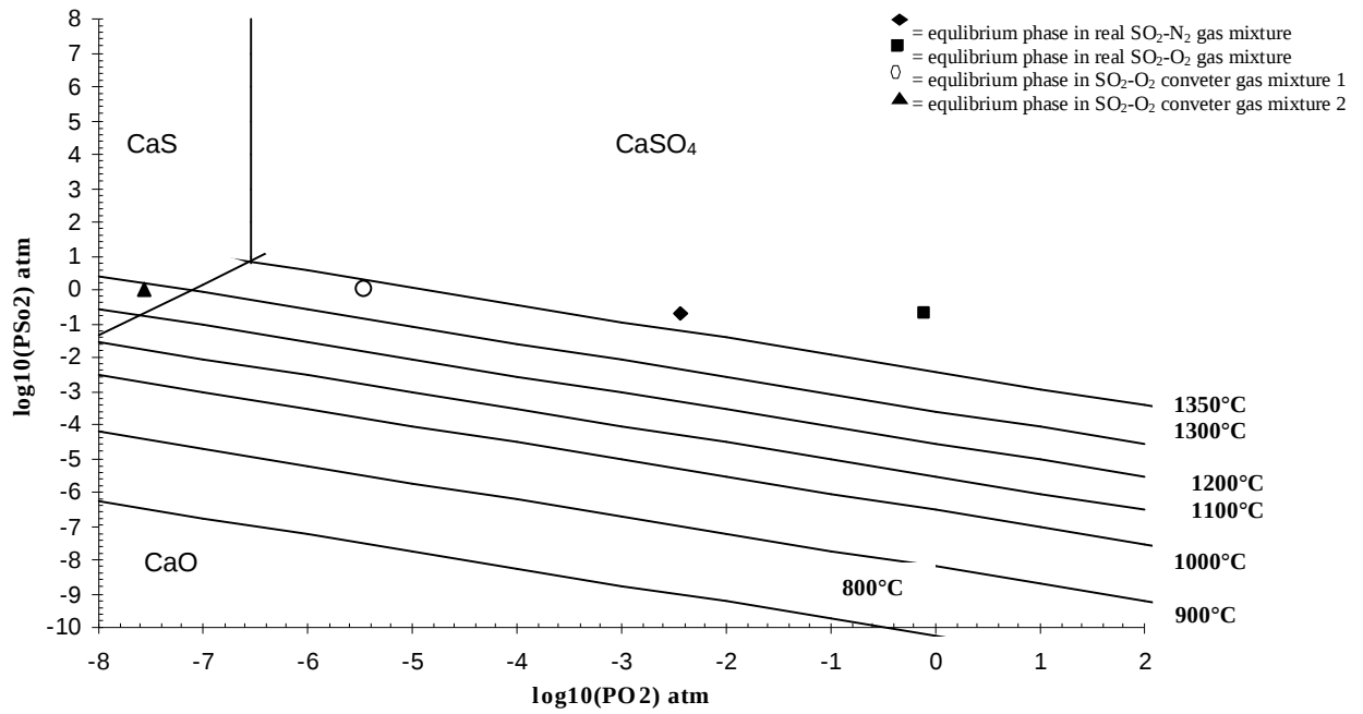
Figure 4.10: Predominance area diagrams for Ca-S-O at 1350°C, and varying partial pressures of oxygen and sulfur dioxide using Kellogg 79 and Richardson and Jeffes 113 data.
