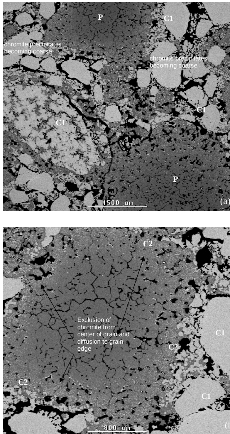
Figure 4.8. SEM-BSE micrographs of (a) Chrome-magnesite A reacted in O_2 gas at 1350^\circ C , showing development and migration of secondary chromites at low magnification (b) Chrome-magnesite A showing magnesia grain with intragranular secondary chromites along the grain boundaries, cracks and high purity interior. Coarse secondary chromites are shown as bright phase= chromite (C1). The gray phase = magnesia (periclase P), black= pores, within magnesia grains borders the bright phase = intragranular chromites precipitate =C2.
