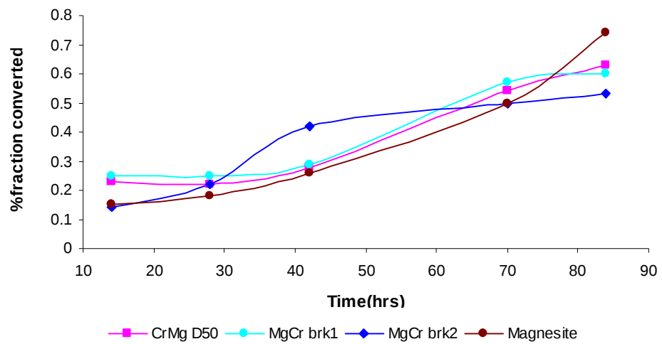
Figure 4.41. Comparison of conversion fractions of basic refractories in \text{SO}_2\text{-N}_2 gas mixtures at 800°C as a function of time.
