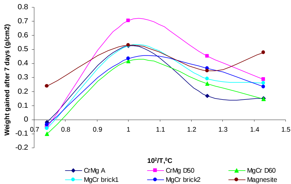
Figure 4.45: The weight gain after 7 days of reaction as a function of the reciprocal absolute temperature at 1atm of \text{SO}_2\text{-O}_2 gas mixture.
