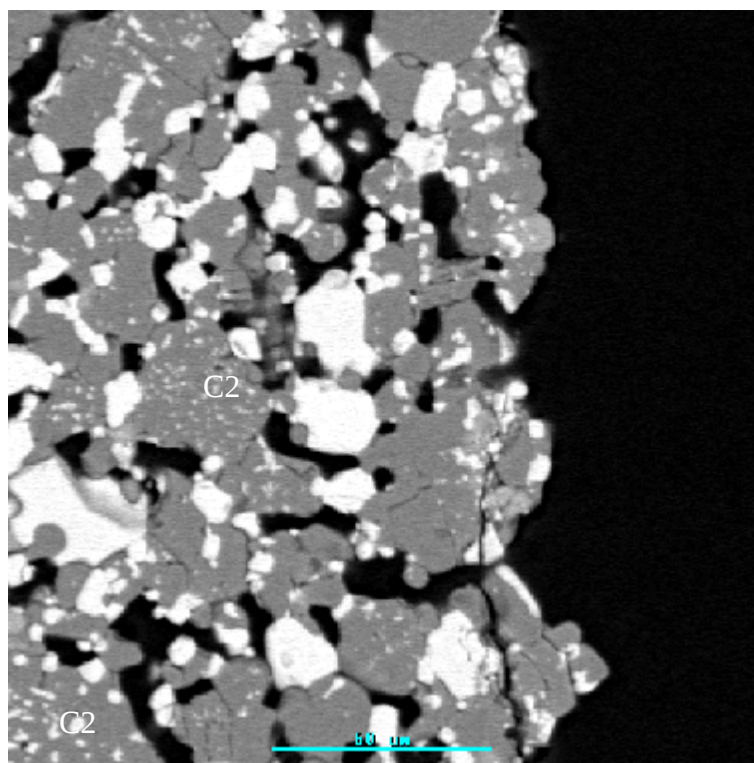
Figure 4.16. SEM-BSE micrograph of a refractory powdered pellet of magnesite-chrome reacted in \text{SO}_2\text{-N}_2 gas mixtures at 1350^\circ\text{C} , showing magnesia-chromite contacts and magnesia spinels. The gray phase = magnesia (periclase P), black= pores, bright phase = chromite and intragranular chromites precipitate =C2.
