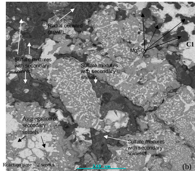
Figure 4.31. SEM-BSE micrographs of magnesite-chrome brick 2 reacted in \text{SO}_2\text{-O}_2 gas mixture at 700^\circ\text{C} , (a) after 7 days, showing reaction of magnesia matrix with gases forming sulfates. The disintegrated dark gray phase = magnesia sulfate, bright phase = chromite (C1), intragranular precipitate chromites = C2, black = pores, (b) after 2 weeks, showing dissolution of magnesia-chromite spinels and crack formation, development of sulfate mixtures with secondary spinels along the magnesia spinel grain boundaries. The bright phase = chromite (C1), gray phase = magnesia sulfate, grey phase with light precipitates = sulfate mixture with secondary spinels, and black = pores.
