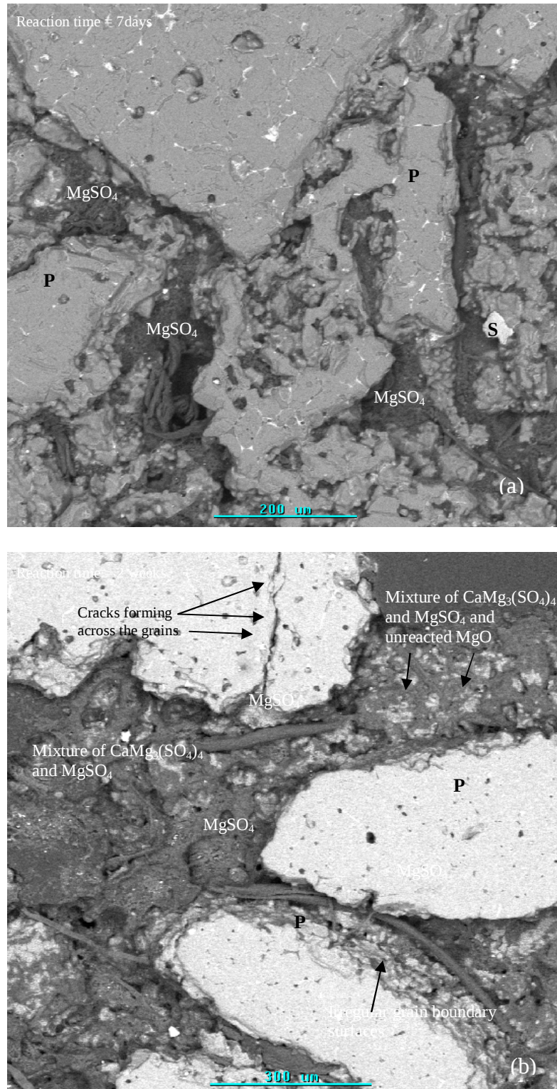
Figure 4.27. SEM-BSE micrographs of magnesite refractory reacted in \text{SO}_2\text{-O}_2 gas mixture at 700^\circ\text{C} where, (a) after 7 days, showing chemical reaction with the magnesia grains, The dark grey phase between grains = magnesium sulfate ( \text{MgSO}_4 ), grey phase = magnesia ( \text{P} ), light grey phase = Silicates ( \text{S} ), (b) shows reaction after 2 weeks, showing crack formation, The dark grey phase along grains (needles) = concentrated magnesium sulfate, dark grey porous phase = magnesium sulfate, light grey porous phase = calcium magnesium sulfate ( \text{CaMg}_3(\text{SO}_4)_4 ).
