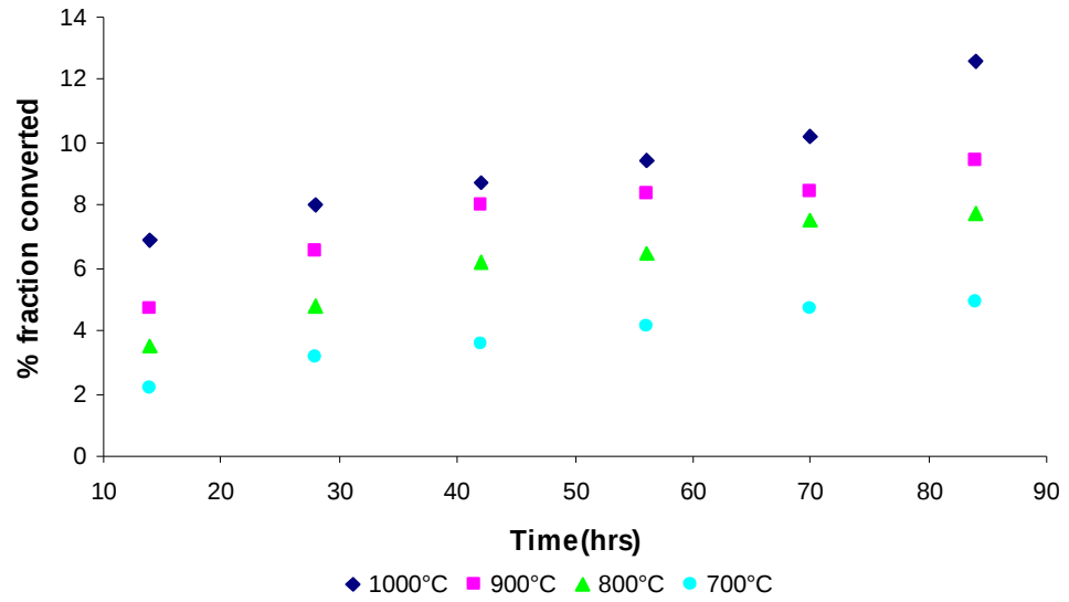
Figure 4.37. Magnesite conversion fractions in \text{SO}_2\text{-O}_2 gas mixtures at different temperatures as a function of time.
