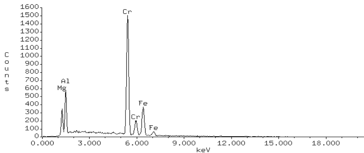
Figure 4.5. EDX spectra of forsterite (a), monticellite (b) and chromite (c) phase showing the elements contained in the minerals.
