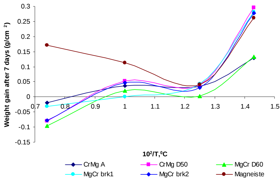
Figure 4.47: The weight gain after 7 days of reaction as a function of the reciprocal absolute temperature at 1atm of \text{SO}_2\text{-N}_2 gas mixture.
