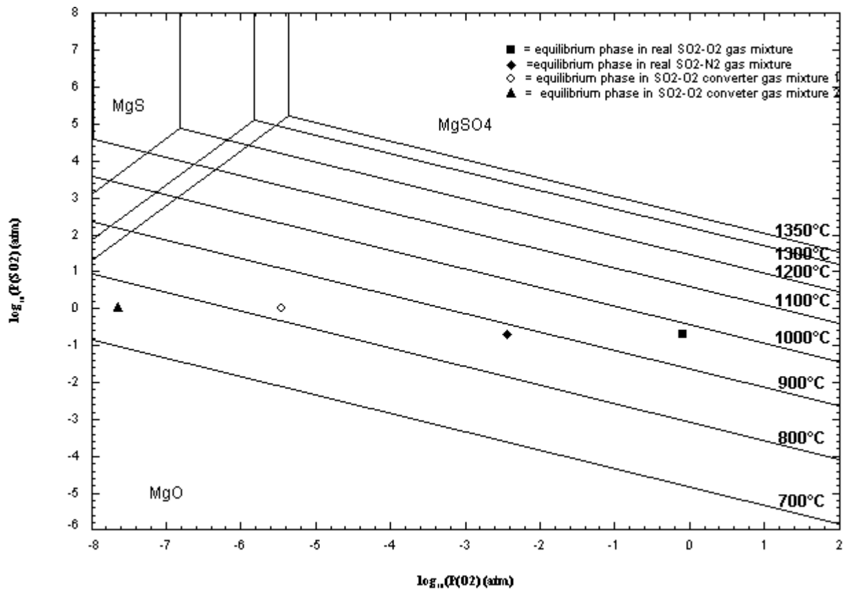
Figure 4.13: Predominance area diagrams of Mg-S-O between 700°C to 1350°, and varying partial pressures of oxygen and sulfur dioxide, using FactSage software 121-122 .
