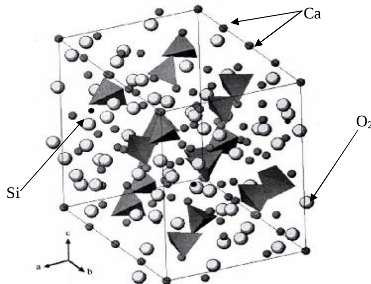
Figure 5.1. The schematic illustration of \text{Ca}_3\text{SiO}_5 , showing [\text{SiO}_4] tetrahedral in dark grey. The Ca, O and Si atoms are presented by the rounded spheres in dark grey, light grey and black, respectively. (Reference: Mori et al. 124 ).
