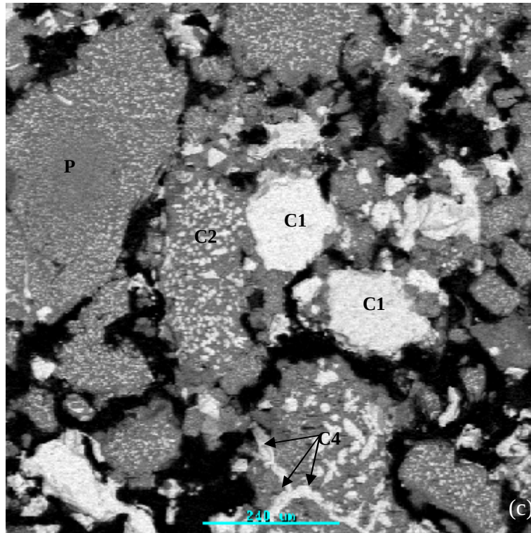
Figure 4.2. SEM-BSE micrograph of unreacted Magnesite-chrome brick 1 showing bright phase= chromite (C1), gray phase = magnesia (periclase P), black= pores. Intragranular precipitate chromites =C2 and precipitate continuous chromites =C4.
