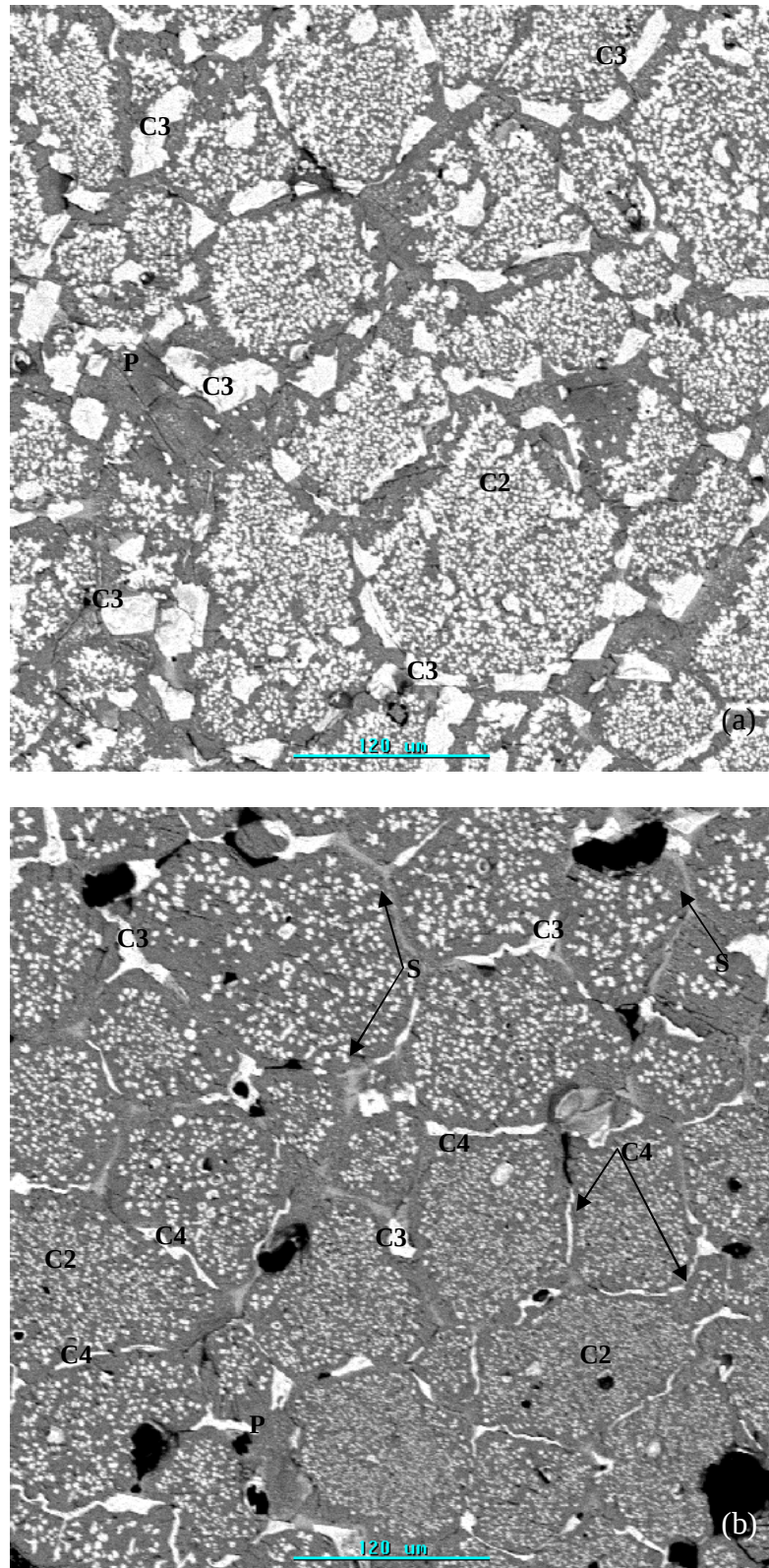
Figure 4.4. SEM-BSE micrographs of unreacted (a) Magnesite-chrome D60/100 showing gray phase = magnesia (periclase P), intragranular precipitate chromites =C2 and intergranular precipitate, blocky chromites = C3 and continuous chromites C4. (b) Magnesite-chrome brick 2 showing gray phase = magnesia (periclase P), black= pores, light-gray phase = silicate (S) and intragranular precipitate chromites =C2 and intergranular precipitate continuous chromites =C4.
