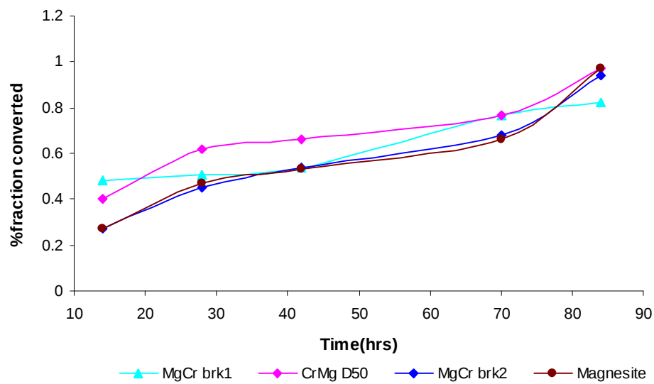
Figure 4.42. Comparison of conversion fractions of basic refractories in \text{SO}_2\text{-N}_2 gas mixtures at 1000°C as the function time.
