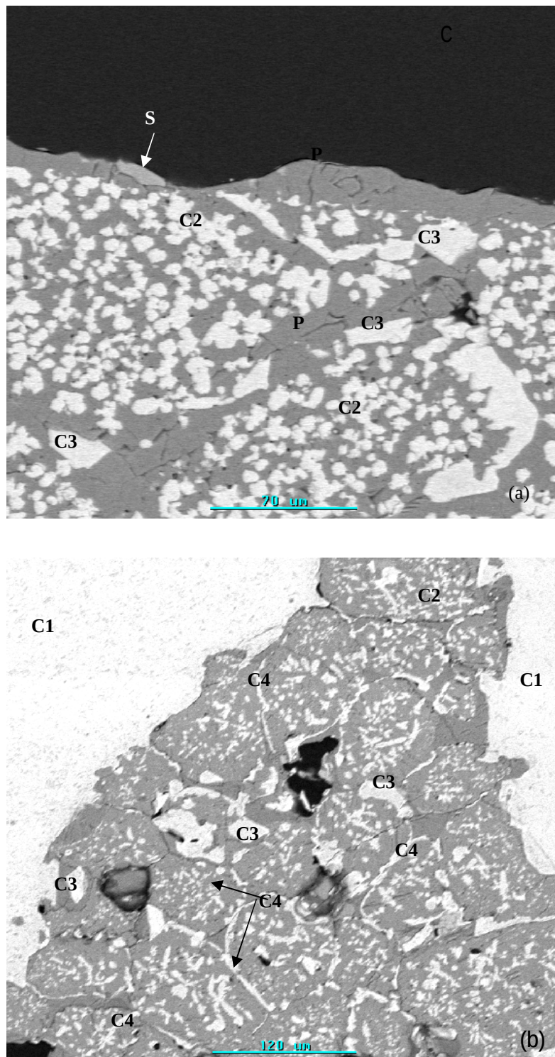
Figure 4.17. SEM-BSE micrographs of (a) Magnesite-chrome D60/100 reacted in \text{SO}_2\text{-N}_2 gas mixture at 1350, showing gray phase = magnesia (periclase P), light-gray phase = silicate (S), black = pores. Intragranular precipitate chromites = C2 and intergranular precipitate chromites = C3. (b) Chrome-magnesite A showing bright phase = chromite (C1), intragranular chromites precipitate = C2 and intergranular precipitate chromites = C3 and C4, gray phase = magnesia (periclase P), black = pores.
