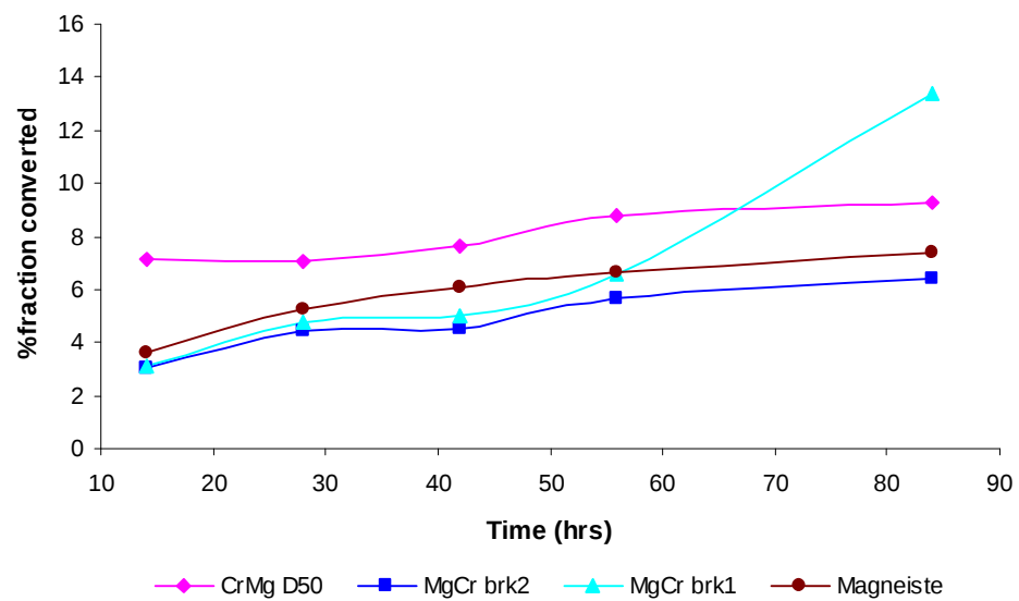
Figure 4.44. Comparison of conversion fractions of basic refractories in \text{SO}_2 gas atmosphere at 1000^\circ\text{C} as the function time.
