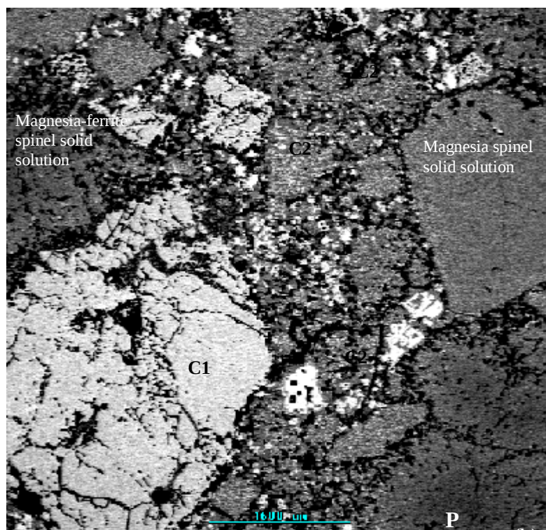
Figure 4.21. SEM-BSE micrographs of (a) magnesite-chrome D60/100 reacted in \text{SO}_2\text{-O}_2 gas mixture at 1350C, showing formation of magnesia-chromite solid solutions. The gray phase = magnesia (periclase P), bright phase = chromite (C1), (C1), intragranular precipitate chromites = C2, black= pores. (b) magnesite-chrome brick 2 showing disintegration of chromite grains and dissolution of chromite precipitates. The bright phase= chromite (C1), gray phase = magnesia (periclase P), black= pores.
