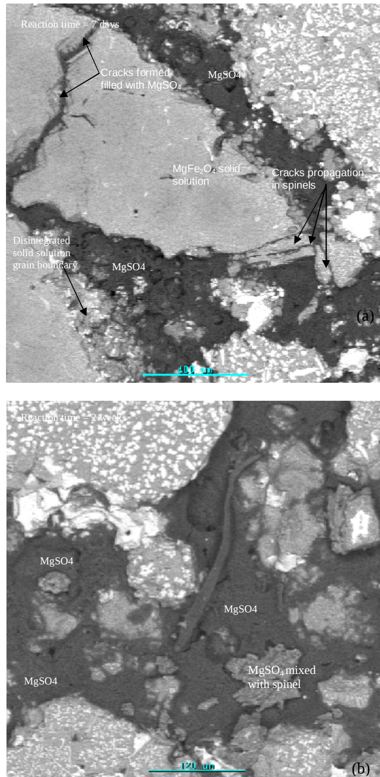
Figure 4.32. SEM-BSE micrographs of magnesite-chrome brick 1 reacted in \text{SO}_2\text{-O}_2 gas mixture at 700^\circ\text{C} where, (a) after 7 days, showing crack formation and dissolution of spinels. (b) after 2 weeks, showing disintegration and sulfation \text{MgFe}_2\text{O}_4 spinels.
