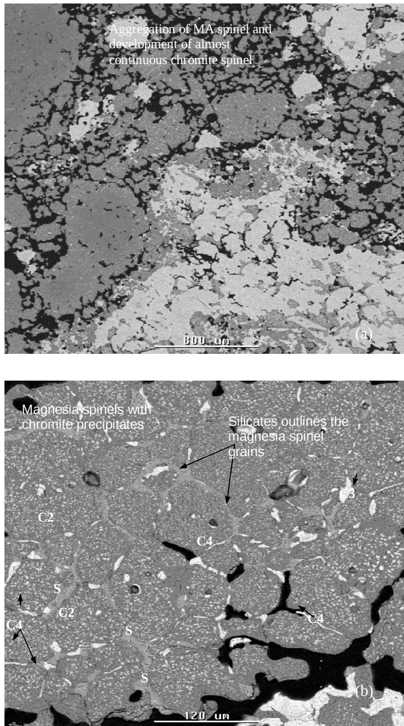
Figure 4.9. SEM-BSE micrographs of (a) Chrome-magnesite D50-C5 reacted in \text{O}_2 gas at 1350^\circ\text{C} , showing dissolution of primary chromite grains and aggregation of magnesium aluminates spinels. (b) Chrome-magnesite D50-C5 showing intragranular secondary chromite precipitates and intergranular silicates between magnesia-chrome spinels. The gray phase = magnesia (periclase P), light-gray phase = silicate (S), black = pores, bright phase = intragranular chromites precipitate = C2 and intergranular precipitate chromites = C3 and C4.
