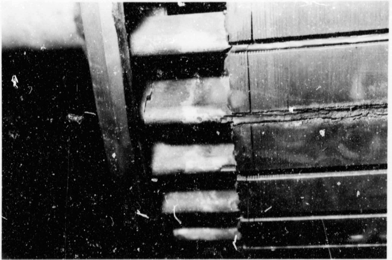
ROTOR BAR DEFECTS IN INDUCTION MOTORS
