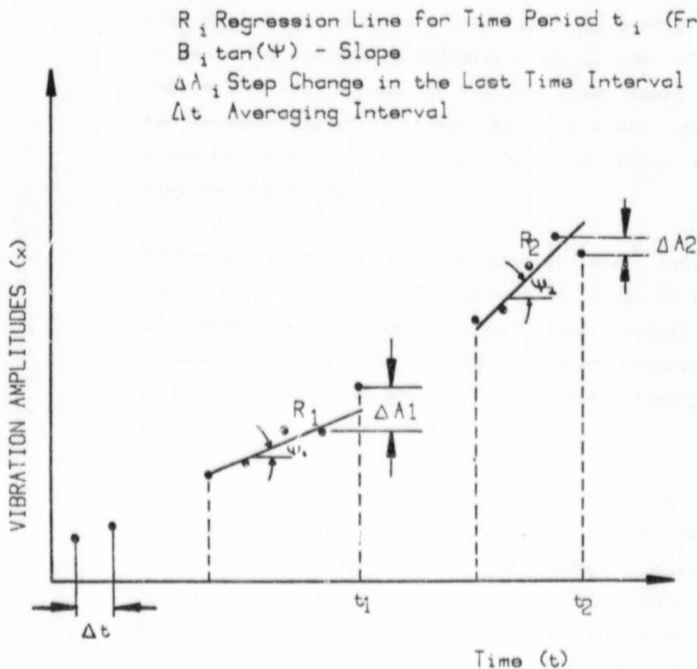
SCHEMATIC REPRESENTATION OF THE CRACK-INDICATING CRITERIA FOR A TURBINE-GENERATOR FIGURE 6.12
