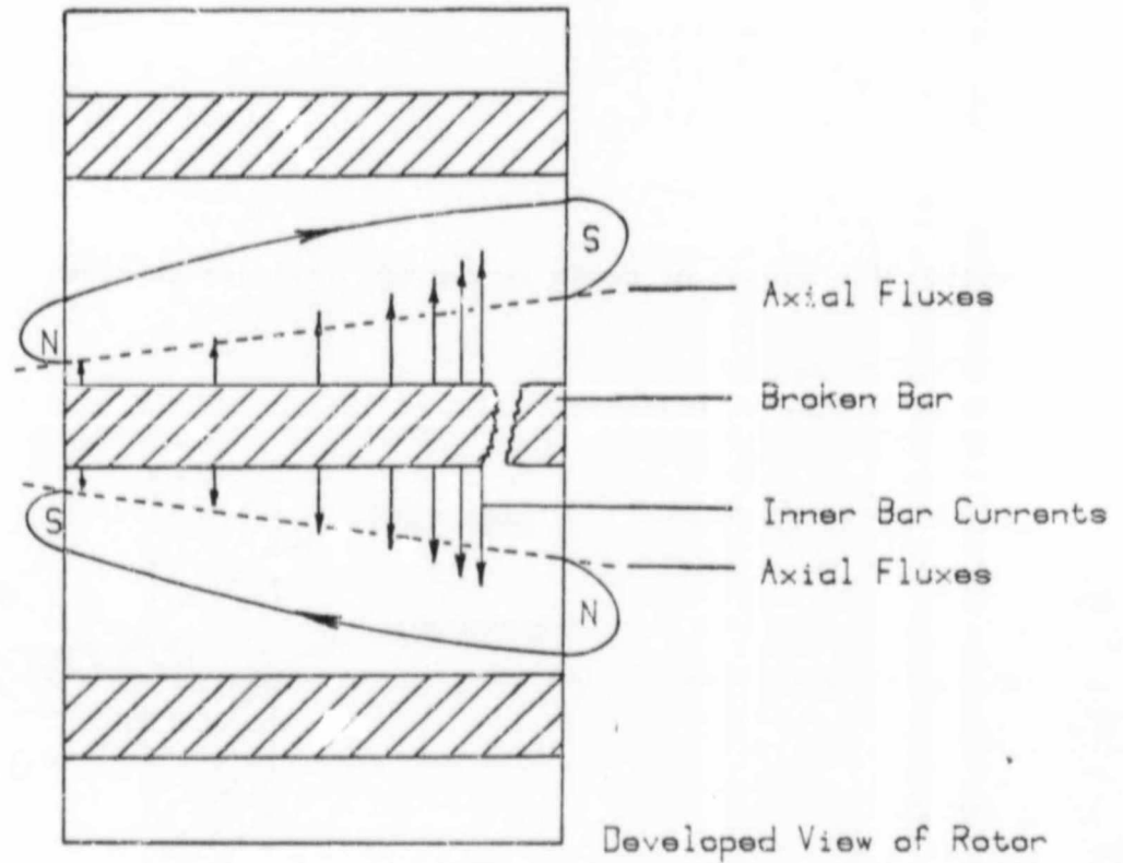
AXIAL FLUXES PRODUCED BY INNER-BAR CURRENTS
