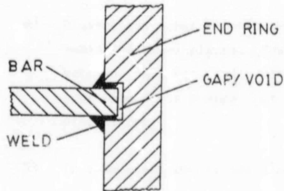
BAR AND END RING WELD
