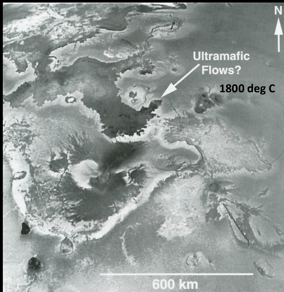
Volcanic eruptions on the moon of Jupiter – Io Compositions of the Comondale komatiite type (High silica and high Mg) Williams, Wilson, Greely (2000) - Journal of Geophysical Research
