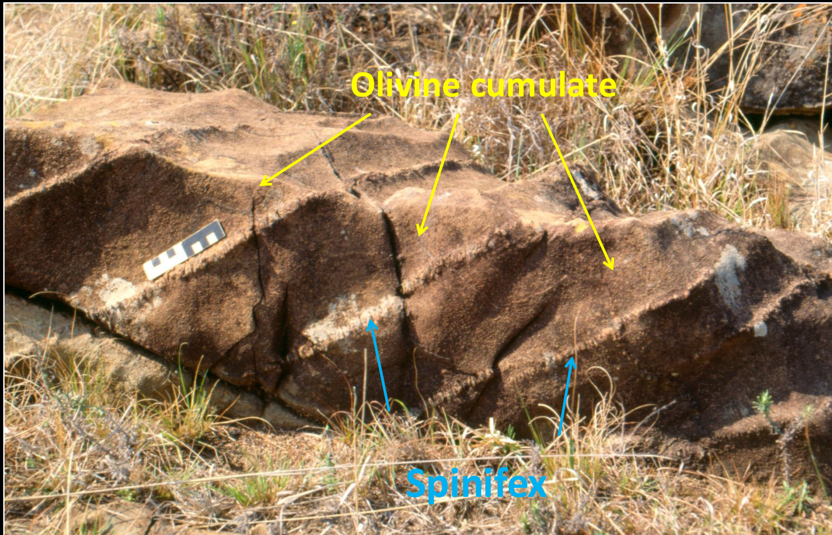
Regular layered spinifex in the Comondale Ultramafic Suite
