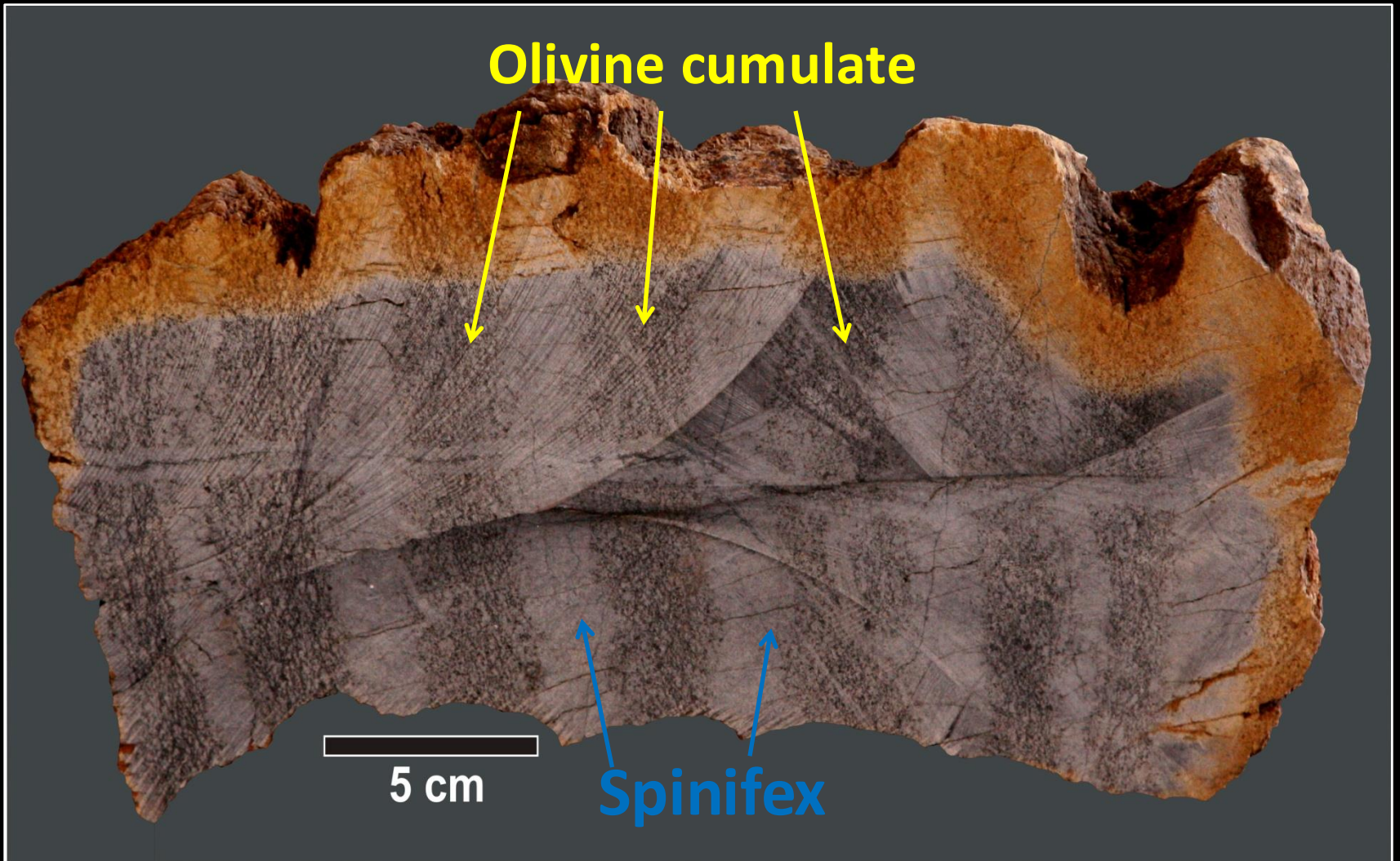
Regular layered spinifex in the Comondale Ultramafic Suite
