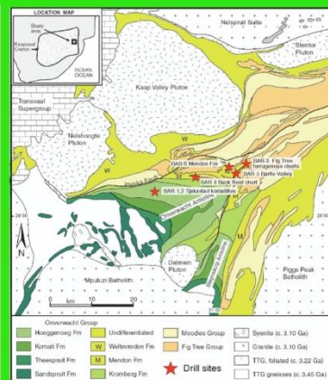
Geological map with drilling sites and stratigraphy of the Barberton Belt.
