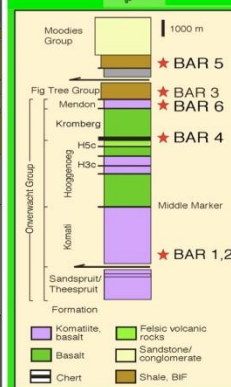
Geological map with drilling sites and stratigraphy of the Barberton Belt.
