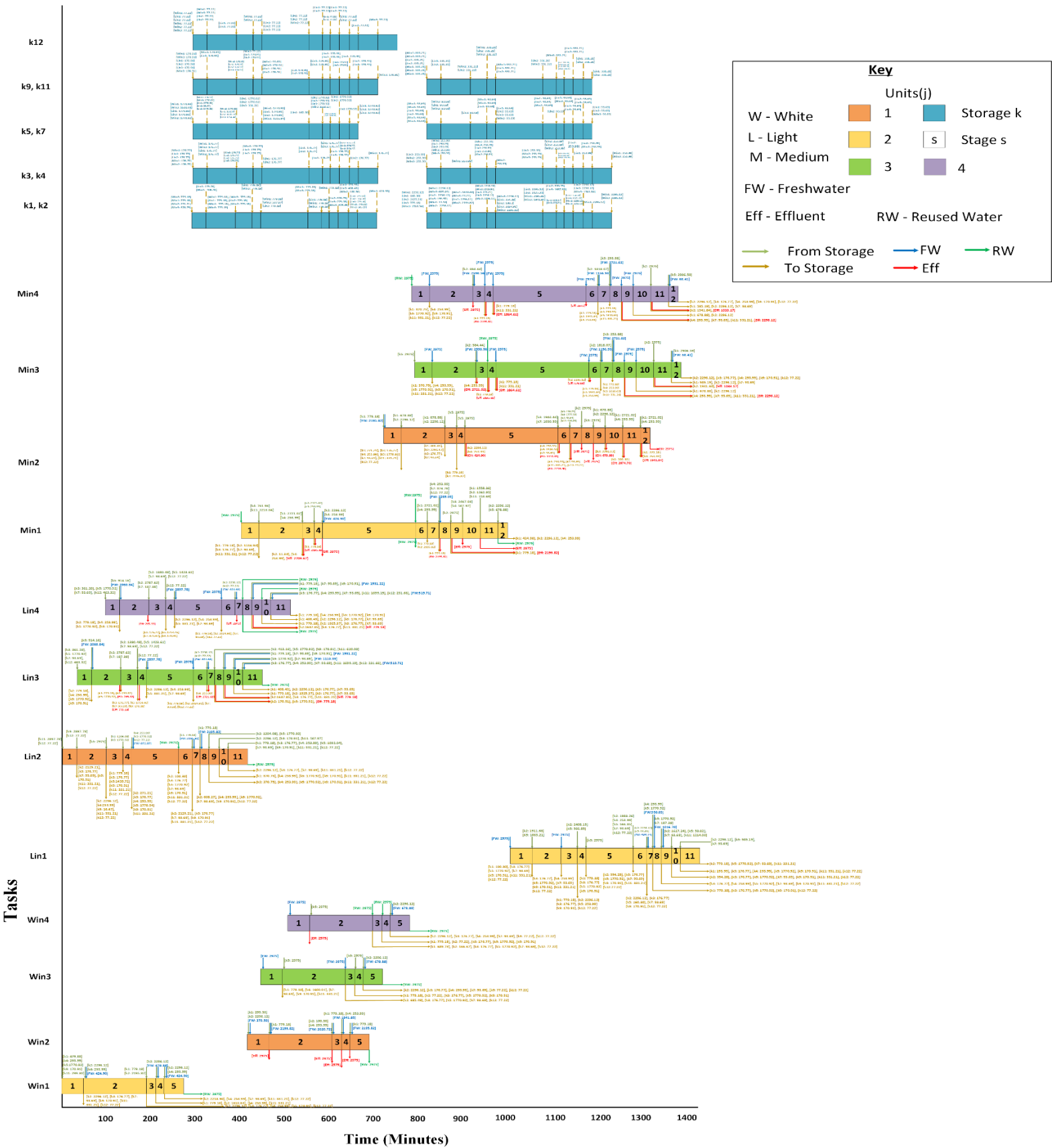
Figure 4.6. Gantt chart for Scenario B with storage tank
