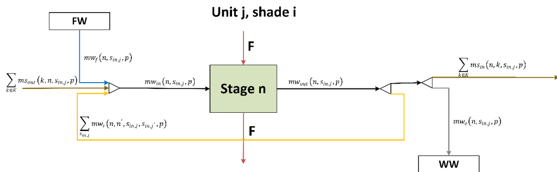
Figure 3.3. Water Network around unit j , shade i
