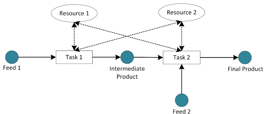
Figure 2.3. Resource Task Network representation
