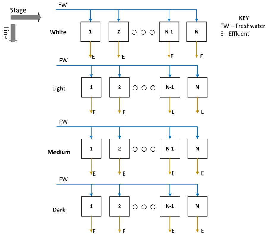
Figure 1.2. Schematic layout showing water motion through a textile plant
