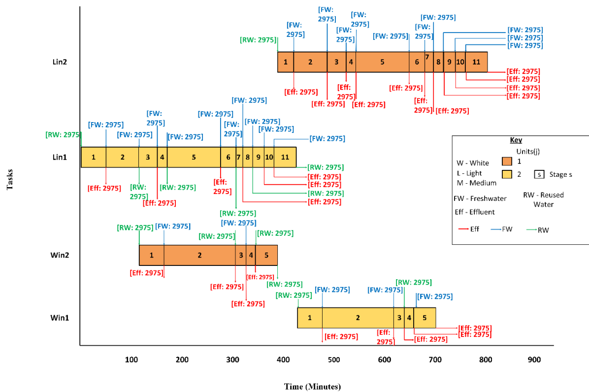
Figure 4.3. Gantt chart for Scenario A without storage tanks
