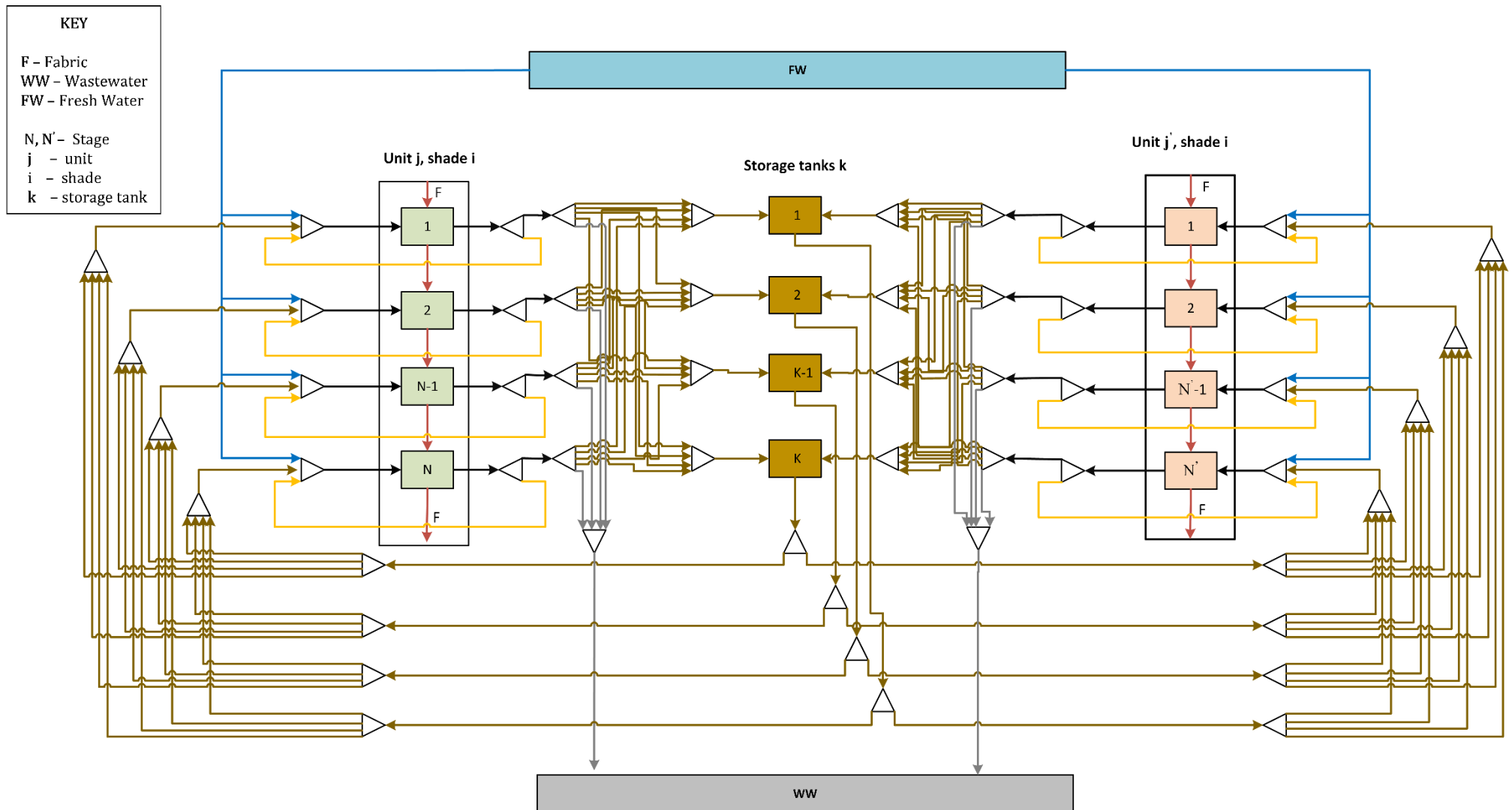
Figure 3.1. General superstructure representation of the water network
