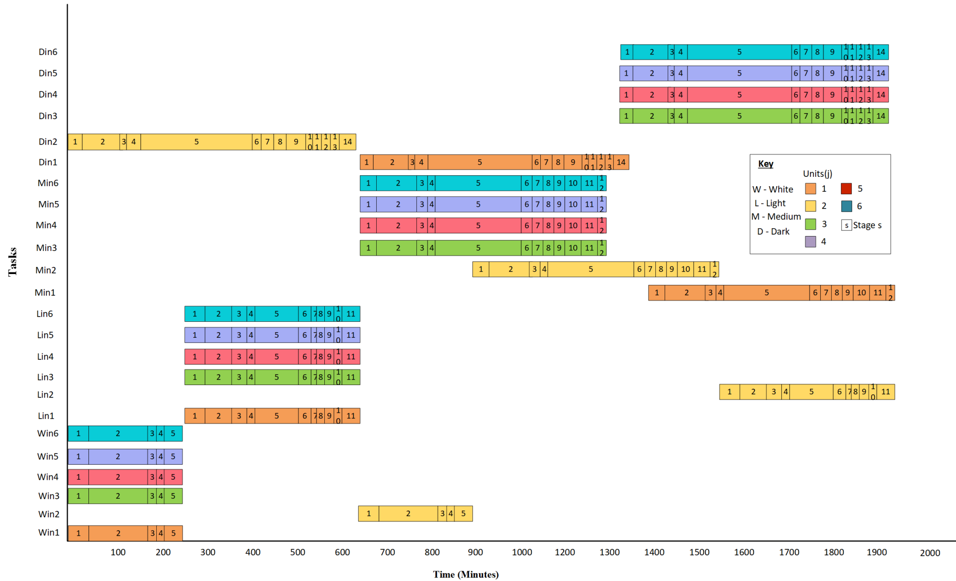
Figure 4.2. Optimal Production Schedule before water integration
