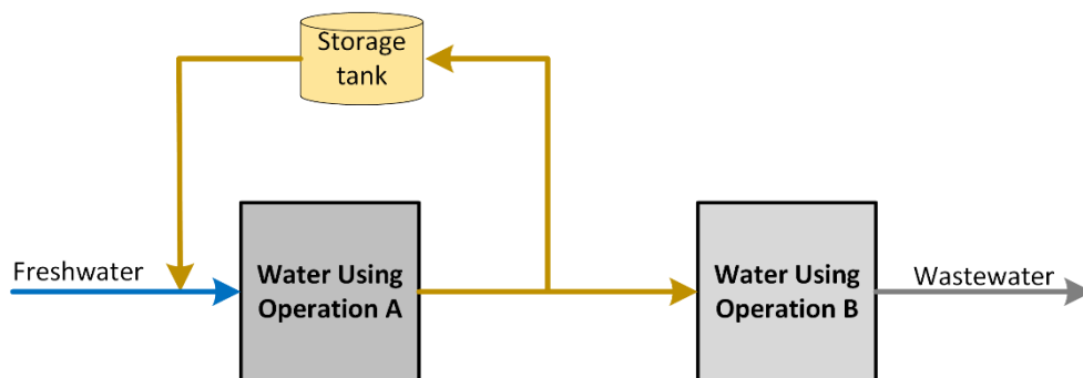
Figure 2.11. Indirect reuse/recycle of water from operation A to B
