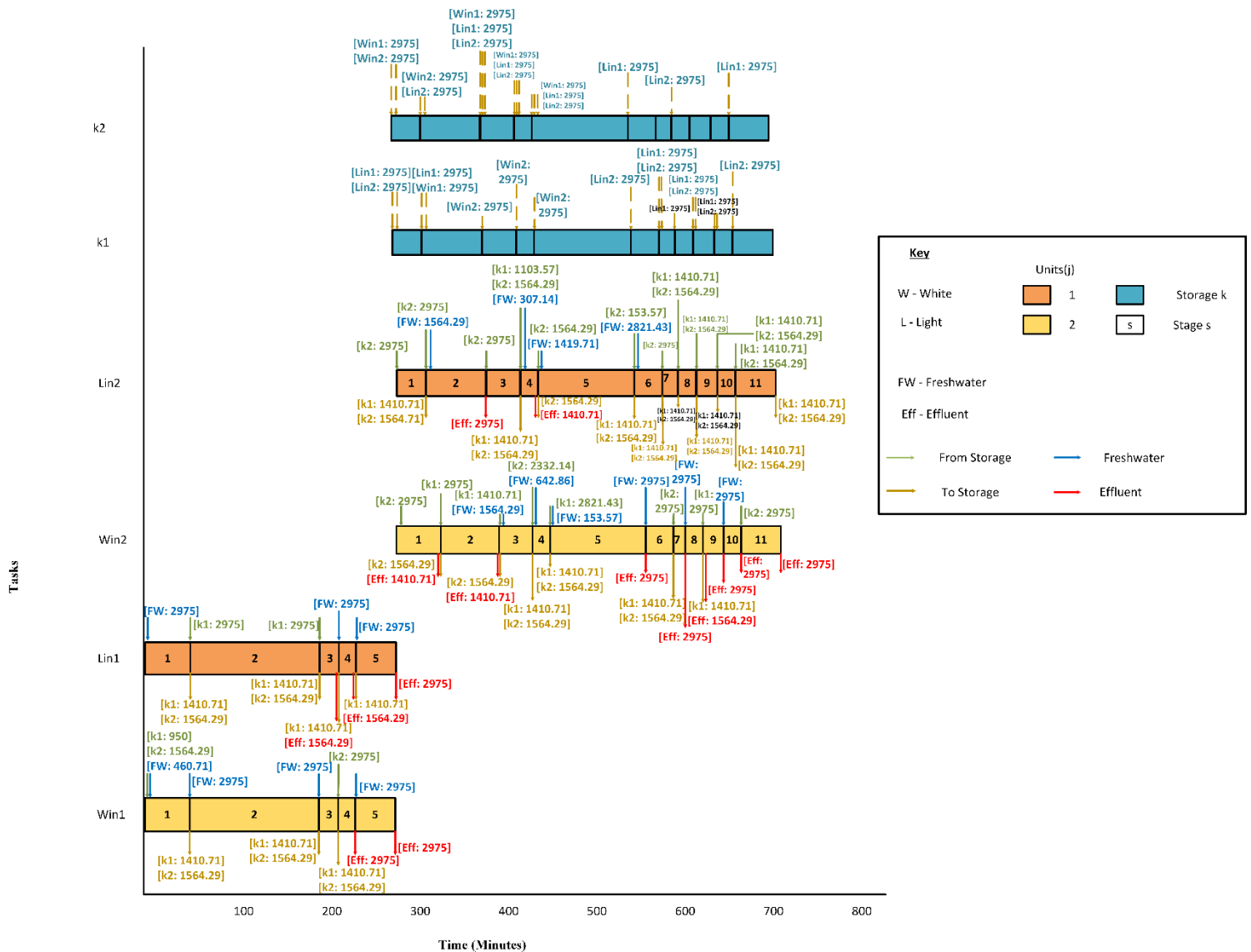
Figure 4.4. Gantt chart for Scenario A with storage tanks
