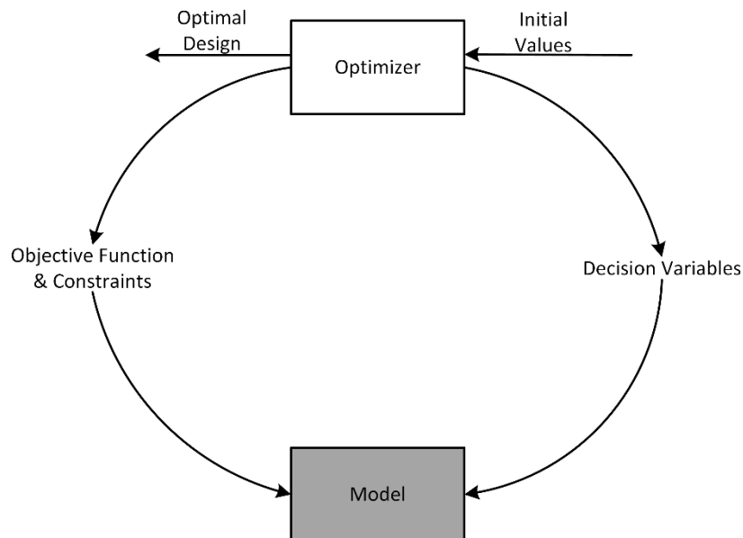
Figure 2.13. An illustration of the numerical optimization framework (Diwekar, 2020)
