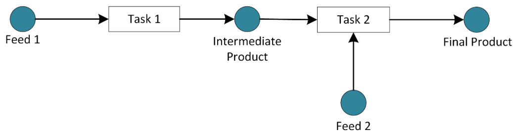
Figure 2.2. State Task Network representation
