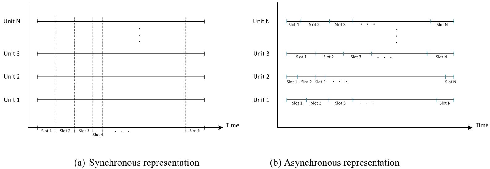
Figure 2.6. Slot-based representation
