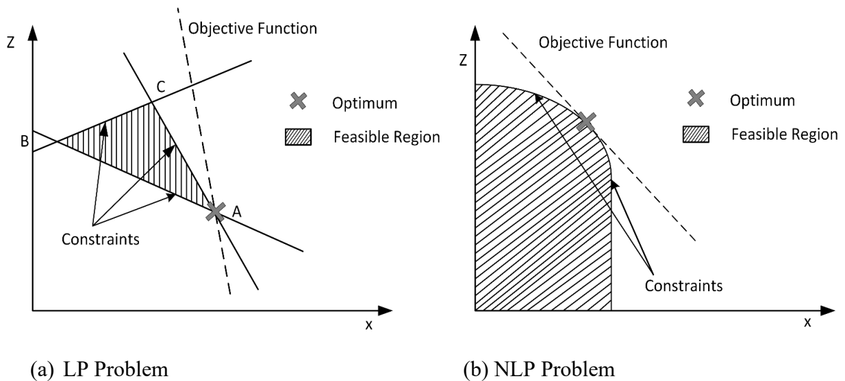
Figure 2.14. Linear and nonlinear programming problems (Diwekar, 2020)
