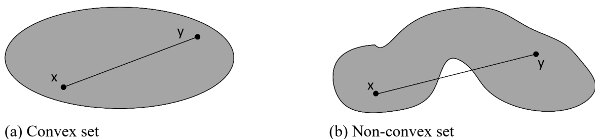
Figure 2.15. Illustration of convex and non-convex sets (Williams, 2013; Diwekar, 2020)
