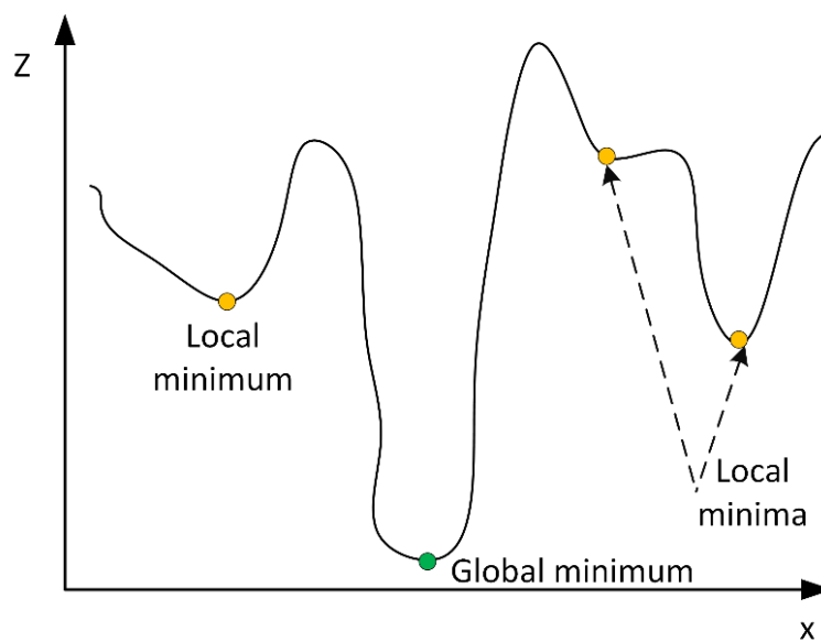
Figure 2.16. Local optima and global optimal solution in non-convex NLP problems
