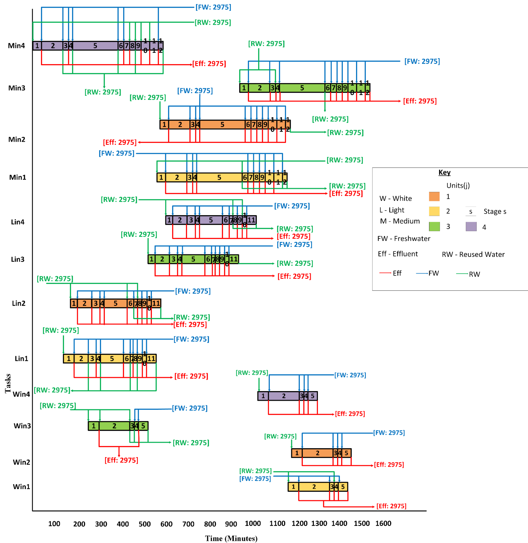
Figure 4.5. Gantt chart for Scenario B without storage tanks
