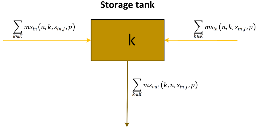
Figure 3.4. Water network around the storage tanks
