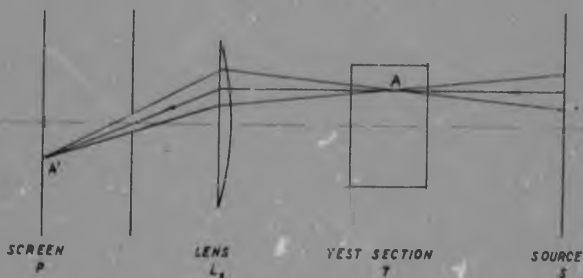
NON-PARALLEL LIGHT EFFECTS FIG. 9
