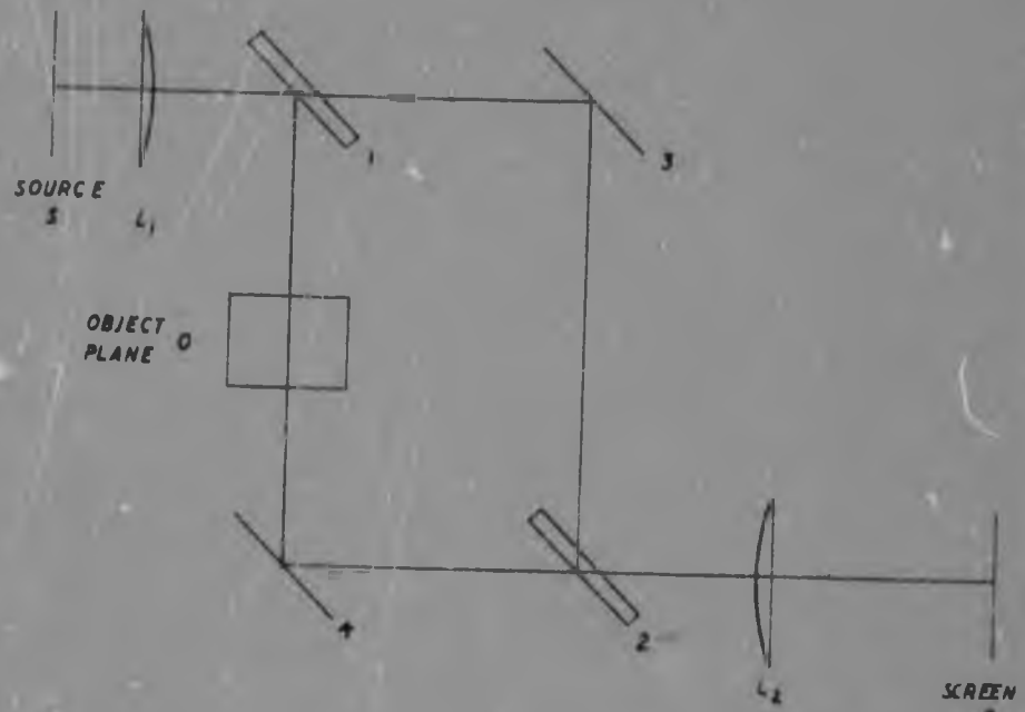
ELEMENTS OF THE INTERFEROMETER FIG. 4
