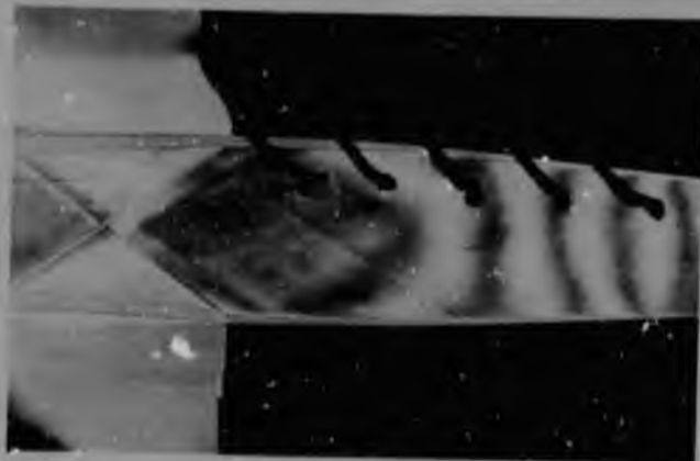
Fig. 24 Infinite Fringes.
