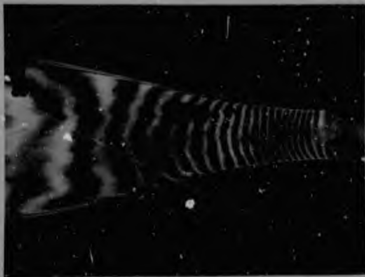
Fig. 40 42 Throat density contours.
