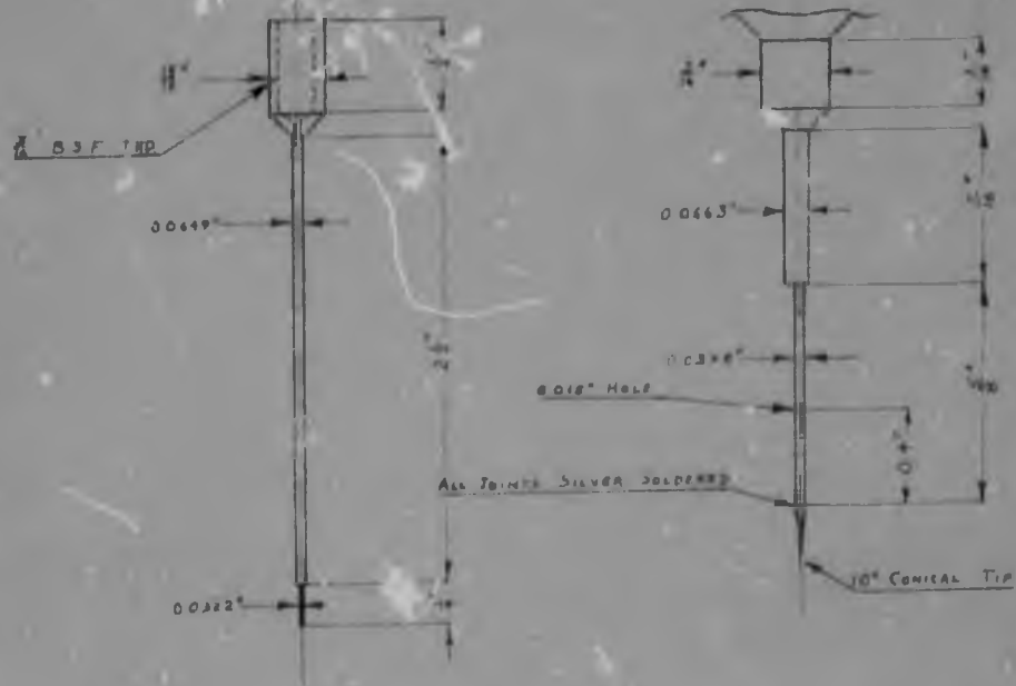
FIG. 34 STATIC PROBE
