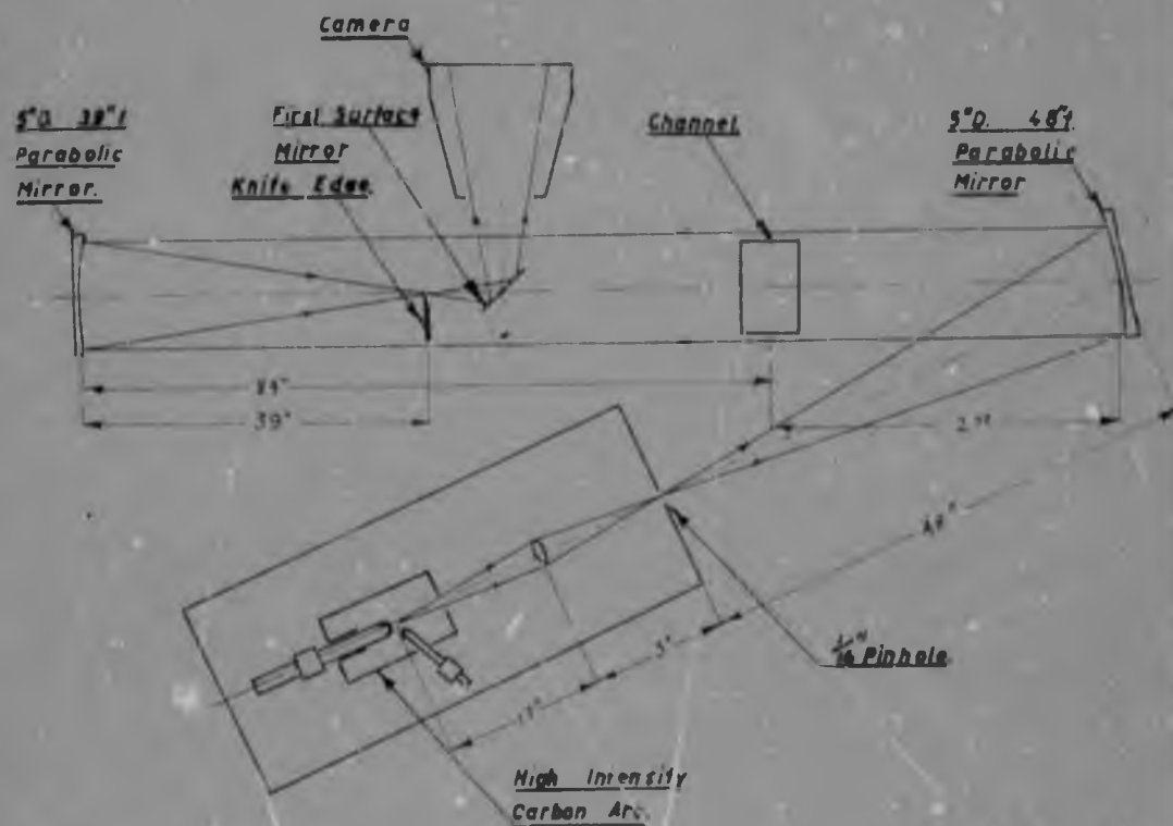
FIG. 32 OPTICAL LAYOUT OF THE SCHLIEREN SYSTEM
