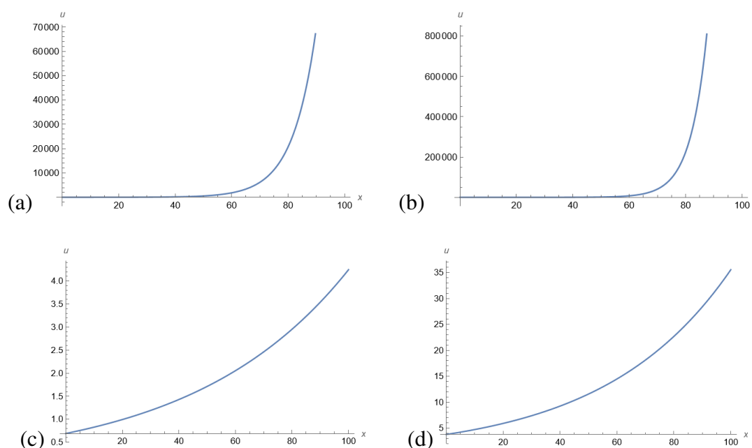
Figure 1. Graphical illustrations of the four analytical solutions ((a)–(d): (3.11), (3.14), (3.17) and (3.20)), showing the relationship between u(x, t) and the asset price x . The respective t value is t = 1.5 in (a)–(d).
