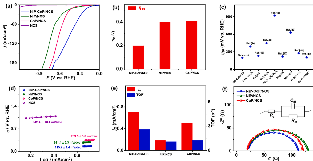
Fig. 4. (a) Comparative HER polarization curves of the electrocatalysts at 2 mV/s, (b) \eta_{10} , (c) Comparative \eta_{10} with literature, (d) Tafel plots, (e) j_0 and TOF, (f) Nyquist plots at -0.197 \text{ V} with Voigt electrical equivalent circuit (EEC, inset) of NiP-CoP/NCS, NiP/NCS, and CoP/NCS in 0.5 M \text{HClO}_4 solution.
