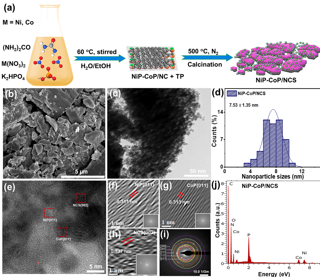
Fig. 1. (a) Synthesis method, (b) SEM, (c) TEM (d) Nanoparticles distribution, (e) HRTEM, (f–h) Fast Fourier transform (FFT) for NiP{011}, CoP{011}, and NCS{002} facets, (i) SAED, and (j) EDX of NiP-CoP/NCS.
