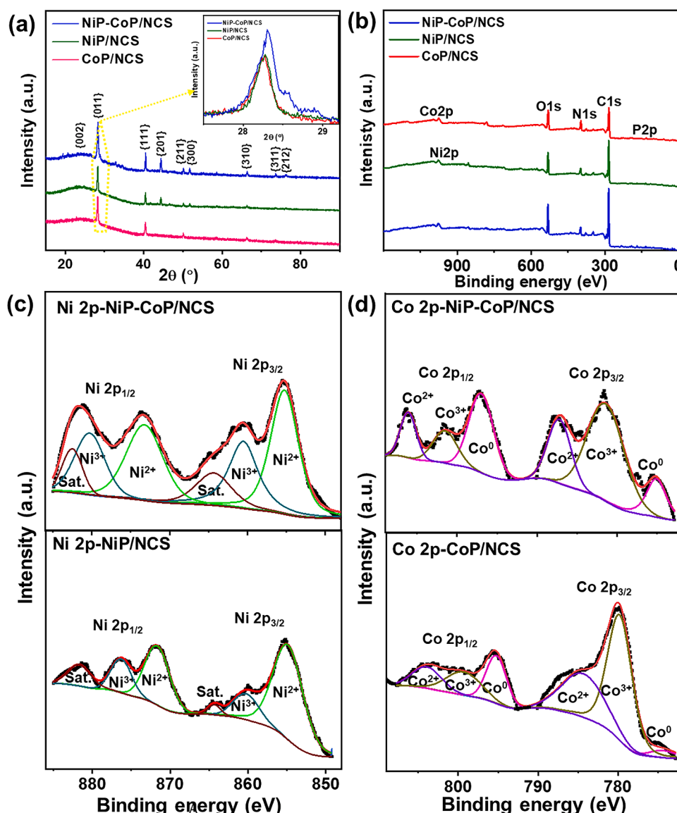
Fig. 2. (a) XRD, (b) XPS survey scan, high-resolution XPS of (c) Ni 2p and (d) Co 2p of NiP-CoP/NCS, NiP/NCS and CoP/NCS.
