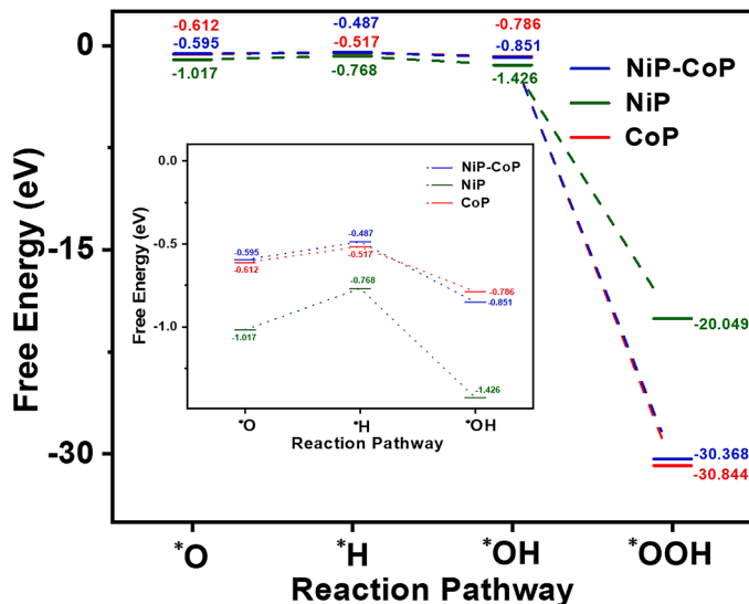
Fig. 6. Reaction coordinates of the adsorbates on the electrocatalysts (NiP-CoP {011}, NiP{011} and CoP{011}).
