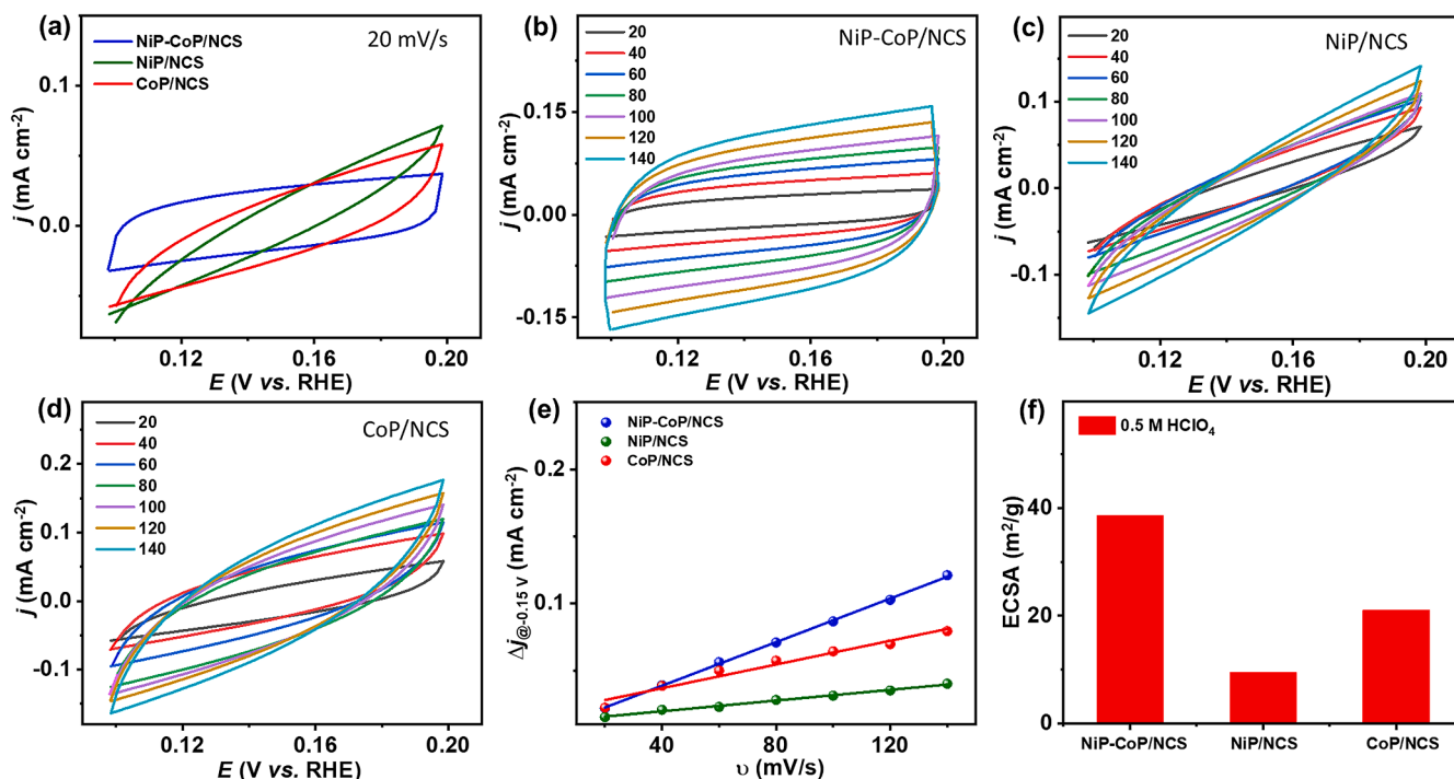
Fig. 3. (a) Comparative CV curves of the electrocatalysts at 20 mV/s, CV curves at varied scan rates ( v ) (b) NiP-CoP/NCS, (c) NiP/NCS, (d) CoP/NCS, (e) Plots of \Delta j_{@-0.15 \text{ V}} vs. v and (f) ECSA of NiP-CoP/NCS, NiP/NCS, and CoP/NCS in 0.5 M \text{HClO}_4 solution.
