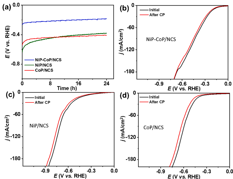
Fig. 5. (a) Chronopotentiometry (CP) plots at 10 \text{ mA/cm}^2 , HER polarization curves at 2 \text{ mV/s} before and after CP of (b) NiP-CoP/NCS, (c) NiP/NCS, and (d) CoP/NCS in 0.5 \text{ M HClO}_4 solution.
