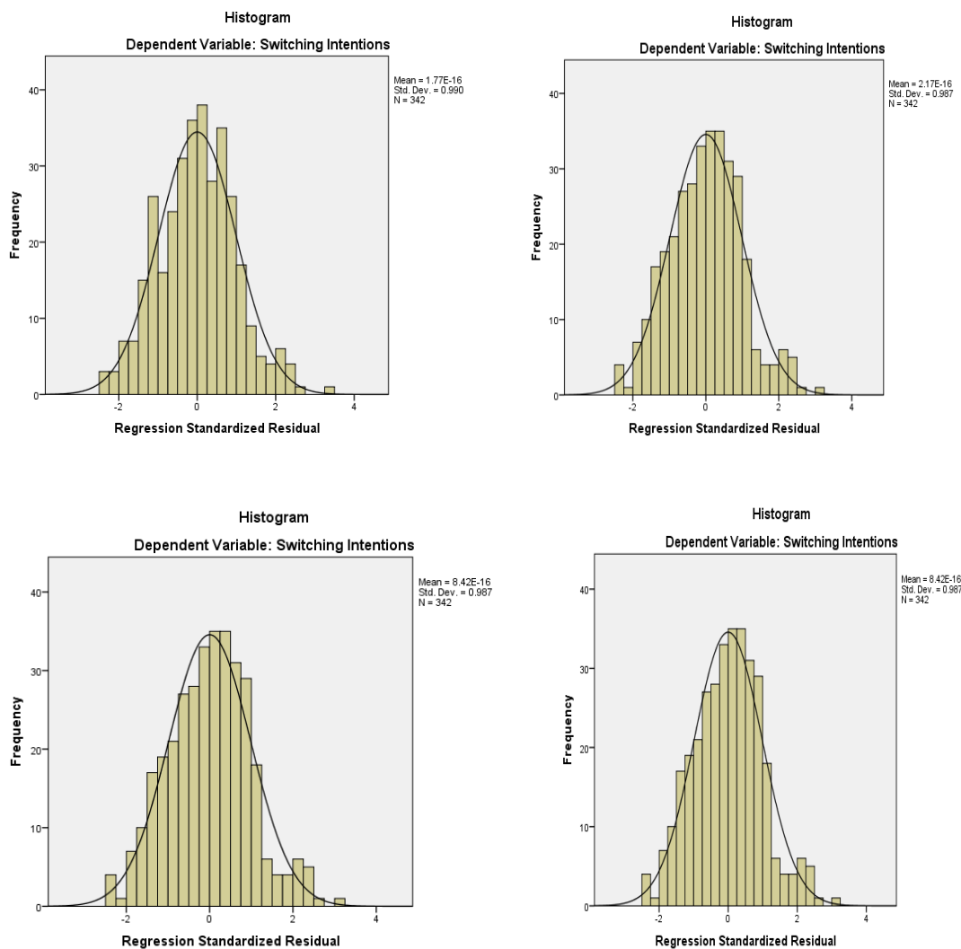
Figure 9: Model diagnostics
