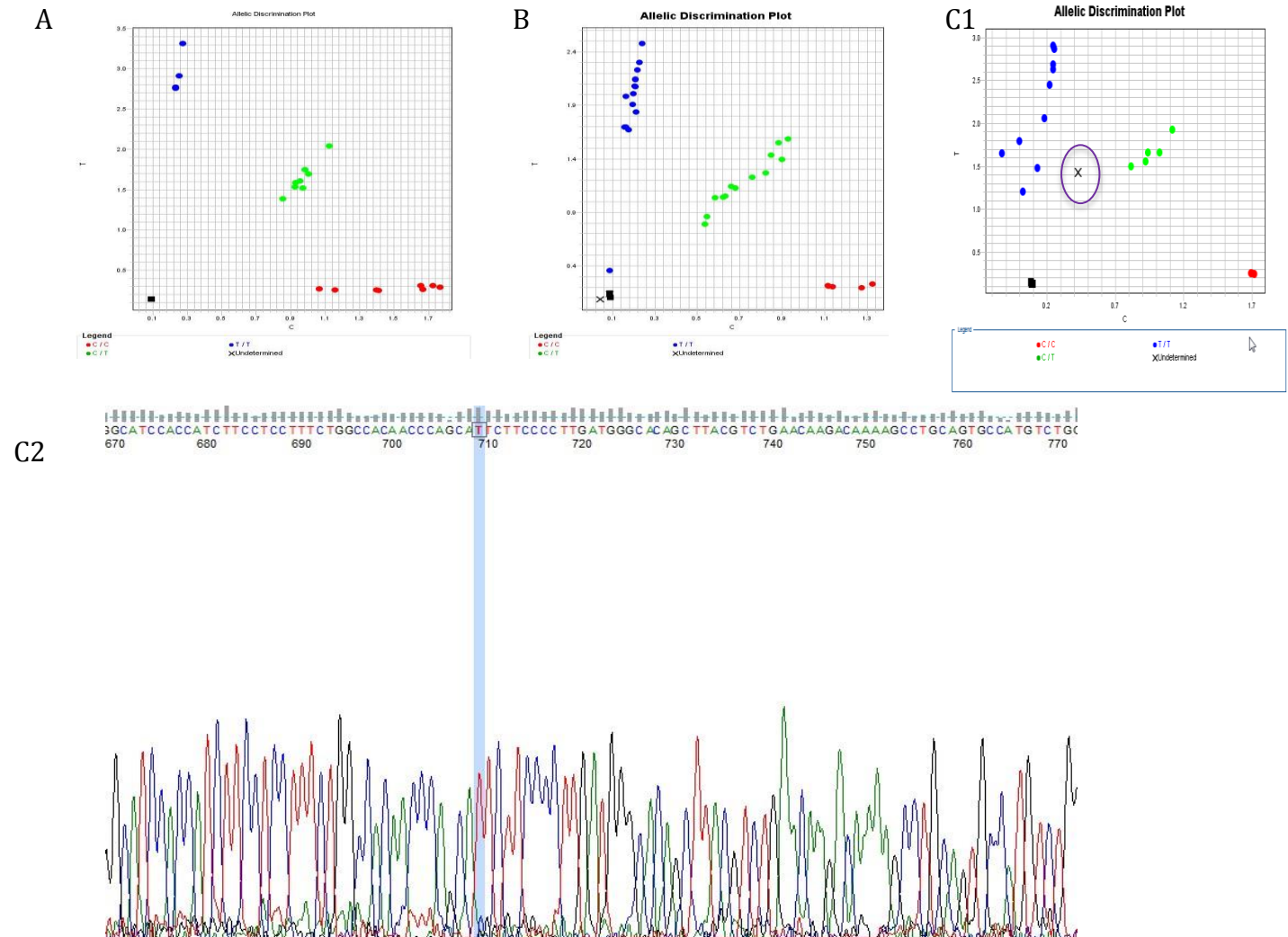
Figure 2. rs212739 assay validation. Allelic discrimination plot for the d4T cohort (A) and TDF cohort (B). Homozygous individuals with the wild-type allele (TT) are clustered in blue. Those possessing heterozygous form of the allele (CT) are cluster in green. The red cluster indicates the patients that are homozygous for the variant allele (CC). The squares represent experimental control (Negative control) and the individual marked X could not be analysed due to low or no amplification and were therefore repeated. The genotypic calls from the d4T cohort were in accordance with the genotypic calls for Ion reporter and Golden Helix. Allele discrimination plots (C1) and chromatogram (C2) images for RC77; the highlighted nucleotide shows the position where the variant rs212739 lied. The TaqMan assay signals (FAM/VIC) for R77 were undetermined (X) low but the assays were sensitive
