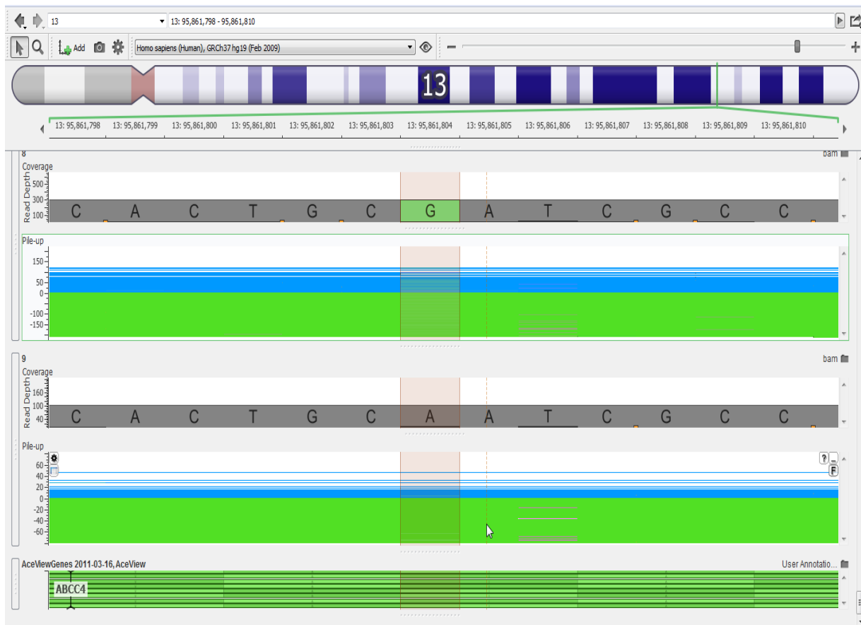
Figure 2.5. Next generation sequencing coverage for individuals 170253 (depicted as Bam file no. 8) and 170245 (Bam file no. 9) for SNP rs899494 located in gene ABCC4 , position chr13:95861804. Individuals 170253 and 170245 had a read depth of 288 and 96, respectively. Individual 170253 carried the variant and could potentially be at risk of TDF-AKI (phosphorous wasting). The blue pile up represents the forward strand and the green pile up represents the reverse strand.
