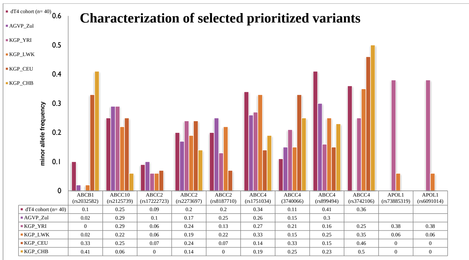
Figure 2.14. Characterisation of 11 prioritised variants. Nine variants have been associated with TDF associated acute kidney injury (TDF-AKI) (Table 2.11), and two additional variants in APOL1 strongly associated with HIV-associated nephrotoxicity (HIVAN) are included. The risk alleles of TDF-AKI occur more frequently in the African populations and the APOL1 variants are rare in the Caucasian (CEU) and Chinese (CHB) populations.
