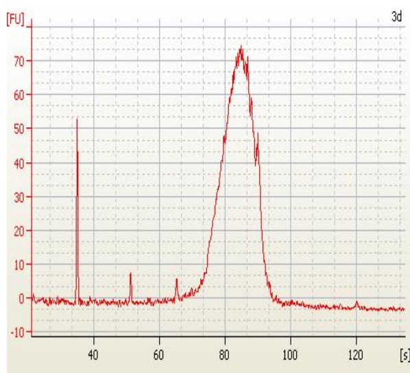
Figure1.2. gDNA structural analysis: Gel image (i) generated by the analysis of samples that were digested with EcoRI to assess the structural integrity of the genomic DNA. Four different samples (1-4) were evaluated at different phased (d=digested and u=undigested). Electropherograms of digested (ii) and undigested (iii) gDNA sample3 are shown.
