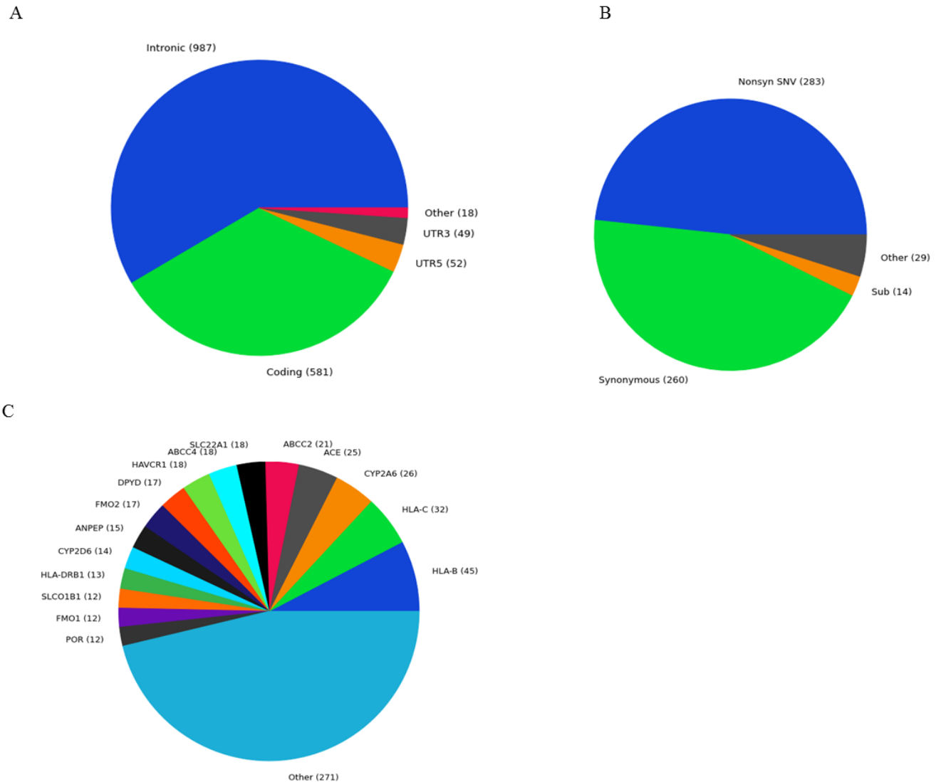
Figure 2.9. Variant classification for data generated via Ion Torrent S5™ sequencing. Pie chart (A) illustrates the classification based on the variant's position relative to the transcript of each variant (n= 1 687). (B) illustrates the nature of the 581 coding variants, this includes variants that lie within a splicing region of the coding transcript, and those within 1 000 bp of the transcript start/stop site (upstream or downstream variants). 'Non syn' SNV refers to non-synonymous SNPs causing an amino acid change; 'Synonymous' refers to a coding SNP that does not cause an amino acid change; 'Sub' refers to other substitutions that do not cause a frameshift change; additional variant classes are represented by 'other', which includes insertions, frameshift insertion, frame shift deletion, stop-loss, stop-gain, initiator codon and deletion. The 29 other variants were grouped together as their respective classification groups had less than 14 variants each. (C) shows the corresponding number of variants that lie in each respective gene.
