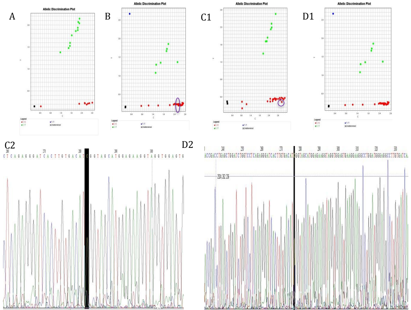
Figure 5. rs3740066 assay validation. Allelic discrimination plot for the d4T cohort (A). Individuals homozygous for the wild-type allele (CC) clustered in red. Those possessing heterozygous form of the allele (CT) cluster in green. The squares represent experimental control (Negative control). The genotypic calls were in accordance with 50 % of the Ion reporter and Golden Helix calls and this is due very low sequencing depth or coverage. The coverage is listed in the parenthesis and the samples with low coverage were incorrectly called. Allelic discrimination plot for the TDF cohort (B), where the plot displayed good clustering of the patients based on their genotype. Allele discrimination plots (C1) and chromatogram (C2) images for samples RC91 (1) and RC66 (2) from the TDF cohort. The highlighted nucleotide shows the position of the variant rs3740066 and Sanger sequencing confirmed the TaqMan genotypic calls.
