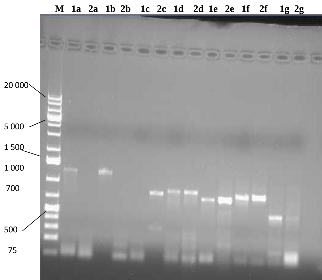
Figure 1. PCR amplicons of DNA fragments that encompass the SNPs of interest (a-g). Initially, PCR reactions were set up using Taq polymerase (1) and iProof™ polymerase (2). The corresponding fragment sizes are indicated in brackets with SNP b not being amplified. Therefore optimised using Iproof polymerase for a, c, d, e, f and Taq polymerase for g . About 10µL loaded on a 1% gel, with 10µL of 1Kb plus marker (ThermoFisher Scientific, Massachusetts, USA).
