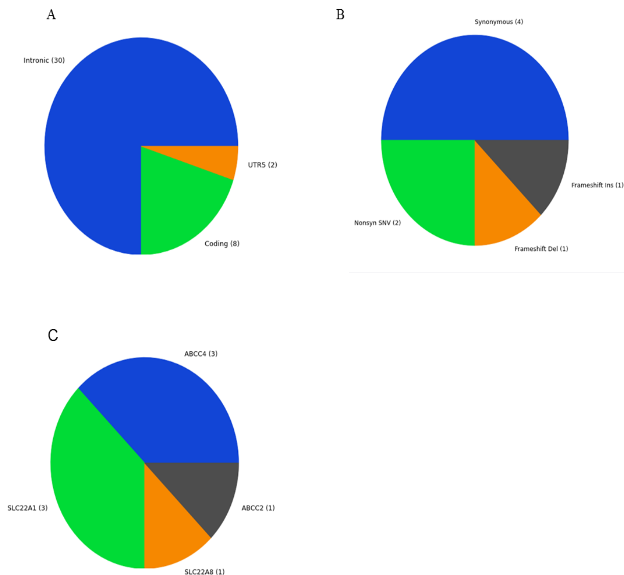
Figure 2.13. Novel variants classification. Pie chart (A) illustrates the classification based on the novel variant's position relative to the transcript of each variant (n= 40). (B) Illustrates the nature of the eight novel coding variants and (C) shows genes and the corresponding number of variants that lie in each respective gene.
