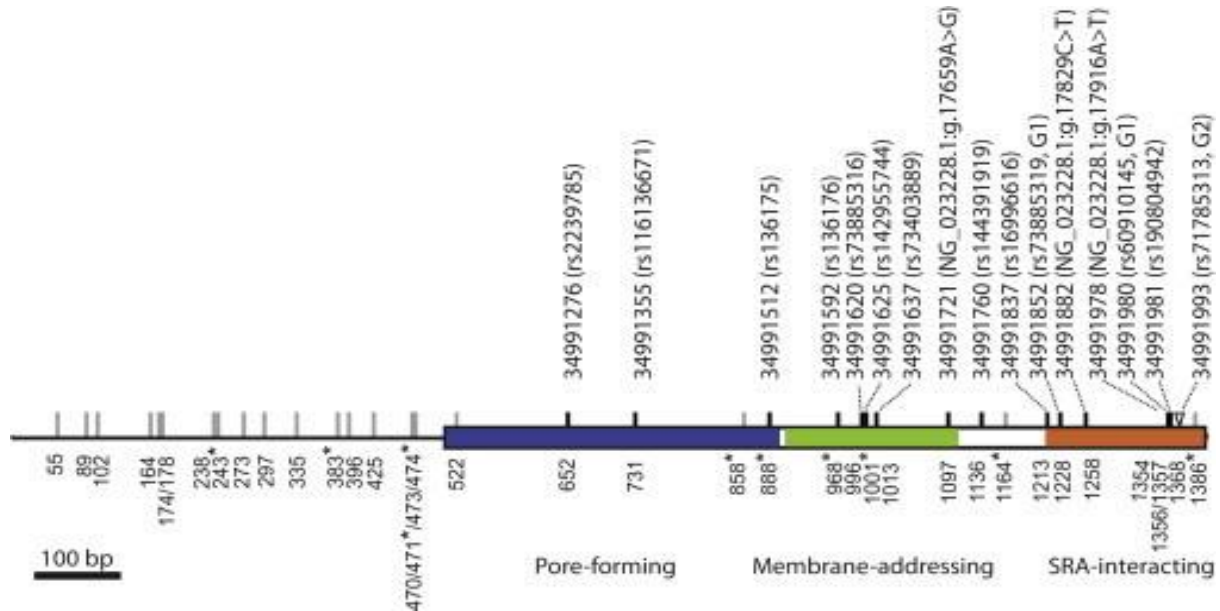
Figure 1.4: APOL1 variants implicated in HIV associated nephropathy (HIVAN). The APOL1 variants rs73885319 (a serine to glycine substitution at amino acid position 342 (p. S342G)), rs71785313 (in-frame deletions which result in asparagine and tyrosine deletions at amino acid positions 388 and 389 respectively (p. N388del: Y389del)) and rs60910145 (an isoleucine to a methionine substitution at position 384 (p. I384M)) are implicated in HIVAN. These alleles are referred to as G1 and G2 alleles where the G1 allele refers to rs73885319 and rs60910145 and the G2 allele refers to. rs71785313. G3 haplotype contains eight SNPs positions across the 1.4 kb region. They include two synonymous variants (positions 858 and 1 164), two non-synonymous variants (positions 888 (rs136175) and 968 (rs136176) located at the pore-forming domain and membrane-addressing domain, respectively) and four intronic variants (positions 243, 383, 471, and 474). Blue indicates the region of which codes for the pore-forming domains, green and orange codes for the membrane-addressing and SRA-interacting domains, respectively. The adjacent intron contains variants in the G3 allele. Copied form (Ko et al. 2013).
