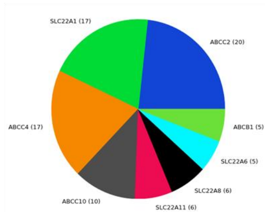
Figure 2.11. Gene panel and filtering of high quality variants identified by the IonS5™. Gene panel filtering was employed to identify variants localised in eight genes implicated in TDF induced AKI and efficacy, where 275 variants were identified and characterised. Pie chart (A) shows a variant classification according to gene position. Pie chart (B) illustrates the classification for each coding variant. ‘Non syn’ SNV refers to non-synonymous SNPs causing an amino acid change. Additional variant classes are represented by ‘other’, which includes frameshift insertion, frame shift deletion, deletion and splicing variants. The four other variants were grouped together as their respective classification groups had few variants each. (C) illustrates the number of variants in each gene.
