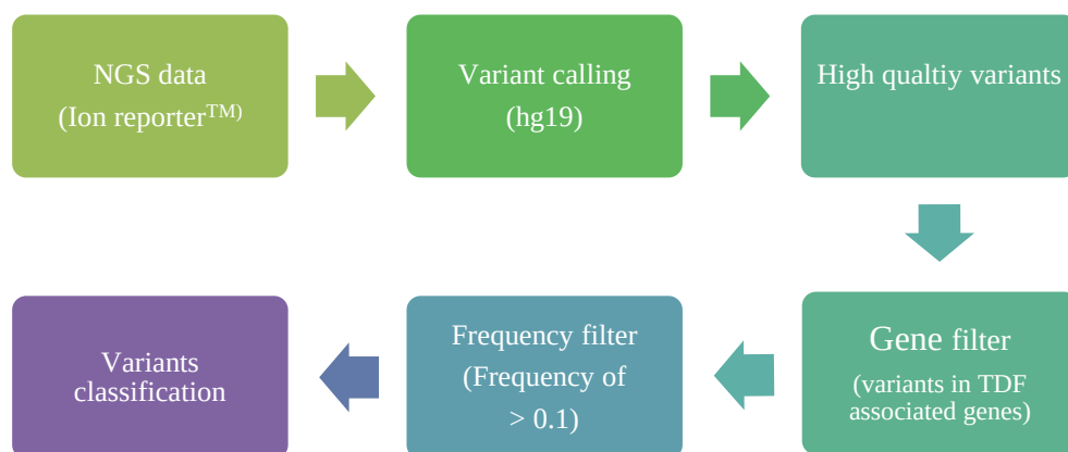
Figure 2.3. Summary of the NGS data filtering strategy that was employed for sequencing data analysis. Variants that lie in the eight selected genes of interest and that occur at a frequency of >0.1 in the cohort of the 40 sequenced individuals. Genes associated with TDF absorption ( ABCB1 ) and elimination ( ABCC2 , ABCC4 , ABCC10 , SLC22A6 and SLC22A8 ) were prioritized. Since TDF elimination is less understood, SLC22A1 and SLC22A11 transporters were also included because they belong to the same class of transporters localized in the kidney.
