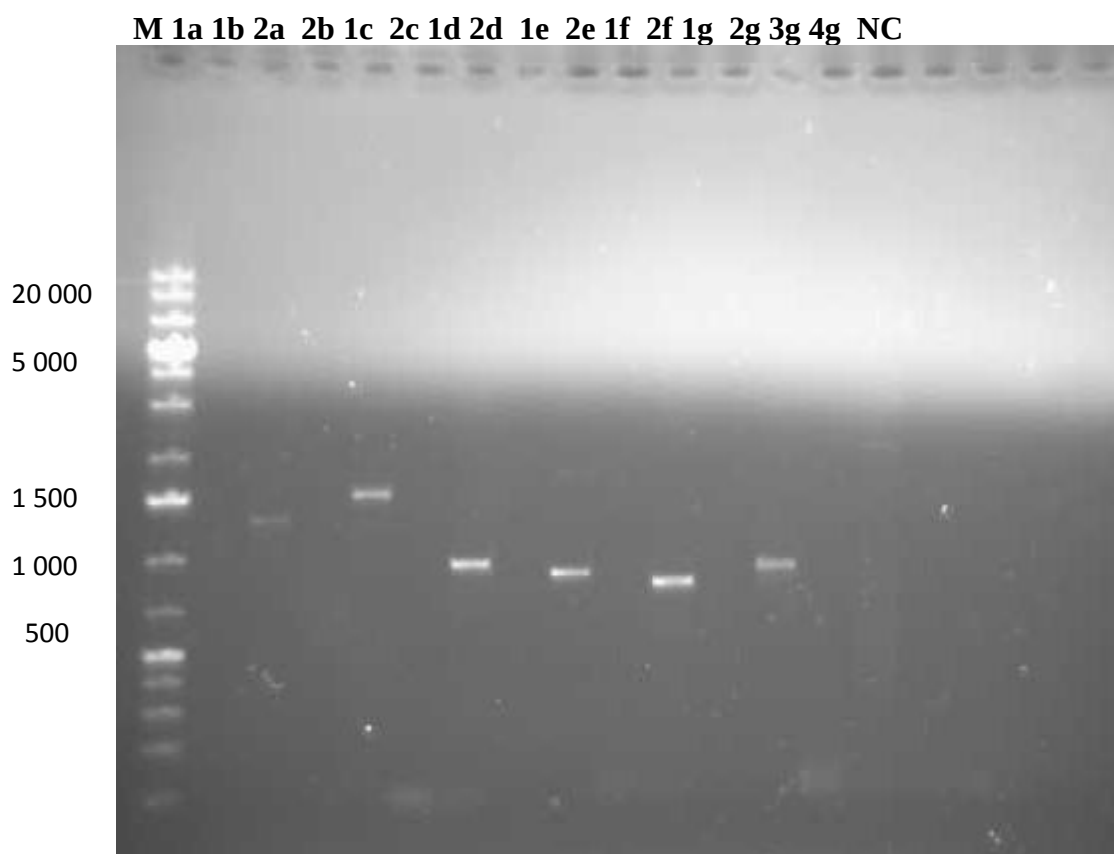
Figure 2: PCR amplicons of DNA fragments that encompass the SNPs of interest (a-g). Initially PCR reactions were set up using iProof TM polymerase (1), iProof TM polymerase with DMSO (2), Taq polymerase (3) and Taq polymerase with DMSO (4). The corresponding fragment sizes are indicated in brackets with the region for SNP g not amplified. The amount gDNA was doubled to 2ul (44ng). About 10ul loaded on a 1% gel, with 10ul of 1Kb plus marker (ThermoFisher Scientific, Massachusetts, USA).
