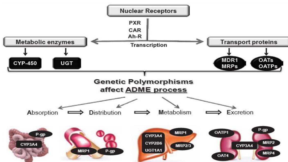
Figure 1.2. Genetic variations in pathways of drug absorption, disposition, metabolism and excretion (ADME) are main targets of HIV pharmacogenetic studies used to explain the inter-patient variability observed in patients treated with drugs such ARVs. Nuclear Receptors (NR) regulate metabolic enzymes and transport proteins and polymorphisms in these genes may influence patient tolerance or susceptibility to ARVs. Abbreviations: Ah-R: Aryl hydrocarbon receptor; PXR: pregnane X receptor; CAR: constitutive androstane receptor; CYP-450: cytochrome-450, UGT: uridine diphosphate glucuronosyl transferase; P-gp: P-glycoprotein; MRPs: multidrug resistance proteins, OATs: organic anion transporters; OATPs: Organic anion transporter polypeptides. Source: (Barco and Nóvoa 2013).
