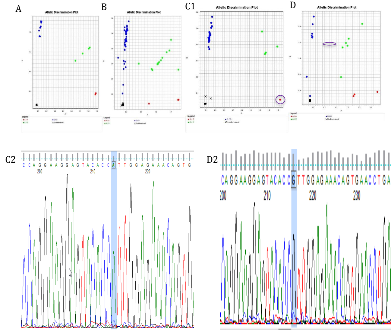
Figure 3. rs2273697 assay validation. Allelic discrimination plot for the d4T cohort (A) and TDF cohort (B). Individuals homozygous for the wild-type allele (GG) are clustered in blue. Those possessing heterozygous form of the allele (GA) cluster in green. Individuals homozygous for the mutated allele (AA) cluster in red. The squares represent experimental control (Negative control). X represents empty wells, as the genotype cannot be clearly distinguished. Genotyping calls from the d4T cohort where the calls were in accordance with the genotypic calls for Ion reporter and Golden Helix. Allele discrimination plots (C1 & D1) and chromatogram (C2 & D2) images for samples RC66 (1) and R26 (2) from the TDF cohort. The highlighted nucleotide shows the position of the variant rs2273697 . Sanger sequencing confirmed the TaqMan genotypic calls.
