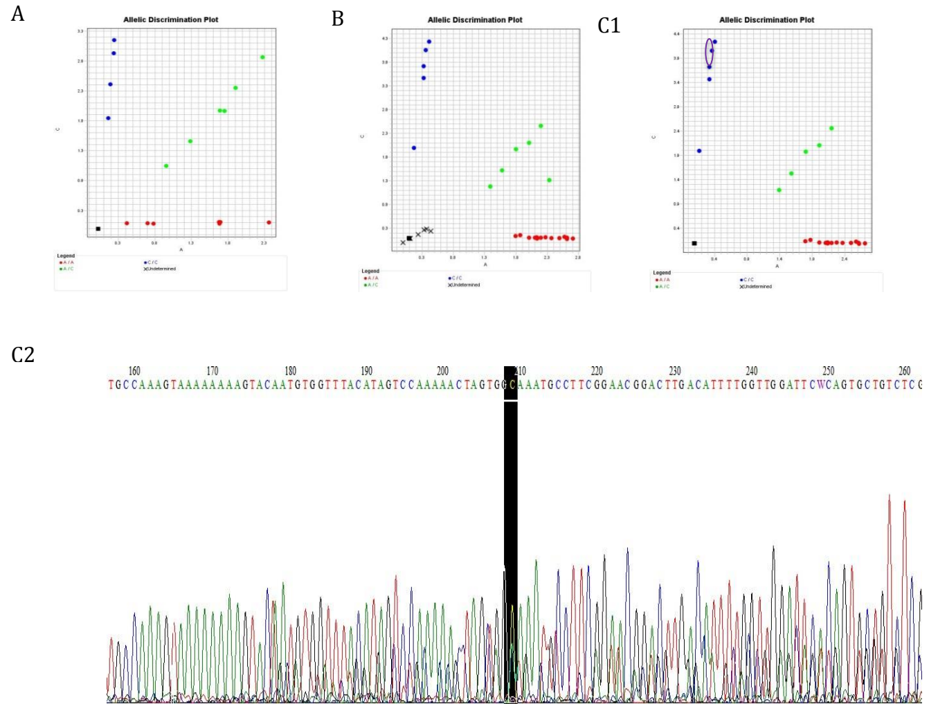
Figure 6. rs3742106 assay validation. Allelic discrimination plot for the d4T cohort (A) and TDF cohort (B) Homozygous individuals with the wild-type allele (AA) are clustered in red. Those possessing heterozygous form of the allele (AC) cluster in green. The blue cluster indicates the patients that are homozygous for the variant allele (CC). The squares represent experimental control (Negative control) and the individuals marked X could not be analysed due to low or no amplification and were therefore repeated. The calls were in accordance with 90% the genotypic calls for Ion importer and Golden Helix. Sample 357 was incorrectly called AA and 3 samples were omitted replicates with no amplification to produce good clustering. Allele discrimination plots (C1) and chromatogram (C2) images for patient samples RC46; the highlighted nucleotide shows the position where the variant rs3742106 was identified by Sanger sequencing, which confirmed the TaqMan genotypic calls for RC46.
