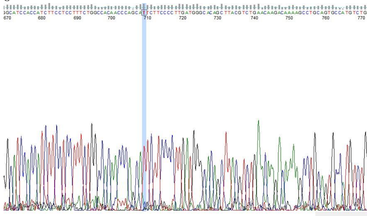
Figure 2. TaqMan SNP genotyping assay C__16173668_10.
