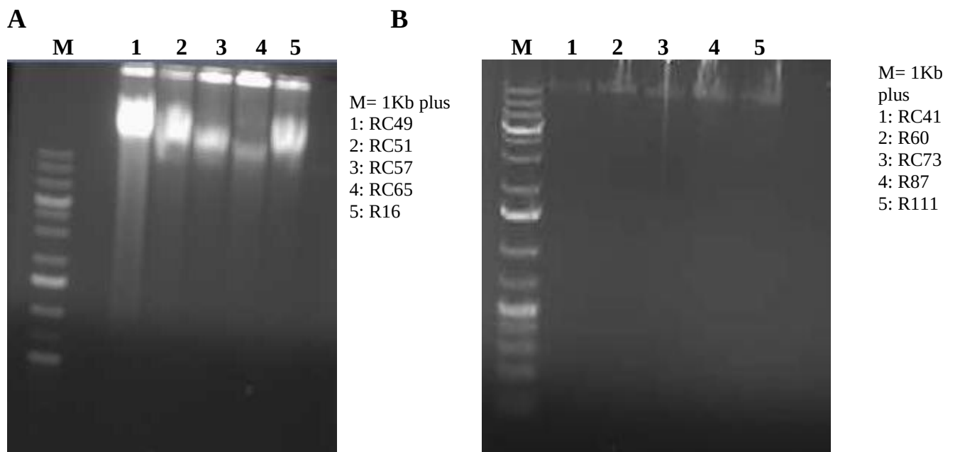
Figure 1.1 (A-B). Agarose gel analysis of TDF samples extracted. High molecular weight gDNA produced by salting out extraction from buffy coat samples from the TDF cohort. The high molecular weight single band indicates the absence of degraded fragments, showing the structural integrity of the gDNA extracted. 10µL of extracted gDNA was loading in gel A and 1 µL of gDNA was loaded in gel B.
