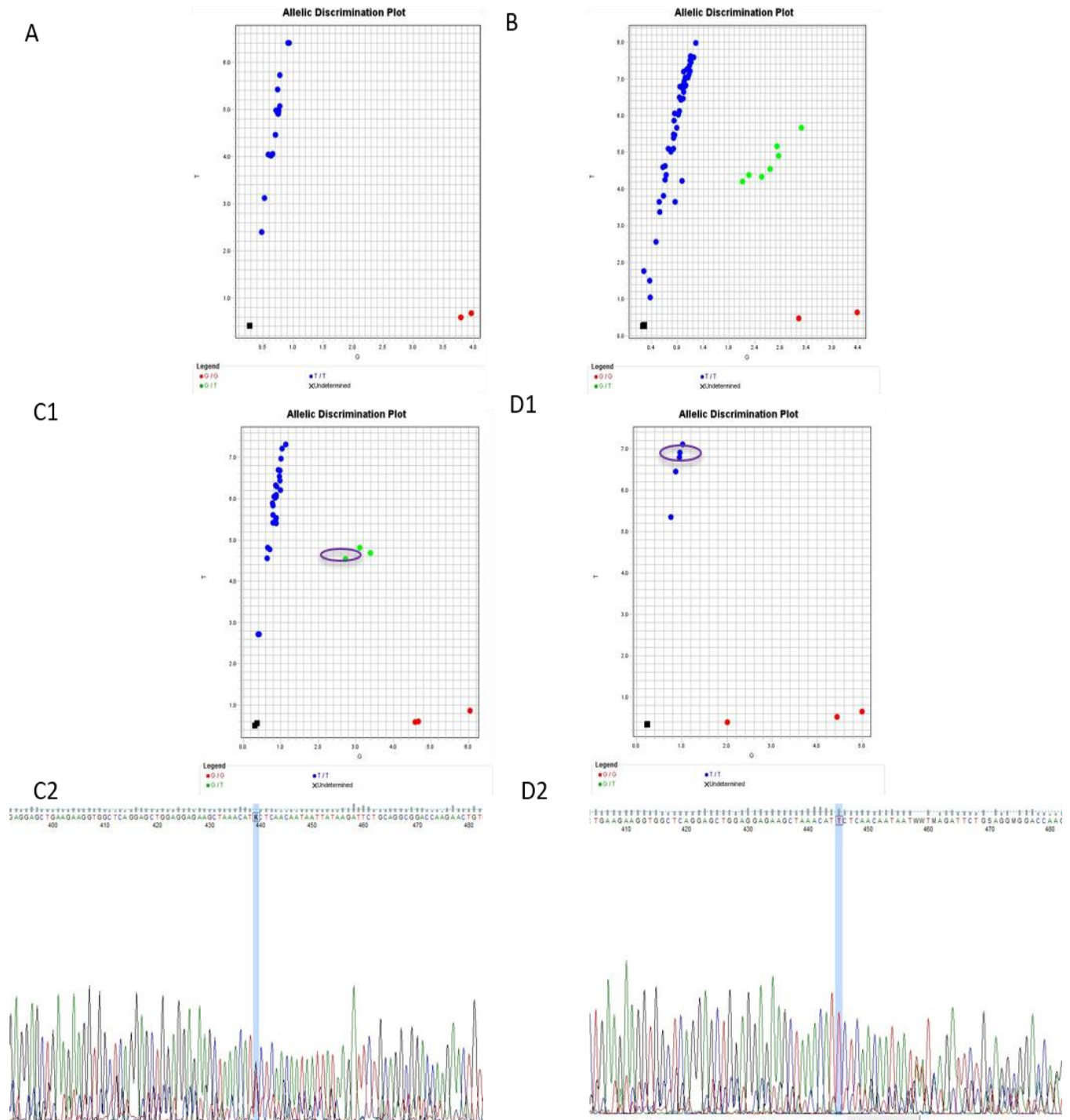
Figure 9. rs60910145 assay validation. Allelic discrimination plot for the d4T cohort (A) and TDF cohort (B) Genotyping calls from the d4T cohort. Individuals both forms of the wild-type allele (AA) are clustered in red. Those possessing homozygous variant allele (GG) are cluster in green. The squares represent experimental control (Negative control) Allele discrimination plots (C1 & D1) and chromatogram (C2 & D2) images for patient samples RC46 (1) and R26 (2); the highlighted nucleotide shows the position where the variant rs60910145 was identified by Sanger sequencing confirmed the TaqMan genotypic calls for RC46 and R26.
