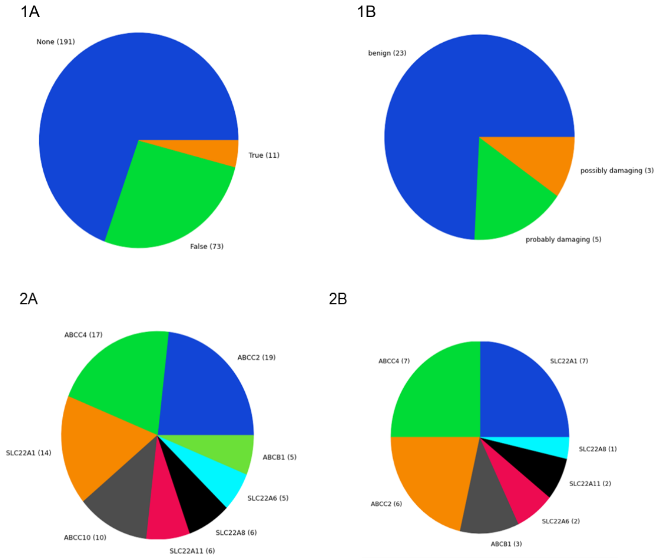
Figure 2.12. SVS version 8.4.4 functional effect analysis of 275 variants identified after gene panel filtering. SIFT ( A ) and PolyPhen ( B ) analysis of the total number of variants that were identified in genes relevant to TDF nephropathy. Pie charts ( 1A and 1B ) illustrates the number of variants classified as true indicates that the variants have a damaging threshold of \leq 0.5 , making them probably damaging and may exert a significant functional change. The corresponding genes in which the variants lie are indicated in the pie charts ( 2A and 2B ).
