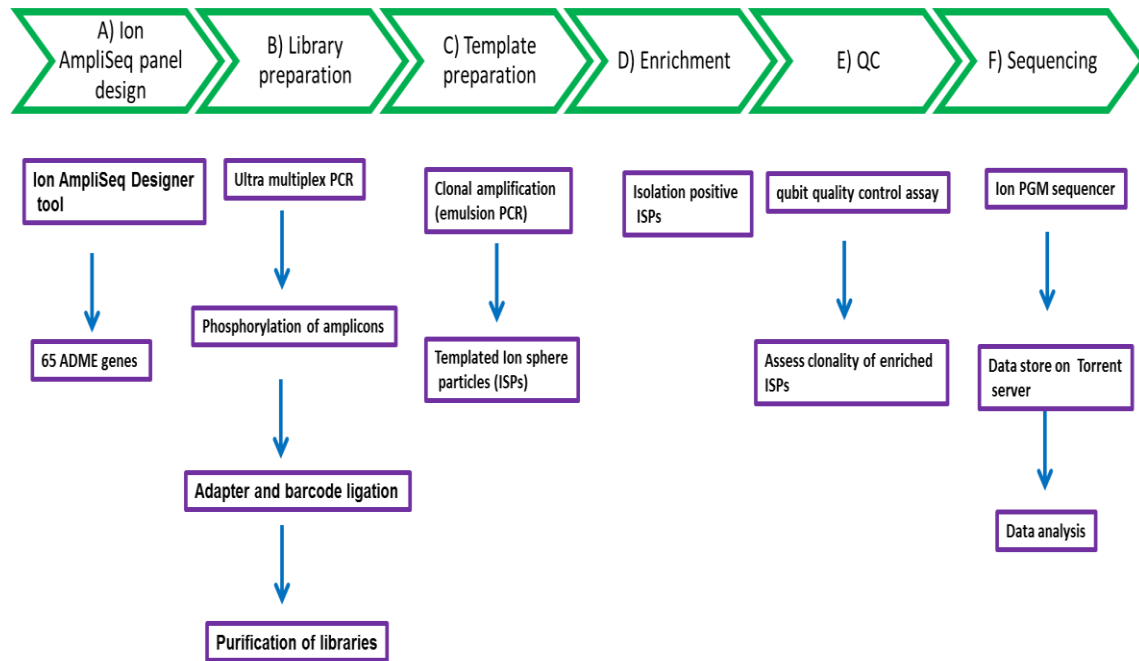
Figure 2.1. Summary of the Next Generation Sequencing (NGS) workflow that was implemented in this study. The sequencing workflow consists of the following steps: A) AmpliSeq™ panel design B) library preparation, C) template preparation, D) enrichment of positive ISPs E) quality control F) sequencing and data processing and variants filtering.
