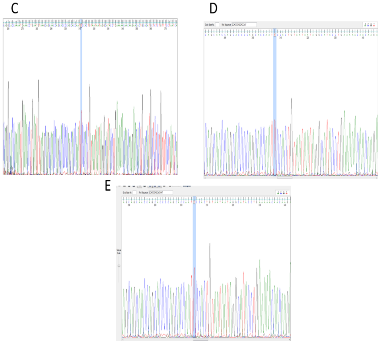
Figure 1.1. Sanger sequencing results (A-E).
