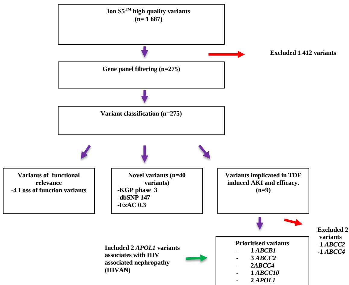
Figure 2.10: Summary of the filtering strategy that was employed for prioritising variants identified in the IonS5 TM data. The criteria for prioritizing the variants included selecting variants that lie in eight genes implicated in TDF induced AKI. These genes are associated with TDF absorption ( ABCB1 ) and elimination ( ABCC2 , ABCC4 , ABCC10 , SLC22A6 and SLC22A8 ). Since TDF elimination is less understood, SLC22A1 and SLC22A11 transporters were also included because they belong to the same class of transporters localized in the kidney. The variants were further prioritized based on functional impact, novelty and association with TDF induced AKI, efficacy and nephropathy.
