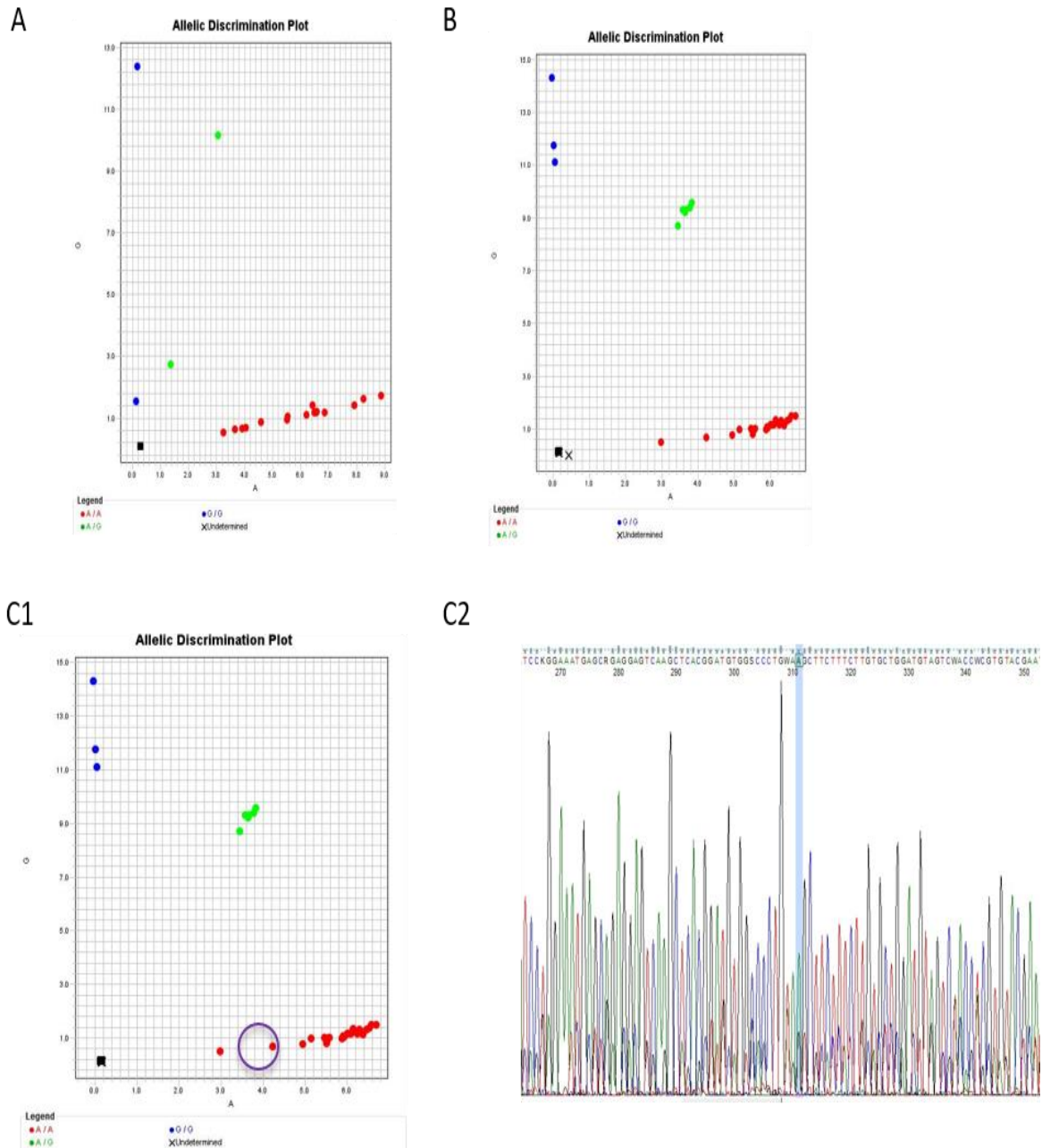
Figure 8. rs73885319 assay validation. Allelic discrimination plot for the d4T cohort (A) and TDF cohort (B). Individuals homozygous for the wild-type allele (AA) are clustered in red. Those possessing heterozygous form of the allele (AG) are clustered in green. Individuals with both forms of the mutated allele (GG) are clustered in blue. The squares represent experimental control (Negative control). Allele discrimination plots (C1) and chromatogram (C2) image for patient samples RC46; the highlighted nucleotide shows the position where the variant rs3742106 was identified by Sanger sequencing, confirming the TaqMan genotypic calls for RC46.
