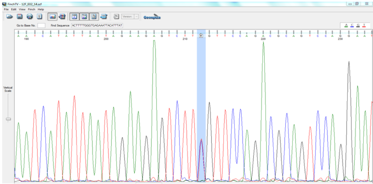
Figure 1.3. Sanger sequencing results (A).
