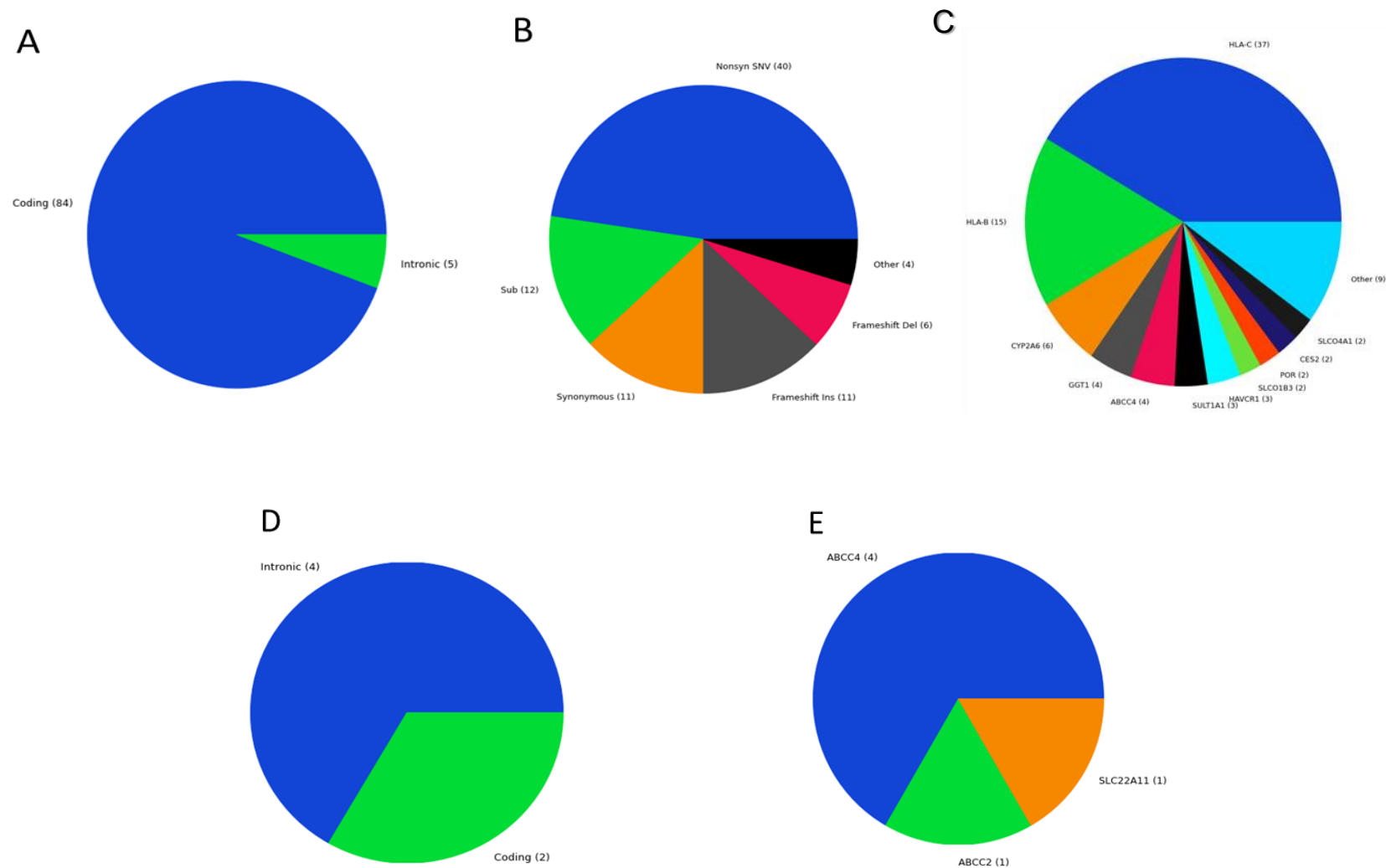
Figure 2.8. Variant classification for data generated using Ion Torrent PGM™ sequencing. Pie chart (A) illustrates the classification based on the variant's position relative to the transcript of each variant (n=89). (B) illustrates the nature of the 84 coding variants, this includes variants that lie within a splicing region of the coding transcript, and those within 1 000 bp of the transcript start/stop site (upstream or downstream variants). 'Non syn' SNV refers to non-synonymous SNPs causing an amino acid change; 'Synonymous' refers to a coding SNP that does not cause an amino acid change; 'Sub' refers to other substitutions that do not cause a frameshift change. 'other' represents additional variant classes which include insertions, frameshift substitution, deletion-substitution and deletion. The 4 other variants were grouped together as their respective classification groups had less than 6 variants. (C) shows the corresponding number of variants that lie in each respective gene (n=64). (D) illustrates the classification class of 6 variants that lie in genes relevant to TDF nephropathy and (E) shows the number of variants that lie in genes relevant to TDF nephropathy. Please note that these data were not used for downstream analysis as several variants could not be validated with Sanger sequencing.
