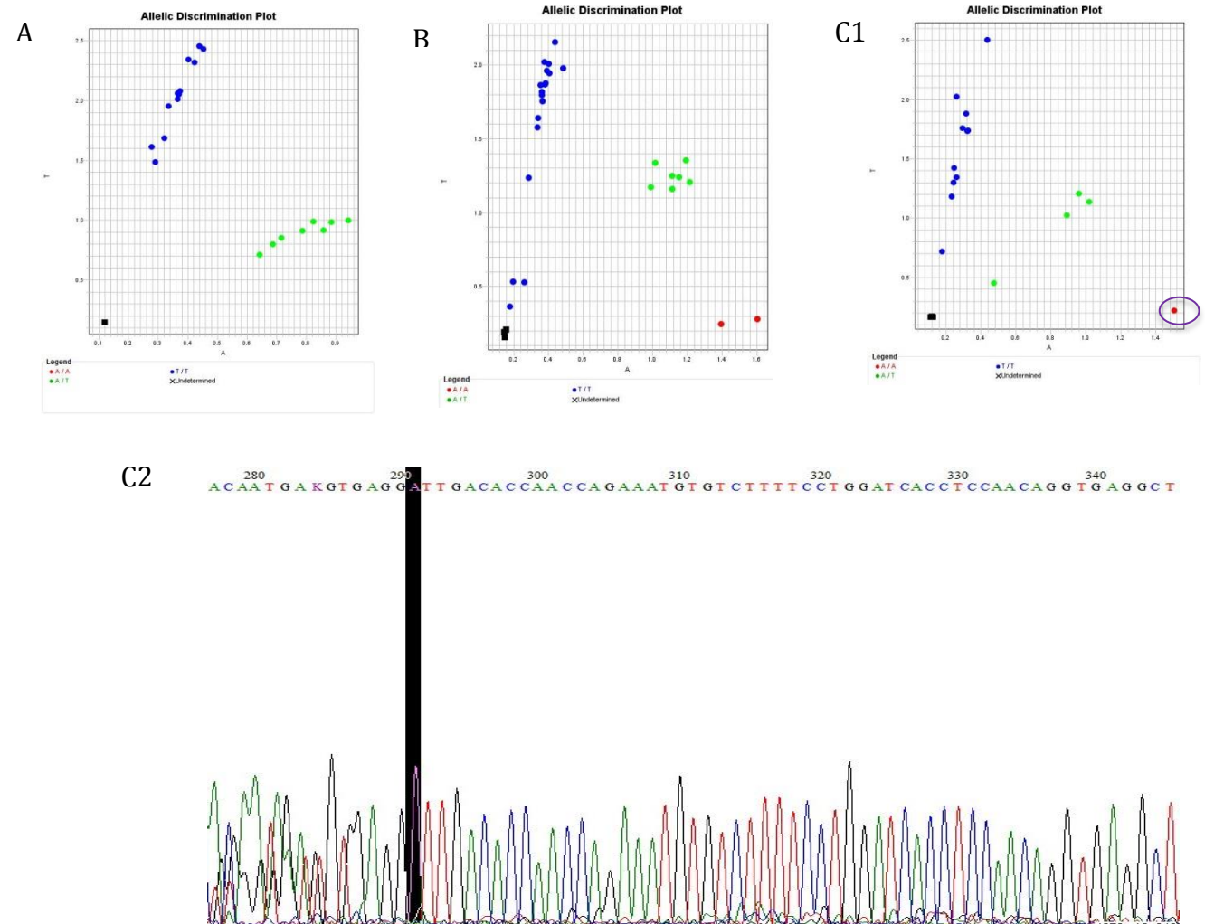
Figure 4. rs17222723 assay validation. Allelic discrimination plot for the d4T cohort (A). Genotyping calls from the d4T cohort where the calls were in accordance with the genotypic calls for Ion importer and Golden Helix. Individuals homozygous for the wild-type allele (TT) clustered in blue. Those possessing heterozygous forms of the allele (AT) cluster in green. The squares represent experimental control (Negative control). Allelic discrimination plot for the TDF cohort (B), where an increase in sample size resulted in the variants genotype being identified and the plot displayed good clustering of the patients based on their genotype. Allele discrimination plots (C1) and chromatogram (C2) images for samples R26 (1) from the TDF cohort. The highlighted nucleotide shows the position of the variant rs17222723 and Sanger sequencing confirmed the TaqMan genotypic calls.
