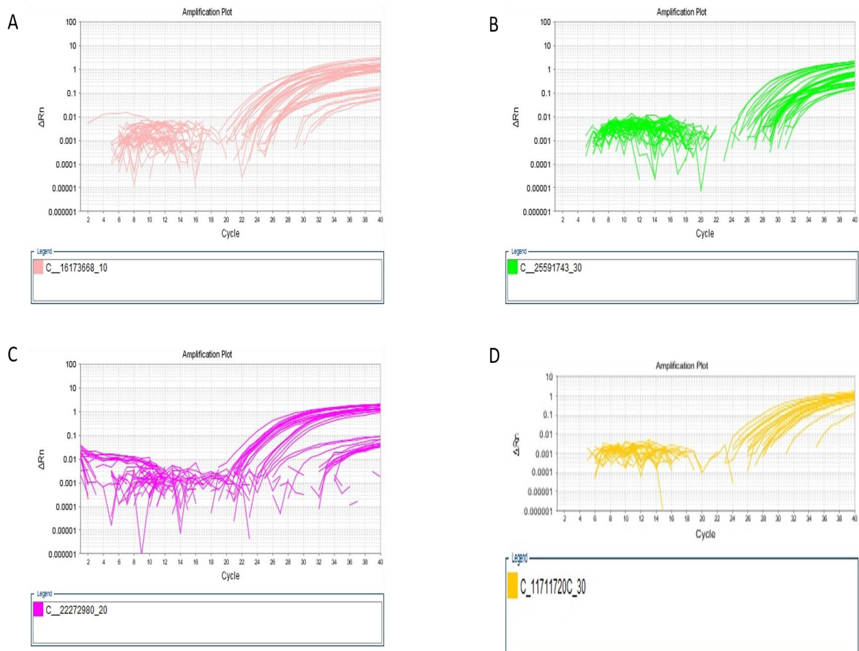
Figure A-D. Amplification plots for four assays tested. A was obtained with 10 ng of gDNA; and B-D was obtained with 20ng of gDNA. Increasing the starting gDNA did not significantly lower the Ct (cycle no. at which amplification begins) therefore increasing the starting gDNA did not increase amplification and fluorescent signals that results in more defined clusters of the genotypes
