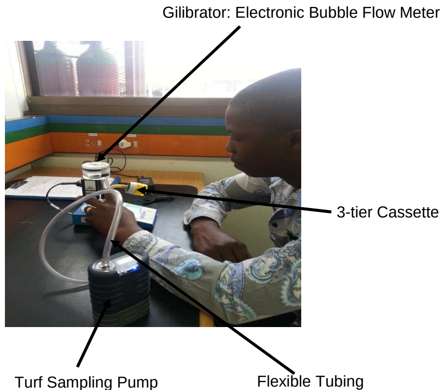
Figure 2: Calibration of the sampling trains
