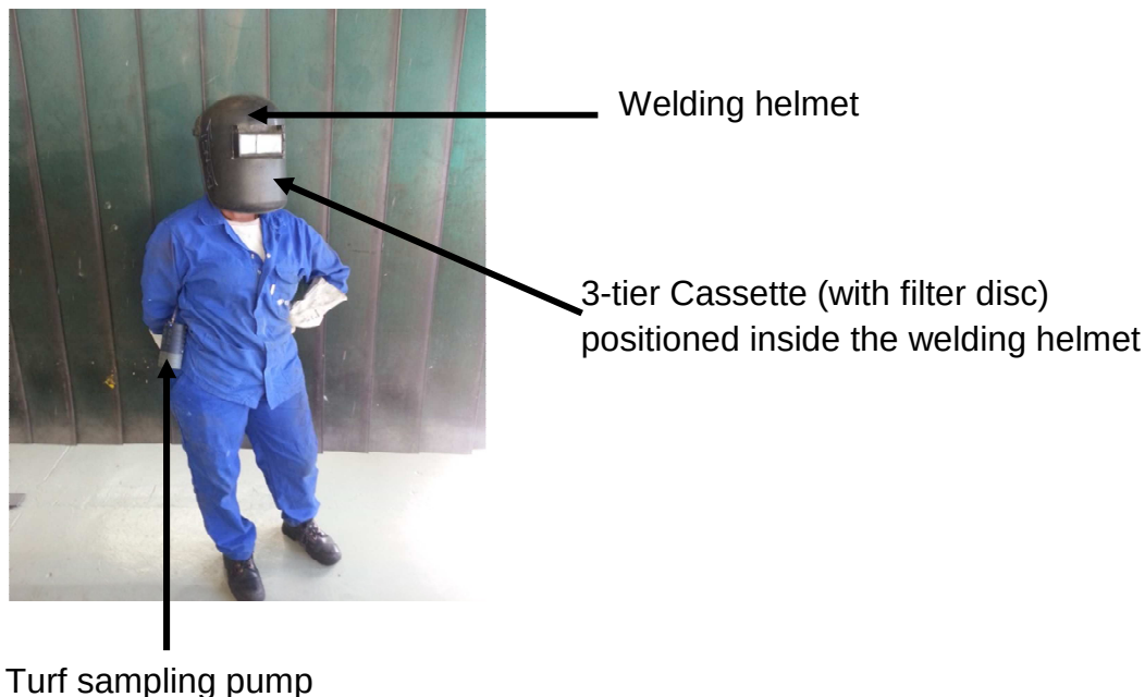
Figure 3: Sampling train positioning within the breathing zone
