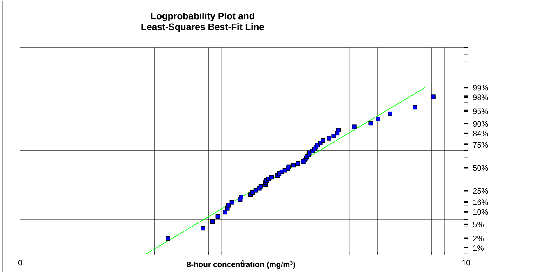
Figure 6: Logprobability plot and least-squares best fit line of personal occupational exposure to total welding fume concentrations in mg/m 3
