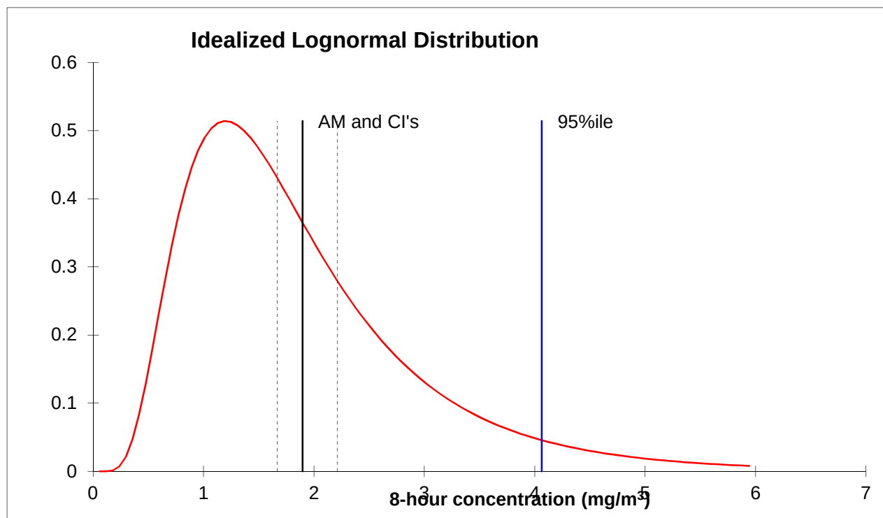
Figure 7: Idealized lognormal distribution curve of personal occupational exposure to total welding fume concentrations in mg/m 3
